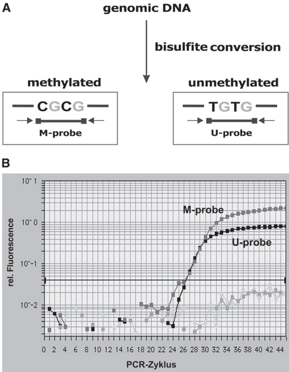
Fig. 2. (A) Principle of real-time MSP. A primer pair containing no potential methylation site in its sequences amplifies a short stretch of DNA containing the CpG sites for which the methylation status is to be determined. The very short length of the amplicon ensures identical amplification efficiencies for methylated and unmethylated alleles. (B) Amplification plots for a 1:1 mixture of methylated and unmethylated DNA, demonstrating equal reaction efficiencies.
