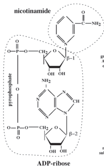
Fig. 1. Schematic diagrams of PARP-1 (A), NAD (B), and poly(ADP-ribose) polymer formation (C). (A) PARP-1 enzyme primary structure and functional domains. The three-domain structure of PARP-1 (DNA binding, auto-modification, and catalytic) first proposed (36) has been both confirmed and refined by gene and cDNA nucleotide sequence determination (37). (B) NAD structure. Dashed lines encircle the nicotinamide and ADP-ribose moieties, which are joined at the \beta C-1'' position of the ribose moiety (indicated as \beta -1). The linkage marked \beta -2 is not affected during ADP-ribose polymerization. (C) Subunit addition. The ADP-ribose polymer is stably attached to a glutamate (Glu) residue of the modified protein via a \beta -1 linkage. The addition of a new subunit is shown at the bottom of the chain, where a ribose-ribose is formed between the incoming ADP ribose and the 2' ribose at the terminus of the growing chain (38,39). Specifically, the \alpha -linkage occurs by an inversion process at the anomeric 1'' -carbon atom of the ribose of substrate NAD. Thus, the configuration at the detectable stable 1'' -carbon in the resultant 2' \rightarrow 1'' linkage is \alpha , as determined by NMR (40–42). This diagram is intended for schematic purposes only and does not attempt to portray accurately either molecular conformations or mechanisms.
