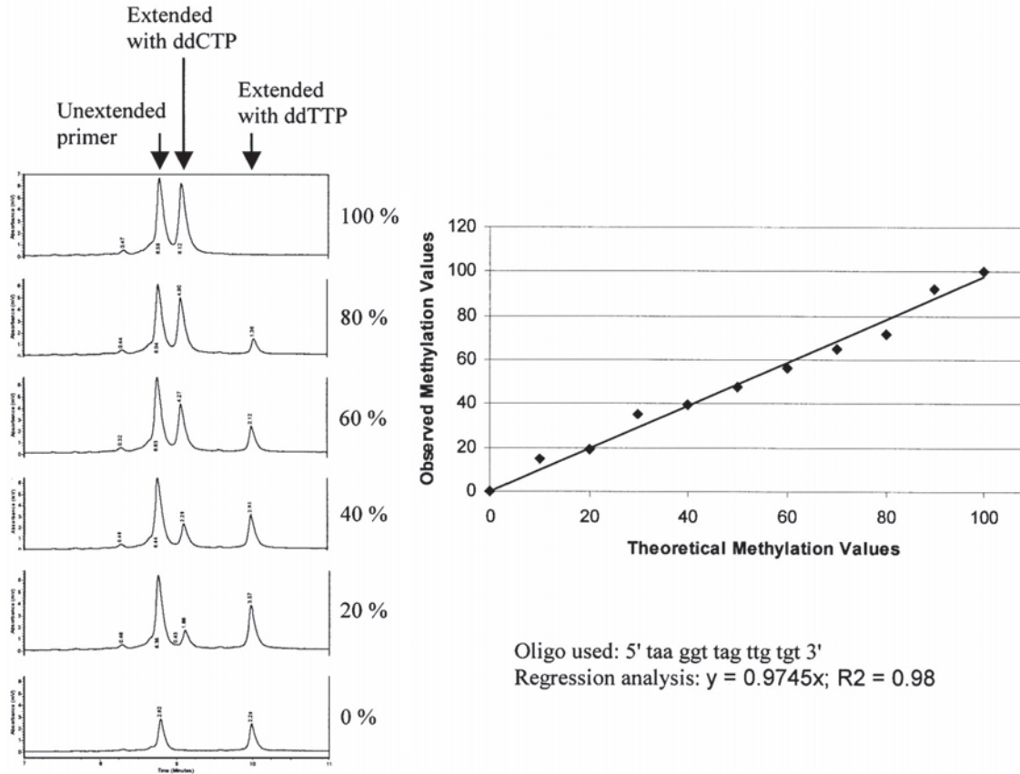
Fig. 2. Linearity of the reaction. A PCR product and a primer in the SNRPN gene was used with a serial mixes of methylated and unmethylated alleles in 10% increments.
