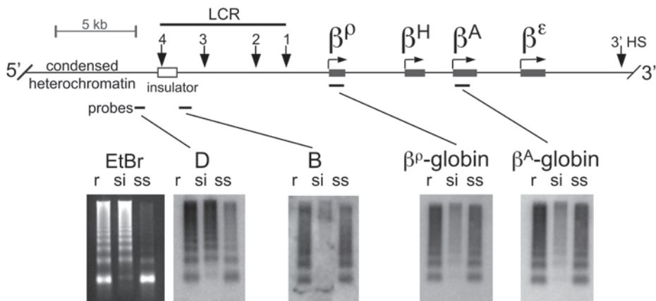
Fig. 1. Southern blot of DNA extracted following MNase digestion of 15-d chicken erythrocyte nuclei from (r) released, (si) salt-insoluble, and (ss) salt-soluble chicken chromatin. Blots were probed with sequences from inside and outside the \beta -globin domain; positions of the probes are indicated by the solid bars. LCR, locus control region.
