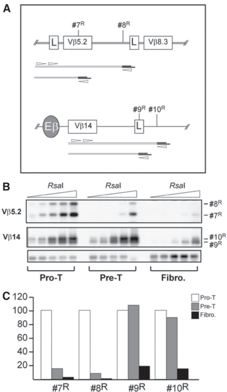
Fig. 1. (continued) CD3 \epsilon locus (data not shown). Similar percentages were obtained in separate restriction enzyme cleavage/LM-PCR experiments. The results demonstrate that, upon pro-T- to pre-T-cell development, the V \beta 5 chromosomal region becomes resistant to enzyme cleavage (and presumably acquires an altered, repressed chromatin structure), whereas the V \beta 14 region remains in an open, nuclease-sensitive state.
