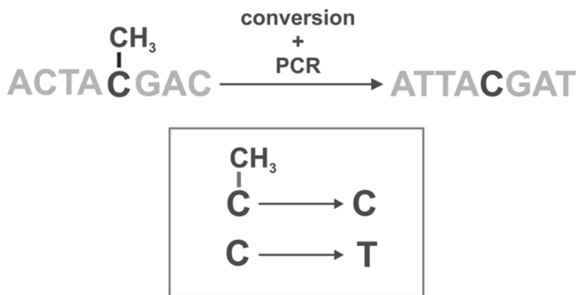
Fig. 1. Principal of bisulfite treatment of DNA. The epigenetic modification is converted into a difference in the primary sequence.
