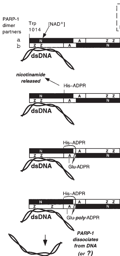
Fig. 3. Schematic of PARP-1 enzymatic activity. The key to the domain structure of PARP-1 is shown in Fig. 1A . The suggested antiparallel arrangement of PARP-1 dimer subunits permits the catalytic and the DNA binding domains to be in close association. Details regarding this schematic are given in reactions 1 and 2, Subheading 3.3. and the accompanying text.
