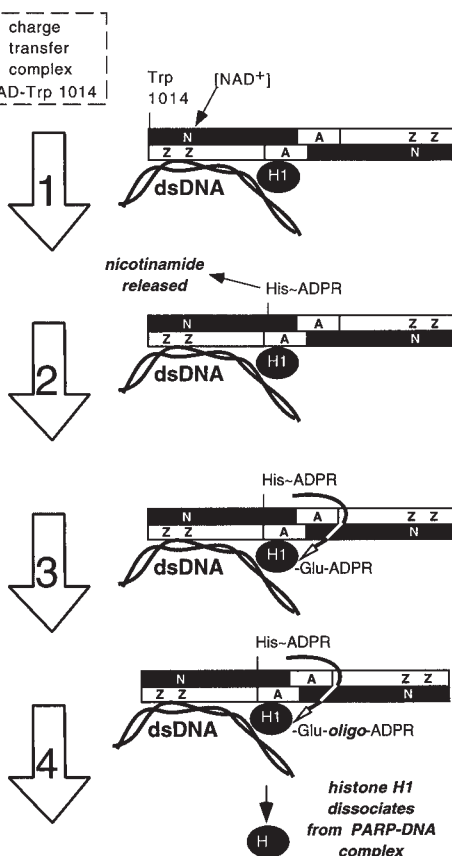
Fig. 3. Schematic of PARP-1 enzymatic activity. The key to the domain structure of PARP-1 is shown in Fig. 1A . The suggested antiparallel arrangement of PARP-1 dimer subunits permits the catalytic and the DNA binding domains to be in close association. Details regarding this schematic are given in reactions 1 and 2, Subheading 3.3. and the accompanying text.
