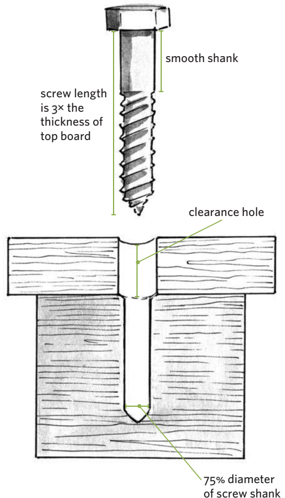
Predrilled hole for a lag screw
