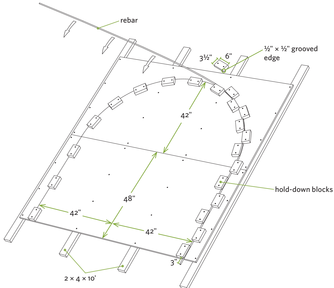
Bending jig
