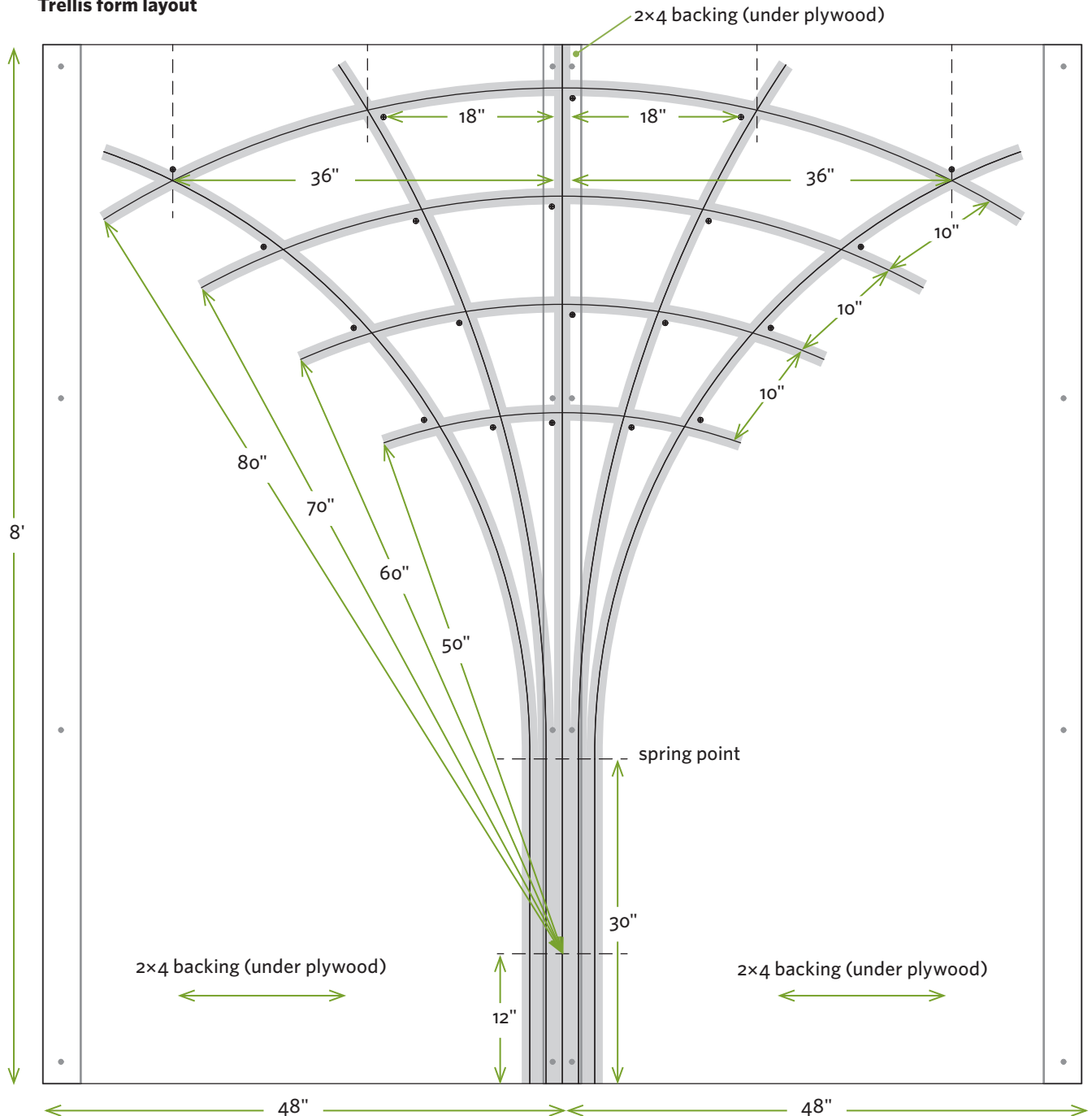
Trellis form layout
