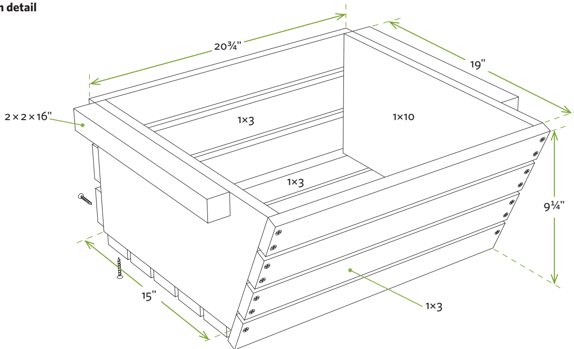
Bin detail
