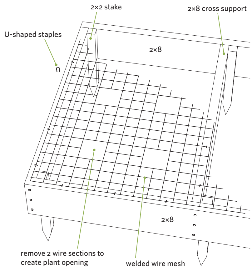
Horizontal gridwork
