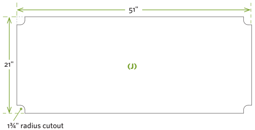
Platform details
