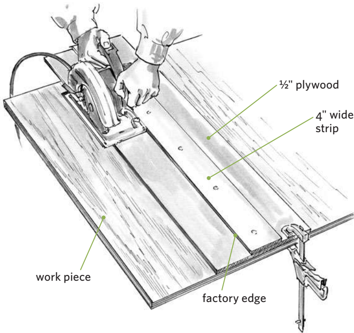
Using a straight-cutting jig
