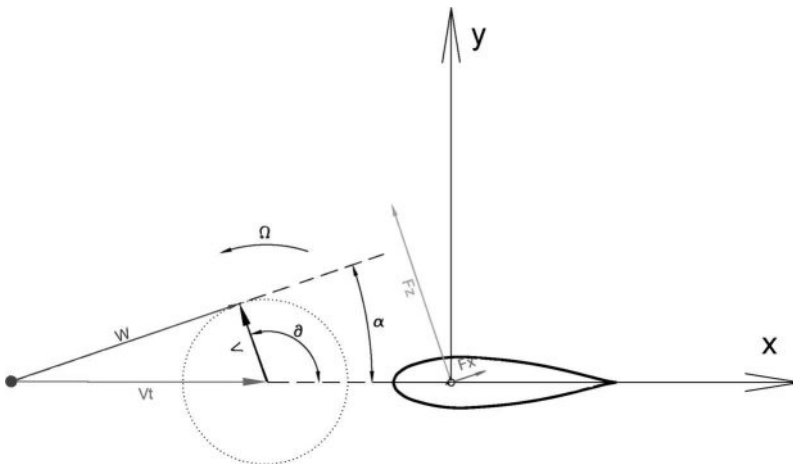
FIGURE 5.7 Condition of maximum pitch angle.
