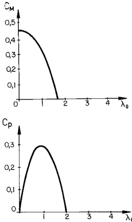
FIGURE 2.13 Characteristic operational curves of the American multi-blade, according to Le Gouirière , graphics by the Author.
