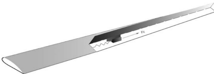
FIGURE 4.11 A centrifugal mass, placed inside the blade, displaces a wedge that in turn moves the spoiler.
