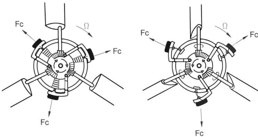
FIGURE 4.10 Operation principle of the centrifugal control of Jacobs turbines. Adaptation of drawings from Le Gourière , with thanks to prof. Arch. Mario Barbaro for the improvements.
