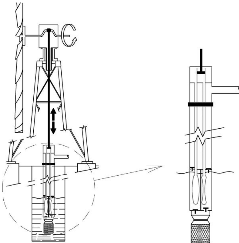
FIGURE 10.7 Double effect bladder pump.
