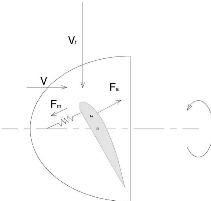
FIGURE 4.12 Pitch control by aerodynamic moment.
