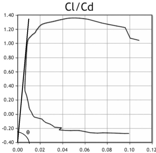
FIGURE 2.7 Polar of the airfoil E371, plotted with the free online aerodynamic simulator and plotter of airfoils www.airfoiltools.com .
