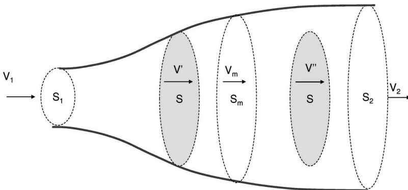
FIGURE 2.2 Hypothesis for the extension of Betz's theorem to two actuator disks disposed in series.
