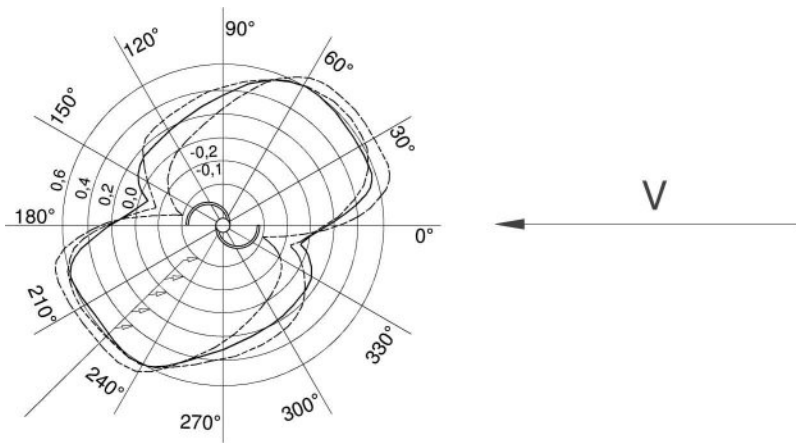
FIGURE 6.4 Start torque, C_a (Nm), as a function of the wind direction. The continuous line corresponds to rotor type II. Data from Le Gourrière , drawings by the author.
