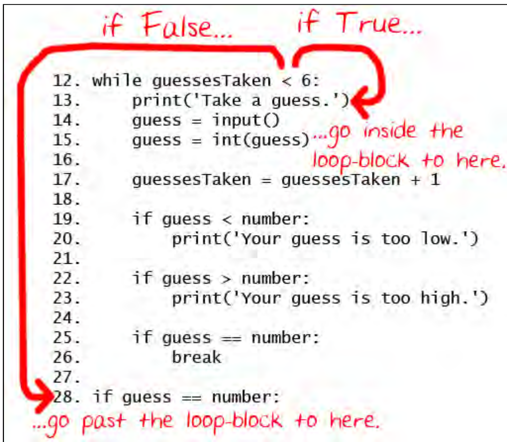
Figure 4-2: The while loop's condition.
