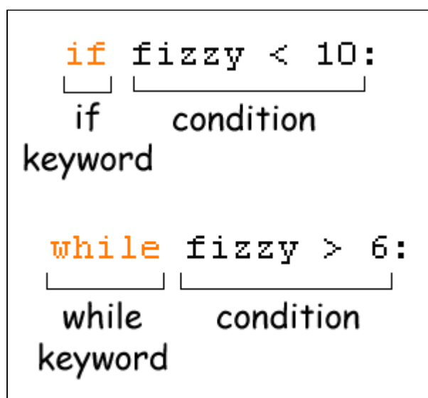
Figure 4-3: if and while statements.
