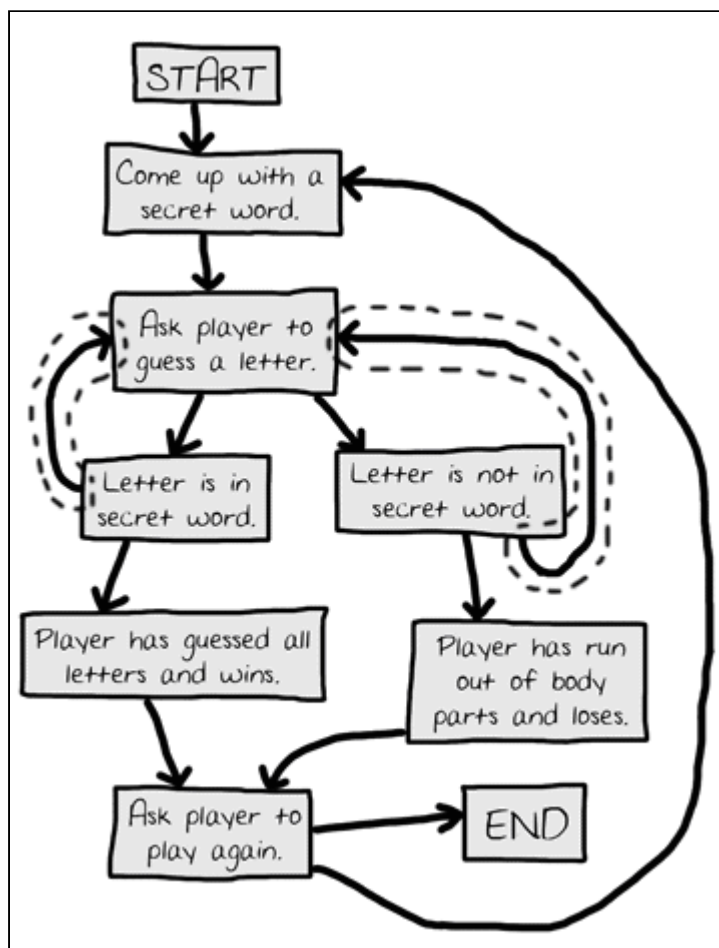
Figure 8-7: The game does not always end after a guess. The new arrows (outlined) show that the player can guess again.
