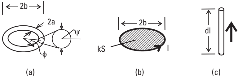
Figure 11.4 Small-antenna geometry showing (a) detail of the wire loop diameter, (b) the parameters kSl making up the loop moment, and (c) the elementary dipole moment ldl .
