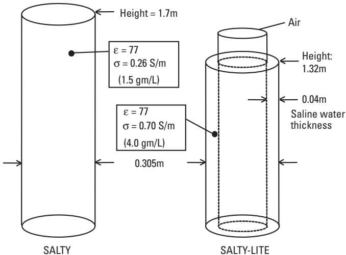
Figure 10.1 Standard human phantoms SALTY and SALTY-LITE. (After [1].)
