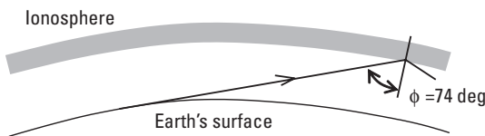
Figure 4.3 A horizontal ray incident on the ionosphere at the largest possible angle.
