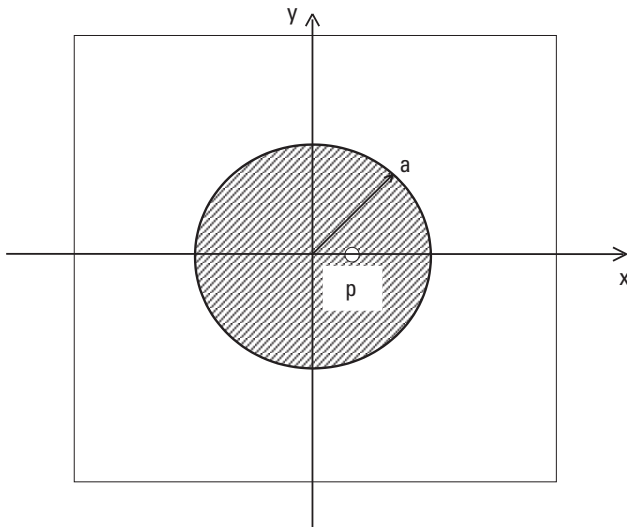
Figure 11.7 Geometry of the circular microstrip patch antenna.
