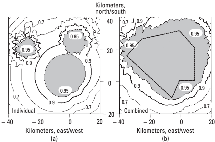
Figure 12.9 (a) Individual and (b) combined coverage probability with 2^\circ down-tilt from site 0.
