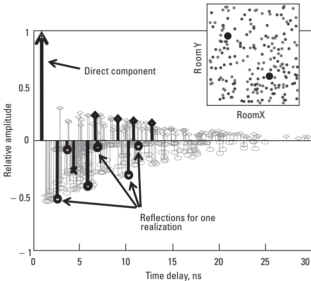
Figure 7.15 Multiple and a specific impulse realization.
