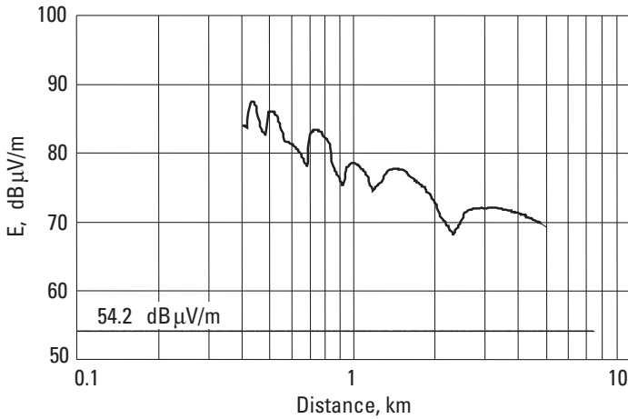
Figure 12.8 Close-in coverage from Site 0 with 2^\circ down-tilt.
