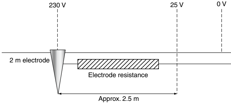
FIGURE 2.5 Electrode resistance.
