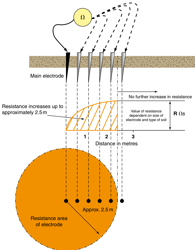
FIGURE 2.4 Earth electrode resistance area.
