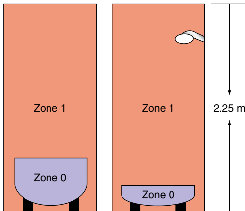
FIGURE 7.2 Zones 0 and 1.
