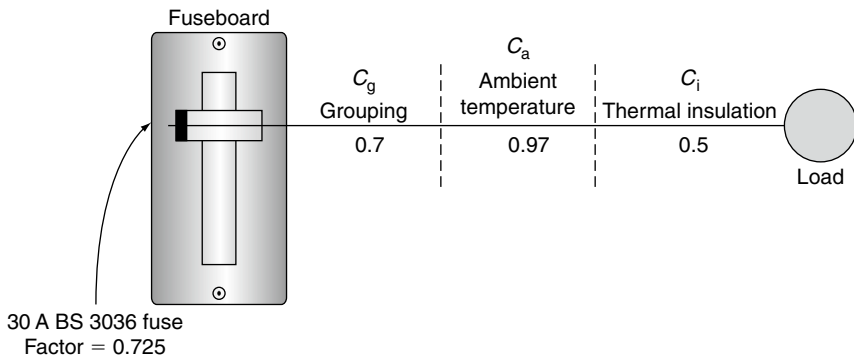
FIGURE 5.4 Conditions along cable route.
