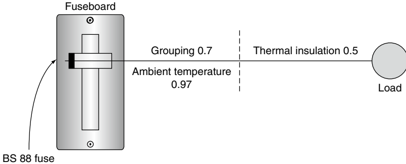
FIGURE 5.3 Conditions along cable route.
