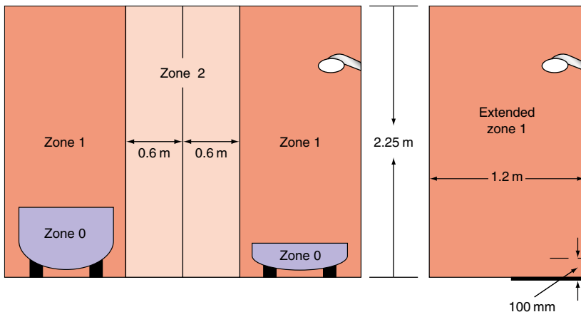
FIGURE 7.3 Zones 0, 1 and 2.
