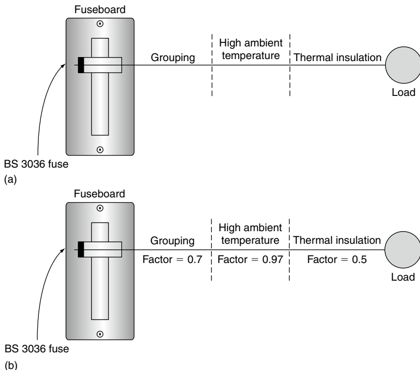
FIGURE 5.2 Conditions along cable route.
