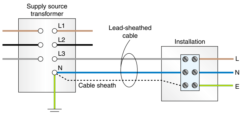
FIGURE 2.8 TN-S system.
