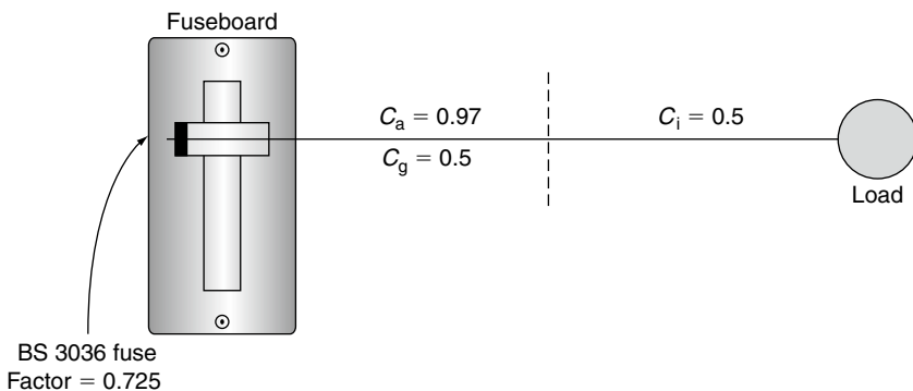
FIGURE 5.5 Conditions along cable route.
