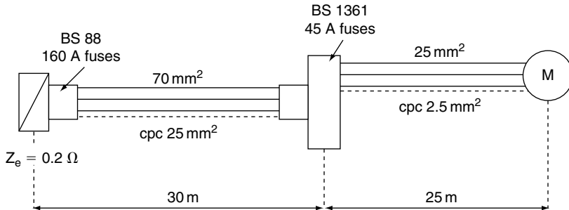
FIGURE 2.12 Diagram for Example 2.2
