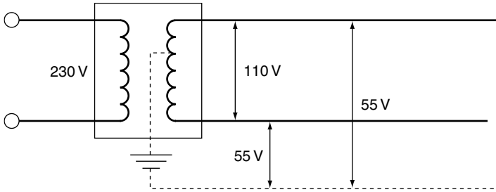
FIGURE 3.3 Reduced low voltage system.
