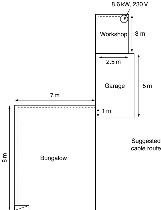
FIGURE 5.19 Diagram for Example on page 83.
