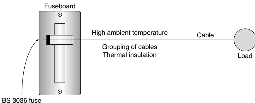
FIGURE 5.1 Conditions along cable route.
