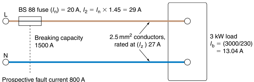
FIGURE 3.6 Breaking capacity and PFC.
