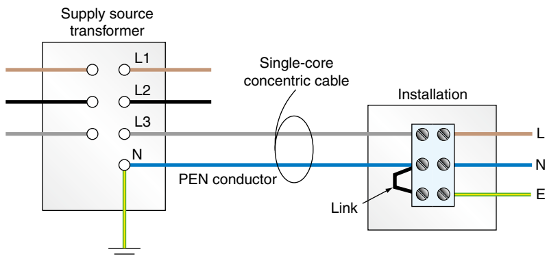
FIGURE 2.9 TN-C-S system.
