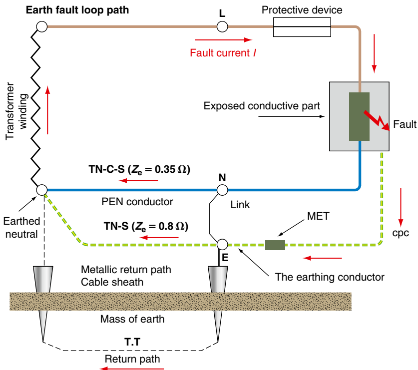
FIGURE 2.10 Earth fault loop path.
