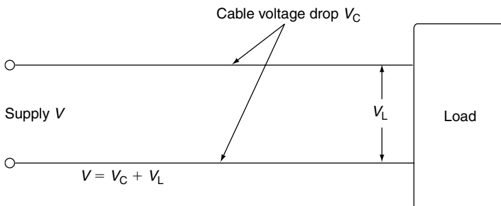
FIGURE 5.6 Voltage drop.
