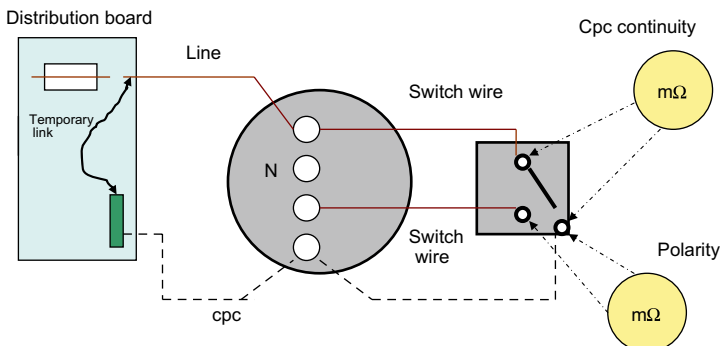
FIGURE 6.8 Lighting polarity.
