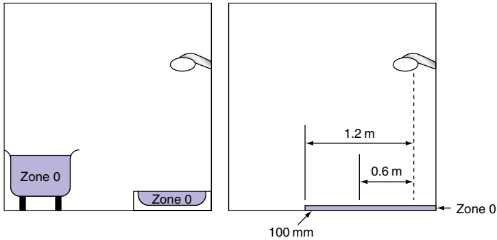
FIGURE 7.1 Zone 0.
