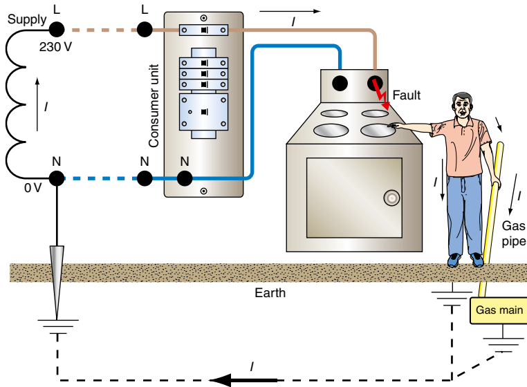
FIGURE 2.2 Shock path.
