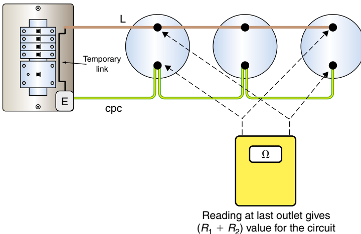
FIGURE 6.2 cpc continuity.
