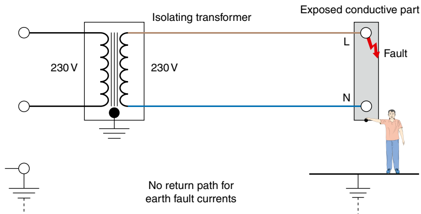
FIGURE 3.2 Electrical separation.
