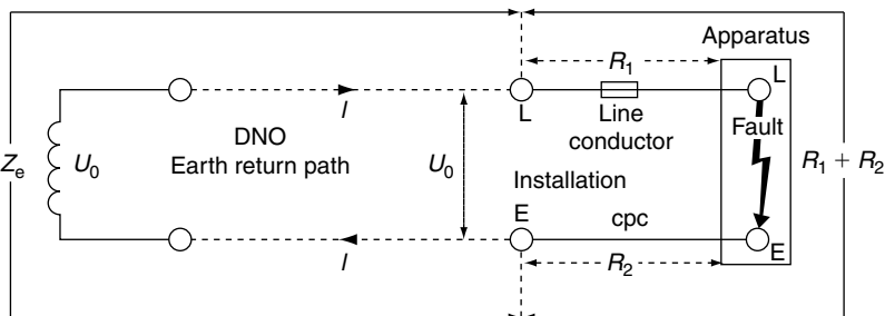
FIGURE 2.11 Simplified loop path.
