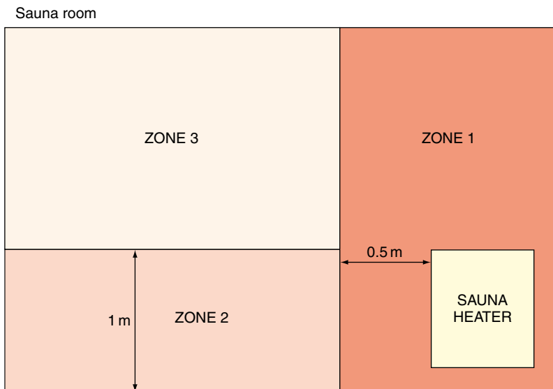
FIGURE 7.4 Sauna room zones.
