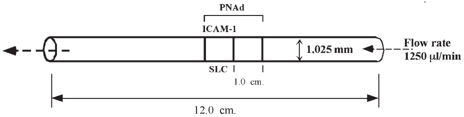
Fig. 1. Dimensions of the capillary tube and example of coating.
