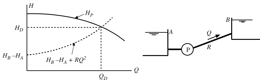
Figure 10.2 Pump and system demand curves.
