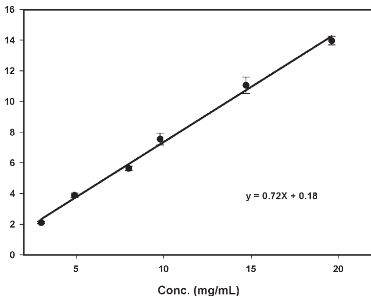
Fig. 2. A 4-d trans -stilbene oxide calibration curve from 3 to 20 mg/mL. The fitted equation y = 0.72x + 0.18 with a correlation coefficient of 0.99. The error bar is the 95% confidence interval.
