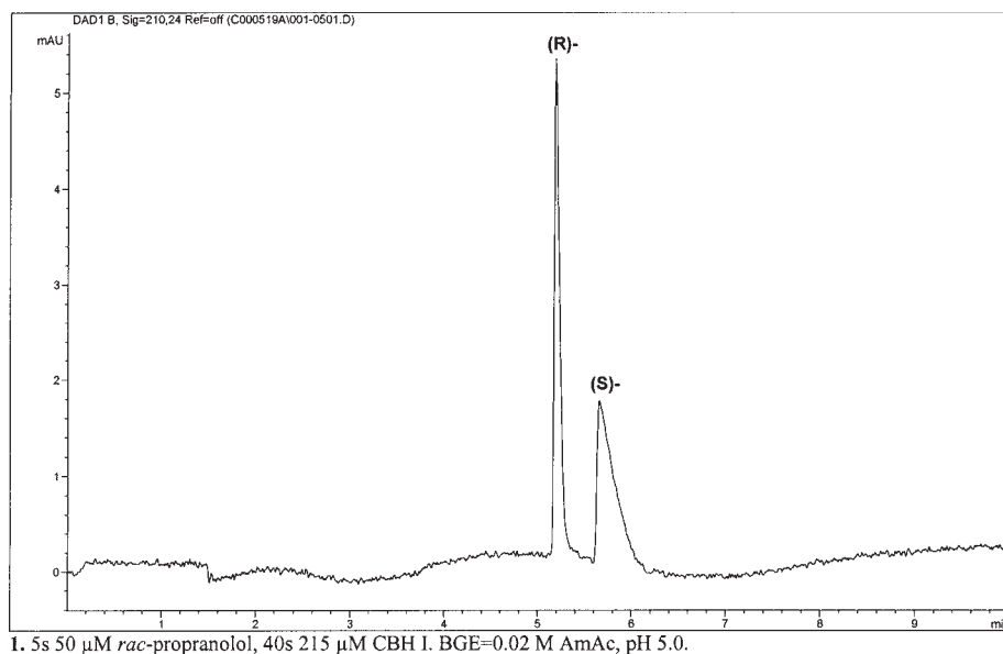
Fig. 1. 5 s 50 \mu M rac -propranolol, 40 s 215 \mu M CBH I. BGE = 0.02 M AmAc, pH 5.0.
