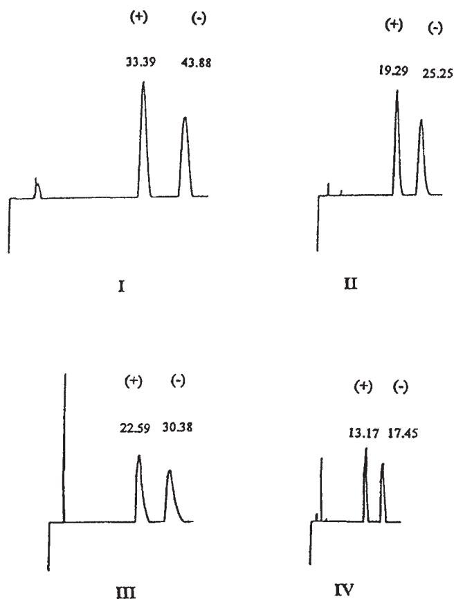
Fig. 4. The chromatograms of the resolved enantiomers of ( \pm )-neбиволol on Chiralpak AD (I and II) column using I: ethanol; II: 1-propanol; and Chiralpak AD-RH column (III and IV) using III: 1-propanol as the mobile phases with 0.5 mL/min as flow rate.
