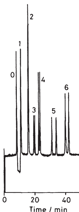
Fig. 5. Chiral separation of six PTH-DL-AAAs by MEKC (12). Corresponding AAs: (1) Ser, (2) Aba, (3) Nva, (4) Val, (5) Trp, (6) Nle; (0) acetonitrile. Micellar solution, 50 mM sodium N -dodecanoyl-L-valinate, 30 mM SDS, 0.5 M urea (pH 9.0) containing 10% (v/v) methanol; separation capillary, 50 \mu\text{m} i.d. \times 65 cm, 50 cm effective; total applied voltage, 20 kV; current, 17 \mu\text{A} ; detection wavelength, 260 nm; temperature, ambient.
