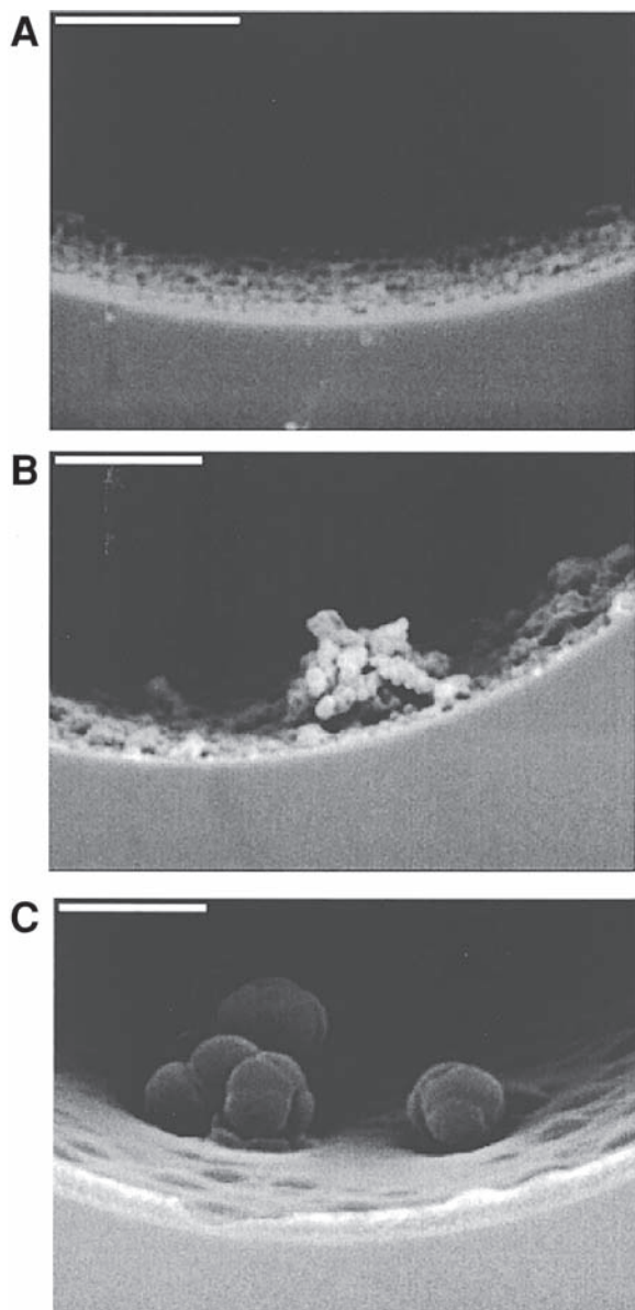
Fig. 2. Scanning electron micrographs of MIP surface coatings on the inner surface of a capillary. The MIP coatings are prepared with (A) toluene, (B) dichloromethane, and (C) acetonitrile as the polymerization solvent. Reprinted with permission from ref. 13 .
