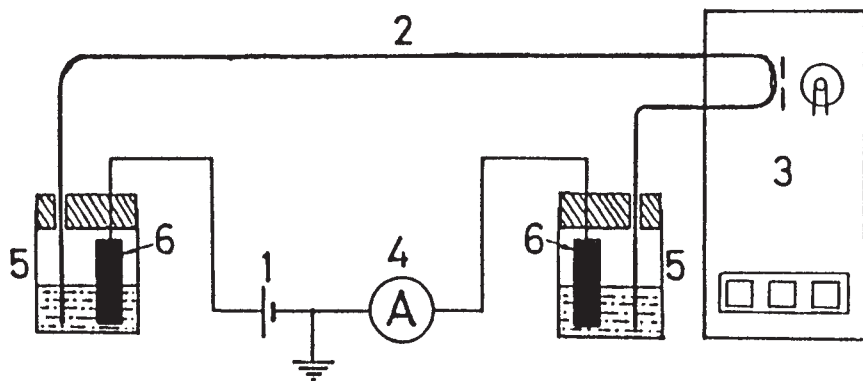
Fig. 2. A schematic illustration of the apparatus. (1) Regulated high voltage DC power supply, (2) fused silica tube, (3) UV detector, (4) ammeter, (5) electrode vessel (buffer reservoir), and (6) electrode.
