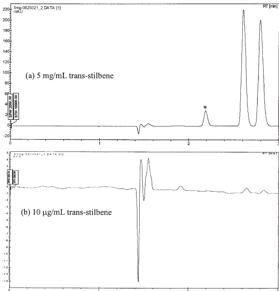
Fig. 1. Chromatogram of 5 mg/mL and 10 \mu g/mL trans -stilbene oxide standard. SFC conditions: injection vol, 2 \mu L; column temperature, 40°C; Berger Analytical SFC with an Agilent diode array detector; mobile phase, 30% (v/v) methanol/CO 2 ; run time, 3 min; detection, UV at 254 nm. *Indicates a chemical impurity.
