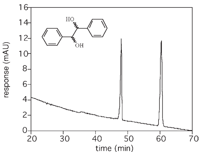
Fig. 5. Electropherogram of the chiral resolution of RR , SS -hydrobenzoin. Conditions: 1.8% \beta -CD, 50 mM borate, pH 9.3, and 20% (v/v) methanol, U = 18 kV, \lambda = 214 nm.
