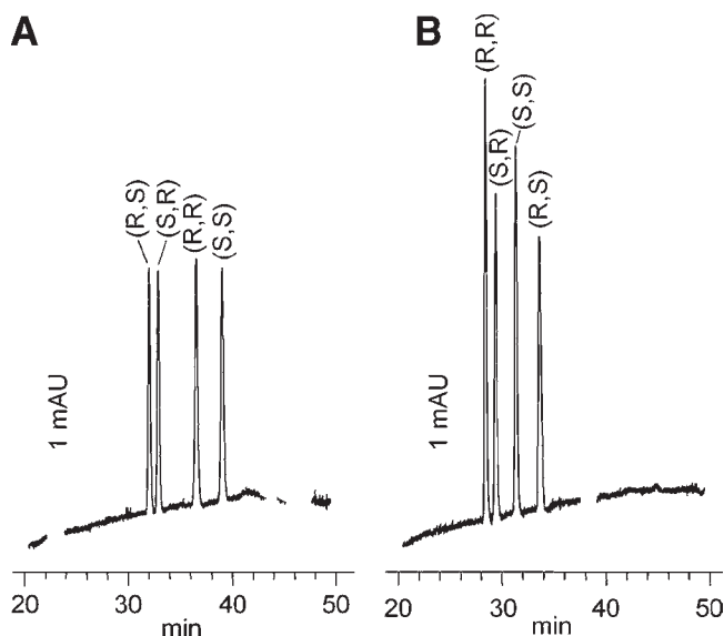
Fig. 3. Separation of all 4 stereoisomers of (A) DNZ-Ala-Ala and (B) DNP-Ala-Ala (reprinted with permission from ref. 14 ). Experimental conditions: polyvinyl alcohol (PVA)-coated capillary, 50 \mu\text{m} i.d., 64.5 cm total length, 56.0 cm effective length; BGE, methanol containing 100 mM acetic acid, and 12.5 mM triethylamine; selector solution, 10 mM O-9-( tert -butylcarbamoyl) quinine in BGE; partial filling, applied plug length: 50.4 cm; applied voltage, -25 kV (plain BGE at both inlet and outlet electrode vessels during run); temperature, 15^\circ\text{C} .
