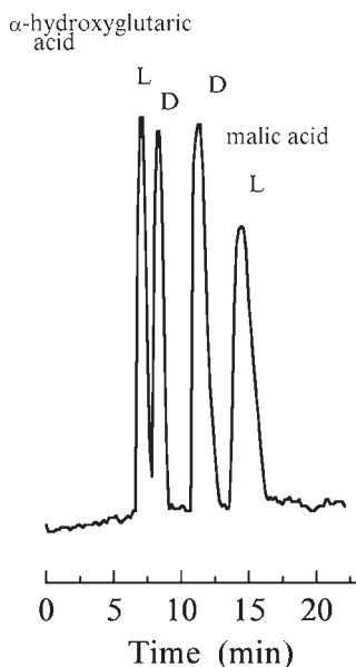
Fig. 1. Chromatogram of a mixture of DL-2-hydroxyglutaric acid and DL-malic acid (5 \mu\text{g} of each). Redrawn from ref. 5 with permission. Conditions: column, Chiral-Si 100 L-HyProCu, 5 \mu\text{m} , 250 \times 4.6 mm I.D.; eluent, 0.1 mM copper sulfate in 0.01 mM \text{KH}_2\text{PO}_4 ; flow rate, 2 mL/min; temperature, 50°C; detection, 223 nm.
