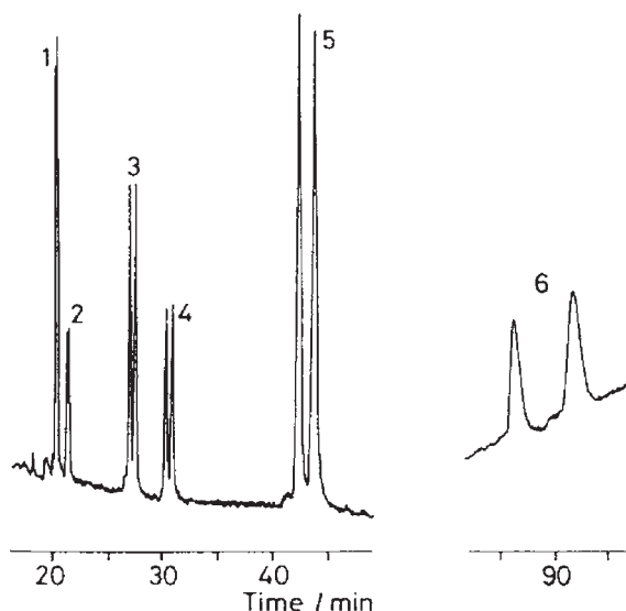
Fig. 4. Chiral separation of six PTH-DL-AAs by MEKC ( II ). Corresponding AAs: (1) Trp, (2) Nle, (3) Nva, (4) Val, (5) Aba, (6) Ala. Micellar solution, 25 mM digitonin, 50 mM SDS (pH 3.0); separation capillary, 50 \mu m i.d. \times 63 cm, 49 cm effective; total applied voltage, 20 kV; current, 34 \mu A; detection wavelength, 260 nm; temperature, ambient.
