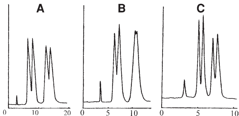
Fig. 13. Temperature effect on separation of \beta -MePhe enantiomers. Column: Chirobiotic T; MP: H 2 O/MeOH (10/90, v/v), detection 202 nm. Flow rate 1 mL/min. (A) 1°C, (B) 20°C (C) 50°C; peaks: 1) erythro-L isomer, 2) erythro-D isomer; 3) threo-L isomer; 4) threo-D isomer. Revised from ref. 14 .
