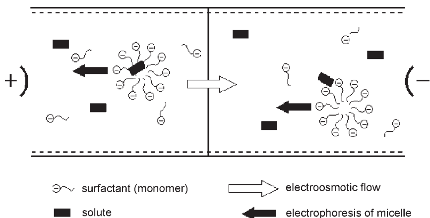
Fig. 1. Schematic illustration of the separation principle of MEKC.
