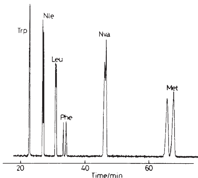
Fig. 2. Chiral separation of Dns-DL-AAs with 50 mM STDC in 50 mM phosphate buffer (pH 3.0) (9). Separation capillary, 50 \mu m i.d. \times 70 cm, 50 cm effective; current, 50 \mu A; temperature, 40°C.
