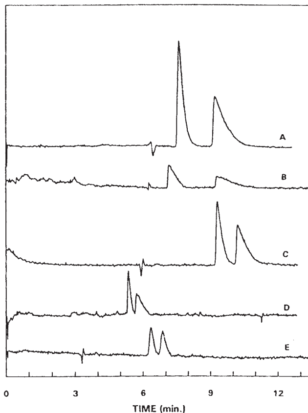
Fig. 4. Electrochromatograms showing the enantiomeric separations of disopyramide ( A ), pentobarbital ( B ), hexobarbital ( C ), cyclophosphamide ( D ) and benzoin ( E ). Reproduced from ref. 6 with permission. Conditions: ( A ) disopyramide (15% 2-propanol/4 mM sodium phosphate buffer, pH 6.8, applied voltage 12 kV, current 2 \mu A); ( B ) pentobarbital (2% 2-propanol/2 mM sodium phosphate buffer, pH 5.5, applied voltage 20 kV, current 2 \mu A); ( C ) hexobarbital (2% 2-propanol/2 mM sodium phosphate buffer, pH 5.5, applied voltage 18 kV, current 2 \mu A); ( D ) cyclophosphamide (3% 2-propanol/2 mM sodium phosphate buffer, pH 6.5, applied voltage 25 kV, current 2 \mu A); ( E ) benzoin (5% 1-propanol/5 mM sodium phosphate buffer, pH 6.5, applied voltage 15 kV, current 3 \mu A).
