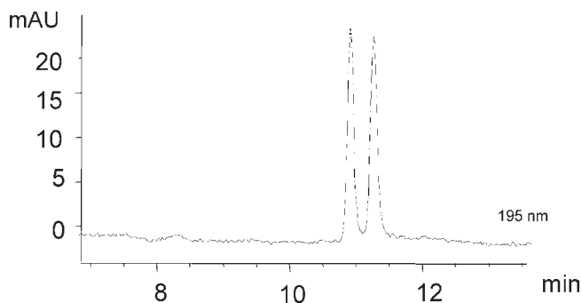
Fig. 4. Electrochromatogram of the enantiomeric separation of propranolol. Modified from ref. 11 . Experimental conditions: capillary, 35 cm total length, 26.5 cm effective length; cm length of vancomycin stationary phase, 75 \mu m I.D.; mobile phase, 100 mM ammonium acetate, pH 6.0 mixed with 90% acetonitrile, 5 mM was the concentration of ammonium acetate. Sample, 0.2 mg/mL of racemic propranolol. Applied voltage, 25 kV, 20°C, pressurized at both sides at 10 bar. Injection, 12 bar \times 0.5 min followed by a buffer plug at 12 bar \times 0.2 min.
