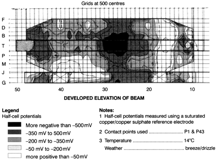
Fig. 2.1 Sample schematic of half-cell data.
