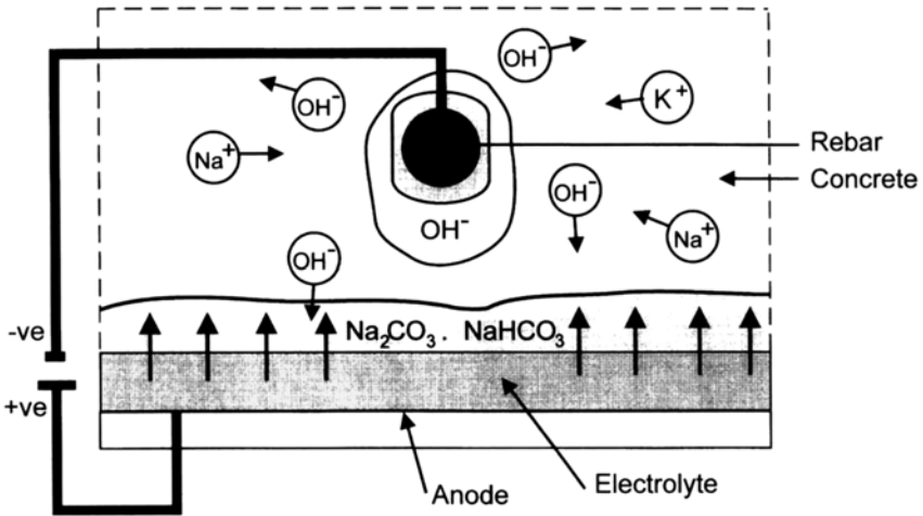
Fig. 8.1 The realkalization process.
