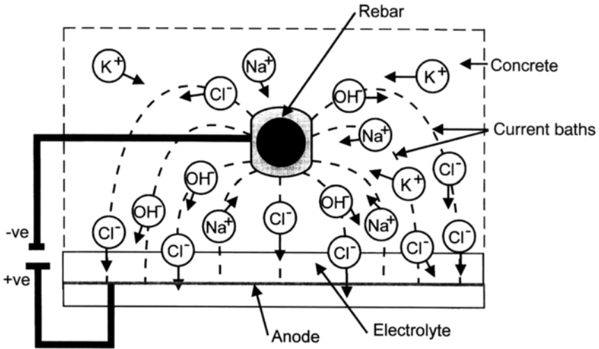
Fig. 8.4 The desalination process.
