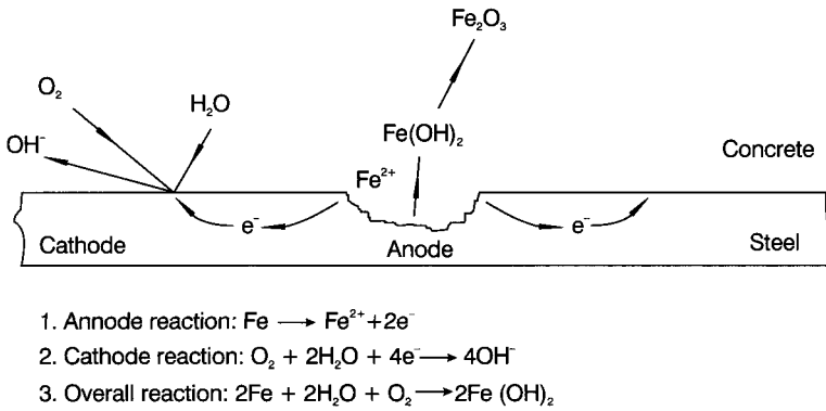
Fig. 6.1 Mechanism of steel corrosion in chloride-contaminated concrete.
