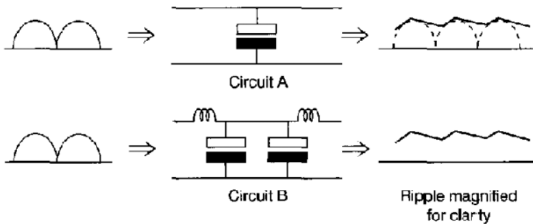
Fig 5.2 Smoothing circuits with results.
