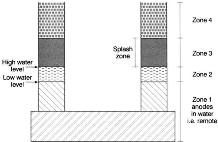
Fig. 3.1 Zoning on a marine support structure.
