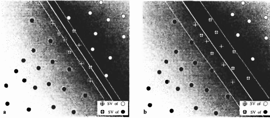
Figure 5.47. SVM linear discrimination of two non-separable classes. (a) C=100 , with nine support vectors; (b) C=\infty , with twelve support vectors.
