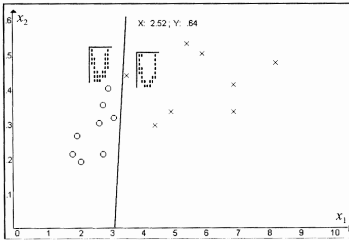
Figure 5.15. Separation of U's (right side) from V's (left side) by a perceptron. Borderline U and V lying near the linear discriminant are also shown.
