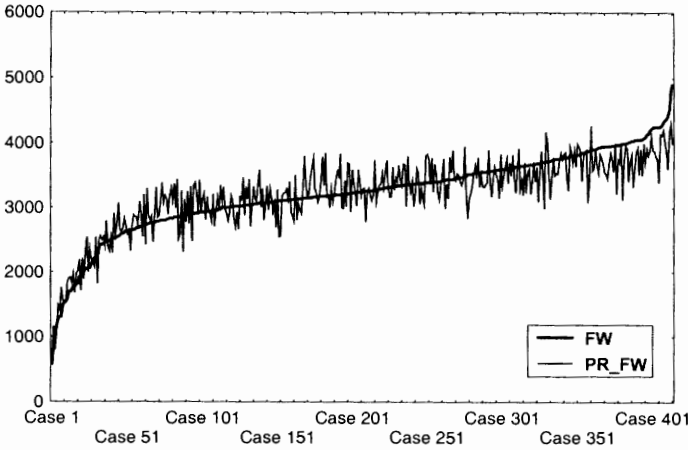
Figure 5.43. Prediction of foetal weight using an RBF4:4:1 network with Gaussian kernel and k-means centroid adjustment (compare with Figure 5.40).
