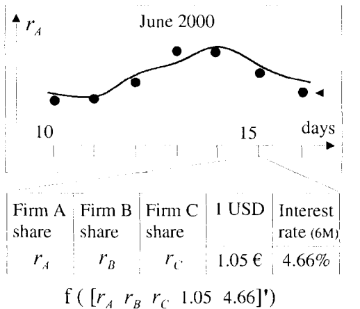
Figure 1.5. Share value forecast one-day ahead. r_A, r_B, r_C are share values of three firms. Functional approximation (black circles) of the true value of r_A (solid curve), is shown for June 16 depending on the values of the shares, euro-dollar exchange rate and interest rate for June 15.
