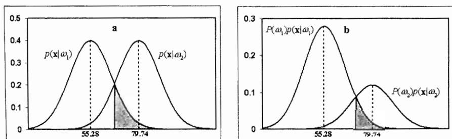
Figure 4.13. Influence of the prevalence threshold on the classification errors, represented by the shaded areas (dark grey represents the errors for class \omega_1 ). (a) Equal prevalences; (b) Unequal prevalences.
