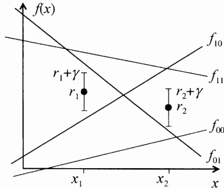
Figure 5.35. The class of functions F = \{ (x, f(x) = ax + b); a, b \in \mathfrak{R} \} pseudo-shatters the set \{x_1, x_2\} . The four functions shown achieve all possible "above/below" combinations of \{r_1, r_2\} .
