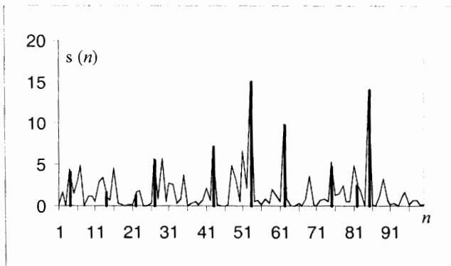
Figure 4.32. One hundred samples of a signal consisting of noise plus signal impulses (bold lines) occurring at random times.
