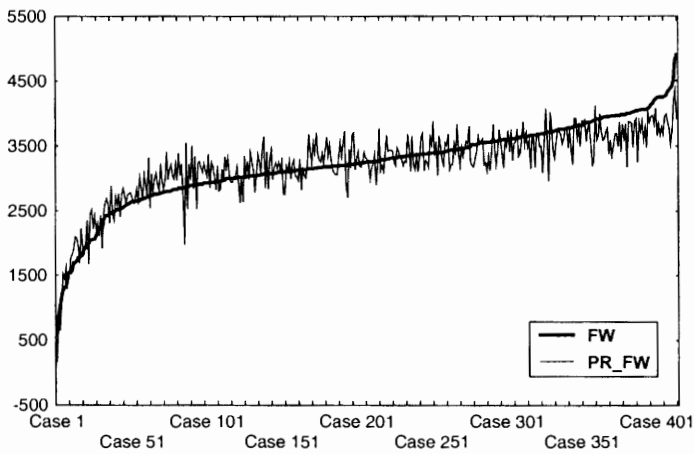
Figure 5.27. Predicted foetal weight (PR_FW) using an MLP3:6:1 trained with the back-propagation algorithm. The FW curve represents the true foetal weight values.
