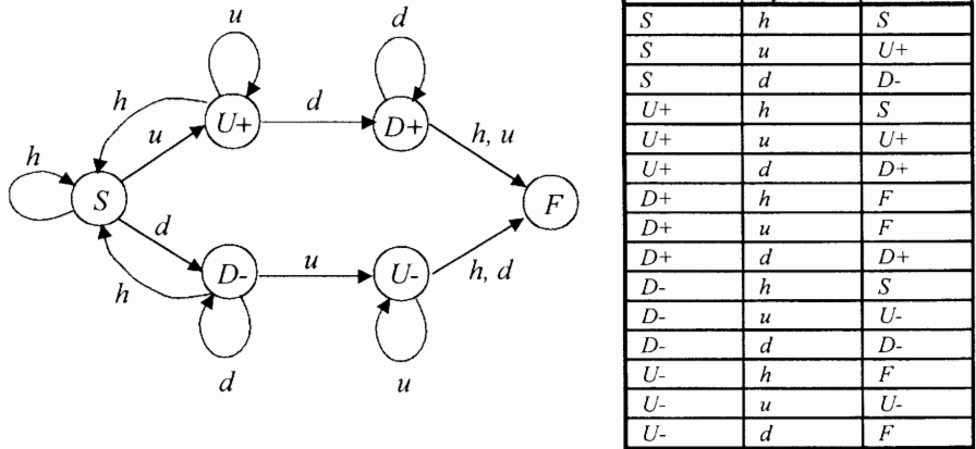
Figure 6.10. Finite-state automaton represented by its state-diagram, with corresponding state-transition table. The automaton recognizes waveform peaks without horizontal plateaus.
