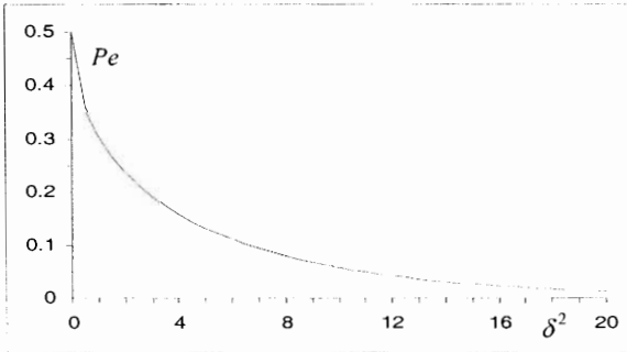
Figure 4.19. Error probability of a Bayesian two-class discrimination with normal distributions and equal prevalences and covariance.
