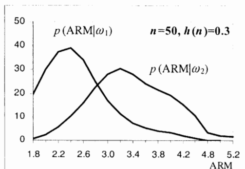
Figure 4.29. Parzen window estimate of feature ARM pdf (multiplied by 50) for two classes of cork stoppers.
