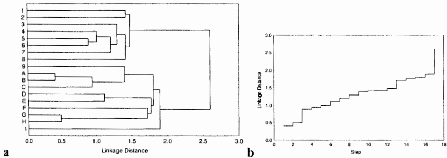
Figure 3.8. Single linkage clustering of filamentary data. (a) Dendrogram; (b) Clustering schedule graph.
