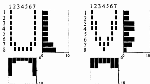
Figure 5.14. Examples of handwritten U and V on a 7x8 grid, with the respective projections.
