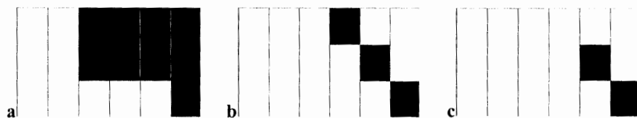
Figure 6.24. Hopfield net illustrating the probabilities associated with the assignments corresponding to the example shown in Figure 6.23. (a) Feasible assignments as solutions to the quadratic problem; (b) A candidate assignment; (c) final assignment corresponding to the previous situation ( q=2 ).
