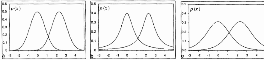
Figure 4.20. Two classes with symmetric distributions and the same standard deviation. (a) Normal; (b) Cauchy; (c) Logistic.
