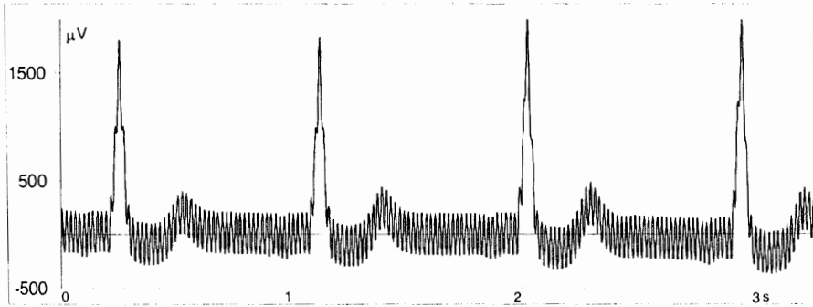
Figure 5.3. Discretized ECG tracing (3.4 seconds) with added 50 Hz noise. Sampling rate is 500 Hz and amplitude is in microvolts. The jagged contour of the signal is due solely to its discrete representation.
