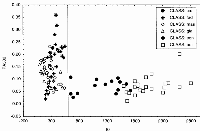
Figure 4.39. Scatter plot of six classes of breast tissue using features I0 and PA500.
