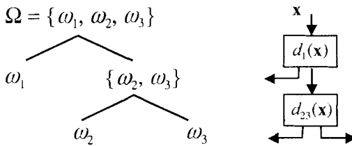
Figure 2.7. Hierarchical classification of a feature vector into one of the classes exemplified in Figure 2.6.
