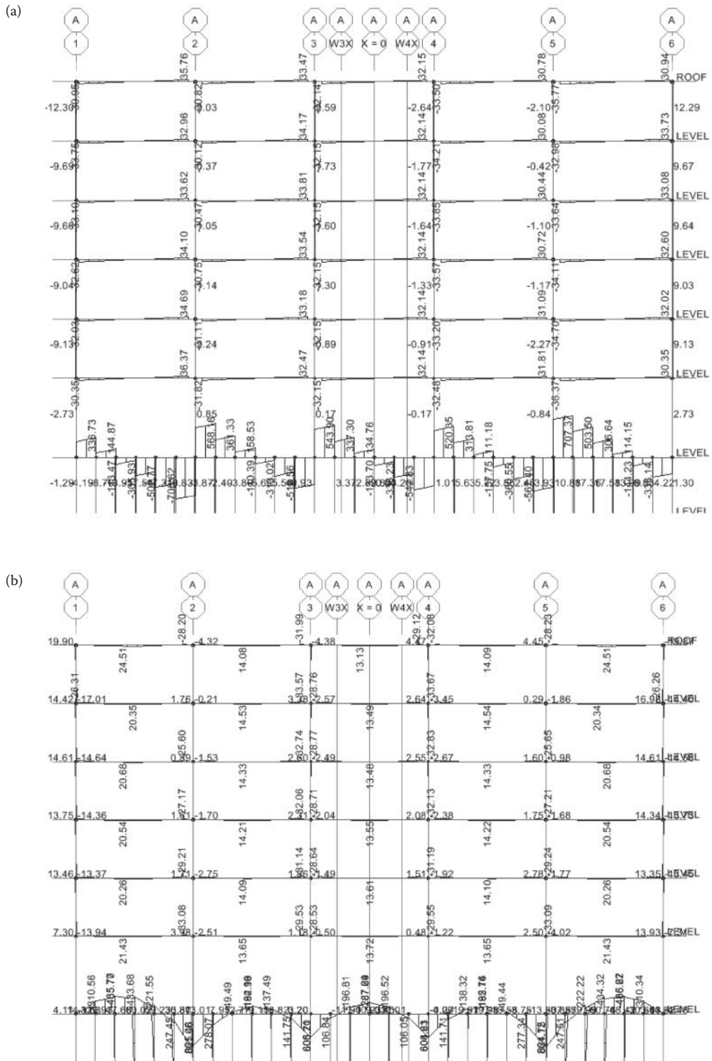
Figure 7.26 Shears (a); and moments (b), for quasi-permanent loads G + \psi_2 Q . Frame A.
