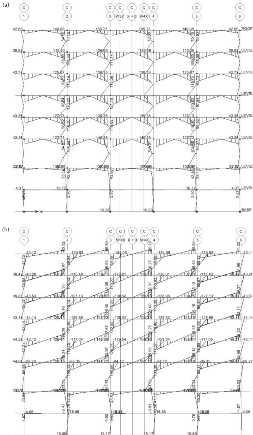
Figure 7.15 Seismic moments: (a) modal analysis; (b) lateral-force method, E_x + 0.3E_y . Frame C.
