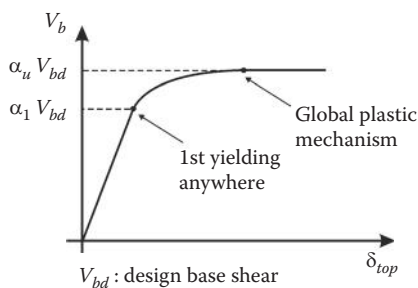
Figure 4.13 Definition of factors \alpha_u and \alpha_1 on the basis of a base shear vs. top displacement diagram from pushover analysis.
