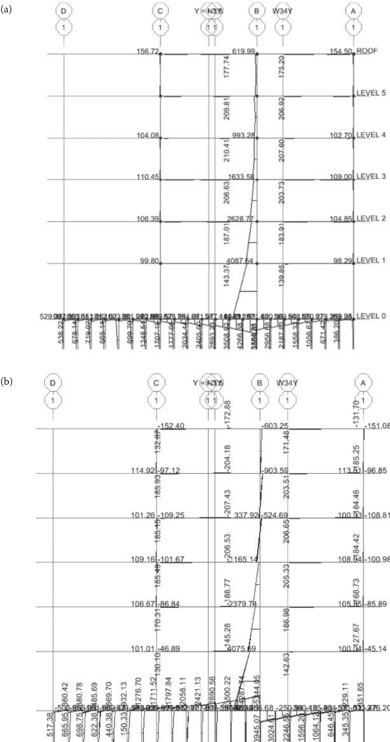
Figure 7.19 Seismic moments (a) modal analysis; (b) lateral-force method, E_y + 0.3E_x . Frame I WL.
