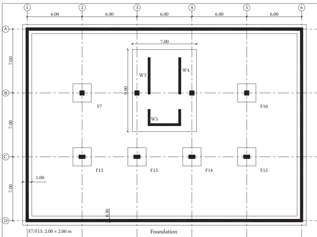
Figure 7.4 Foundation plan.
