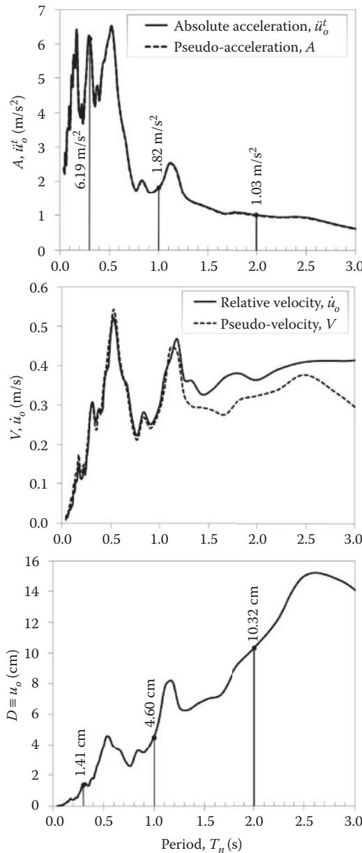
Figure 3.6 Spectra for the relative displacement u_o \equiv D , relative velocity \dot{u}_o and absolute acceleration \ddot{u}_o^t , as well as the pseudo-velocity V and pseudo-acceleration spectra A for the Ulcinj (Albatros, N–S direction) ground motion and 5% damping.
