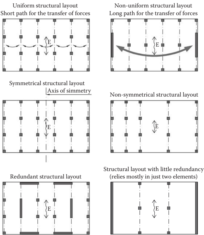
Figure 4.2 Uniformity in plan, symmetry and redundancy.
