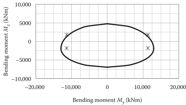
Figure 7.48 Biaxial design moments (seismic action effects) at the base of wall W5 (displayed as asterisks) compared to the biaxial moment resistance diagram (local y-axis is parallel to global Y and corresponds to bending in the X-plane; local z-axis: parallel to global X, bending in the Y-plane).
