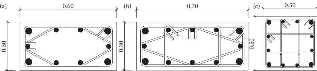
Figure 7.43 Column vertical reinforcement and tie layout: (a) corner columns C1, C6, C11, C16 (vertical bars 4\phi 18 + 6\phi 14 ); (b) intermediate columns in frames A and C: C2 to C5, C12 to C15 (vertical bars 4\phi 18 + 8\phi 14 ); (c) interior columns C7 to C10 (vertical bars 4\phi 18 + 8\phi 14 ).
