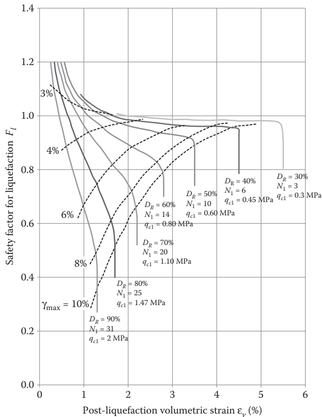
Figure 6.7 Post-liquefaction volumetric strains.
