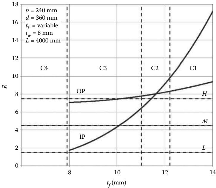
Figure 5.41 Parametrical study: Influence of flange thickness.
