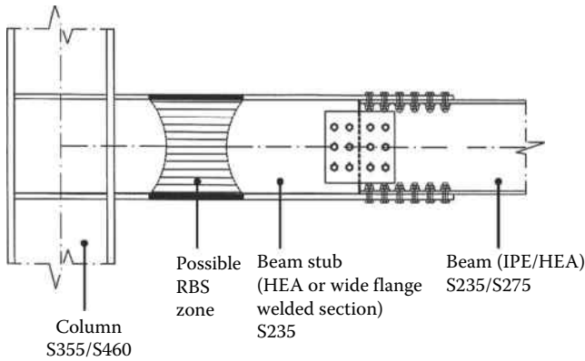
Figure 5.69 Structural details enhancing the ductile capacity of a beam in a frame.
