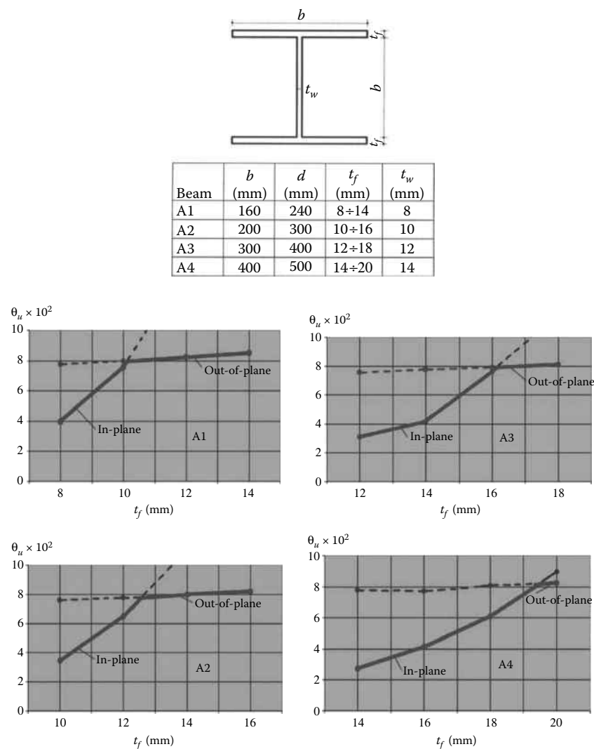
Figure 5.31 Ultimate rotations for in-plane and out-of-plane mechanisms for different double T sections.
