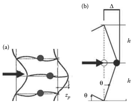
Figure 5.II0 Modeling of story drift.
