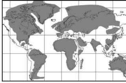
Figure 3.23 Stable continental areas. (Gioncu, V., Mazzolani, F.M. 2011: Earthquake Engineering and Structural Design . Taylor & Francis, London; after Mooney, W.D., Schulte, S., Detweiler, S.T. 2004: 26th Seismic Research Review, Trend in Nuclear Explosion Monitoring , 439–448.)
