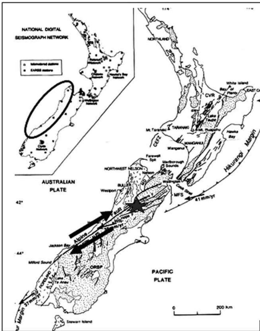
Figure 1.49 Christchurch earthquake produced by strike-slip Alpine fault. (Gioncu, V., Mazzolani, F.M. 2011: Earthquake Engineering for Structural Design . Spon Press, London.)
