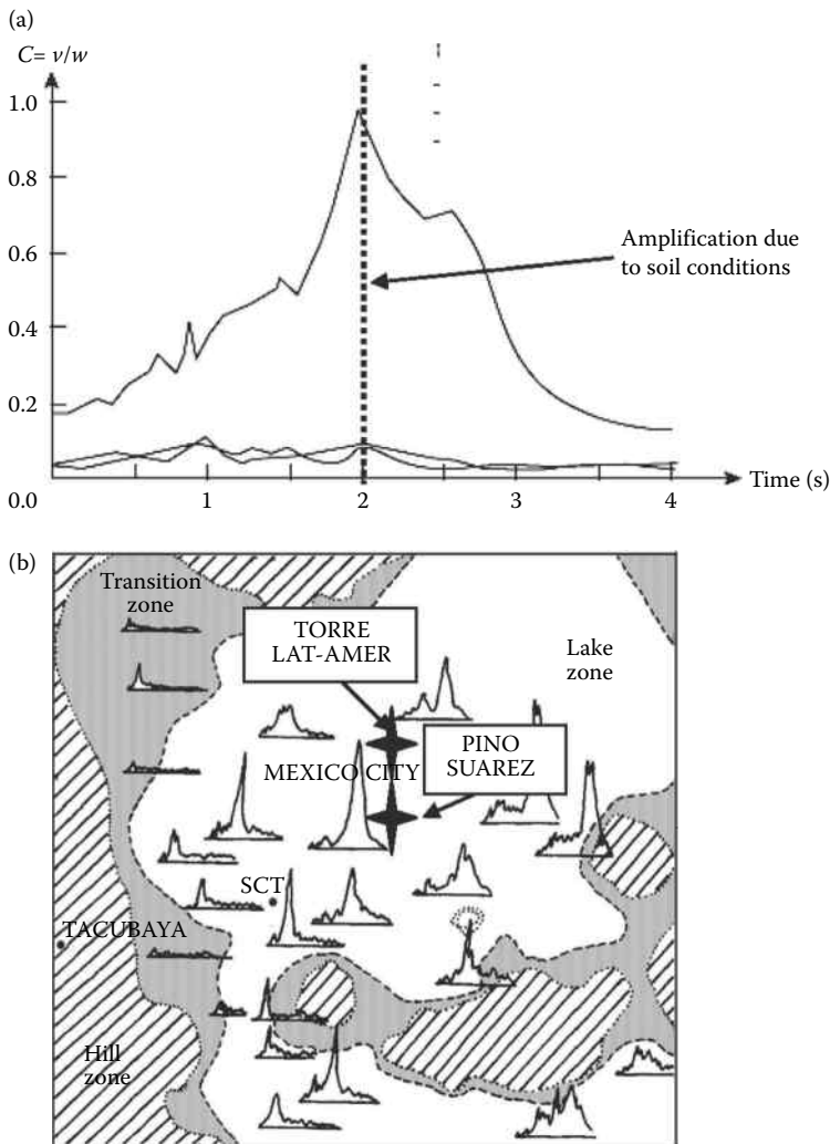
Figure 1.9 Accelerations amplification: (a) response spectra. (After Scawthorn, C. 2003: Earthquake Engineering Handbook (eds. W.F. Chen and C. Scawthorn), CRC Press.) (b) Distribution of spectra for Mexico City Valley. (From Gioncu, V., Mazzolani, F.M. 2002: Ductility of Seismic Resistant Steel Structures . Spon Press, London.)
