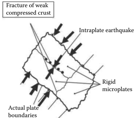
Figure 3.24 Fracture of weak compressed crust. (Gioncu, V., Mazzolani, F.M. 2011: Earthquake Engineering and Structural Design . Taylor & Francis, London.)
