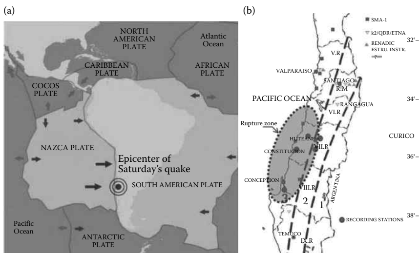
Figure 1.47 The Maule earthquake in Chile: (a) contact between Nazca and South American plates; (b) affected area. (After Herrera R.A., Beltrán J.F., Aguirre C., Verdugo A. 2012: Behavior of Steel Structures in Seismic Areas, STESSA 2012 (eds. F.M. Mazzolani, R.A. Herrera), Santiago, January 9–11, CRC Press, 37–43.)
