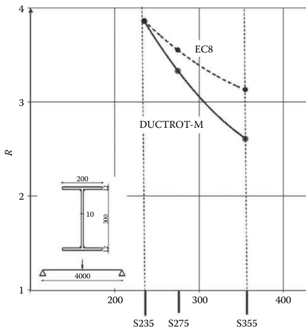
Figure 5.39 Influence of steel grade on rotation capacity.
