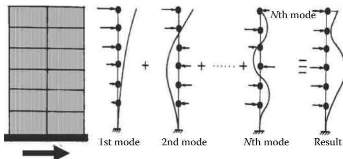
Figure 5.80 Vibration approach.
