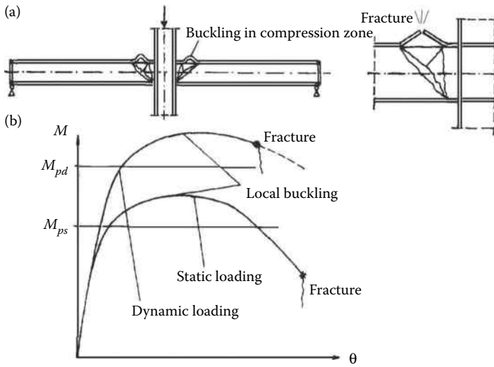
Figure 5.100 Strain-rate effects for beams.
