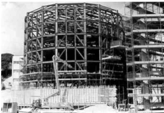
Figure 2.23 Steel EBF structure of the Messina University library.
