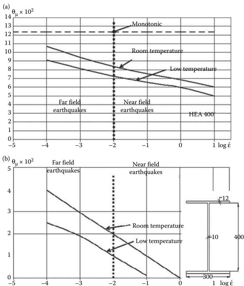
Figure 5.9I Influence of strain rate on rotation capacity: (a) rolled profile HEA400; (b) welded profile.
