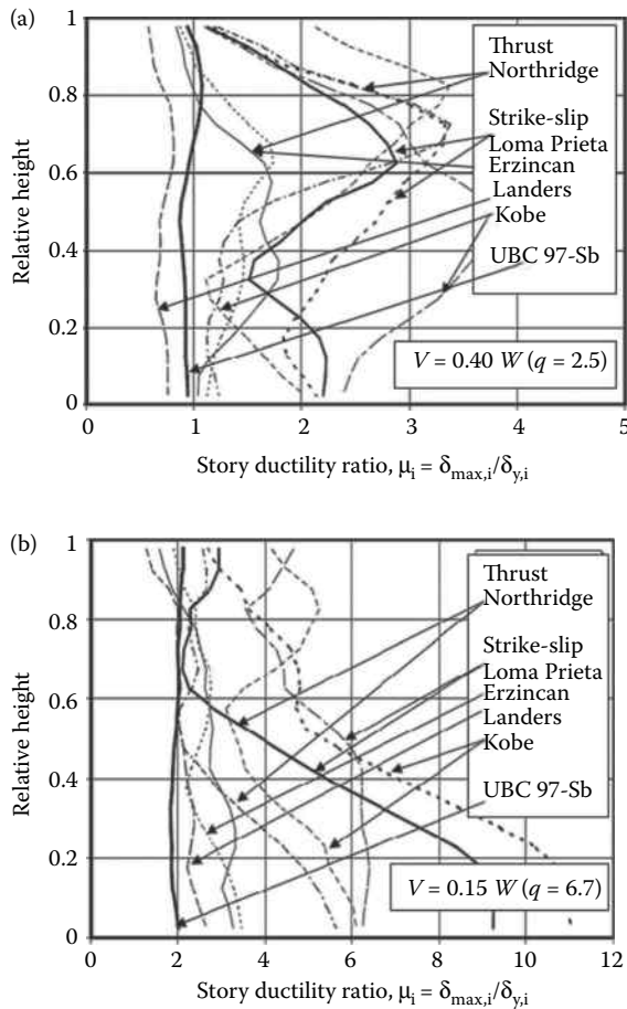
Figure 3.18 Ductility demands for near-source ground motions: (a) moderate ductility frame; (b) high ductility frame. (Gioncu, V., Mazzolani, F.M. 2011: Earthquake Engineering and Structural Design . Taylor & Francis, London; after Alavi, B., Krawinkler, H. 2001: Effects of near-fault ground motions on frame structures. Blume Earthquake Engineering Center, Department of Civil and Environmental Engineering, Stanford University, Report No. 138.)
