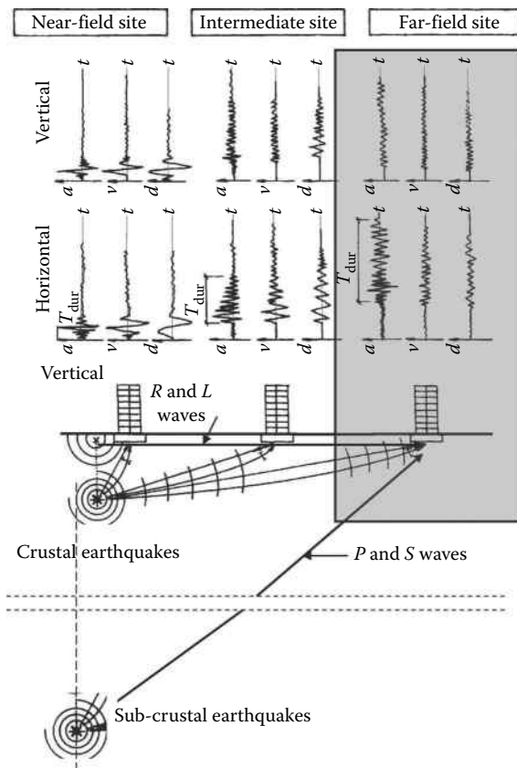
Figure 5.48 Far-field earthquakes.
