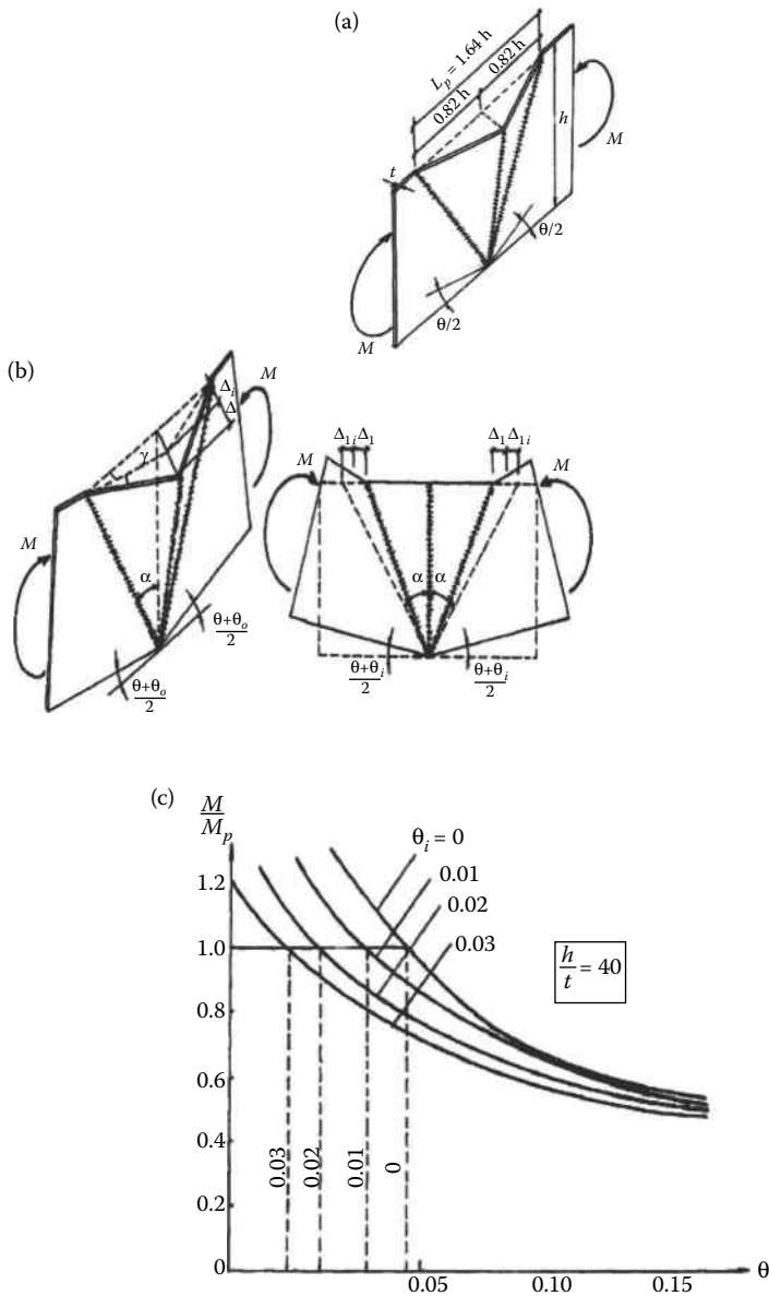
Figure 5.60 Yielding mechanism of a bended plate: (a) mechanism configuration; (b) mechanism with initial deformations; (c) moment–rotation curve relation, influence of initial deformations.
