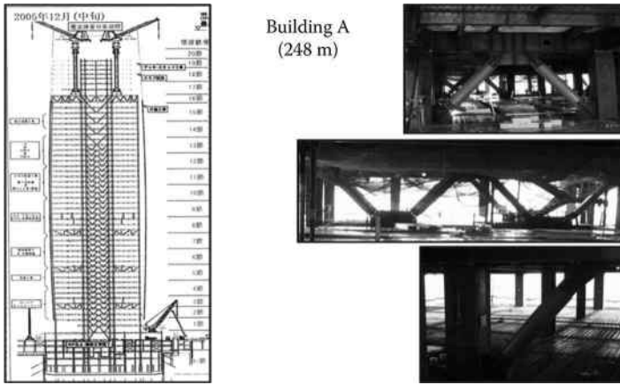
Figure 4.29 The BRB structural system in the Midtown building in Tokyo.
