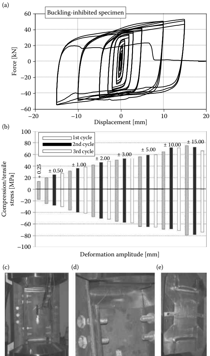
Figure 4.79 Buckling-inhibited pure aluminum specimen: (a) hysteretic behavior; (b) strength for each cycle; (c, d, e) collapse mode.
