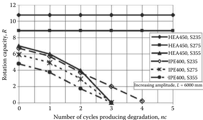
Figure 5.72 Influence of steel quality on the available cyclic member ductility.
