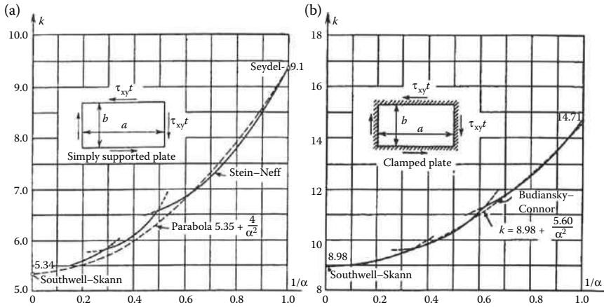
Figure 4.50 Values of the plate factor k for (a) simply supported and (b) clamped plates.
