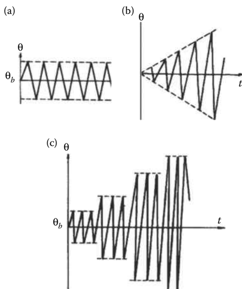
Figure 5.53 Cycle loading types: (a) constant amplitude; (b) gradually increasing amplitude; (c) ECCS experimental proposal.
