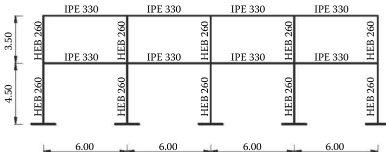
Figure 6.31 Steel MRF structure analyzed as case study [m].
