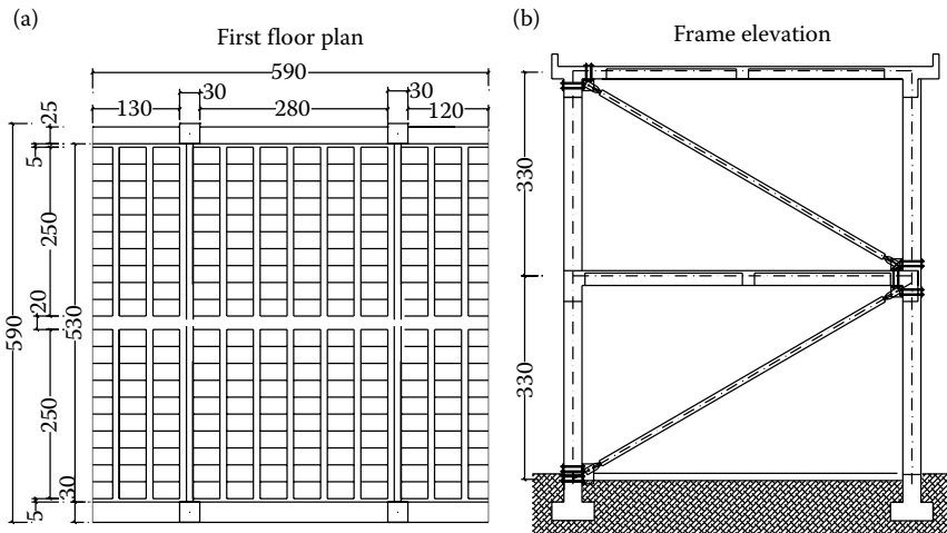
Figure 4.34 Features of the tested RC structure: (a) plane; (b) elevation.
