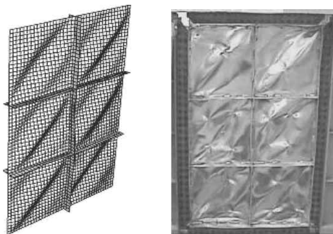
Figure 4.84 Numerical-experimental comparison for AW1050A panels type B.
