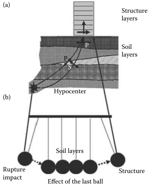
Figure 5.78 Waves propagation in soil and in site with structure: (a) soil-structure system; (b) Newton's cradle—effect of last ball.
