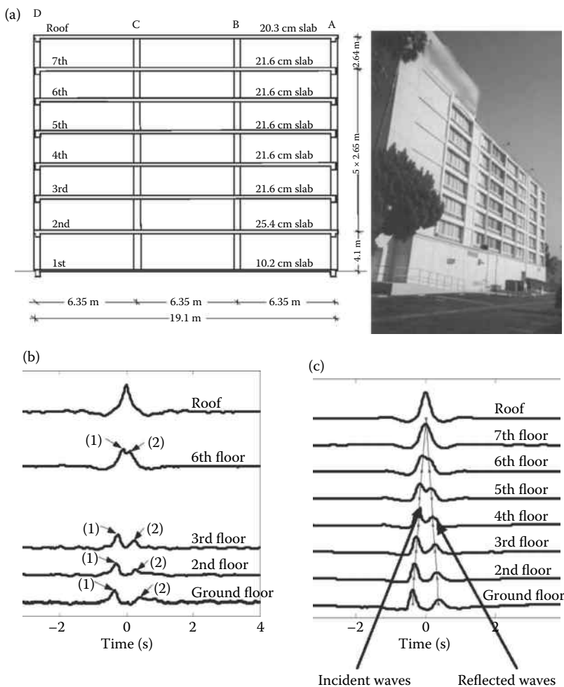
Figure 5.83 Van Nuyts hotel: (a) structure and view; (b and c) wave propagation. (Modified after Kawakami, H., Oyungchimeg, M. 2004: 13th World Conference on Earthquake Engineering , Vancouver, 2004, 1–6 August, Paper No. 317.)
