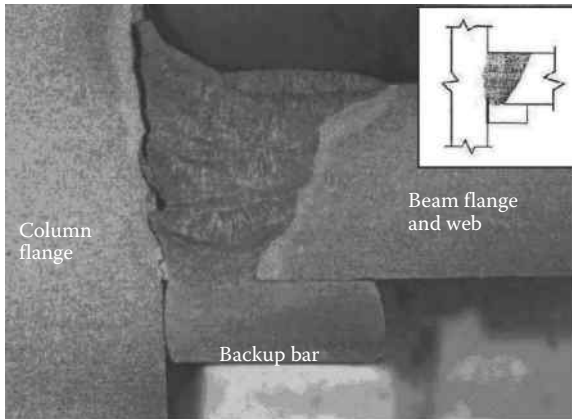
Figure 1.24 Fracture of the welds due to backup bar. (After Chi, W.M., Deierlein, G., Ingrassia, A. 2000: Journal of Structural Engineering , 126(1), 88–97.)
