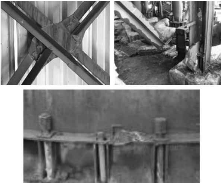
Figure 1.48 Fracture of braces and bolt anchors. (Herrera R.A., Beltran J.F., Aguirre C., Verdugo A. 2012: Behavior of Steel Structures in Seismic Areas , STESSA 2012 (eds. F.M. Mazzolani, R.A. Herrera), Santiago, January 9–11, CRC Press, 37–43.)
