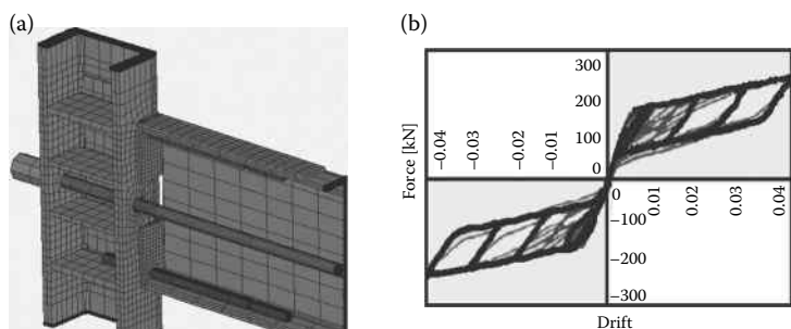
Figure 4.119 Numerical model of the PTED connection with PT- and ED-bars: (a) finite element mesh; (b) numerical versus experimental results. (Esposto, M., Faggiano, B., Mazzolani, F.M. 2006b: In Proceedings of 8th International Conference on Computational Structures Technology , Las Palmas de Gran Canaria, Spain, 12–15 September, Paper No. 117.)
