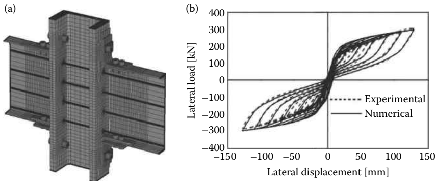
Figure 4.123 Numerical model of the PTED connection with PT-strands and ED-angles: (a) finite element mesh; (b) numerical versus experimental results. (Esposito, M., Faggiano, B., Mazzolani, F.M. 2006a: In Proceedings of 5th International Conference on the Behaviour of Steel Structures in Seismic Areas (STESSA 2006) , Yokohama, Japan, 14–17 August, 299–304.)
