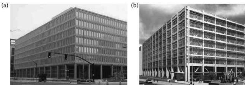
Figure 4.30 Wallace F. Bennett Federal Building (USA): before (a) and after (b) seismic retrofitting.
