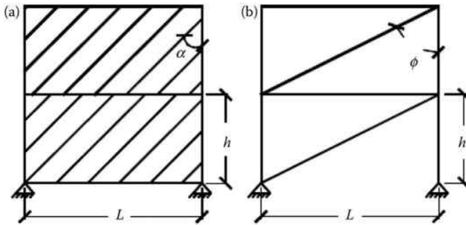
Figure 4.54 Shear panels modeling: (a) strip model and (b) equivalent brace model.
