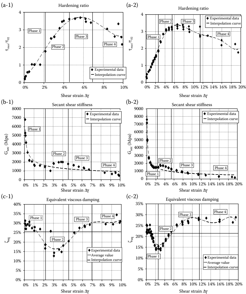
Figure 4.82 Cyclic performance of full bay shear panel type F (a-1, b-1, c-1) and type B (a-2, b-2, c-2).
