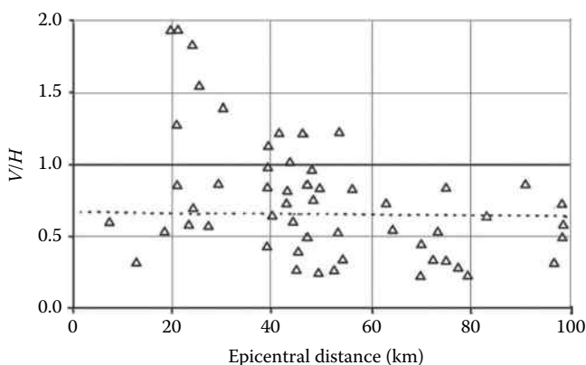
Figure 1.28 Vertical components related to the horizontal ones. (Gioncu, V., Mazzolani, F.M. 2002: Ductility of Seismic Resistant Steel Structures . Spon Press, London; after Elnashai, A.S., Bommer, J.J., Martinez-Pereira, A. 1998: Engineering implication of strong motion records from recent earthquakes. In 11th European Conference on Earthquake Engineering , Paris, September 6–11, No. 59.)
