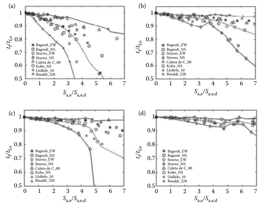
Figure 6.19 Fire resistance rating reductions for steel MR frames subjected to earthquakes. (a) P-ULS frame; (b) P-SLS frame; (c) S-ULS frame; (d) S-SLS frame.
