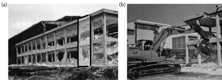
Figure 4.99 The original RC building after the partition removal (a) and subdivision in separate modules (b).
