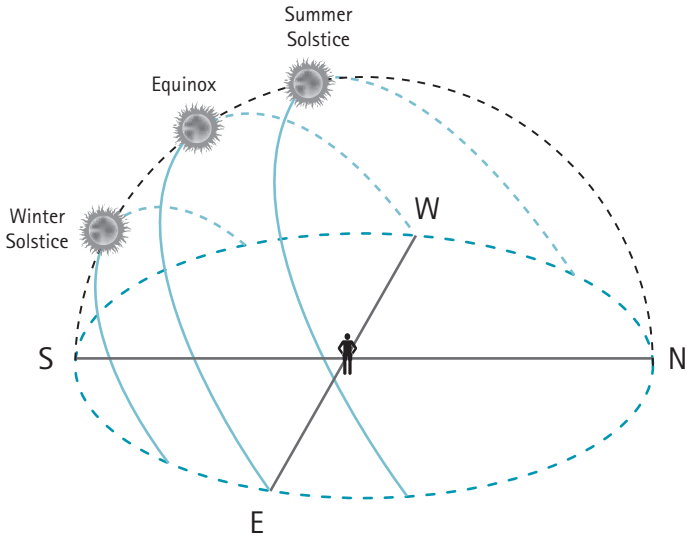
Figure 4.12 The sun paths as viewed from the earth. This is what the sun path looks like in areas that are not in the tropics or the arctic, which is most of the United States and Canada. In the tropics, the sun will be overhead sometimes and in the arctic, it will not rise at the dark of winter.
