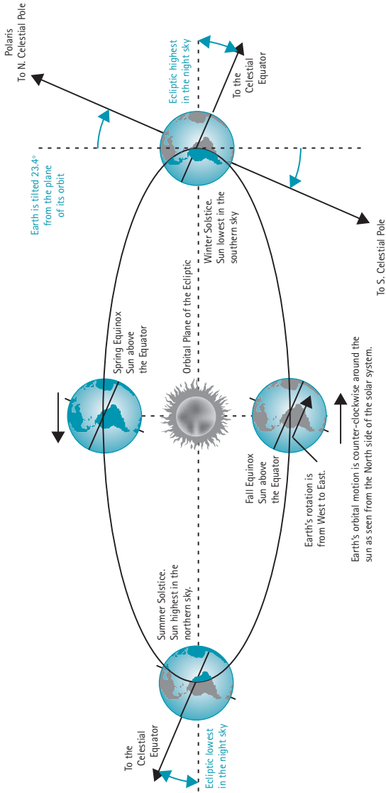
Figure 4.2 Earth's orbit
