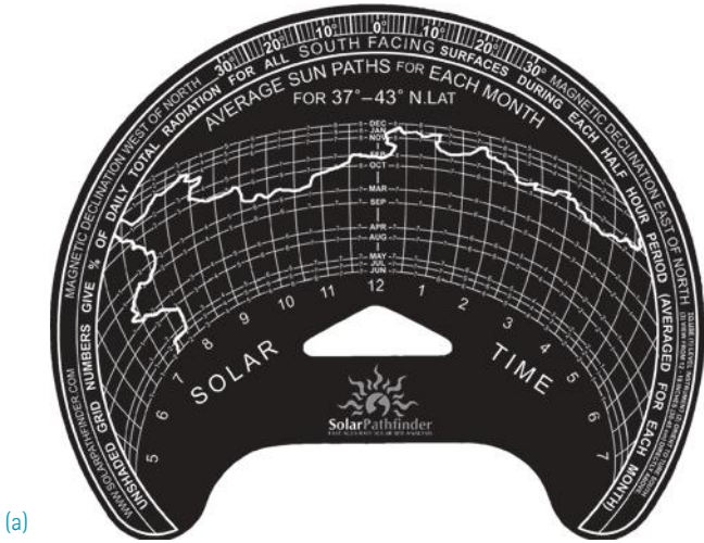
Figure 4.9a and b The Solar Pathfinder is another popular device used to predict shading and the path of the sun throughout the year.
