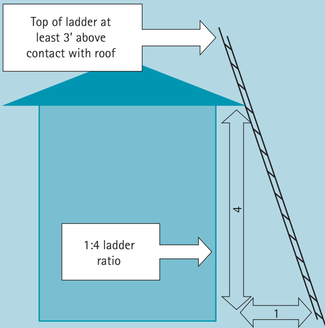
Figure 2.1 1:4 Ladder ratio
