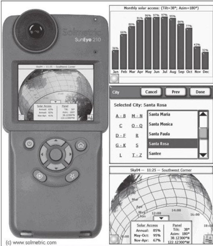
Figure 4.8 The Solmetric Suneye is a popular device used for shade analysis and can predict the path of the sun throughout the year.
