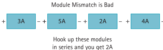
Figure 5.7 Module Mismatch
