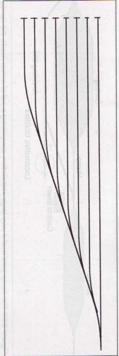
Figure 8/26 Turning now to freight yards, the obvious way to lay out a yard is the ladder track, a single straight lead linking all roads. For up to four tracks of reasonable length this is fine, but when there are, for example, eight tracks as here, the furthest siding is very short.
