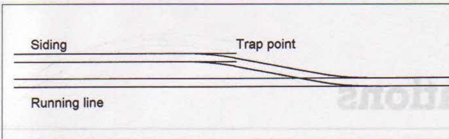
Figure 8/5 Having mentioned trap sidings and sand drags, we can look at trap points. These were no more than a pair of blades, occasionally a single blade, which derailed a train. In the steam age they were lavishly provided to prevent a runaway wagon fouling the running road. They were also fitted at the head of a passing loop on a single-track line to minimise the chances of a head-on collision. They are often miscalled catch points. These are physically similar, but were fitted on steep double track inclines to derail runaway wagons, and were spring-loaded. The virtual elimination of the steam age unbraked, loose-coupled goods train has eliminated the need for this precaution.
