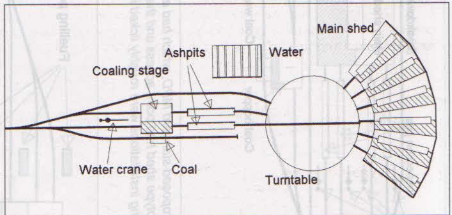
Figure 11/6 Although the true roundhouse shed is rare in Britain, the enclosed rectangular 'roundhouse' shed was fairly common. The design is extremely old; the London & Birmingham shed at Camden, now The Roundhouse, originally had its turntable in the centre of the circular building. However, rectangular sheds were preferred, as the roof is a more straightforward proposition. The layout of this type of shed can be seen at York Railway Museum, which was originally the York MPD; however, the present roof is new. The design does not lend itself to modelling, since it is impossible to see what is going on unless the roof is removed.
