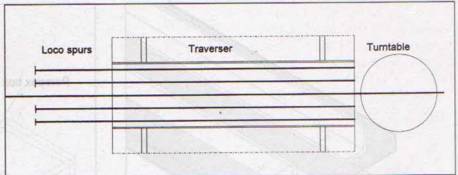
Figure 15/10 The parallel movement of the traverser makes it much easier to connect auxiliary features. In this elaborate arrangement not only is there a turntable for tender locomotives at the far end, but also a series of loco spurs is provided at the other end. This appears something of a complication, but as it gives the fiddle yard operator more to do, it makes the job much less boring.
