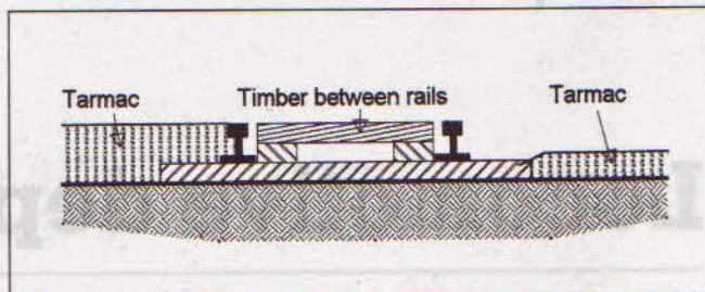
Figure 10/13 Where the road needs to cross the tracks, the tarmac is brought up to rail level, and in most cases timber balks are laid between the rails; occasionally timber is laid outside the rails as well, but there is no hard and fast rule about this.
