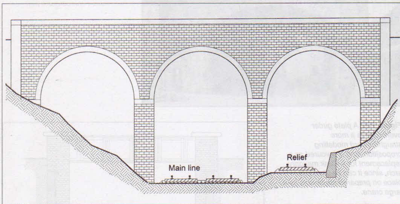
Figure 12/4 Where a road spans a deep cutting, a three-arch bridge was frequently adopted. It had the added advantage that, if extra tracks were needed, they could use the outer spans.
