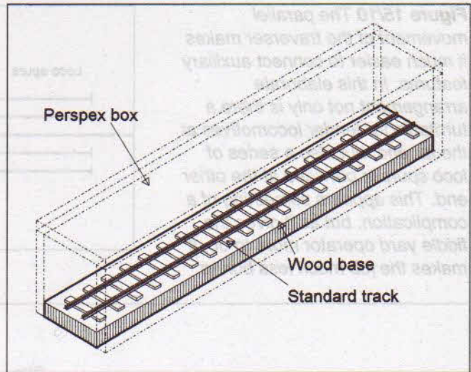
Figure 15/14 A development of the train cassette encases the whole in perspex, with removable ends. Instead of angle, standard track is used and, when not in use, the whole makes a lovely display case.
