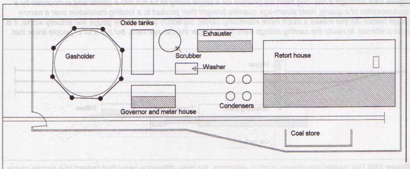
Figure 13/1 A simplified plan for a lineside gasworks, showing the principal parts of the complex. In practice, the retort house, governor house and above all the gasholder – usually miscalled the gasometer – are the essential features. This plan is based on information supplied by Peter Denny, who has no less than three gasworks on his 'Buckingham' layout – one at each station.
