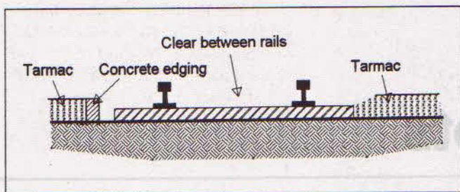
Figure 10/12 Goods yards are always provided with metallised surfaces between the tracks so that carts and lorries can drive alongside the wagons. In the majority of cases this is plain tarmac brought up to the edge of the sleepers; concrete block edging is sometimes provided.
