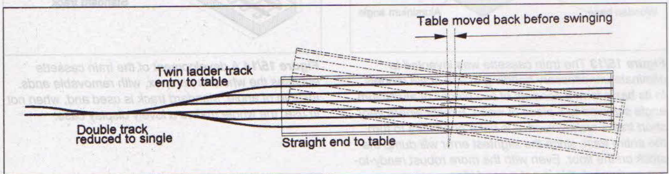
Figure 15/11 The most sophisticated type of train turntable is that devised by Peter Denny. Here the tracks are fed by a fan of points and the table has straight ends. Before turning, the pivot point is wound back, allowing the table to be turned. With a five-track table and a well-planned timetable it is only necessary to make two reversals in a 'day's' operation. The entry points are readily worked by remote control from the main panel or, as with the 'Buckingham' yard, by computer. The electro-mechanical device used at 'Buckingham' just meets this definition, but it is more accurately described as a programme machine, being identical in principle to those used on the London Underground.
