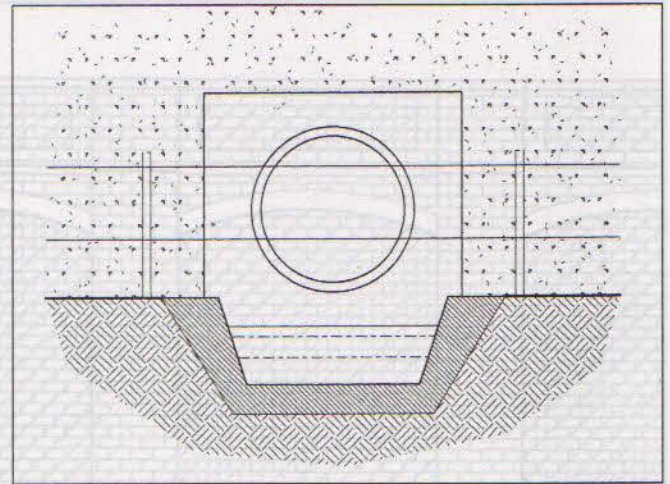
Figure 12/29 Today, culverts are made from pre-cast concrete pipes. These are rarely smaller than 1.5 metres in diameter, so it is possible to crouch and shuffle through to clear obstructions, as culverts are prone to blockage. They are frequently closed with steel grilles, which in turn are often dislodged.
