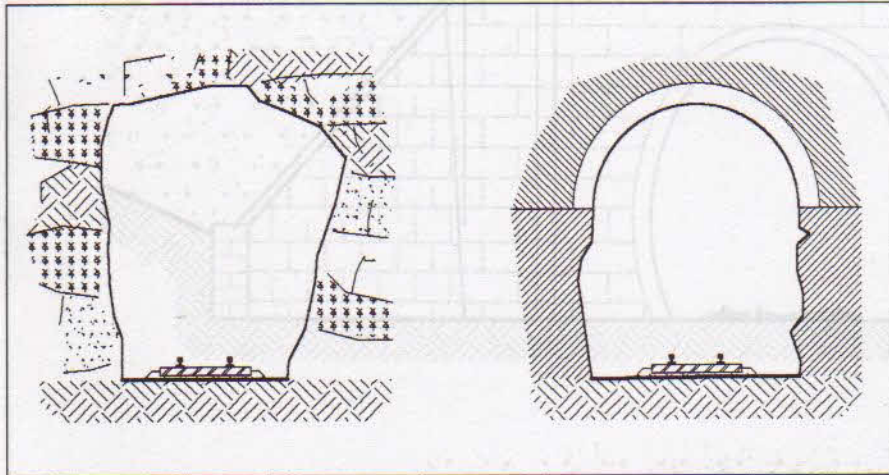
Figure 12/39 Occasionally, where a tunnel was blasted through hard, homogeneous rock, no internal lining was required. This was rare, however; even in firm strata an upper arch was built to secure the roof.
