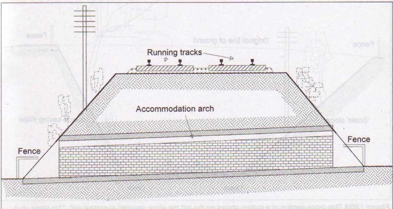
Figure 12/27 Embankments are made from tipped spoil, and are normally much wider than they are high. Again some steepening of the slope is advisable to save width on the model. In this sketch I have shown an accommodation arch passing through the embankment to provide passage for a farmer.
