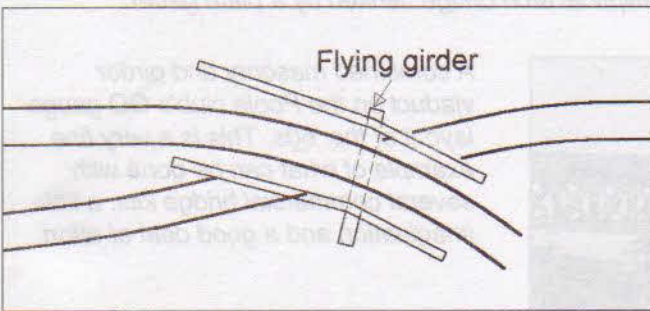
Figure 12/8 Skew bridges are more readily constructed with steel or pre-stressed concrete girders, today the favoured solution. In situations where curved tracks cross one another, more common on the model than on the prototype, a flying girder can be employed. Here the bridge is divided into two or more sections, supported on portal frames spanning the lower track.
