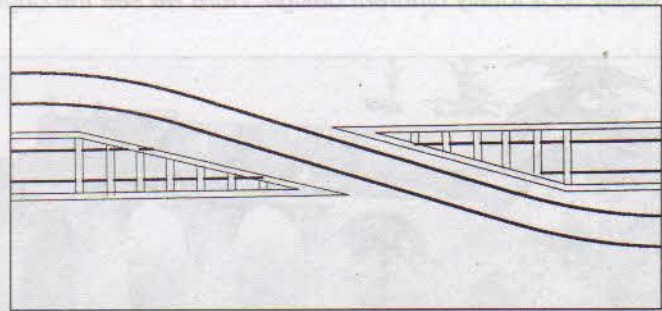
Figure 12/9 Flying junctions frequently cross the lower track at an acute angle. While a single girder could carry the upper roads, it would have to be very deep and correspondingly expensive. An alternative is the gridiron bridge, where the lower track is spanned by a series of short cross girders that support the relatively light girders carrying the upper track. A well-known example is to be found at Farringdon, where the London Underground Circle Line crosses over the Thameslink tracks.
