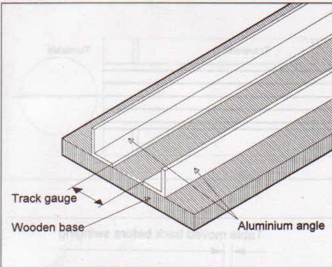
Figure 15/13 The train cassette was invented to eliminate unnecessary handling of fine-scale models. In its basic form it consists of two pieces of aluminium angle screwed to a piece of wood. Except where very short trains are involved, it is not a good idea to turn the entire train, since the slightest error will dump the stock on the floor. Even with the more robust ready-to-run equipment, this is not a good idea.
