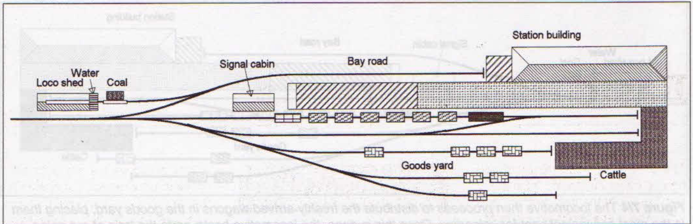
Figure 7/1 Shunting freight traffic: a goods train, headed by a steam or diesel loco and rounded off with the old-pattern brake-van, arrives at the main platform. The locomotive stops with the train between the sets of points so that there is no need to back up before running round.
