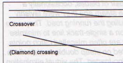
Figure 8/1 There is a considerable degree of confusion between a crossing – or, as it is often called, a diamond crossing – and a crossover. The former passes one track across another, the latter links a pair of parallel tracks.
