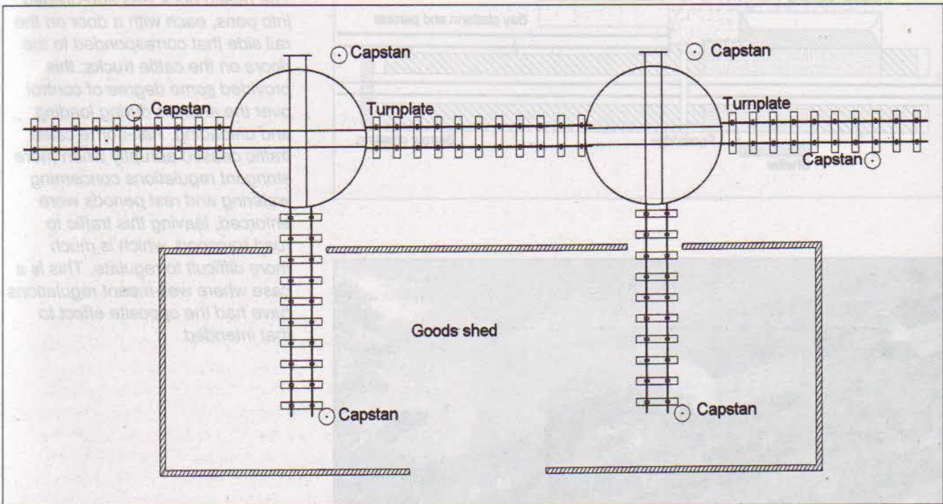
Figure 10/11 The wagon turntable or turnplate was an important feature of early rail layouts, but fell into disuse around the 1890s. However, some remained where space considerations ruled, and there was even a new coal handling yard equipped in this fashion built in the 1950s at St Pancras. The later installations relied on capstan power for shunting, the wagons being moved by ropes passed round vertical revolving spindles. Modern safety regulations would rule this out.
