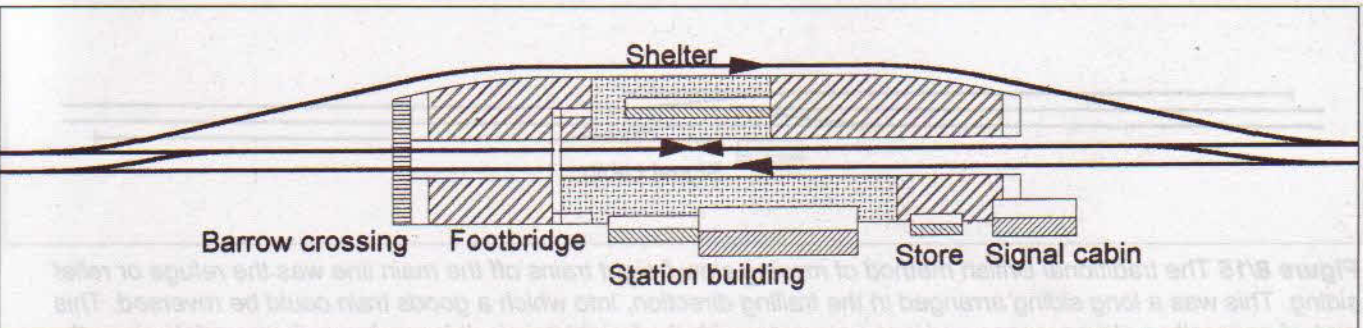
Figure 8/18 While this looks similar to Figure 8/17, here the centre road is the reversible one. It is of greatest value on a large system layout where it provides reversal for suburban services, although it has advantages on a simple continuous system. It is very rare on the prototype.
