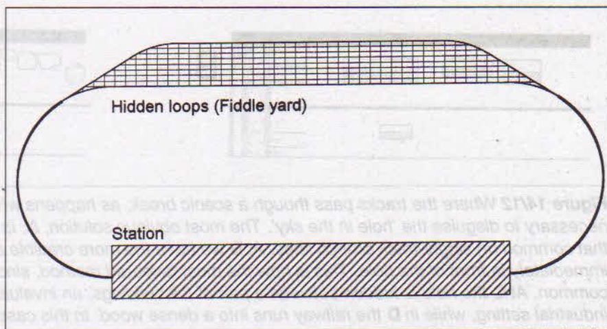
Figure 15/1 The least complicated type of fiddle yard is where hidden loops allow a succession of trains to be brought out to parade through the visible through station. This is the same arrangement as the American staging track.
