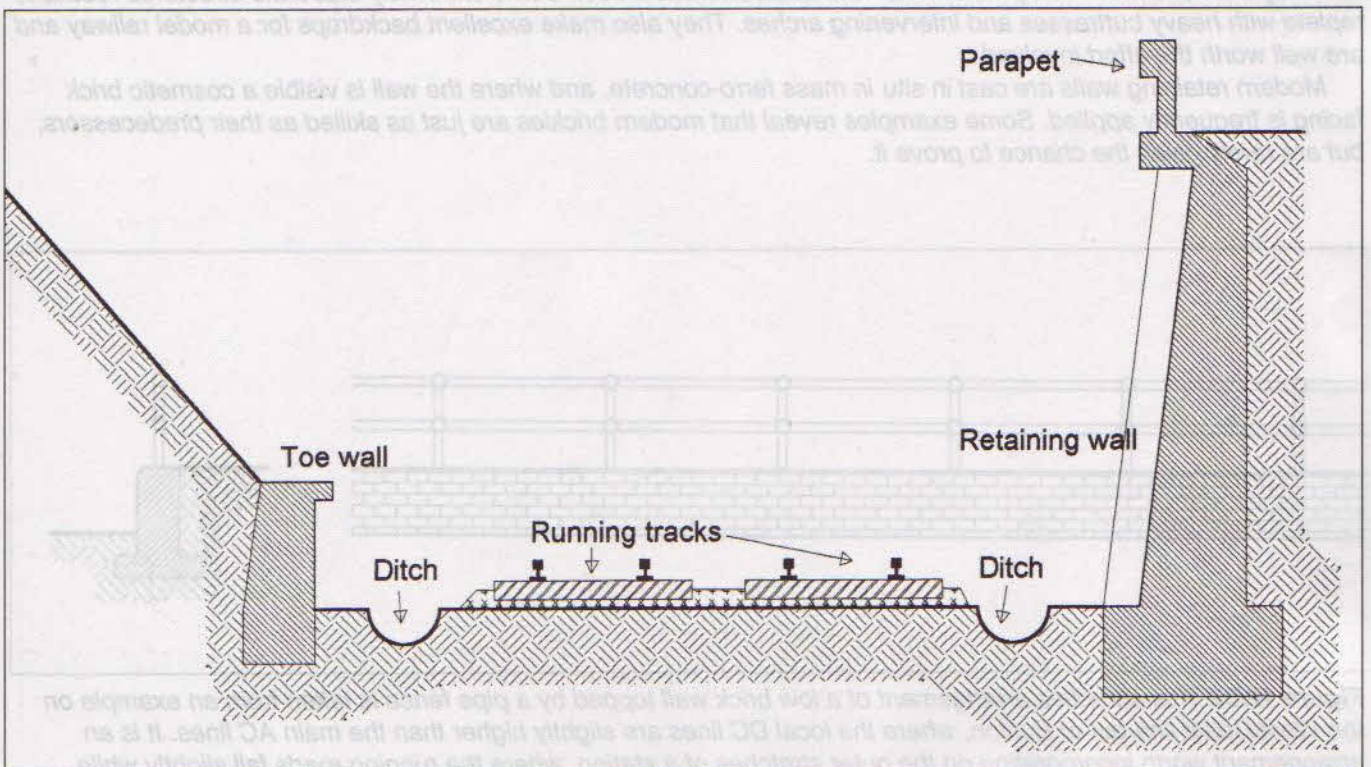
Figure 12/30 Retaining walls are more common on model railways than they are on the prototype, where cost considerations restrict their use to urban areas. The smaller toe wall is usually employed to widen an existing cutting, but has also been used when the angle of rest for the soil turns out to be shallower than first expected. The toe wall then reduces the risk of a landslip blocking the tracks.
