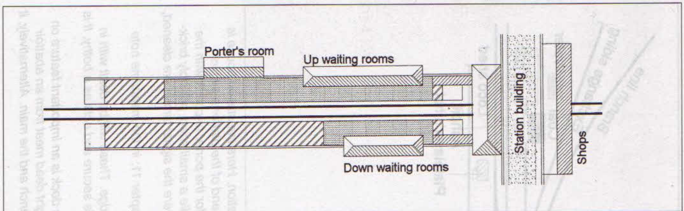
Figure 9/5 A more common type of suburban halt is shown here. Once again the booking office is situated on a road bridge, but with flanking platforms, stairway access is supplied. Furthermore, the up platform has a larger awning and waiting room, while the down platform is more spartan. The reason for this disparity is that the commuters join up trains, and therefore this platform is well loaded with people who have either arrived in good time, or cut things too fine and have seen their train leave as they pass through the barrier in the booking office. On the return journey, no one lingers around the station.
