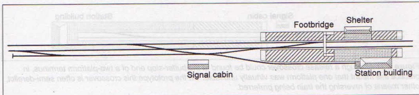
Figure 8/19 A more conventional means of reversing a passenger service at a through station is to run the trains into a bay platform. Here the bay is combined with a loop that also serves the goods yard. Facing entries to both the bay and loop are provided to ease model operation; despite a common belief that facing entries to goods facilities were outlawed, they did occur where traffic on the main line was at all intensive.
