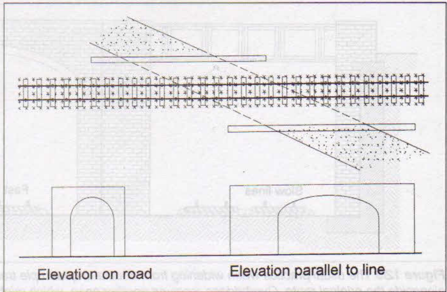
Figure 12/7 The skew masonry bridge is one of the more complex of civil engineering structures, since the arch courses are arranged as a spiral. Thankfully, none of this affects the modelmaker. The point to bear in mind is that although the side elevation shows an elliptical arch, when viewed along the bore the cross-section is a semi-circle.
