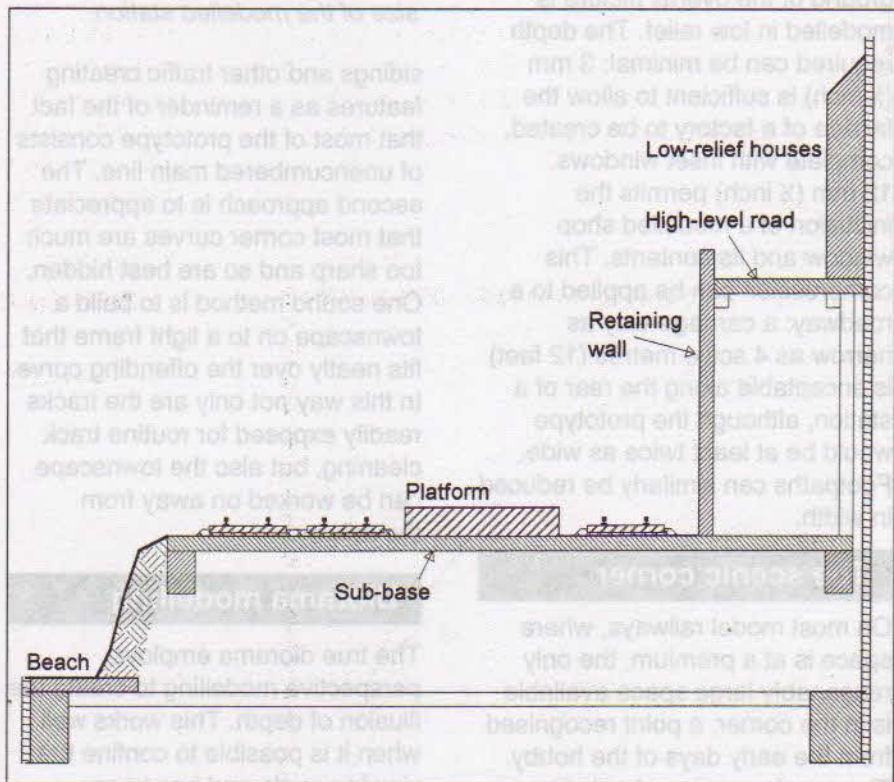
Figure 14/2 It is a good idea to raise the rear scenic features above track level so that the low-relief buildings are not masked by the trains. This is very important where these models are highly detailed – never hide a good model. Likewise, the foreground interest is best brought below track level. Here I've suggested a beach, complete with bathing figures. Lest anyone feels I have introduced an air of fantasy, this arrangement is based on the layout at St Ives, Cornwall.
