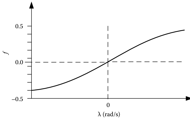
FIGURE 19.14 Relation between \lambda and f for bilinear transformation.
