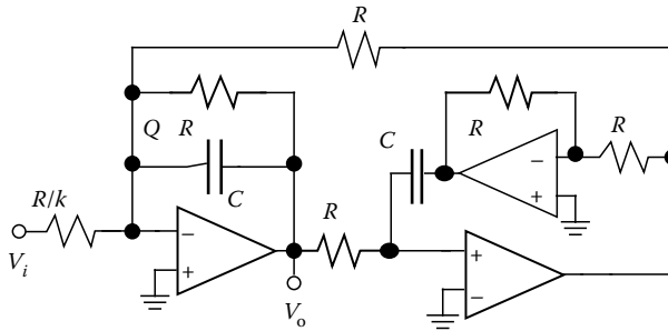
FIGURE 15.2 Åkerberg–Mossberg bandpass circuit.
