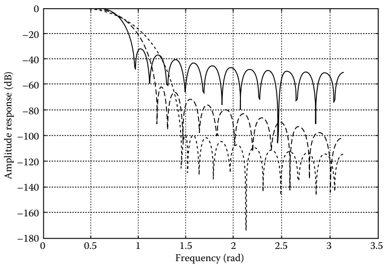
FIGURE 18.14 Magnitude responses of low-pass FIR filter design using a 31-point Kaiser window with \beta = 1 (solid line), \beta = 6 (dash line), and \beta = 10 (dotted line).
