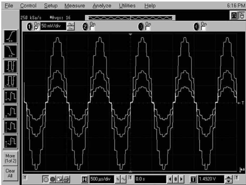
FIGURE 17.31 Measured output signal of the sinewave generator.
