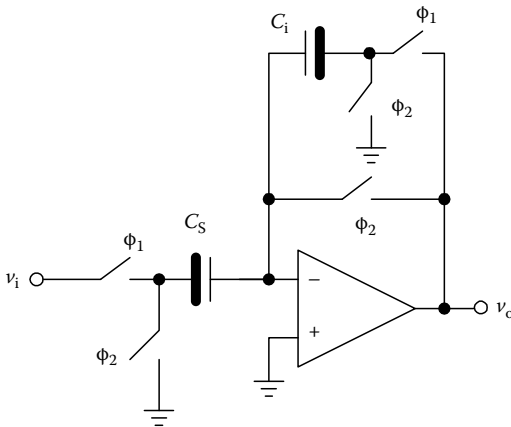
FIGURE 17.2 Voltage amplifier available during the \phi_1 clock phase.
