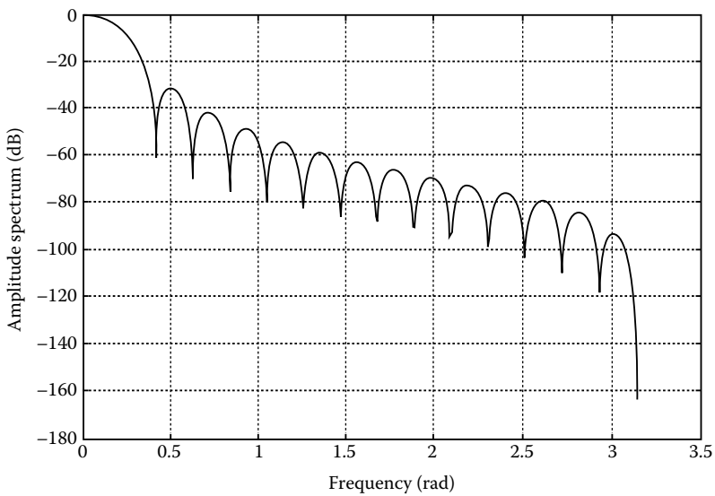
FIGURE 18.8 Fourier transform of the Hanning window.
