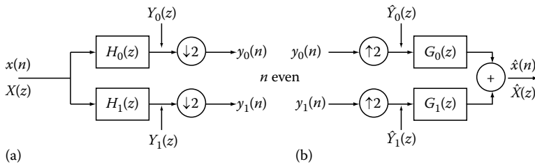
FIGURE 24.1 Two-band filter banks for analysis (a) and reconstruction (b).
