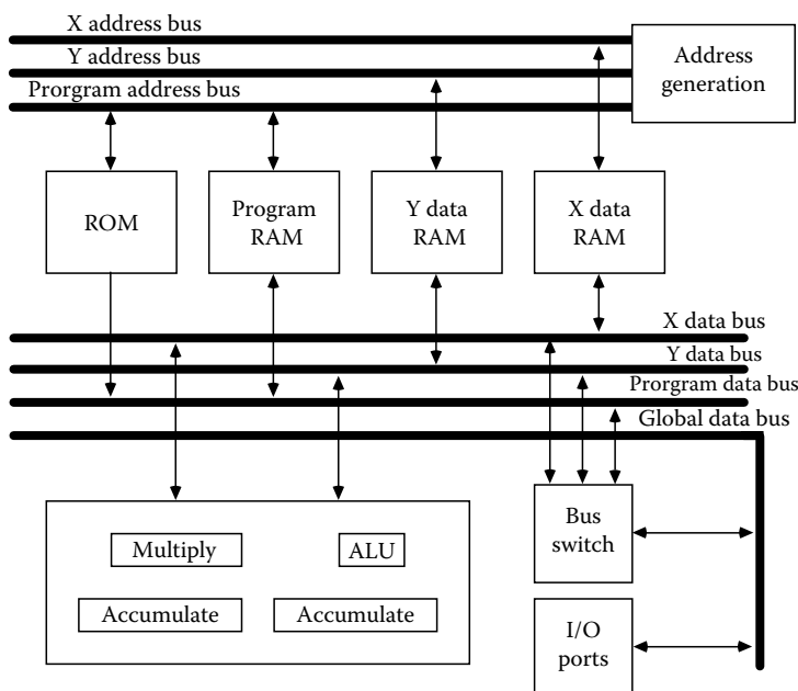
FIGURE 21.4 Motorola 56001 architecture.
