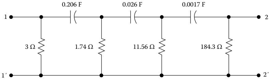
FIGURE 8.17 \alpha -Ladder.
