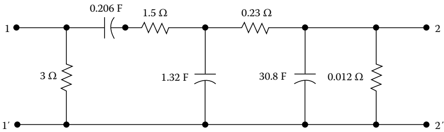
FIGURE 8.18 \beta -Ladder.
