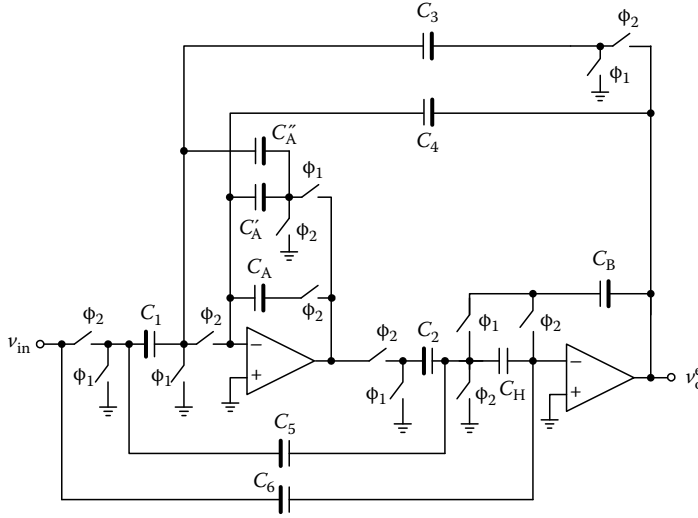
FIGURE 17.9 An improved capacitance area SC biquadratic section.
