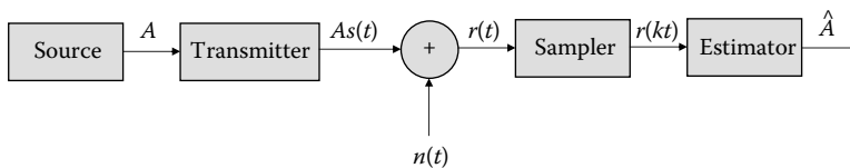
FIGURE 26.11 Baseband communication model: s(t) denotes the combined impulse response of the transmitter and the channel, and As(t) is corrupted by additive white noise n(t) .
