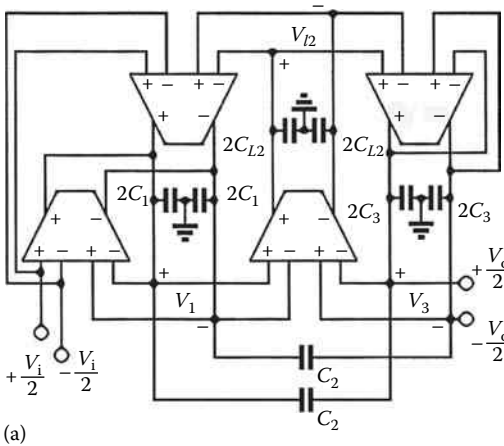
FIGURE 16.30 (a) SFG g_m -C third-order elliptic low-pass filter; (b) experimental performance in 2- \mu m CMOS technology.
