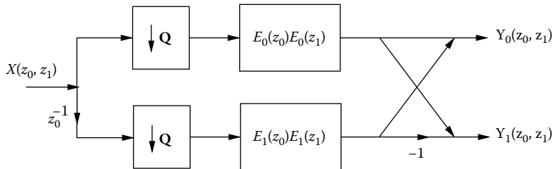
FIGURE 25.11 Efficient polyphase domain implementation of diamond filter bank. The filtering operations are separable.
