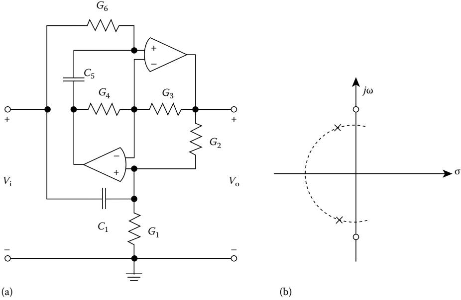
FIGURE 13.20 Second-order Cauer low-pass building block. (a) The circuitry. (b) The pole and zero locations.
