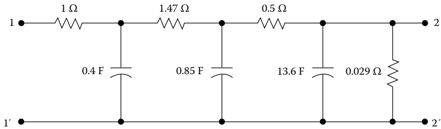
FIGURE 8.19 \gamma -Ladder.
