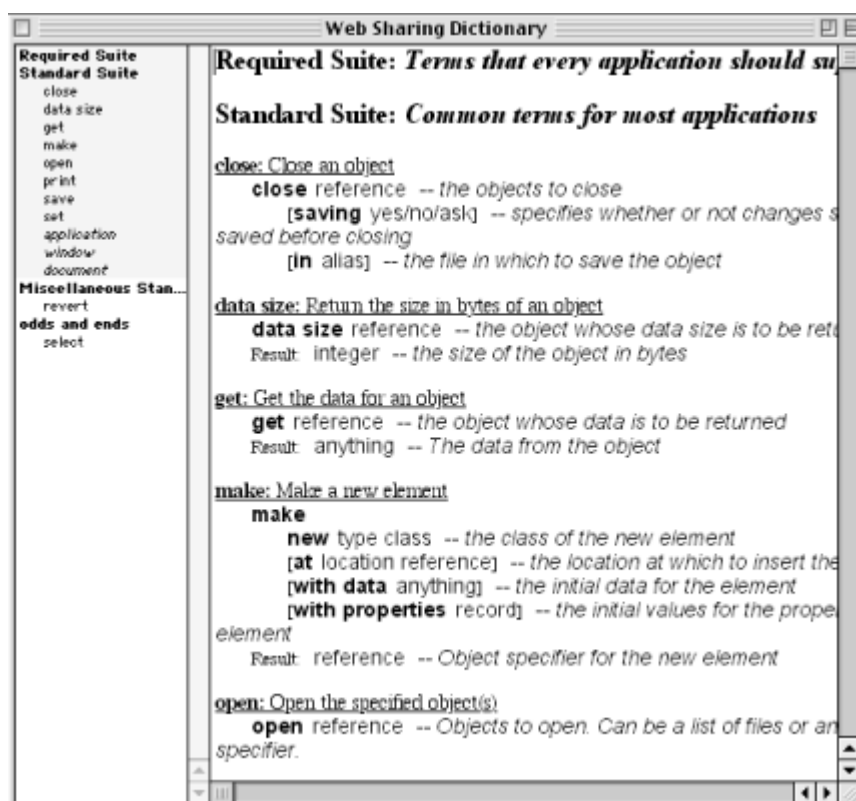
Figure 31-3. Web Sharing control panel's dictionary
