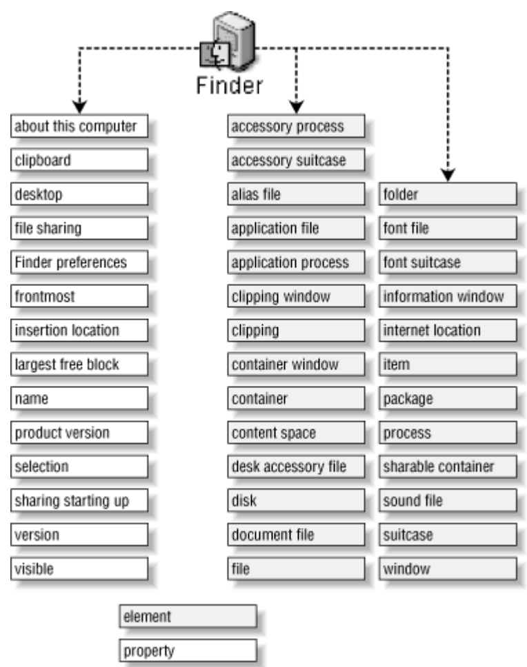
Figure 15-1. Finder's object model
