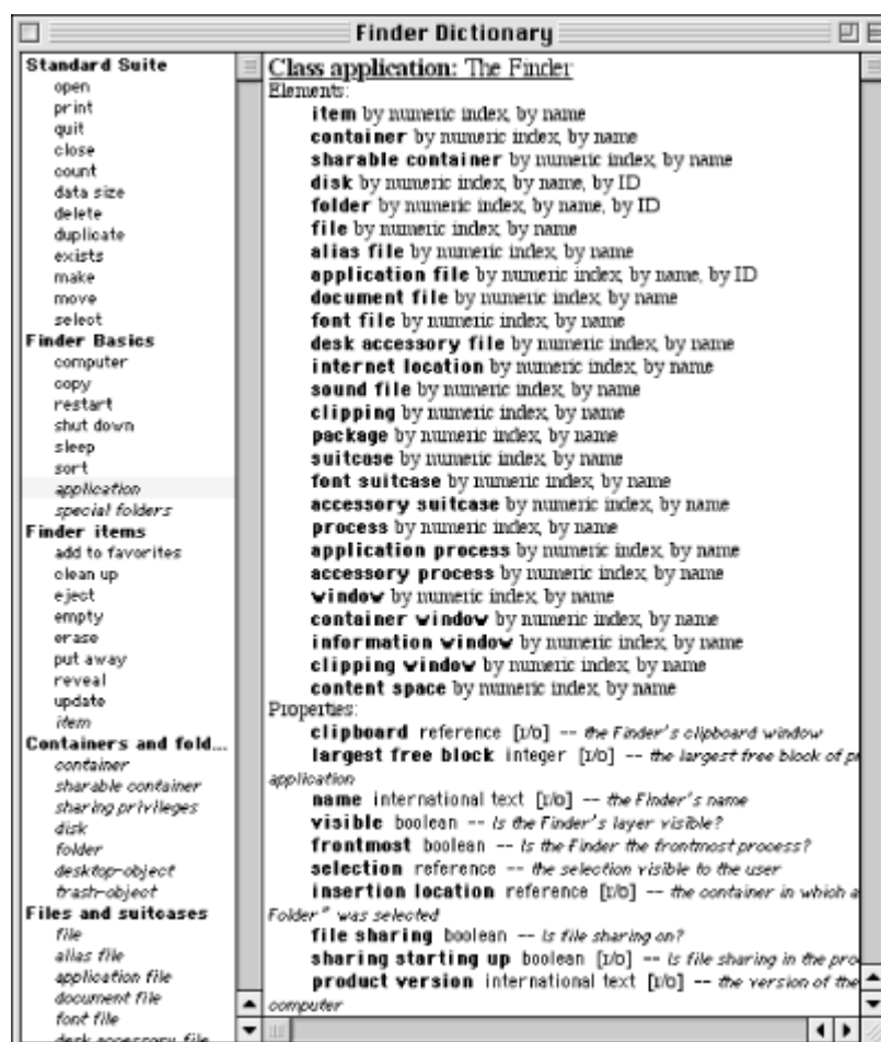
Figure 14-2. Finder dictionary window
