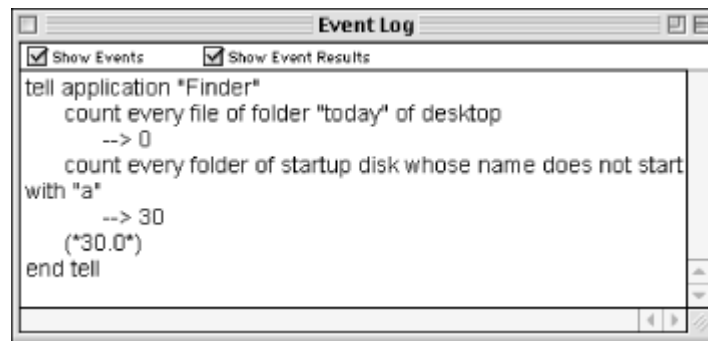
Figure 2-8. Event Log window
