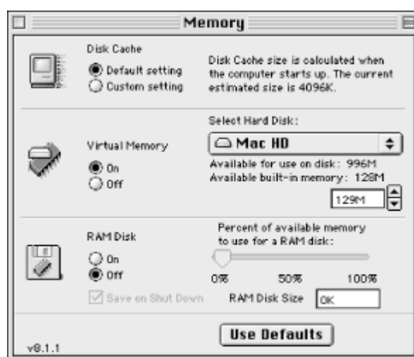
Figure 29-1. The Memory control panel
