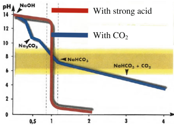
Fig. 7 Neutralization of basic solution via CO 2 compared to strong acid (Source AIR LIQUIDE)
