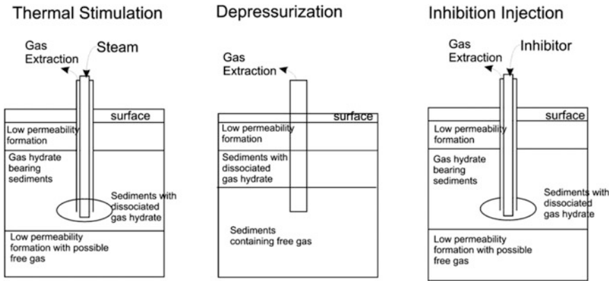
Fig. 9 Methods for methane from hydrates extraction (adapted from Ruppel 2007)
