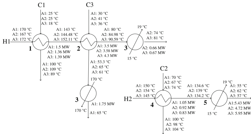
Fig. 8 Heat exchanger network design for plant A (modified from Čuček and Kravanja 2015a)
