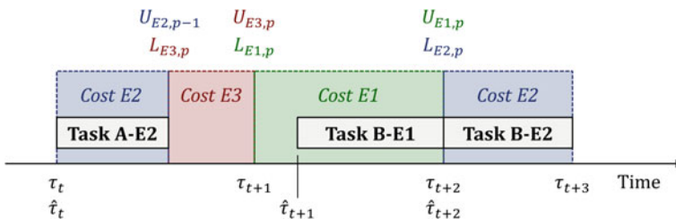
Fig. 3 Illustration of continuous time representation with timing constraints (Castro et al. 2009)
