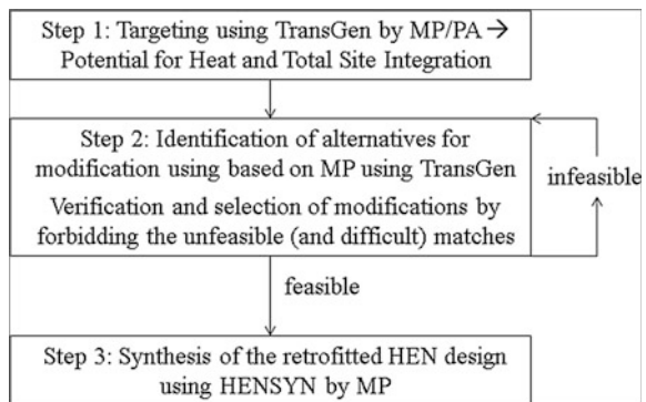
Fig. 6 Procedure for retrofitting of Total Sites using TransGen and HENSYN (modified from Čuček et al. 2015b)
