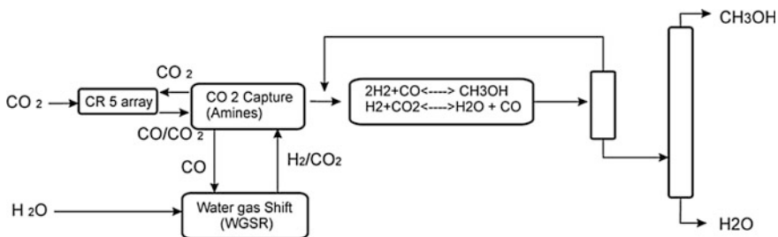
Fig. 18 Methanol production from water and CO_2
