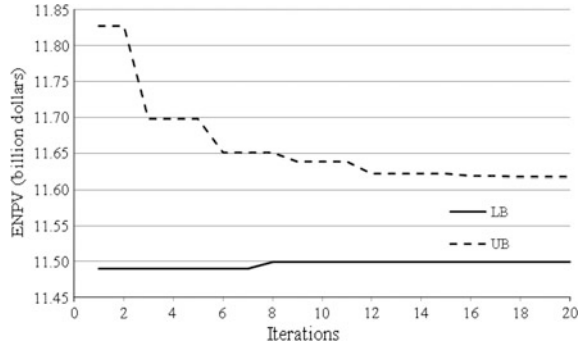
Fig. 27 Standard Lagrangian decomposition results for 3 oilfield example (Instance 3)
