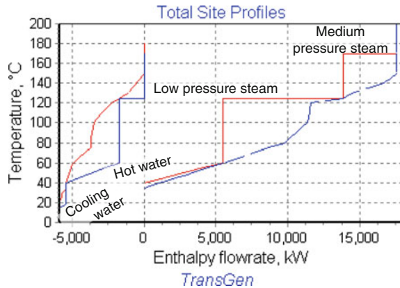
Fig. 3 Total Site Profiles with levels of intermediate utilities (modified from Čuček and Kravanja 2014)
