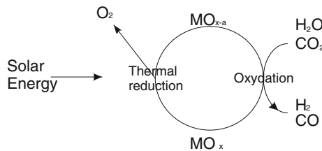
Fig. 17 CO_2 decomposition cycle
