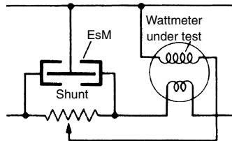
Figure 18.13 Electrostatic wattmeter used for calibration purposes
