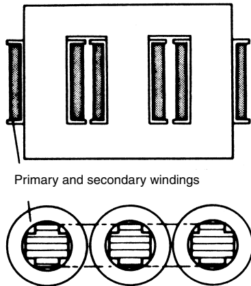
Figure 10.4 Core-type 3-phase transformer
