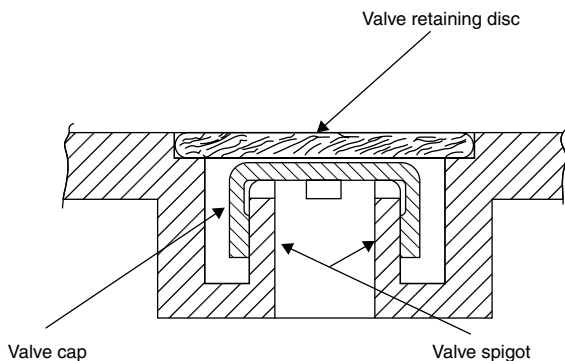
Figure 21.2 Valve assembly
