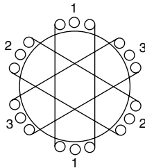
Figure 14.8 Three-phase stator winding to produce rotating field
