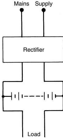
Figure 13.7 Circuit for a single floating battery system
