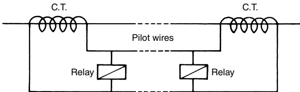
Figure 15.12 Balanced current system
