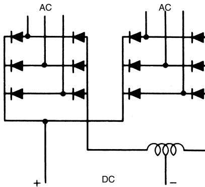
Figure 5.4 Transformer 12-pulse circuit for 2-wire d.c. output from parallel bridges with inter-circuit reactor
