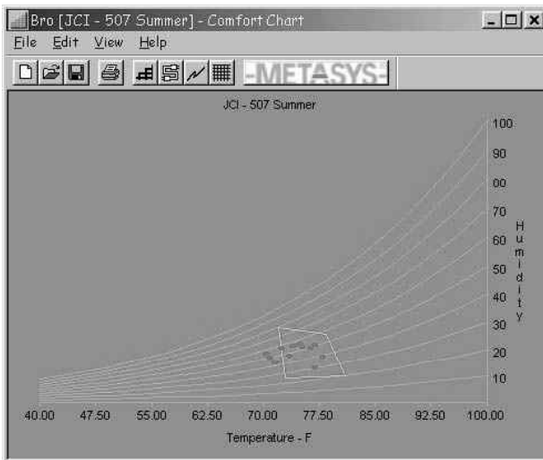
Figure 17.5 Comfort chart
