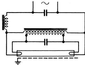
Figure 13.4 Quickstart circuit for single-lamp operation
