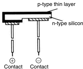
Figure 4.25 Photain photovoltaic cell
