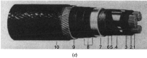
Figure 9.1c Three-core 11 kV 150 mm 2 lead sheathed screened cable; single wire armoured and served.
