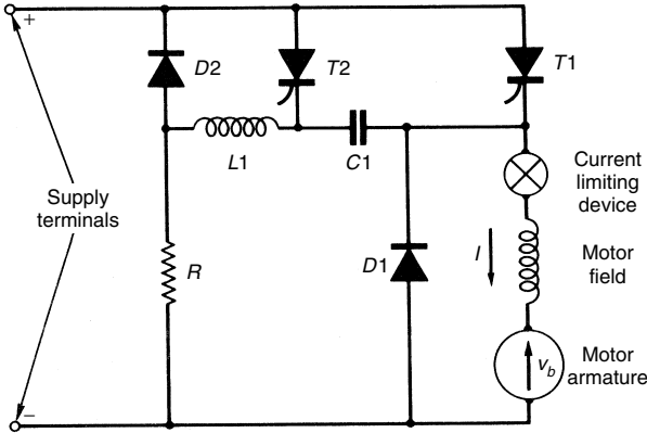
Figure 4.13 Basic circuit
