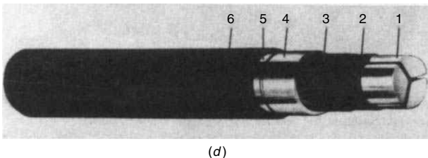
Figure 9.1d Typical Consac cable for use in low voltage PME systems.
