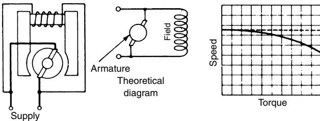
Figure 14.2 Shunt-wound motor
