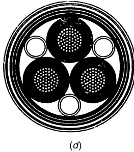
Figure 9.2d 3-core ducted type served cable. By courtesy of Pirelli Cables Ltd
