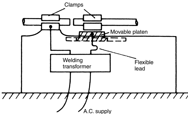
Figure 19.6 Basic arrangement for flash welding
