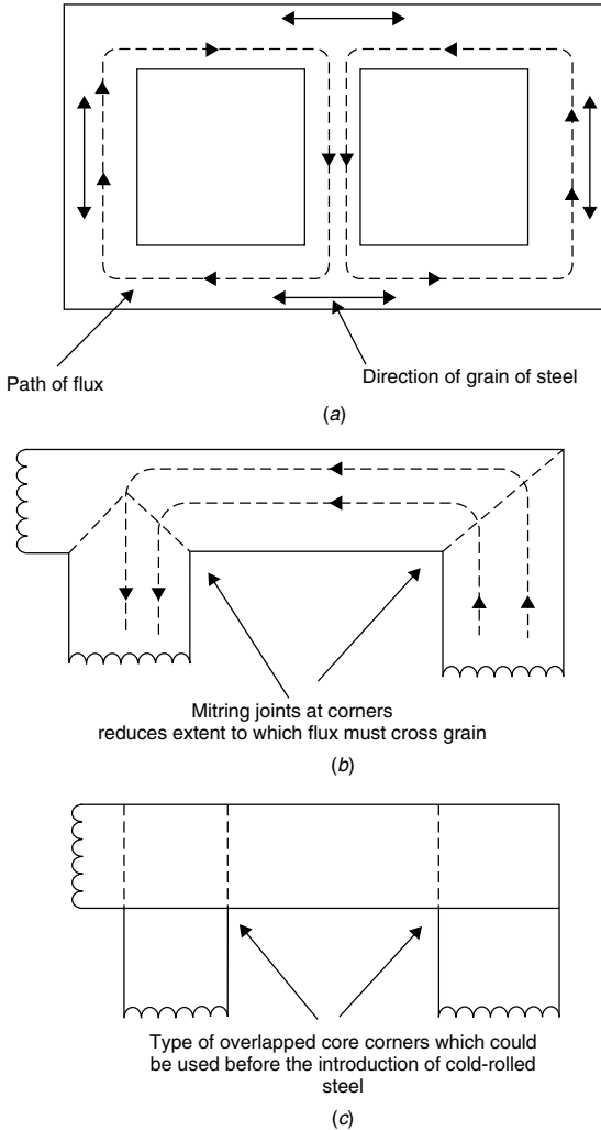
Figure 2.2 Mitring joints at intersection of limbs and yokes reduces extent of flux crossing grain orientation
