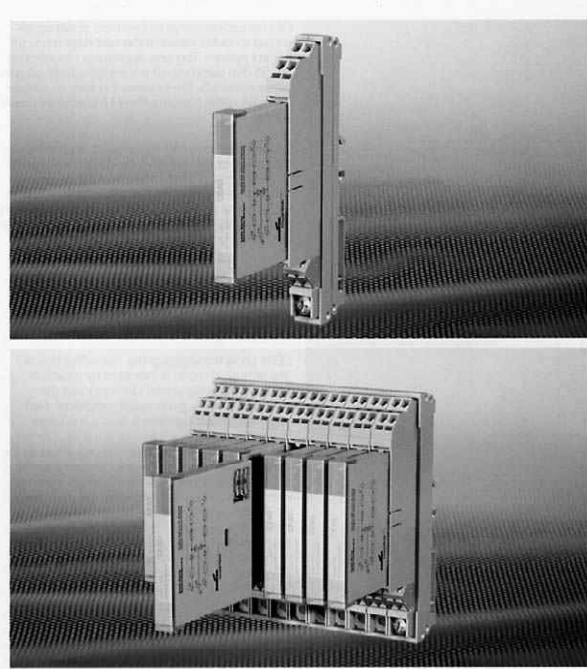
Figure 23.11 The 'intrinsically safe engineering system' – a rack to accommodate various galvanically isolated IS interface cards for control and instrumentation circuits (CEAG Crouse Hinds)
