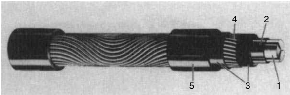
Figure 9.1g Typical Waveconal cable as used in low voltage p.m.e. systems.
