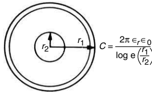
Figure 1.3 Concentric capacitor
