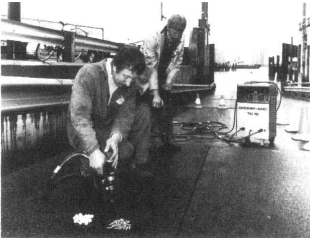
Figure 19.4 A Crompt-Arc TC12 electronic welding system being used to install a new anti-skid surface at a ferry terminal (Crompton Parkinson)
