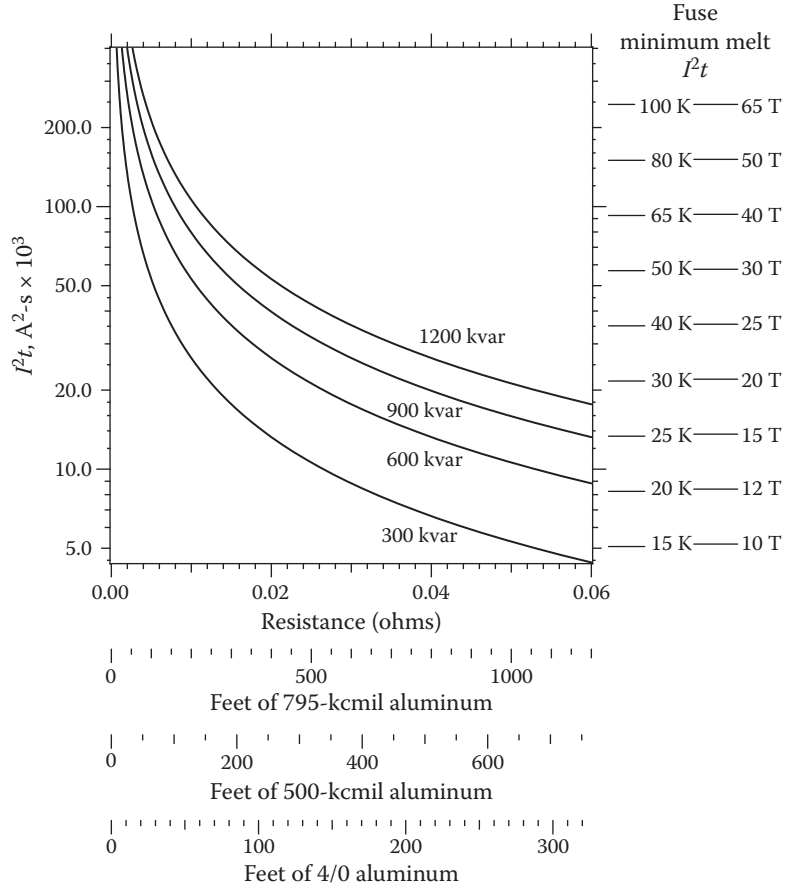
Figure 7.19 Outrush as a function of the resistance to the fault for various size capacitor banks (the sizes given are three-phase kvar; the resistance is the resistance around the loop, out and back; the distances are to the fault).
