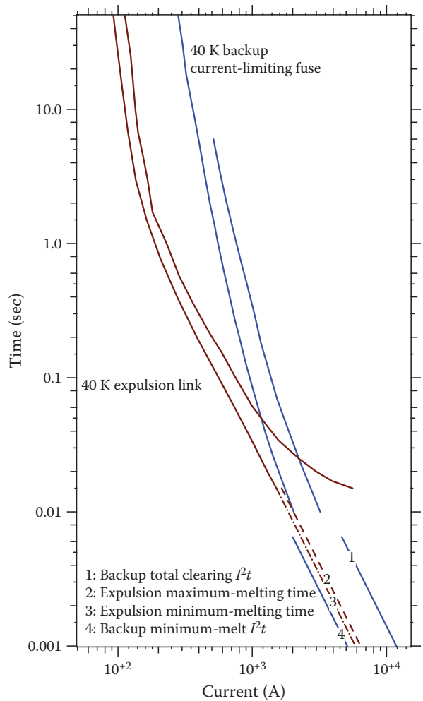
Figure 9.13 Coordination between a 40-K expulsion link and a 40-K backup current-limiting fuse using the relaxed matched-melt criteria.
