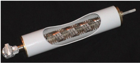
Figure 9.10 Example backup current-limiting fuse. (From Hi-Tech Fuses, Inc. With permission.)
