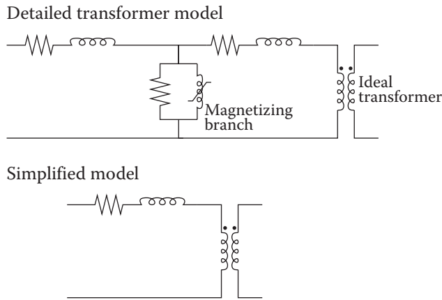
Figure 5.2 Transformer models.
