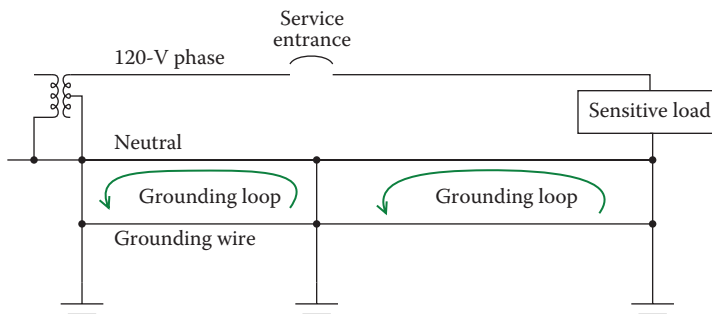
Figure 12.4 Ground loops within a facility.
