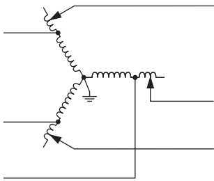
Open-delta connection
