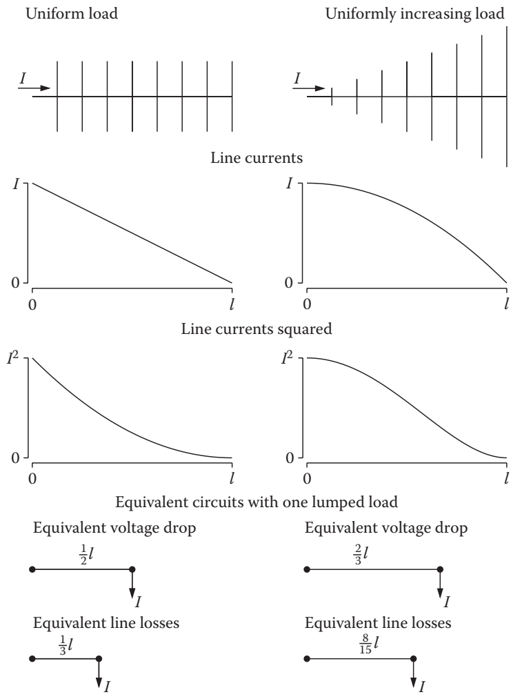
Figure 6.9 Equivalent circuits of uniform loads.
