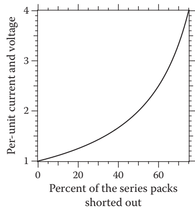
Figure 7.16 Per-unit current drawn by a failing bank depending on the portion of the bank that is failing (assuming an infinite bus). This is also the per-unit voltage applied on the series sections still remaining.
