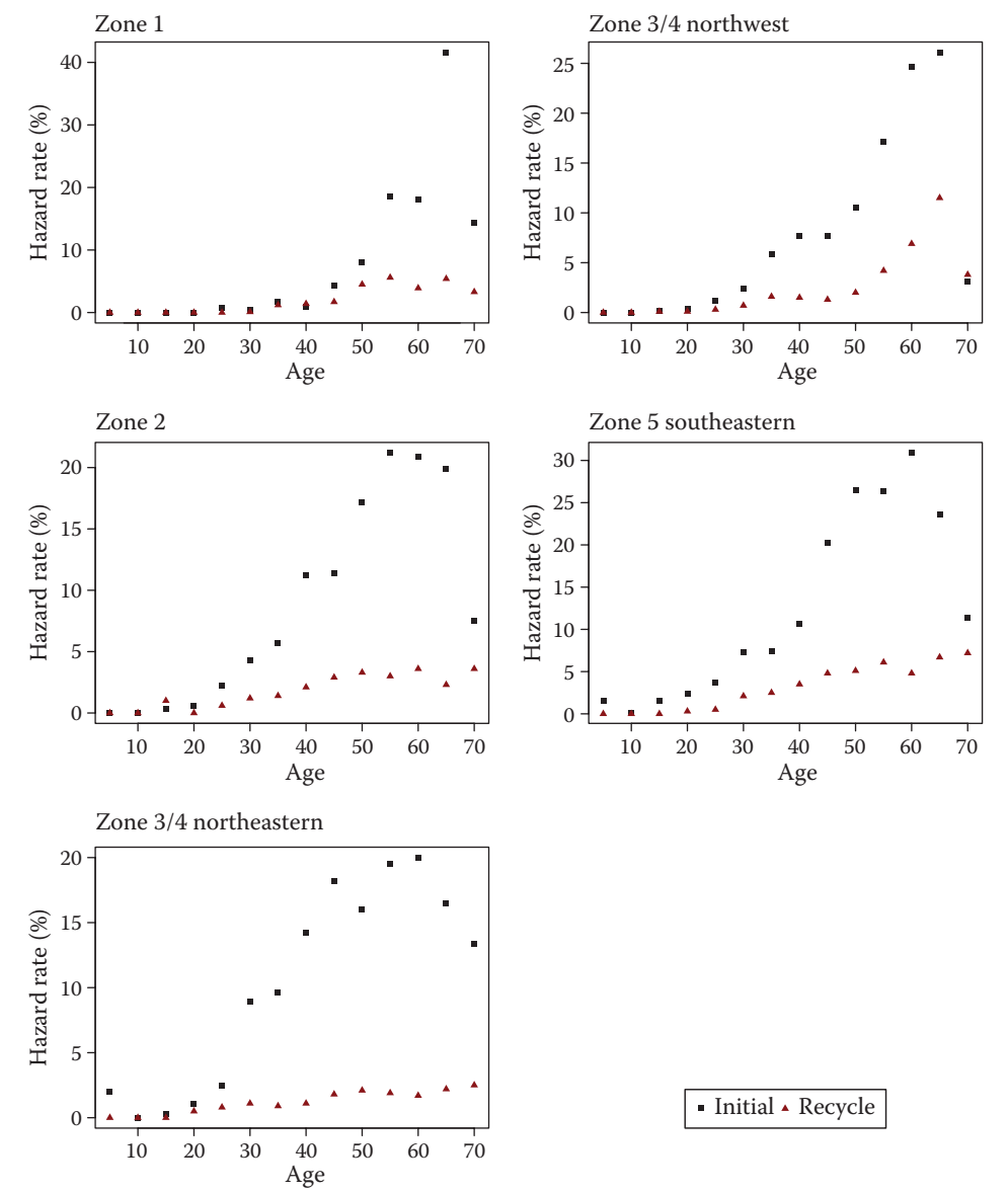
Figure 3.27 Pole inspection rejection rates as a function of pole age. (From EPRI 1012500, Guidelines for Intelligent Asset Replacement: Volume 4: Wood Poles (Expanded Edition) , Electric Power Research Institute, Palo Alto, CA, 2006. Copyright 2006. Reprinted with permission.)
