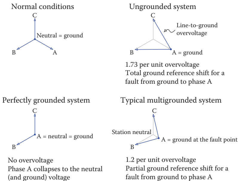
Figure 14.3 Ground potential shifts and overvoltages depending on the grounding configuration.
