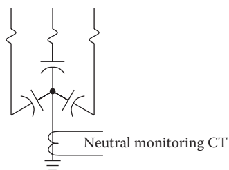
Figure 7.26 Neutral monitoring of a capacitor bank.
