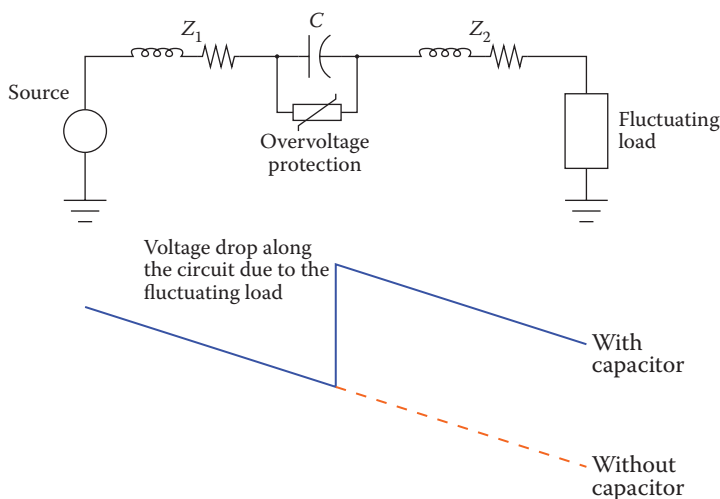
Figure 12.26 Series capacitor.
