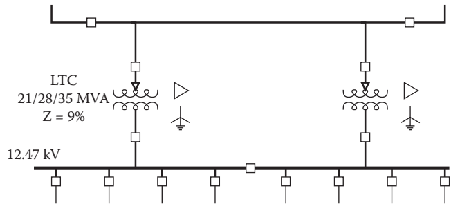
Figure 1.13 Example of a suburban distribution substation.
