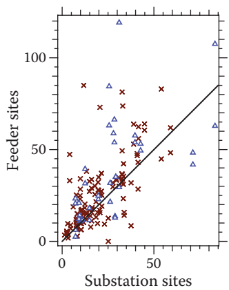
Figure 11.16 SARFI ITIC at substation sites plotted against SARFI ITIC at that substation's feeder sites (triangles indicate rural sites).
