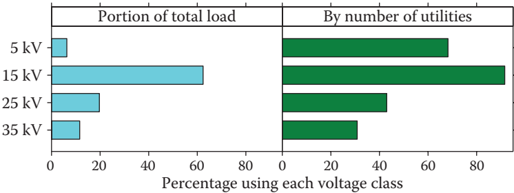
Figure 1.11 Usage of different distribution voltage classes ( n = 107 ). (Data from IEEE Working Group on Distribution Protection, Distribution line protection practices industry survey results, IEEE Transactions on Power Delivery , vol. 10, no. 1, pp. 176–86, January 1995.)
