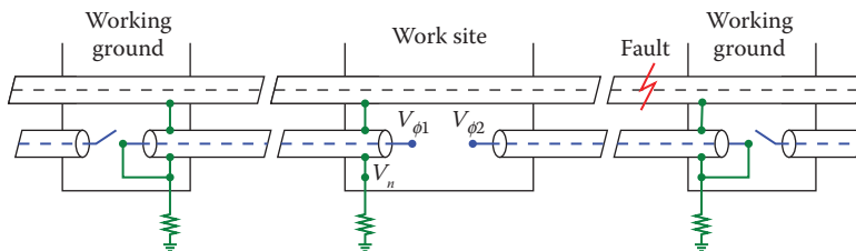
Figure 14.31 An underground cable under repair with a fault on an adjacent cable. (Adapted from Rajotte, Y. et al., IEEE Transactions on Power Delivery , vol. 5, no. 2, pp. 1026–1033, April 1990. Copyright 1990 IEEE. With permission.)
