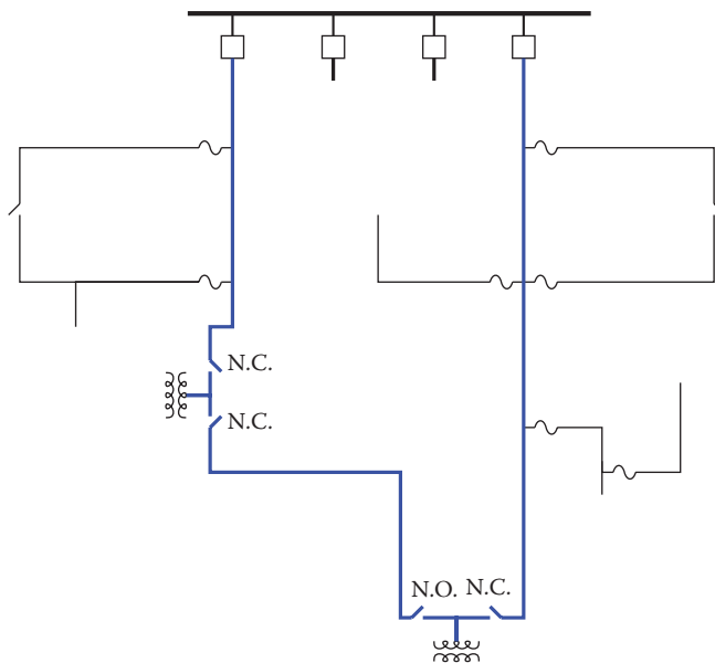
Figure 1.6 Primary-loop distribution arrangement. (From EPRI 1000419, Engineering Guide for Integration of Distributed Generation and Storage into Power Distribution Systems , Electric Power Research Institute, Palo Alto, CA, 2000. Copyright 2000. Reprinted with permission.)
