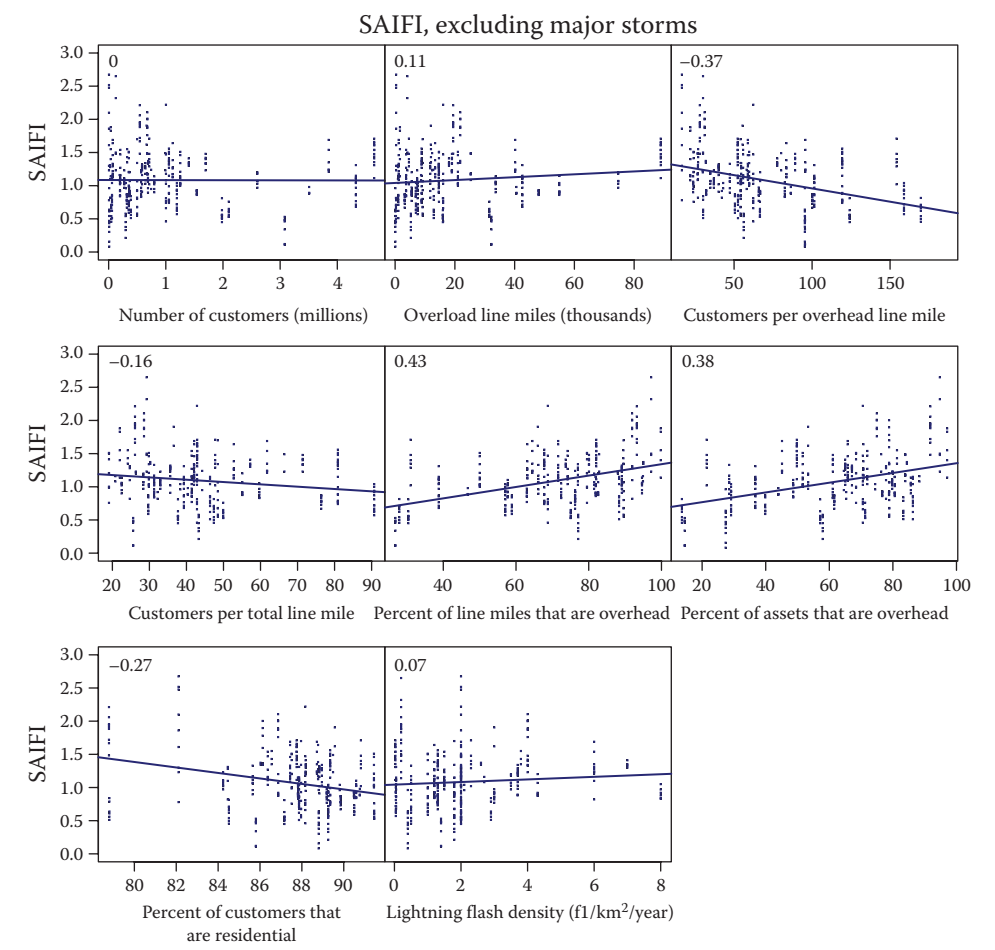
Figure 10.18 Variables impacting SAIFI. (From EPRI 1010658, Distribution Reliability Trends and Correlations , Electric Power Research Institute, Palo Alto, CA, 2005. Copyright 2005. Reprinted with permission.)
