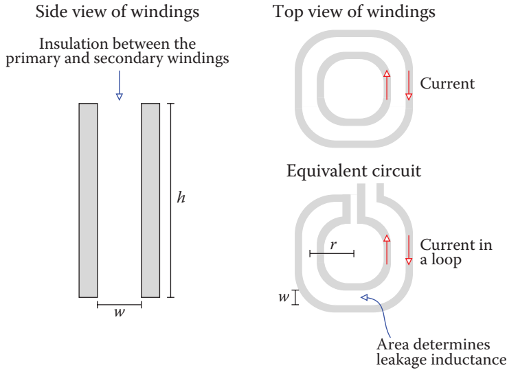
Figure 5.3 Leakage reactance.
