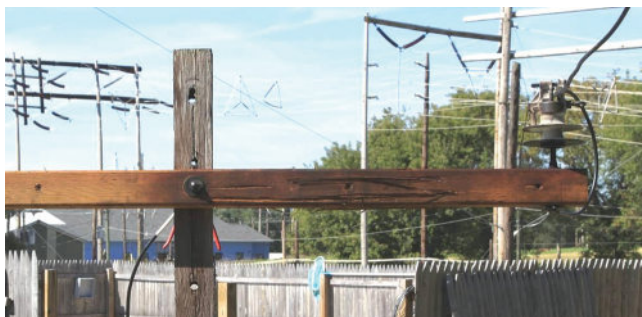
Figure 13.34 Near-surface damage from impulses. (From EPRI 1021995, Distribution Composite Crossarm Laboratory Testing , Electric Power Research Institute, Palo Alto, CA, 2011. Copyright © 2011. Reprinted with permission.)
