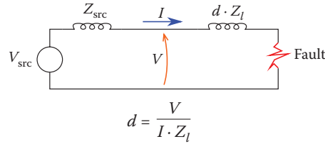
Figure 8.20 Fault location calculations.
