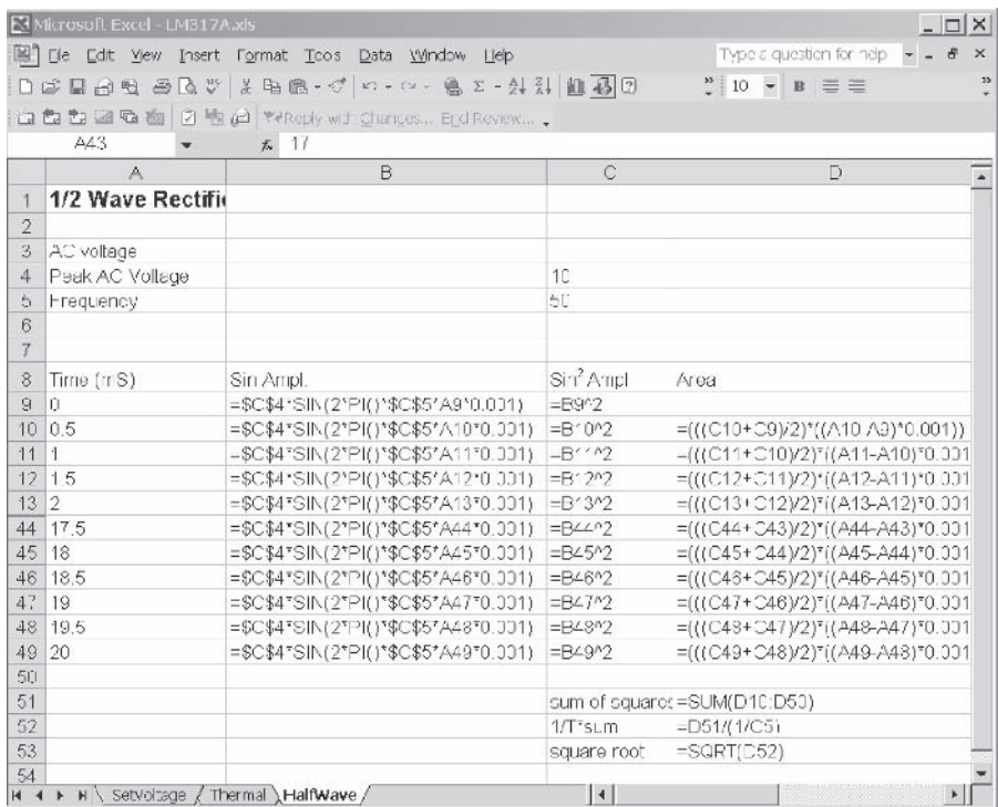
Figure 10-21: Formulas to calculate the RMS value of a sine wave. Note that the worksheet has been renamed.
