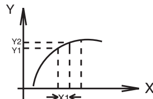
Figure 10-20: Trapezium method of calculating the area under a curve.
