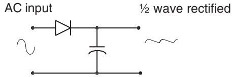
Figure 10-19: Half-wave rectification circuit.
