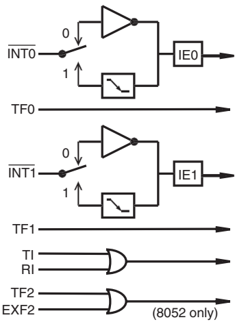
Figure 6-34: Interrupt configuration.
