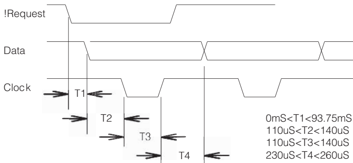
Figure 15-4: Caliper timing diagram. Note that if !Request is kept low continuously the sequence is repeated about every 90 mS. !Request can be taken high at anytime before the start of the next sequence to prevent a new transmission.
