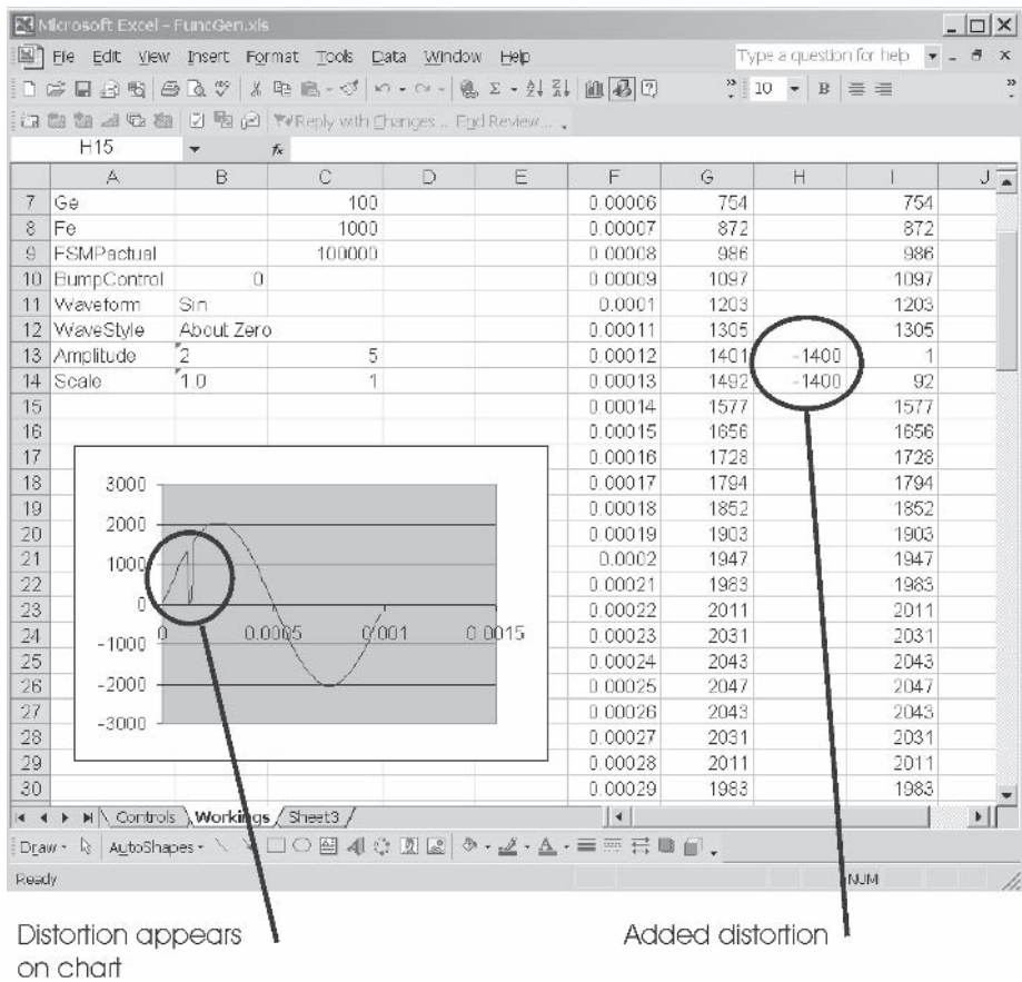
Figure 16-12: Dynamic chart on the Workings sheet. Note that I have added two entries in cells H13 and H14 to distort the waveform and to see the immediate effect on the chart.
