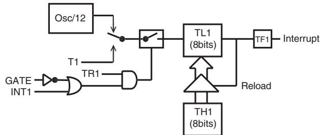
Figure 6-28: Timer/Counter 1, Mode 2.
