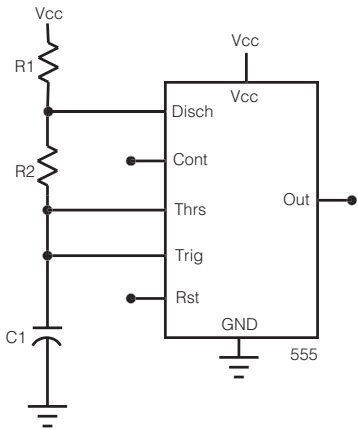
Figure 12-18: 555 Timer in Astable Configuration.
