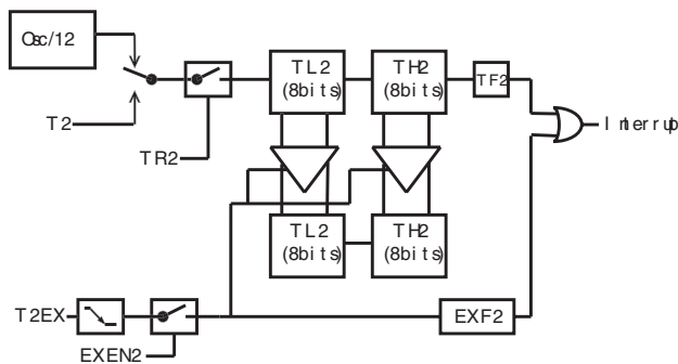
Figure 6-30: Timer/Counter 2, Capture mode.
