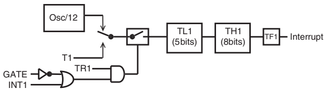
Figure 6-26: Timer/Counter 1, Mode 0.
