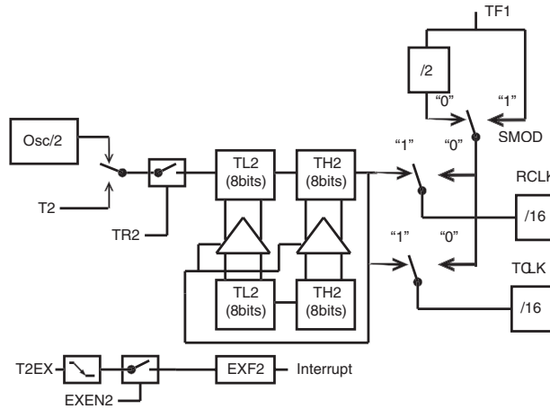
Figure 6-31: Timer/Counter 2, Baud Rate Generator mode.
