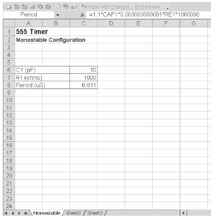
Figure 12-2: Preparation for monostable model.
