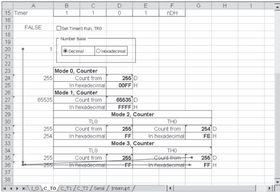
Figure 6-16: Modes 0–3 for Counter input, counter type “count from”. In usage, only one of the modes will be visible at a time, depending on the mode.
