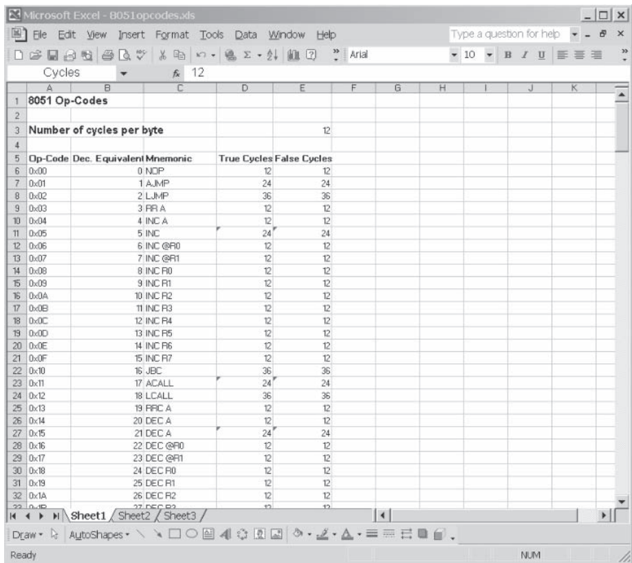
Figure 4-7: Lookup table of 8051 op-codes.
