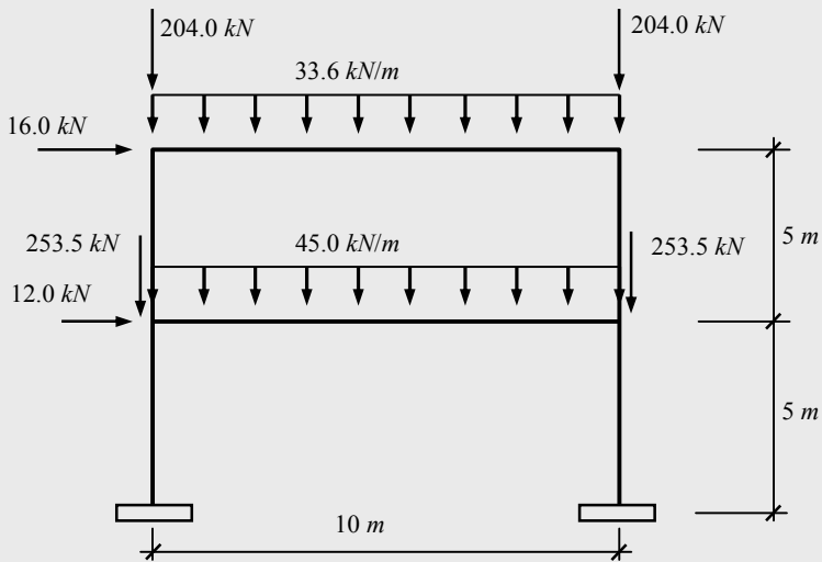
Figure 4.10 – Load arrangement for load combination 1
