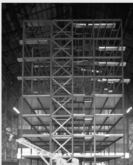
Figure 4.30 – Side elevation view
