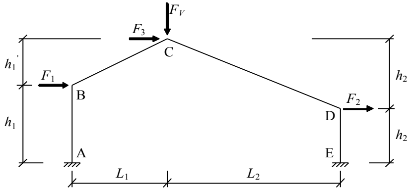
Figure 5.8 – Structural model
