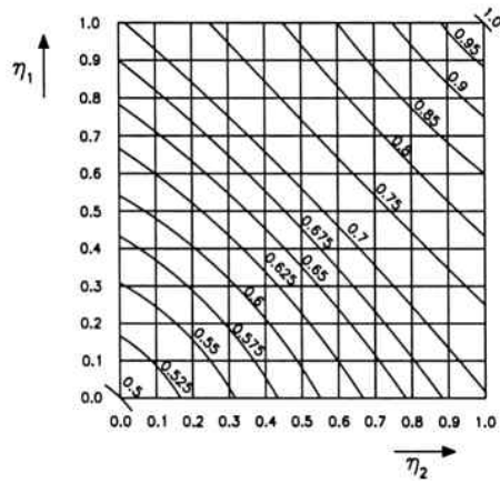
a) Frame with no lateral displacements
