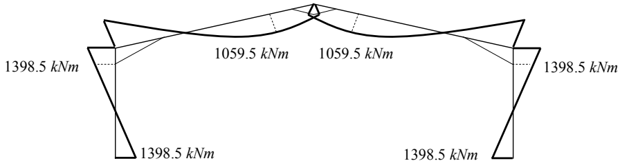
Figure 5.16 – Bending moment diagram at collapse
