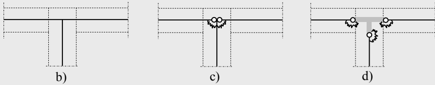
Figure 2.37 – Modelling of the internal node joint
