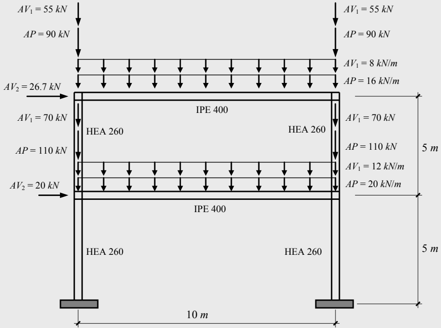
Figure 4.3 – Steel frame
