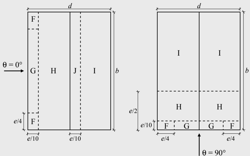
Figure 5.60 – Pressure zones on the roof
