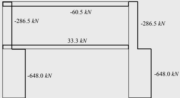
Figure 2.73 – Axial forces due to vertical loads (comb. 2)
