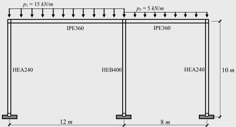
Figure 2.35 – Steel frame
