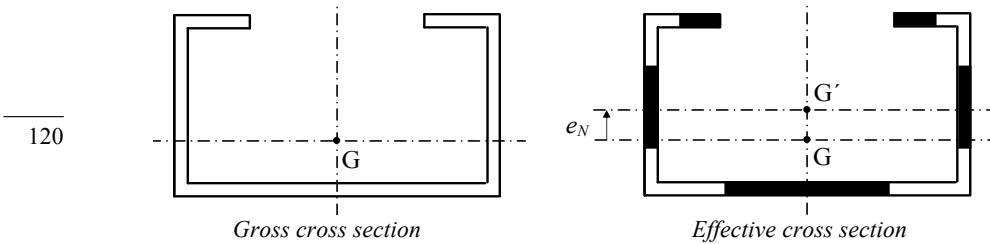
Figure 3.4 – Class 4 cross section submitted to a compressive axial force
