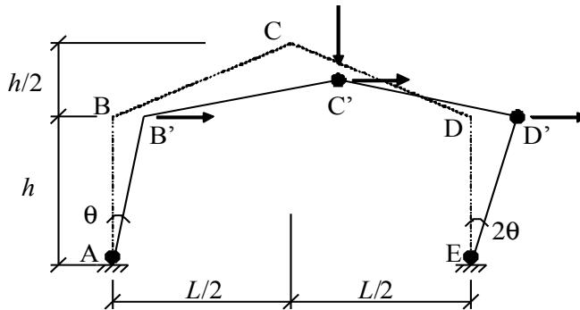
Figure 5.4 – Mechanism 2
