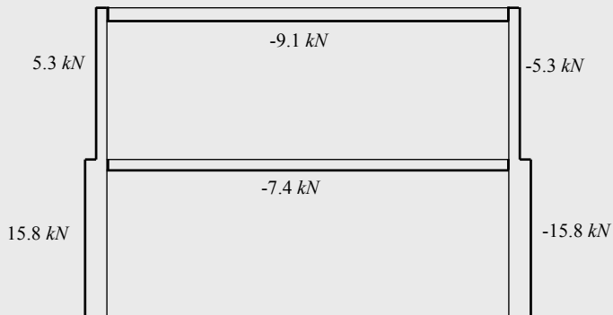
Figure 2.66 – Axial force due to horizontal loads (comb. 1)
