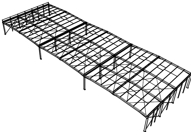
Figure 2.2 – Industrial building
