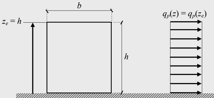
Figure 4.36 – Velocity pressure distribution on face D ( \theta = 90^\circ )
