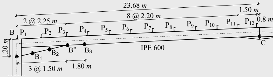
a) Detail of the rafter
