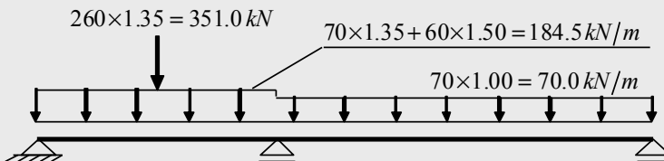
Figure 3.27 – Load combination 2
