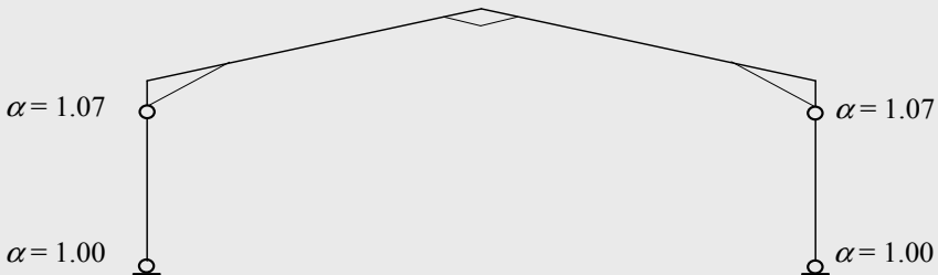
Figure 5.39 – Collapse mechanism and sequence of formation of the plastic hinges
