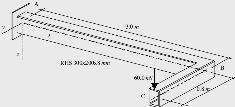
Figure 3.40 – Cantilever beam
