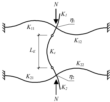
a) Frame with no lateral displacements
