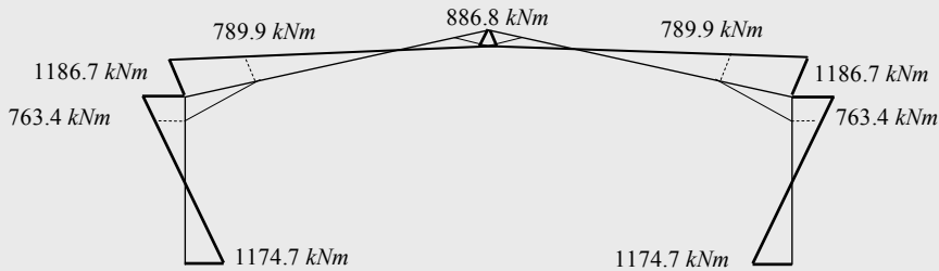
Figure 5.37 – 1 st order bending moment diagram, M_{\zeta}^I
