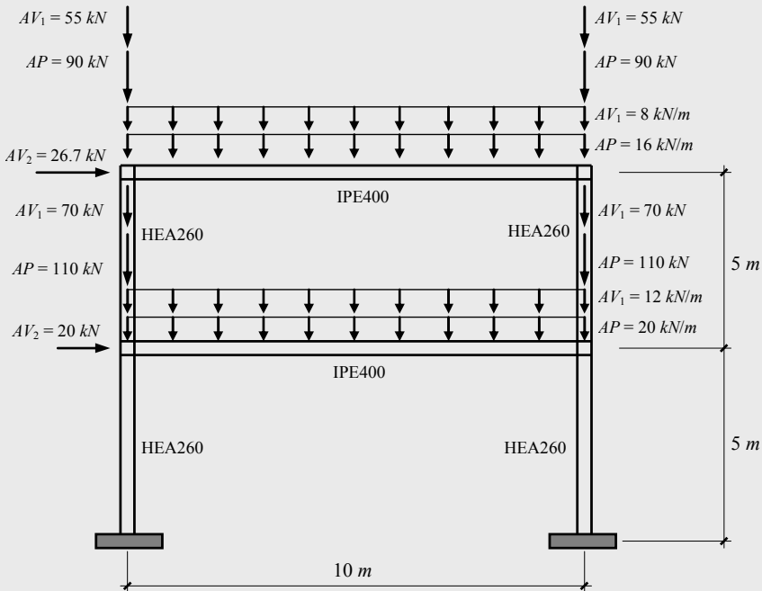
Figure 2.58 – Steel frame
