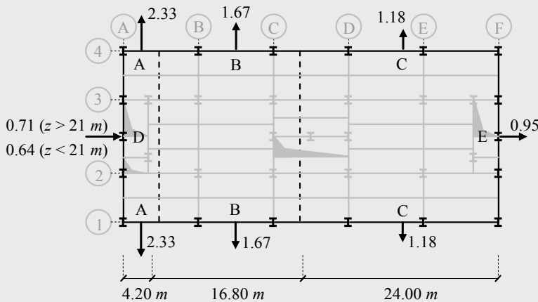
Figure 4.40 – Wind pressures ( \text{kN/m}^2 ) on walls, \theta = 0^\circ
