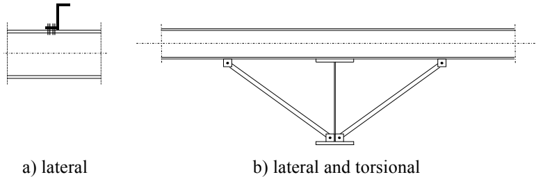
Figure 5.46 – Typical bracing
