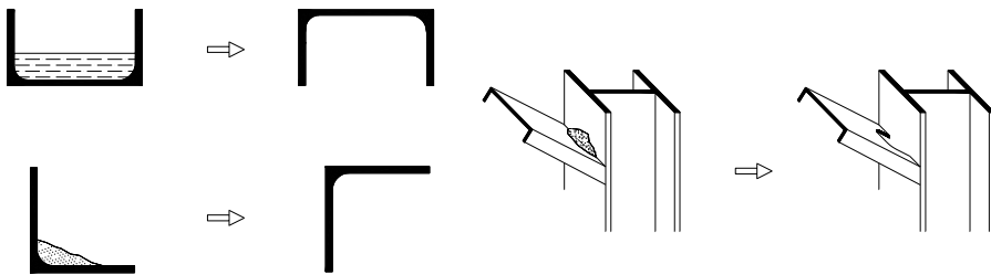
Figure 1.4 – Anti-corrosion details
