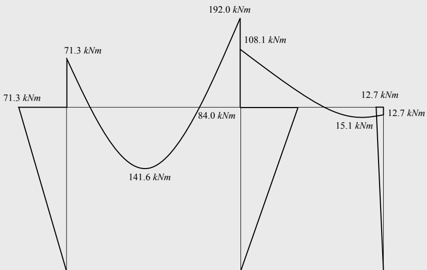
Figure 2.38 – Bending moment diagram
