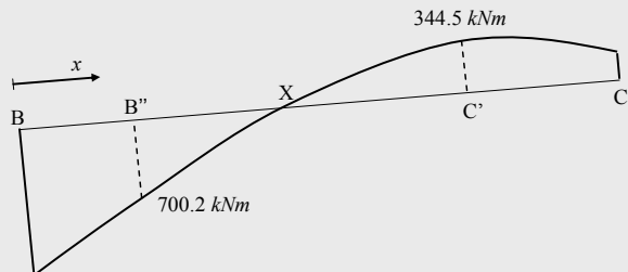
Figure 5.77 – Bending diagram in the rafter for Combination 3
