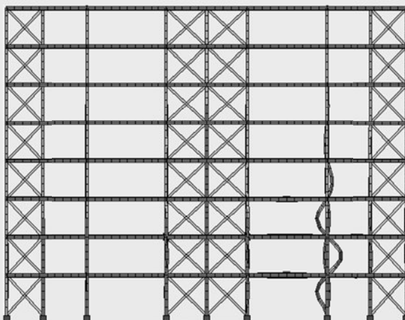
Figure 4.45 – 1 st buckling mode for combination 1 – frontal view
