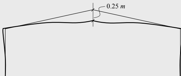
Figure 5.76 – Displacements (LEA) for C4
