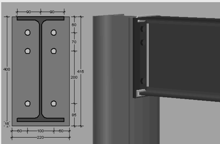
Figure 2.33 – Partial-strength joint at top beam level
