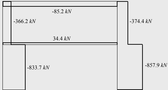
Figure 2.46 – Axial force diagram
