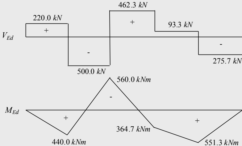
Figure 3.31 – Design internal forces after redistribution
