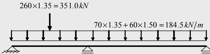
Figure 3.26 – Load combination 1
