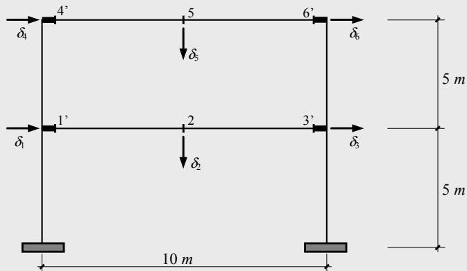
Figure 2.28 – Calculation model with eccentricities
