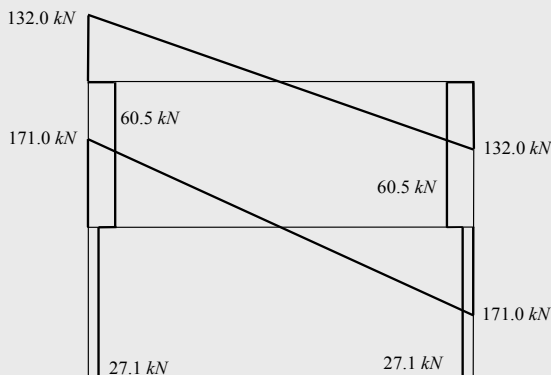
Figure 2.72 – Shear forces due to vertical loads (comb. 2)
