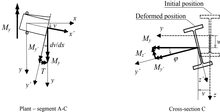
b) Internal forces at-section C
