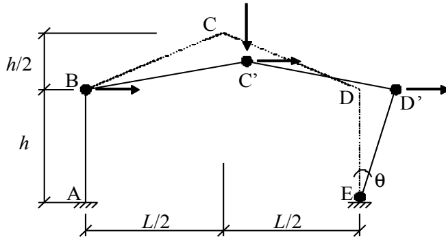
Figure 5.3 – Mechanism 1
