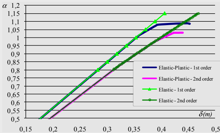
Figure 5.43 – Load factor-horizontal displacement diagram at the apex
