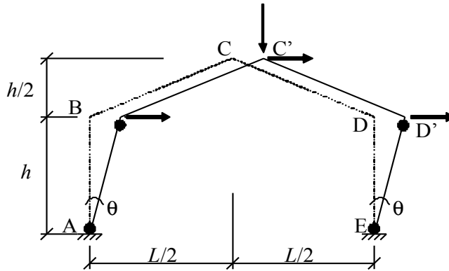
Figure 5.5 – Mechanism 3
