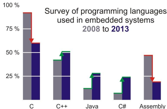
Figure 2-3. Percent of programming languages used in embedded systems (with multiple responses, totals are greater than 100 %). Recreated from http://electronicdesign.com/embedded/developers-discuss-iot-security-and-platforms-trends .
