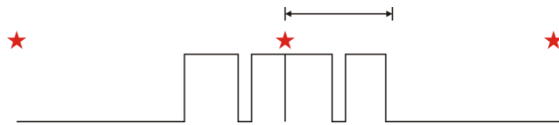
Figure 7-6. A close-to minimum separation between completion times for a task scheduled under RM scheduling.
