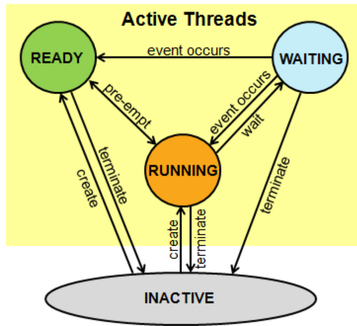
Figure 7-11. The CMSIS state diagram (from http://www.keil.com/pack/doc/cmsis/RTOS/html/modules.html ).
