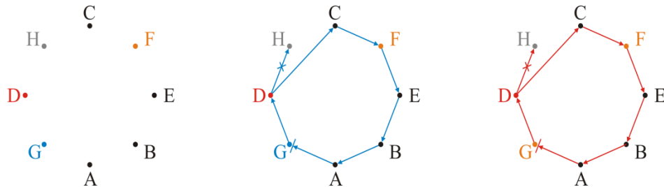
Figure 12-9. Task G begins participation, and thus sends an election message. Task D modifies the message to identify itself as the coordinator, and Task F leaves it unchanged. Task G then sends a victory message identifying Task D as the coordinator.
