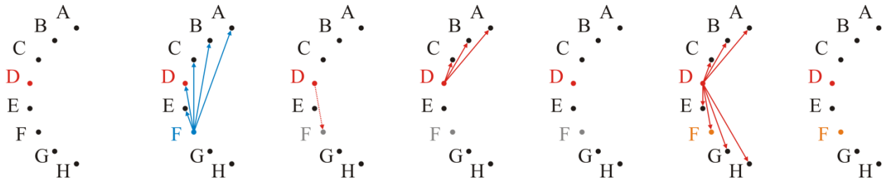
Figure 12-3. Task F calls an election, forcing Task D to call an election while acknowledging Task F. Task D receives no acknowledgment from its election, so it broadcasts a victory notice.
