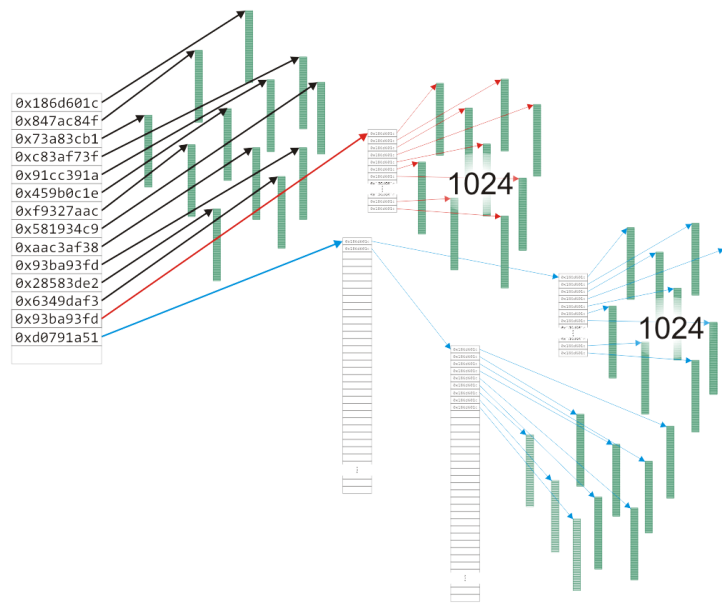
Figure 17-6. The inode of a file occupying 12 + 2048 + 9 = 2069 blocks.
