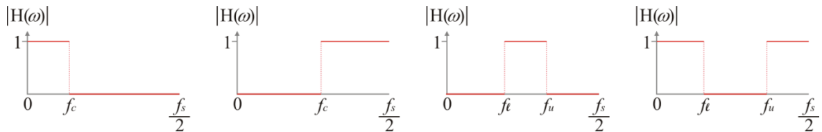
Figure 20-33. Ideal response for low-pass, high-pass, band-pass and band-stop digital filters.
