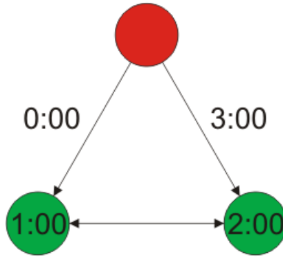
Figure 13-22. A malfunctioning clock sends two separate times to two different clocks.
