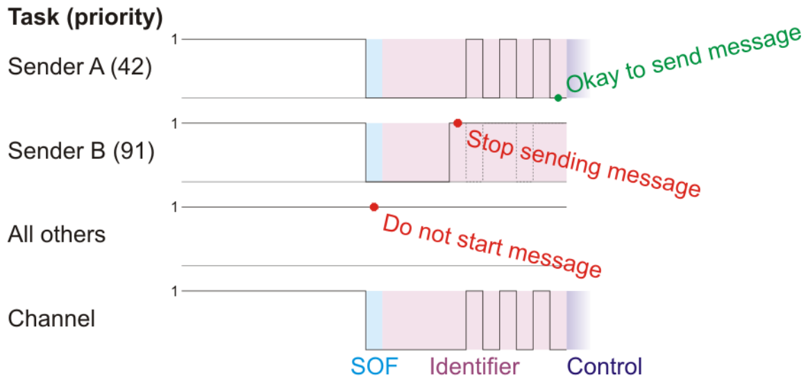
Figure 12-13. Priorities with CAN message frames.
