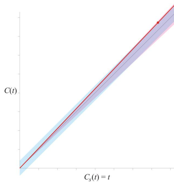
Figure 13-18. Breaking the first requirement: the clock is too fast.
