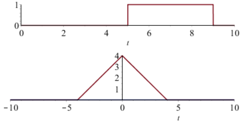
Figure 20-42. The signal equal to 1 on [5, 9] and zero elsewhere, and its autocorrelation.
