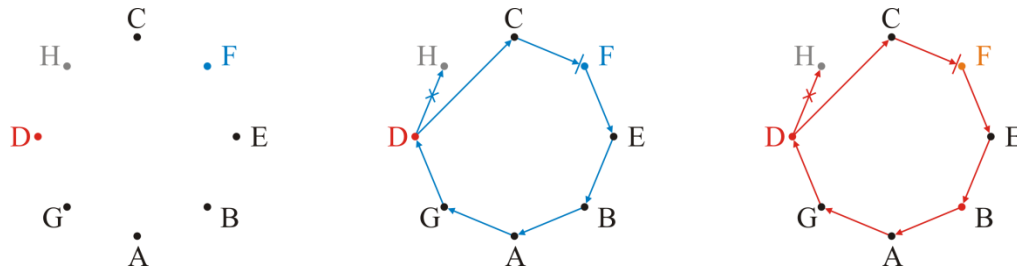
Figure 12-8. Task F begins participating, so it sends an election message identifying itself as a candidate for the coordinator. When the message reaches Task D, it updates the message to identify itself as the coordinator. The message is ultimately received by Task F which then sends a victory message identifying Task D as the coordinator.
