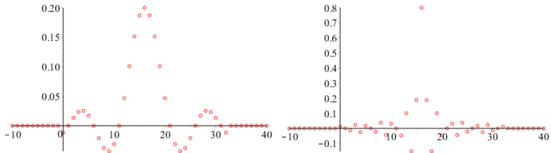
Figure 20-35. Ideal filters delayed by 16 units and truncated to the range [0, 32] .
