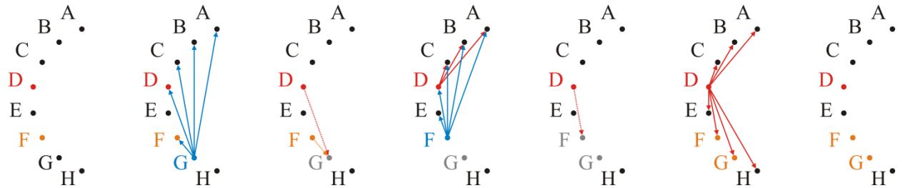
Figure 12-4. Task G calls an election, forcing both Tasks D and F to call elections while acknowledging Task G. Subsequently, Task F receives an acknowledgment from Task D, but Task D receives no acknowledgement from its election, so it broadcasts a victory notice.
