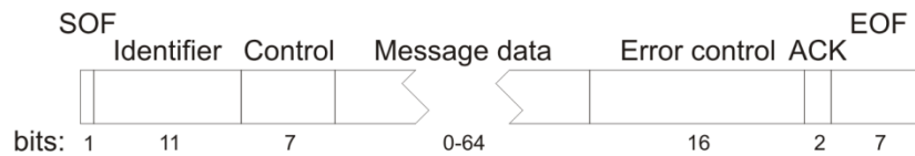
Figure 12-11. Format of a short CAN message frame.
