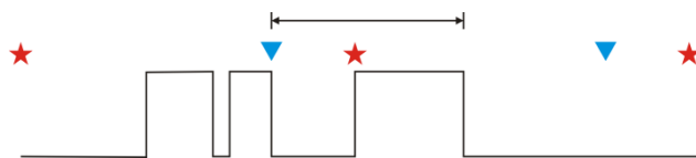
Figure 7-7. The worst-case inter-completion time for a task with a deadline marked with inverted triangles.
