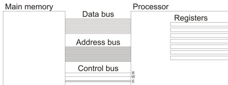
Figure 3-7. The data, address and control buses.
