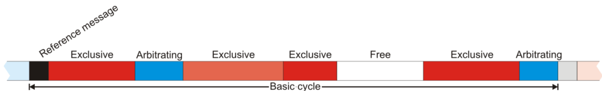
Figure 12-14. A basic cycle of TTCAN broken into seven windows.
