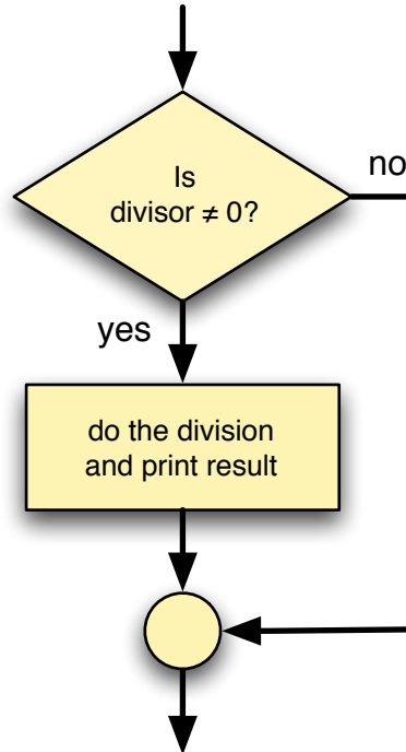
Figure 4.1: if flowchart
