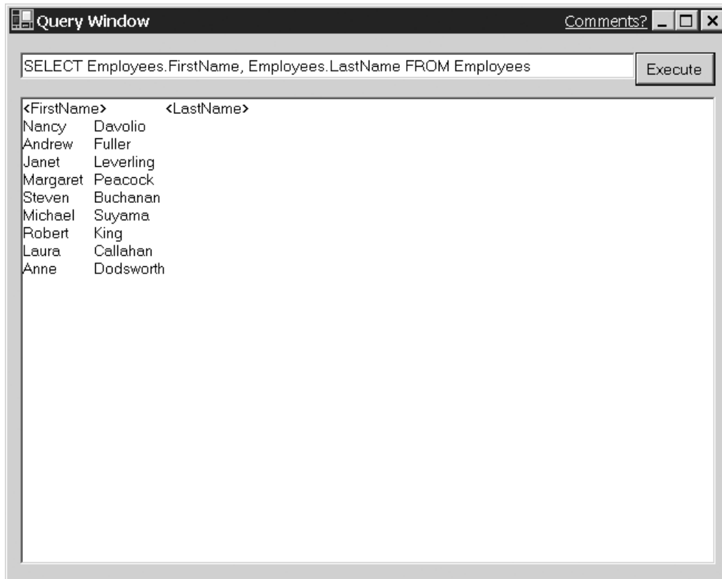
Figure 11-4. The results of querying the Northwind database
