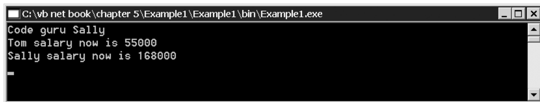
Figure 5-3. Shadowing causes polymorphism to fail.
