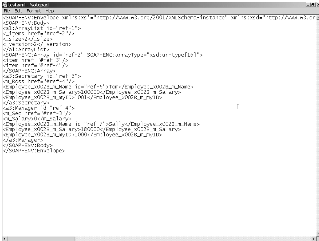
Figure 9-4. A SOAP-based serialization in Notepad
