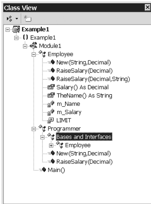
Figure 5-1. Class View in an inheritance chain
