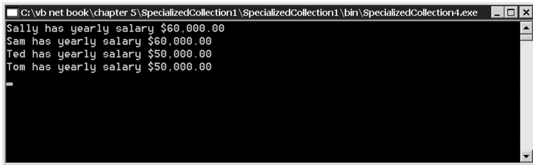
Figure 5-10. The result of using IComparer to sort by multiple conditions
