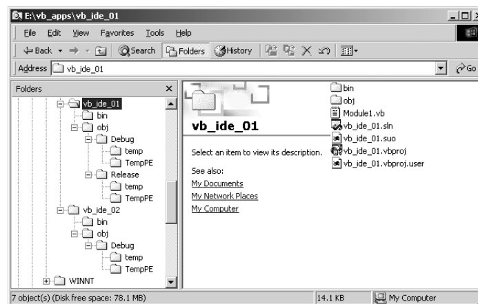
Figure 2-25. Build options
