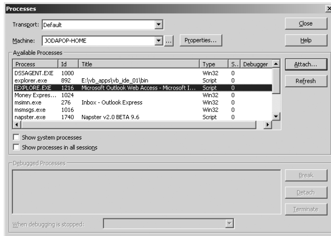
Figure 2-28. Process debugging
