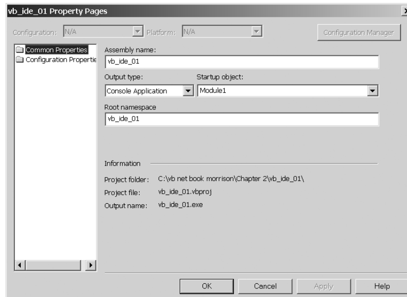
Figure 2-24. Project properties
