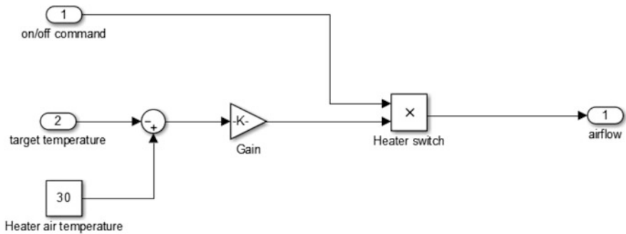
Fig. 5.19 Heater model
