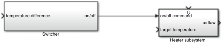
Fig. 5.23 Linking the heater to the switcher
