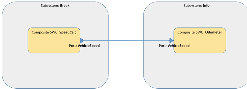
Fig. 4.3 Example of the logical system design done by OEMs (1)
