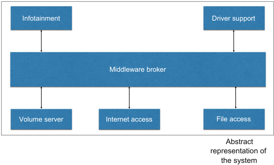
Fig. 2.22 Middleware architectural style
