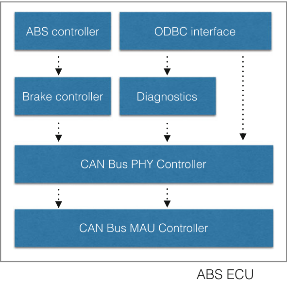
Fig. 2.13 An example of a layered architecture
