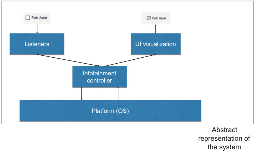
Fig. 2.21 Event-driven architectural style
