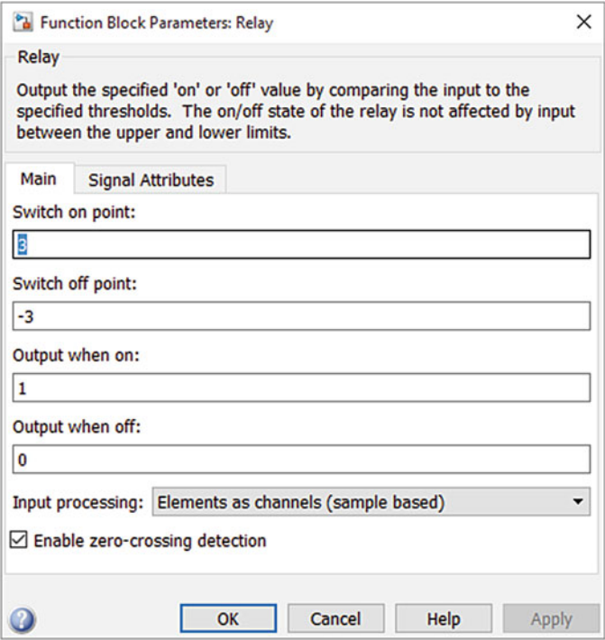
Fig. 5.22 Switcher model—relay properties
