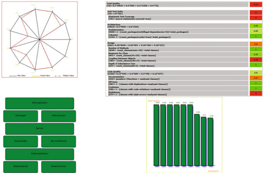
Fig. 5.35 Screenshot from XRadar static analysis software
