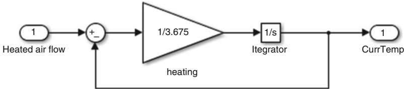
Fig. 5.25 Model of the interior of the car
