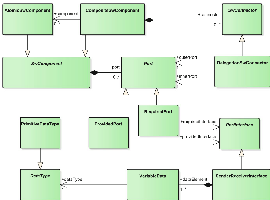
Fig. 4.10 Logical and ECU design example ( SwComponentTemplate )
