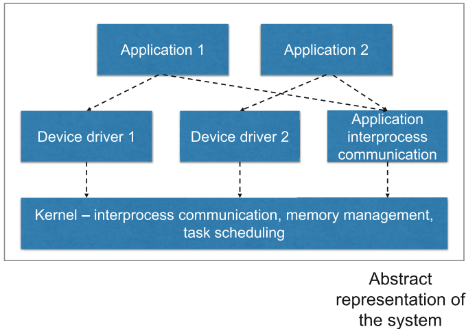
Fig. 2.17 Microkernel architectural style
