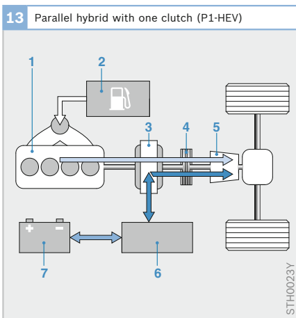
Fig. 13 1 Internal-combustion engine 2 Tank 3 Electric motor (IMG) 4 Clutch 5 Transmission 6 Inverter 7 Battery
