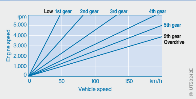
3 Span of a CVT transmission compared with 5-speed automatic (characteristic)
