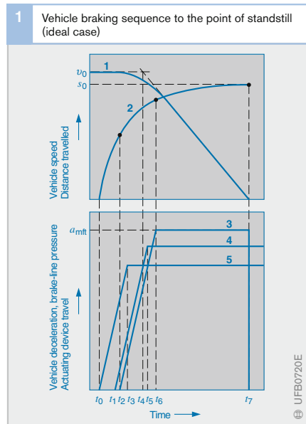
Fig. 1 1 Vehicle speed 2 Distance travelled while braking 3 Vehicle deceleration 4 Brake-line pressure (brake pressure) 5 Actuation device travel t_0 Time at which the driver first applies force to actuation device t_1 Brake-line pressure (brake pressure) starts to rise t_2 Vehicle deceleration begins t_3 Actuation device has reached intended position t_4 Intersection of extended speed curve sections t_5 Brake-line pressure has reached stabilised level t_6 Vehicle deceleration has reached stabilised level t_7 Vehicle comes to a halt
