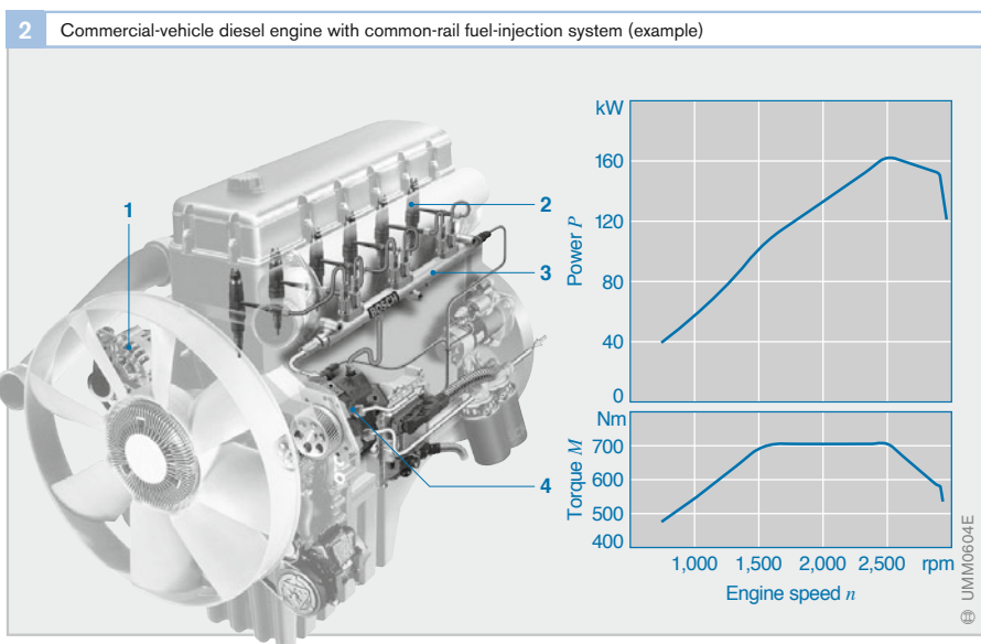
Fig. 2 1 Alternator 2 Injector 3 Fuel rail 4 High-pressure pump
