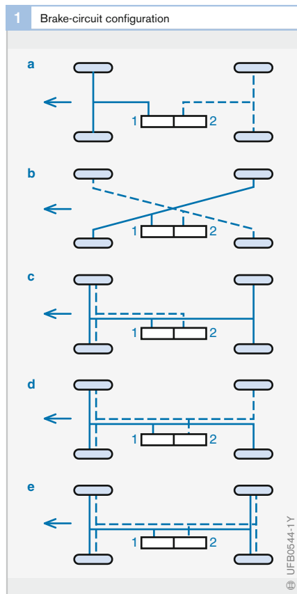
Fig. 1 a II configuration b X configuration c HI configuration d LL configuration e HH configuration 1 Brake circuit 1 2 Brake circuit 2 ← Direction of travel
