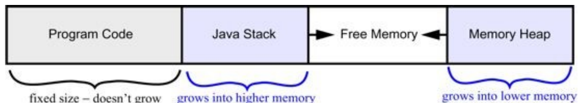
Figure 14.2: A schematic view of the layout of memory addresses in the Java Virtual Machine.
