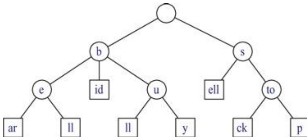
Figure 12.8: Compressed trie for the strings bear, bell, bid, bull, buy, sell, stock, stop. Compare this with the standard trie shown in Figure 12.6 .
