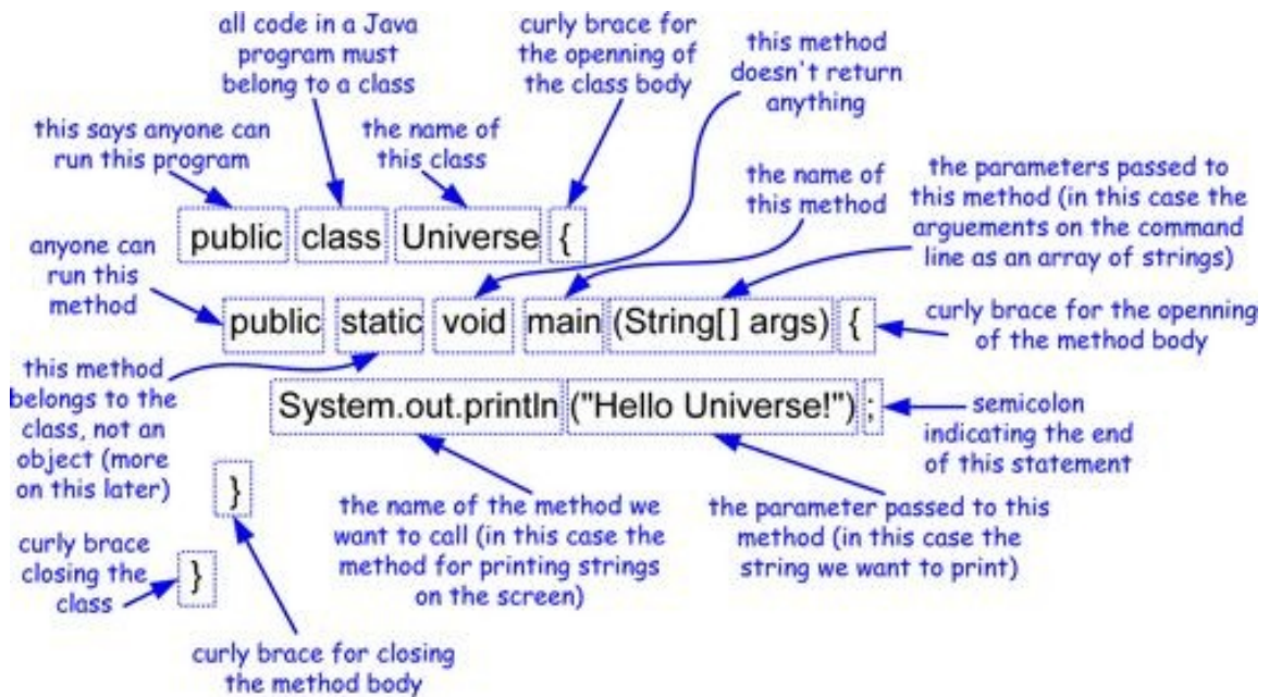
Figure 1.1: A "Hello Universe!" program.
