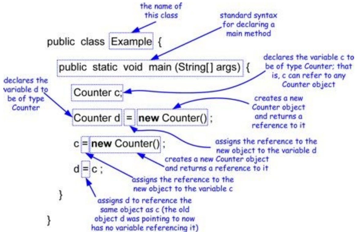
Figure 1.3: Example uses of the new operator.
