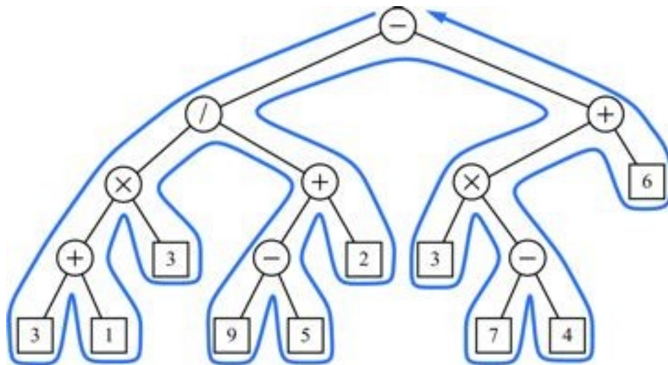
Figure 7.20: Euler tour traversal of a binary tree.
