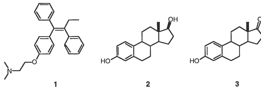
Fig. 1. Tamoxifen (1) and the naturally occurring estrogens 17β-estradiol (2) and estrone (3).
