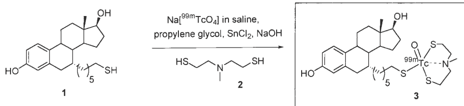
Scheme 2. Synthesis of [3-( N -methyl)azapentane-1,5-dithiolato][7 \alpha -6-mercaptohex-1-yl] estr-1,3,5(10)-triene-3,17 \beta -diol]oxo- ^{99m}\text{Tc} (V) ( 3 ).
