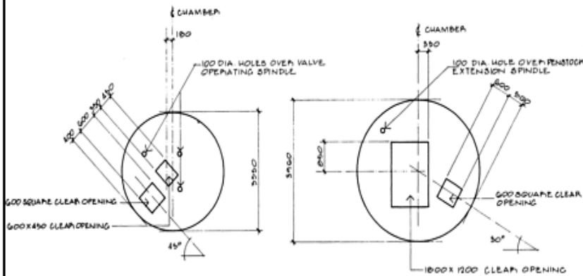
PLAN ON ROOF SLABS
