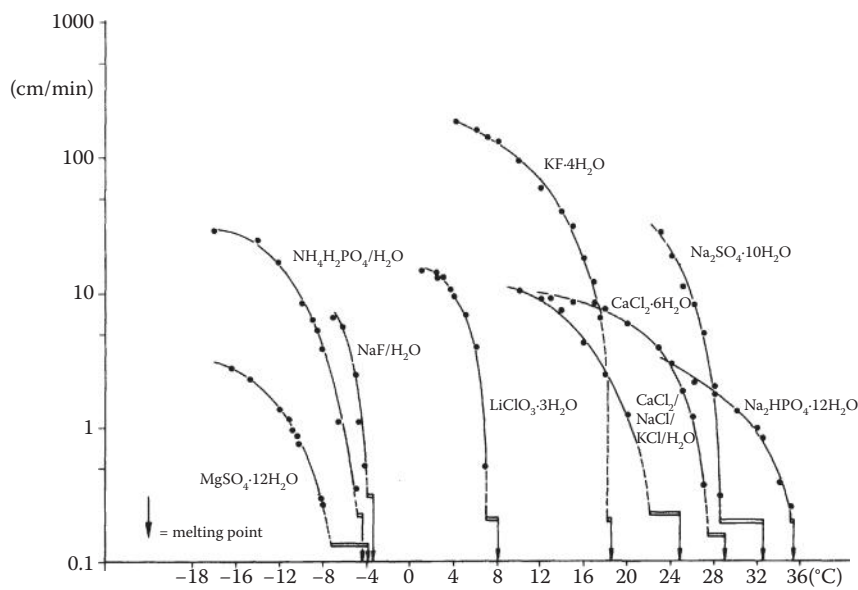
FIGURE A4.2 Rate of crystallization of several low-temperature hydrates and eutectics. Note that \text{Na}_2\text{SO}_4 \cdot 10\text{H}_2\text{O} and \text{CaCl}_2/\text{NaCl}/\text{KCl}/\text{H}_2\text{O} have very inadequate rates without substantial sub-cooling. (From Schröder, J., Philips GmbH Forschungslaboratorium [Aachen] Report, 1977.)
