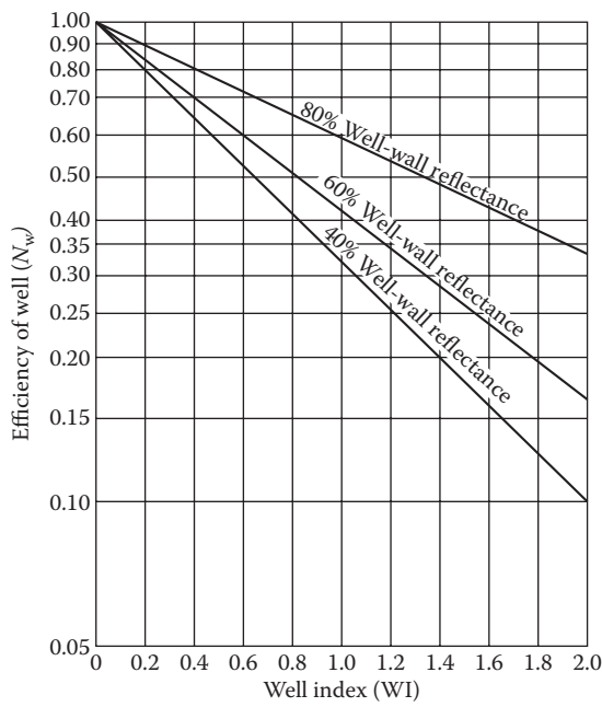
FIGURE 7.16 Efficiency of well versus well index. (From IES, Lighting Handbook, Applications Volume , Illumination Engineering Society, New York, 1987.)
