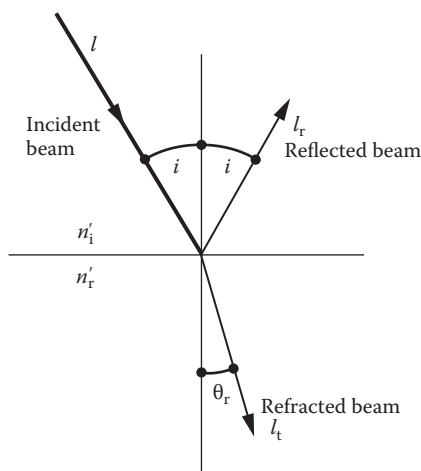
FIGURE 3.6 Diagram showing incident, reflected, and refracted beams of light and incidence and refraction angles for a transparent medium.
