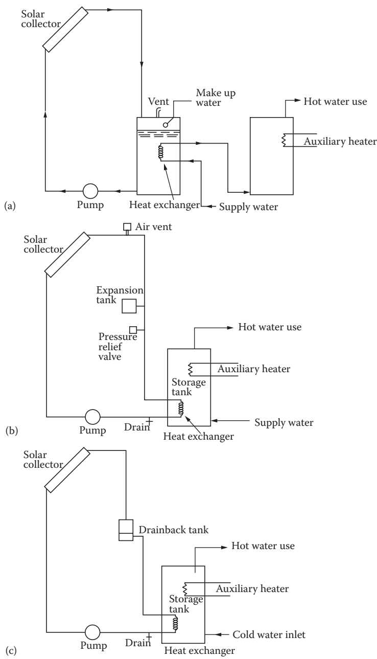
FIGURE 5.6 Typical configurations of solar water-heating systems: (a) open loop system, (b) closed loop system, and (c) closed loop drainback system. (Adapted from Goswami, D.Y., Alternative Energy in Agriculture , Vol. 1, Boca Raton, FL, CRC Press, 1986.)
