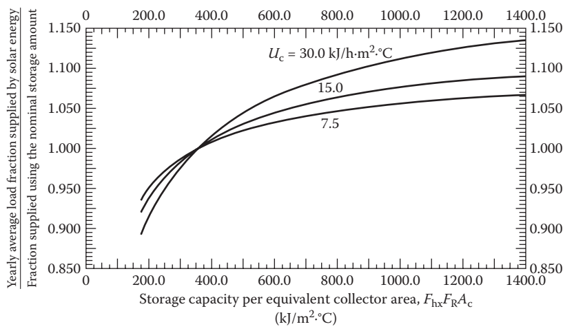
FIGURE 5.10 Effect of liquid storage capacity on liquid-based solar heating system energy delivery. (From Klein, S.A., A design procedure for solar heating systems, PhD dissertation, University of Wisconsin, Madison, WI, 1976.)
