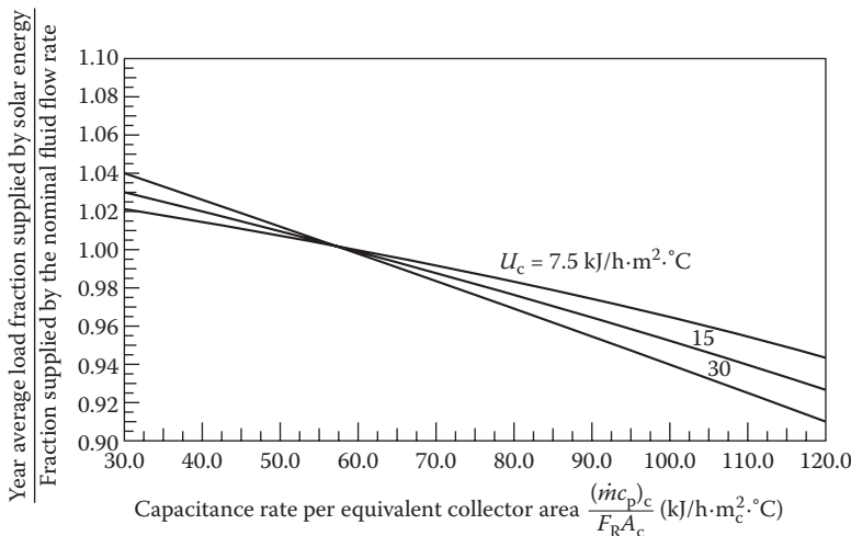
FIGURE 5.17 Effect of collector fluid flow rate on annual energy delivery in an air-based solar heating system. The effect of the collector loss coefficient U_c is also shown. The nominal fluid flow rate is 58\text{ kJ/m}^2\cdot^\circ\text{C}\cdot\text{h} , based on the equivalent areas F_R A_c (\dot{m}c_p)_{\text{air}} . (Adapted from Klein, S.A., A design procedure for solar heating systems, PhD dissertation, University of Wisconsin, Madison, WI, 1976.)
