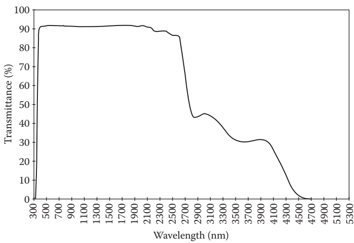
FIGURE 3.10 Spectral transmittance of a 3-mm low-iron float glass.
