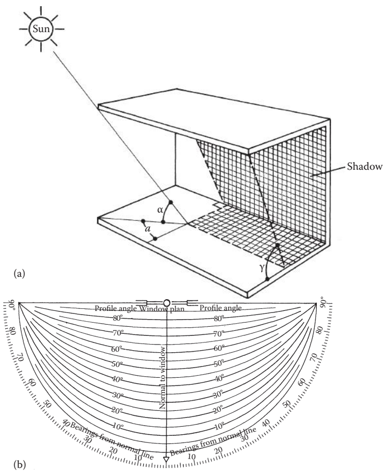
FIGURE 2.13 (a) Sketch showing the profile angle \gamma and the corresponding solar altitude angle \alpha for a window shading device; (b) the shadow-angle protractor. (With permission from the Libby-Owens-Ford Glass Co.)
