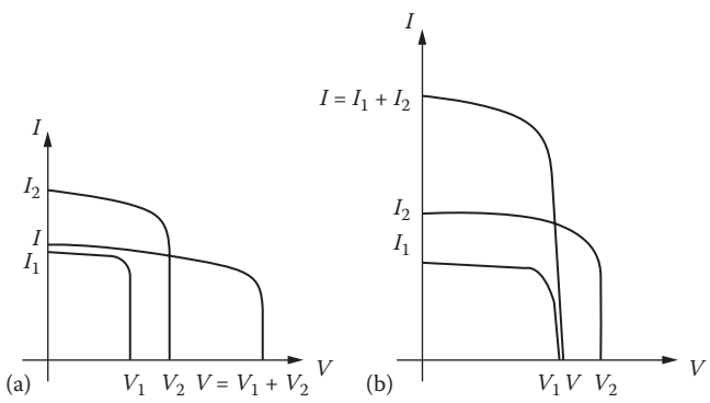
FIGURE 9.20 Characteristics of two dissimilar cells connected in (a) series and (b) parallel.
