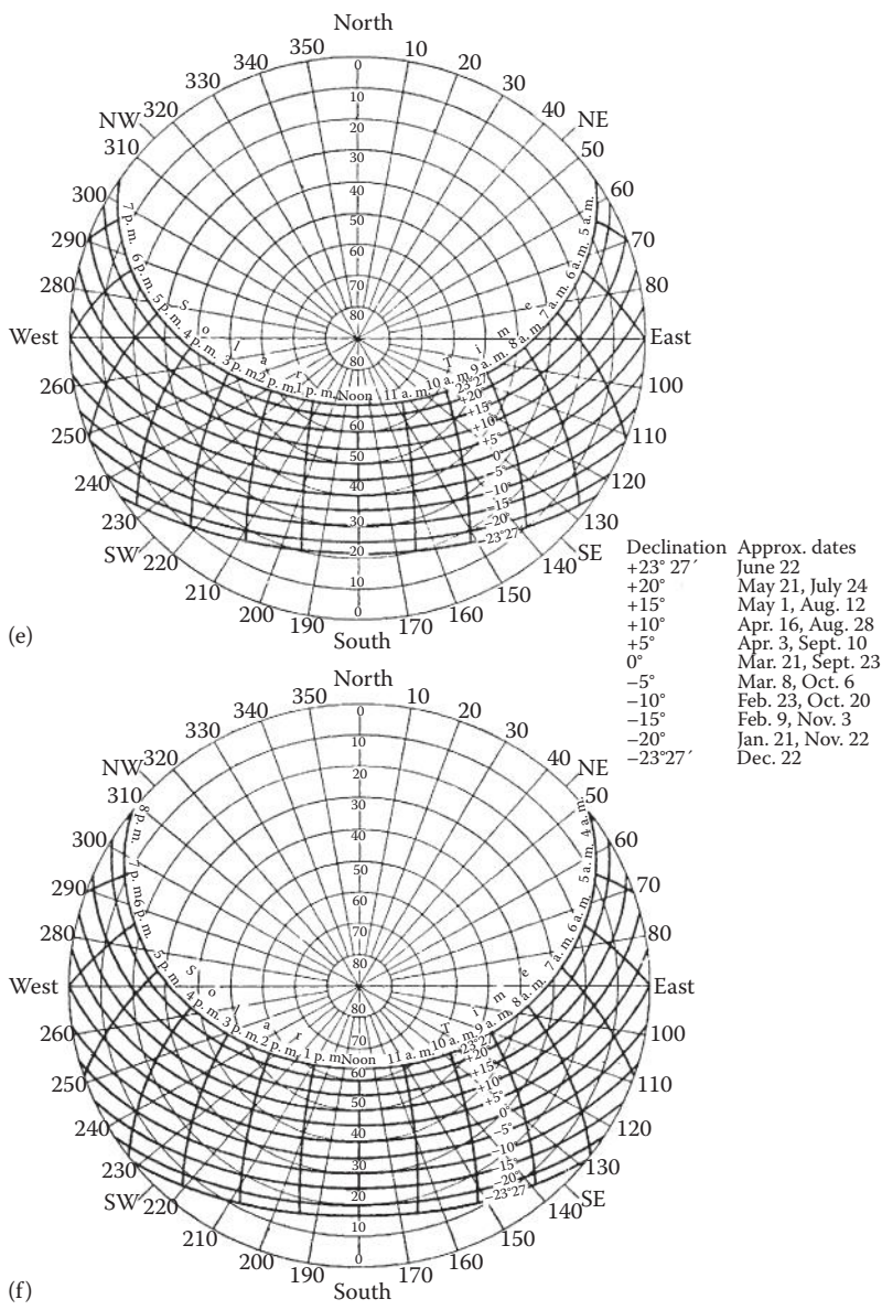
FIGURE A2.1 (CONTINUED) Description of method for calculating true solar time, together with accompanying meteorological charts, for computing solar altitude and azimuth angles. (e) 45°N latitude; (f) 50°N latitude.
