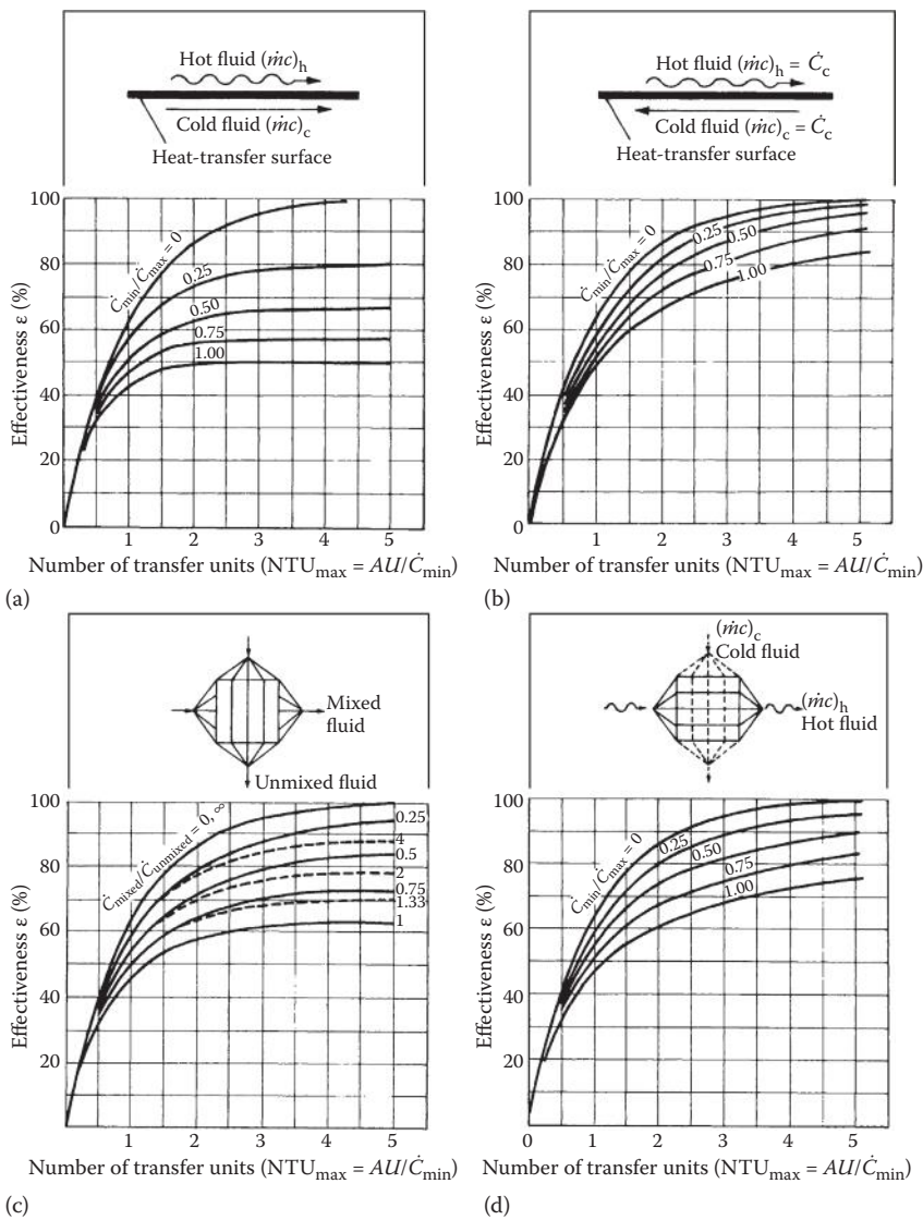
FIGURE 4.13 Heat-exchanger effectiveness as a function of NTU and C; (a) parallel flow, (b) counterflow, (c) cross flow, one fluid mixed, and (d) cross flow, no mixing. (From Kays, W.M. and A.L. London, Compact Heat-Exchangers , McGraw-Hill, New York, 1980. Copyright 1964. With permission from McGraw-Hill Book Company.)
