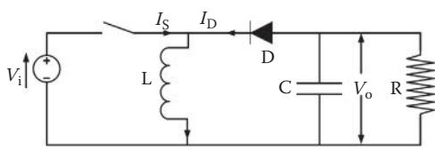
FIGURE 9.11 Schematic of a buck-boost converter. (Adapted from http://en.wikipedia.org/wiki/File:Buckboost_conventions.svg .)
