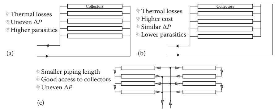
FIGURE 8.16 Solar field layout loops. (a) Direct return. (b) Inverse return. (c) Central feed. (Adapted from Romero-Alvarez, M. and E. Zarza, Concentrating solar thermal power, In Energy Conversion , D.Y. Goswami and F. Kreith (eds.), Boca Raton, FL: CRC Press, 2008.)
