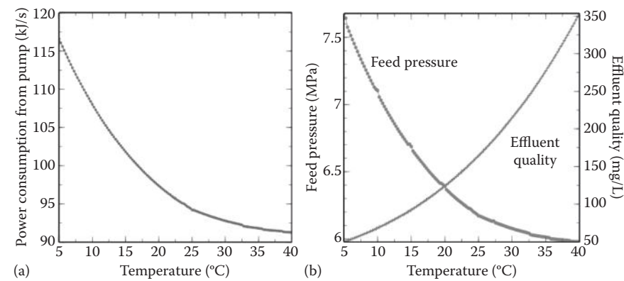
FIGURE 8.57 (a) Power consumption of the designed RO versus seawater temperature; (b) RO system pressure and effluent TDS versus seawater temperature.
