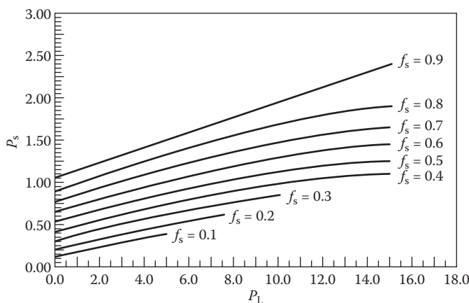
FIGURE 5.22 The f -chart for air-based solar space-heating systems. (From Klein, S.A., A design procedure for solar heating systems, PhD dissertation, University of Wisconsin, Madison, WI, 1976.)
