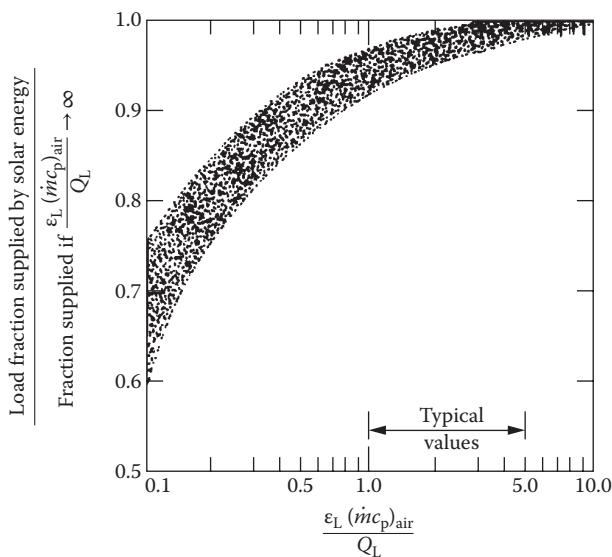
FIGURE 5.13 Effect of load device capacity for forced-air heating systems. Q_L is the building heat load expressed in units consistent with (\dot{m}c_p)_{air} . (From Klein, S.A., A design procedure for solar heating systems, PhD dissertation, University of Wisconsin, Madison, WI, 1976.)
