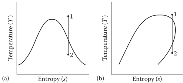
FIGURE 8.11 T - s characteristics of (a) wetting and (b) drying types of working fluids.
