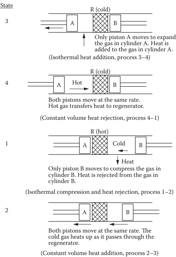
FIGURE 8.25 Stirling cycle states and processes with reference to Figure 8.24.
