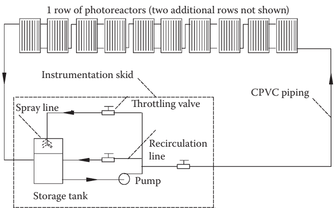
FIGURE 10.16 Schematic diagram of solar groundwater treatment test facility at TyAFB.
