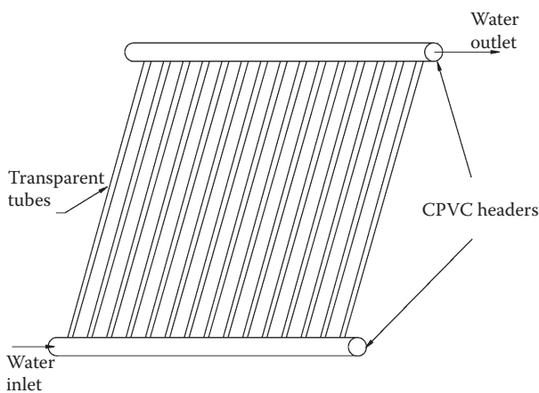
FIGURE 10.7 Flat plate reactor with rigid transparent tubes.
