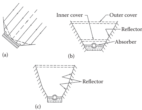
FIGURE 3.32 Examples of flat reflectors used to concentrate sunlight. (a) Flat-plate collector with reflective wings. (b) Trapezoidal design. (c) Two-facet design. (From ASHRAE 93-2003, Methods of testing to determine the thermal performance of solar collectors, ASHRAE, Atlanta, GA.)
