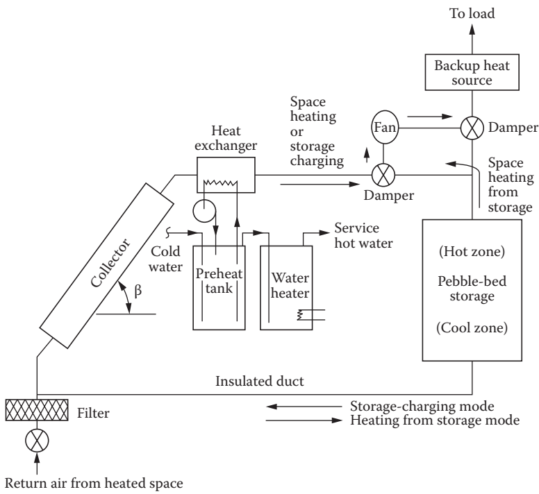
FIGURE 5.14 Typical air-based solar space-heating system showing directions of fluid flow and important components.
