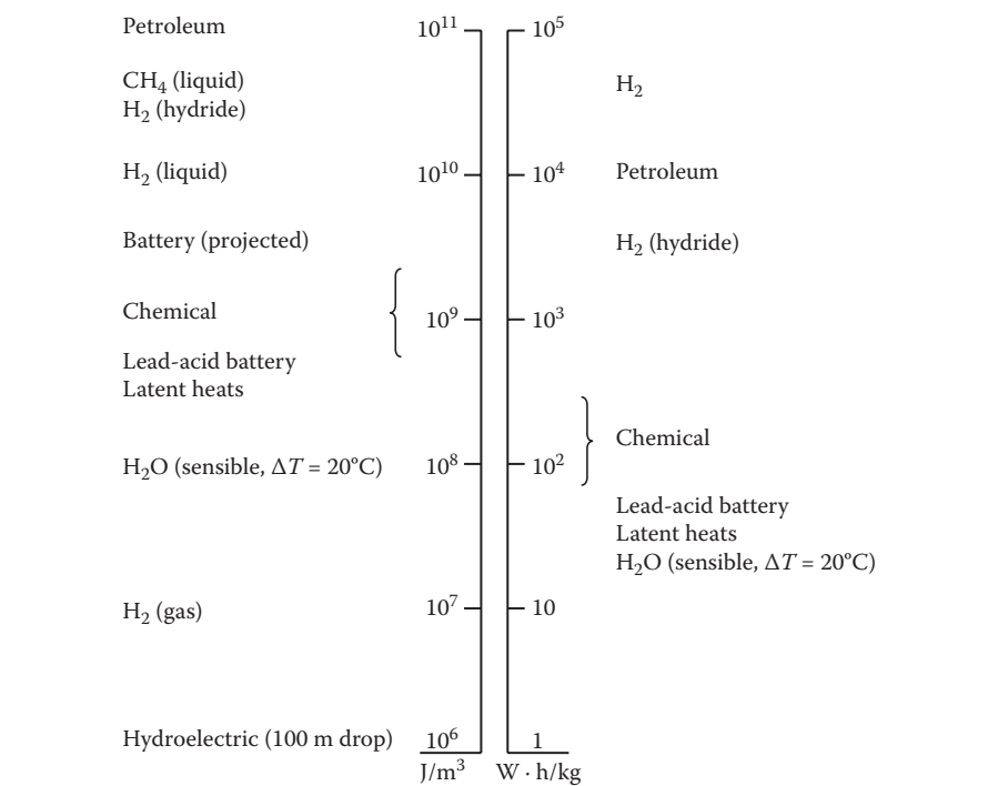
FIGURE 1.11 Mass and volumetric energy densities for typical energy-storage media. (Redrawn from Offenhartz, P.O.D., Classical methods of storing thermal energy. In: K.W. Böer (ed.), Sharing the Sun-Solar Technology in the Seventies , vol. 8, Solar Energy Society of Canada, Winnipeg, 1976.)
