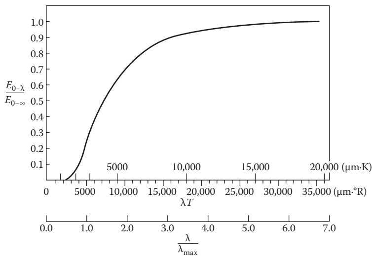
FIGURE 2.4 Fraction of total emissive power in spectral region between \lambda = 0 and \lambda as a function of \lambda T and \lambda/\lambda_{\text{max}} .
