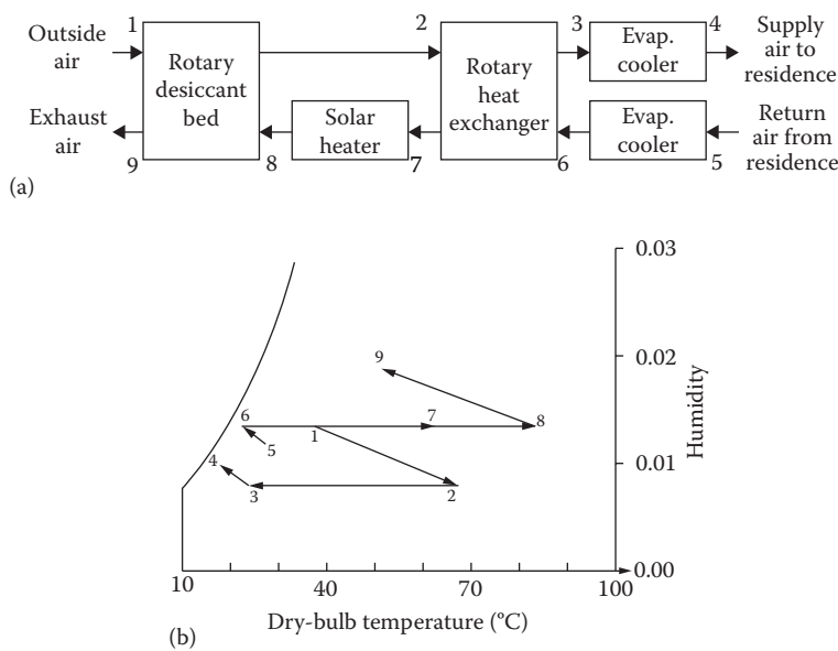
FIGURE 6.13 Schematic of a desiccant cooling ventilation cycle: (a) schematic of airflow, (b) process on a psychrometric chart.
