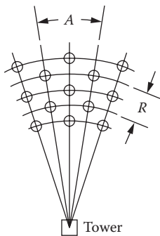
FIGURE 8.48 The radial stagger heliostat layout pattern developed by the University of Houston.
