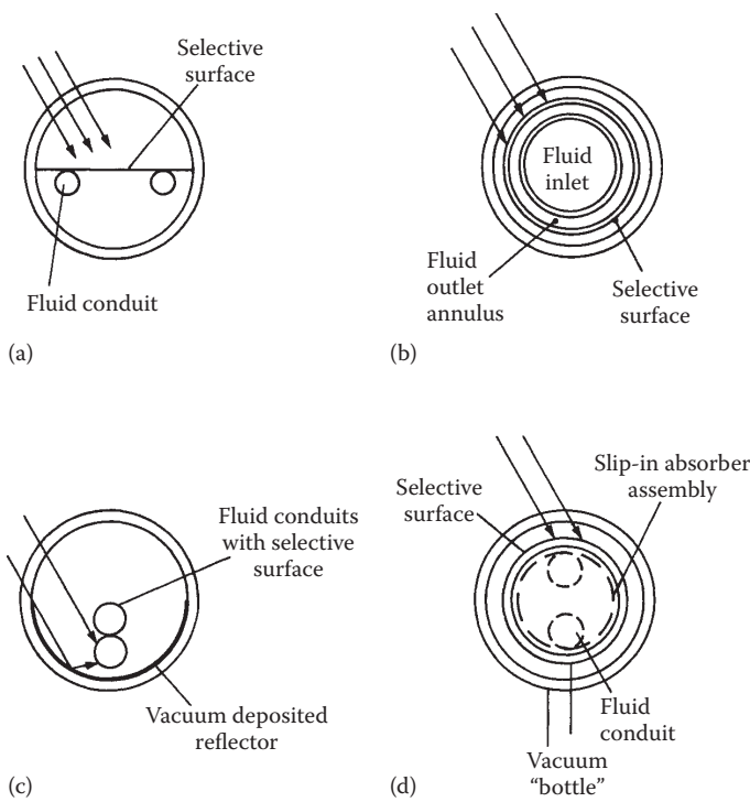
FIGURE 3.19 Evacuated-tube solar energy collectors: (a) flat plate, (b) concentric tubular, (c) concentrating, (d) vacuum bottle with slip-in heat exchanger contacting rear surface of receiver.
