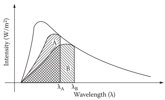
FIGURE 9.12 Energy conversion from a two-layered stacked cell.
