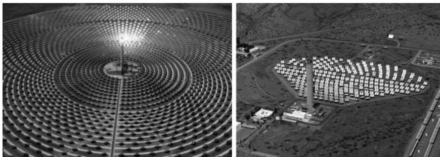
FIGURE 8.47 Aerial views of the plants Gemasolar (19.9 MW) and CESA-1 (1.2 MW) in Spain.
