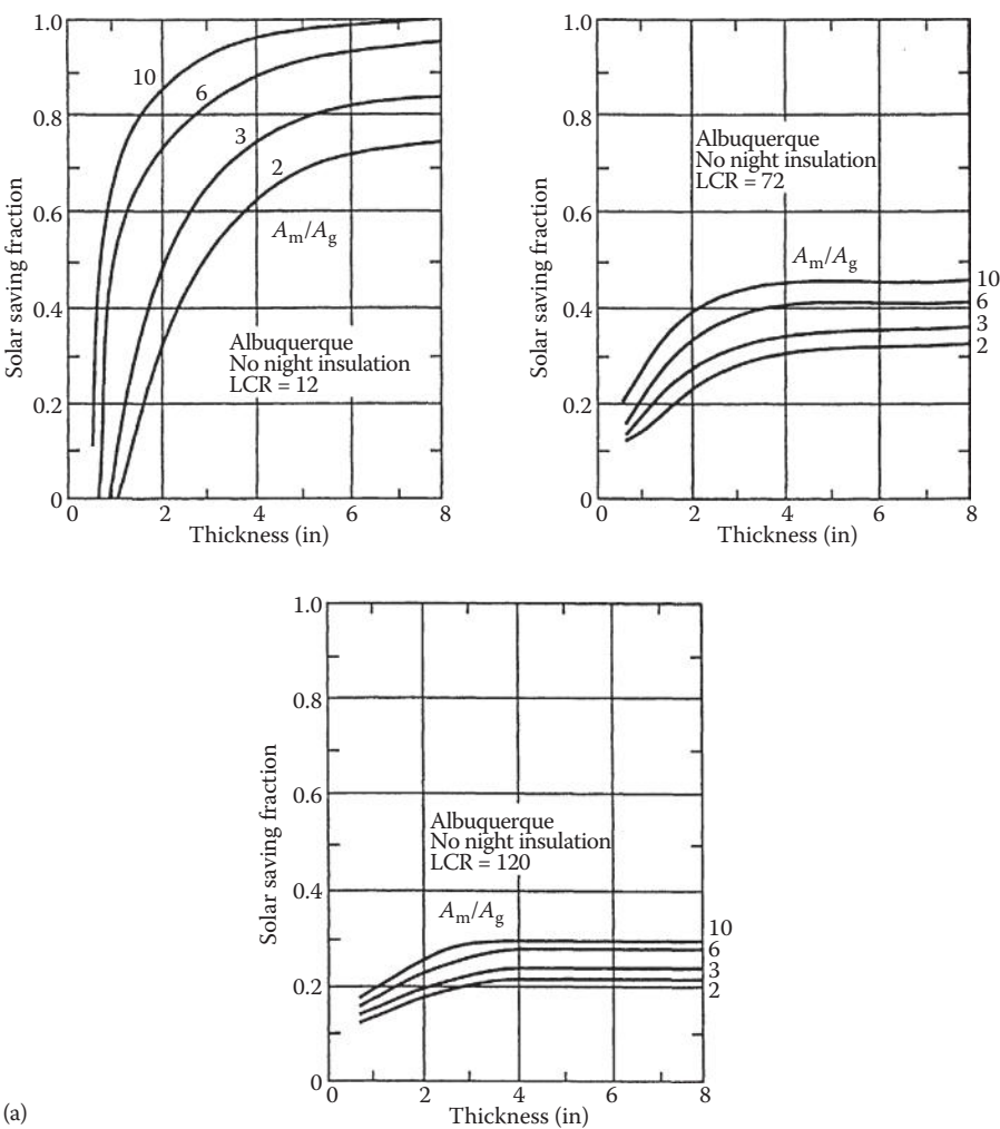
FIGURE A7.1 (a) Storage wall: mass thickness sensitivity of SSF to off-reference conditions.
