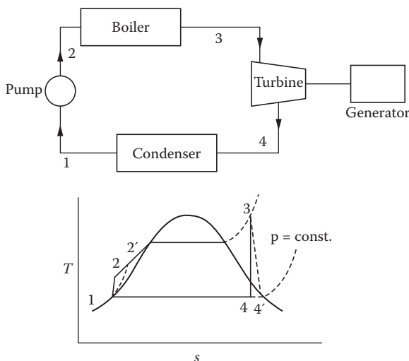
FIGURE 8.5 Basic Rankine power cycle.
