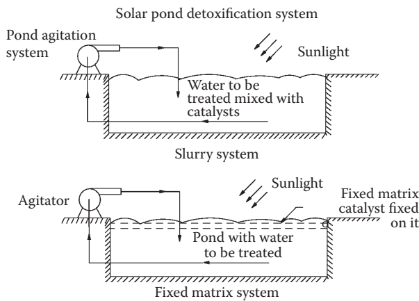
FIGURE 10.9 Shallow solar pond reactors. (From Bedford, J. et al., J. Sol. Energy Eng. , ASME 116(1): 8–13, 1994.)
