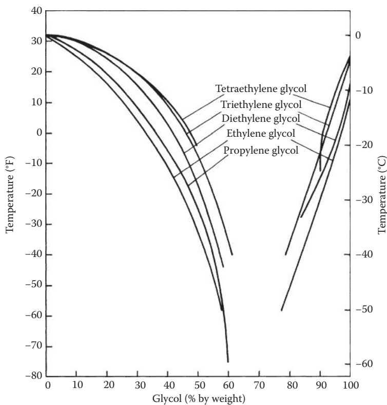
FIGURE A4.6 Freezing-point depression of aqueous solutions of common glycol antifreezes. (From Union Carbide, Glycols, F-41515A 7/71-12M, p. 17, 1971.)
