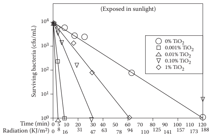
FIGURE 10.19 Effect of concentration of \text{TiO}_2 on survival of Serratia marcescens bacteria. (From Block, S.S., and D.Y. Goswami, Chemically enhanced sunlight for killing bacteria. Solar Engineering, Proceedings of the ASME International Solar Energy Conference , Hawaii, March, pp. 431–438, 1995.)
