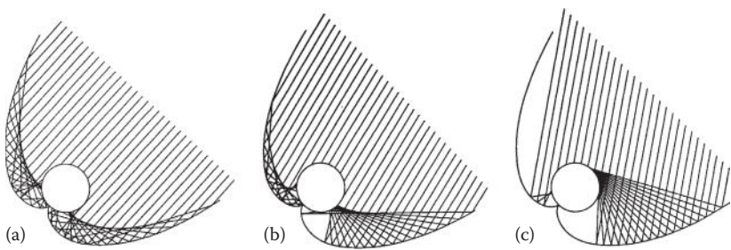
FIGURE 3.48 Ray trace diagrams of the tubular CPC collector at three values of incidence angle: (a) normal incidence, (b) intermediate, and (c) the limit of acceptance. (Courtesy of W. McIntire, Argonne National Laboratory.)
