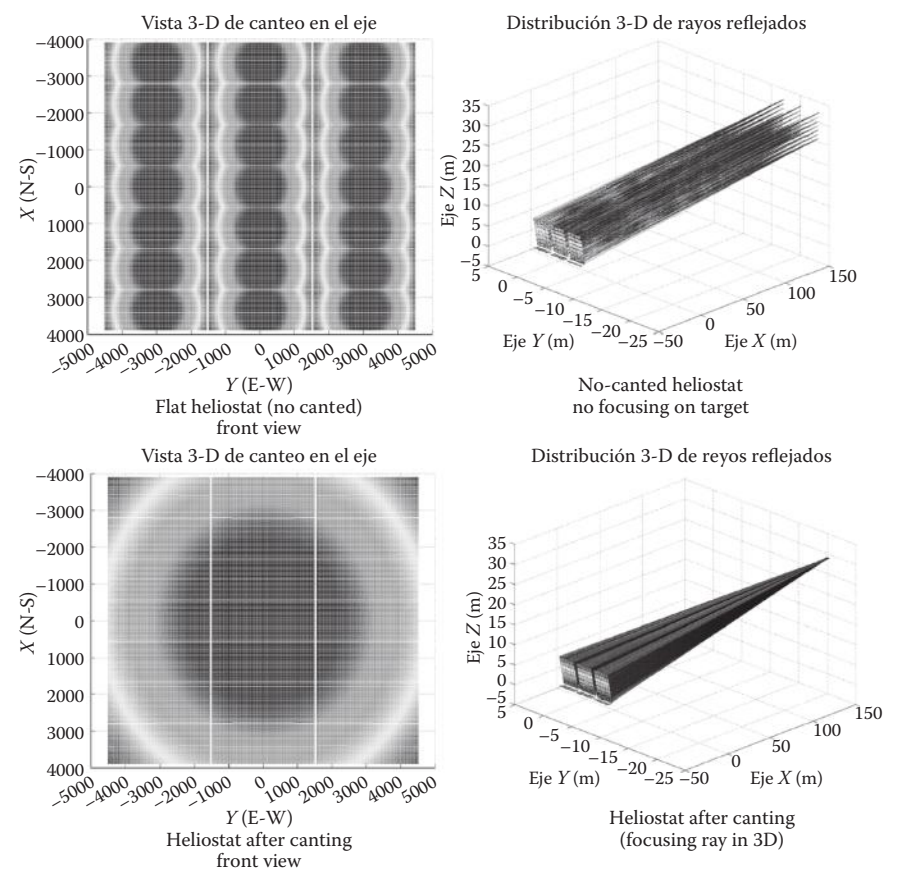
FIGURE 8.35 Effect of canting facets in a glass metal heliostat. (From Jones, S.A., A comparison of on-axis and off-axis heliostat alignment strategies, Report SAND96-0566C, Sandia National Lab., Albuquerque, NM, 1996.)
