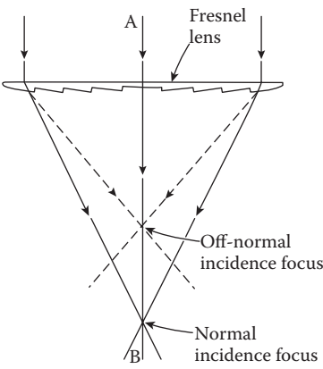
FIGURE 3.52 Line-focus Fresnel lens concentrator section showing nominal focus for normal incidence and shortened focal length at off-normal incidence.
