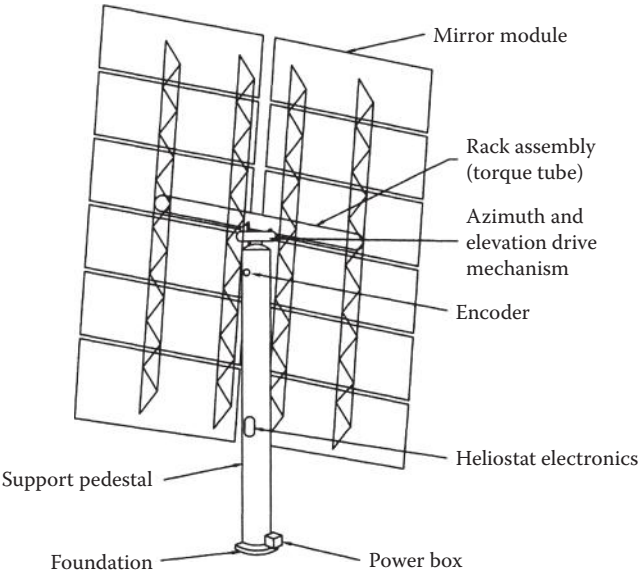
FIGURE 8.33 A heliostat consisting of glass mirrors supported on a structure (back view).
