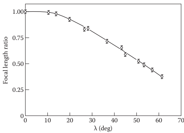
FIGURE 3.53 Effect of off-normal incidence angle \lambda (measured in plane AB out of the plane of Figure 3.52) on apparent focal length of a line-focus Fresnel lens. The focal length ratio is the focal length at \lambda \neq 0 divided by the focal length at \lambda = 0 (i.e., normal incidence). (From Rabl, A., Proc. Sol. Thermal Cone. Coll. Tech. Symp. , B. Gupta, ed. Denver, CO, 1–42, 1978.)
