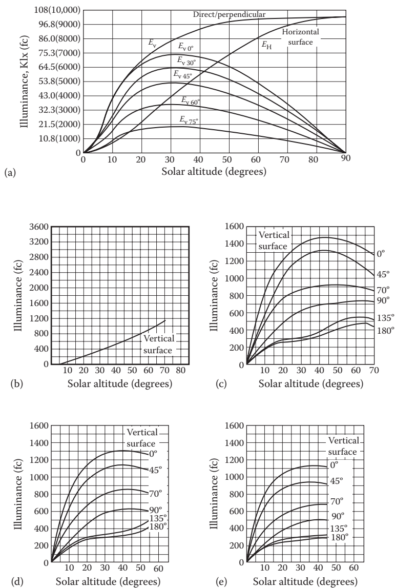
FIGURE 7.13 Vertical illuminance from (a) direct sunlight. (b) Overcast skylight. (c) Clear summer skylight. (d) Clear autumn/spring skylight. (e) Clear winter skylight, skylight, for various sun–window azimuth angle differences. (From IES, Lighting Handbook, Applications Volume , Illumination Engineering Society, New York, 1979.)
