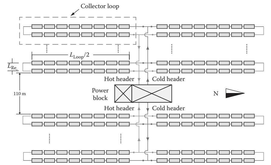
FIGURE 8.17 I solar field layout. (Adapted from Vasquez-Padilla, R., Simplified methodology for designing parabolic through solar power plants. PhD dissertation, University of South Florida, Tampa, FL, 2011.)
