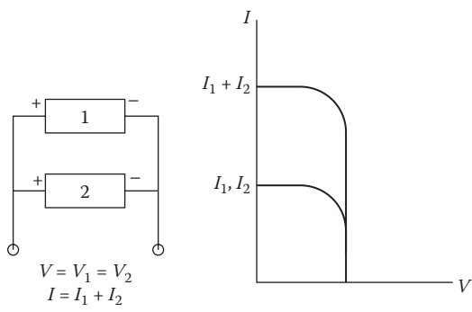
FIGURE 9.19 Characteristics of two similar cells connected in parallel.
