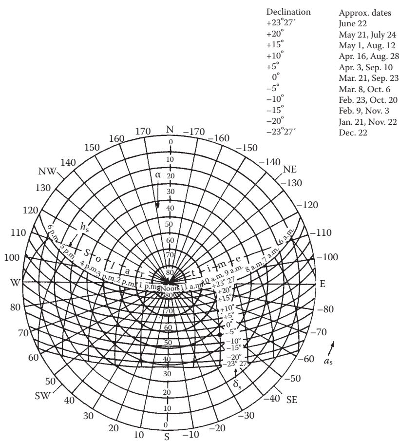
FIGURE 2.12 Sun-path diagram for 30°N latitude showing altitude and azimuth angles. (Modified from Kreider, J.F. and F. Kreith, Solar Heating and Cooling , revised 1sted. Washington, DC: Hemisphere Publ. Corp., 1977.)
