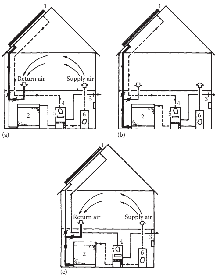
FIGURE 5.15 Schematic diagram of operating modes of solar air system: (a) space heating from collector; (b) storing solar heat, and (c) space heating from storage. The components are (1) collector, (2) storage, (3) control, (4) fan, (5) hot-water preheater (optional), and (6) backup heater. (Courtesy of the Solaron Corp.)
