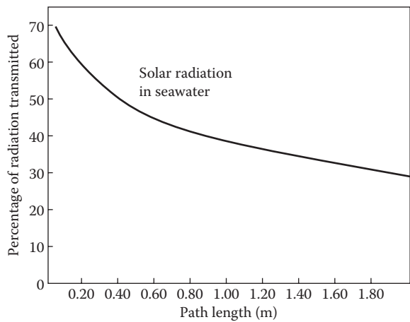
FIGURE 8.61 Transmittance of water to solar radiation as a function of the thickness of the water layer. See Table 8.10 for numerical values.
