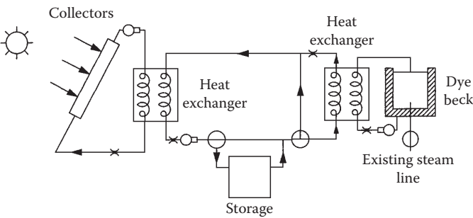
FIGURE 5.27 Schematic of solar energy system at Riegel Textile Corporation plant at LaFrance, South Carolina.
