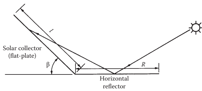
FIGURE 3.31 Horizontal reflecting surface used to boost flat-plate collector performance.
