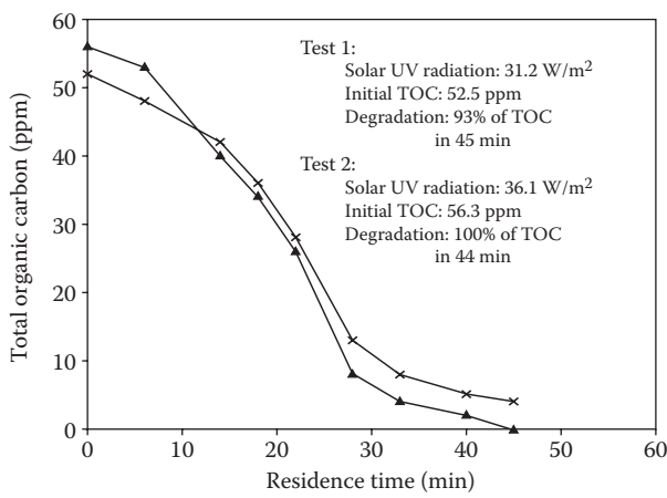
FIGURE 10.17 Treatment of industrial wastewater containing organic contaminants. (From Blanco, J., and S. Malato., Solar photocatalytic mineralization of real hazardous waste water at pre-industrial level. In Solar Engineering 1994 , D.E. Klett, R.E. Hogan, and T. Tanaka, eds. pp. 103–109, 1994.)
