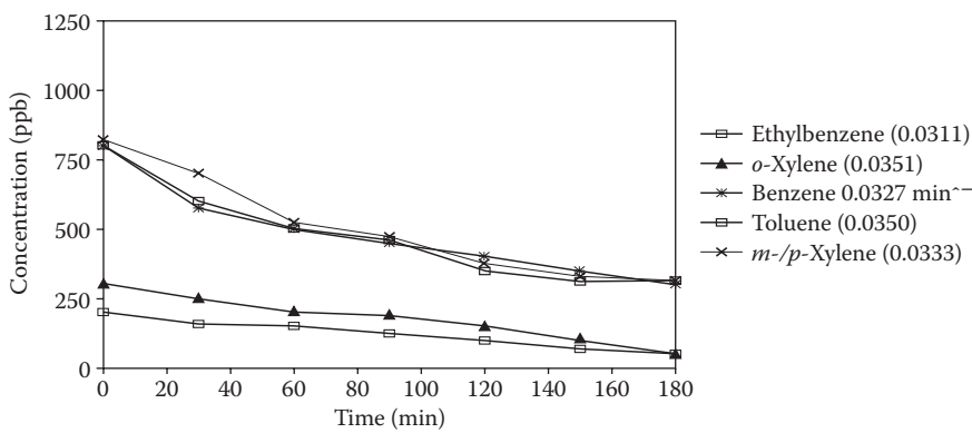
FIGURE 10.8 Destruction of BTEX in groundwater at Tyndall AFB using nonconcentrating tubular reactors. (From Goswami, D.Y. et al., Solar photocatalytic treatment of groundwater at Tyndall AFB, field test results. Solar 1993, Proceedings of the American Solar Energy Society Annual Conference , pp. 235–239, 1993.)
