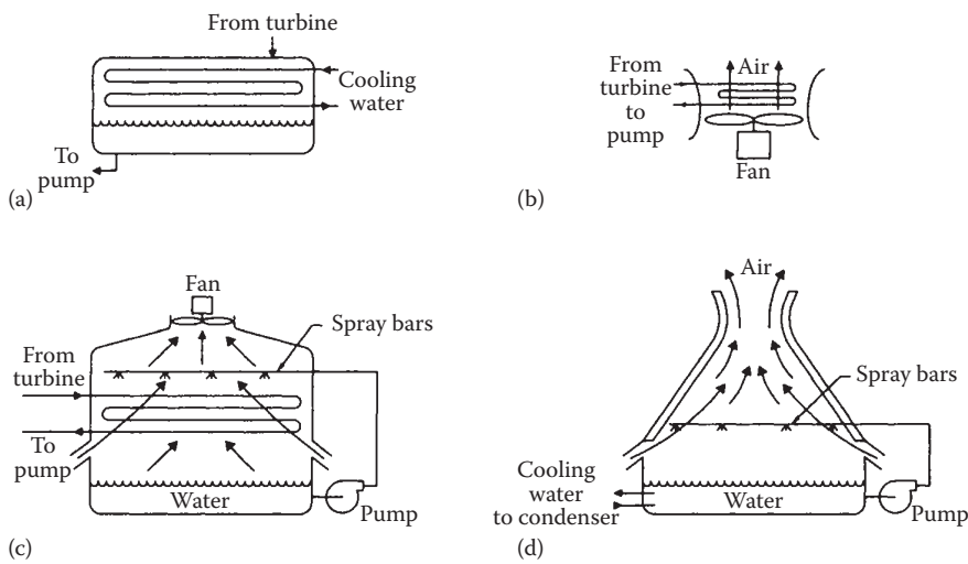
FIGURE 8.10 Types of condenser or heat rejection used in Rankine cycle solar power systems: (a) tube-and-shell condenser, (b) dry cooling tower, (c) wet cooling tower, and (d) natural-draft cooling tower. (Stine, W.B. and R.W. Harrigan: Solar Energy Fundamentals and Design: With Computer Applications . 1985. Copyright Wiley-VCH Verlag GmbH & Co. KGaA. Reproduced with permission.)
