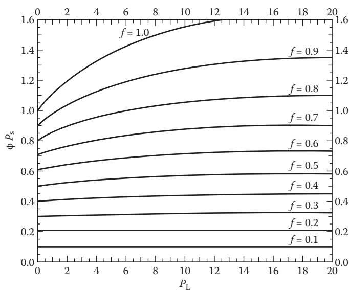
FIGURE 5.23 The \bar{\phi}, f chart used to calculate average, monthly solar fraction f (f_s) of solar thermal systems.
