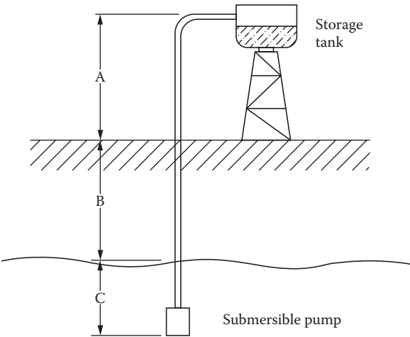
FIGURE 9.32 Water pumping using a submersible pump.
