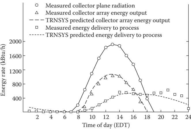
FIGURE 5.28 Actual and predicted system operation, August 16, 1983.
