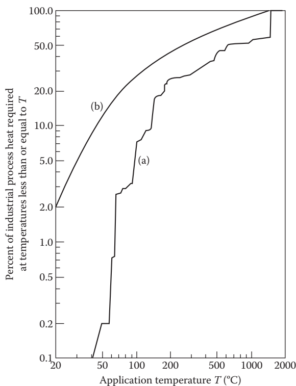
FIGURE 5.24 Distribution of US process heat use by required temperature level: (a) heat requirements; (b) IPH requirements plus preheat from 15°C.
