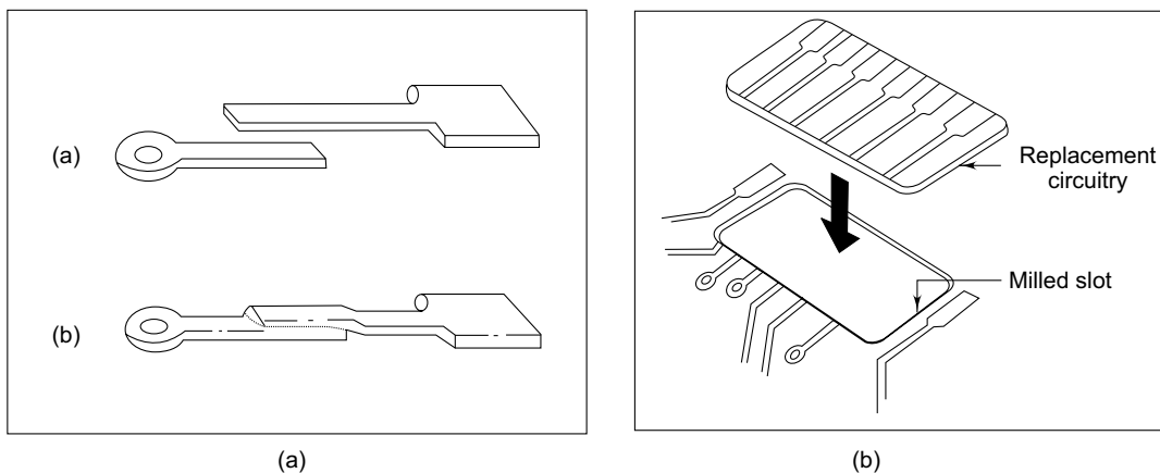
Fig. 13.53 (a) working repair (b) serviceable repair
