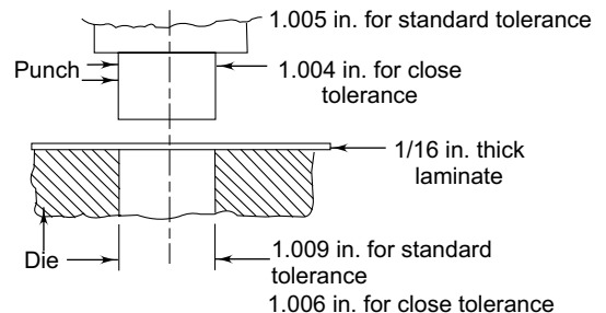
Fig. 10.2 Proper tolerance of a punch and die
