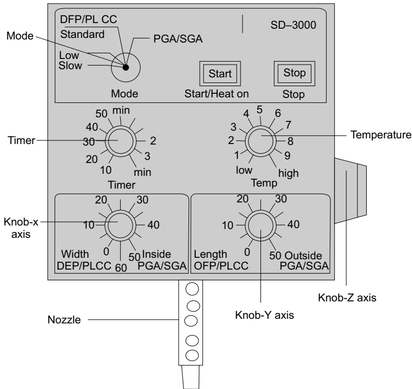
Fig. 13.55 Controls on typical re-work station
