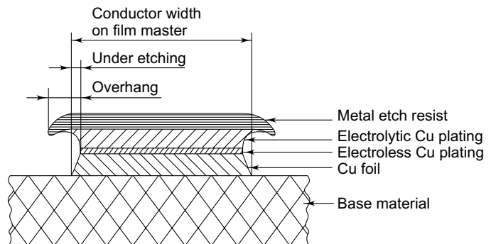
Fig. 9.10 Overhang and undercut in pattern-plated PCBs
