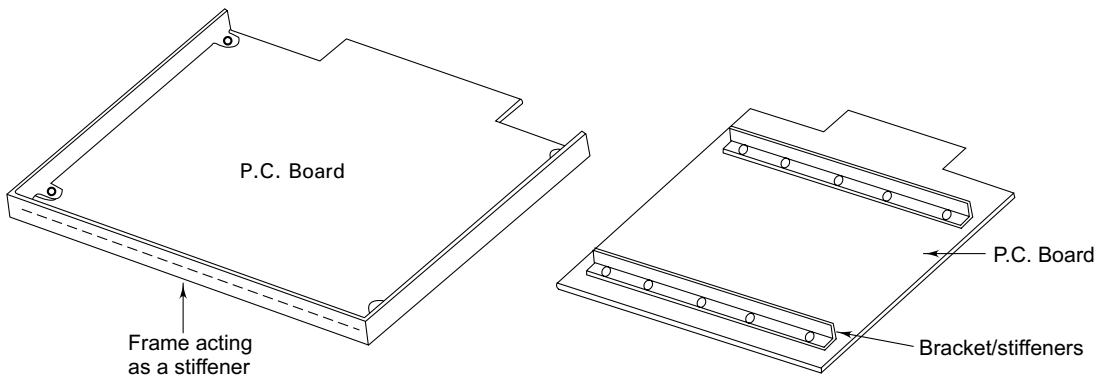
Fig. 3.4 Use of stiffeners for mounting of printed circuit boards
