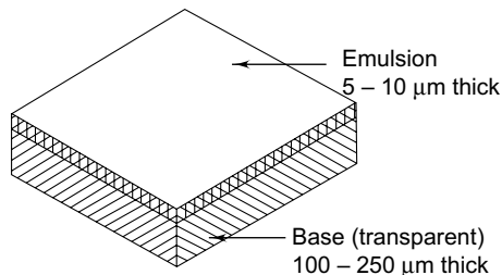
Fig. 5.17 Components of photographic film
