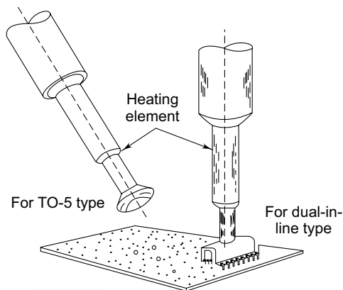
Fig. 13.52 Special de-soldering tip for integrated circuits
