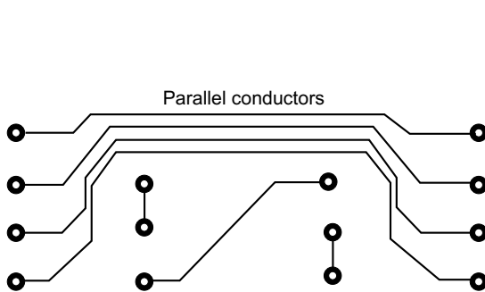
Fig. 5.7 Conductor routing — parallel pattern
