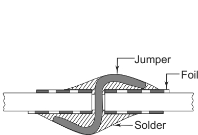
Fig. 1.3 Interconnection with clinched jumper
