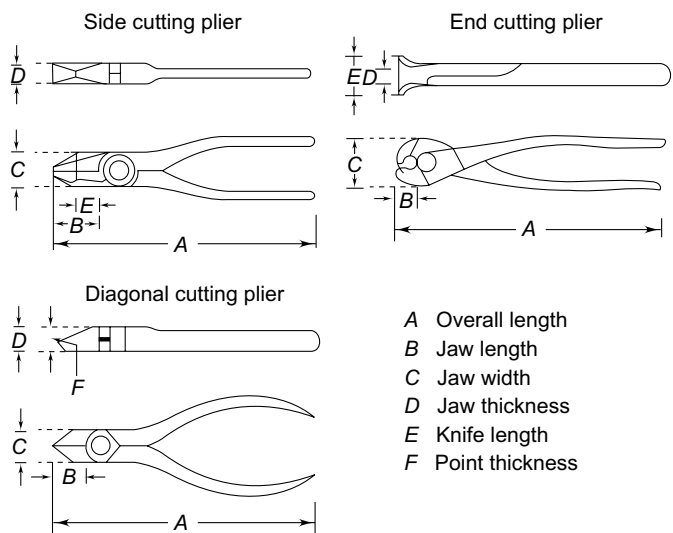
Fig. 13.9 Side cutter
