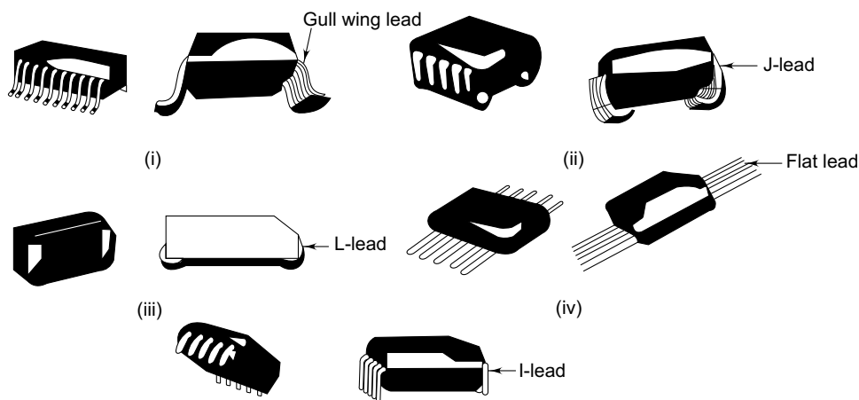
Fig. 2.80 Shapes of components with different lead styles (i) gull wing lead: metal lead that bends down and away (ii) J-lead: metal lead that bends down and underneath a component in the shape of letter J (iii) L-lead: inward formed underneath a component (iv) flat lead: protrudes directly out from the body of the component (v) I-lead: a through-hole lead cut short for surface mounting
