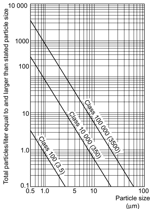
Fig. 15.9 Particle size distribution for three clean room standard classifications (redrawn after Haskard, 1998)
