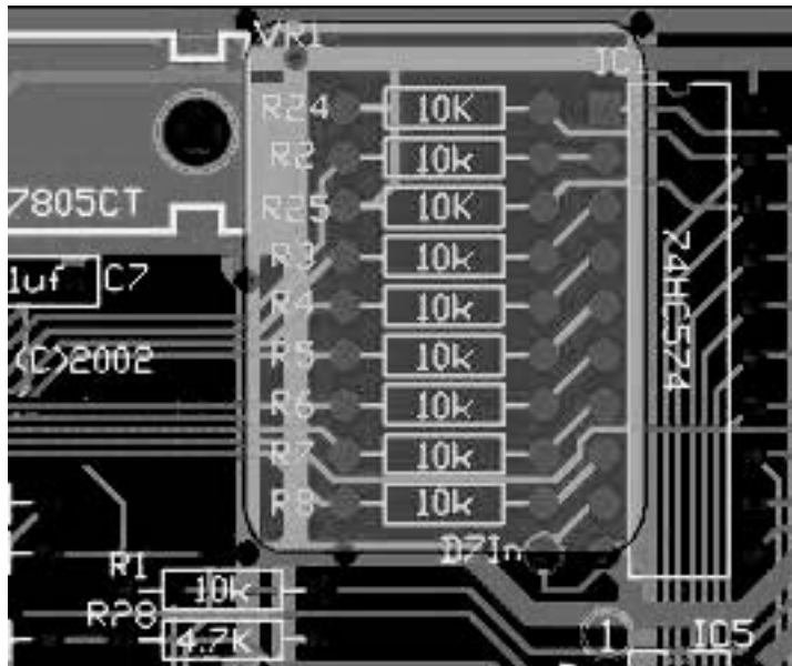
Fig. 4.42 The concept of loop area for EMI compliance in PCB Design (courtesy M/s AirBorn Electronics)
