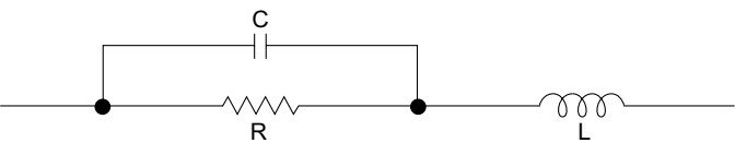
Fig. 2.10 Lumped model of a resistor C = 0.1-2 pf, L = 0.1 \mu H (for a leaded component)
