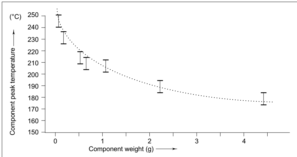
Fig. 13.35 Component peak temperature vs component mass during 1R processing (after Reithinger, 1991)
