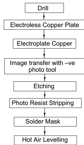
Fig. 8.25 Process sequence for solder mask over bare copper by tenting process
