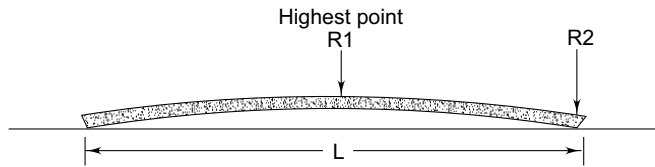
Fig. 14.18 Bow measurement
