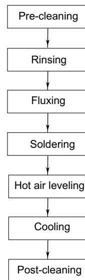
Fig. 8.6 Hot air levelling system
