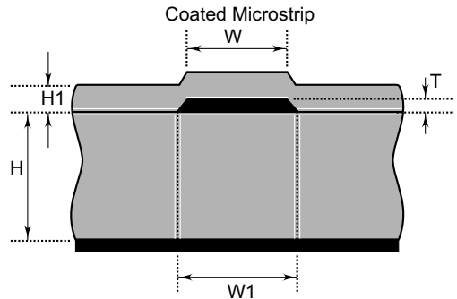
Fig. 4.30 Coated microstrip
