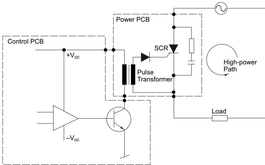
Fig. 4.36 Division of circuit into high- and low-power parts (after Bosshart, 1983)
