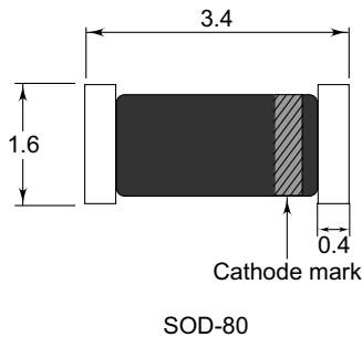
Fig. 2.89 Small outline diode package
