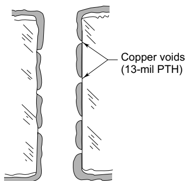
Fig. 8.7 PTH vertical cross-section illustrating copper voids
