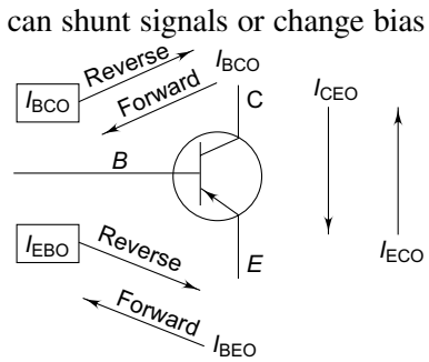
Fig. 2.42 Leakage paths in a transistor
