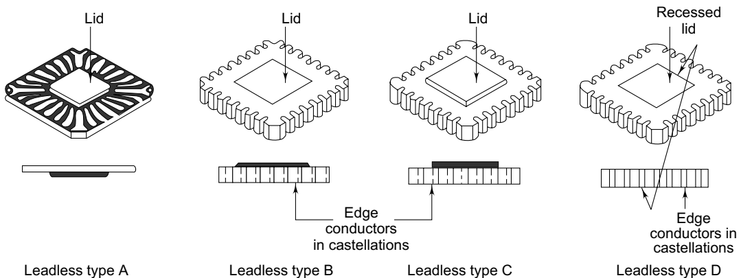
Fig. 2.91 Leadless ceramic chip carrier (LCCC)
