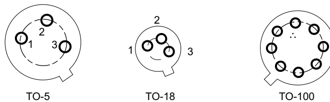
Fig. 3.16 Footprints TO-100/TO-5/TO-18
