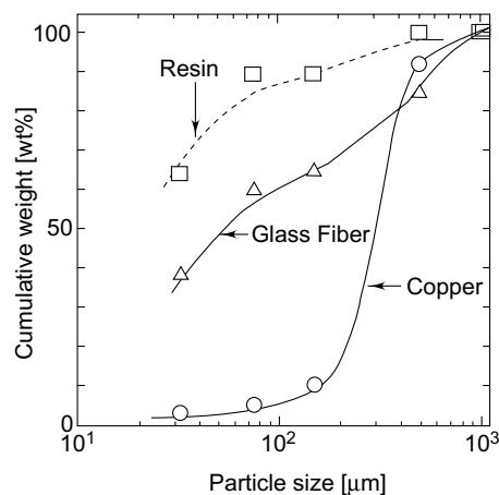
Fig. 15.13 Size distribution of pulverized PCB components (redrawn after Yokoyama and Iji, 1995)
