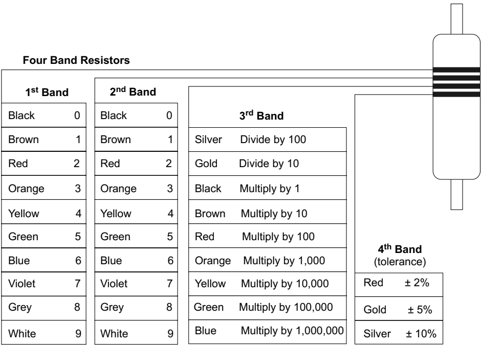
Fig. 2.11 Colour code for carbon composition and metal film resistors—four band colour code
