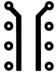
Fig. 14.24 Insulation resistance, dielectric withstanding voltage and moisture resistance test patterns
