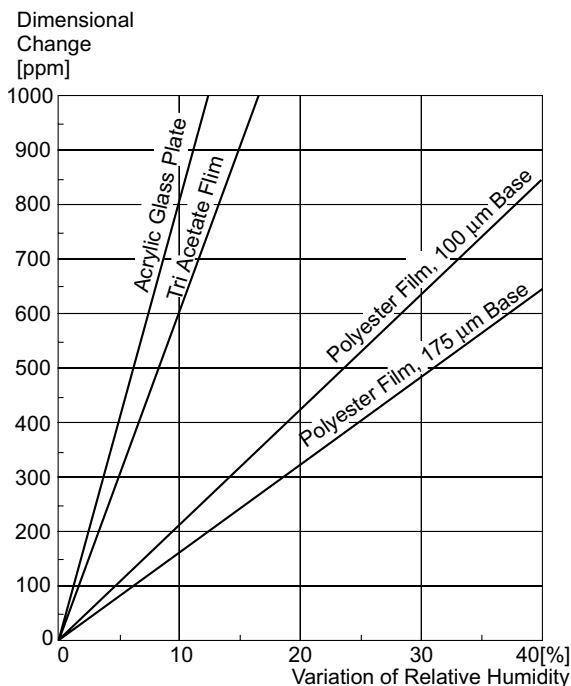
Fig. 5.19 Typical values for dimensional changes caused by a change in the relative humidity (redrawn after Bisshart, 1983)
