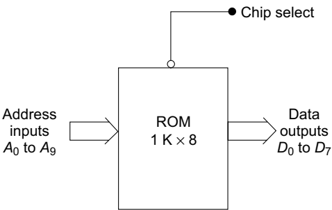
Fig. 2.74 Typical symbol of ROM
