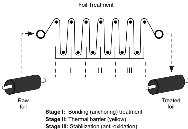
Fig. 12.5 Stages for treatment and stabilization of foils (after Savage, 1992)
