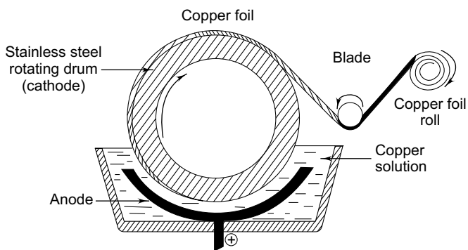
Fig. 6.1 Cell for manufacturing electrolytic copper foil. Cathode is made of stainless steel and anode of copper
