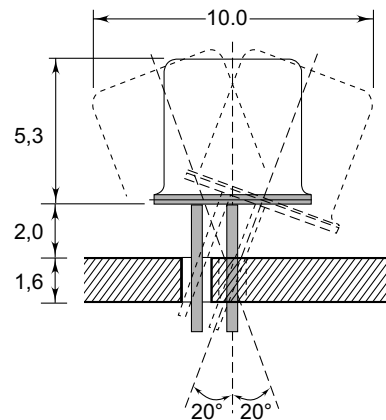
Fig. 3.13 Deviation from the vertical of a TO-18 package, mounted at a distance of 2 mm from the PCB. If the hole diameter is 1mm, the deviation can be up to 20^\circ without any deviation of the leads
