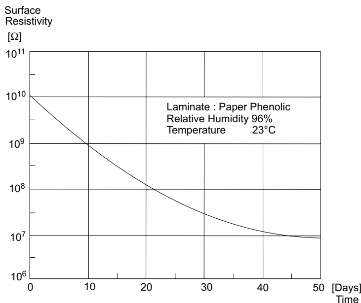
Fig. 6.10 Impact of moisture on surface resistivity of paper phenolic laminates (redrawn after Bosshart, 1983)
