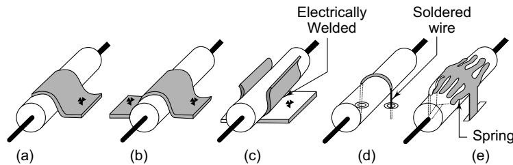
Fig. 3.14 Common methods of fastening heavy components to the board (a) single-sided clamp (b) double-sided clamp (c) electrically welded holder (d) fixing with soldered wire (e) holding with a spring loaded tape
