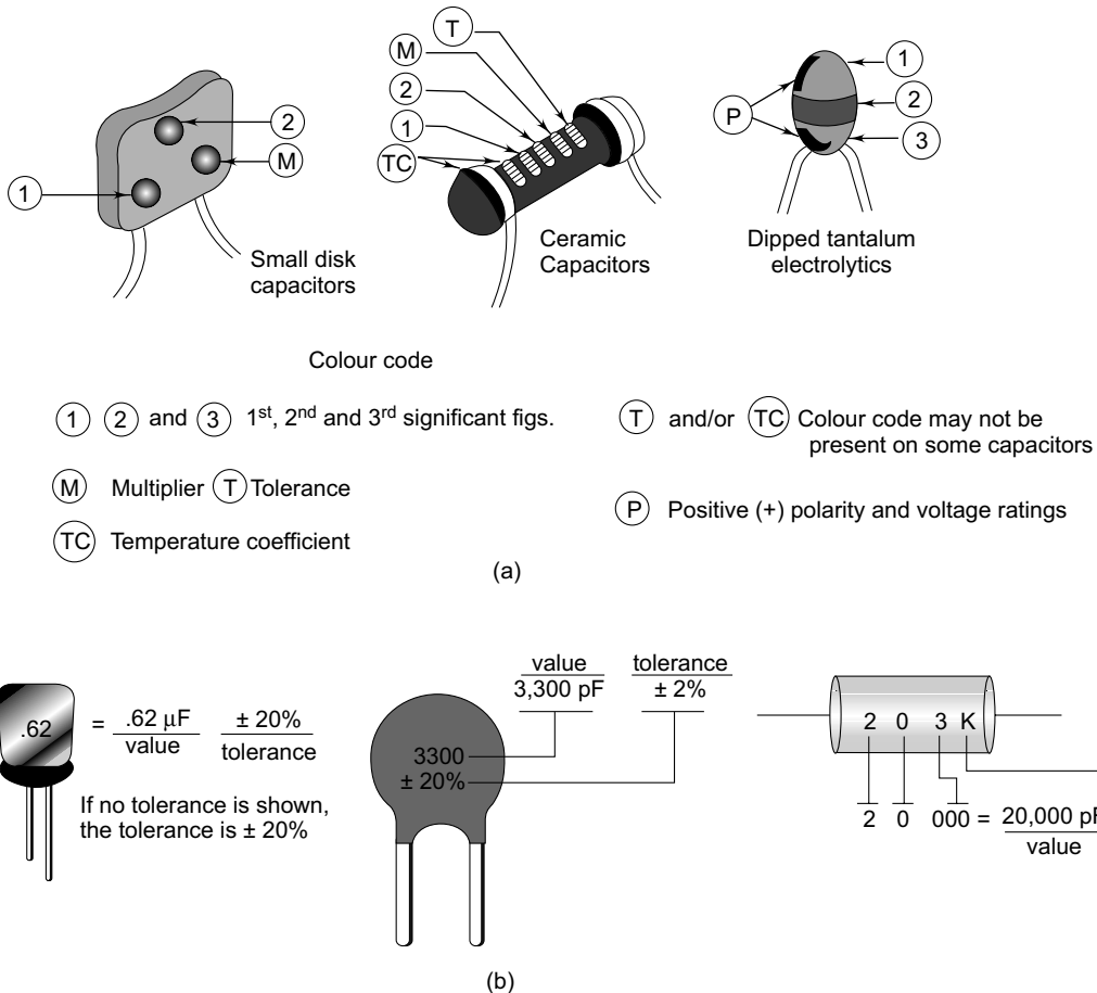
Fig. 2.19 (a) capacitor colour code; and (b) code for numbered capacitors
