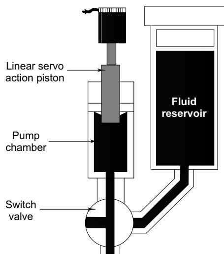
Fig. 13.23 (c) Positive displacement linear pump
