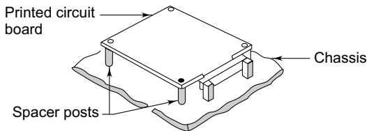
(b) Mount on tapered spacers Any size board can be accommodated by this simple mounting. It can be a space-saver on walls and doors of enclosures.
