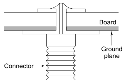
Fig. 4.27 Use of coaxial connectors inserted through the ground plane on a PCB
