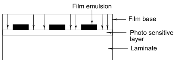
Fig. 7.13 (b) Exposing photo sensitive resist
