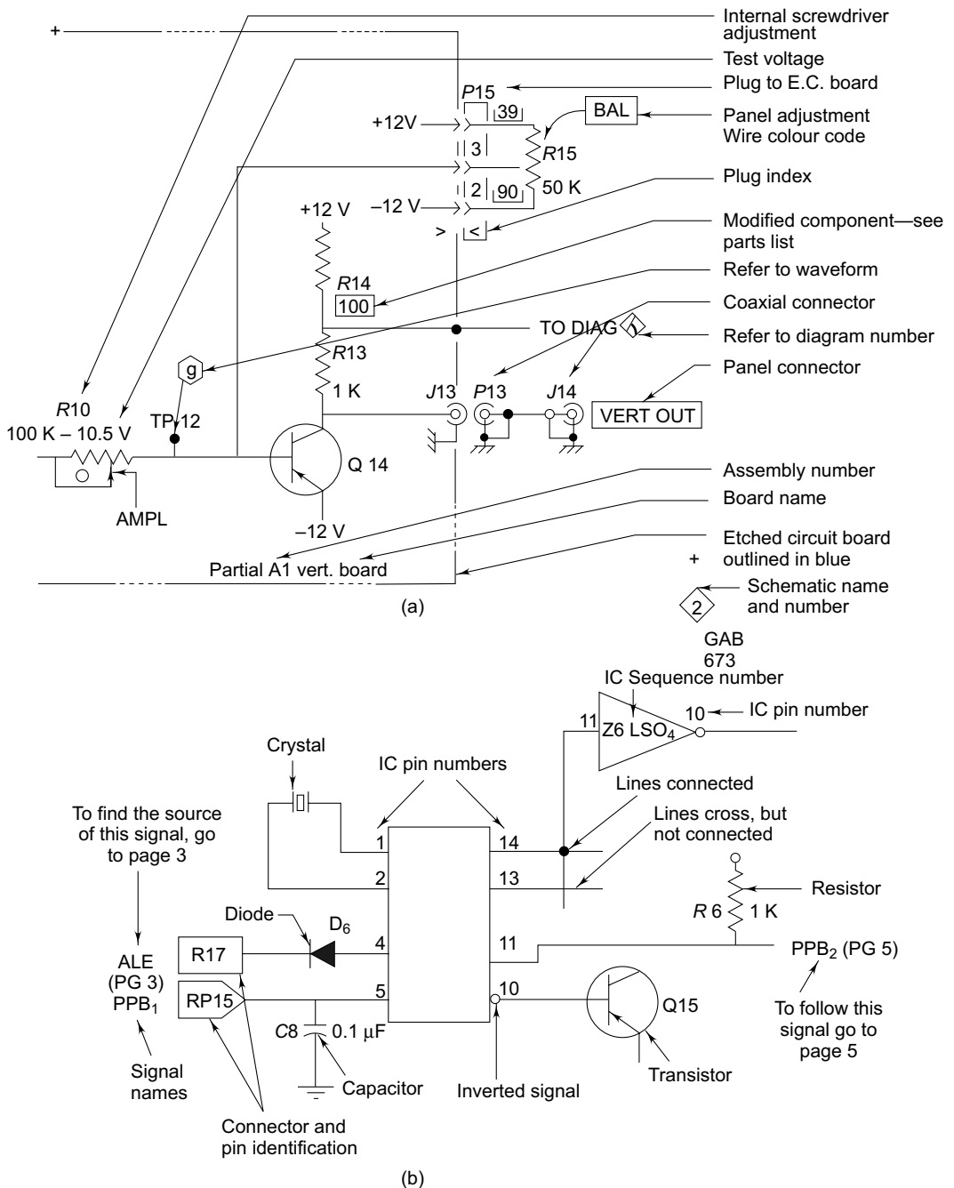
Fig. 3.2 Schematic circuit with symbols as per the American National Standard Institute (a) Circuit with discrete components (b) Circuit with integrated circuit
