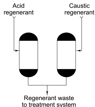
Fig. 15.3 Ion exchange system: regeneration system
