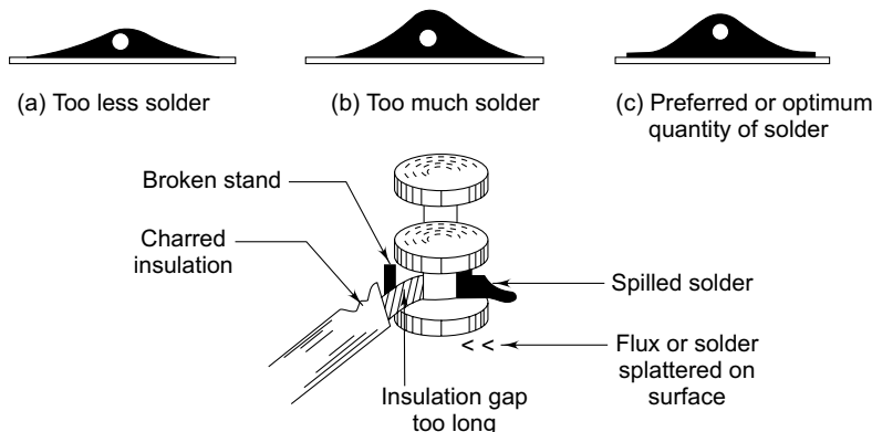
Fig. 13.42(b) Bad soldering examples
