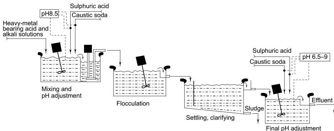
Fig. 15.7 Principle of heavy metal precipitation (adopted from Bosshart, 1983)
