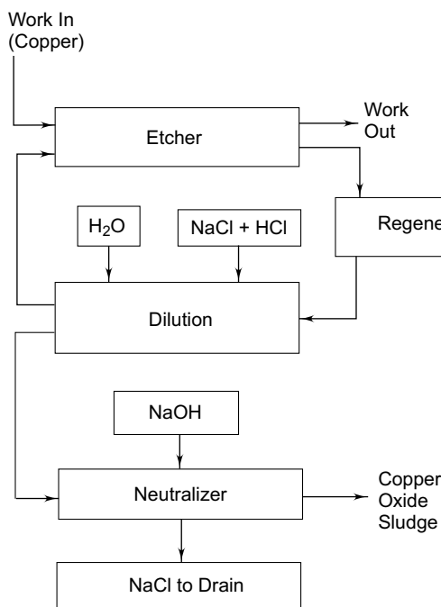
Fig. 9.3 Cupric chloride chlorination regeneration system (after Coombs, 1988)
