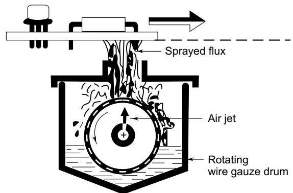
Fig. 13.27 Spray fluxing arrangement
