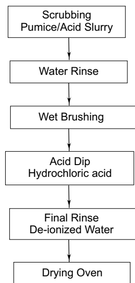
Fig. 7.1 Simple manual cleaning process
