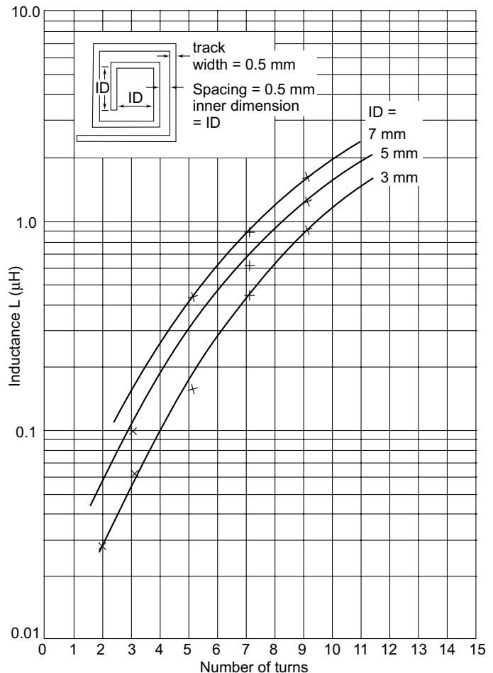
Fig. 4.32 Inductance values and shape of printed flat spiral inductors transmission line connecting a source to a load (redrawn after Haskard, 1998)
