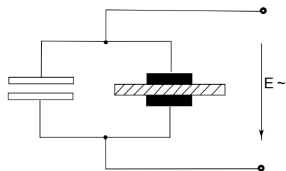
Fig. 6.4 Electrode arrangement for testing dielectric constant
