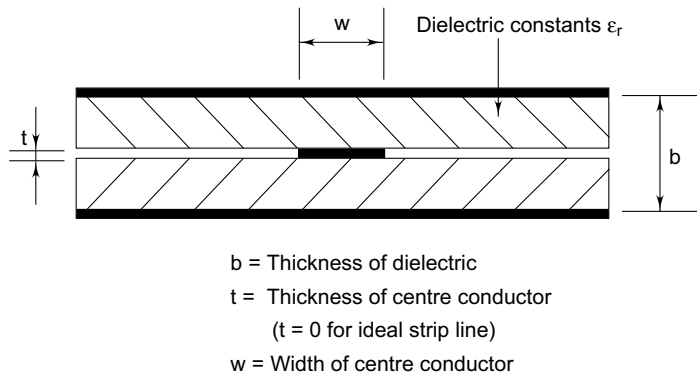
Fig. 4.21 Practically realized strip line
