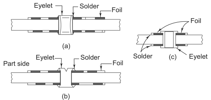
Fig. 1.4 Interconnections with (a) funnel-flanged eyelet (b) split funnel-flanged eyelet (c) fused-in-place eyelet
