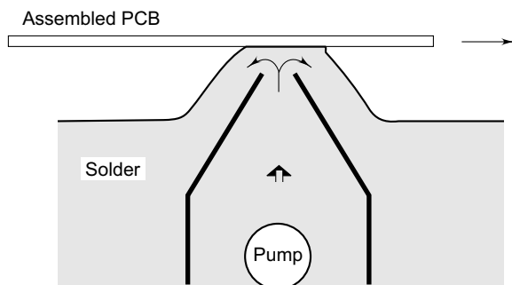
Fig. 13.28 Wave soldering machine
