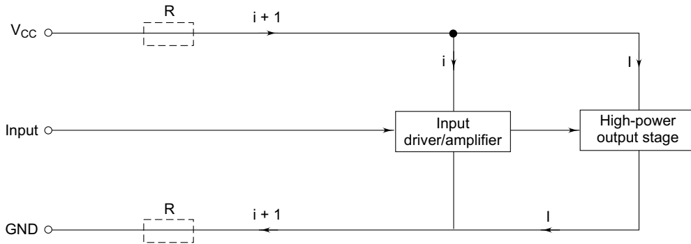
Fig. 4.8 Multi-stage amplifier with high-power output stage: providing separate power supply and ground conductors to avoid common supply/ground path
