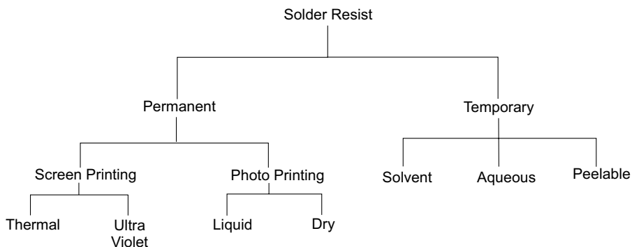
Fig. 8.20 Types of solder resist
