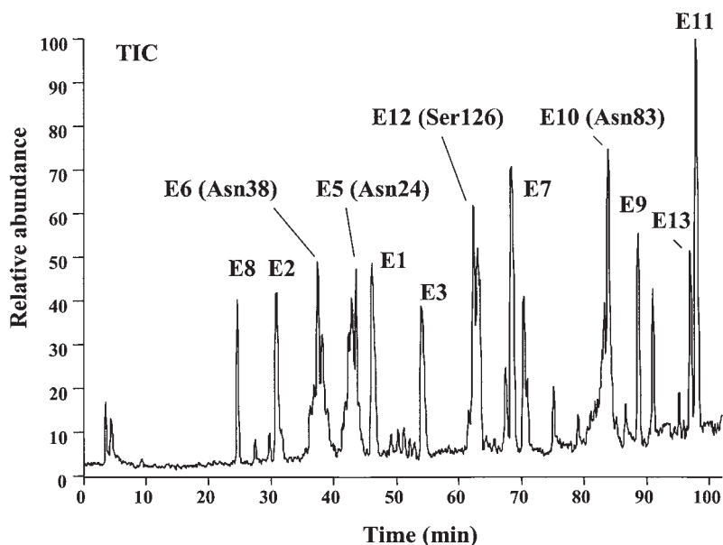
Fig. 3. Glu-C peptide/glycopeptide map of erythropoietin. Column, Vydac 218TP52 (250 \times 2.1 mm); eluent A, 0.05% TFA; eluent B, 0.05% TFA/50% (v/v) acetonitrile; gradient, 1 to 90% of B in 130 min; flow rate, 0.2 mL/min; acquired mass, m/z 550–2400; ion mode, negative; sample amount, 50 \mu g erythropoietin.
