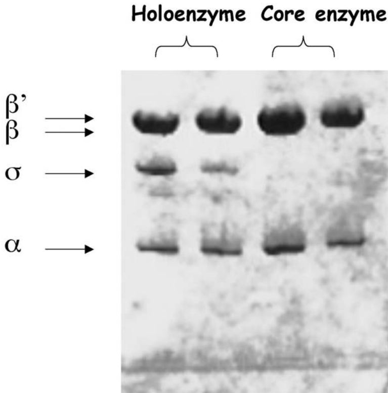
Fig. 2. SDS-PAGE analysis of RNA polymerase. RNA polymerase isolated as described is applied to a 10–15% acrylamide gel that allows separation of the four subunits [ (\alpha)_2\beta'\beta\sigma ]. Approx 0.5 \mu\text{g} of total protein is present in each lane. The gel is visualized by staining with Coomassie blue.
