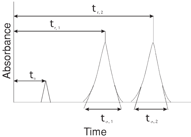
Fig. 1. Diagram of the retention parameters that describe a chromatographic separation. The retention time of a nonretained solute is denoted by t_o , while the retention times of two retained solutes, 1 and 2, are given by t_{r,1} and t_{r,2} . The corresponding peak-widths for solutes 1 and 2 are denoted \sigma,1 and \sigma,2 , and together with the retention times are they used to determine the resolution of the separation according to Eq. 9 .
