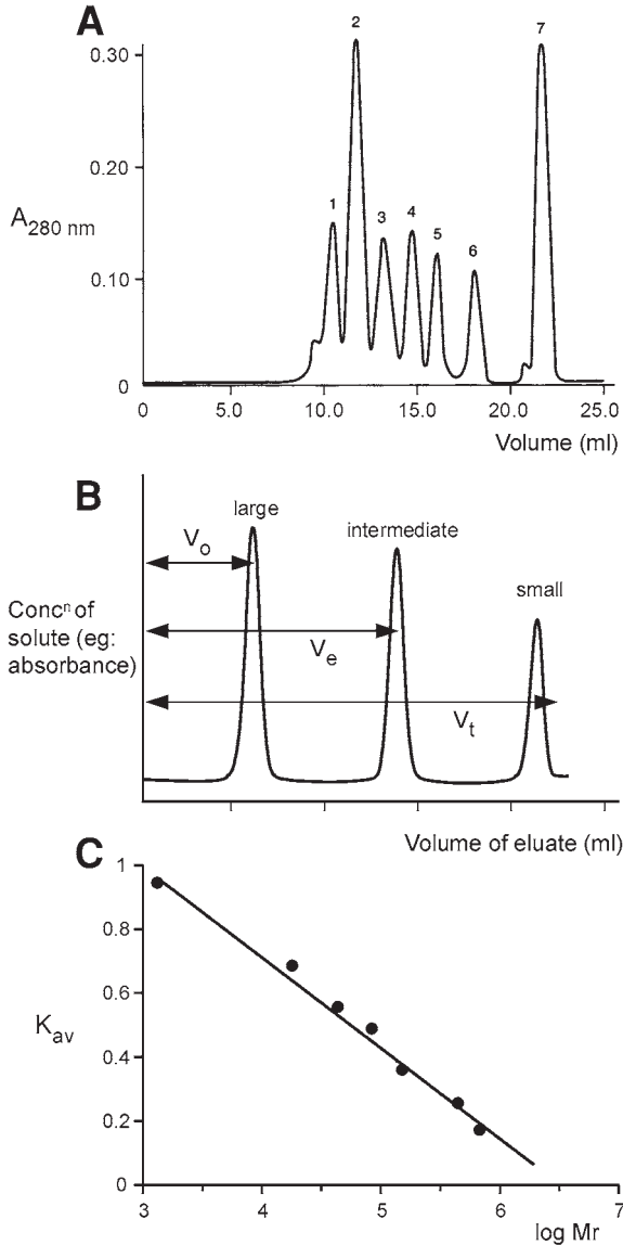
Fig. 1. ( continued ) proteins ( see panel A) under optimal conditions for flow rate and sample size. From these measurements the coefficient K_{av} can be derived, K_{av} = (V_e - V_0)/(V_t - V_0) . (C) The selectivity curve for a particular gel filtration media is a plot of K_{av} vs \log molecular weight, and the data shown here has been derived from panel A. Selectivity curves as provided by the manufacturer are used to choose the gel filtration media that best suits the application, whereas in the laboratory they are useful for estimation of the molecular mass of an unknown protein.
