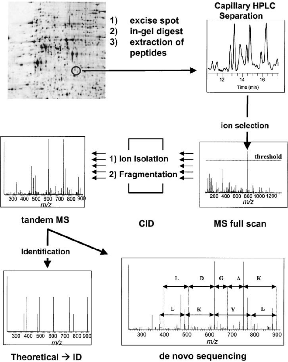
Fig. 1. Overview of the process of proteome analysis by capillary HPLC-MS/MS.
