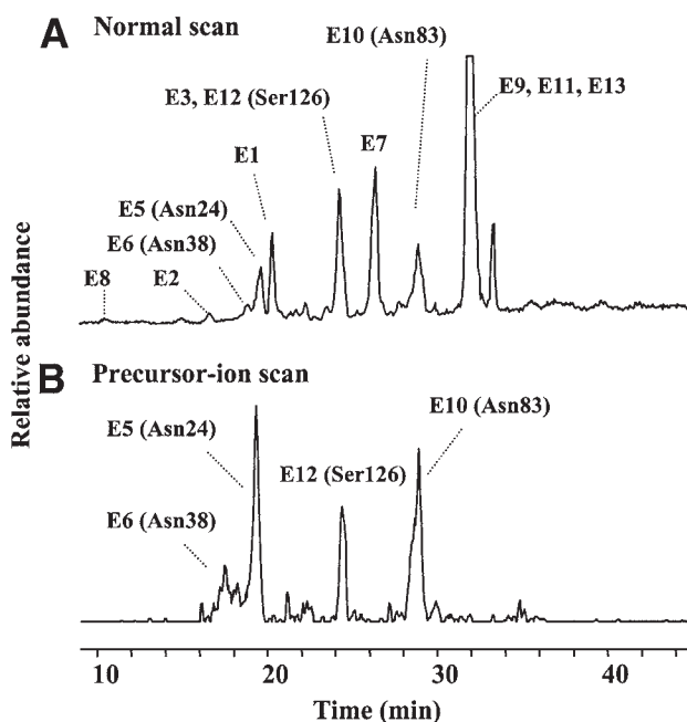
Fig. 6. Normal scan ( A ) and precursor-ion scan ( B ) of Glu-C-digested EPO. Column, Magic C18 (150 × 1 mm); eluent A, 0.05% TFA/2% acetonitrile; eluent B, 0.05% TFA/80% acetonitrile; gradient, 5 to 45% of B in 40 min; flow rate, 50 \mu L/min; acquired mass (Q1), m/z 400–2400. Set mass (Q3), m/z 204; ion mode, positive; sample amount, 2 \mu g (A) and 8 \mu g (B) of erythropoietin.
