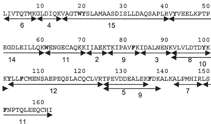
Fig. 2. Identification of the peaks separated in Fig. 1 . Aromatic residues are shown in bold. The two peptides labeled 11 are linked by a disulphide bond (Cys66–Cys160). Peptide 12 has an internal disulphide bond. The peptides labeled 9 elute very close together (see Fig. 1 ).
