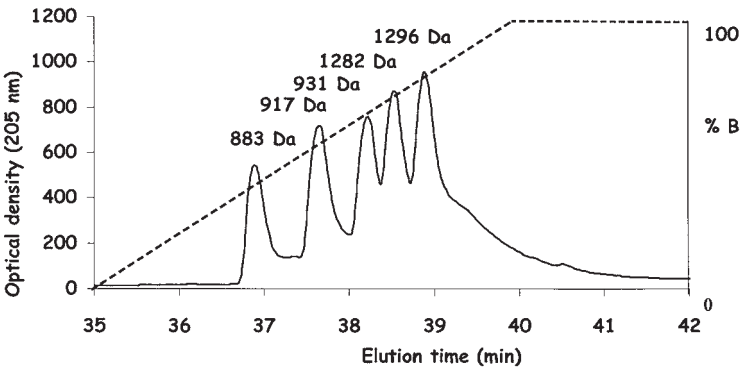
Fig. 4. Separation of peptides by RP chromatography. A mixture of peptides (2.0 \mu L of 10 ng/ \mu L) is applied to a 5 \mu L 200 Å, 0.3 mm × 150 mm C18 MAGIC column (Michrom BioResources Inc.) on an Ettan LC. The gradient from 3% acetonitrile, 0.05% TFA to 70% acetonitrile, 0.05% TFA allows separation of the following peptides which in this instance are identified on line using an ESIToF mass spectrometer from Amersham Biosciences. 883 Da, RVYVHPI; 917 Da, RVYVHPF; 931 Da, RVYIHPF; 1282 Da, QRVYVHPFHL; 1296 Da, QRVYIHPFHL.
