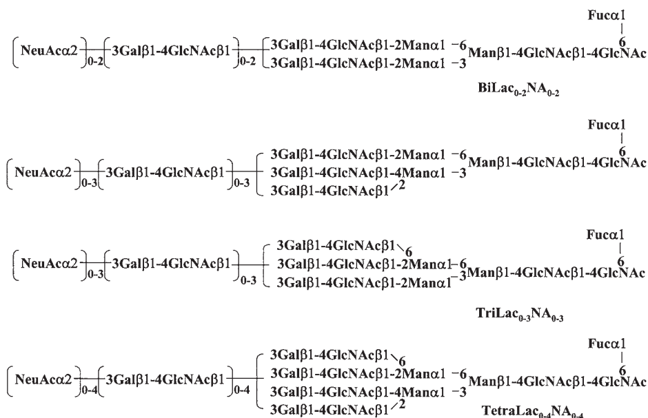
Fig. 2. Carbohydrate structures of erythropoietin. Bi, biantennary; Tri, triantennary; Tetra, tetraantennary; Lac, N -acetylglucosamine; NA, NeuAc.
