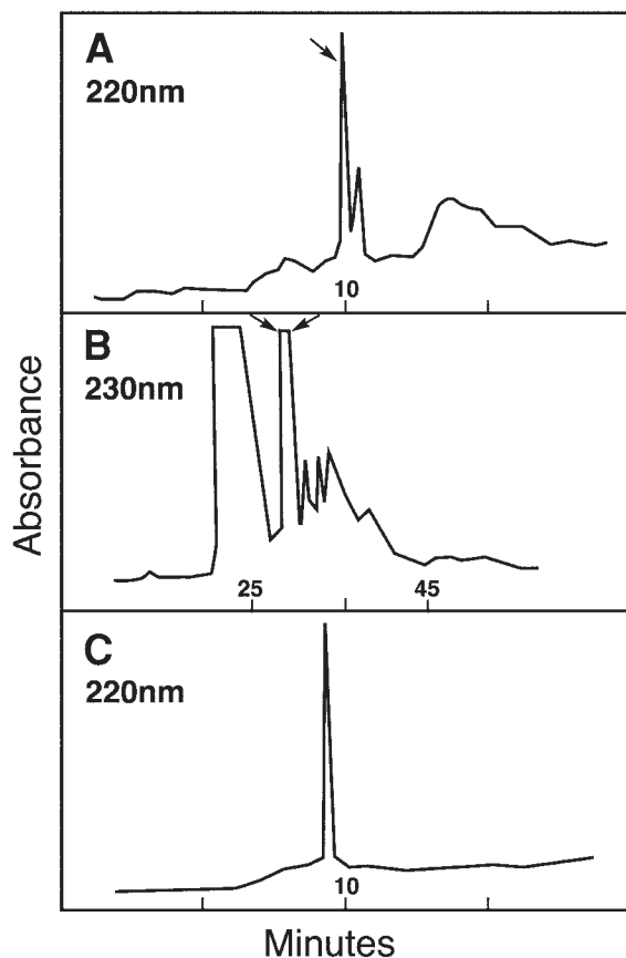
Fig. 5. c(RSRNR): (A) Crude analytical trace: TFA buffer, 1.5 mL/min, 0–60%B over 30 min. (B) Prep trace, 60 mg sample: Phenomenex Aqua semiprep column, 0–25%B over 50 min. (C) Pure analytical trace: TFA buffer, 1.5 mL/min, 0–60%B over
