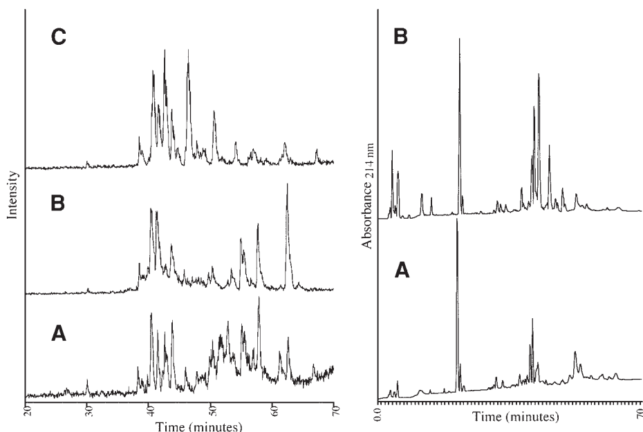
Fig. 3. A comparison of the RP-HPLC chromatograms from the juvenile, female, and mature male venom of Atrax sp.: Illawarra. (A) RP-HPLC/ESI-MS (left panel) and RP-HPLC/UV (right panel) chromatogram data obtained for the female Atrax sp.: Illawarra venom sample. (B) RP-HPLC/ESI-MS and RP-HPLC/UV chromatogram data obtained for the juvenile male Atrax sp.: Illawarra venom sample. (C) RP-HPLC/ESI-MS chromatogram data for the venom sample obtained from the Atrax sp.: Illawarra postmaturing moult mature male specimen.
