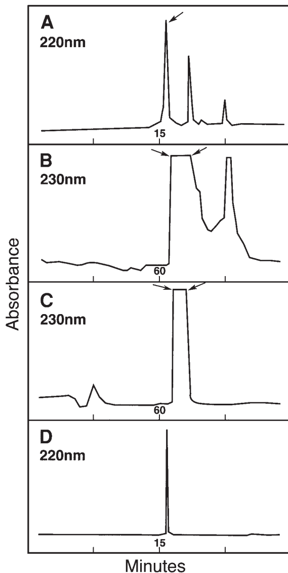
Fig. 4. Conotoxin MII: (A) Crude analytical trace (1 disulfide bond, 2 \times Cys(Acm)): TFA buffer, 1.5 mL/min, 0–60%B over 30 min. (B) Prep trace, 1.8 g sample (1 disulfide bond, 2 \times Cys(Acm)): TFA buffer, 30 mL/min, 0–50% B over 100 min. (C) Prep trace (2 \times disulfide bonds), 180 mg sample: 25 mM ammonium acetate buffer, 30 mL/min, 0–12%B over 30 min, 12%B isocratic 30–40 min, 12–40%B 40–100 min. (D) Pure analytical trace: TFA buffer, 1.5 mL/min, 0–60%B over 30 min.
