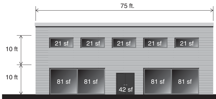
FIGURE 16-A-2. South elevation for building with proposed openings.
