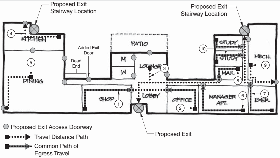
EXAMPLE PROJECT FIGURE 10-2. The egress paths for the first story. Each path is tagged with a number, which corresponds to the information indicated in the table below.
