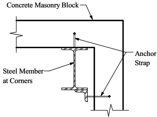
FIGURE 8.2: Masonry Anchors
