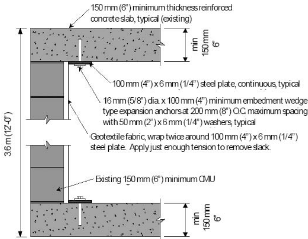
FIGURE 10.16: Geotextile Retrofit Behind Masonry Non-Load Bearing Wall
