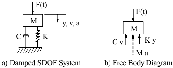
FIGURE 6.3: SDOF Model for Dynamic Analysis
