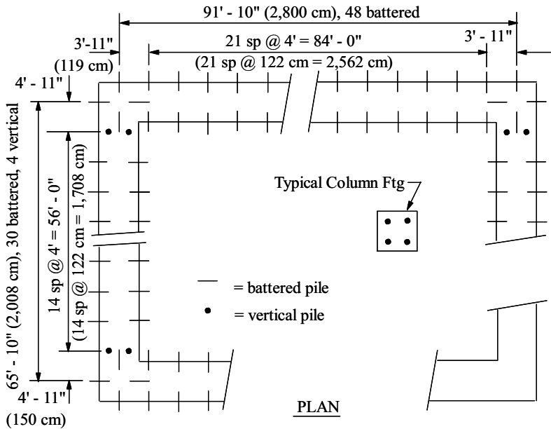
FIGURE 11.3: Foundation Plan
