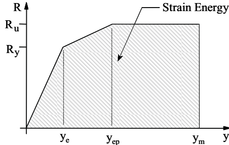
FIGURE 5.1: Typical Resistance-Deflection Curve
