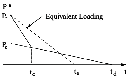
FIGURE 3.7: Front Wall Loading
