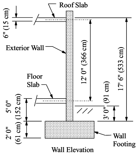
FIGURE 11.2: Wall Elevation
