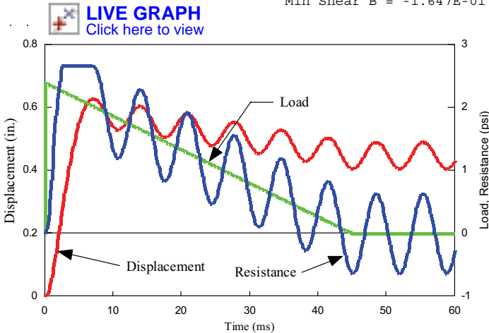
FIGURE 12.4: Wall Panel Numerical Integration
