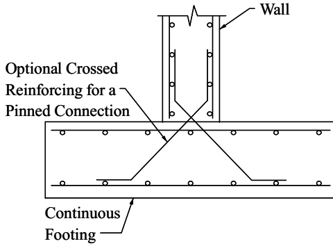
FIGURE 8.10: Cast-in-Place Wall to Foundation Joint
