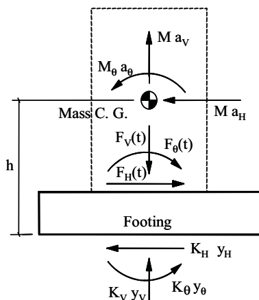
FIGURE 7.4: External Forces on a Foundation (from UFC 3-340-02)
