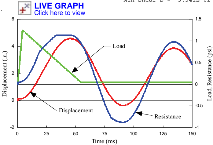
FIGURE 12.5: Roof Purlin Numerical Integration
