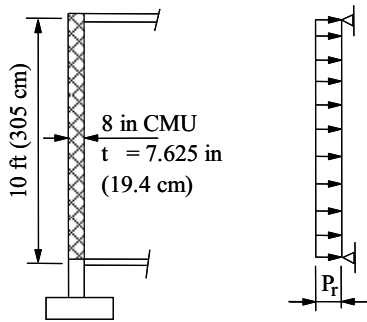
FIGURE 13.2: Wall Section
