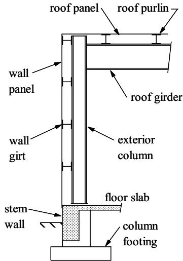
FIGURE 12.2: Wall Elevation
