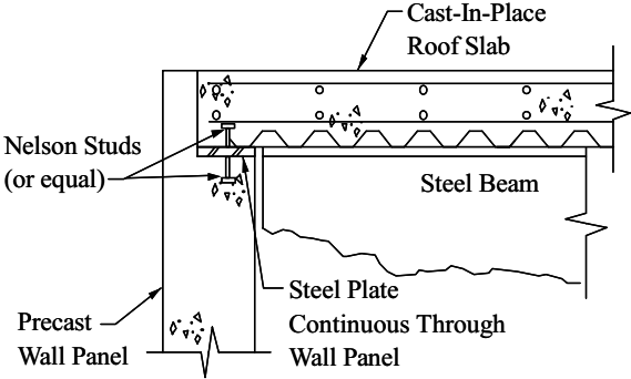
FIGURE 8.5: Precast Panel Connection to Roof Slab
