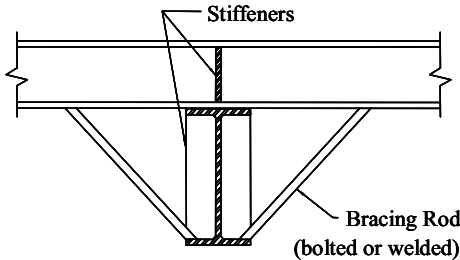
FIGURE 10.3: Typical Bracing Details
