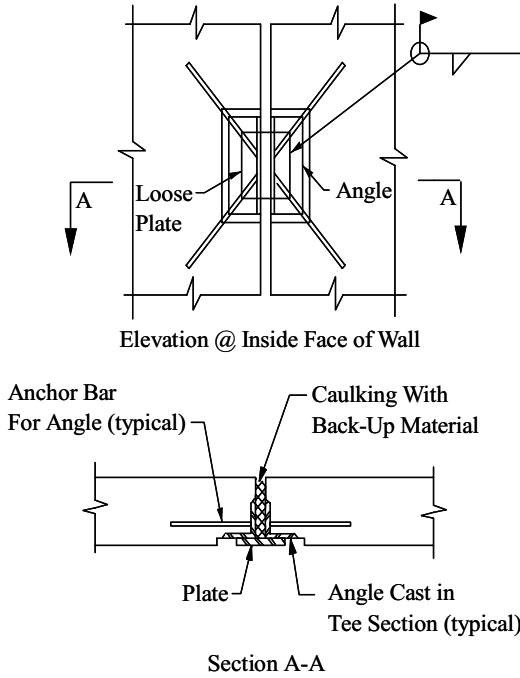
FIGURE 8.6: Precast Panel Vertical Joint
