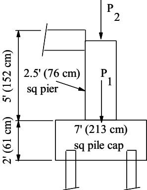
FIGURE 11.6: Column Foundation
