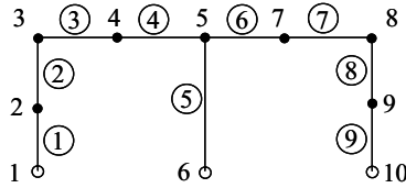
FIGURE 12.10: MDOF Model
