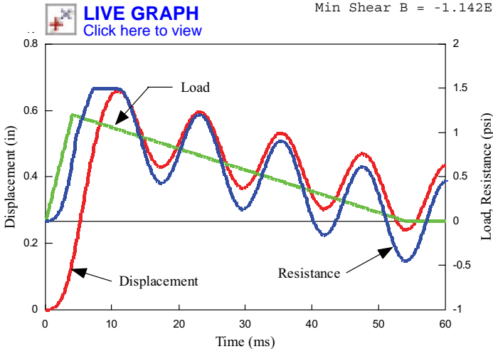
FIGURE 12.3: Roof Deck Numerical Integration
