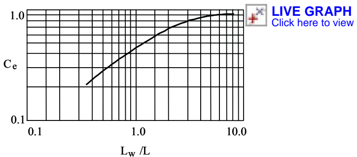
FIGURE 3.9: Effective Overpressure Values (from UFC 3-340-02)
