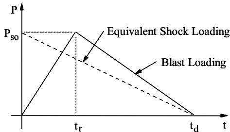
FIGURE 3.4: Idealized Equivalent Pressure Load
