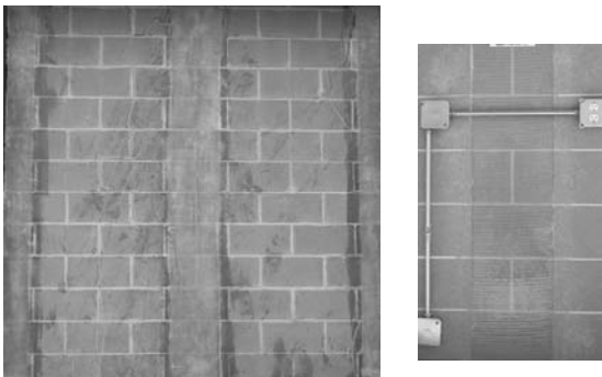
FIGURE 10.12: FRP Strips on Walls and Around Existing Interferences
