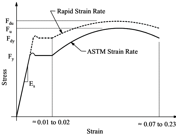
FIGURE 5.5: Effect of Strain Rate on Stress-Strain Curve for Steel (from UFC 3-340-02)
