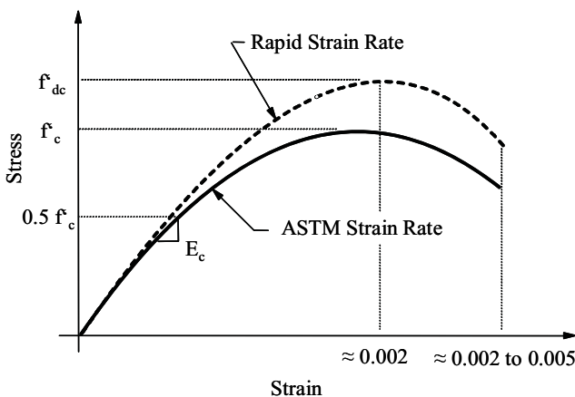
FIGURE 5.6: Effect of Strain Rate on Stress-Strain Curve for Concrete (from UFC 3-340-02)
