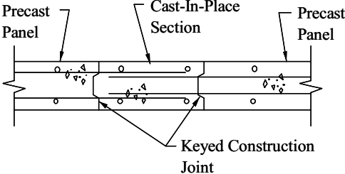
FIGURE 8.9: Precast Panel Vertical Joint
