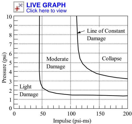
FIGURE 6.7: P-I Versus Structural Damage
