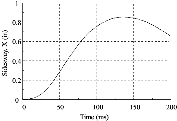
FIGURE 12.12: Plot of Node 3 Sidesway Response
