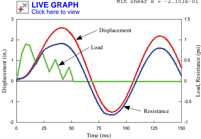
FIGURE 12.6: Wall Panel Numerical Integration
