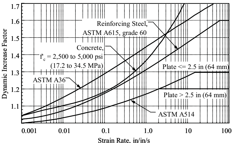
FIGURE 5.7: Effect of Strain Rate on Dynamic Material Strength
