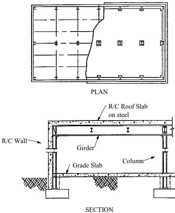
FIGURE 4.3: Cast-in-Place Concrete Wall Building (steel frame)
