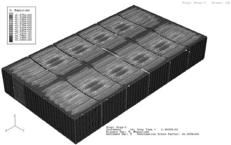
FIGURE 4.8: Deflected Shape under Roof Blast Loading on Six-Module Complex
