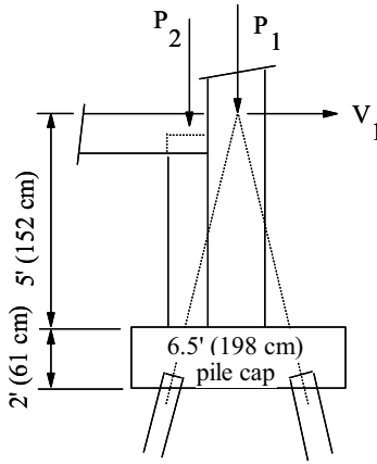
FIGURE 11.4: Side Wall Elevation
