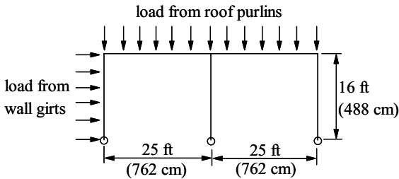
FIGURE 12.9: Frame Elevation
