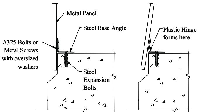
FIGURE 10.5: Base Angle Detail for Flexible Connection
