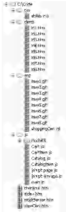
Figure 10-6. Directory layout of the Shopping Cart application
