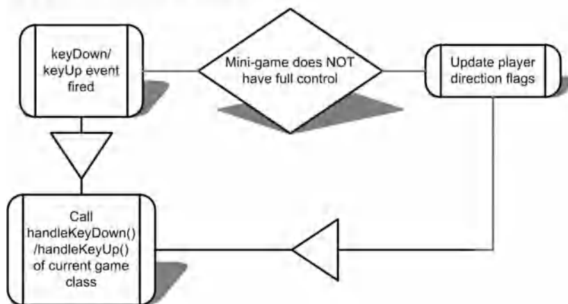
Figure 11-8. Basic flow diagram of how K&G Arcade works, at a high level
