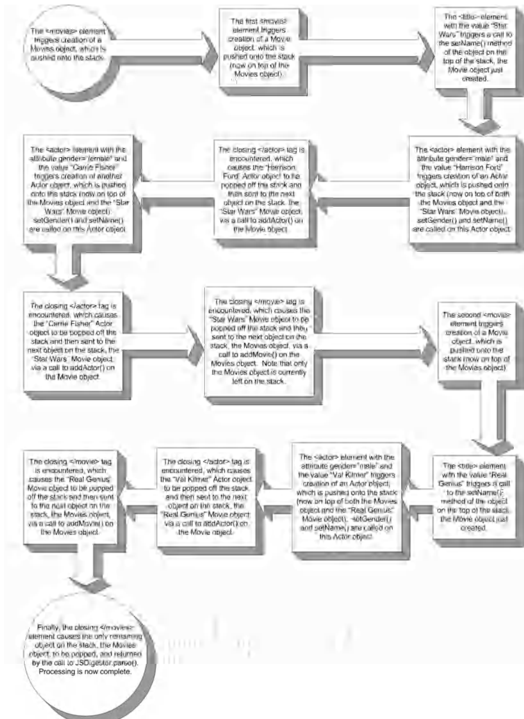
Figure 7-4. JSDigester parsing sequence of events
