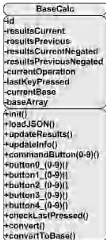
Figure 4-10. UML diagram of the BaseCalc class
