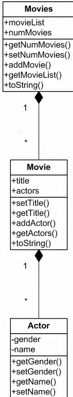
Figure 7-3. The test class hierarchy in UML
