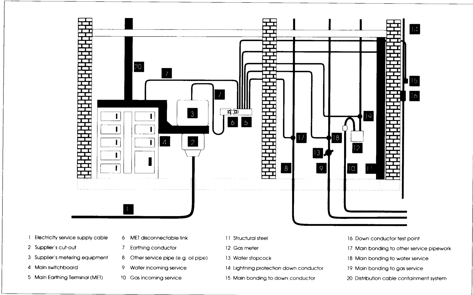
Figure 12.9: Typical main bonding connections
