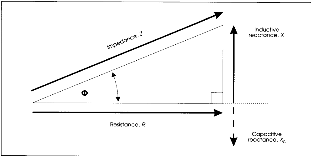
Figure 7.5: Impedance triangle
