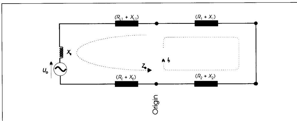
Figure 7.10: Phase-to-earth fault equivalent circuit
