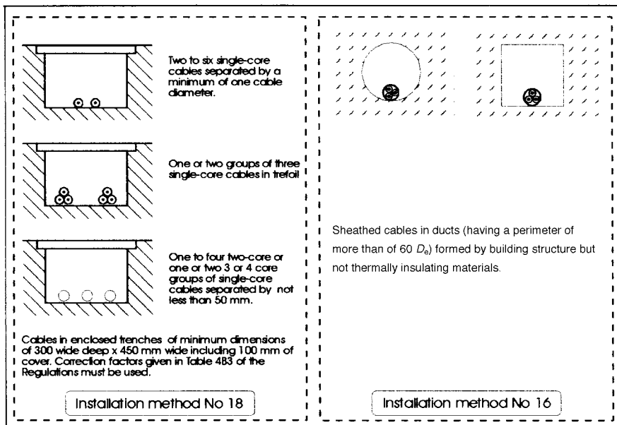
Figure 10.11: Reference method 18
