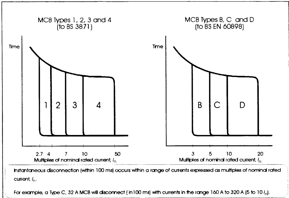
Figure 11.9: MCB characteristics
