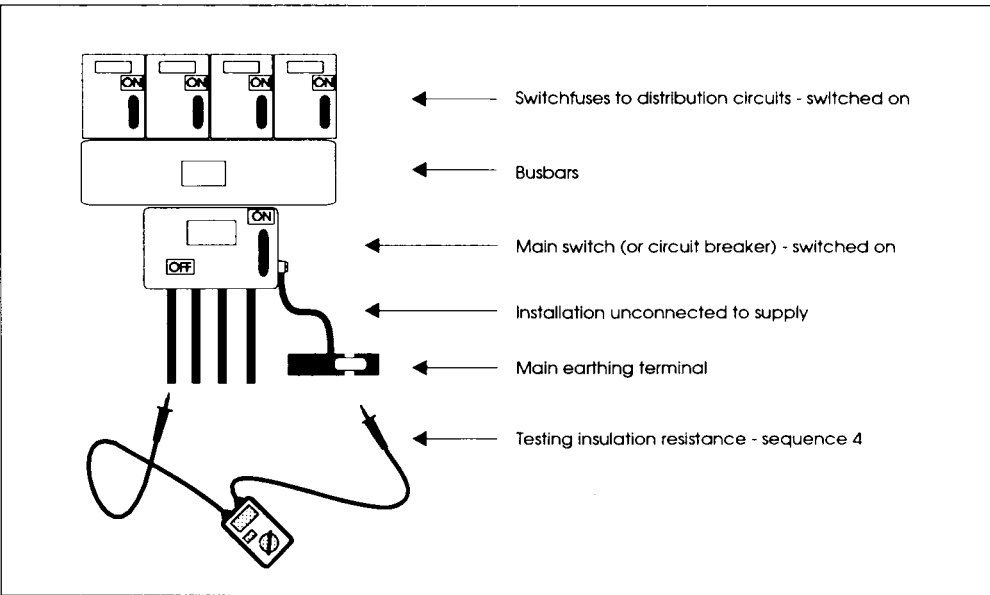
Figure 17.3: Testing insulation
