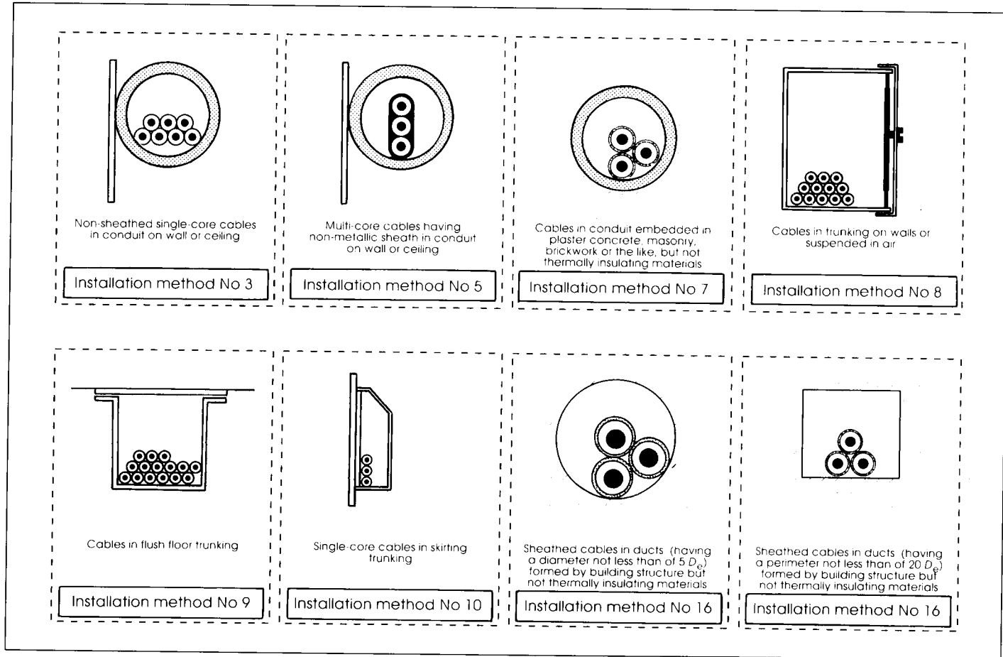
Figure 10.6: Reference method 3
