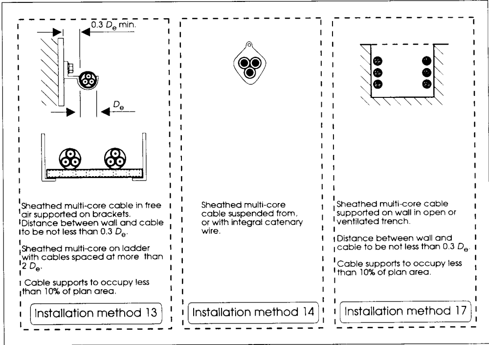
Figure 10.10: Reference method 13
