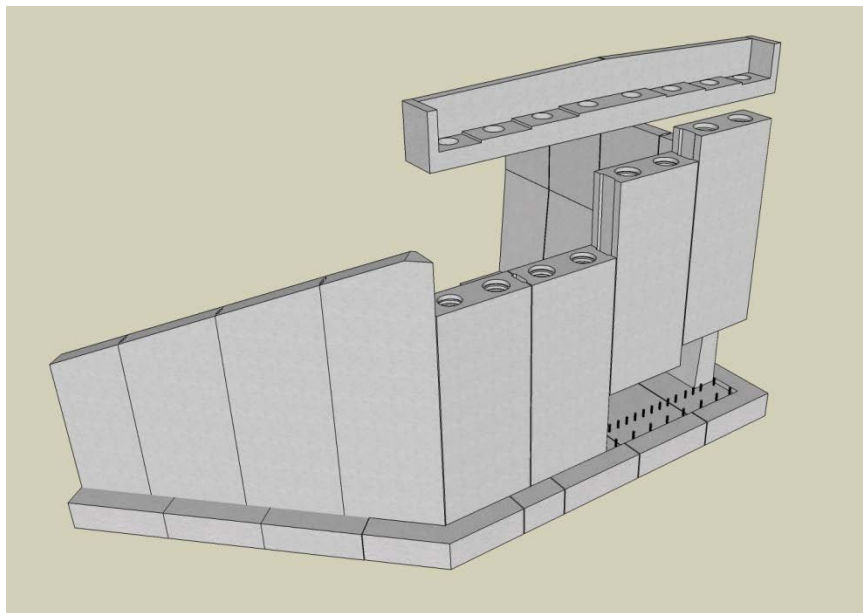
Figure 5.3.2.1-1 Precast Concrete Cantilever Abutment
