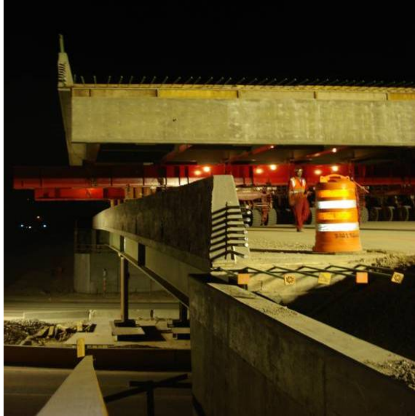
Figure 3.2.1.3-1 SPMT Bridge Move over another Bridge (source: Utah DOT)
