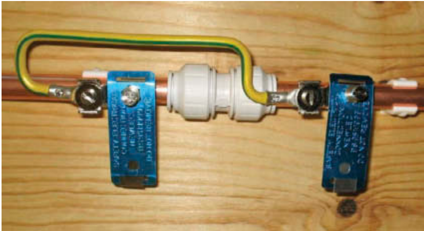
Figure 4.23 Fitting bonded across
