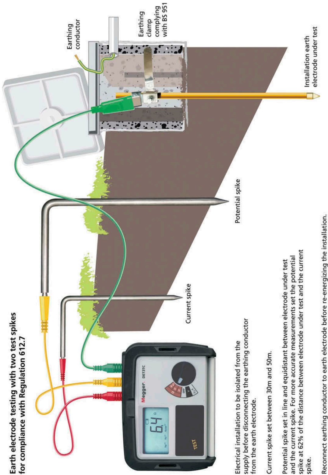
Figure 5.2 Electrodes in the ground
