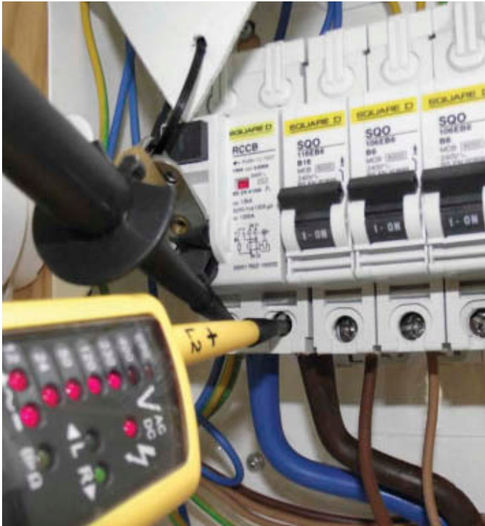
Figure 4.65 Live supply
