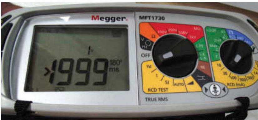
Figure 5.39 No trip
