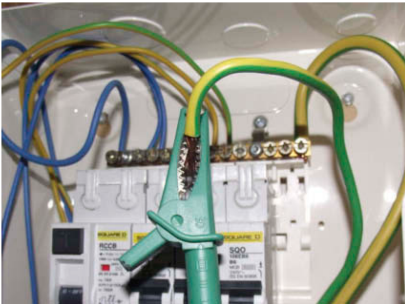
Figure 4.15 Lead connected
