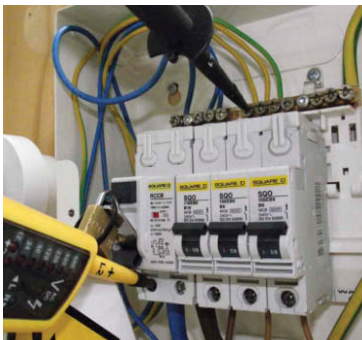
Figure 4.67 No reading
