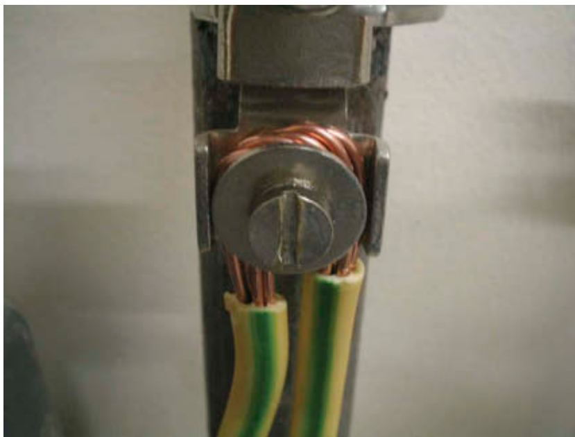
Figure 4.20 Correct!
