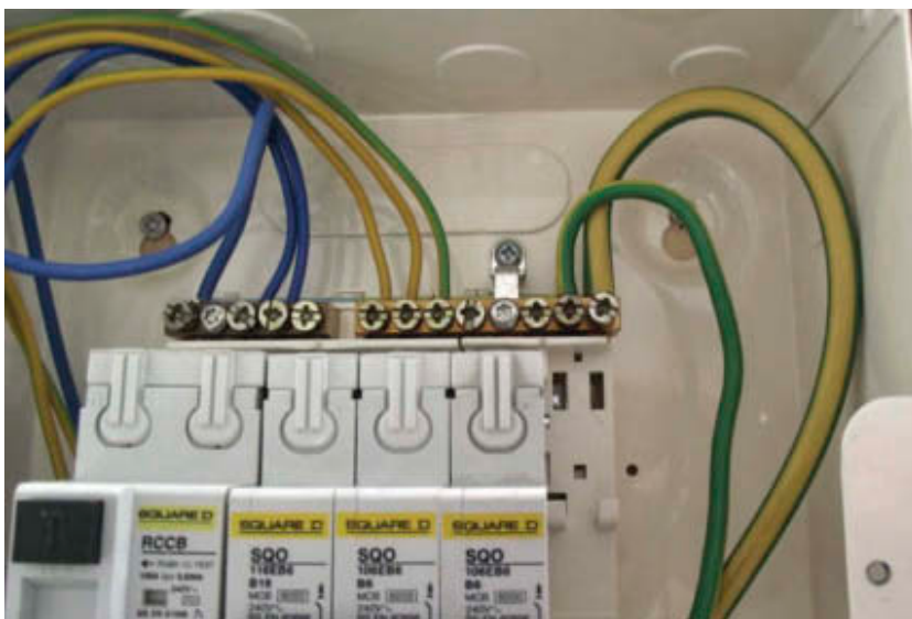
Figure 4.18 Reconnect bonding
