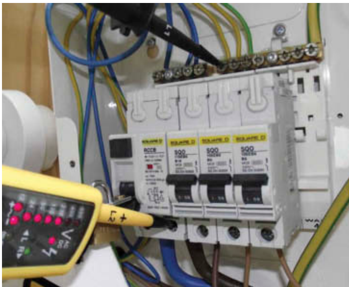
Figure 4.66 Live supply
