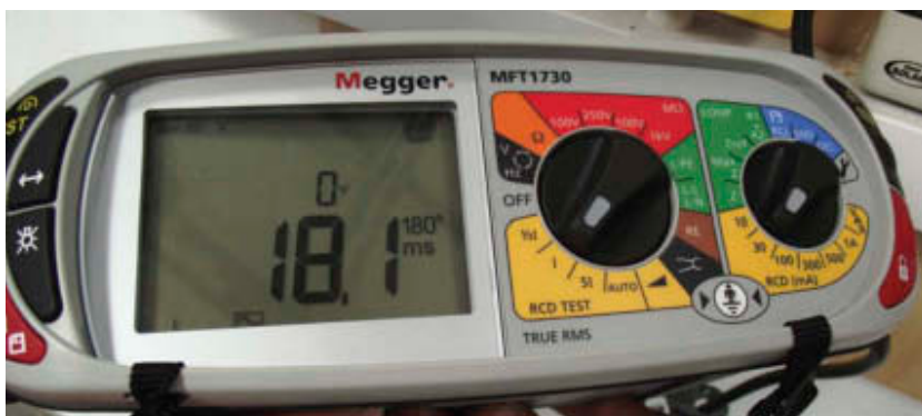
Figure 5.41 Test at 180°
