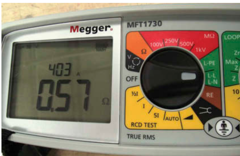
Figure 5.26 Measured value
