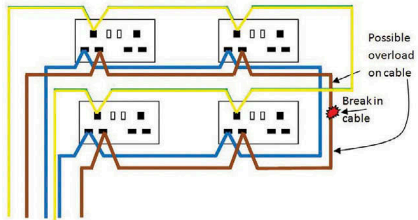
Figure 4.30 Broken conductor
