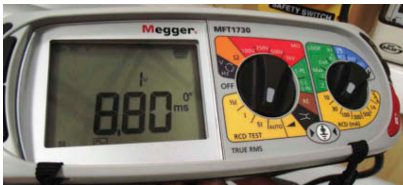
Figure 5.43 Test at zero degrees
