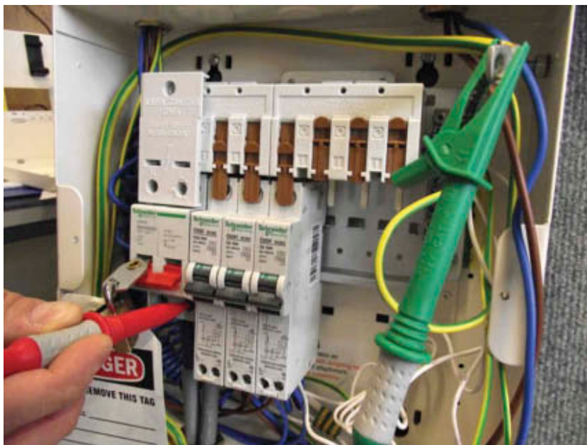
Figure 5.3 Tester connected
