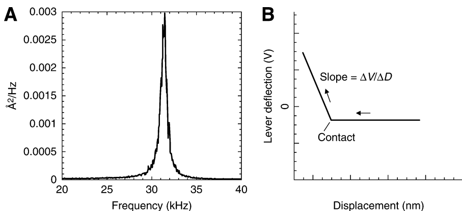
Fig. 7. Data used for calibration of cantilever force (spring) constant k . (A) Power spectrum of cantilever motion (Z deflection) in air at room temperature. The peak is the natural resonance frequency in air. The area under the peak is integrated to obtain k . This requires determination of the cantilever deflection sensitivity (V/nm) as shown in (B). Based on ref. 24 .
