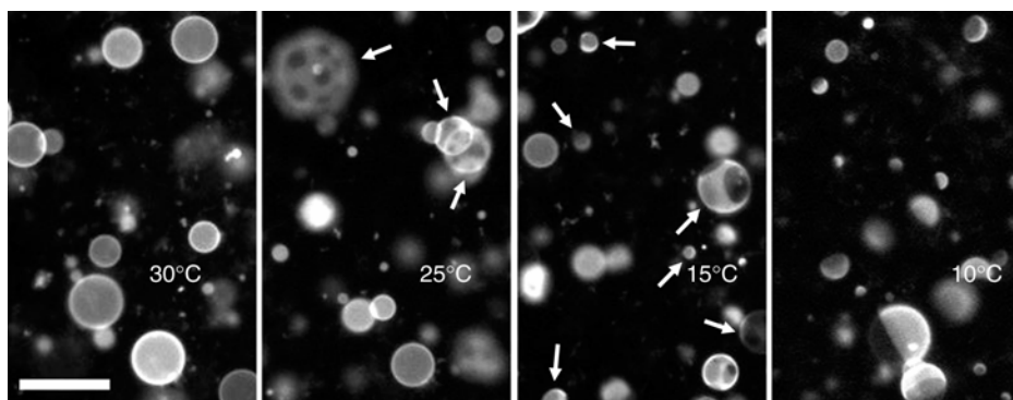
Fig. 6. Miscibility transition temperatures vary between vesicles in a single GUV preparation owing to slight variations in lipid composition. At 30°C, all vesicles of 2:1 diphytanoyl PC/DPPC + 50% cholesterol are in one uniform phase. At 25 and 15°C, a fraction of vesicles contain coexisting liquid phases (arrows). In this sample, all vesicles are phase separated at 10°C. Bar = 50 \mu m.
