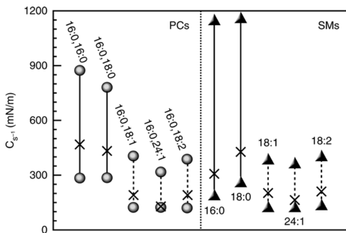
Fig. 5. Changes in surface compressional moduli ( C_{s-1} ) induced on mixing of equimolar cholesterol with PC or SM. Lower symbols represent the C_{s-1} values of the pure lipids in the absence of cholesterol. Upper symbols represent the experimentally observed C_{s-1} values for binary mixtures with equimolar cholesterol. The X along each line represents the ideal C_{s-1} values calculated based on additivity of each pure lipid component in the binary mixtures. All C_{s-1} values were determined at a surface pressure of 30 mN/m. The notation X:Y refers to the acyl chain length in carbon atoms (X) and the number of cis -double bonds (Y) present in the different molecular species of PC or SM.
