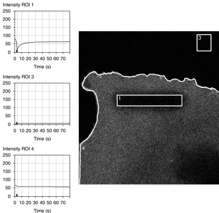
Fig. 2. Example of how to quantitate fluorescence intensities from a confocal FRAP experiment. Examples of ROIs for bleach region, surrounding cell, and background and corresponding plots of mean fluorescence intensity vs time for each are shown.
