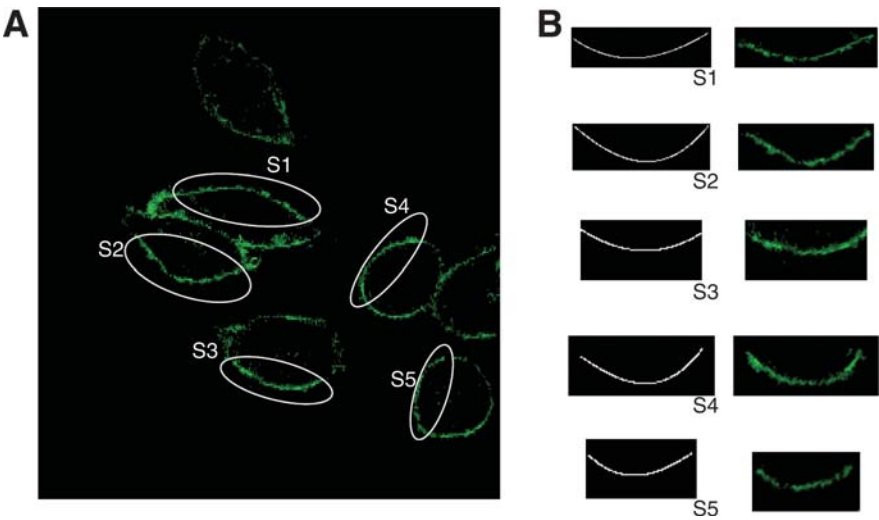
Fig. 5. Five segments of the DHE emission in extracted PMs from MPLSM images of living fibroblasts. (Panel A) The monomeric DHE along the PM with the five segments marked that were used for spatial measurement study. (Panel B) The geometric reference lines from a third-order polynomial fitting routine on the PM and the corresponding raw data values for each segment.
