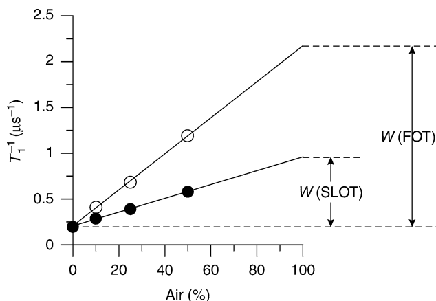
Fig. 5. Plot of T_1^{-1} for 5-PC in SLOT and FOT domains of DMPC membrane containing 20 mol% cholesterol at 30°C as a function of fraction of air in the equilibrating gas mixture. Experimental points show a linear dependence of up to 50% air, and extrapolation of up to 100% air is performed to indicate a way of calculating oxygen transport parameters. W(\text{SLOT}) and W(\text{FOT}) are oxygen transport parameters in SLOT (liquid-ordered) and FOT (liquid-disordered) domains.
