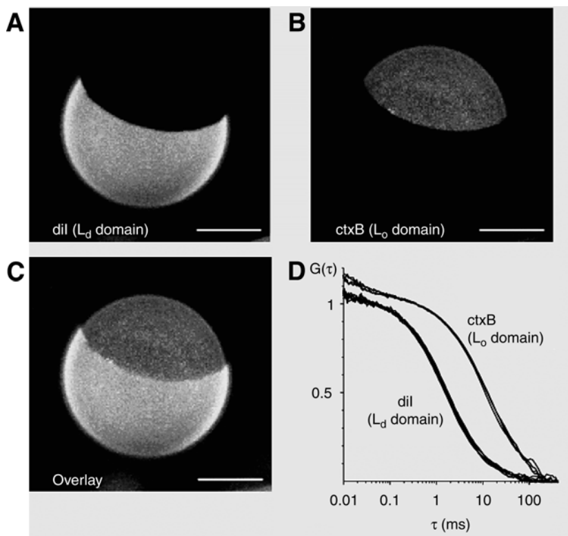
Fig. 2. Three-dimensional confocal reconstruction of a GUV made up of DOPC:SM: Chol, 1:1:1, with 0.1% GM1 and 0.1% diI. Bar = 10 \mu\text{m} . (A) Red channel showing diI fluorescence enriched in one phase. (B) Green channel showing fluorescence from Alexa-488-labeled ctxB bound to GM1, enriched in the other phase. (C) Overlay. (D) FCS measurements of lipid analog (diI) and ctxB (ctxB-488) show distinct diffusion characteristics and allow assignment of diI to the more fluid L d phase ( \tau_{\text{diff}} = 1.5 ms, D = 5 \times 10^{-8} cm 2 /s) and ctxB-GM1 to the more ordered L o phase ( \tau_{\text{diff}} = 12 ms, D = 5 \times 10^{-9} cm 2 /s).
