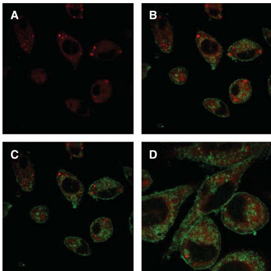
Fig. 1. MPLSM of DHE and Nile red in murine L-cell fibroblasts. Excitation at 920 nm. (Panel A) Image of L-cells labeled with DHE and Nile red at low power (25% attenuation). (Panel B) Image of L-cells labeled with DHE and Nile red at high power (40% attenuation). (Panel C) Image with high-power DHE (green channel, panel B ) merged with the low-power Nile red (red channel, panel A ). (Panel D) Image acquired at high power with zoom = 2.
