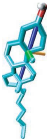
Fig. 5. Body center coordinate system for Chol, z -axis is represented by blue, x -axis is represented by green, and y -axis is represented by orange cylinders.
