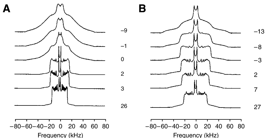
Fig. 1. (A) Deuterium NMR spectra of 1-stearoyl(d35)-2-oleoyl- sn -glycero-3-phosphocholine (SOPC-d35) recorded at -9, -1, 0, 2, 3, and 26°C. (B) ^2\text{H} NMR spectra SOPC-d35/cholesterol (7/3, mol/mol) recorded at -13, -8, -3, 2, 7, and 27°C.
