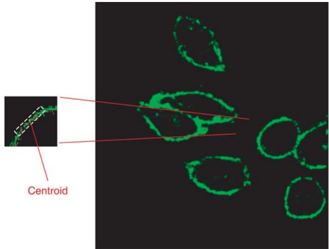
Fig. 4. Image smoothing using a nonlinear median window filter based on a moments functions. The smoothed image shows the result after application of a continuous planar model of the DHE image using window size 20 \times 20 and neighborhood 5 \times 5 . Each pixel in the smoothed image represents the intensity centroid calculated from the application of this filter to the raw data. A blowup of a particular PM region from the raw data was shown to illustrate the window and its intensity centroid.
