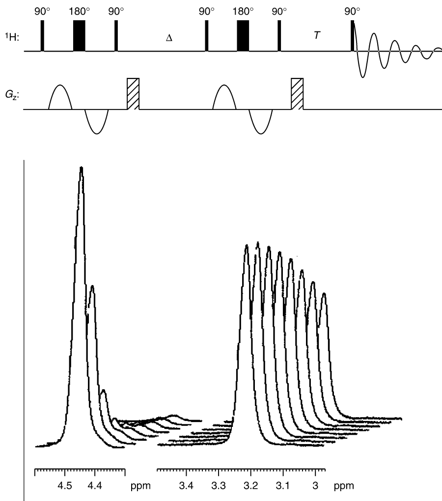
Fig. 7. Stimulated echo sequence with shaped bipolar gradient pulses for diffusion measurements by ^1\text{H} MAS-NMR. The spectra show water ( left ) and lipid resonances ( right ) of multilamellar liposomes, recorded at increasing strength of pulsed magnetic field gradients. The water signal decays much faster with increasing gradient strength, indicating higher rates of lateral diffusion of water molecules.
