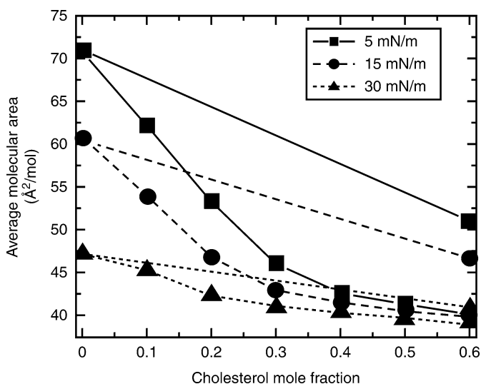
Fig. 4. 16:0 SM-cholesterol average molecular area vs composition analysis. Plots are shown for three different surface pressures in mN/m (5, squares; 15, circles; 30 triangles). The linear plots show the average molecular area obtained by calculation using the molecular areas of pure 16:0 SM and cholesterol, each apportioned by mole fraction. The nonlinear curves represent the experimentally observed areas for the mixtures. Negative deviation from ideal additivity (linear plots) shows the condensing or ordering effect of cholesterol.
