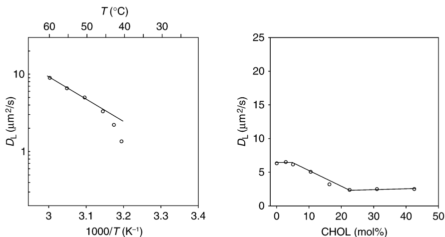
Fig. 7. Lipid lateral diffusion in the egg sphingomyelin eSM/CHOL system. The left panel shows the temperature dependence for a CHOL concentration of 10.5 mol% and the right panel gives the dependence of D_L on the CHOL concentration at 50°C. The curved feature of the Arrhenius plot and the kinks in the concentration plot are indicative of an inhomogeneous membrane in which the domains are sufficiently small so that fast exchange occurs. The lines are merely guides for the eye. From ref. 24 .
