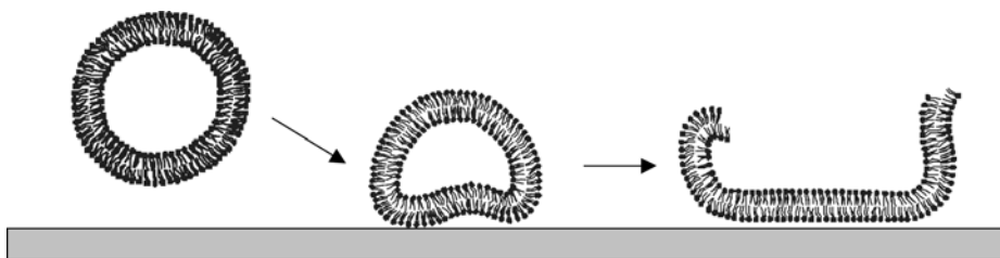
Fig. 3. Highly schematic depiction of vesicle fusion on a solid substrate (e.g., glass or mica). From left to right: A single 100 nm vesicle adsorbs to the substrate, deforms due to spreading, and finally ruptures. The ruptured vesicle will fuse with others to form a complete bilayer. This is just one of several proposed mechanisms ( see text ). A 1–2 nm water layer separates the lipid bilayer from the substrate.
