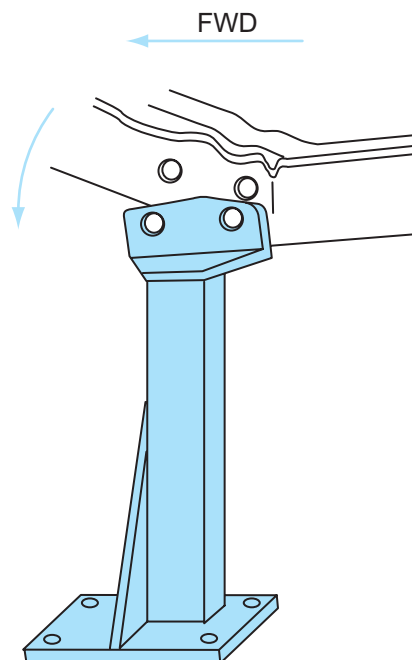
Figure 14-20 When holes in the body are behind and above the openings in the dedicated fixture, the unitized body must be pulled forward and downward in that area.
