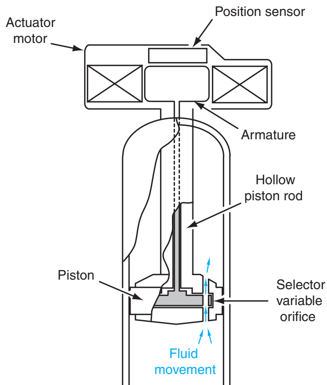
Figure 8-27 Strut actuator.
