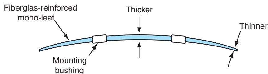
Figure 6-6 Transversely mounted fiberglass mono-leaf spring.
