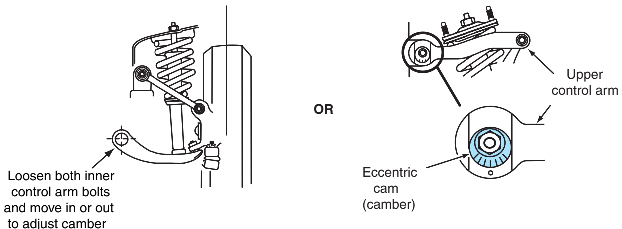
Figure 1-35 Rear wheel camber.
