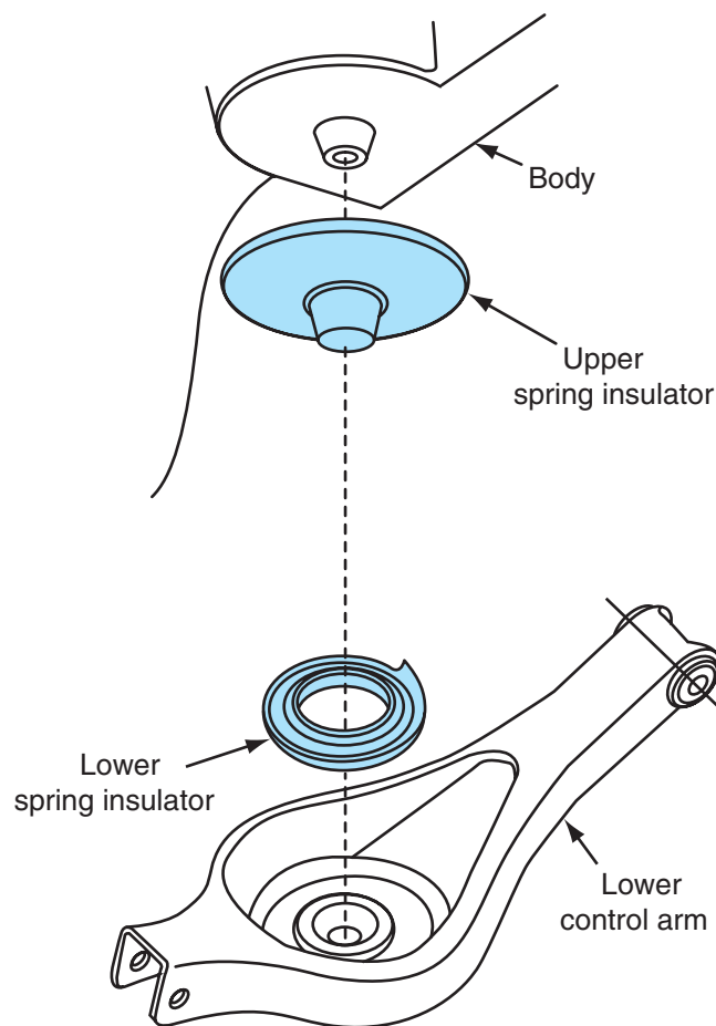
Figure 7-31 Lower control arm with upper and lower spring insulators.
