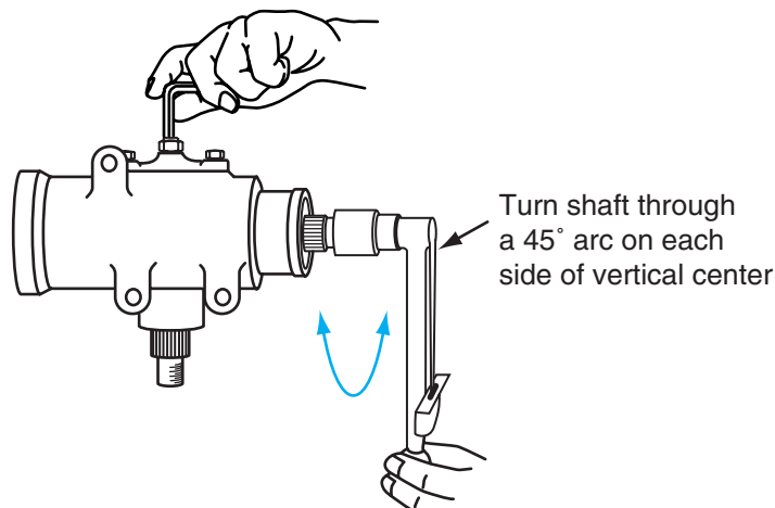
Figure 11-8 Measuring wormshaft turning torque to adjust pitman backlash adjuster screw.
