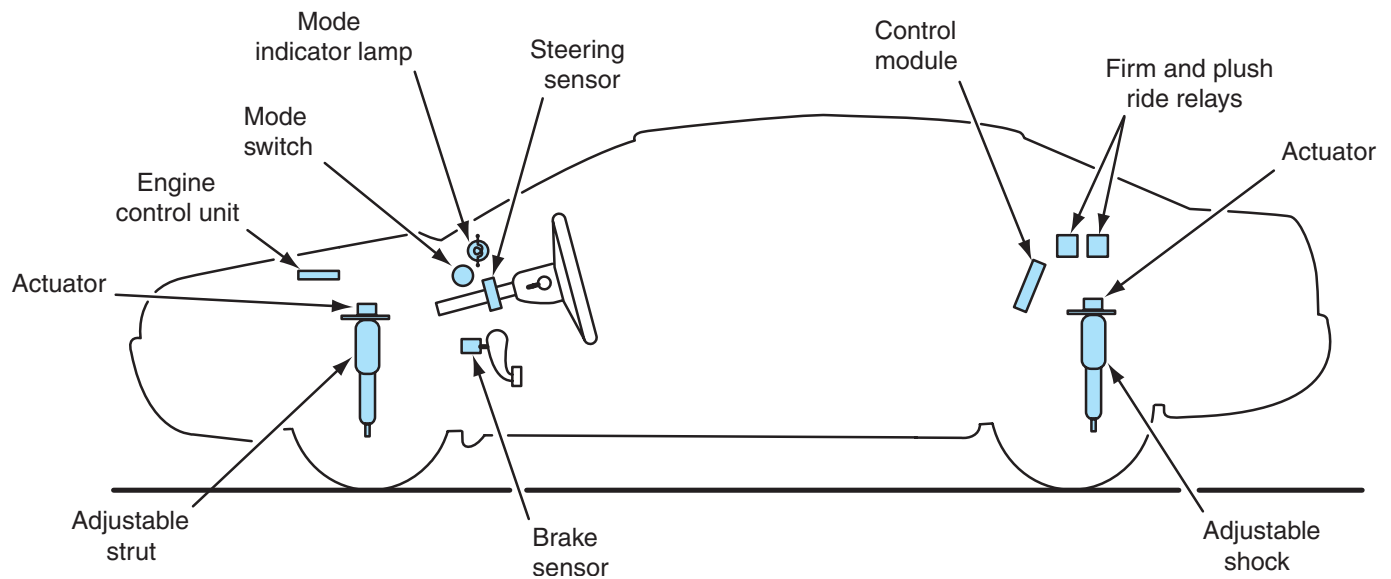
Figure 8-1 Programmed ride control (PRC) system components.
