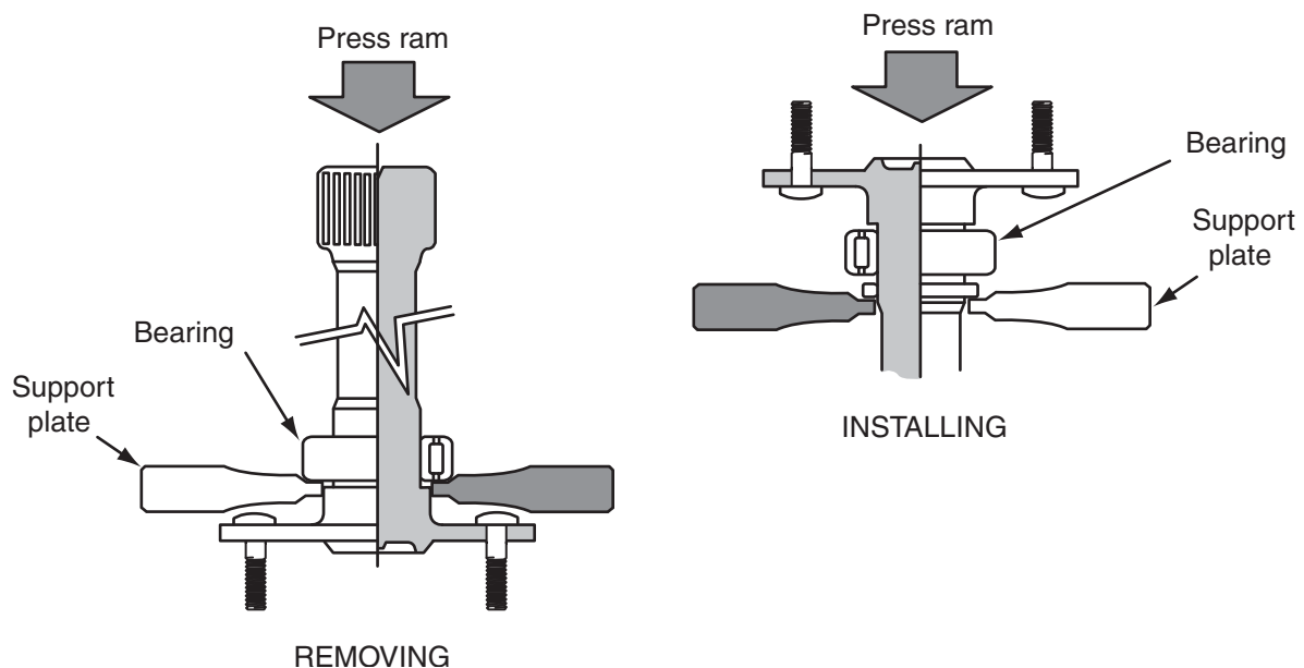
Figure 3-33 Axle bearing and adaptor ring removal and replacement.
