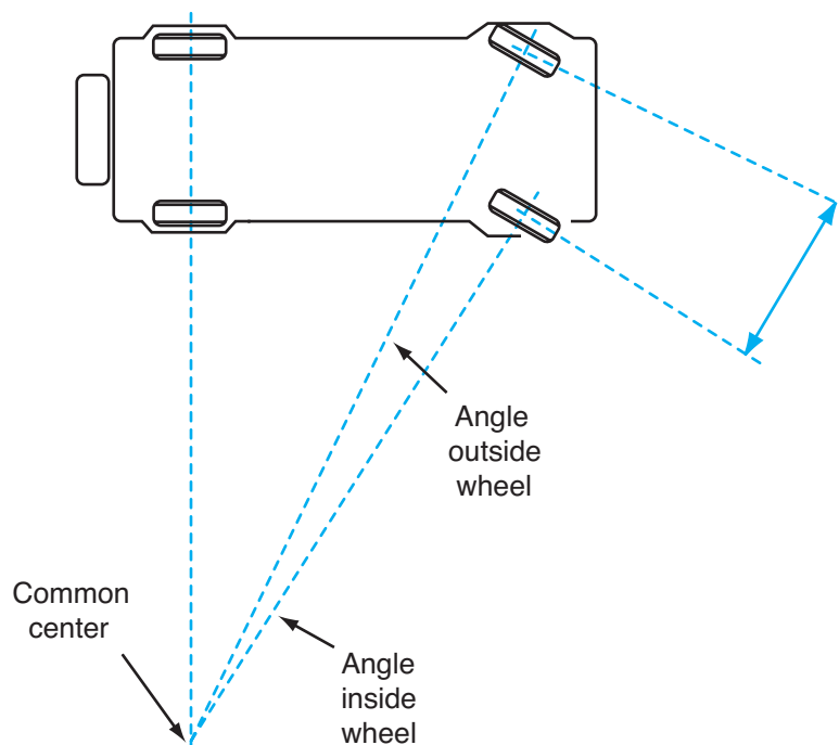
Figure 16-9 Front and rear wheels turning around a common center.
