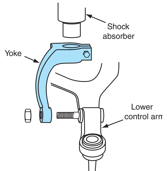
Figure 6-27 Shock absorber with yoke attachment to lower control arm.
