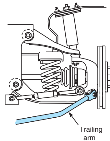
Figure 7-33 The trailing arm is connected from the lower end of the knuckle to the frame.
