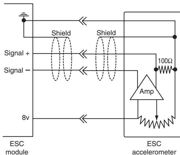
Figure 8-34 Accelerometer internal design and wiring diagram.
