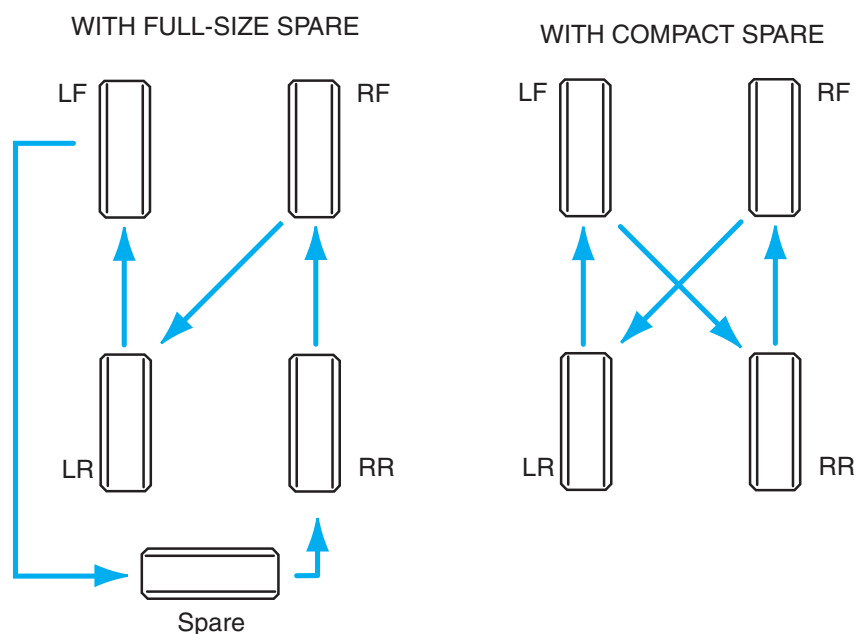
Figure 4-3 Radial tire rotation procedure.
