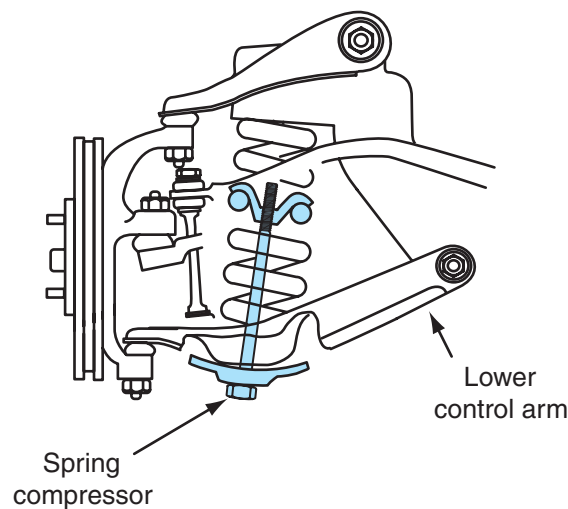
Figure 6-37 Spring compressing tool installed on a spring in a short-and-long arm suspension system.
