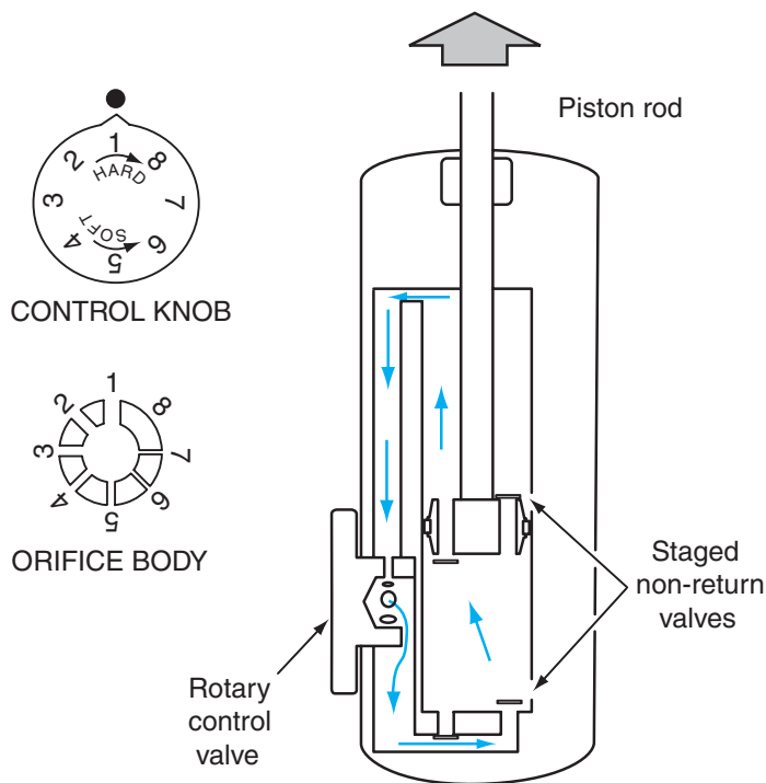
Figure 5-14 Adjustable strut.
