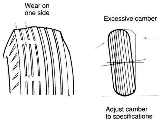
Figure 15-35 Tire tread wear caused by incorrect camber adjustment.
