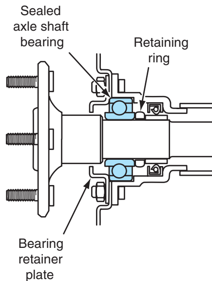
Figure 3-5 Some rear axle bearings are sealed on both sides and retained on the axle with a retainer ring.
