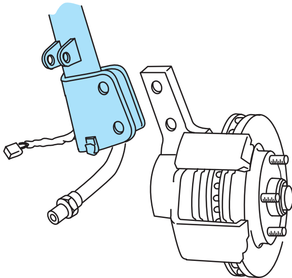
Figure 7-15 Removing the strut from the rear spindle.
