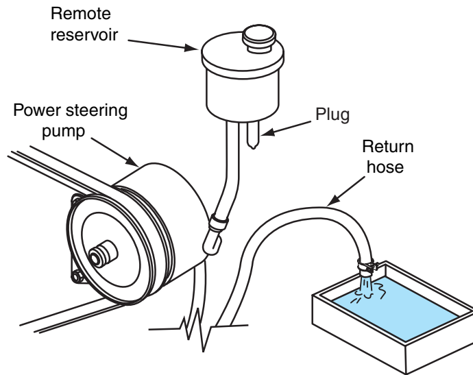
Figure 10-9 Return hose installed in drain pan for power steering draining and flushing.
