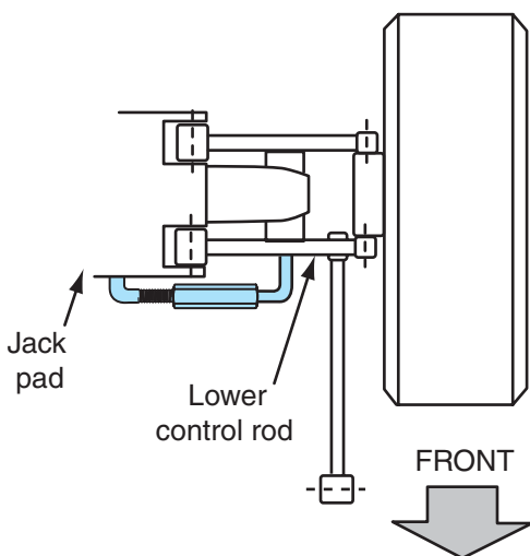
Figure 16-55 Special toe adjusting tool for transverse leaf-spring rear suspension.
