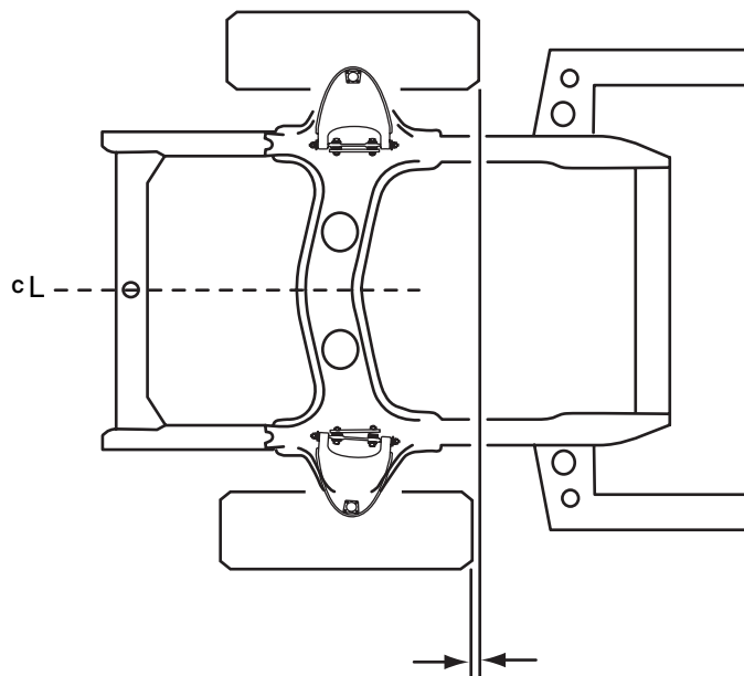
Figure 14-7 Setback occurs when one front wheel is positioned rearward in relation to the other front wheel.
