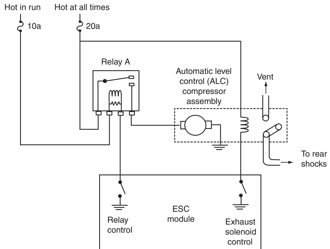
Figure 8-40 Rear automatic level control (ALC).
