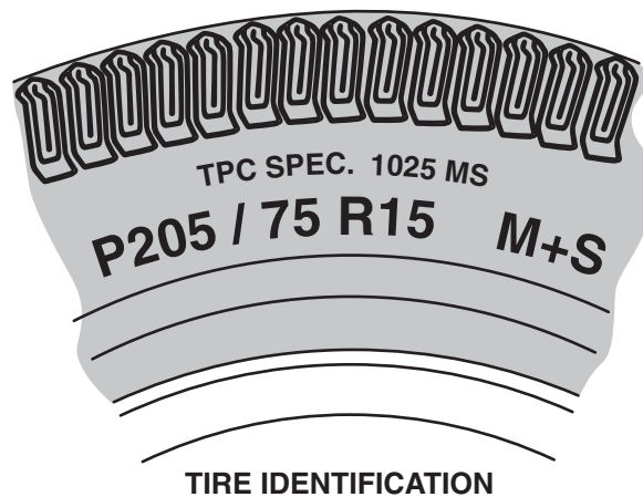
Figure 4-10 Tire performance criteria (TPC) number.
