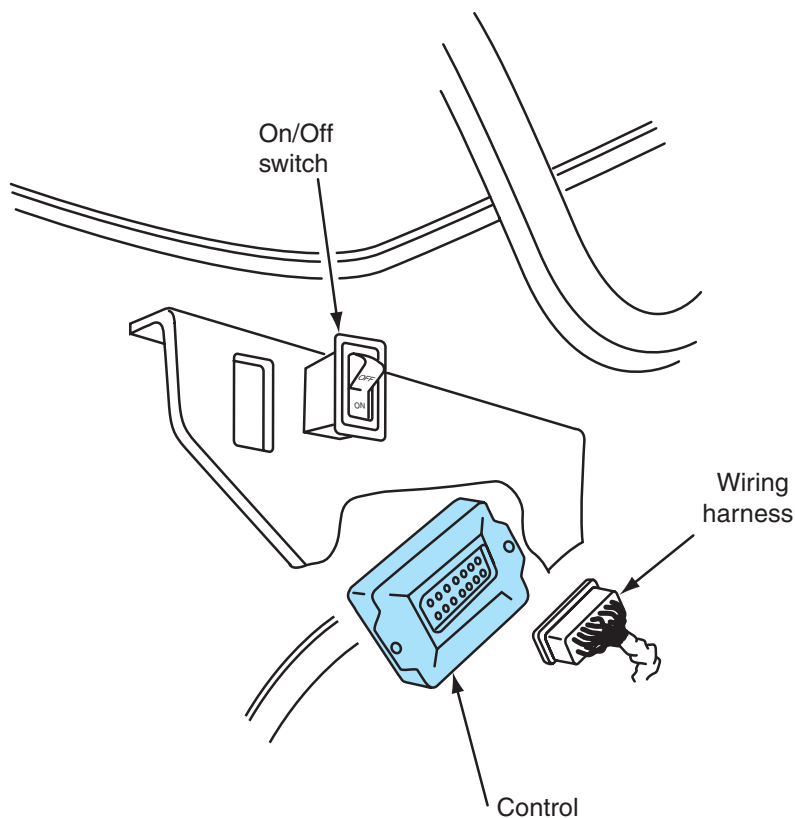
Figure 8-18 Control module.
