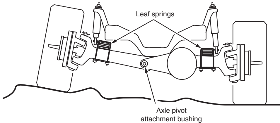
Figure 6-51 Four-wheel-drive twin I-beam front suspension system with leaf springs.
