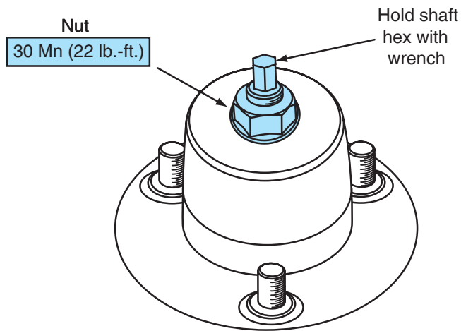
Figure 8-21 Removing the nut from the upper end of the shock absorber rod.
