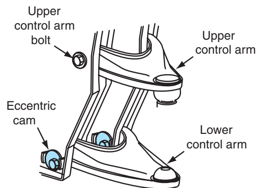
Figure 16-6 Cam adjustment on the inner ends of the lower control arms.
