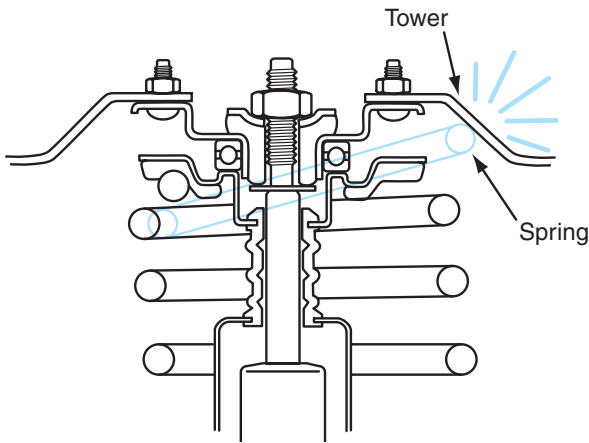
Figure 5-3 Coil spring to upper strut tower interference.
