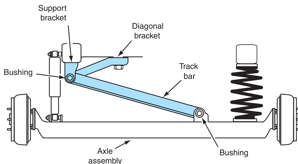
Figure 7-31 Checking track bar bushings.
