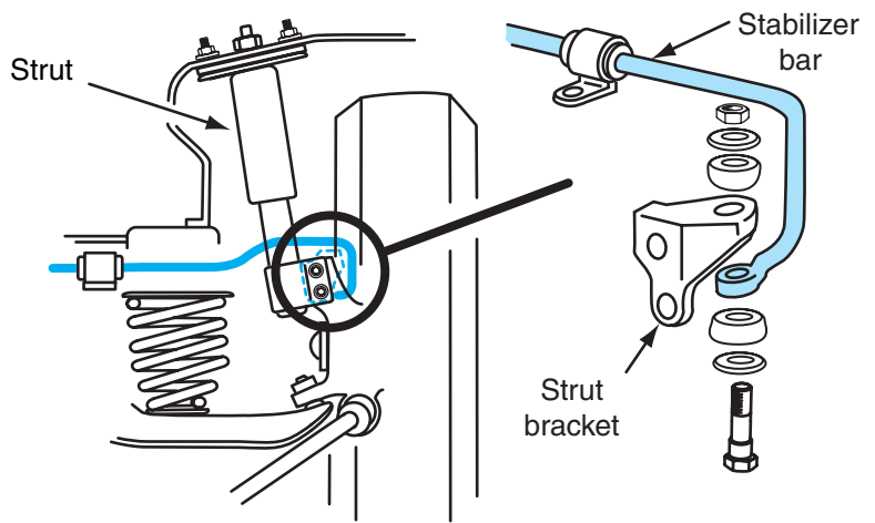
Figure 7-25 Stabilizer bar mounting.
