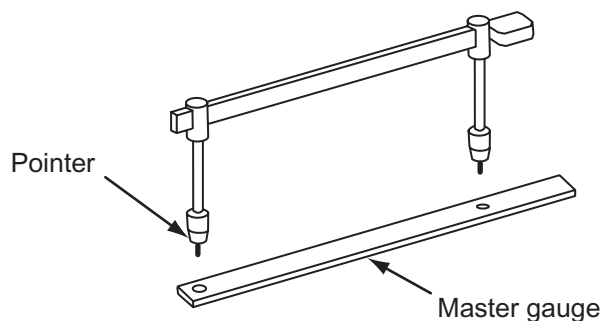
Figure 14-8 Tram gauge for frame measurements.
