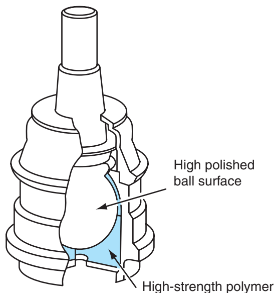
Figure 6-14 Low-friction ball joint.
