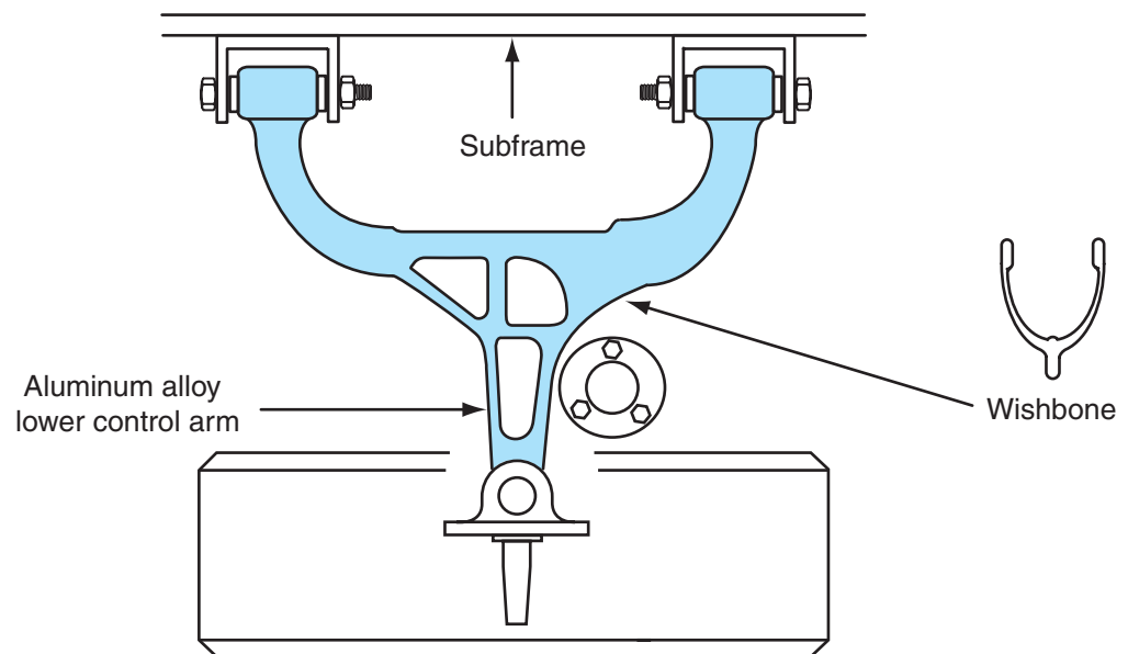
Figure 7-44 Double wishbone rear suspension and subframe.
