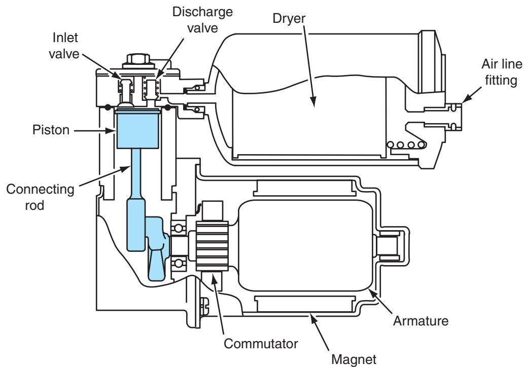
Figure 8-15 Air compressor.
