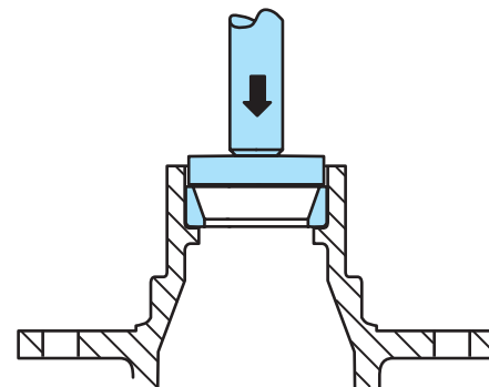
Figure 3-6 Bearing race installation.
