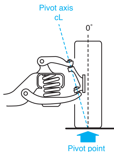
Figure 16-4 If the SAI line meets the tire vertical centerline at the road surface, tire wear is reduced, steering effort is decreased, and stress on the steering components is diminished.
