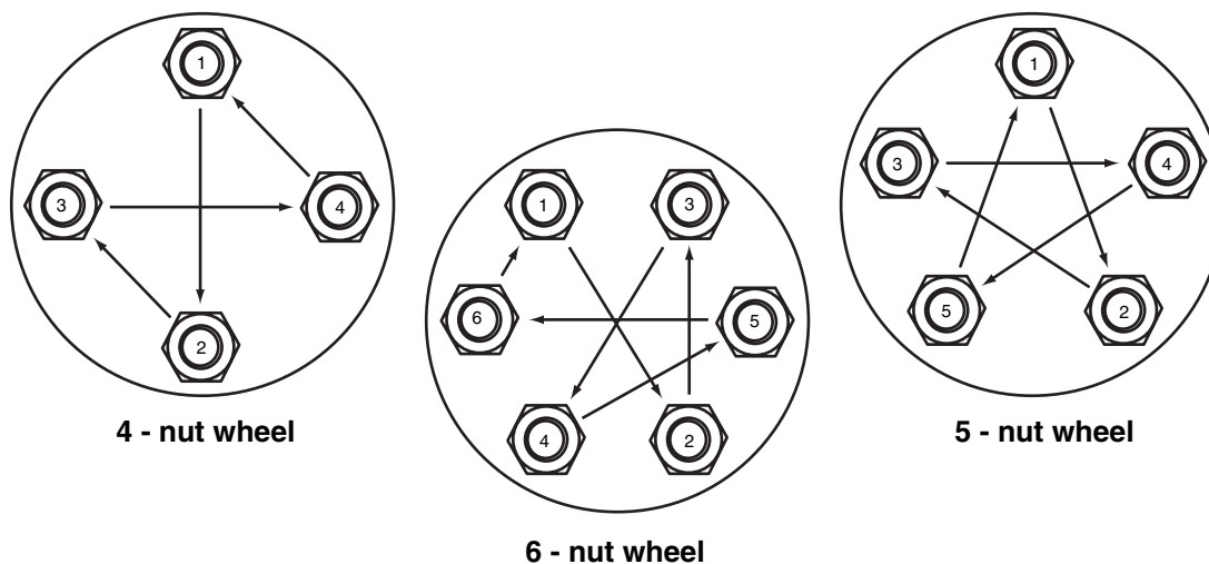
Figure 3-27 Wheel nut tightening sequence.
