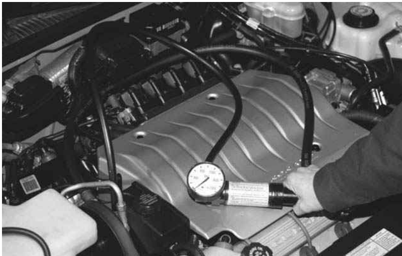
Figure 10-13 Pressure gauge connection to power steering pump.
