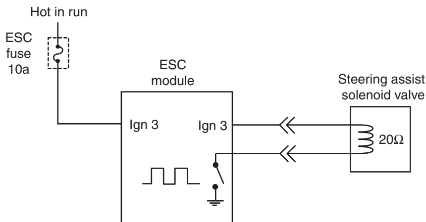
Figure 8-42 Steering solenoid and ESC module wiring diagram.
