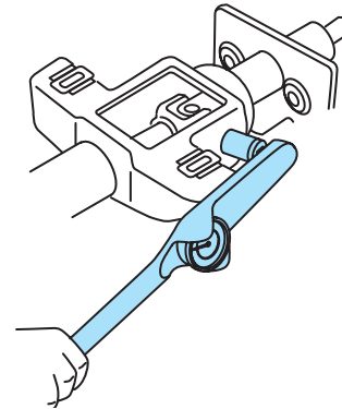
Figure 9-34 Tightening pivot bolt nuts.
