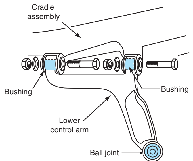
Figure 14-15 Lower control arm-to-cradle attachment.
