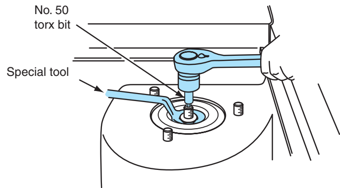
Figure 5-27 Removing nut from strut piston rod.
