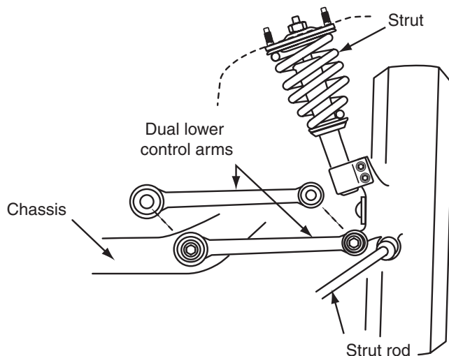
Figure 7-19 MacPherson strut independent rear suspension system.
