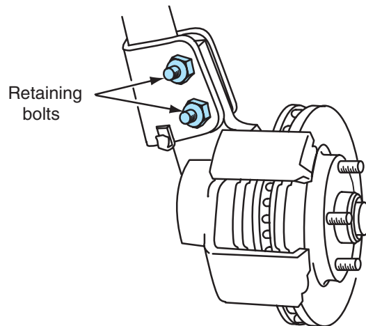
Figure 5-23 Lower end of strut installed in steering knuckle.
