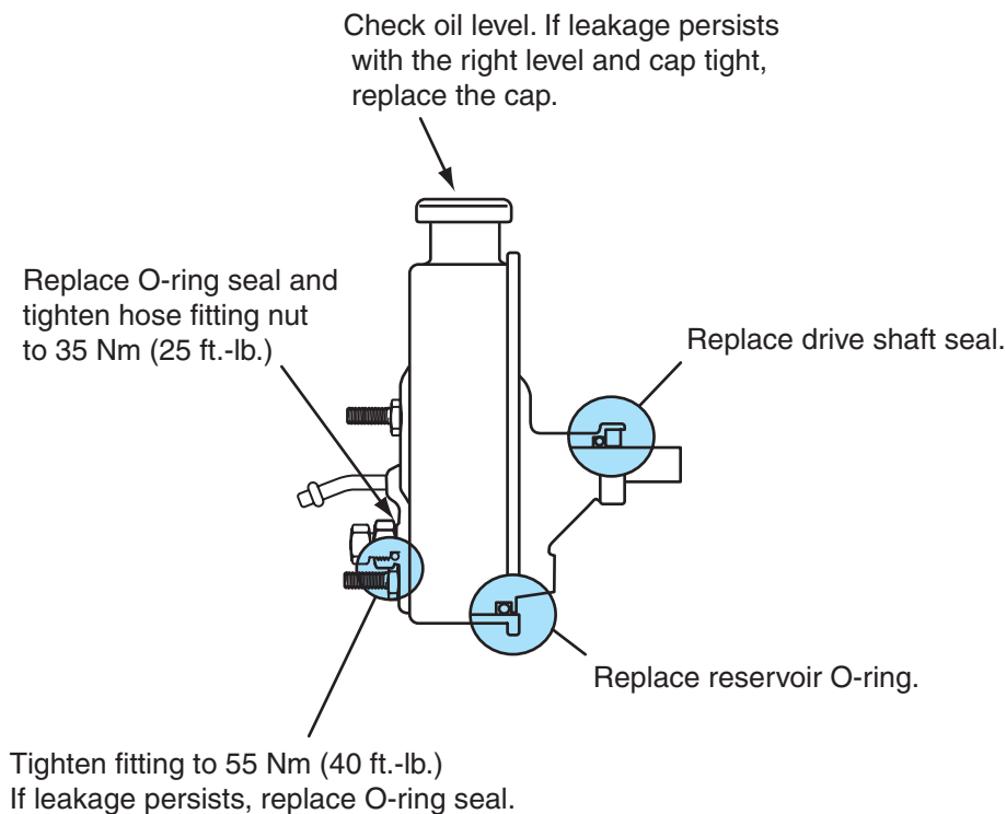
Figure 10-19 Power steering pump oil leak diagnosis.
