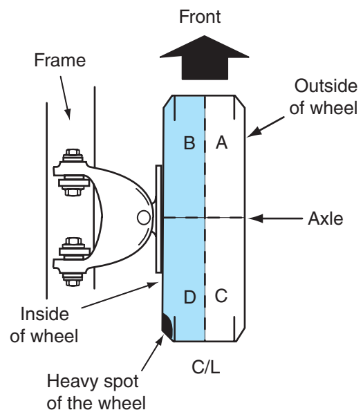
Figure 4-39 Dynamic wheel unbalance.
