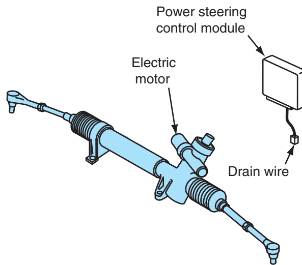
Figure 12-38 Pinion-drive electronic power steering (EPS) steering gear.
