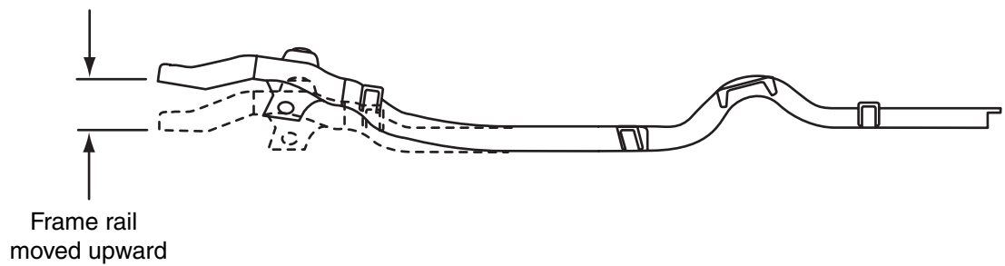
Figure 14-12 Frame sag caused by direct front or rear collision damage.
