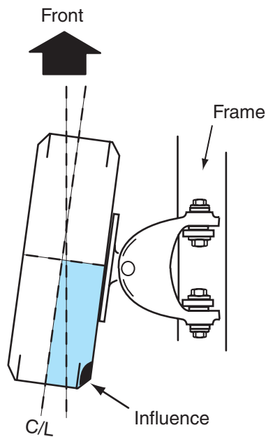
Figure 4-40 Dynamic wheel unbalance with heavy spot at the rear of the left front tire.
