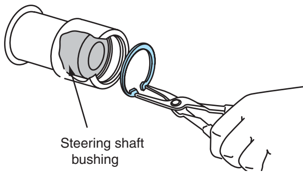
Figure 9-31 Installing steering shaft bushing and snapping.
