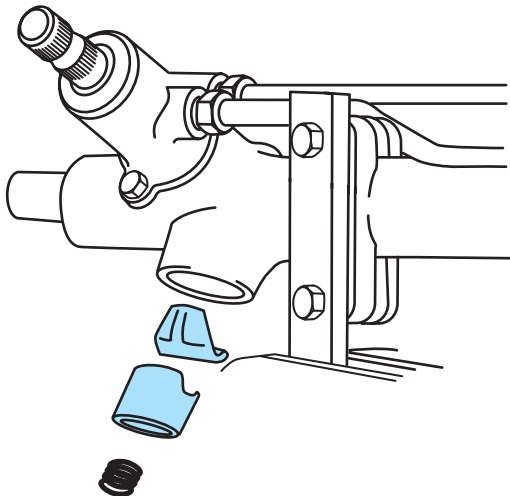
Figure 12-31 Installing rack guide seat, rack guide, and spring.
