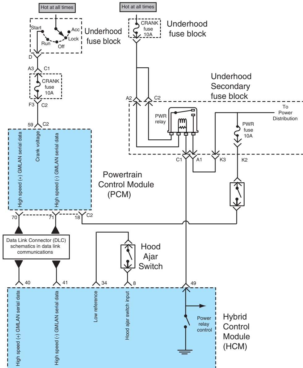
Figure 10-31 The HCM receives inputs from the PCM through the LAN bus.
