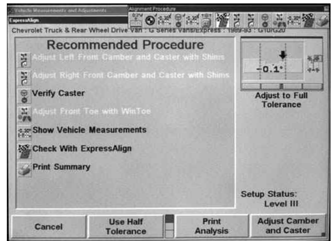
Figure 15-23 Wheel alignment procedure screen.
