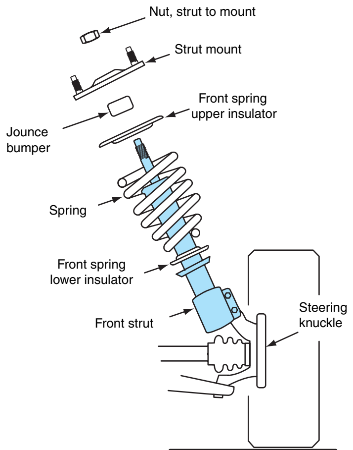
Figure 1-16 Front strut and spring assembly.
