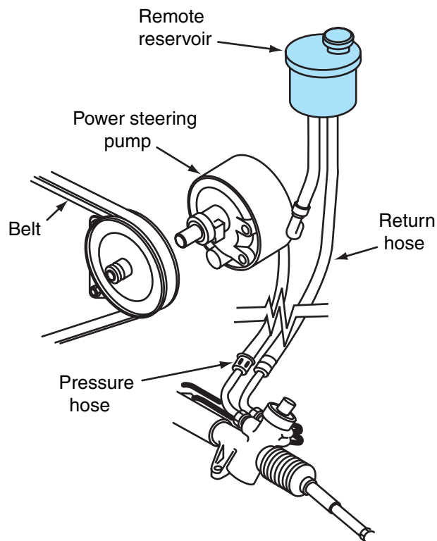
Figure 10-6 Remote reservoir on power-assisted rack and pinion steering system.
