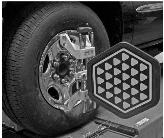
Figure 15-12 Each target contains a polished aluminum face plate with no electronics, glass, or cables.
