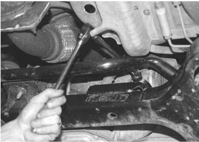
Figure 12-9 Removing steering gear mounting bolts.
