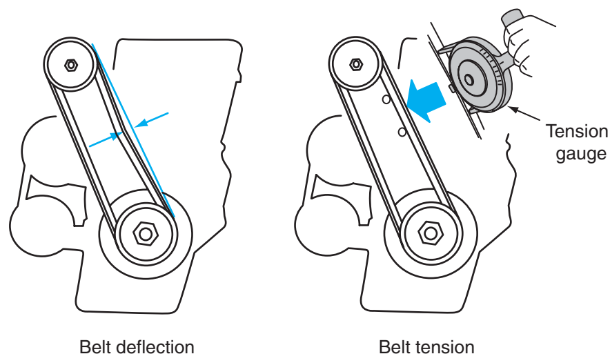
Figure 10-2 Methods of checking belt tension.
