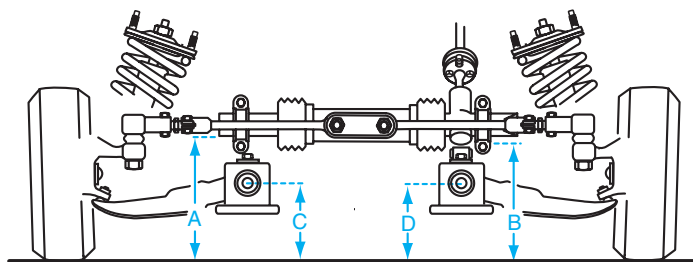
Figure 15-45 Measuring rack and pinion steering gear height at various locations.
