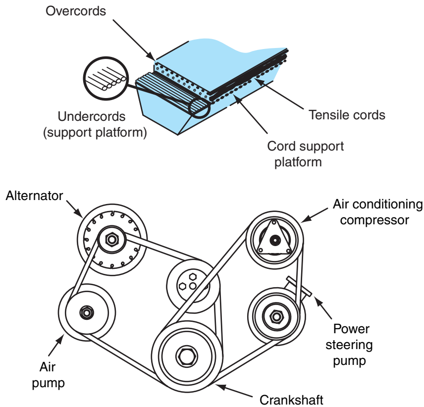
Figure 1-26 Conventional V-belt.
