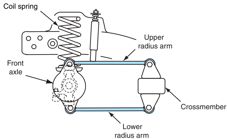
Figure 6-53 Four-wheel-drive front suspension with straight drive axle and coil springs.
