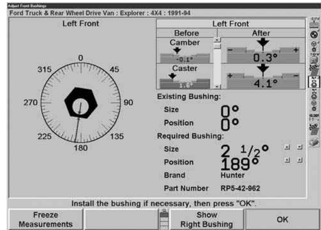
Figure 15-38 Automatic bushing calculation screen. (Courtesy of Hunter Engineering Company.)
