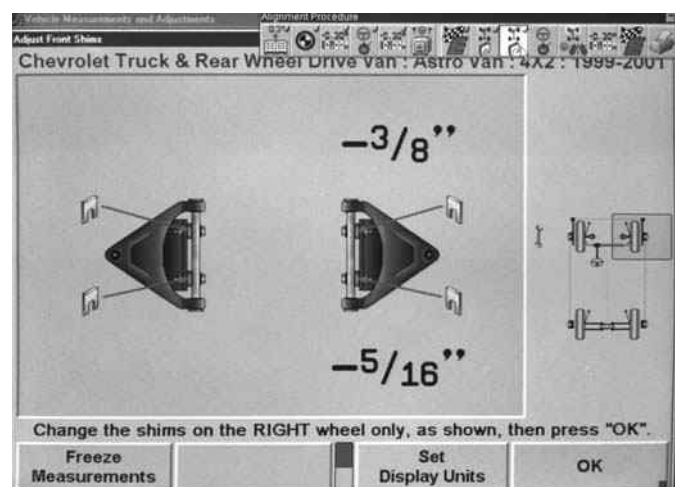
Figure 15-39 Control arm movement monitor indicates the required shim thickness to provide specified camber and caster.
