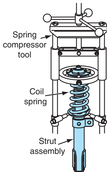
Figure 5-10 Coil spring and strut assembly mounted in a spring compressing tool.
