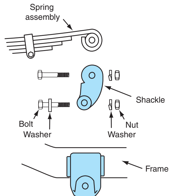
Figure 7-8 Rear leaf-spring shackle.
