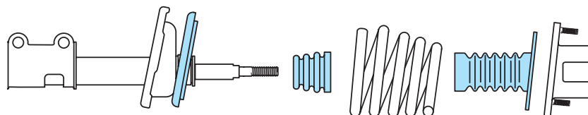
Figure 7-19 Assembly of rear strut, spring bumper, spring, upper mount, and insulator.
