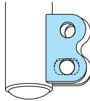
Figure 16-21 Elongated lower strut-to-knuckle bolt hole for camber adjustment.
