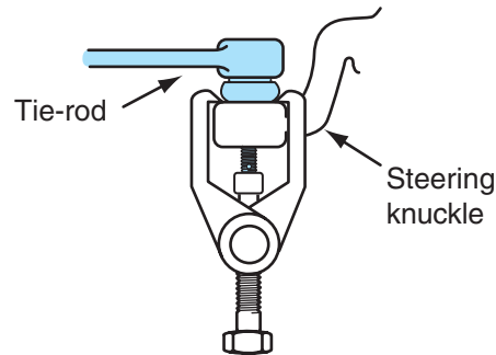
Figure 6-16 Removing the outer tie-rod end from the steering knuckle.
