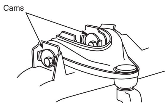
Figure 16-5 Cam adjustment on the inside ends of the upper control arm.
