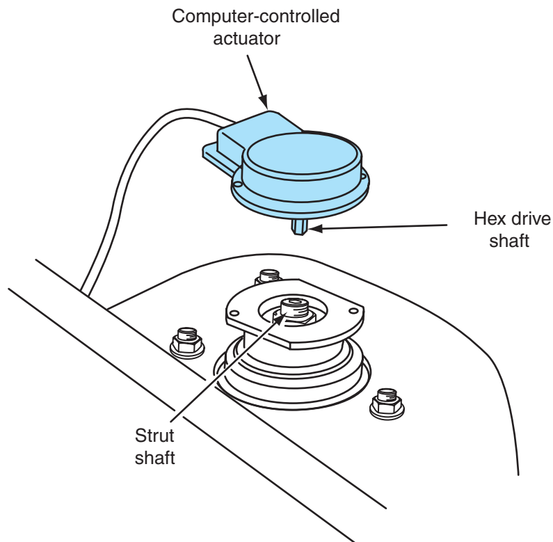
Figure 5-16 Computer-controlled strut actuator.
