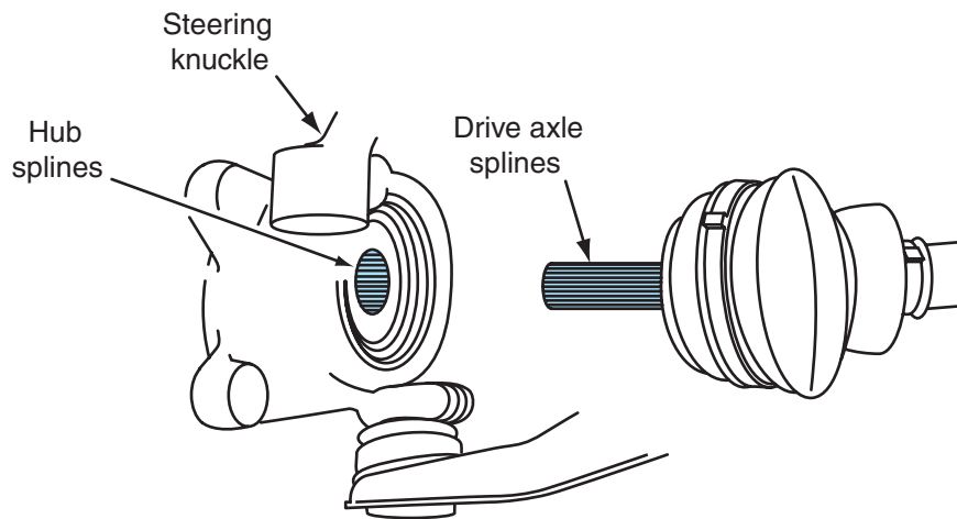
Figure 3-16 Front drive shaft installed in wheel bearing hub.
