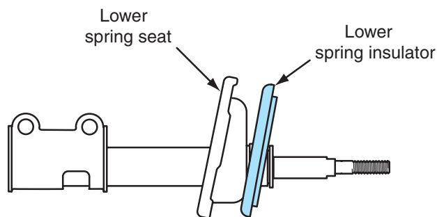
Figure 7-18 Inspecting lower spring seat and insulator.
