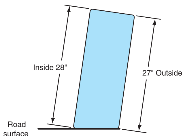
Figure 15-34 Excessive positive camber causes a smaller diameter on the outside edge of the tire compared to the inside edge of the tire.
