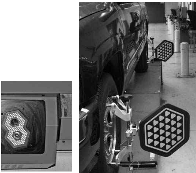
Figure 15-11 One digital camera is aimed at each wheel target.
