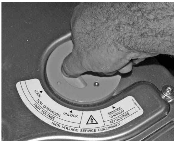
Figure 12-40 High voltage service disconnect on a hybrid vehicle.
