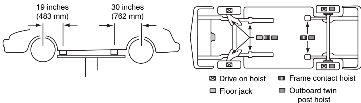
Figure 2-39 Lift points for a typical unibody vehicle.
