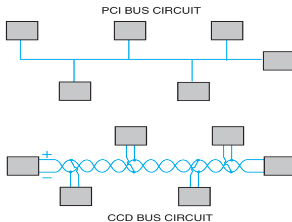
Figure 8-44 Comparison between PCI and CCD data link systems.
