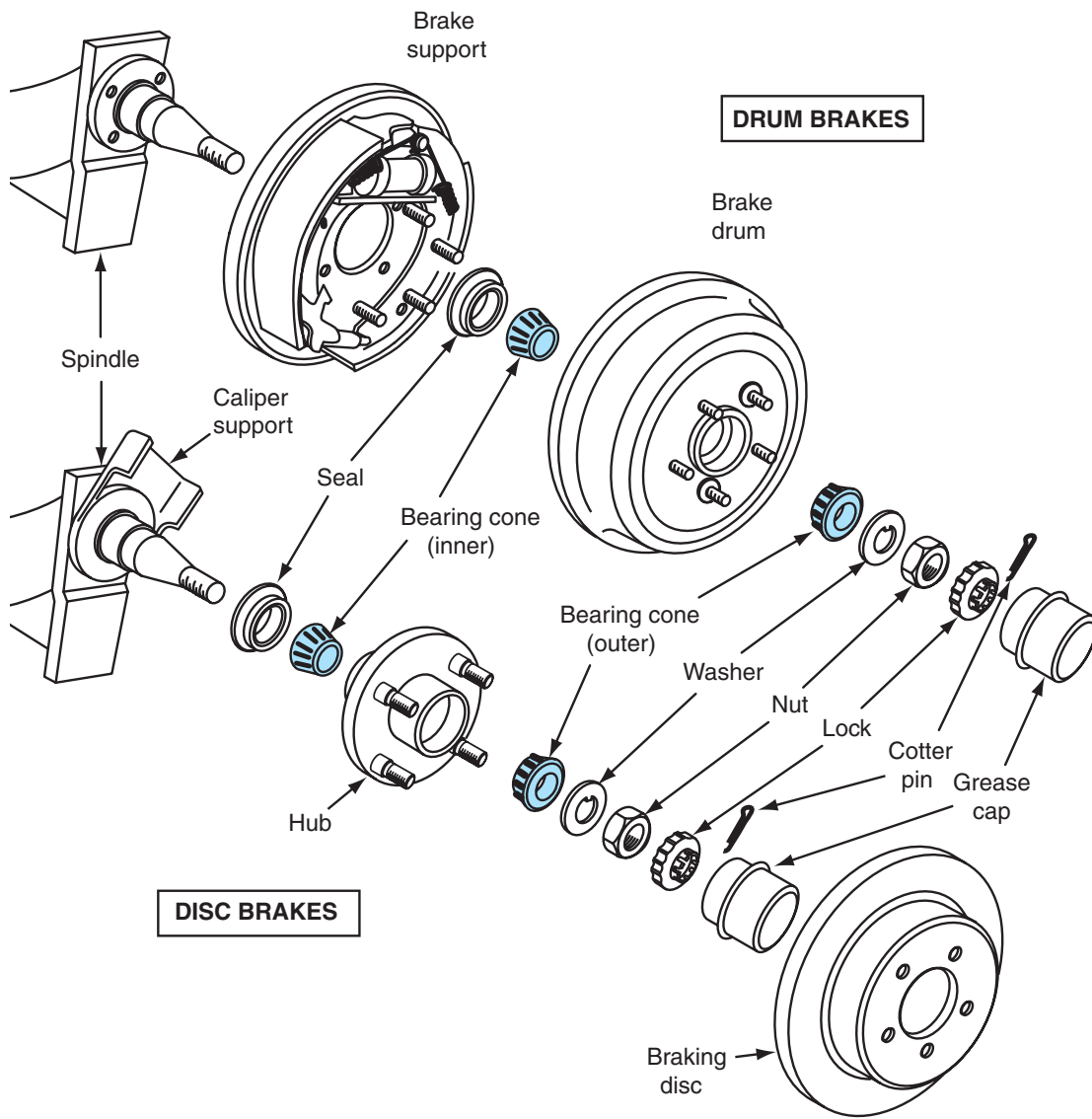
Figure 3-21 Rear wheel hub with tapered roller bearings for drum or disc brakes, front-wheel-drive car.
