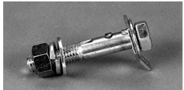
Figure 16-10 Camber adjustment kits provide 2\frac{1}{2}^\circ camber adjustment on some vehicles.
