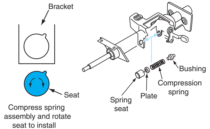
Figure 9-38 Installing tension spring.
