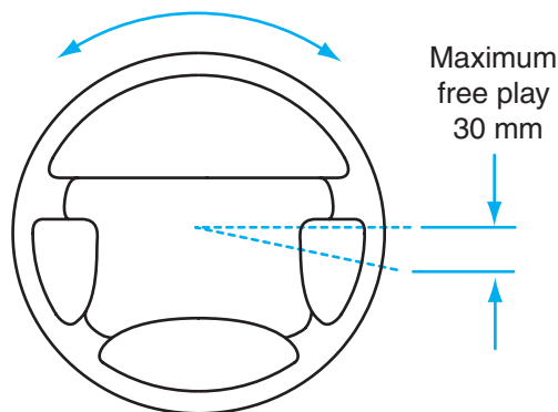
Figure 9-41 Measuring steering wheel free play.
