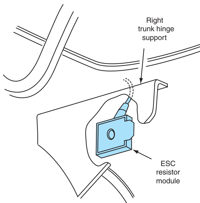
Figure 8-39 Resistor module mounting location.
