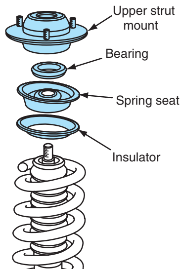
Figure 5-12 Removal of the upper strut mount, bearing, upper spring seat, and insulator.
