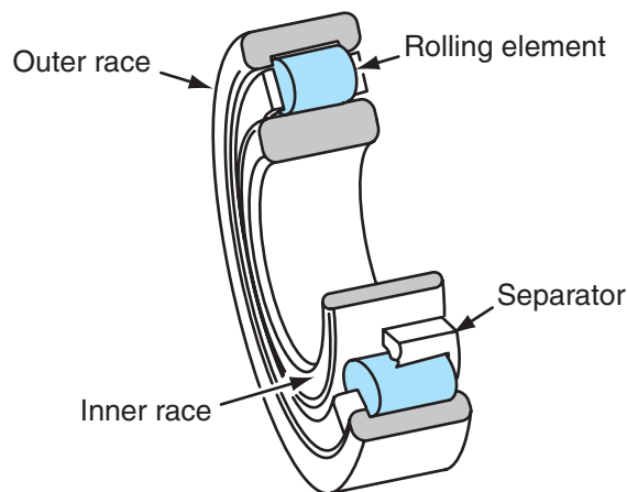
Figure 3-6 Parts of a roller bearing.
