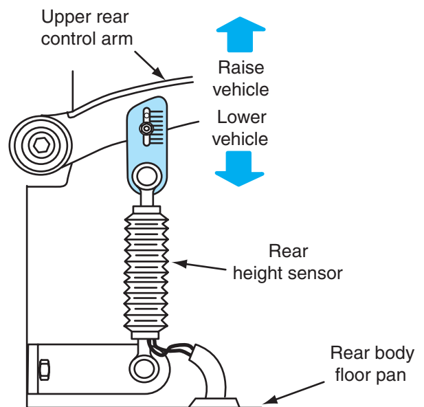
Figure 8-11 Rear trim height adjustment.
