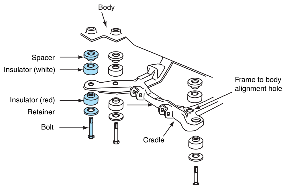
Figure 16-38 Cradle insulators and alignment holes in cradle and body.
