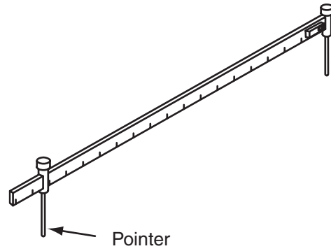
Figure 2-23 Tram gauge.
