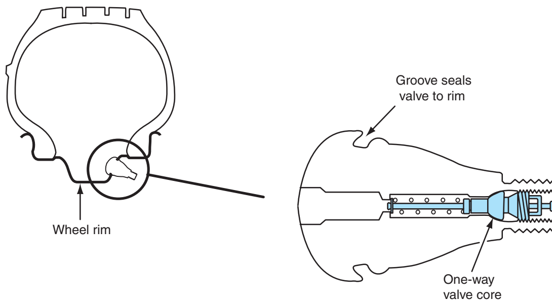
Figure 4-13 Valve core.
