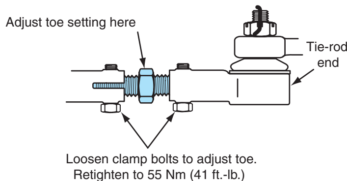
Figure 16-42 Rack and pinion steering gear with externally threaded toe adjuster and internal threads on the tie-rod and outer tie-rod end.
