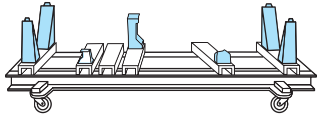
Figure 14-19 Dedicated fixtures are bolted to the transverse beams in specific locations depending on the body style.
