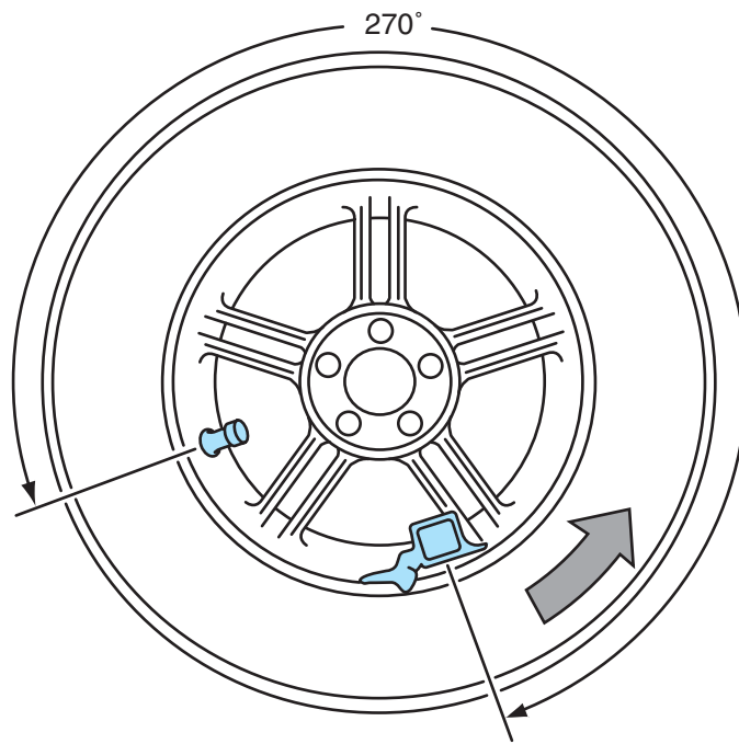
Figure 4-15 Proper tire and wheel position on a tire changer.
