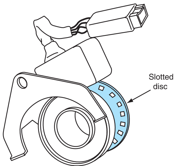
Figure 8-2 Steering sensor.
