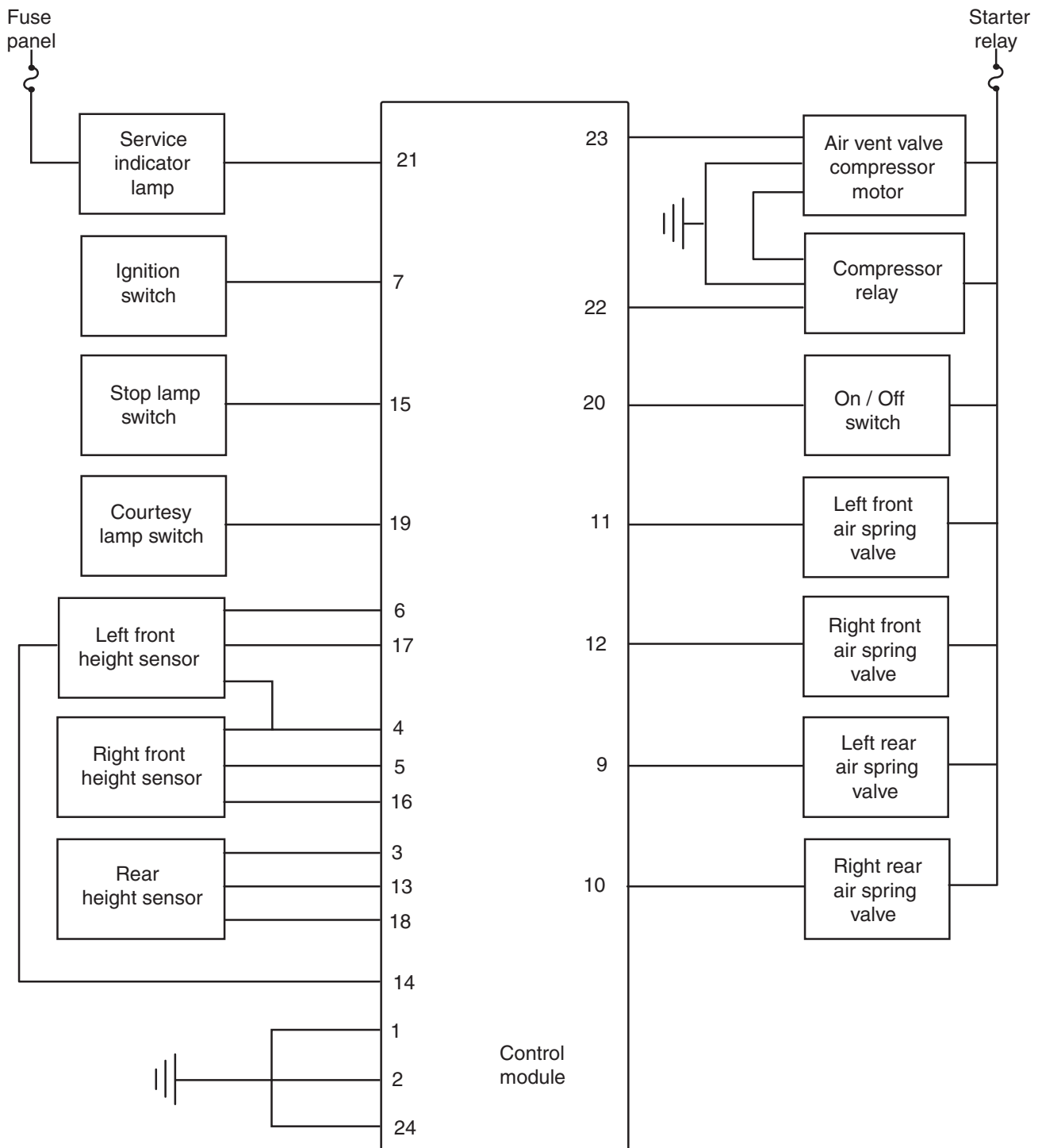
Figure 8-25 Air suspension wiring diagram.
