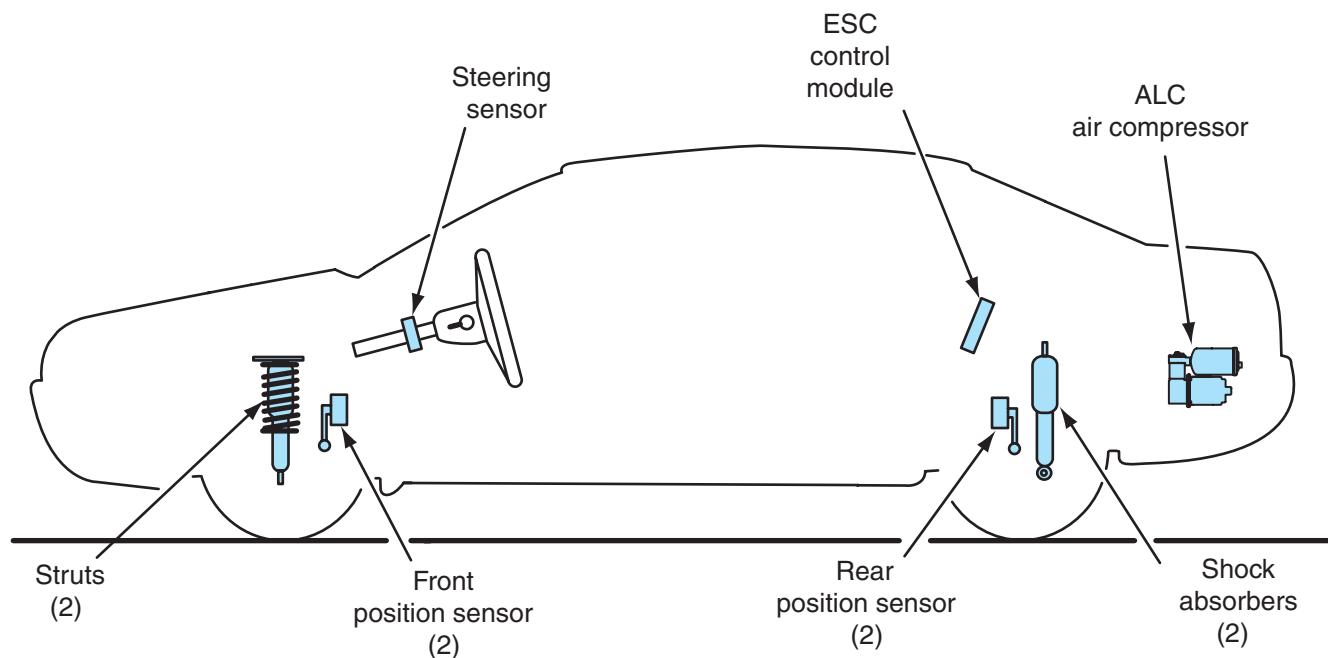
Figure 8-28 Electronic suspension control (ESC) system.
