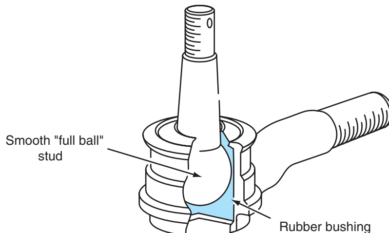
Figure 9-21 Outer tie-rod end with rubber encapsulated ball stud.
