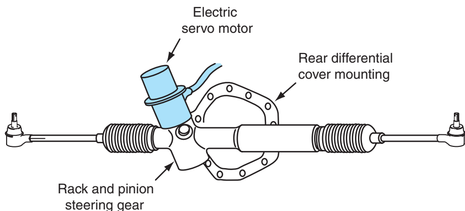
Figure 1-31 Rear electronic power steering gear, four-wheel steering.
