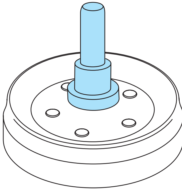
Figure 3-9 Seal installation.
