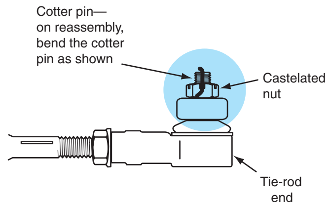
Figure 13-27 Proper installation of cotter pin in the tie-rod end.
