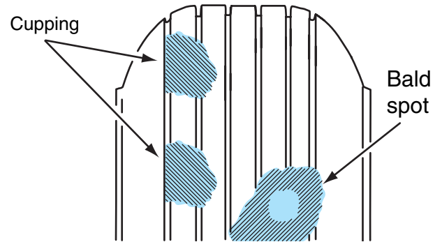
Figure 4-28 Cupped tire tread wear with bald spots on the tread caused by improper static or dynamic wheel balance.
