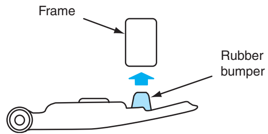
Figure 6-39 Rebound bumper.
