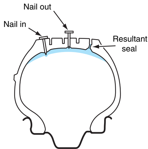
Figure 4-11 Puncture sealing tire.
