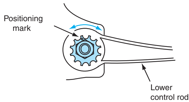
Figure 16-57 Eccentric star wheel on inner end of lower control rod for toe adjustment.
