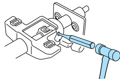
Figure 9-36 Staking upper column tube.
