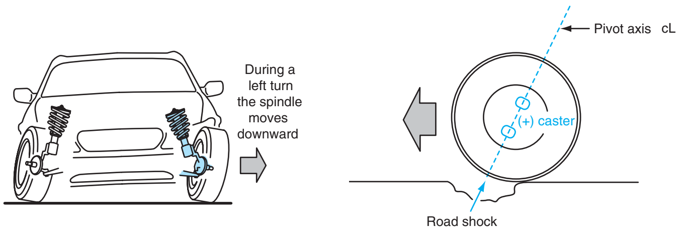
Figure 15-43 Left front spindle movement during a left turn.
