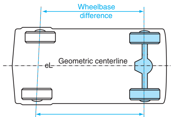
Figure 15-29 Wheelbase difference.
