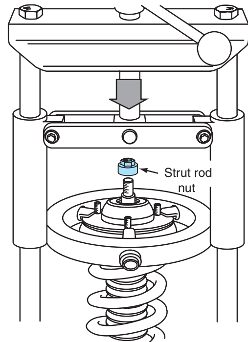
Figure 7-16 A spring compressing tool is used to compress the coil spring.
