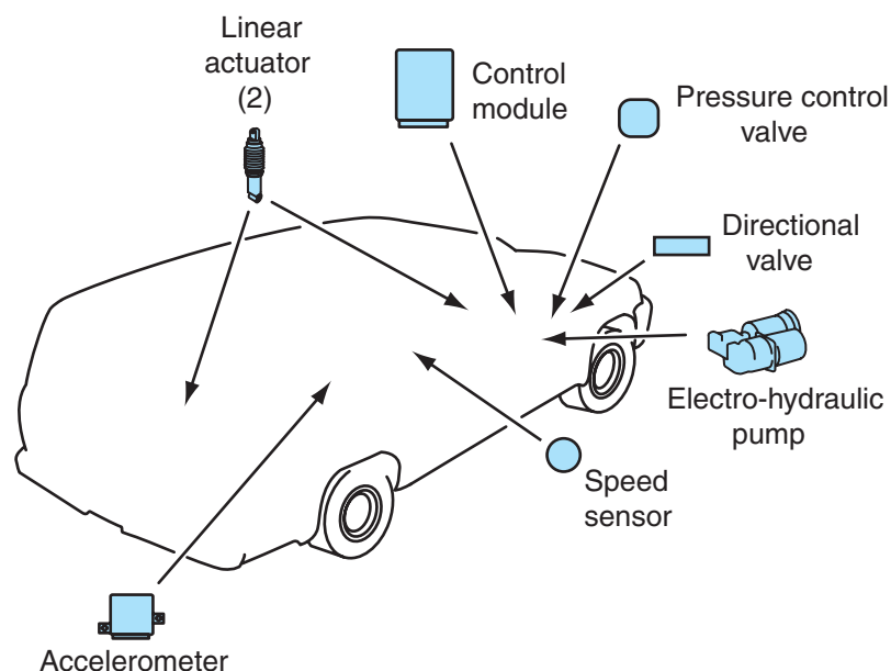
Figure 8-57 Active roll control system components.
