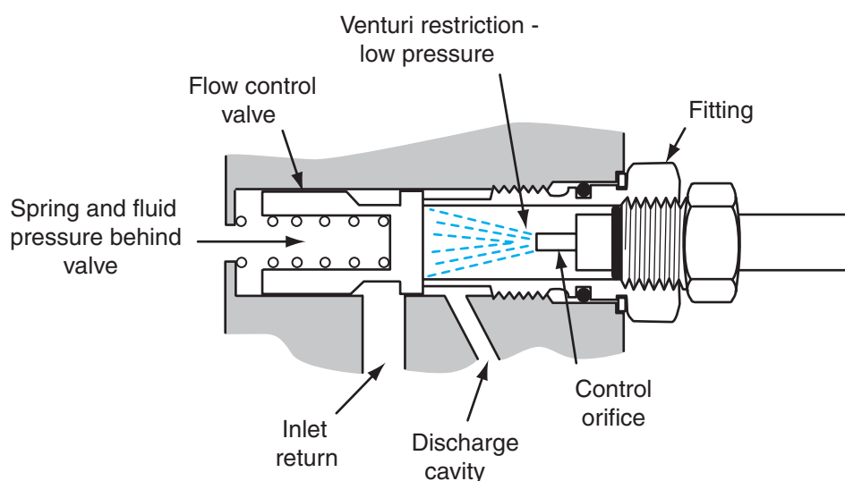
Figure 10-14 Power steering pump fluid flow to control valve and outlet fitting.
