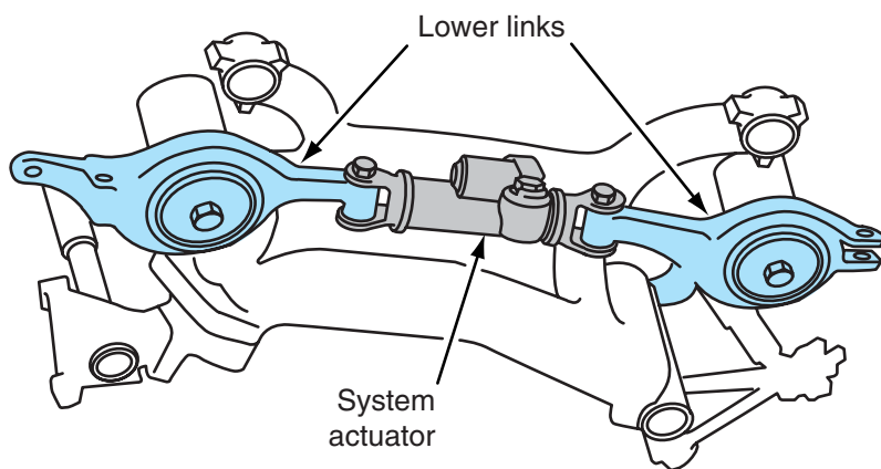
Figure 13-18 Rear steering actuator and adjustable lower links.
