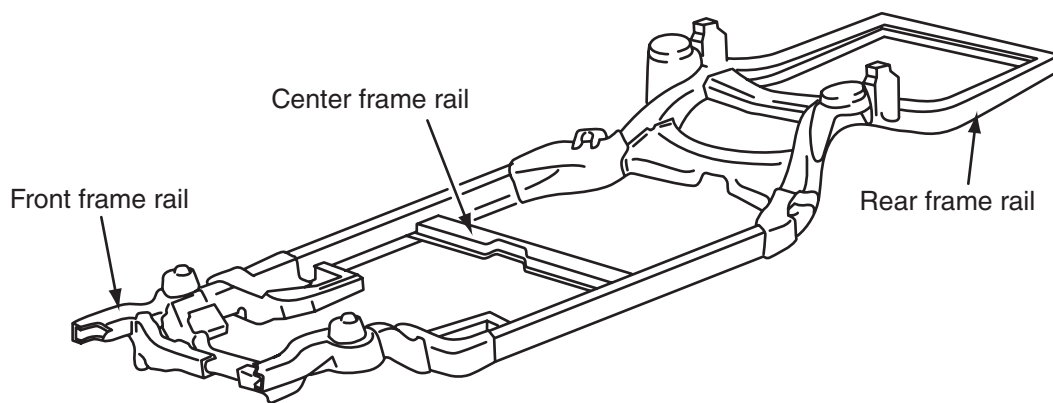
Figure 14-3 Perimeter-type frame components.
