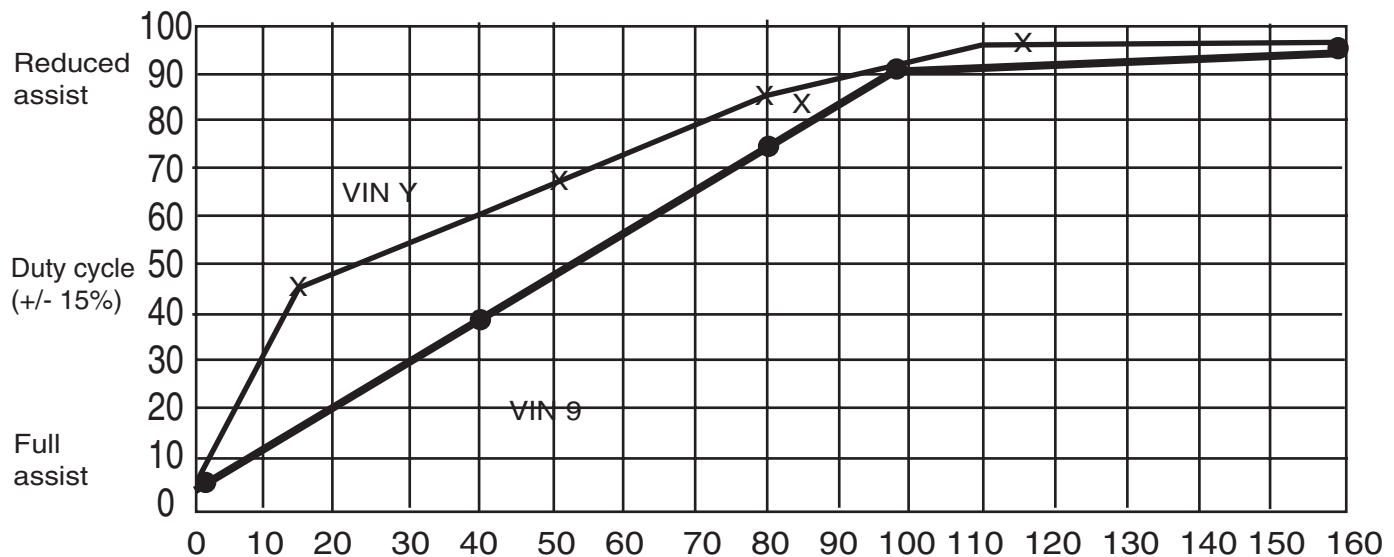
Figure 8-43 Power steering assist in relation to vehicle speed.
