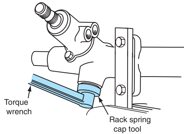
Figure 12-32 Installing rack spring cap.
