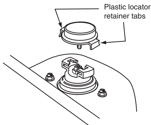
Figure 5-36 Electronically controlled strut actuator.
