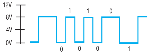
Figure 8-46 Voltage level and duration required for 0 and 1 signals.
