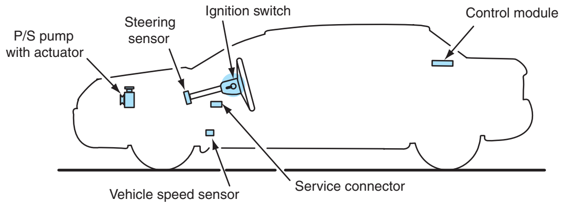
Figure 12-14 Control module and main components, electronic variable orifice steering.
