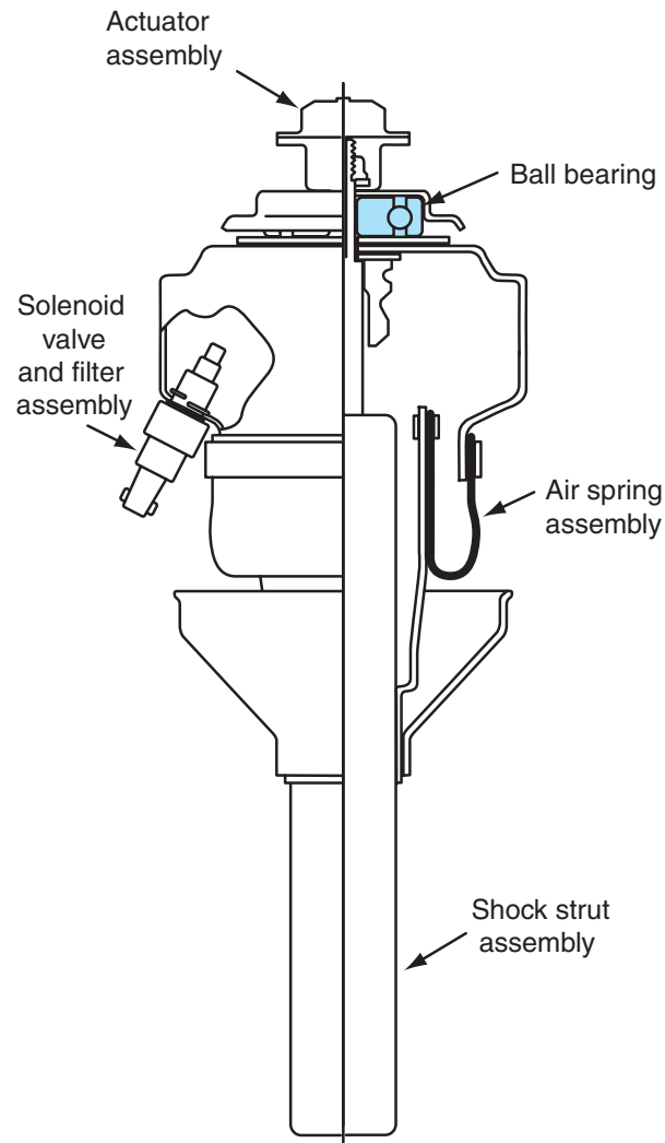
Figure 1-19 Air spring and strut assembly.
