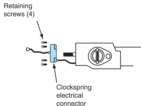
Figure 9-6 Removing clock spring electrical connector.
