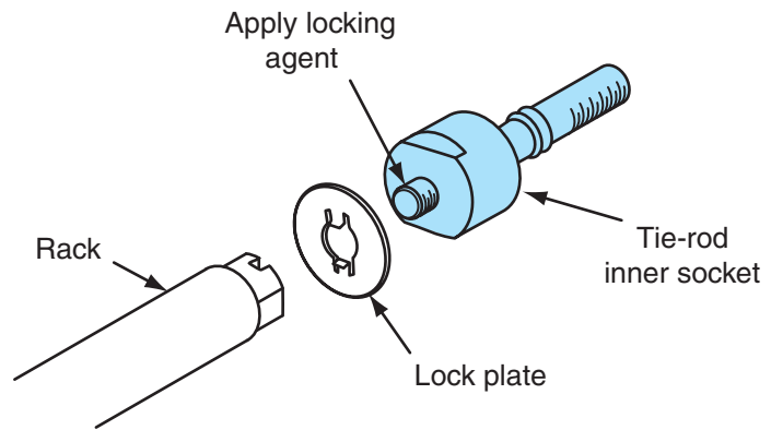
Figure 12-15 Removing inner tie-rod end from the rack.
