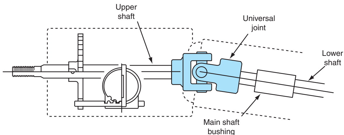
Figure 9-10 Tilt steering column components.
