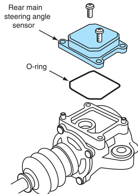
Figure 13-25 Removing the rear main steering angle sensor.
