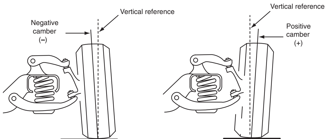
Figure 15-29 Negative and positive camber angles on a short-and-long arm front suspension system.
