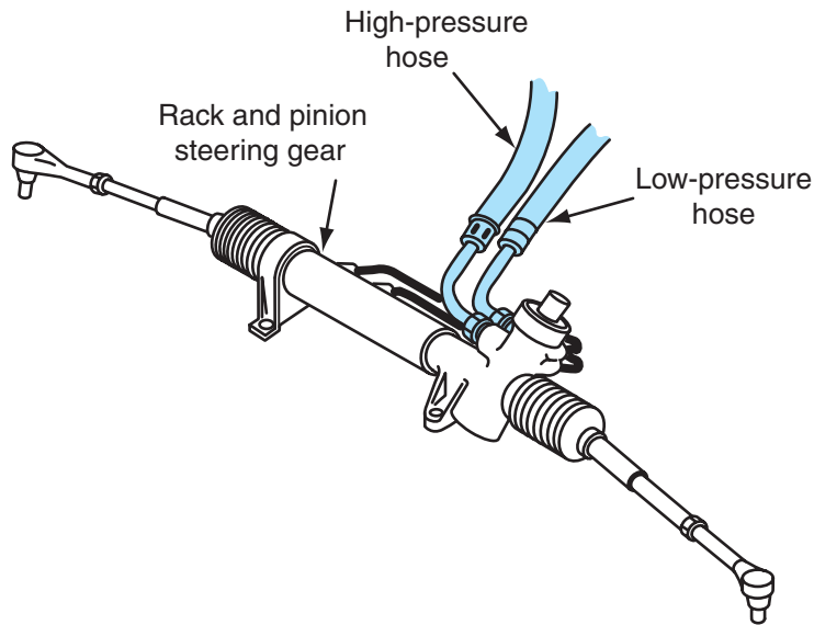
Figure 10-5 Power steering pump to gear hoses.
