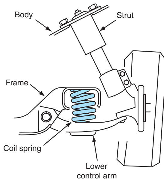
Figure 6-37 Modified MacPherson strut front suspension system.
