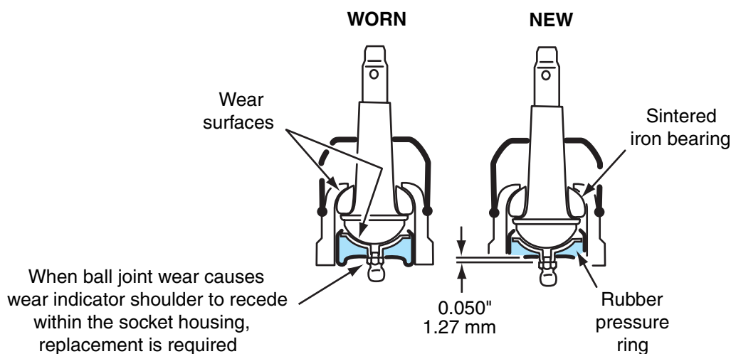
Figure 6-6 Ball joint wear indicator with grease fitting extending from ball joint surface.
