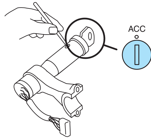
Figure 9-27 Depressing stop pin in release ignition switch cylinder.
