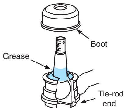
Figure 13-17 Packing the boot and tie-rod end with grease.
