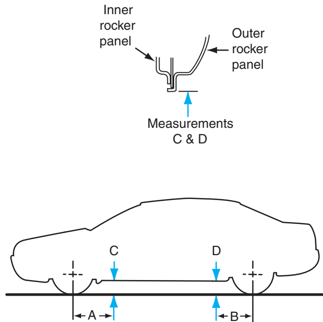
Figure 7-49 Front and rear curb riding height measurement locations.
