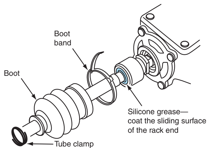
Figure 13-21 Lubricating of the inner tie-rod joint housing.
