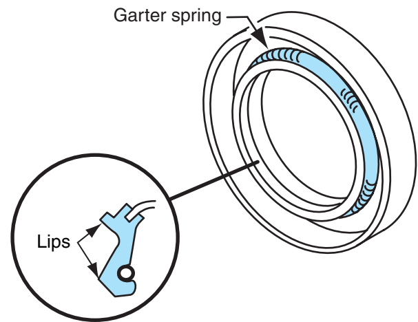
Figure 3-11 Spring-loaded seal.
