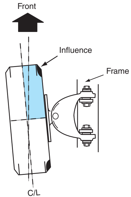
Figure 4-41 Dynamic wheel unbalance with heavy spot at the front of the left front tire.
