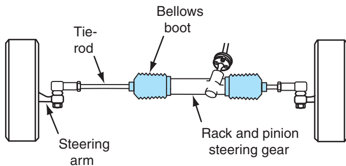
Figure 9-27 Rack and pinion steering gear.
