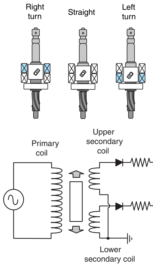
Figure 12-26 Slider movement when turning the steering wheel.
