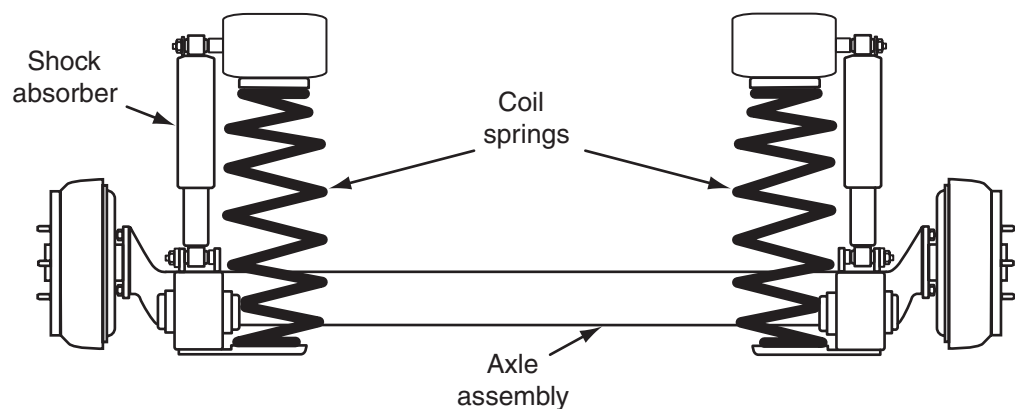
Figure 7-17 Semi-independent rear suspension system with coil springs and shock absorbers mounted separately.
