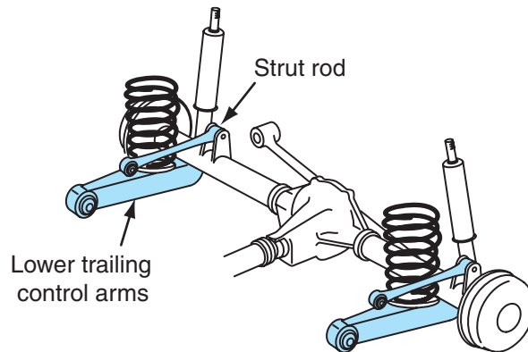
Figure 1-7 Live-axle rear suspension system with coil springs.
