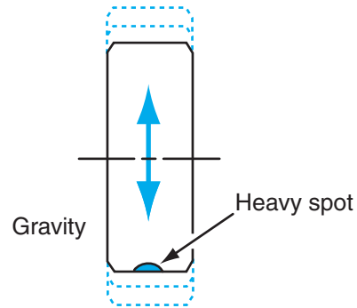
Figure 4-35 Effects of static unbalance.
