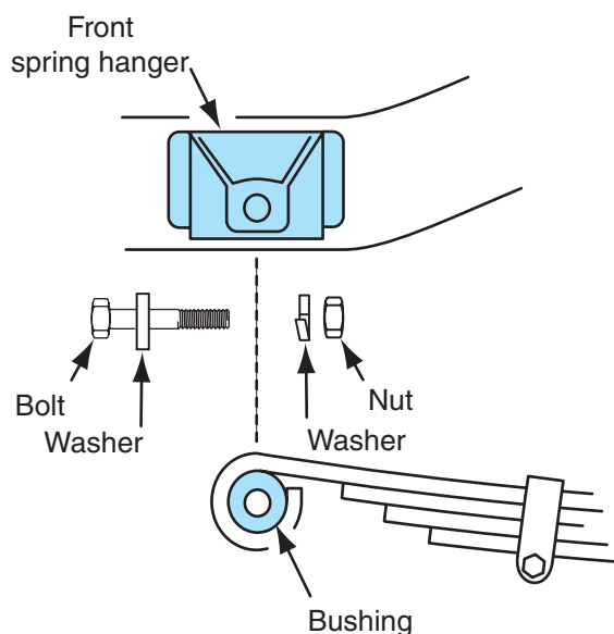
Figure 7-7 Rear leaf-spring eye bushing.
