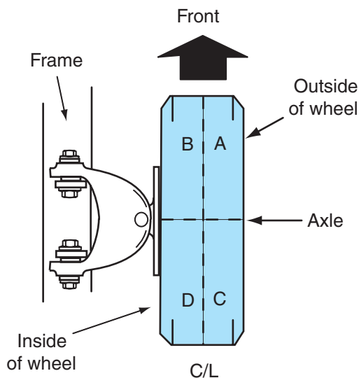
Figure 4-38 Dynamic wheel balance theory.
