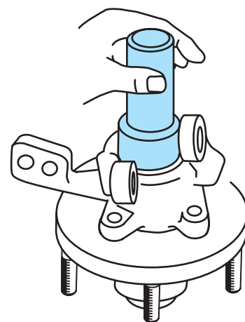
Figure 6-20 Installing dust deflector in the steering knuckle.
