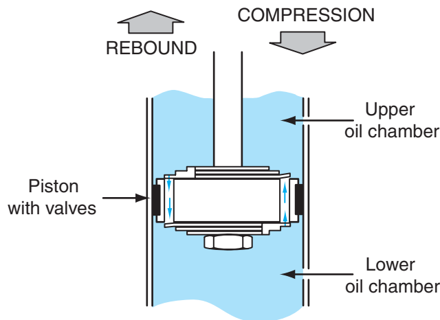
Figure 5-2 Shock absorber action.
