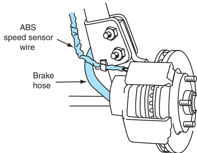
Figure 5-24 Brake hose and ABS wire installed in strut clamps.
