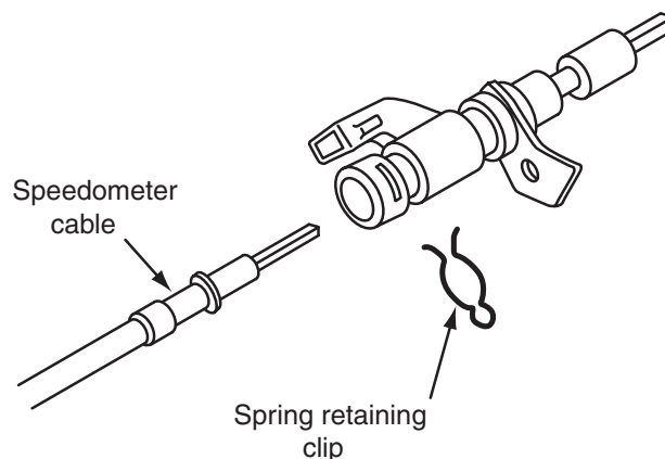
Figure 8-4 Vehicle speed sensor.
