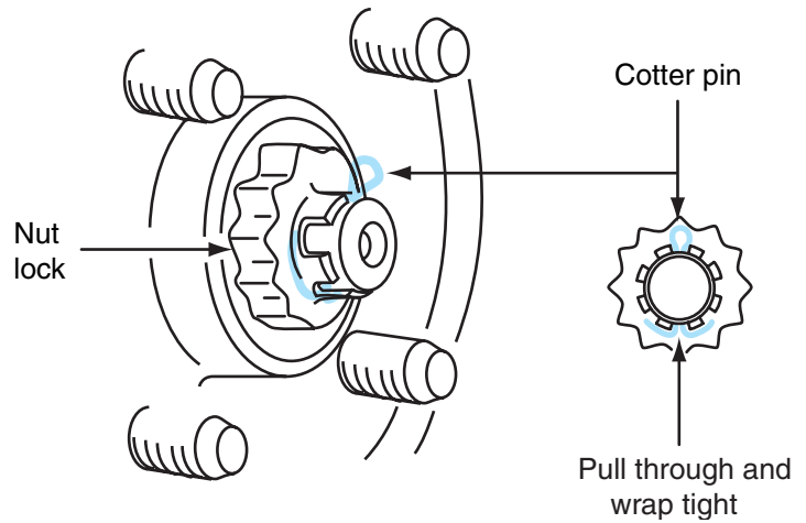
Figure 3-26 Nut lock and cotter pin installation.
