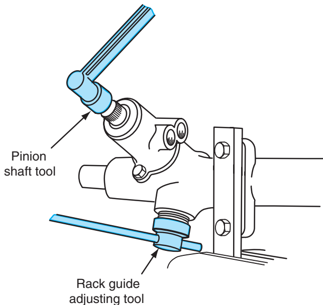
Figure 12-33 Adjusting pinion shaft turning torque.
