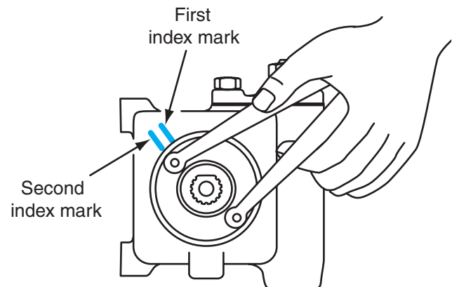
Figure 11-5 Aligning adjuster plug hole with the second index mark placed on steering gear housing.
