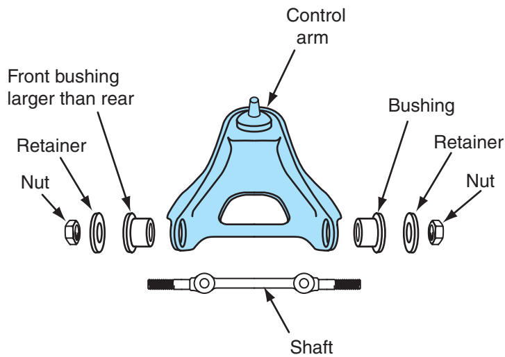
Figure 6-38 Upper control arm components.
