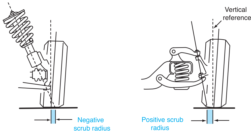
Figure 16-5 Scrub radius.
