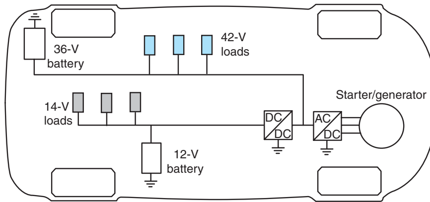
Figure 10-18 42-volt electrical system components.
