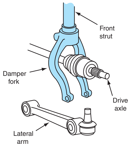
Figure 6-44 Multilink front suspension damper fork.
