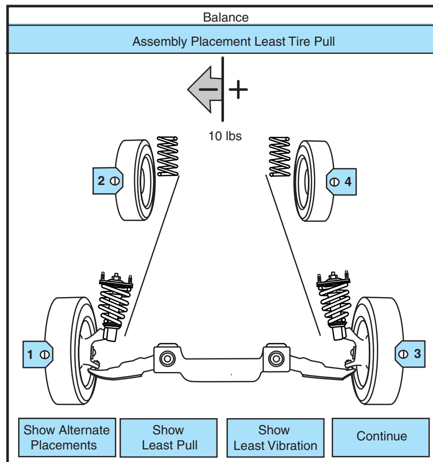
Figure 4-31 The balancer display indicates the location on the vehicle where each numbered tire should be installed.
