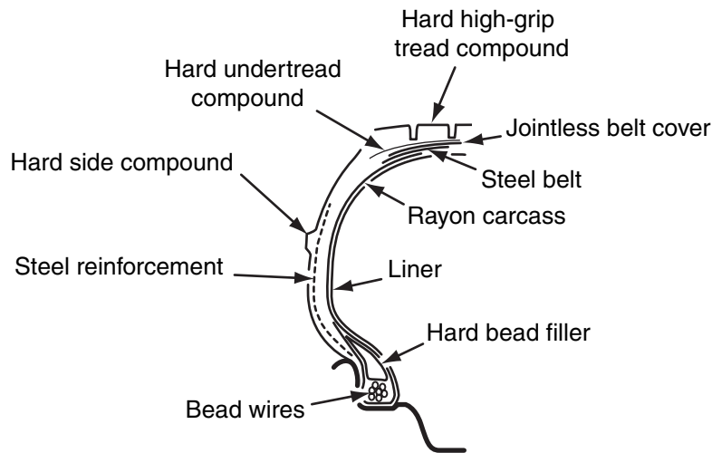
Figure 4-1 Tire design.
