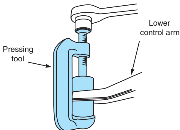
Figure 6-25 Removing the pressed-in ball joint from the lower control arm.
