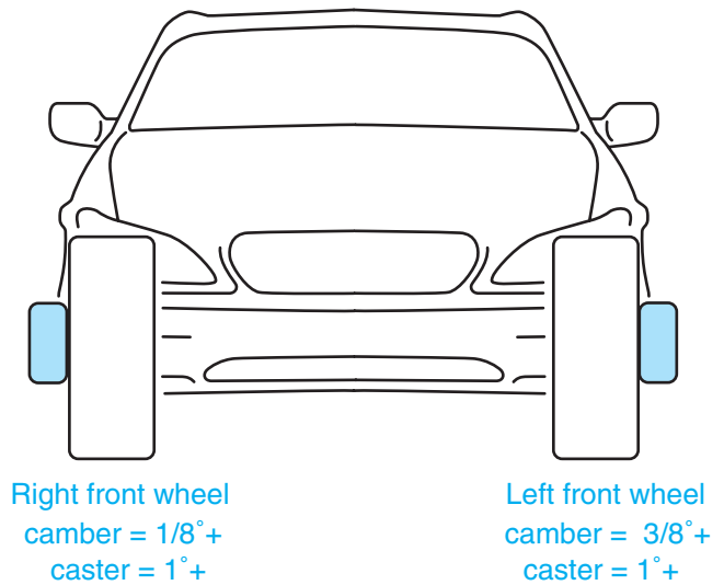
Figure 15-38 Camber setting to offset road crown.
