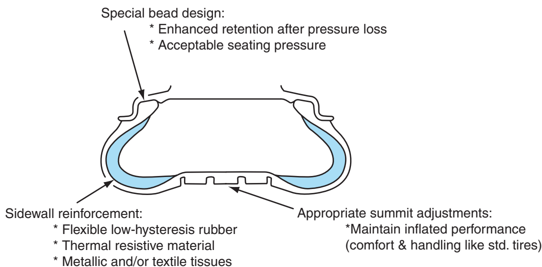
Figure 4-16 Run-flat tire with sidewall reinforcement.
