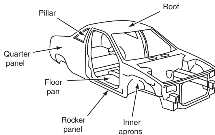
Figure 1-2 Unitized body design.
