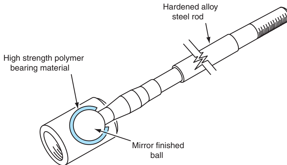
Figure 9-29 Inner tie-rod design.
