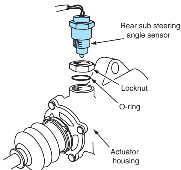
Figure 13-24 Removing the rear sub steering angle sensor.
