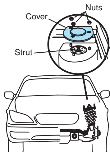
Figure 8-8 Removing the upper strut mount retaining nuts.
