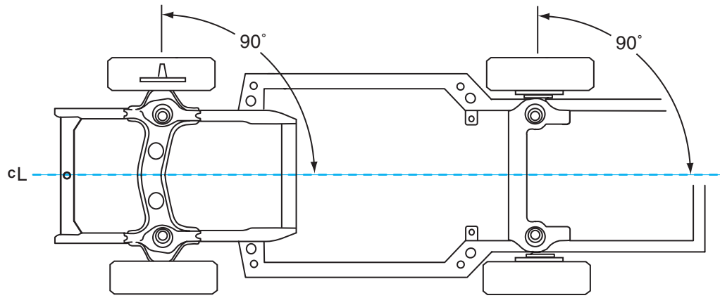
Figure 14-6 To provide accurate wheelbase measurement, the front spindle centerlines and the rear axle centers must be at a 90° angle to the vehicle centerline.
