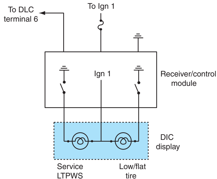
Figure 4-21 Warning lights in tire pressure monitoring system.
