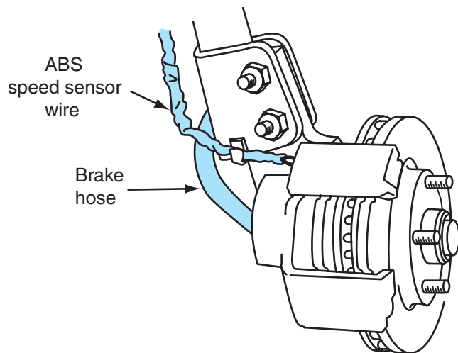
Figure 7-11 Disconnecting brake hose and ABS wire from the rear strut.
