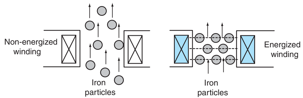
Figure 1-18 Magneto-rheological fluid action in a strut or shock absorber.
