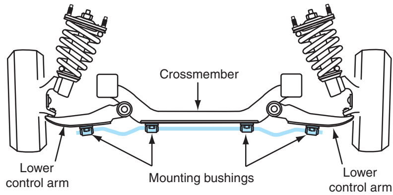
Figure 6-15 Stabilizer bar with mounting bushings.
