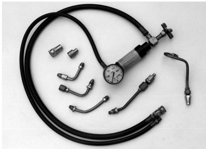
Figure 2-16 Power steering pressure gauge.
