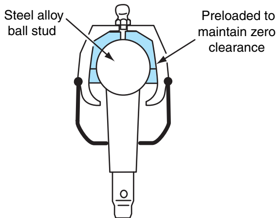
Figure 6-8 Compression-loaded ball joint.
