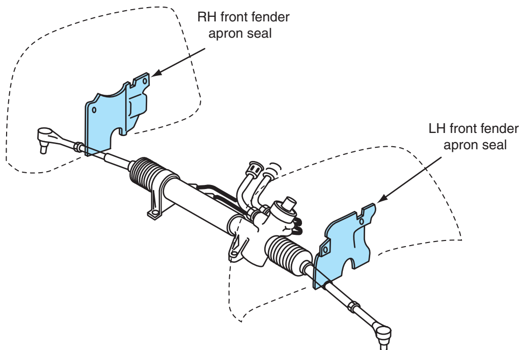
Figure 12-4 Left and right fender apron seals.
