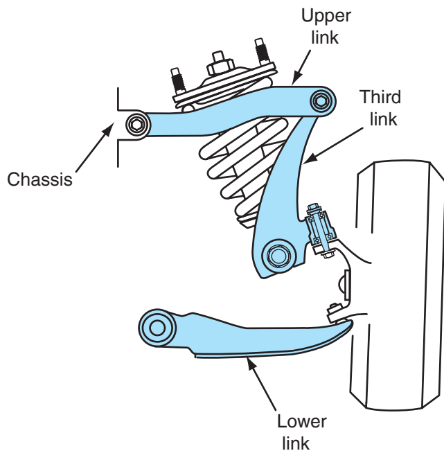
Figure 5-7 Multilink front suspension with strut connected between the upper link and the strut tower.
