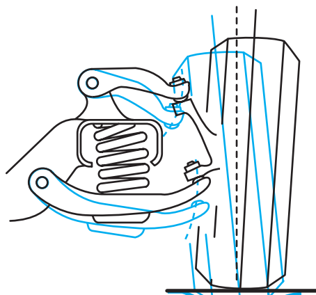
Figure 15-31 Camber change during wheel rebound.
