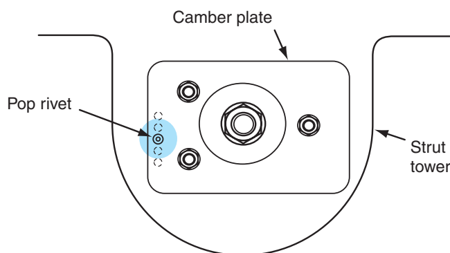
Figure 16-19 Upper strut mount with camber plate and rivet, modified MacPherson strut front suspension.
