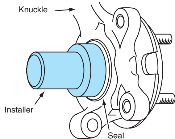
Figure 3-24 Seal installation in steering knuckle.
