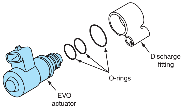
Figure 12-18 Actuator solenoid.
