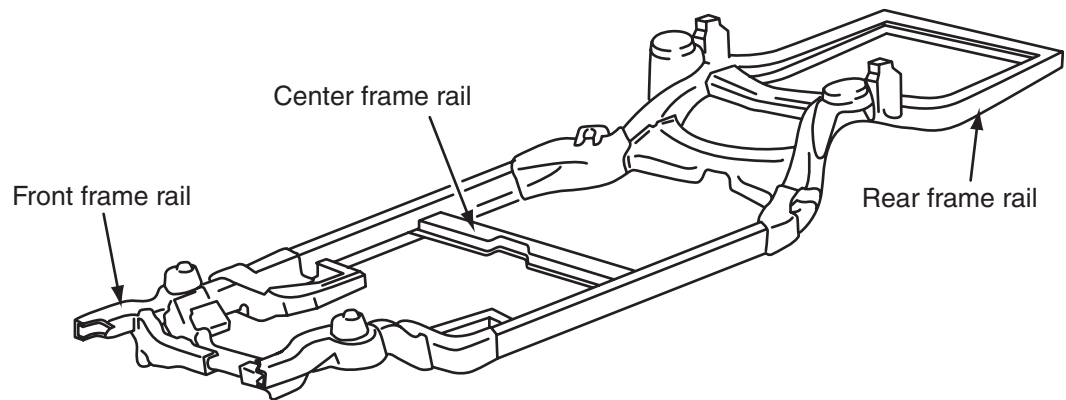
Figure 1-1 Vehicle frame.
