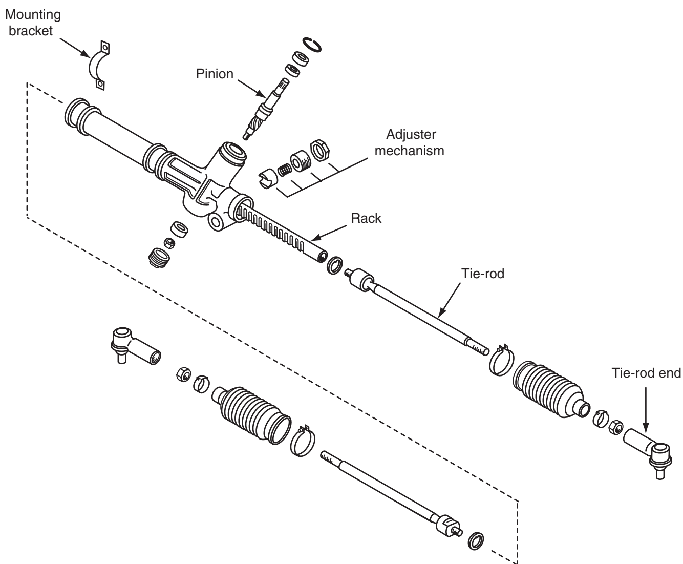
Figure 12-1 Manual rack and pinion steering gear components.
