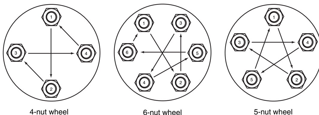
Figure 4-5 Wheel nut tightening sequence.
