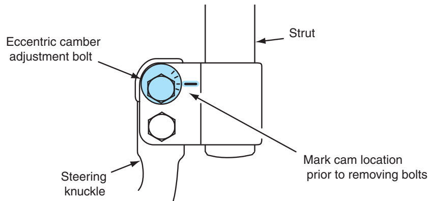
Figure 16-8 Eccentric steering knuckle-to-strut camber adjusting bolt, MacPherson strut front suspension.
