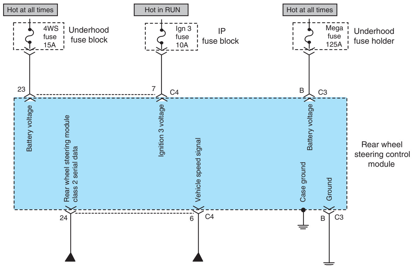
Figure 13-7 Battery and ignition voltage inputs to the rear wheel steering control module.
