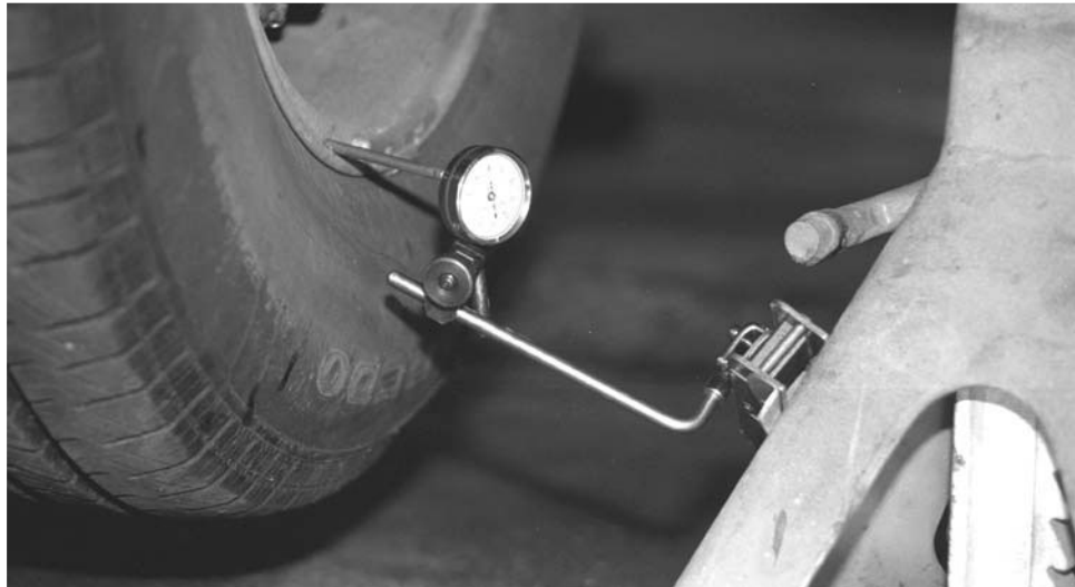
Figure 2-43 Dial indicator installed to measure horizontal joint movement.
