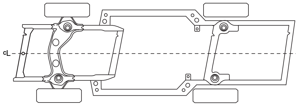
Figure 14-14 Diamond-frame condition.
