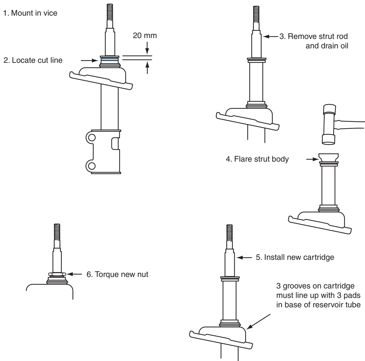
Figure 5-25 Installation of strut cartridge.
