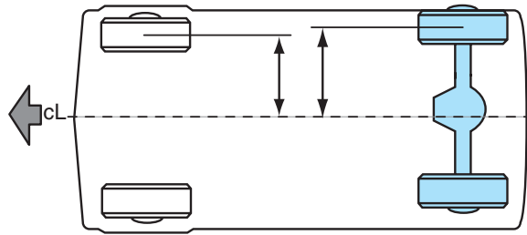
Figure 14-9 Axle sideset occurs when the rear axle moves inward or outward and the axle centerline remains at a 90° angle in relation to the vehicle centerline.
