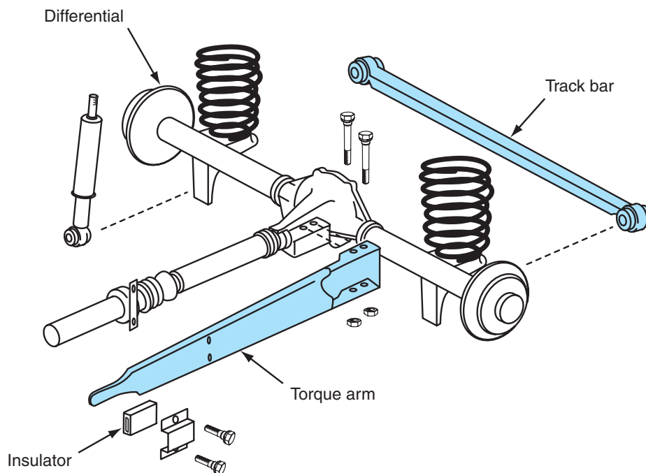
Figure 7-11 Rear suspension system with long torque arm and track bar.
