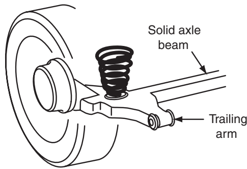
Figure 7-16 Semi-independent rear suspension system.
