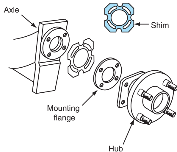
Figure 16-54 Adjusting rear wheel toe by changing shim thickness between rear spindle and mounting flange.
