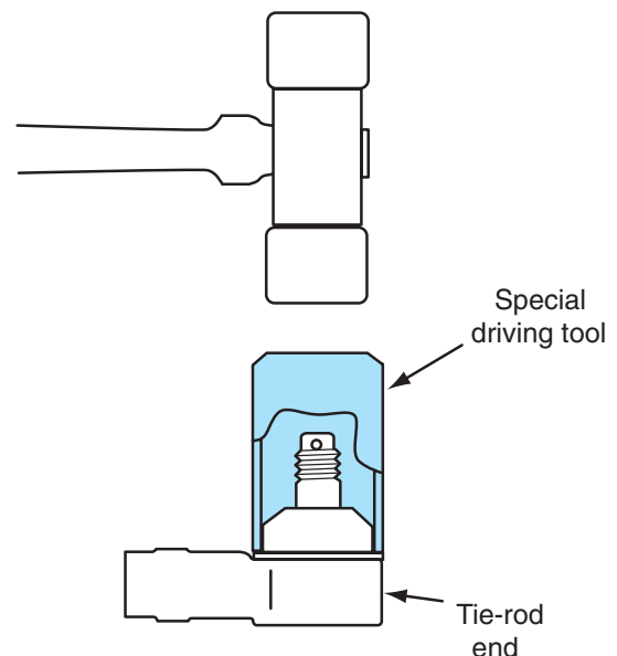
Figure 13-18 Driving the boot onto the tie-rod end with a special driving tool.
