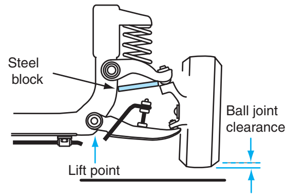
Figure 6-8 Floor jack position to check ball joint wear with spring between the upper control arm and the chassis.
