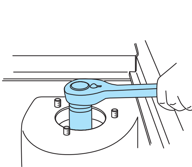
Figure 5-30 Removing jounce bumper retainer.
