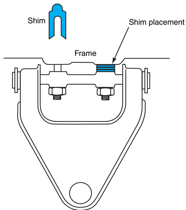
Figure 16-4 Shim-type camber adjustment between upper control arm mounting and the outside of the frame.
