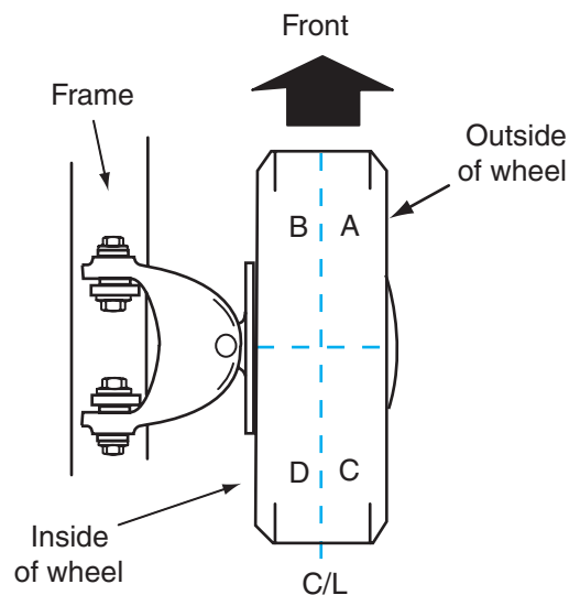
Figure 2-13 Weight must be distributed equally in relation to the tire and wheel centerline.
