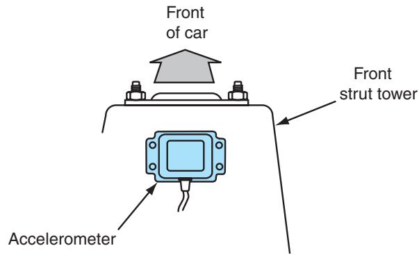
Figure 8-32 Front accelerometer mounting location.
