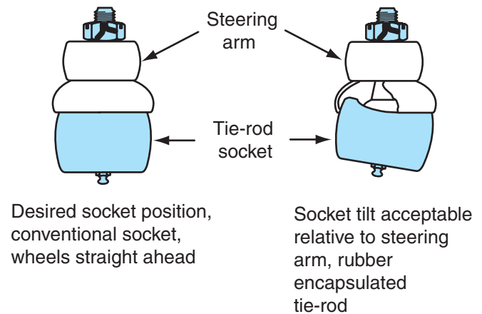
Figure 9-49 Rubber-encapsulated tie-rod end housing may be tilted to one side after it is installed and tightened.
