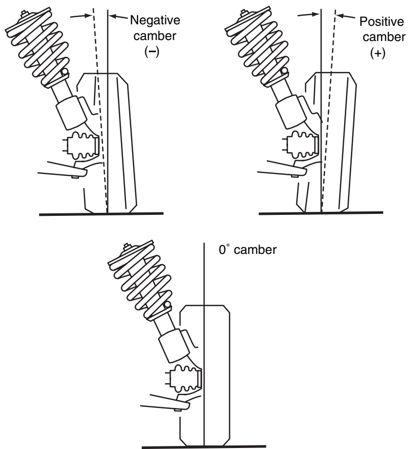
Figure 15-28 Negative and Positive camber angles on a MacPherson strut front suspension system.
