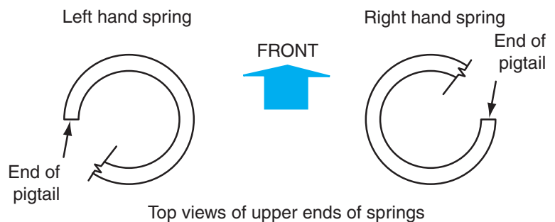
Figure 7-29 Proper location of upper coil spring ends in relation to the front of the vehicle.
