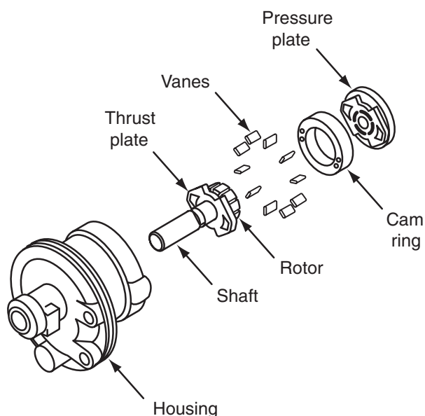
Figure 10-11 Power steering pump housing with shaft and rotor, vanes, cam ring, and pressure plate.
