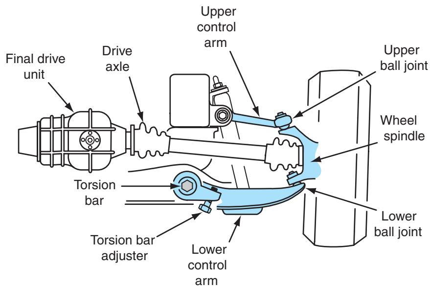
Figure 6-47 Front suspension system with longitudinal torsion bars.
