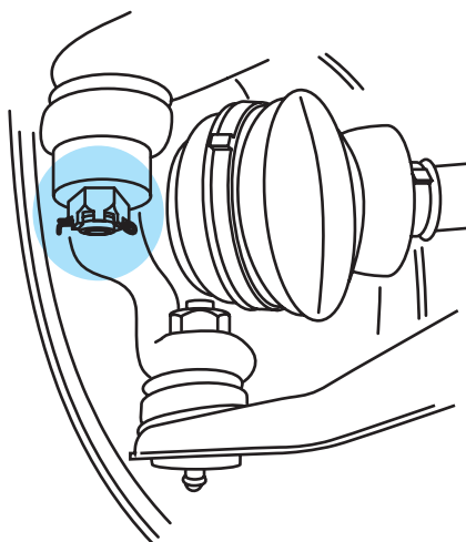
Figure 9-46 Tie-rod nut and cotter pin installation.
