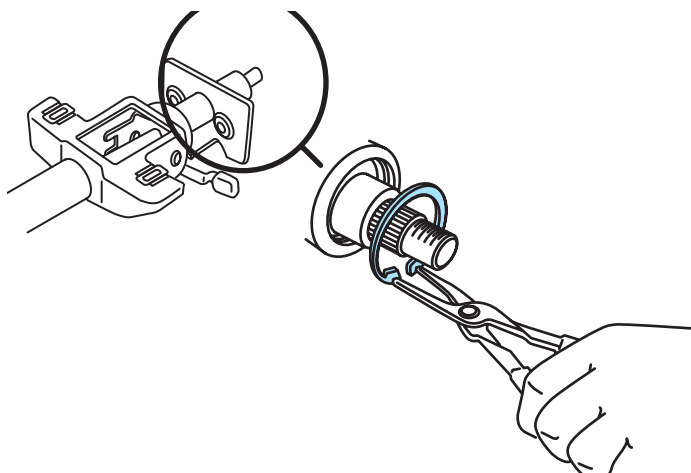
Figure 9-19 Removing snapping from upper column tube.
