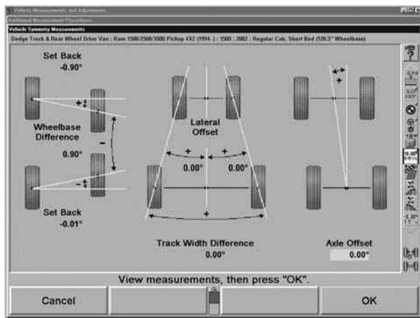
Figure 15-27 Symmetry angle measurements. (Courtesy of Hunter Engineering Company.)
