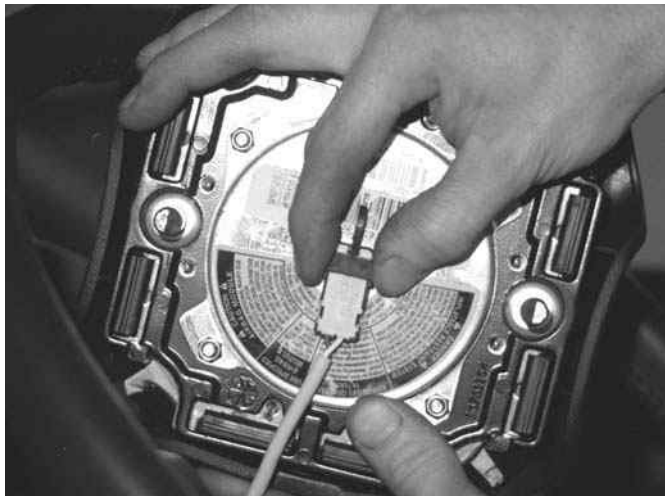
Figure 9-3 Disconnecting the air bag module electrical connector.
