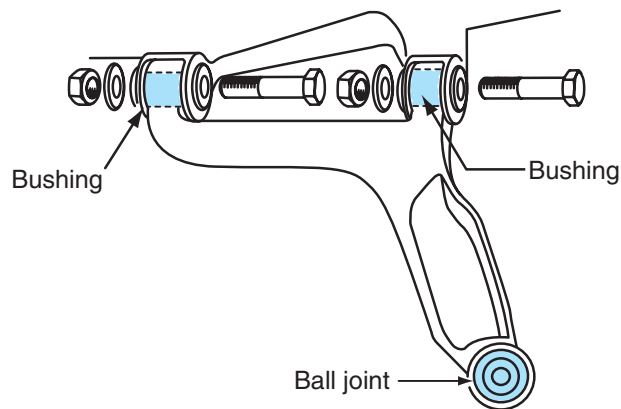
Figure 7-32 The upper control arm is connected from the frame to the top of the knuckle.
