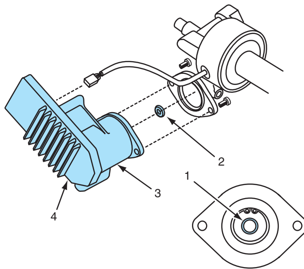
Figure 12-45 Removing and replacing the PSCM and motor assembly.
