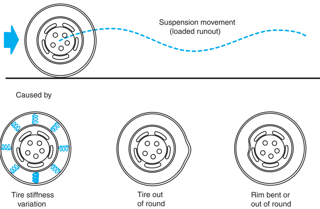
Figure 4-17 Vertical tire and wheel vibrations caused by radial tire or wheel runout, or variation in tire stiffness.
