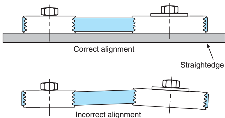
Figure 10-6 Checking pulley alignment.
