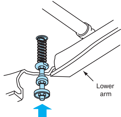
Figure 7-10 Disconnecting nut from small spring in the lower arm.
