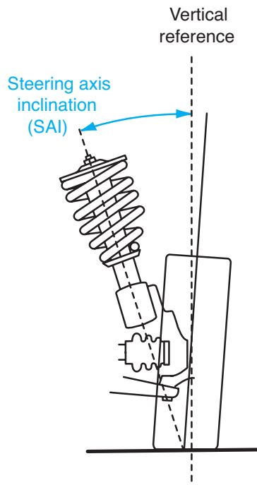
Figure 16-1 Steering axis inclination angle.
