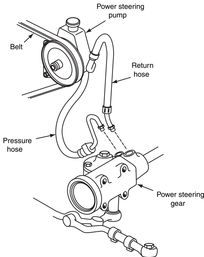
Figure 1-28 Power steering system.
