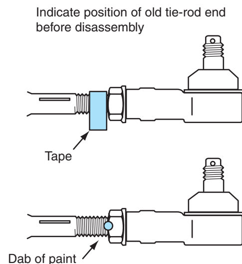
Figure 12-13 Marking outer tie-rod end and jam nut position.
