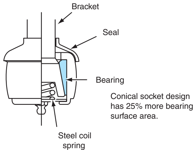
Figure 9-25 Idler arm with conical bearing.
