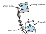
Figure 3-6 Parts of a roller bearing.
