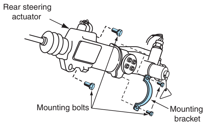
Figure 13-26 Installing the rear steering actuator, four mounting bolts, and bracket.
