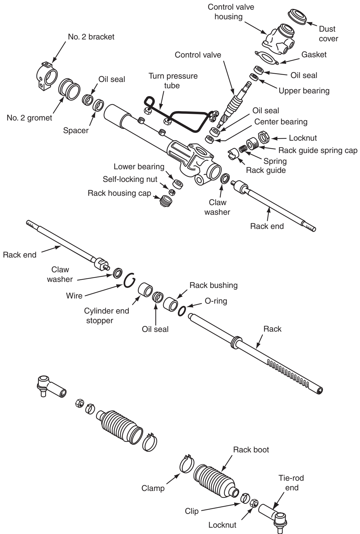
Figure 12-11 Toyota power rack and pinion steering gear.
