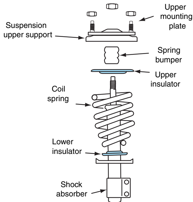
Figure 7-20 Upper and lower spring insulators, MacPherson strut independent rear suspension.
