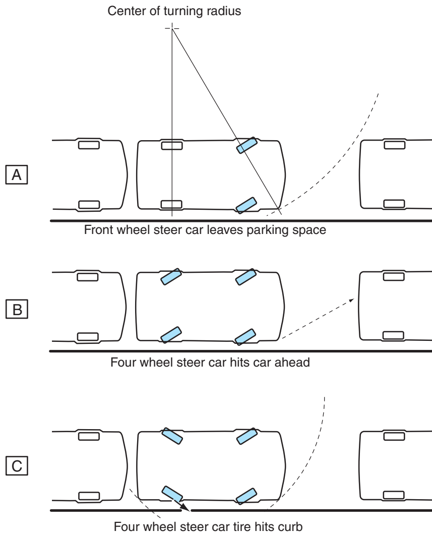
Figure 13-1 Parallel parking with conventional front wheel steering and four-wheel steering.
