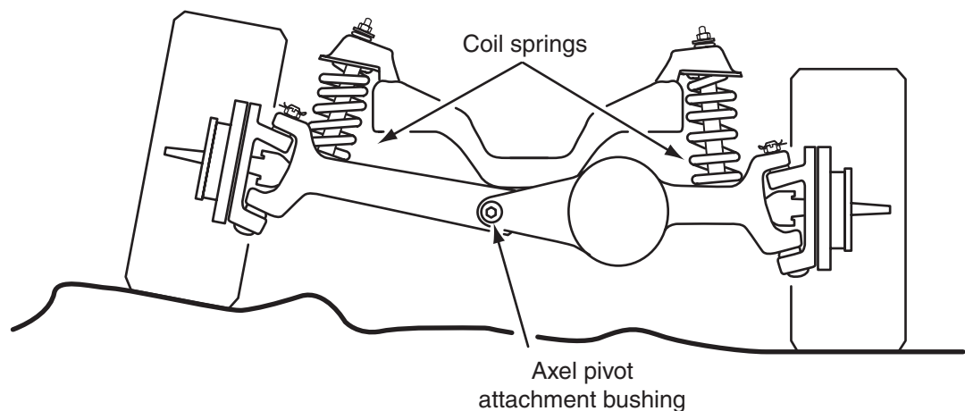
Figure 6-49 Four-wheel-drive twin I-beam front suspension with coil springs.
