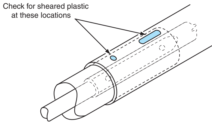
Figure 9-10 Inspecting for sheared plastic in jacket openings.
