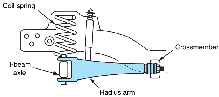
Figure 6-50 Radius arms on a twin I-beam front suspension system with coil springs.
