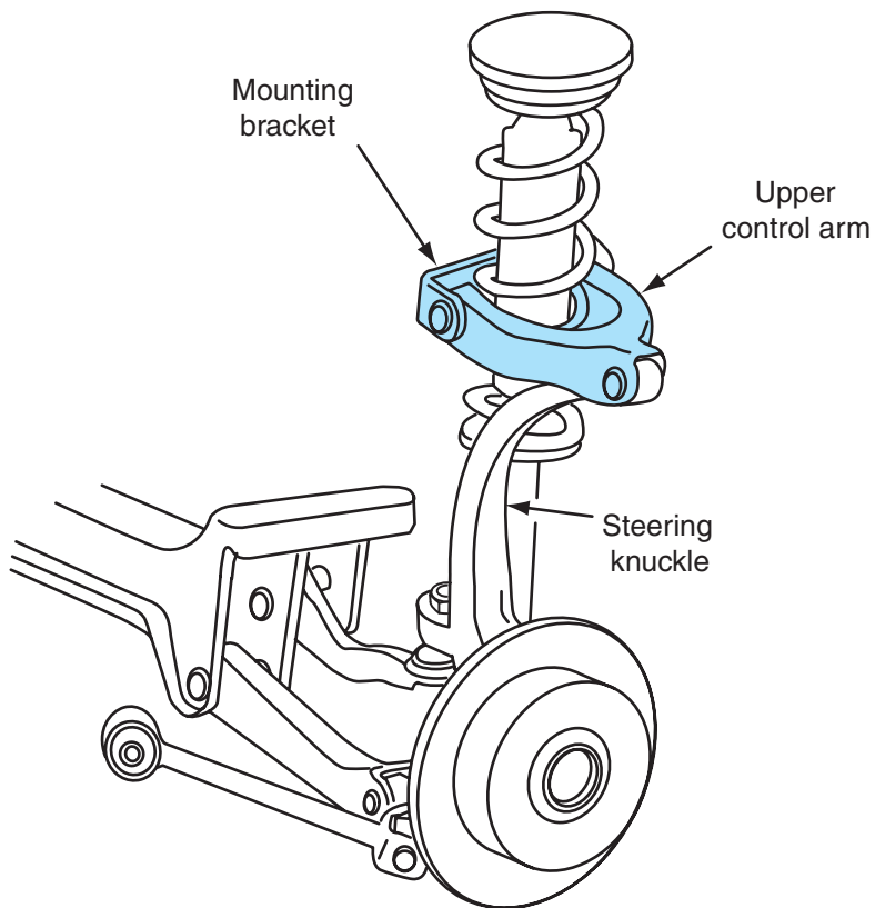
Figure 7-41 Upper control arm and strut in multilink rear suspension.
