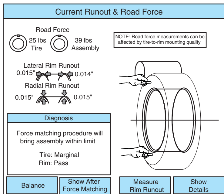
Figure 4-33 The balancer display indicates the necessary correction for excessive force variation.
