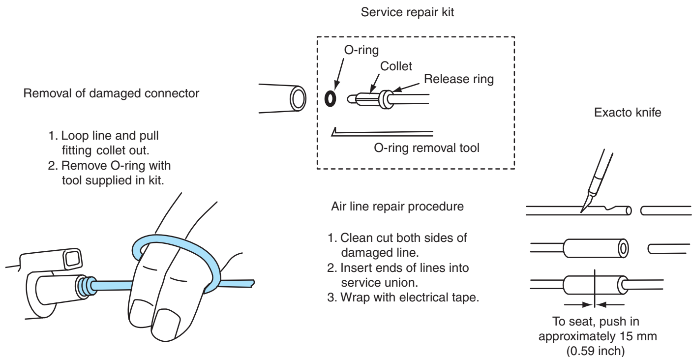
Figure 8-14 Removing the quick disconnect fittings and air line repairs procedure.
