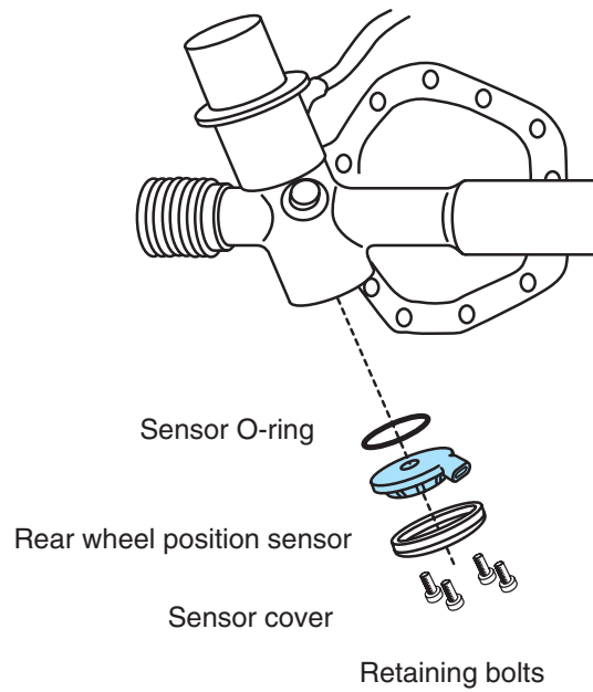
Figure 13-12 Rear wheel position sensor.
