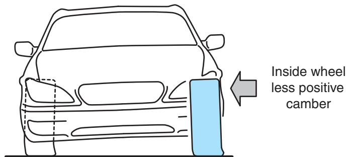
Figure 15-32 While cornering at high speed, the camber on the inside front wheel becomes less positive and the inside edge of the tire grips the road surface to resist lateral skidding.
