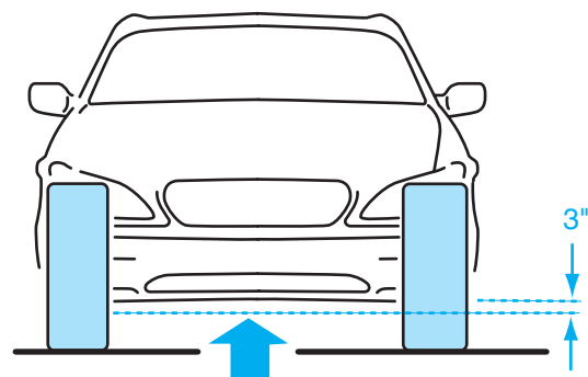
Figure 15-43 Pull the chassis upward 3 in. (7.6 cm) to check for improper toe change indicating unequal steering linkage height.
