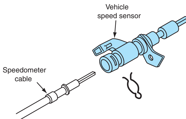
Figure 12-13 Vehicle speed sensor (VSS).
