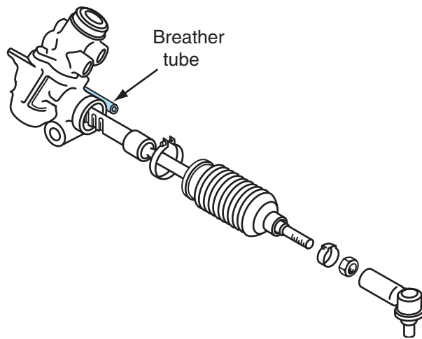
Figure 12-7 Breather tube and boot.
