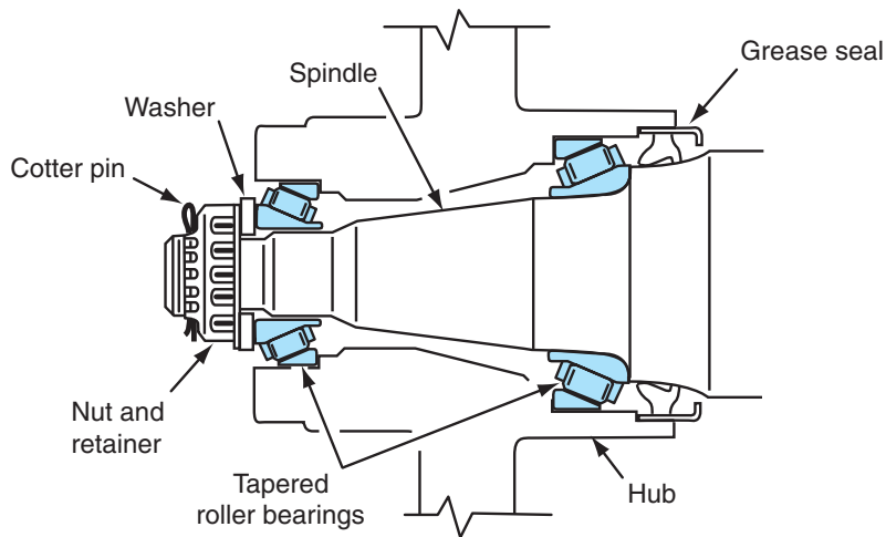
Figure 3-20 Front wheel bearing assembly, rear-wheel-drive car.
