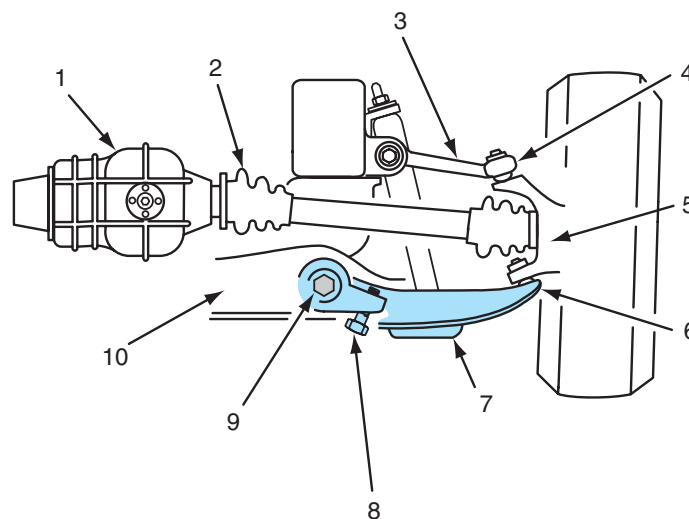
Figure 6-54 Four-wheel-drive light-duty truck torsion bar front suspension.
