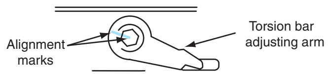
Figure 6-53 Alignment marks placed on the torsion bar and adjuster.
