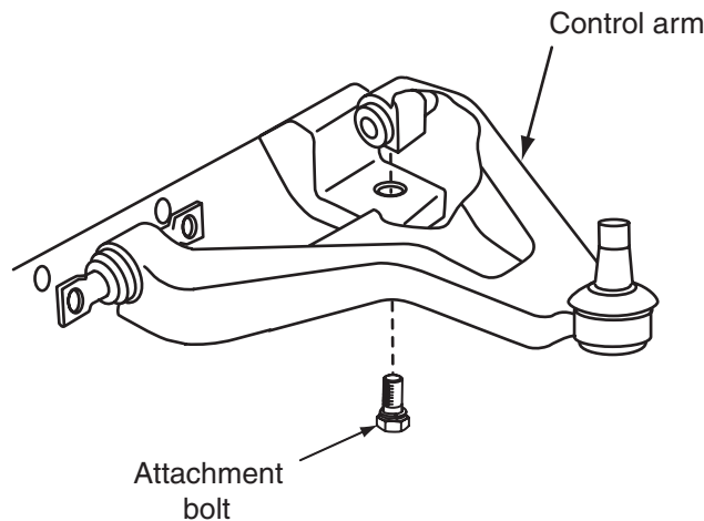
Figure 6-36 Removing the bolt and nut from the rear side of the lower control arm.
