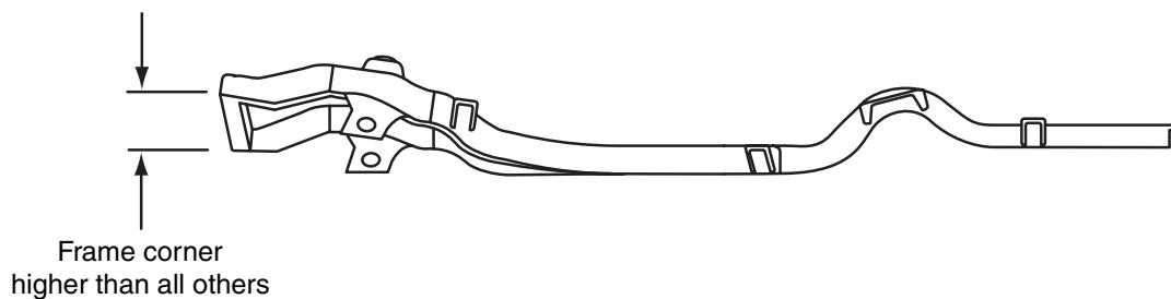
Figure 14-15 Frame twist.
