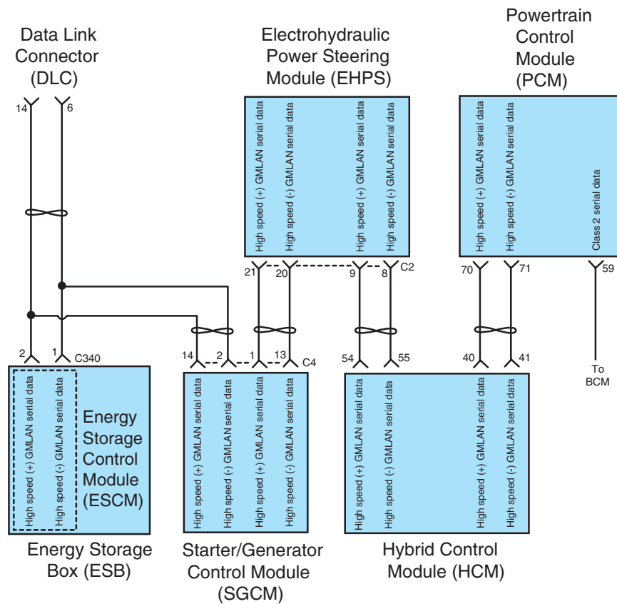
Figure 10-29 The LAN bus interconnects the SGCM, PCM, EHPS module, ESB, and DLC.
