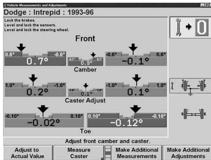
Figure 15-24 Alignment angle adjustment screens. (Courtesy of Hunter Engineering Company.)
