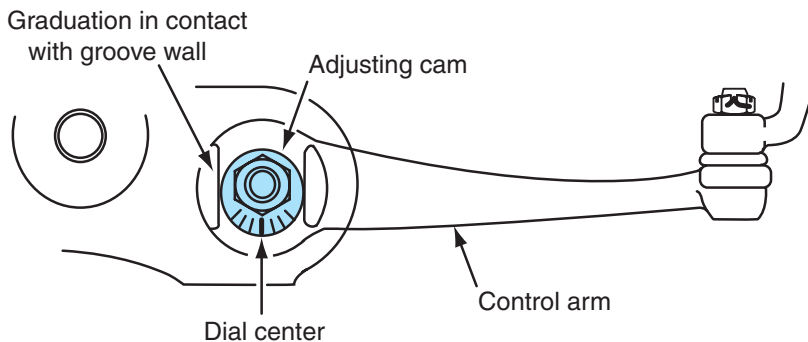
Figure 16-11 Camber adjustment double-wishbone front suspension.
