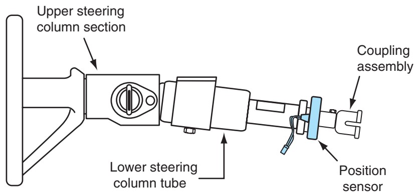
Figure 10-20 Steering wheel position sensor.
