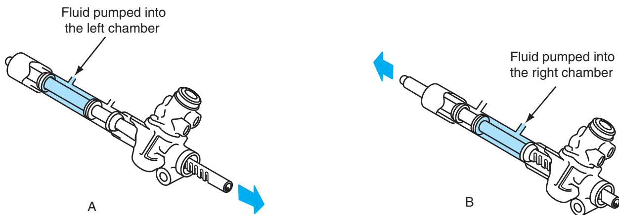
Figure 12-3 Rack movement during left and right turns.
