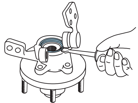
Figure 6-18 Removing dust deflector from the steering knuckle.
