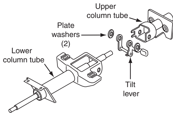
Figure 9-33 Installing upper column tube, tilt lever mechanism, and two plate washers.
