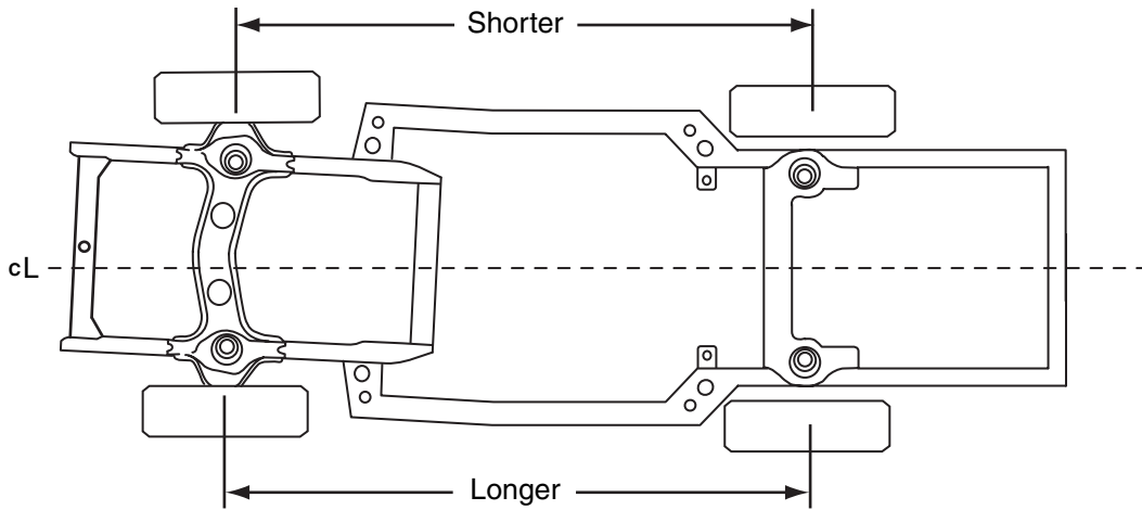
Figure 14-10 Side sway frame condition caused by collision damage.
