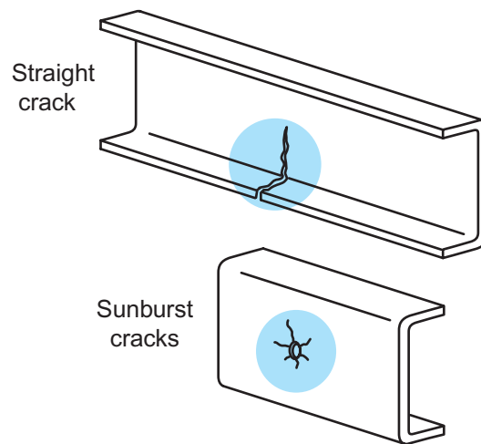
Figure 14-5 Straight cracks may occur in the frame flange; sunburst cracks may radiate from a hole in the frame web or cross member.
