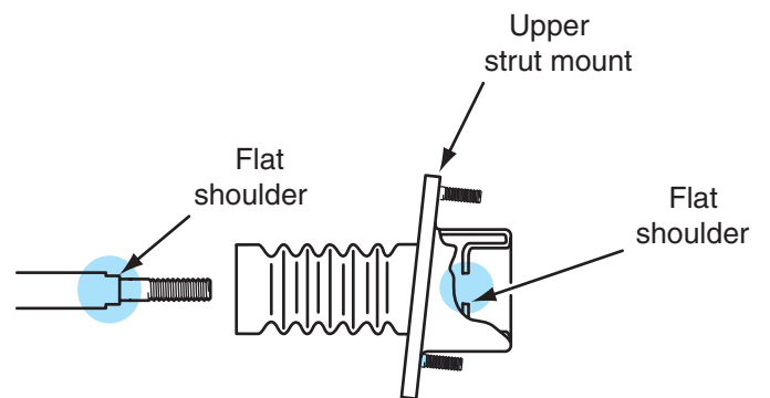
Figure 5-19 Upper strut mount properly positioned on strut piston rod.
