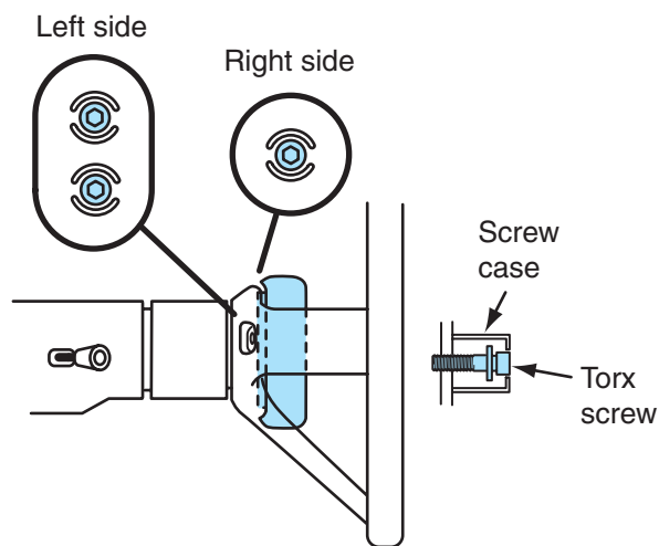
Figure 9-1 Three air-bag-retaining Torx screws.
