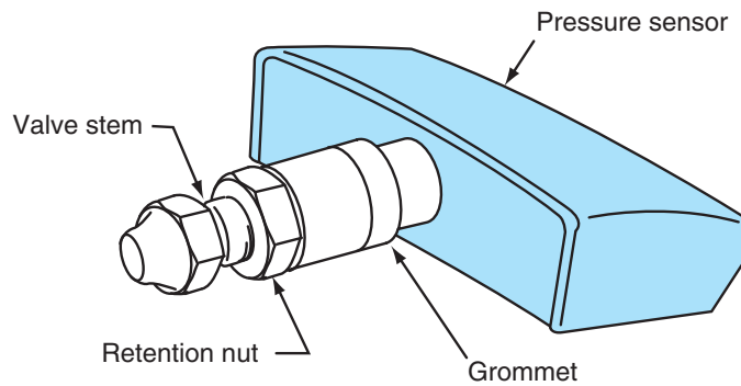
Figure 4-24 Tire pressure sensor mounted on the valve stem.
