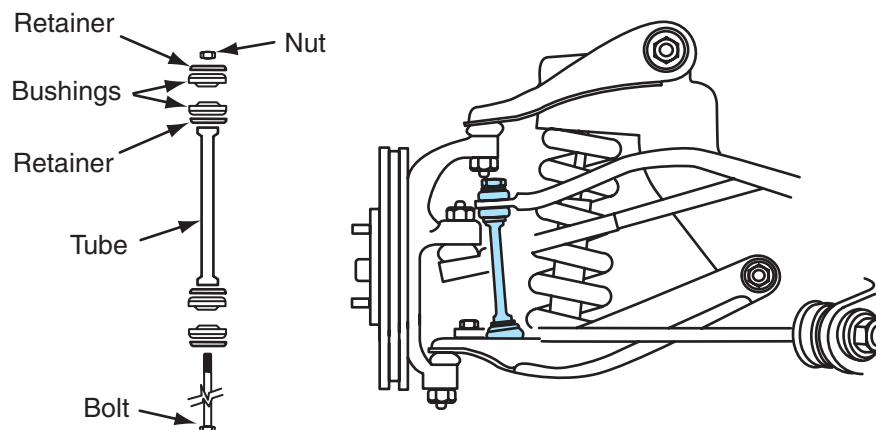
Figure 6-46 Stabilizer bar components.
