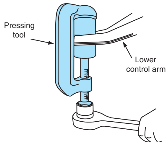
Figure 6-26 Installing the pressed-in ball joint in the lower control arm.
