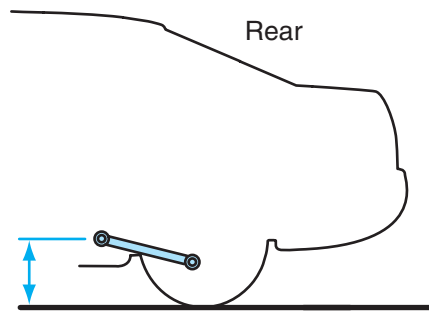
Figure 7-7 Curb riding height measurement, rear suspension.
