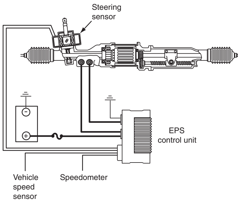
Figure 12-22 Steering gear with electronic assist and related system components.
