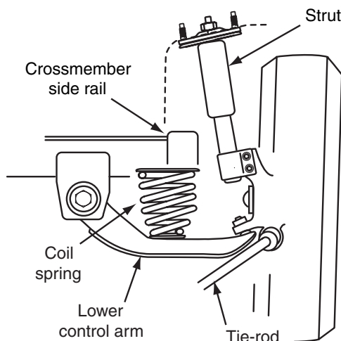
Figure 7-21 Modified MacPherson strut independent rear suspension.
