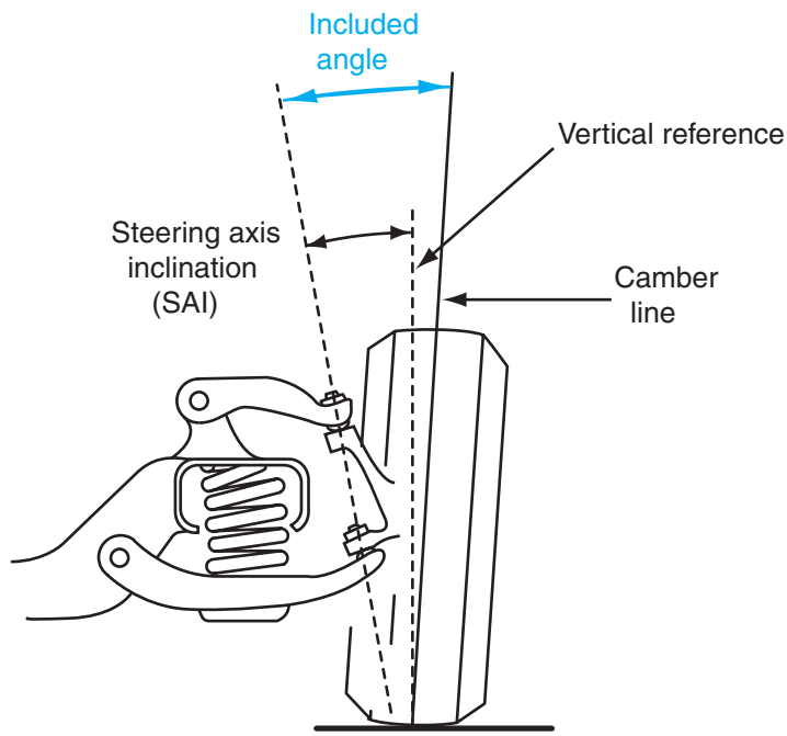
Figure 1-37 Steering axis inclination and included angle.
