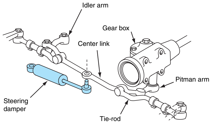
Figure 9-32 Steering gear damper and linkage.
