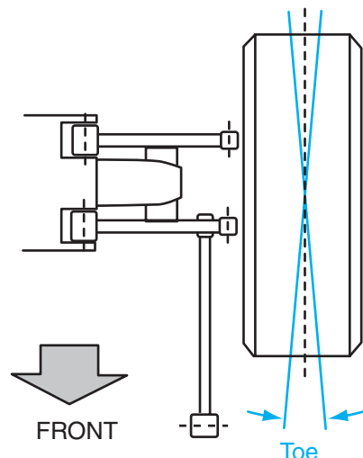
Figure 16-56 Moving lower rear control rod position to adjust rear wheel toe.
