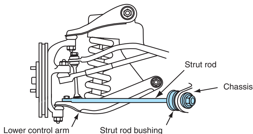
Figure 6-47 Strut rod.
