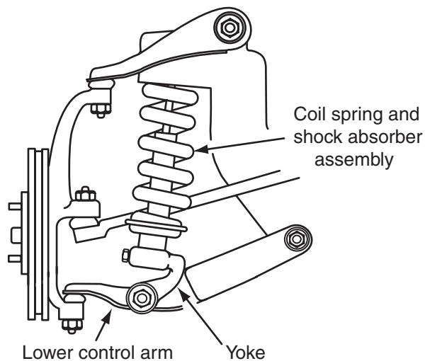
Figure 6-26 Short-and-long arm front suspension with yoke-type shock absorber mounting.
