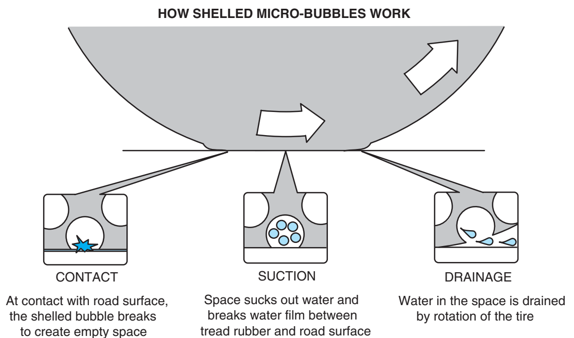
Figure 4-7 Advantages of micro-bubbles in the tire tread.
