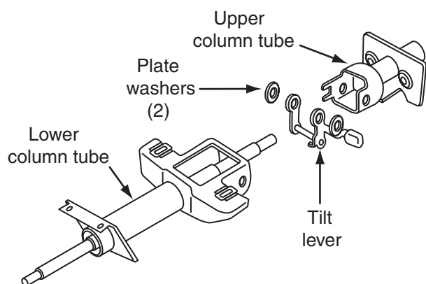
Figure 9-23 Removing upper column tube, tilt lever assembly, and plate washers.
