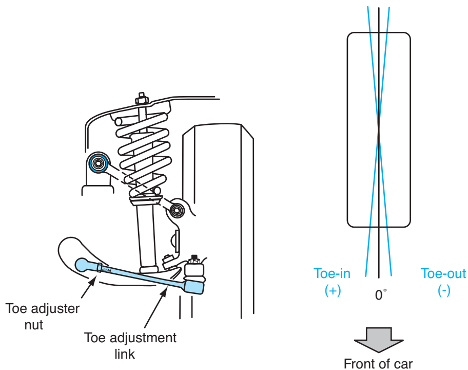
Figure 16-15 Rear wheel toe.
