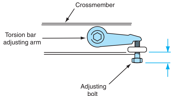
Figure 6-50 Measuring the torsion bar adjusting bolt position.
