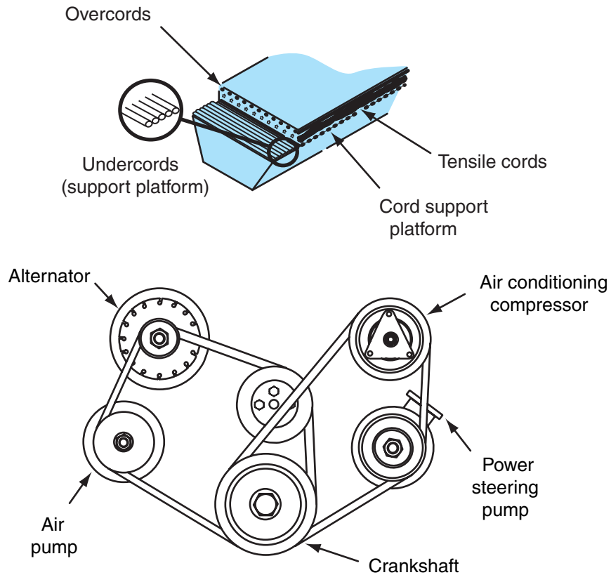
Figure 10-1 Conventional V-belt.
