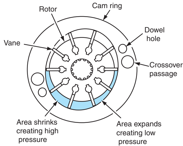
Figure 10-9 Power steering pump rotor and vanes.
