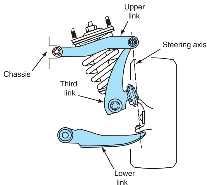
Figure 6-38 Multilink front suspension system.
