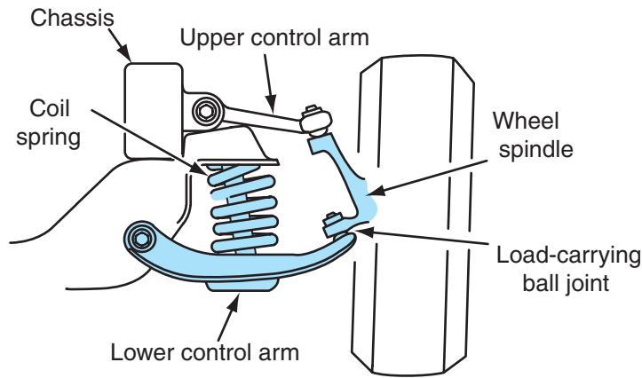
Figure 6-7 Load-carrying ball joint mounted on the control arm on which the spring is seated.
