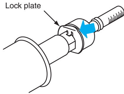
Figure 12-14 Straightening lock plate where it is bent over the inner tie-rod end.
