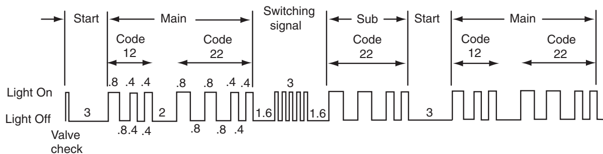
Figure 13-6 Trouble codes in main and sub processors obtained with engine running.
