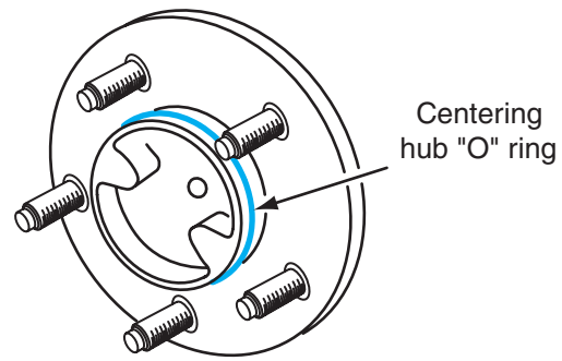
Figure 4-32 Hub O-ring that provides wheel centering.
