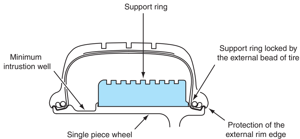
Figure 4-18 Run-flat tire with support ring.
