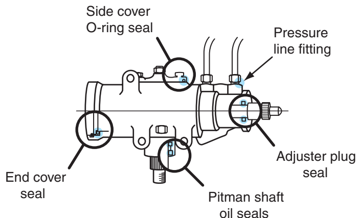
Figure 11-9 Power recirculating ball steering gear oil leak locations.
