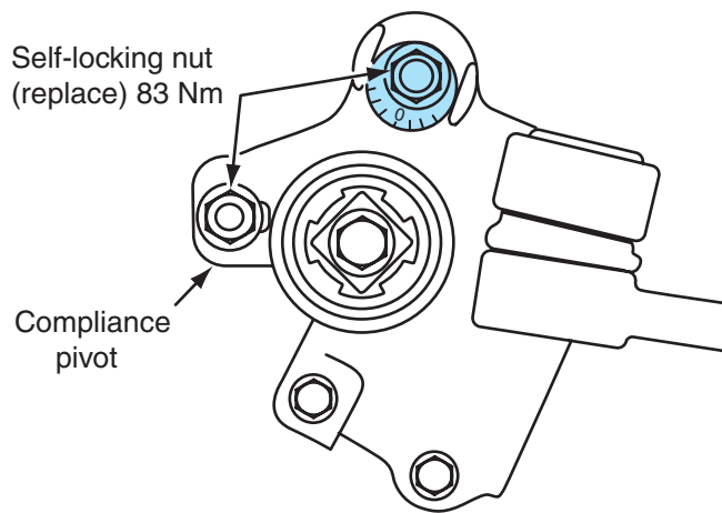
Figure 16-30 Graduated cam for caster adjustment, double-wishbone front suspension.
