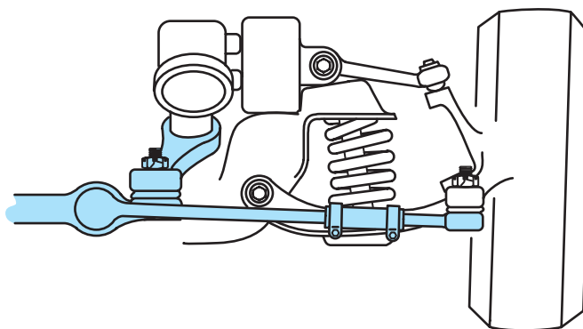
Figure 9-18 Parallelogram steering linkage in front of the front suspension.
