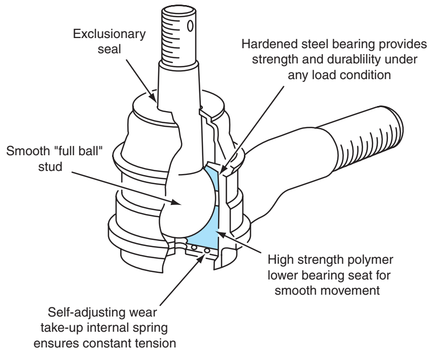
Figure 9-20 Outer tie-rod end with hardened steel upper bearing and high-strength polymer lower bearing.
