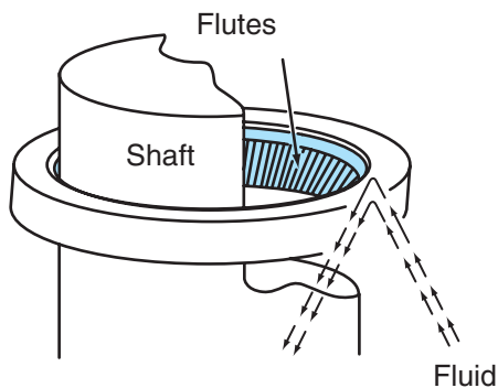
Figure 3-12 Fluted lip seal redirect oil back into the housing.
