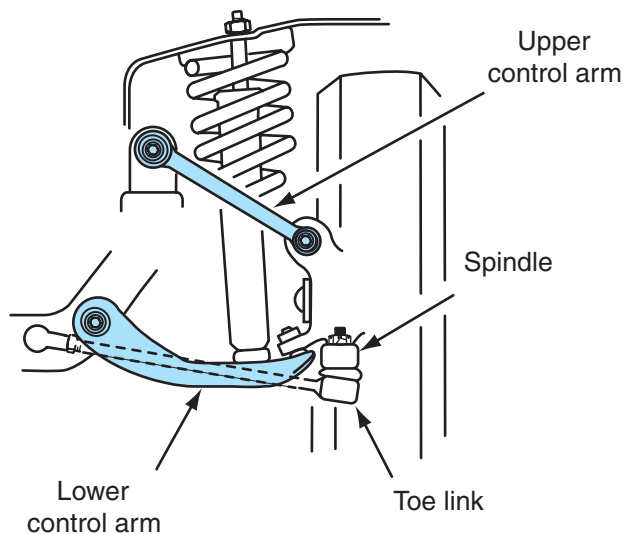
Figure 7-28 Short-and-long arm independent rear suspension system.
