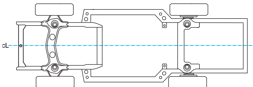
Figure 16-62 When all four wheels are parallel to the geometric centerline, the thrust line is positioned at the geometric centerline and the rear wheels track directly behind the front wheels.
