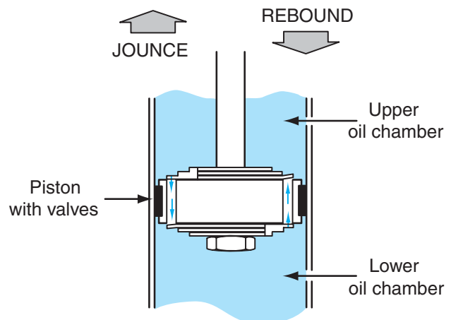
Figure 1-15 Shock absorber action.
