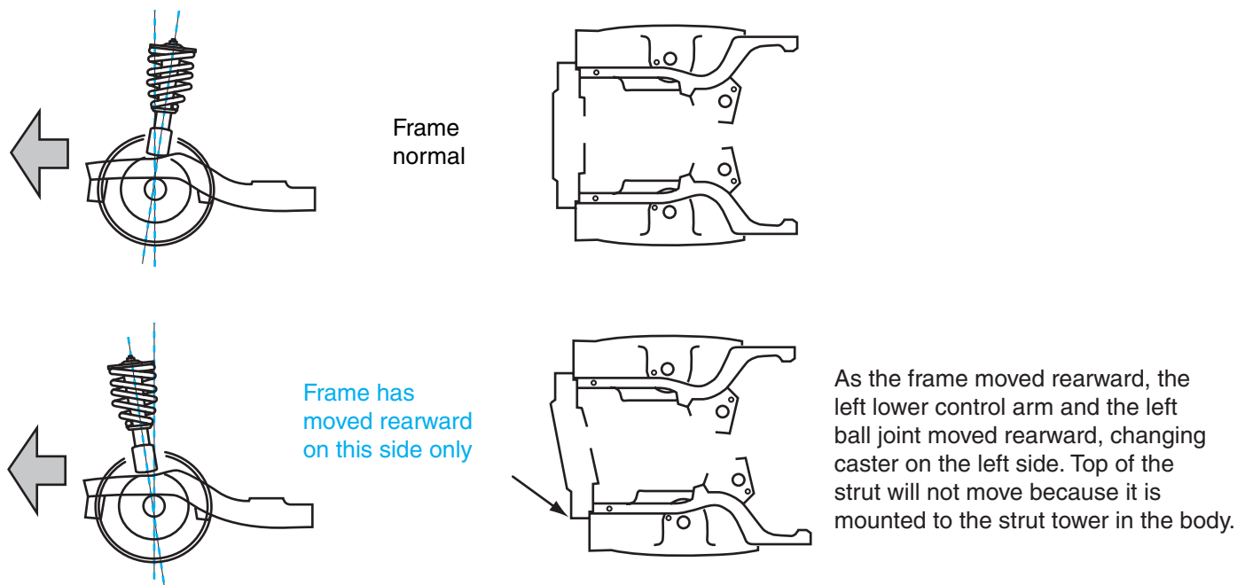
Figure 16-34 Collision damage on the left front moves the cradle and strut rearward to a setback condition and shifts the caster to a negative position.
