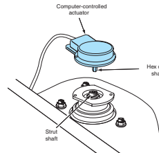
Figure 1-17 Strut actuator.
