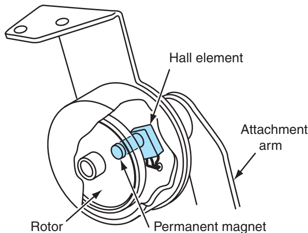
Figure 8-22 Electronic rotary height sensor.
