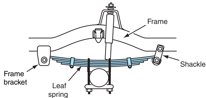
Figure 6-52 Leaf spring mounting, four-wheel-drive twin I-beam front suspension.
