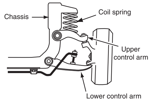
Figure 6-21 Short-and-long arm front suspension with the coil spring between the upper control arm and the chassis.
