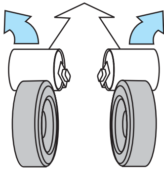
Figure 4-29 Tire conicity sensed by the roller on the balancer causes lateral force and steering pull.
