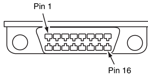
Figure 12-40 Data link connector (DLC) on-board diagnostic II (OBD-II) system.
