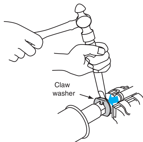
Figure 12-36 Staking claw washer on inner tie-rod end.
