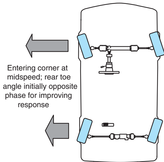
Figure 13-19 Rear wheel steering during negative phase operation.
