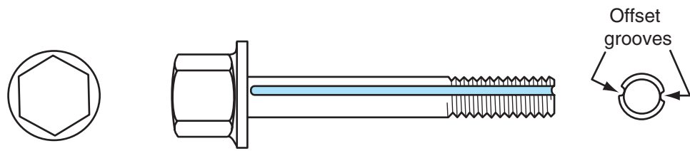
Figure 16-23 Camber/caster adjustment bolt with offset grooves.
