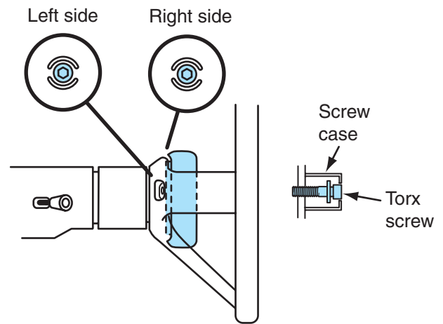
Figure 9-2 Two air-bag-retaining Torx screws.
