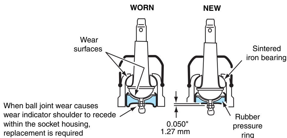
Figure 7-21 Ball joint wear indicator.
