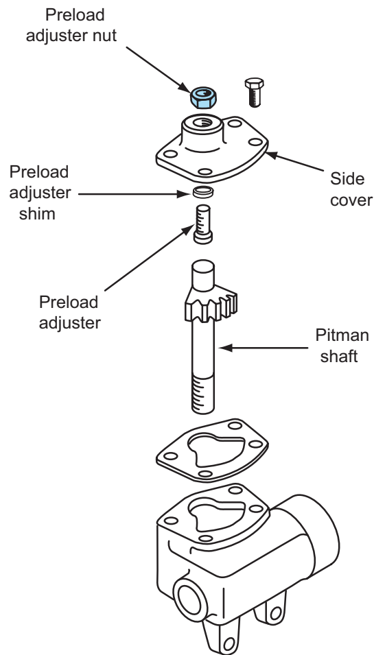
Figure 11-2 Sector shaft adjusting nut.
