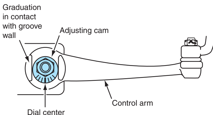
Figure 16-51 Graduated cam for rear camber adjustment, double wishbone suspension.
