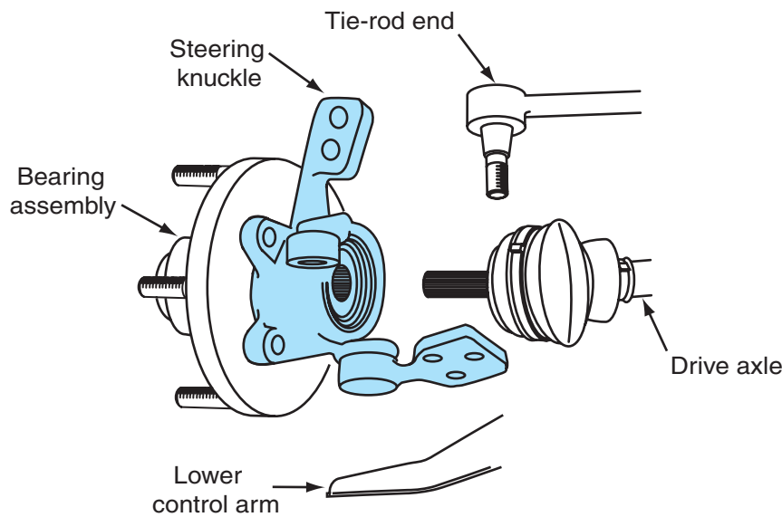
Figure 6-17 Removing the steering knuckle from the lower control arm.
