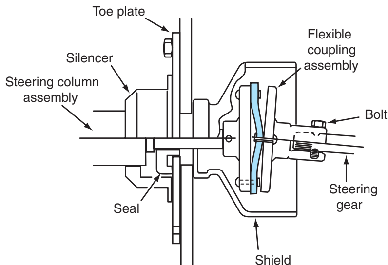
Figure 9-3 Flexible coupling.
