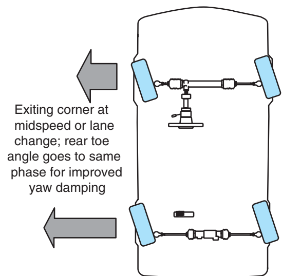
Figure 13-20 Rear wheel steering during positive phase operation.
