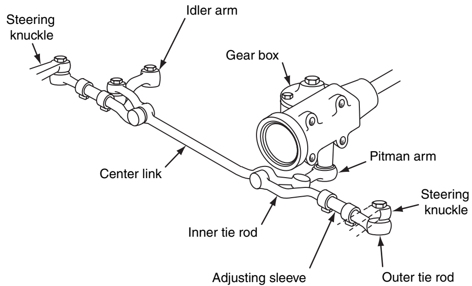
Figure 1-21 Parallelogram steering linkage.
