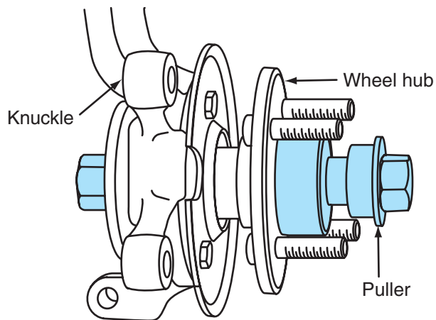
Figure 3-23 Wheel hub installation in wheel bearing.
