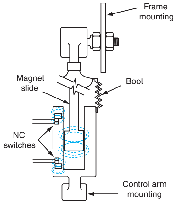
Figure 8-21 Rear height sensor mounting.
