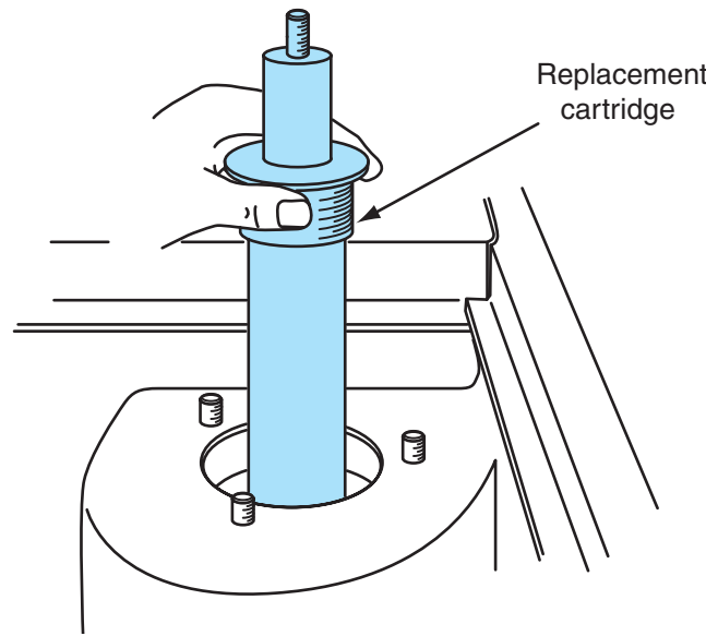
Figure 5-35 Installing new strut cartridge.
