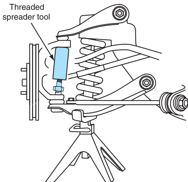
Figure 6-21 Removing the lower ball joint from the steering knuckle.
