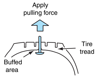
Figure 4-13 Plug installation procedure.
