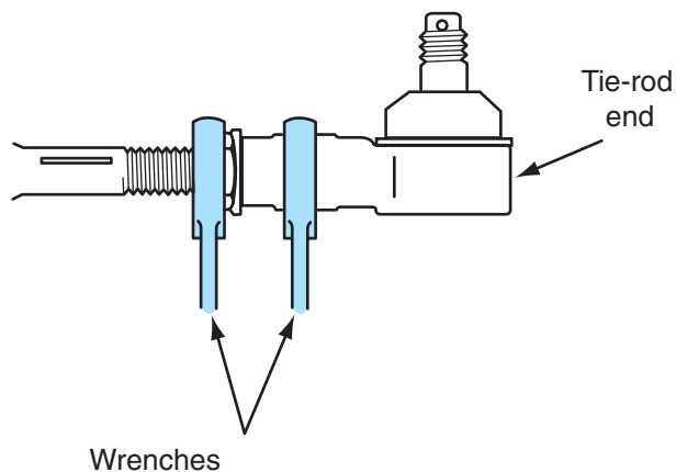
Figure 13-13 Loosening the tie-rod end locknut.
