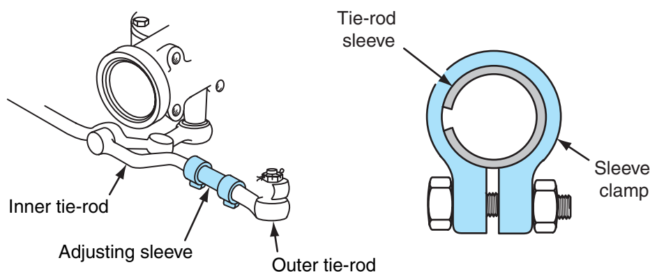
Figure 9-47 Proper slot and clamp position on tie-rod sleeves.
