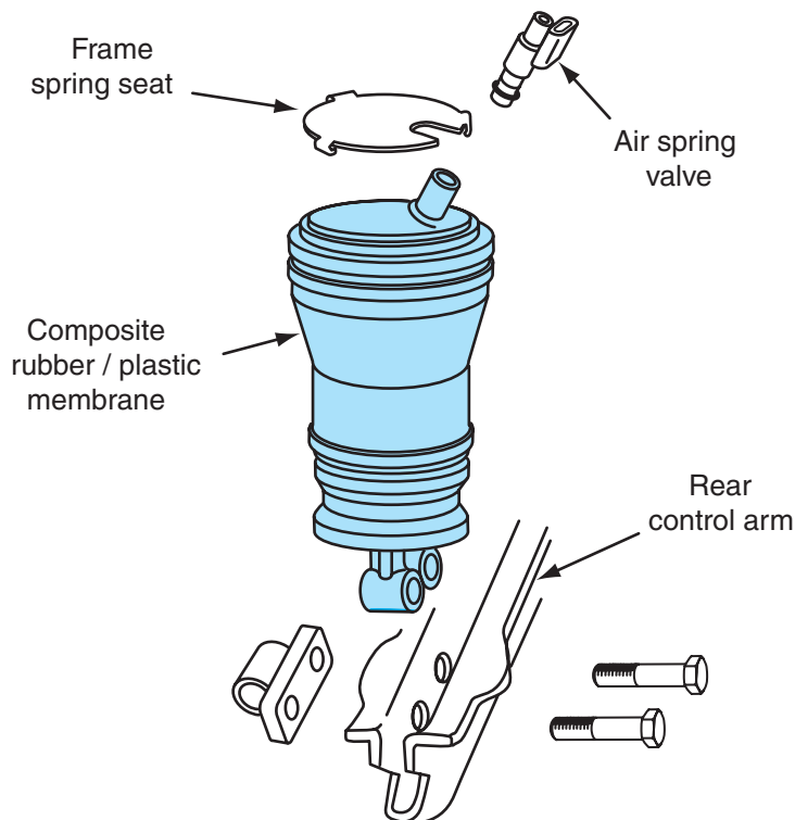
Figure 8-12 Rear air spring mounting.
