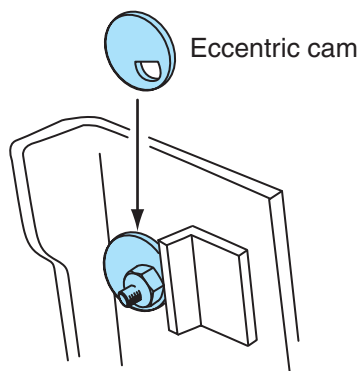
Figure 16-13 Eccentric cam installed behind upper control arm attaching nut.
