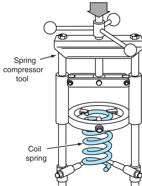
Figure 7-20 Compressing the coil spring in the compressing tool prior to strut and spring assembly.
