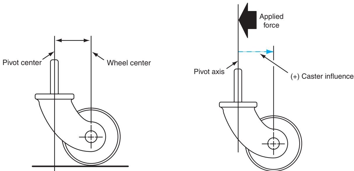
Figure 2-6 Distance between the wheel center and the pivot center on a caster.
