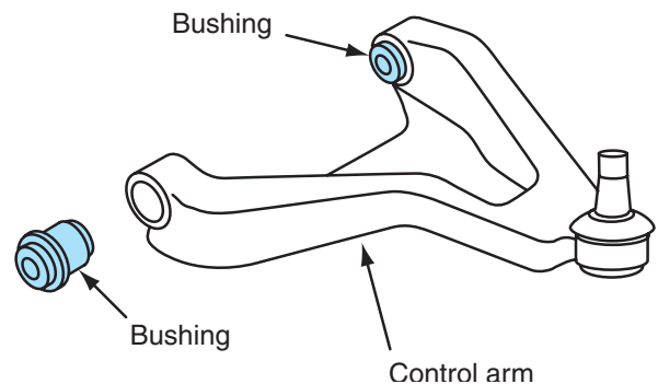
Figure 7-23 Lower control arm bushings.
