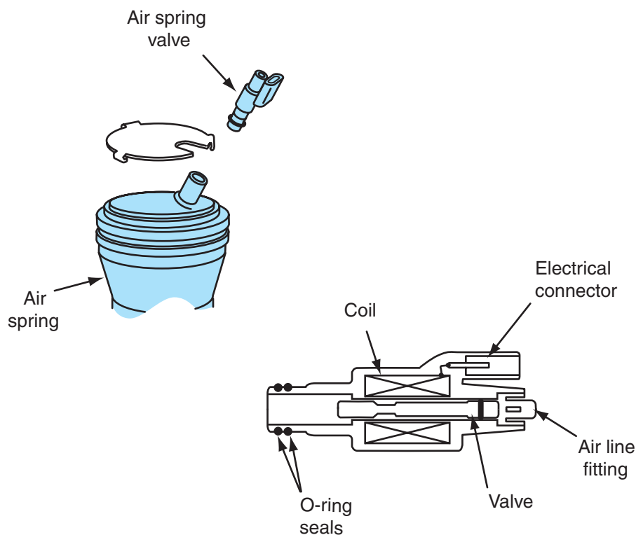
Figure 8-14 Air spring valve.
