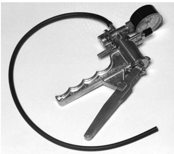
Figure 2-18 Vacuum hand pump.
