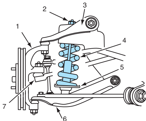
Figure 6-22 Short-and-long arm front suspension system with coil spring mounted on the shock absorber.
