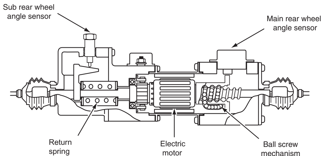
Figure 13-3 Rear steering actuator, electronically controlled 4WS system.
