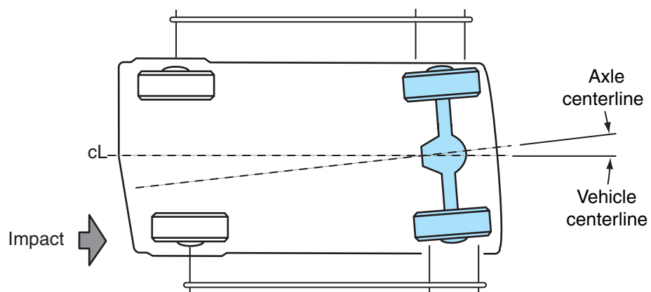
Figure 16-67 A severe left front collision impact moves the entire left side of the vehicle rearward resulting in front wheel setback and rear axle offset, which provides a diamond-shaped chassis.
