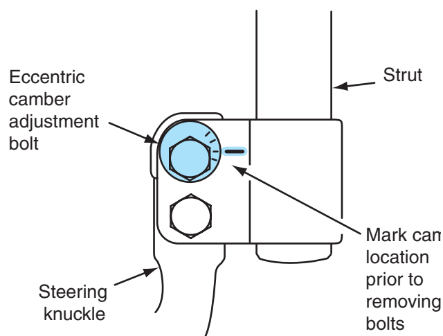
Figure 5-6 Camber bolt marking for strut removal.
