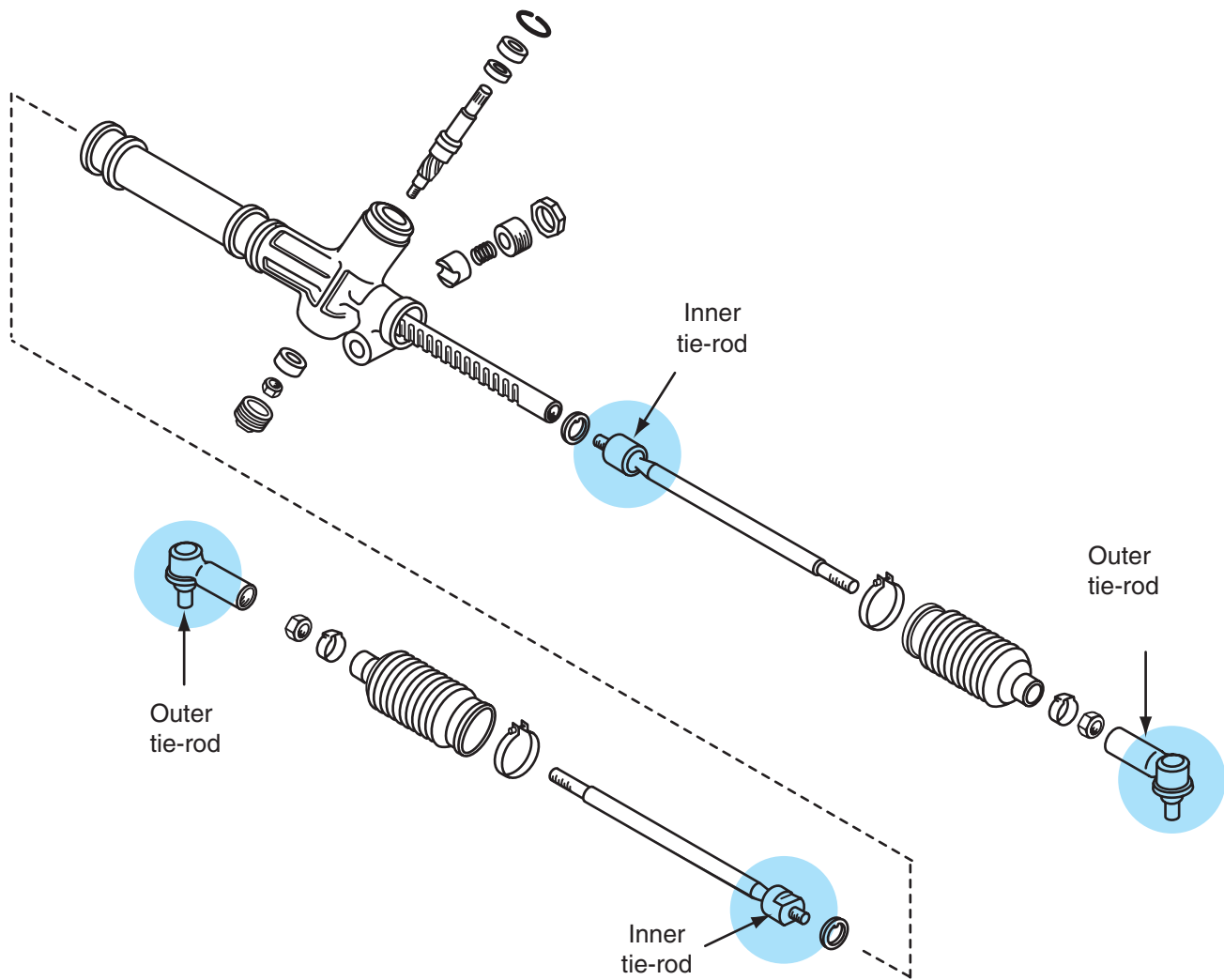
Figure 12-1 Wear points at the inner and outer tie-rod ends in a rack and pinion steering gear.
