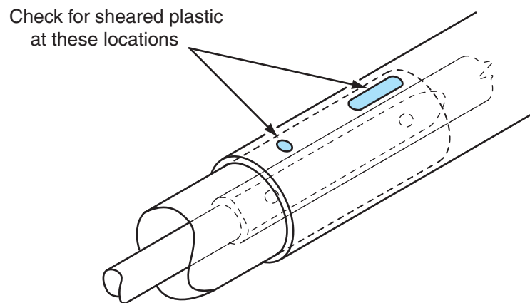
Figure 9-4 Injection plastic in collapsible outer steering column jacket.
