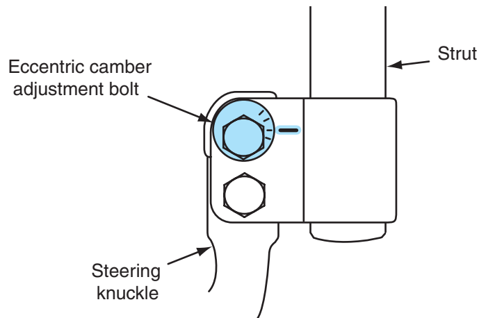
Figure 3-16 Marking eccentric strut bolt before removal.
