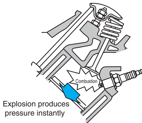
Figure 2-2 Thermal energy in the fuel is converted to mechanical energy in the engine cylinders. The piston, crankshaft, and drive train deliver this mechanical energy to the drive wheels.
