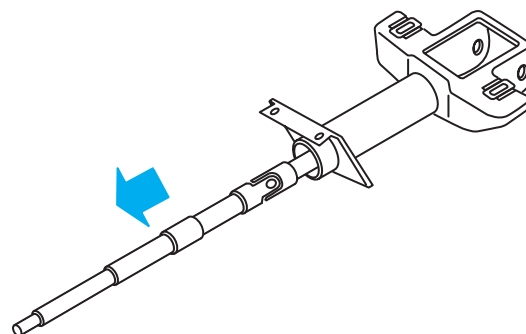
Figure 9-24 Removing steering shaft from the steering column.
