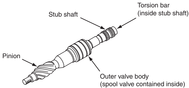
Figure 12-4 Pinion assembly for a power rack and pinion steering gear.
