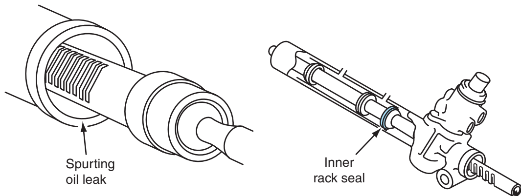
Figure 12-16 Oil leak diagnosis at outer rack seal.
