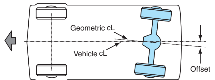
Figure 15-32 Axle offset.
