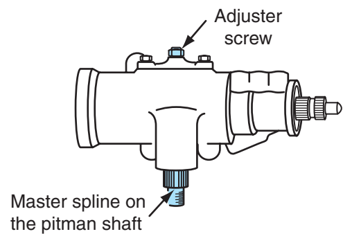
Figure 11-7 Pitman shaft master spline aligned with the pitman backlash adjuster screw.
