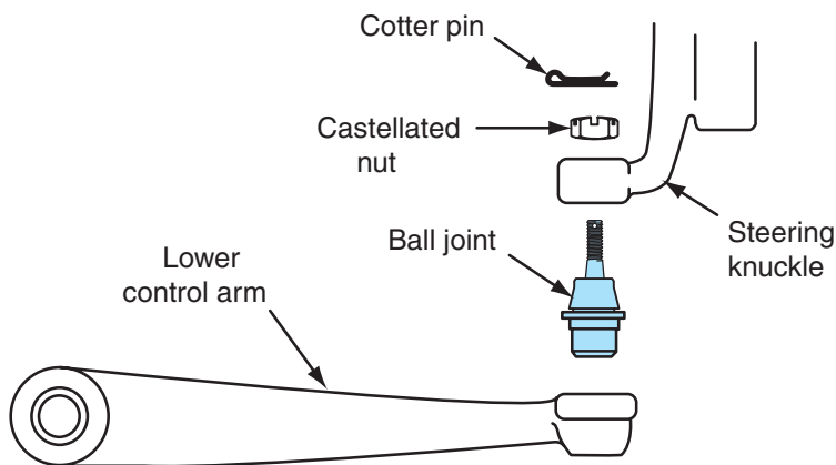
Figure 7-22 Lower control arm and ball joint.
