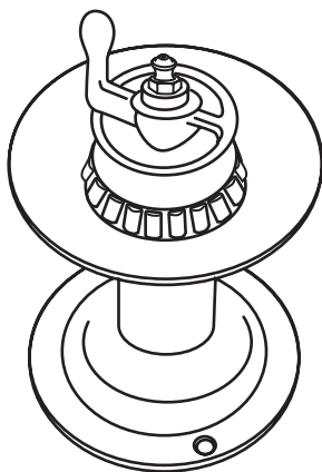
Figure 3-7 Mechanical wheel bearing packer.
