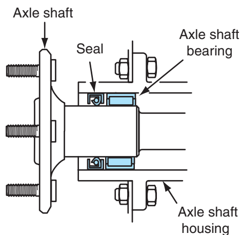
Figure 3-28 Rear axle roller bearing and seal, rear-wheel-drive car.
