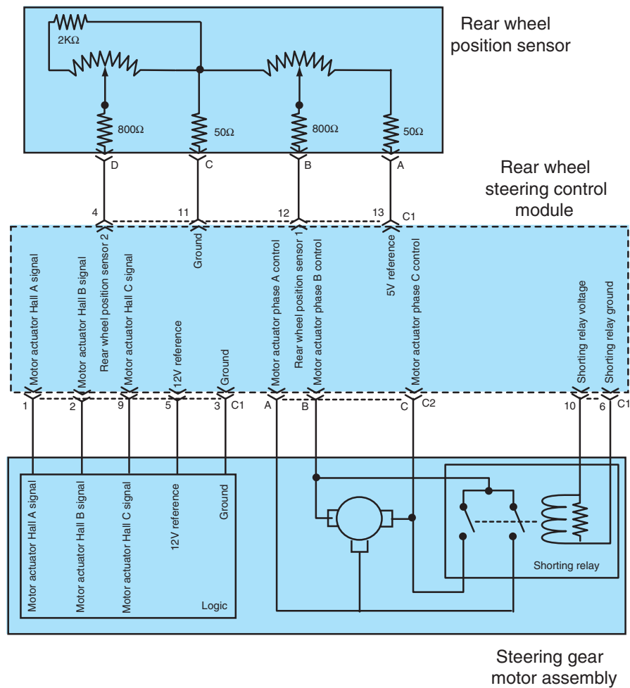
Figure 13-13 Rear wheel position sensor inputs to the rear wheel steering control module.
