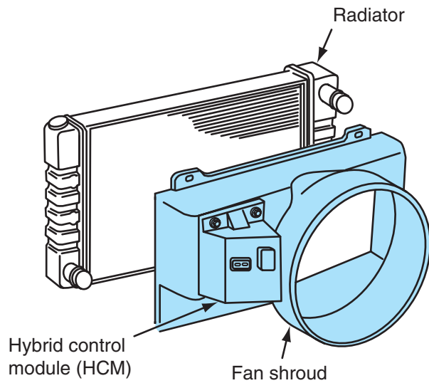
Figure 10-28 Hybrid control module (HCM).
