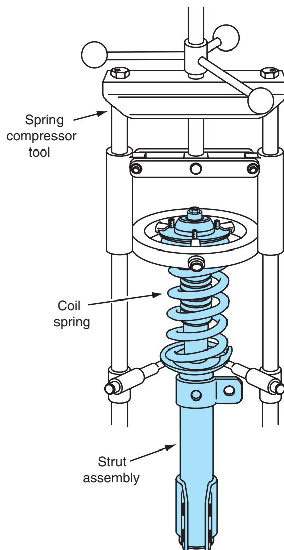
Figure 2-44 Coil spring and strut assembly mounted in a spring compressing tool.
