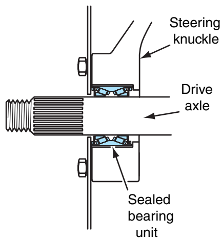
Figure 3-17 Steering knuckle with pressed-in bearing.
