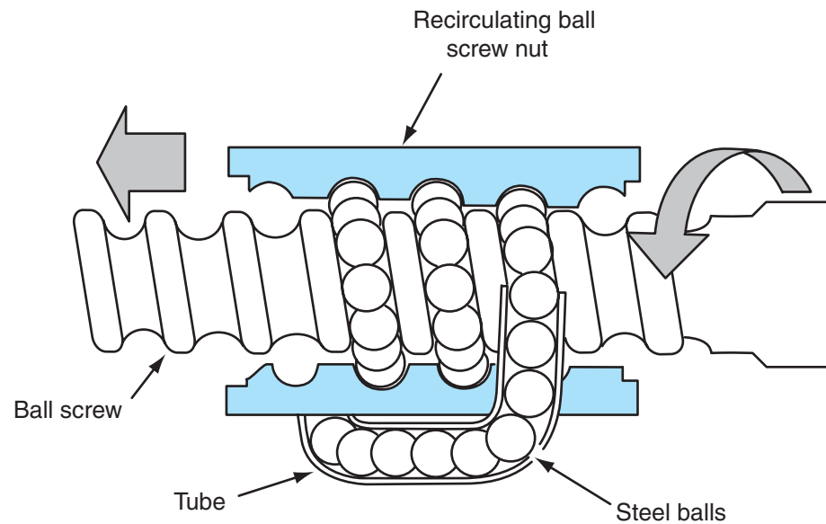
Figure 12-30 Ball screw shaft and recirculating ball screw nut.
