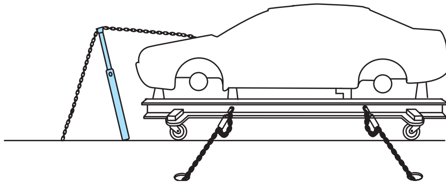
Figure 14-21 Single-pull unitized body straightening system.
