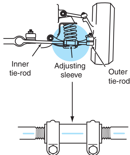
Figure 16-43 Marking tie-rod sleeves in relation to the tie-rods and outer tie-rod ends.
