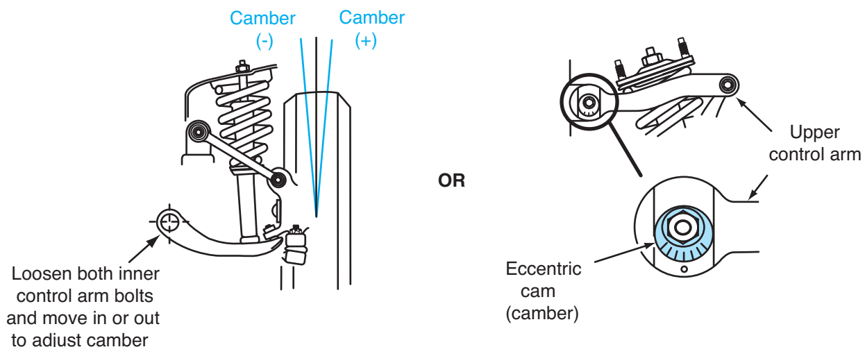
Figure 16-14 Rear wheel camber.
