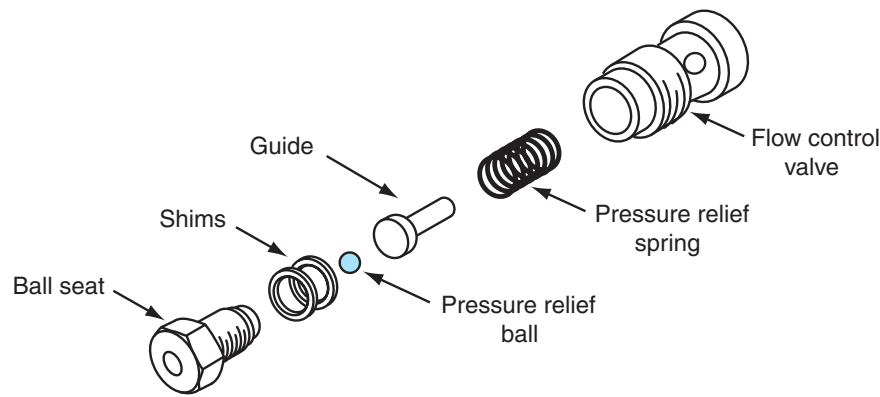
Figure 10-26 Pressure relief valve removal.
