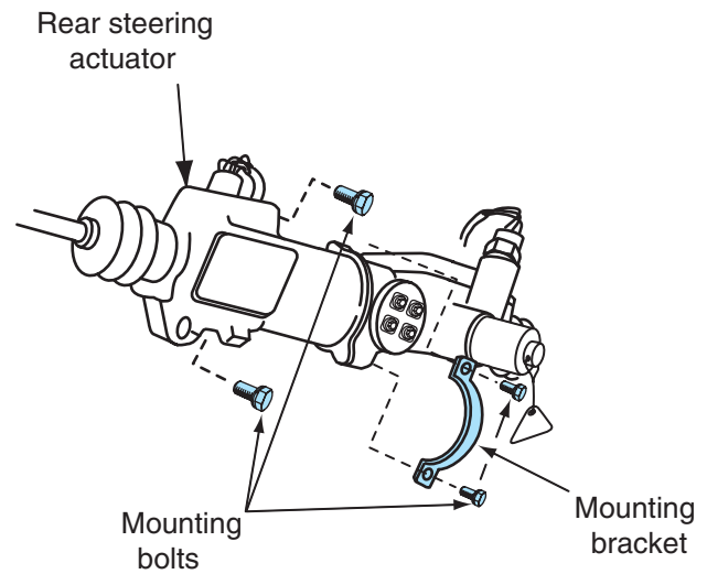
Figure 13-12 Removing the four mounting bolts, bracket, and rear steering actuator.
