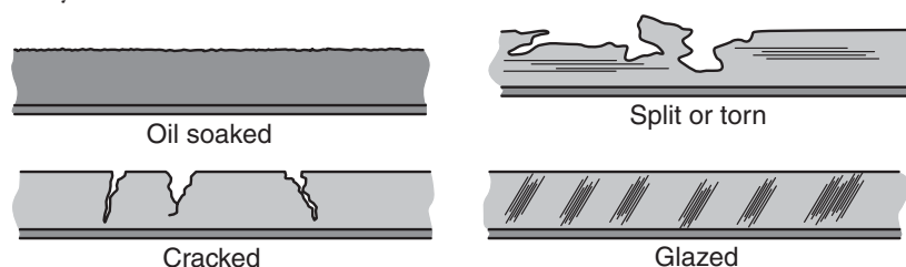
Figure 10-1 Defective belt conditions.
