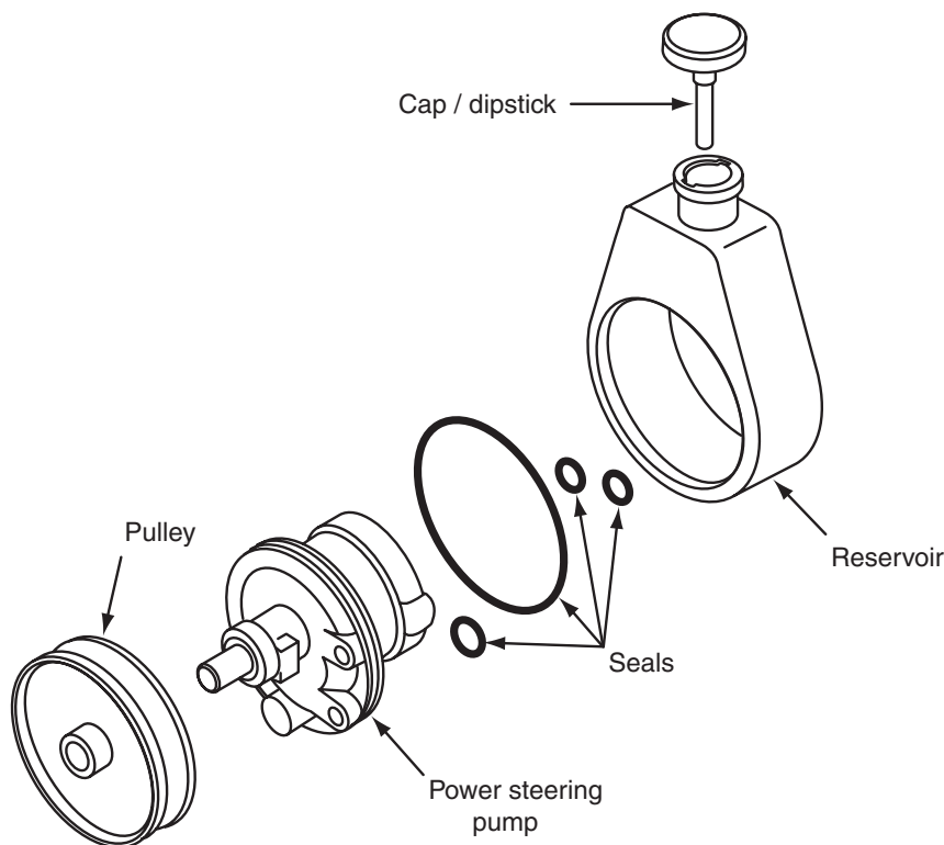
Figure 10-10 Power steering pump housing and reservoir.
