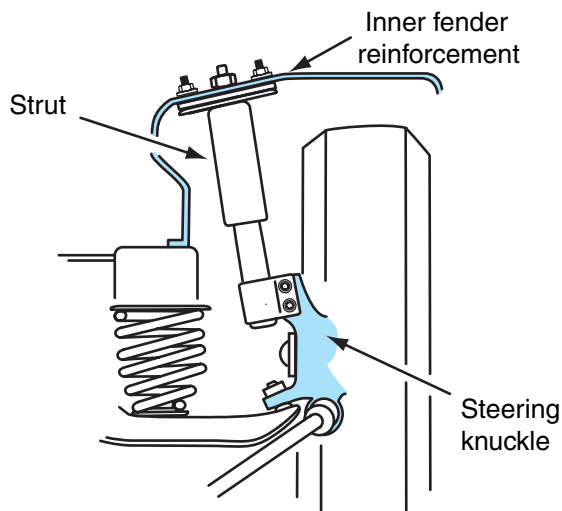
Figure 7-24 Upper and lower strut mounting.
