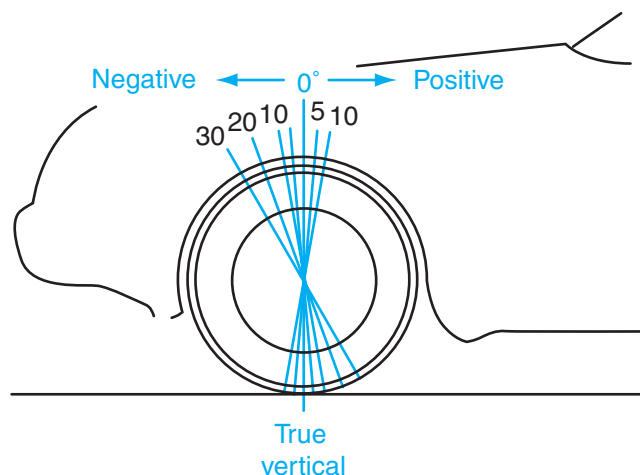
Figure 15-39 Positive and negative caster.
