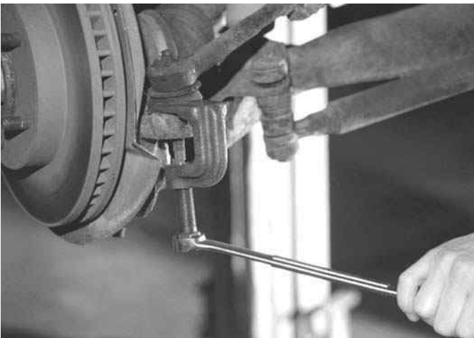
Figure 6-30 Removing the outer tie-rod end.
