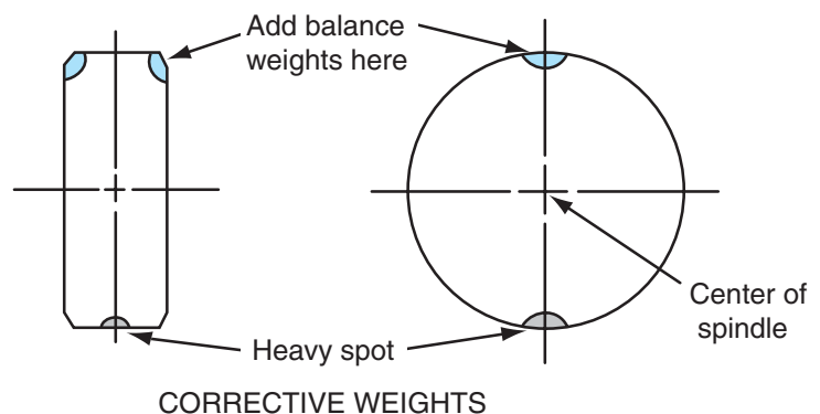
Figure 4-26 Static wheel balance procedure.
