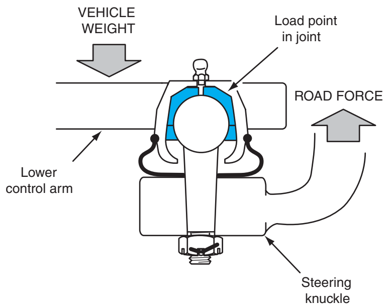
Figure 6-9 Compression-loaded ball joint mounting.
