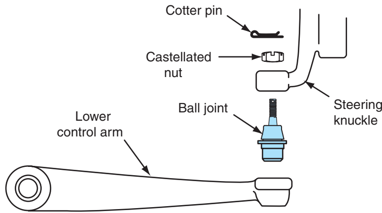
Figure 6-34 Lower ball joint.
