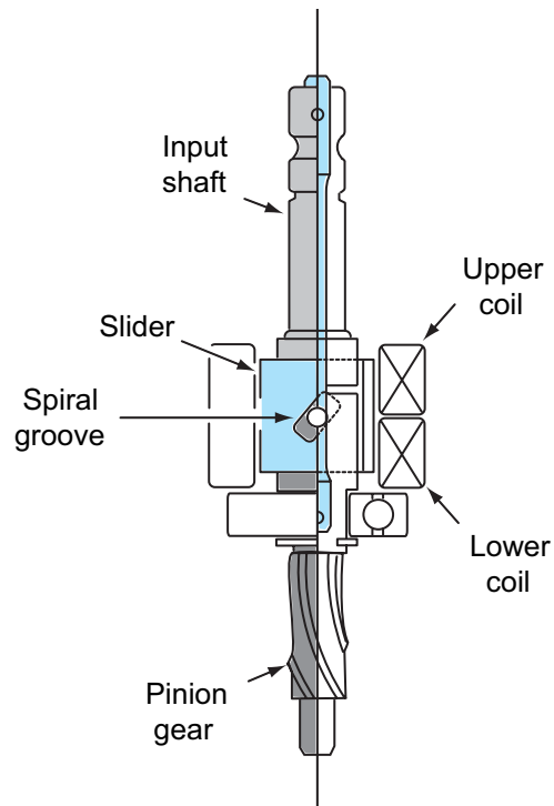
Figure 12-25 Pinion shaft with slider and variable differential transformer.
