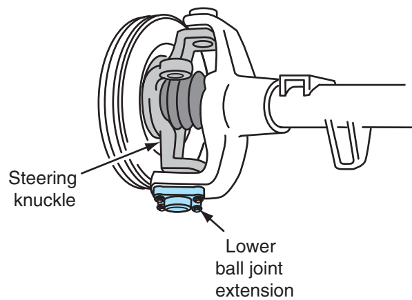
Figure 13-14 Lower ball joint, rear wheel steering.
