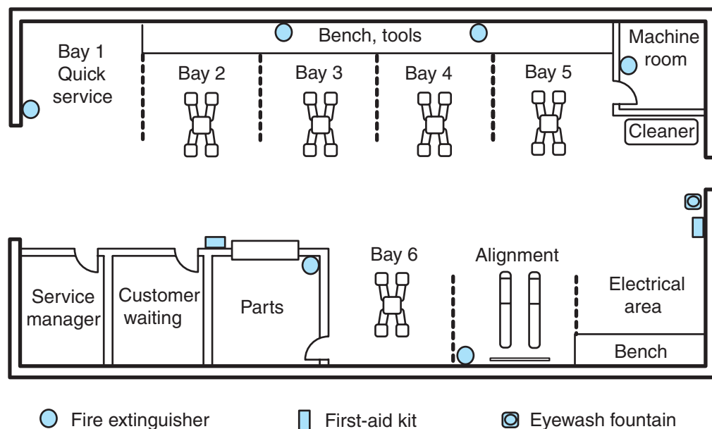
Figure 1-8 Shop layout.
