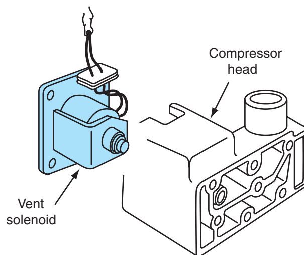
Figure 8-16 Air vent valve.
