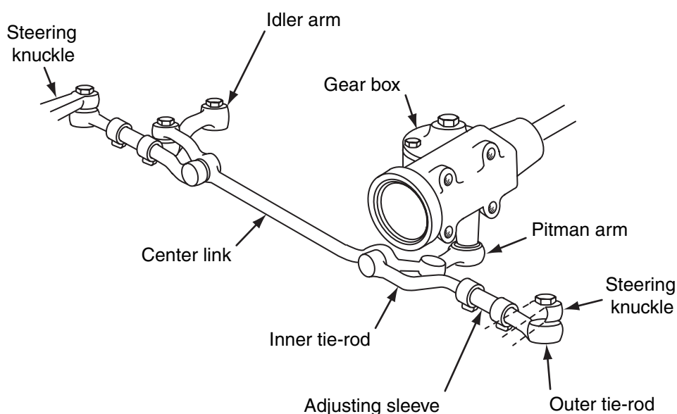
Figure 9-17 Parallelogram steering linkage behind the front suspension.
