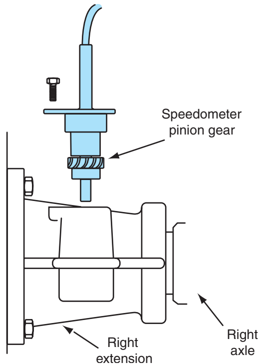
Figure 3-17 Speedometer drive gear removal before right axle removal.
