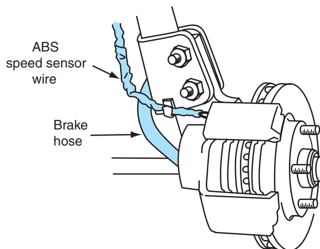
Figure 5-7 Brake line and ABS wheel-speed sensor wire removed from the strut.
