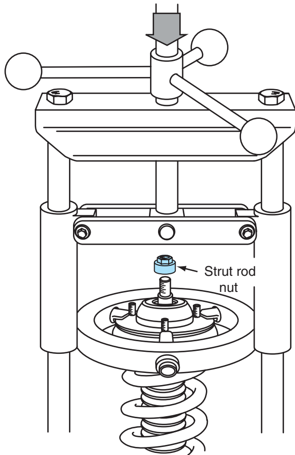
Figure 2-45 After the compressing tool is operated to remove all the spring tension, remove the strut rod nut.
