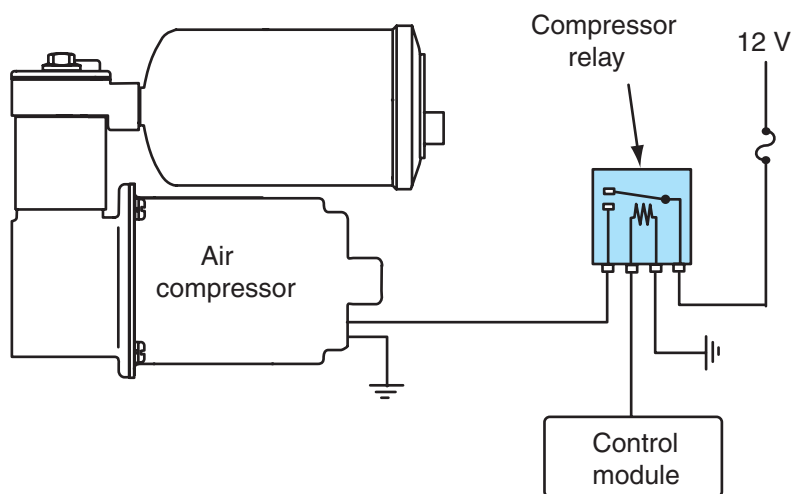
Figure 8-17 Compressor relay.
