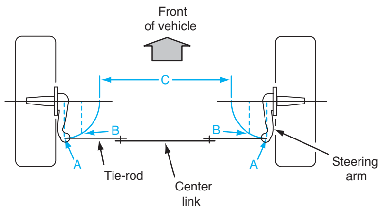
Figure 16-11 Steering arms are closer together at the point where the tie-rods connect than at their spindle pivot points.
