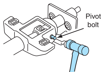
Figure 9-22 Removing pivot bolts from steering column.
