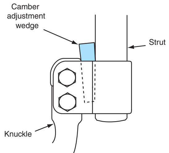
Figure 16-49 Camber adjusting wedge installed between the top of the rear knuckle and strut.
