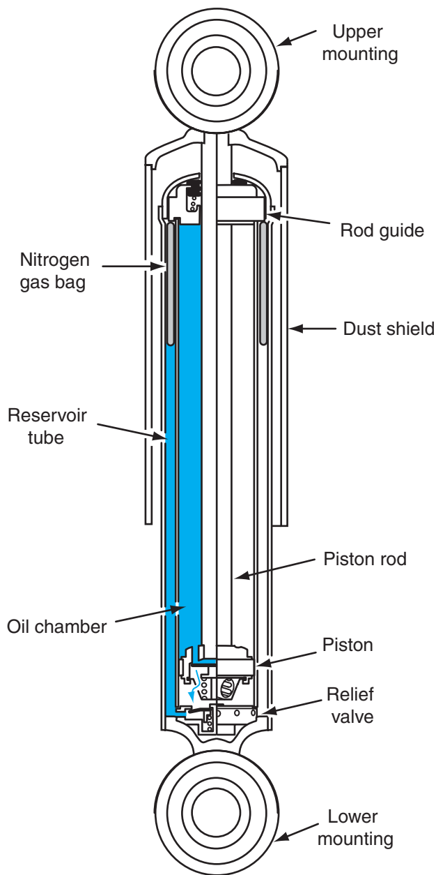
Figure 1-14 Shock absorber design.
