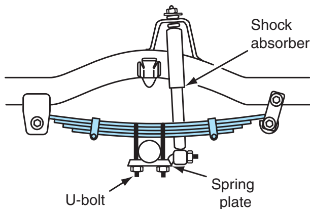
Figure 7-30 Leaf-spring rear suspension.
