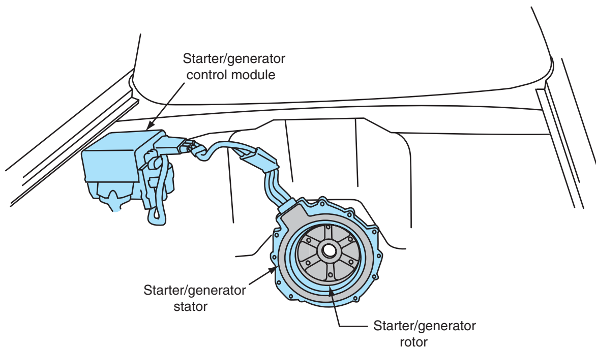
Figure 10-23 Starter/generator and starter/generator control module (SGCM).
