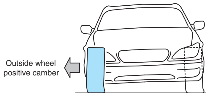
Figure 15-33 While cornering at high speed, the camber on the outside front wheel moves to a slightly more positive position and the outside edge of the tire grips the road surface to resist lateral skidding.
