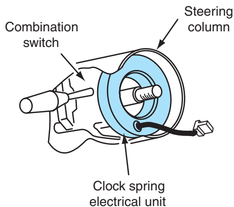
Figure 9-13 Clock spring electrical connector, or spiral cable, maintains electrical contact between the air bag inflator module and the air bag electrical system.
