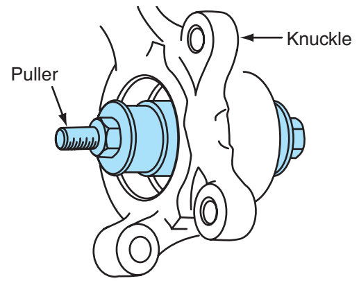
Figure 3-21 Wheel bearing removal from knuckle.
