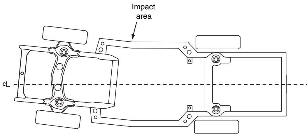
Figure 14-11 When a frame has overall side sway damage, it is slightly V-shaped.
