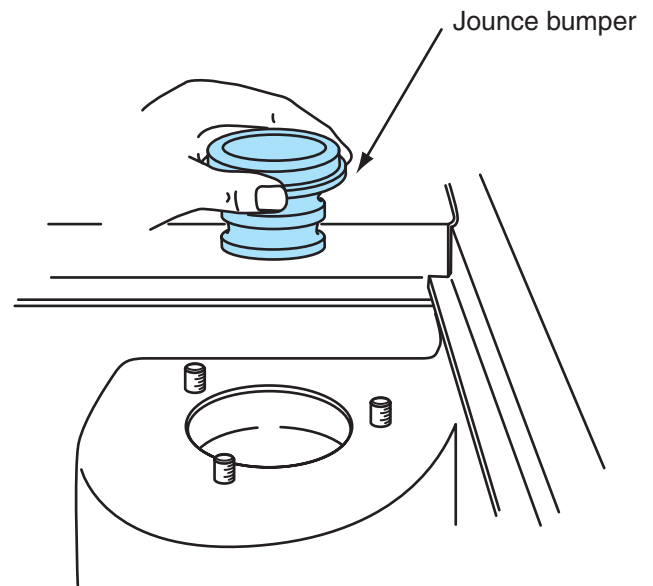
Figure 5-31 Removing jounce bumper.
