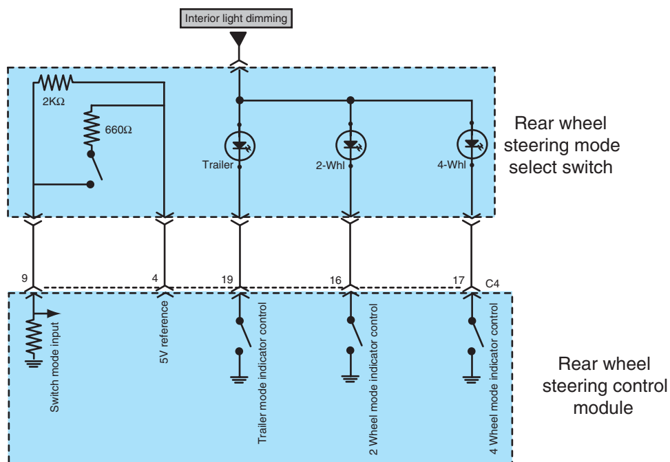
Figure 13-9 Rear wheel steering mode select switch inputs to the control module.
