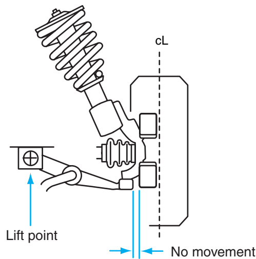
Figure 6-13 Ball joint wear measurement on MacPherson strut front suspension.
