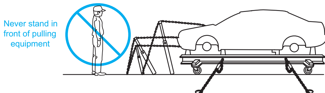
Figure 14-12 Do not stand in front of pulling equipment while it is in operation.
