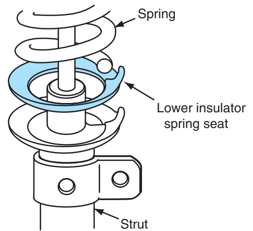
Figure 5-17 Installing strut in coil spring with proper lower spring seat alignment.
