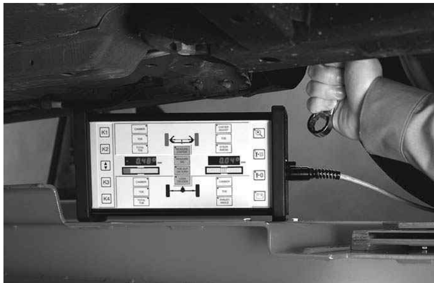
Figure 15-26 Remote display for computer wheel aligner. (Courtesy of Hunter Engineering Company.)
