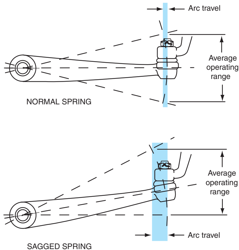
Figure 6-58 Sagged springs change the normal operating arc of the lower ball joint and cause excessive lateral tire movement during wheel jounce and rebound with resulting tire wear.
