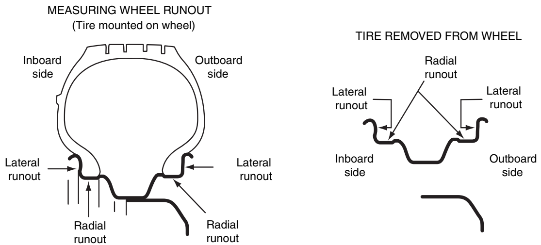
Figure 4-19 Measuring wheel radial and lateral runout.
