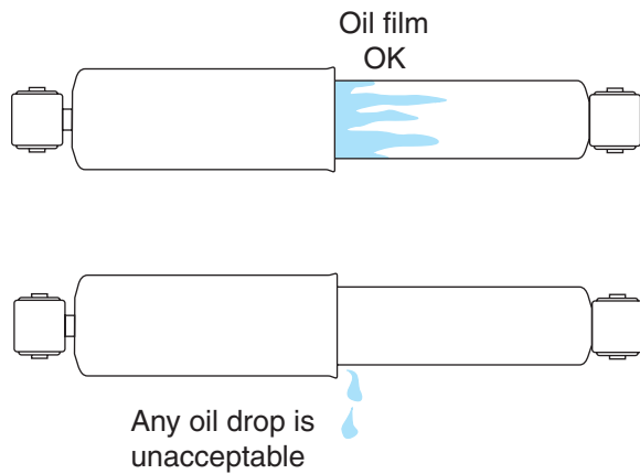
Figure 5-1 Shock absorber and strut oil leak diagnosis.
