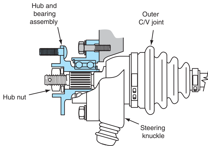
Figure 3-14 Wheel bearing and hub assembly.
