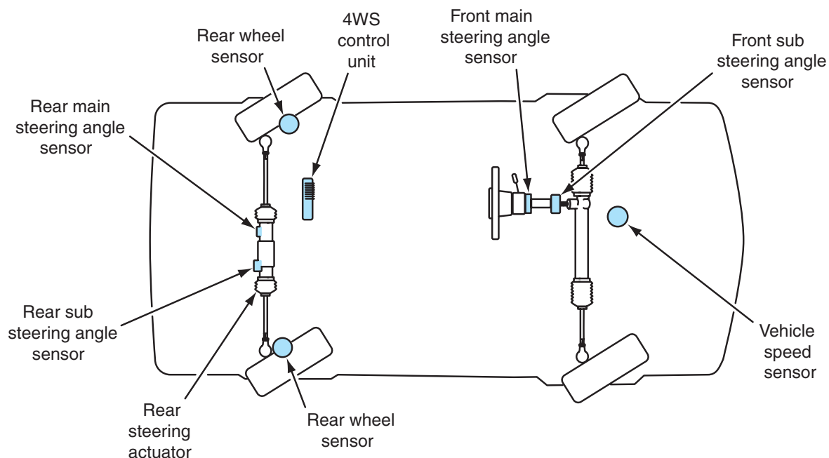
Figure 13-2 Electronically controlled 4WS with control unit mounted in the trunk.
