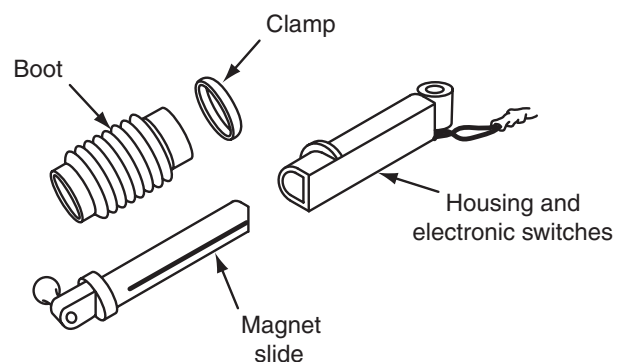
Figure 8-20 Height sensor.
