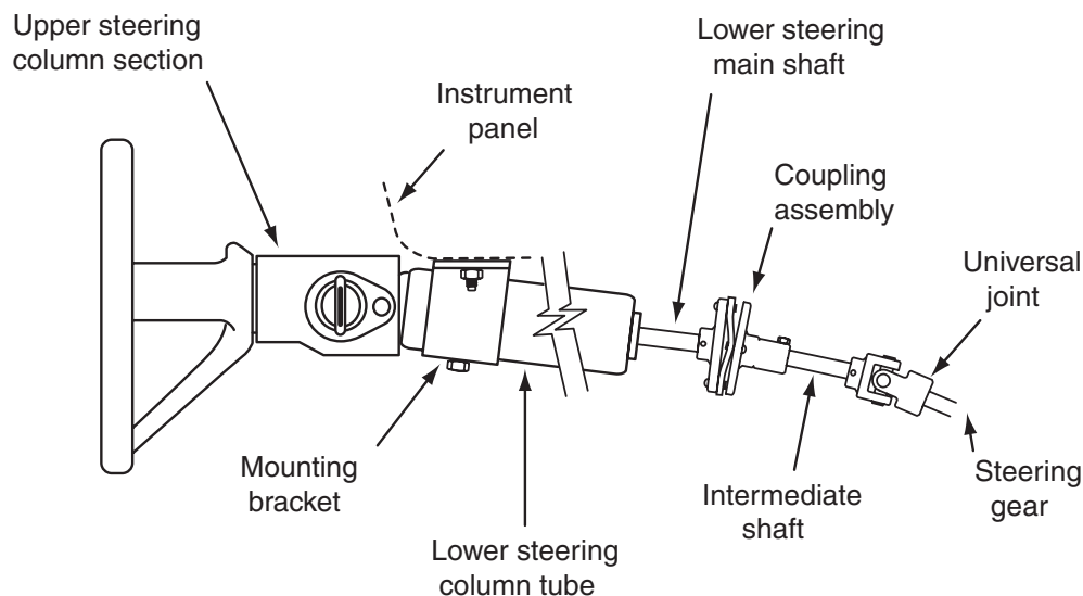
Figure 1-20 Tilt steering column.
