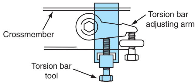
Figure 6-51 Torsion bar tool and adapters.
