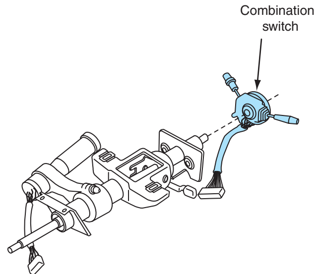
Figure 9-14 Removing combination switch and wiring harness.
