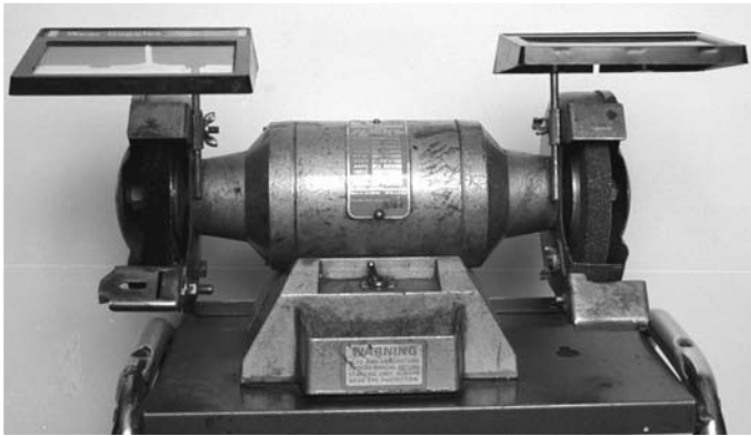
Figure 2-33 Bench grinder.
