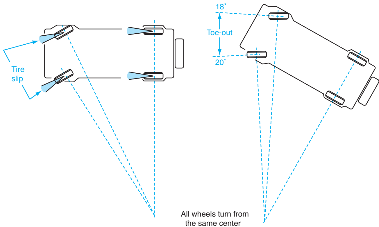
Figure 16-13 Slip angle during a turn.
