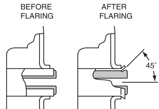
Figure 6-43 Front control arm bushing after flaring.
