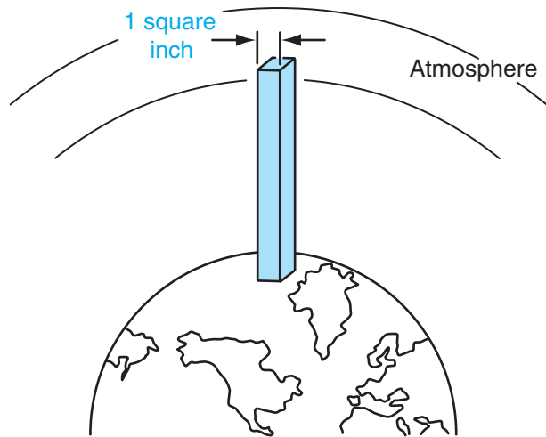
Figure 2-22 A column of air one inch square extending from the earth's surface at sea level to the outer edge of the atmosphere weighs 14.7 pounds.
