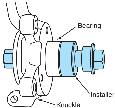
Figure 3-22 Wheel bearing installation in knuckle.
