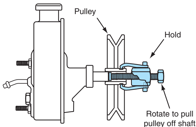
Figure 10-20 Press-on power steering pump pulley removal.
