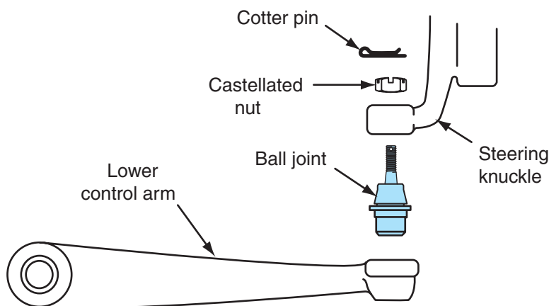
Figure 7-24 Removing the lower control arm and ball joint.
