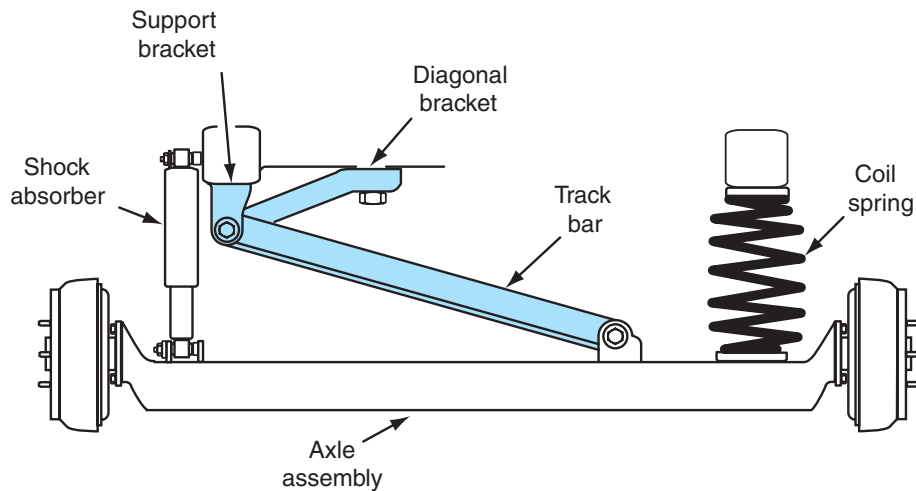
Figure 7-18 Semi-independent rear suspension with track bar and brace.
