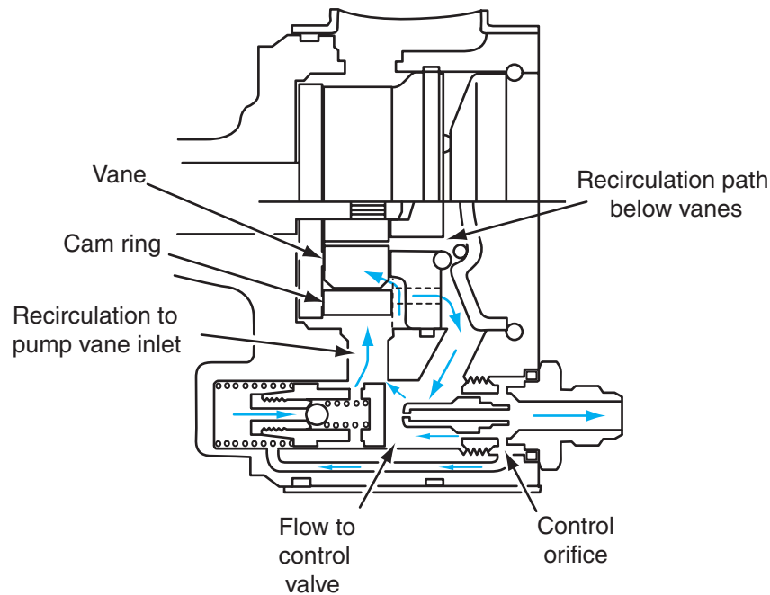
Figure 10-15 Flow control valve operation under various conditions.
