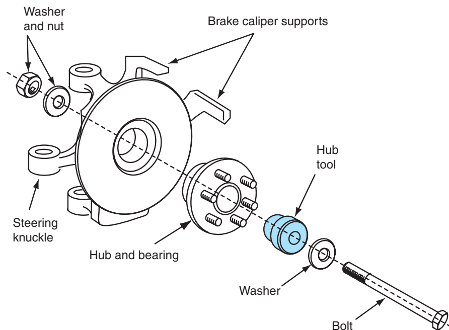
Figure 2-6 Front bearing hub tool.
