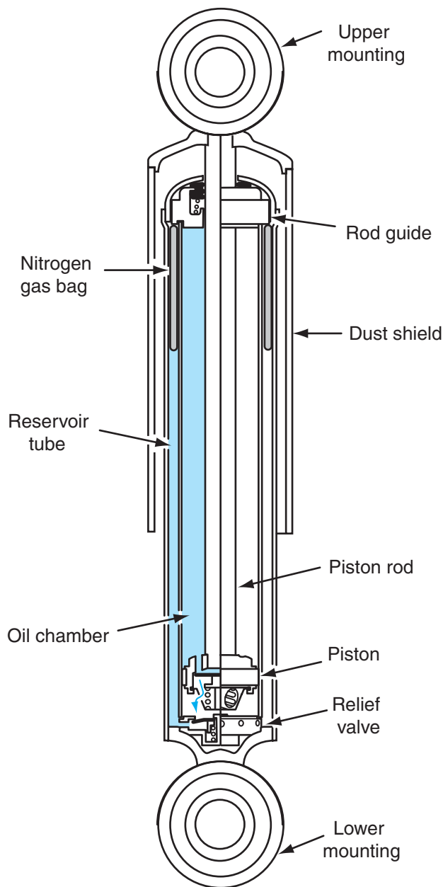
Figure 5-1 Shock absorber filled with hydraulic oil and nitrogen gas.
