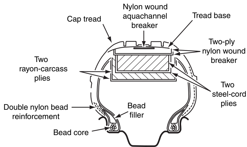
Figure 4-2 Tires designed for improved steering and handling with a nylon bead reinforcement and a hard bead filler with a slim tapered profile.
