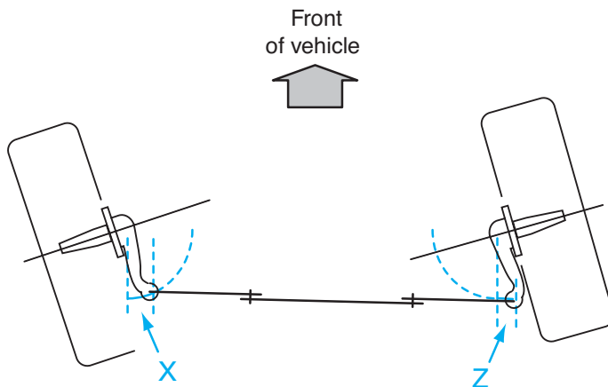
Figure 16-12 Steering arm operation while turning.
