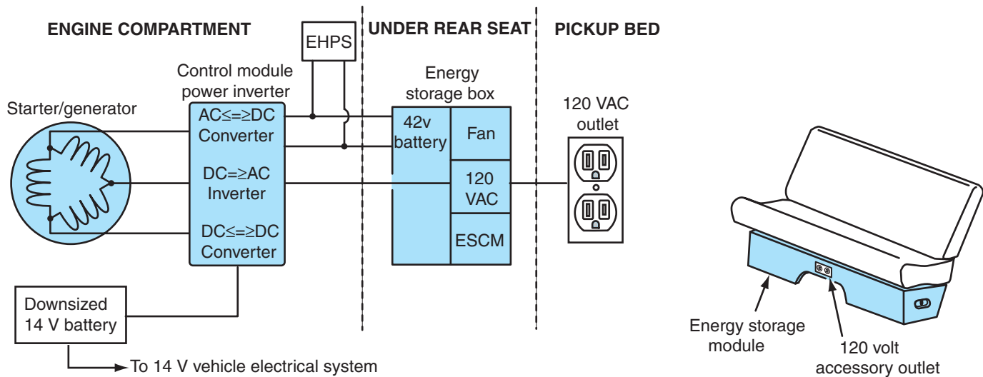
Figure 10-26 SGCM internal voltage converters and external battery connections.
