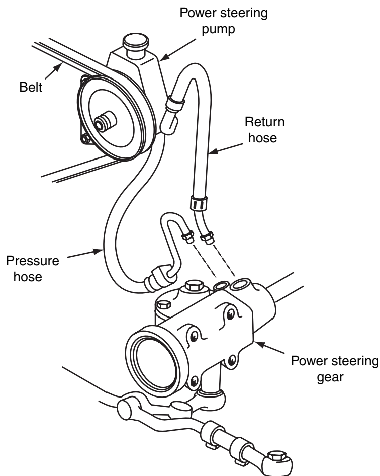
Figure 10-7 Integral power-assisted steering system.
