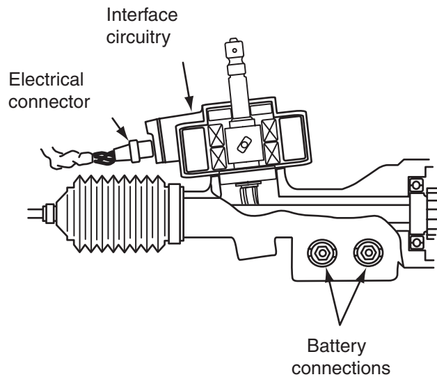
Figure 12-28 Interface in the steering sensor.
