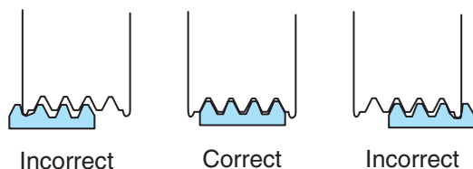
Figure 10-3 Proper and improper installation of ribbed V-belt on a pulley.
