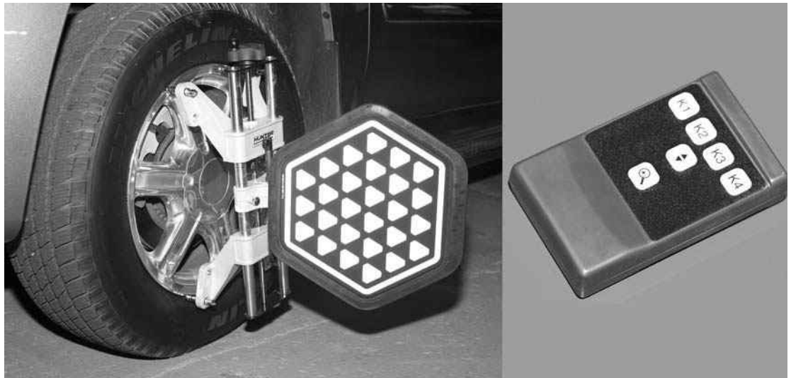
Figure 15-13 A handheld remote control transmits ride height measurements electronically to the console and monitor.
