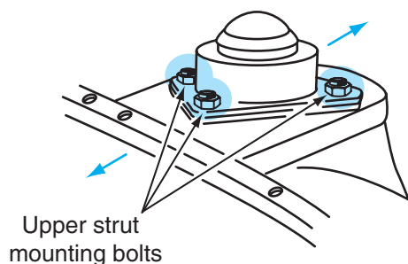
Figure 16-17 The upper strut mounting bolts can be loosened and the mount moved inward or outward to adjust camber on some MacPherson strut front suspension systems.
