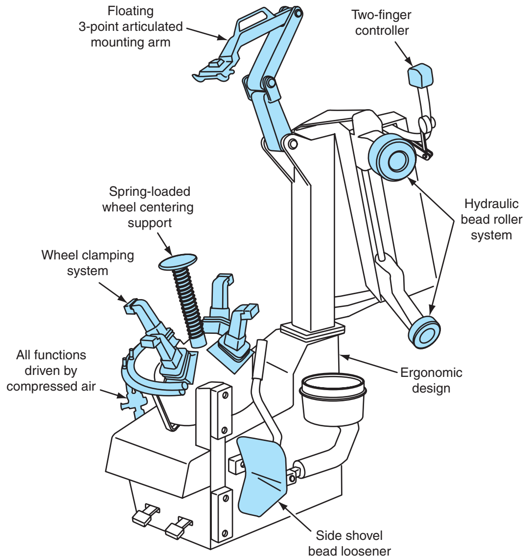
Figure 4-6 Tire changer.
