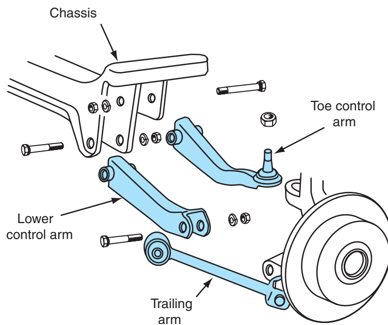
Figure 7-39 Multilink rear suspension with parallel lower control arm and toe control arm.
