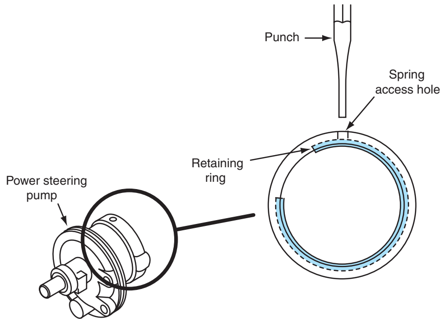
Figure 10-24 Retaining ring removal.
