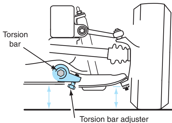
Figure 6-3 Curb riding height measurement, torsion bar front suspension.
