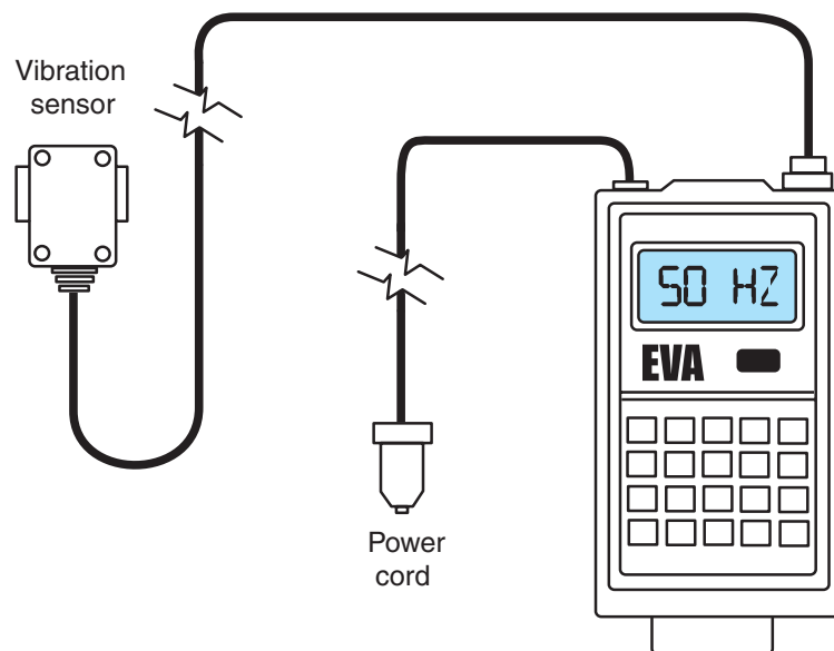
Figure 7-1 Electronic vibration analyzer (EVA).
