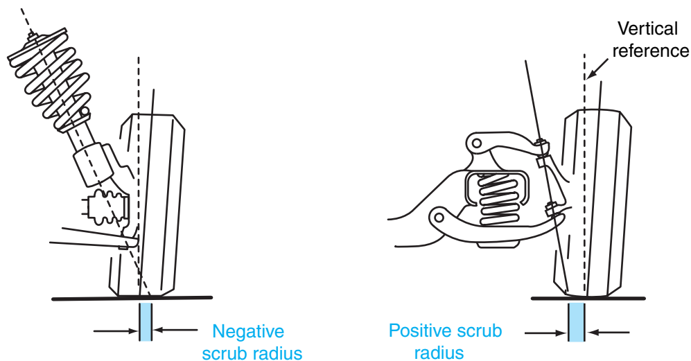
Figure 1-38 Scrub radius.
