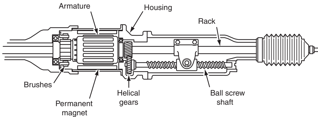
Figure 1-30 Electronic power steering gear.
