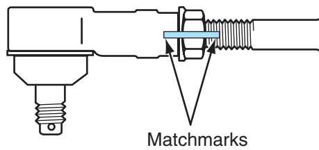
Figure 12-39 Aligning marks on the outer tie-rod ends, jam nuts, and tie-rods.
