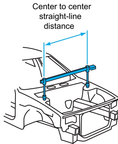
Figure 14-13 Performing an upper strut tower measurement with a tram gauge on a unitized body vehicle.
