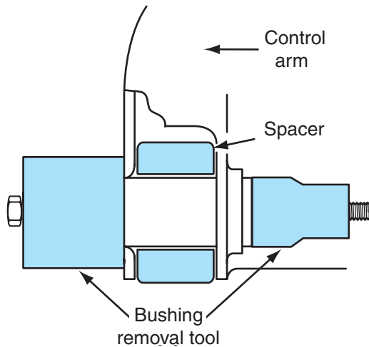
Figure 6-44 Removing the rear control arm bushing.
