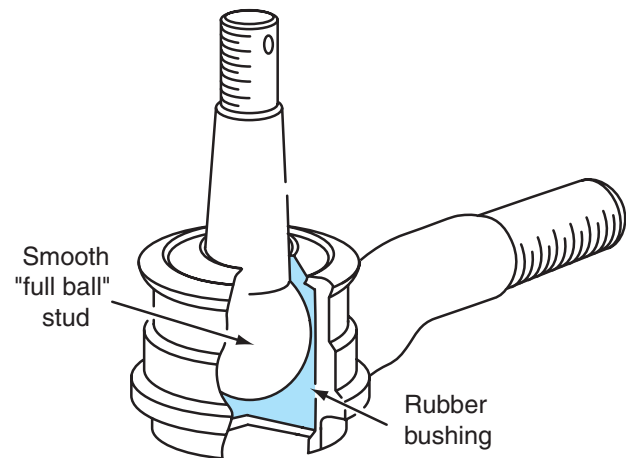
Figure 9-44 Tie-rod end with rubber encapsulated ball stud.
