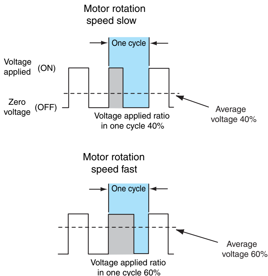
Figure 12-33 Pulse width modulated (PWM) voltage signal.
