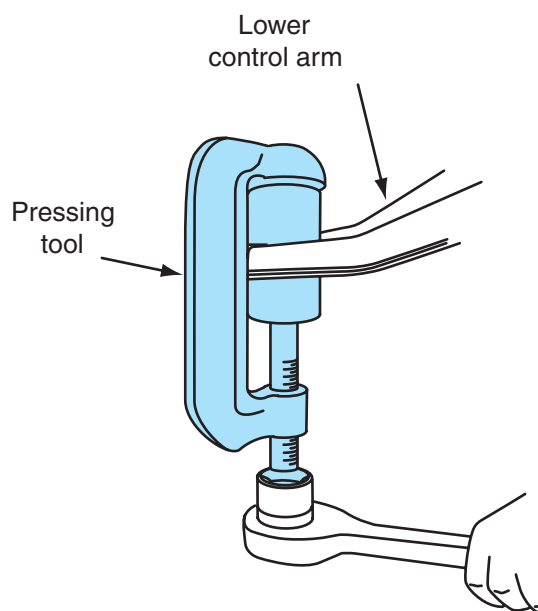
Figure 7-26 Installing the ball joint in the lower control arm.
