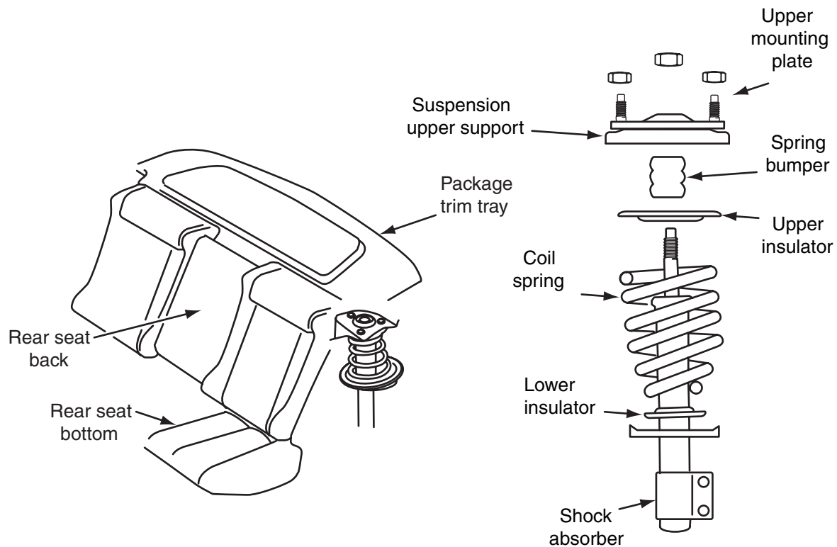
Figure 7-8 Rear suspension with rear seat and package trim tray.
