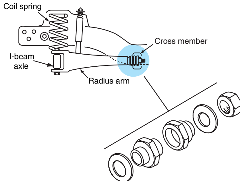
Figure 16-33 Radius arm bushing for caster adjustment on some twin I-beam suspension systems.
