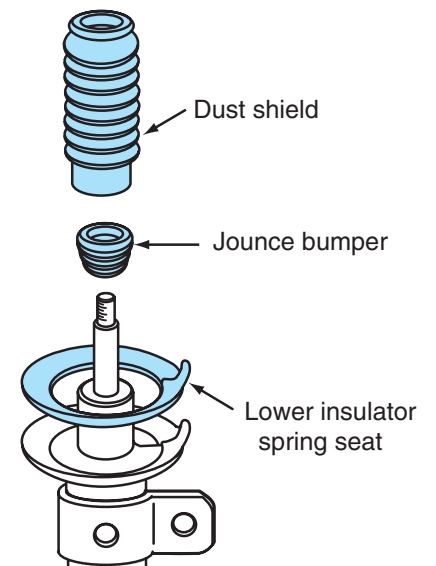
Figure 5-13 Removal of the dust shield, jounce bumper, and lower spring insulator.
