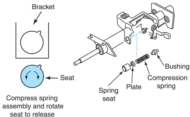
Figure 9-17 Removing compression spring, seat, and bushing.
