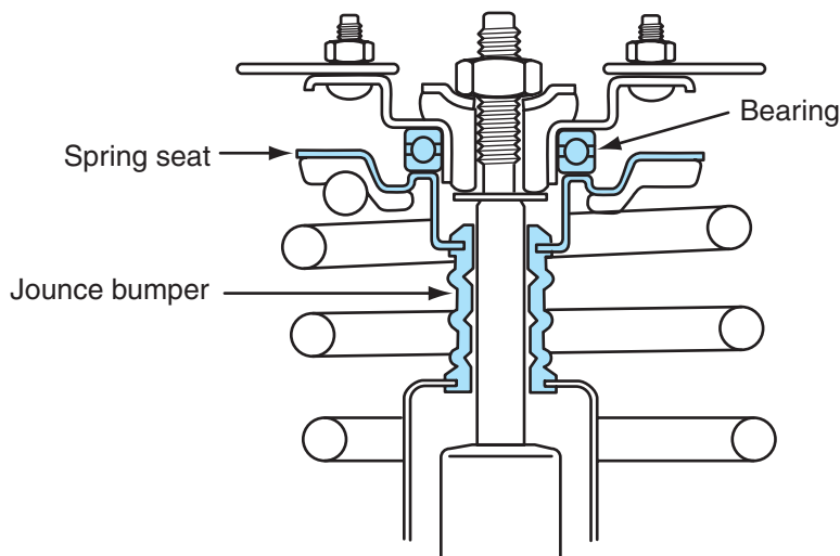
Figure 5-6 Upper strut mount.
