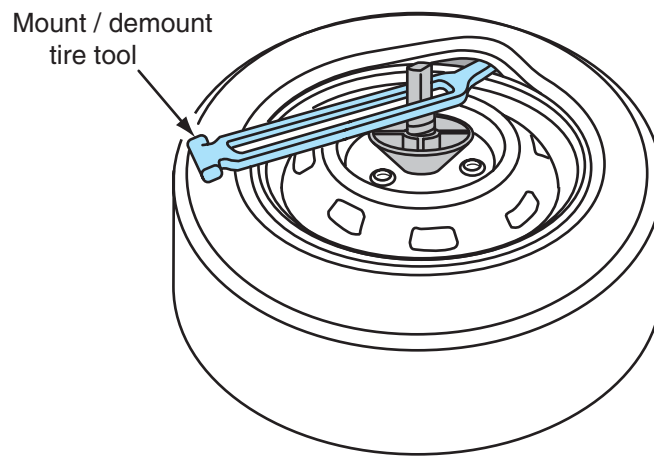
Figure 4-11 Steel mount/demount tool for steel rims.
