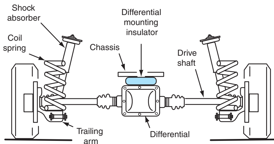
Figure 7-30 Independent rear suspension with rear axle carrier.
