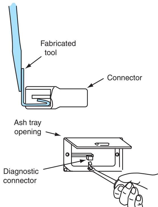
Figure 8-1 Self-test terminals, programmed ride control system.
