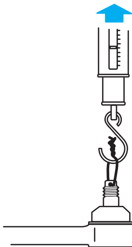
Figure 12-12 Measuring inner tie-rod end articulation effort.
