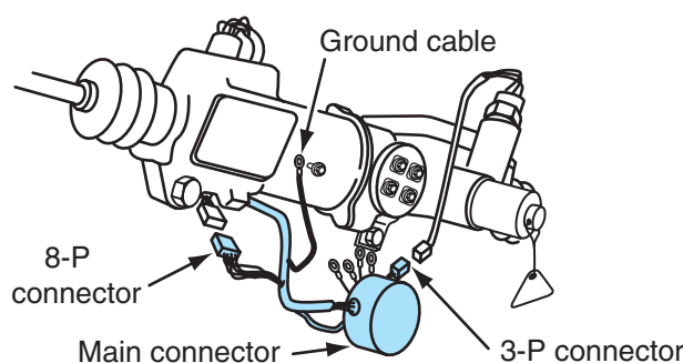
Figure 13-28 Installing wiring connectors on the rear steering actuator.
