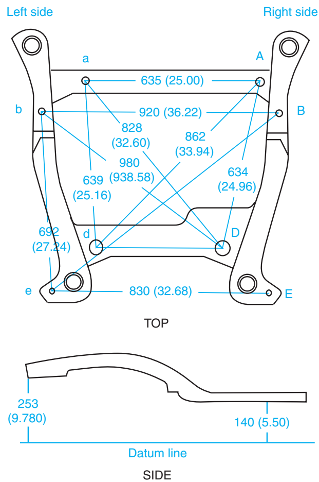
Figure 16-37 Front cradle measurements.
