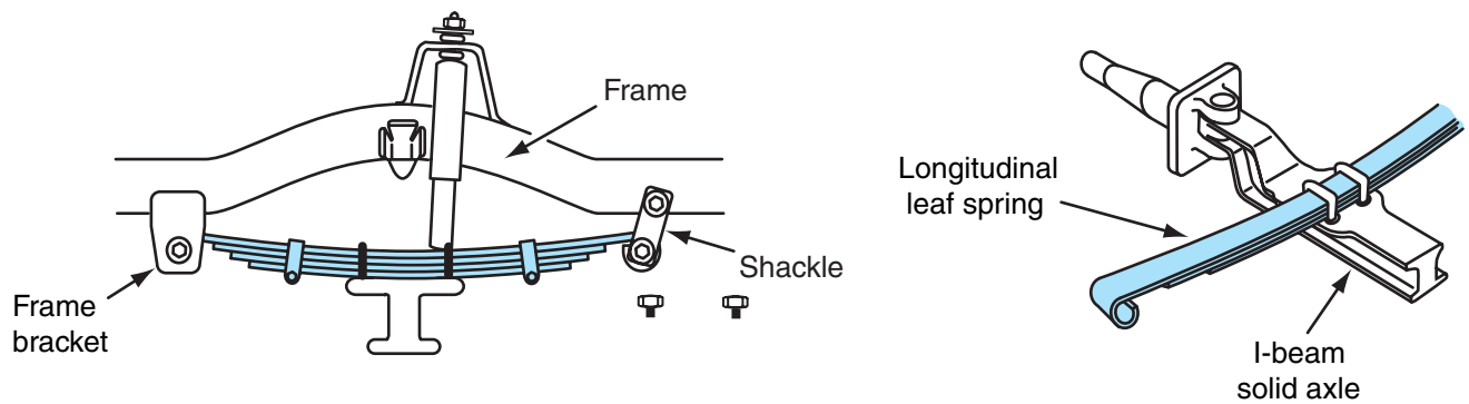
Figure 6-48 Front leaf spring.
