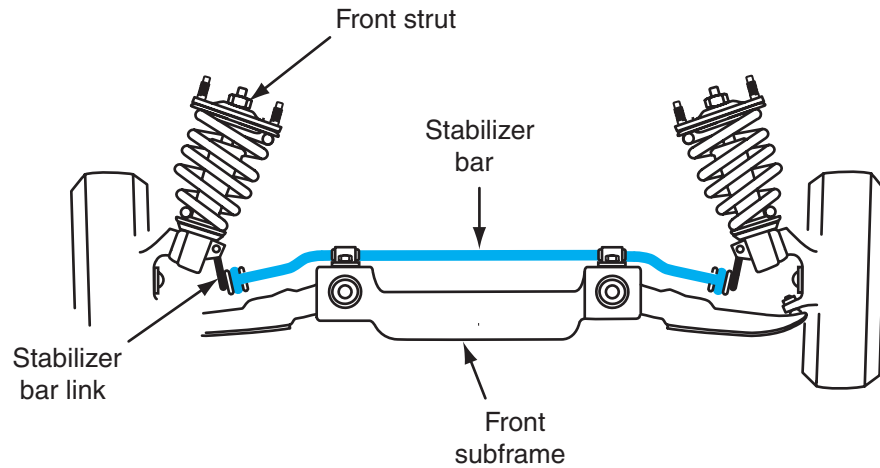
Figure 6-32 Stabilizer bar connected to the front strut.
