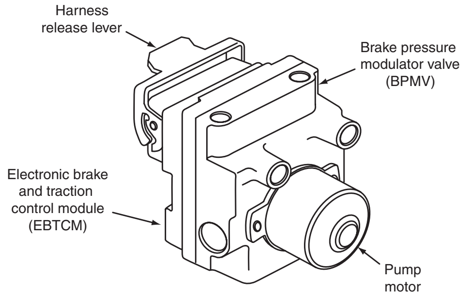
Figure 8-49 The electronic brake and traction control module (EBTCM) contains the antilock brake system (ABS), traction control system, and stability control modules.
