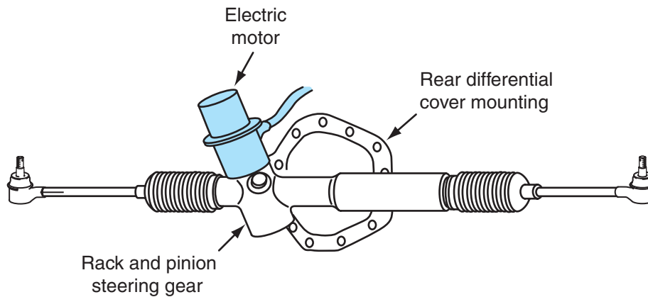
Figure 13-16 Four-wheel steering gear and motor.
