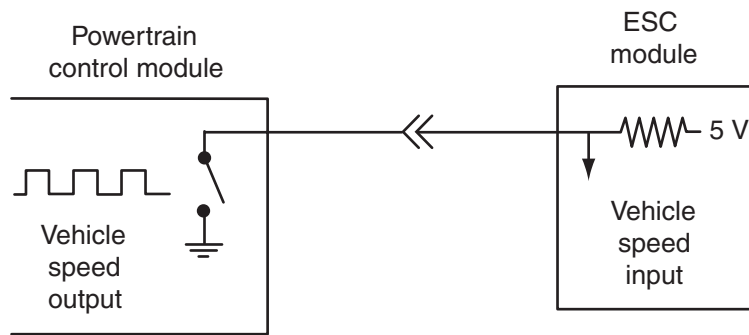
Figure 8-35 The vehicle speed sensor (VSS) signal is sent to the powertrain control module (PCM) and transmitted to the ESC module.
