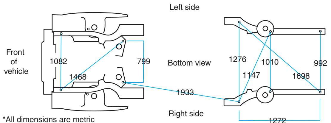
Figure 16-36 Front and rear underbody measurements.
