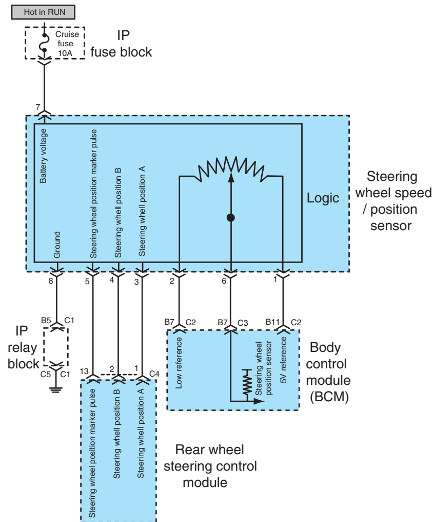
Figure 13-11 SWPS inputs to the control module.
