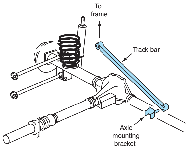
Figure 7-15 Track bar and brace.
