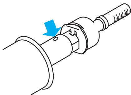
Figure 12-37 Rack vent holes must be open.
