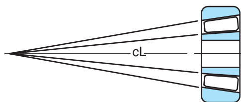
Figure 3-7 Imaginary lines extending from tapered roller bearing races eventually meet at a point extending from the bearing center.
