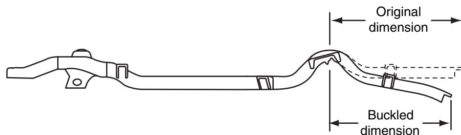
Figure 14-13 Rear frame buckle.
