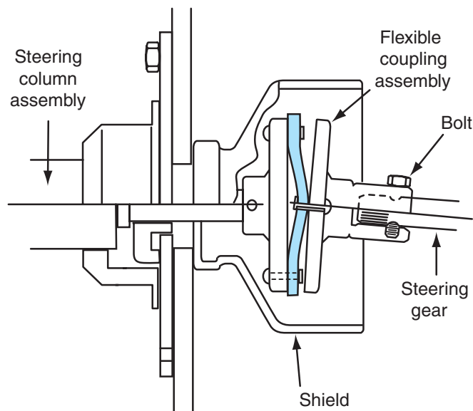
Figure 9-42 Flexible coupling installation.
