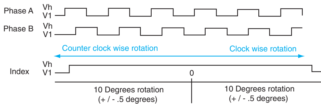
Figure 13-3 Steering wheel position sensor phase A, phase B, and marker pulse signals.
