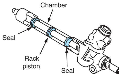
Figure 12-2 Hydraulic chamber in a power rack and pinion steering gear.
