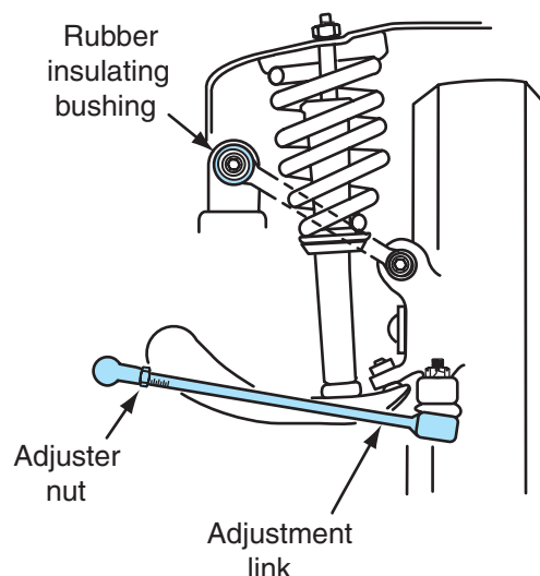
Figure 1-11 Short-and-long arm independent rear suspension system.
