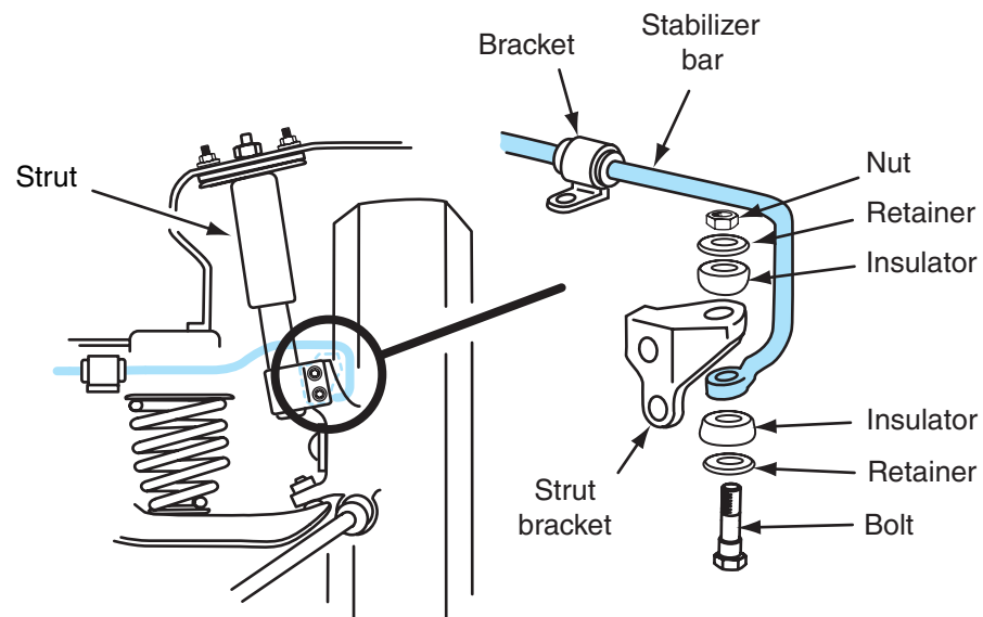
Figure 7-32 Stabilizer bar, bushings, grommets, and brackets.
