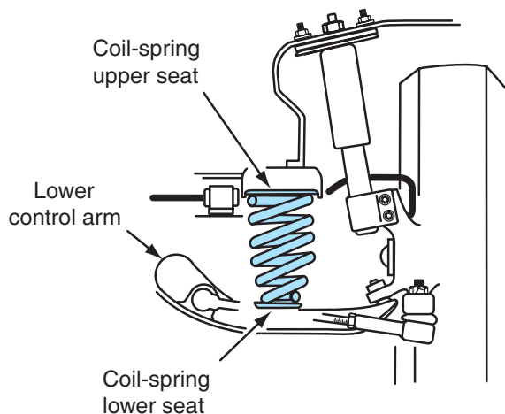
Figure 7-28 Installing the spring and insulators.
