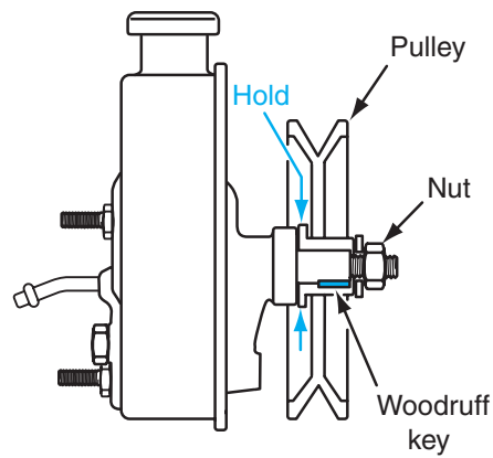
Figure 10-22 Removing power steering pump pulley and nut.
