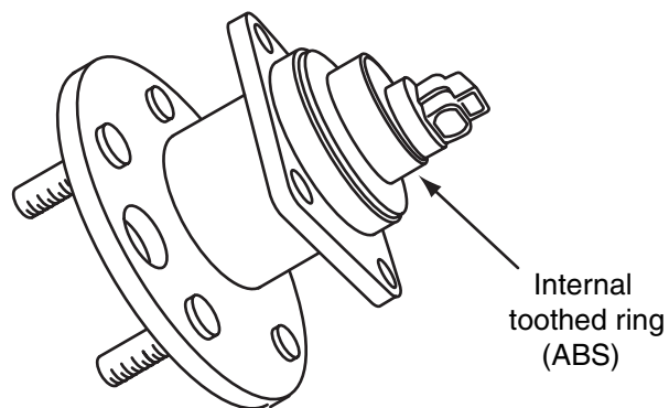
Figure 7-42 One-piece rear wheel bearing assembly.
