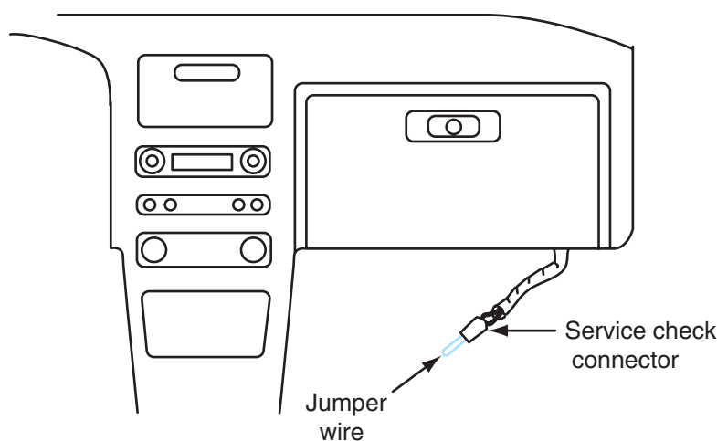
Figure 12-42 EPS system service check connector and special jumper wire.
