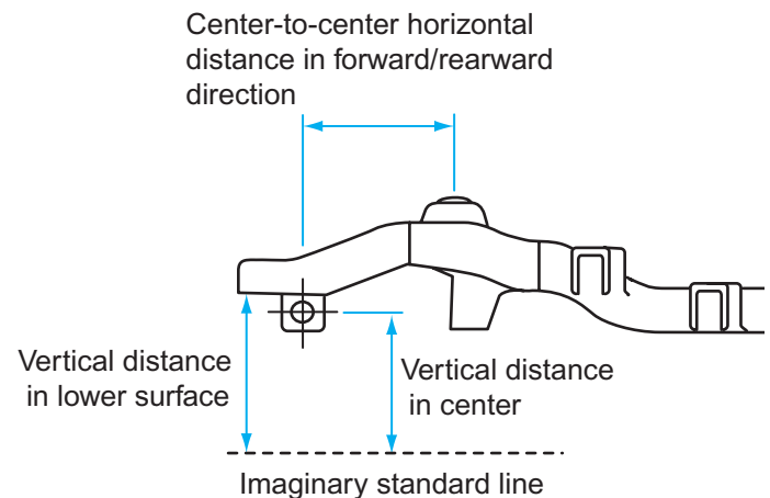
Figure 14-9 Horizontal and vertical frame measurements.
