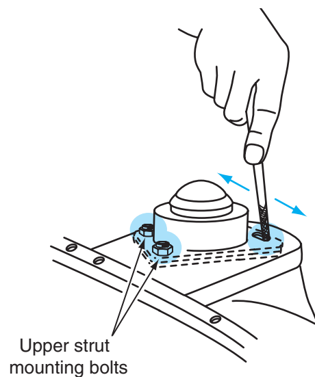
Figure 16-31 Elongating upper strut mount bolt openings to provide caster adjustment.
