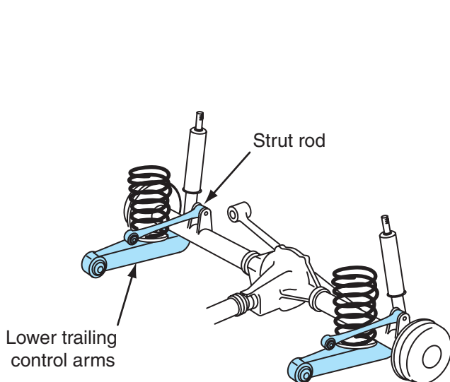
Figure 7-12 Live-axle coil-spring rear suspension.
