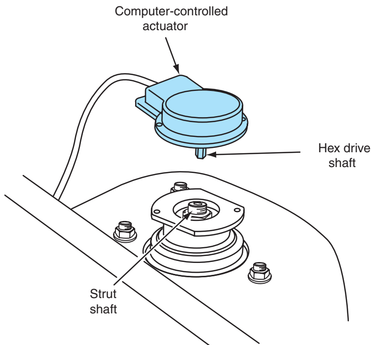
Figure 1-17 Strut actuator.
