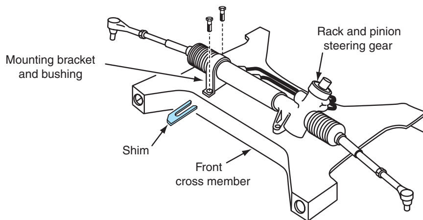
Figure 15-44 On some imported vehicles, shims between the rack and pinion steering gear and the chassis adjust the steering linkage height.
