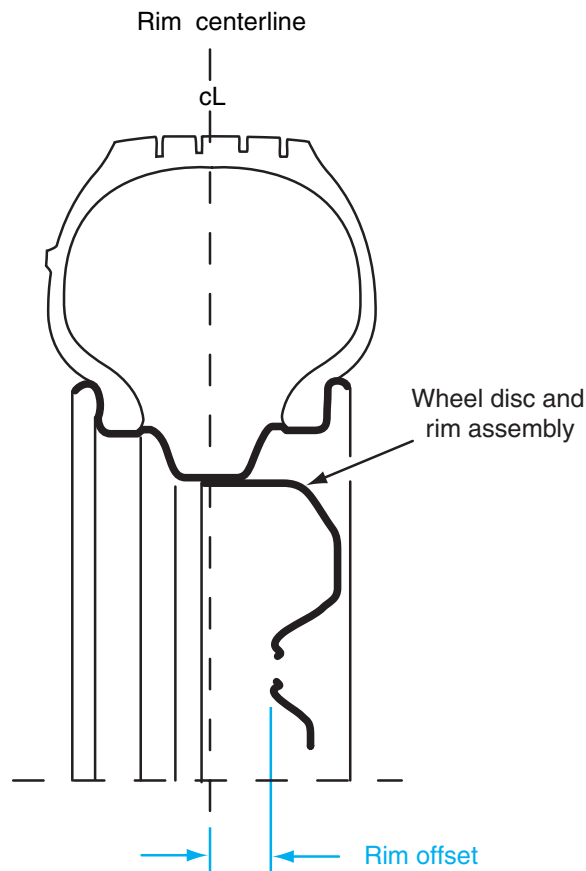
Figure 1-12 Wheel rim design.
