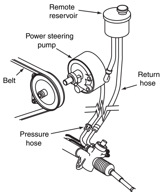
Figure 10-27 Power steering hoses and lines.
