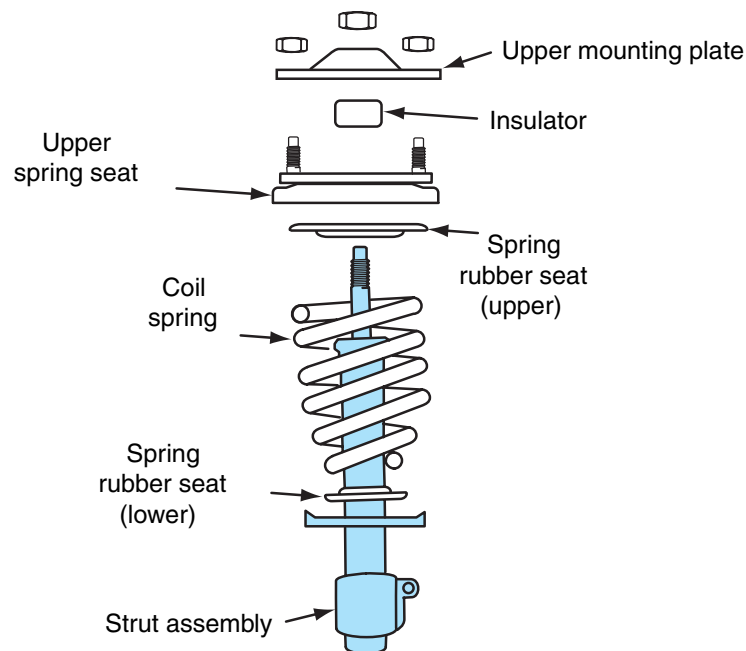
Figure 5-10 Rear suspension system with coil springs mounted on the struts.
