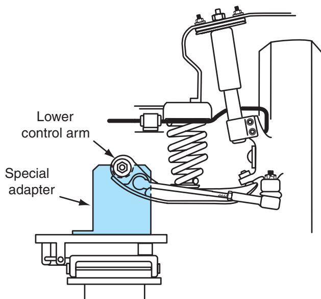
Figure 7-22 Special tool installed to support the inner end of the lower control arm.
