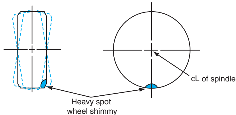
Figure 4-42 Dynamic wheel unbalance causes wheel shimmy.
