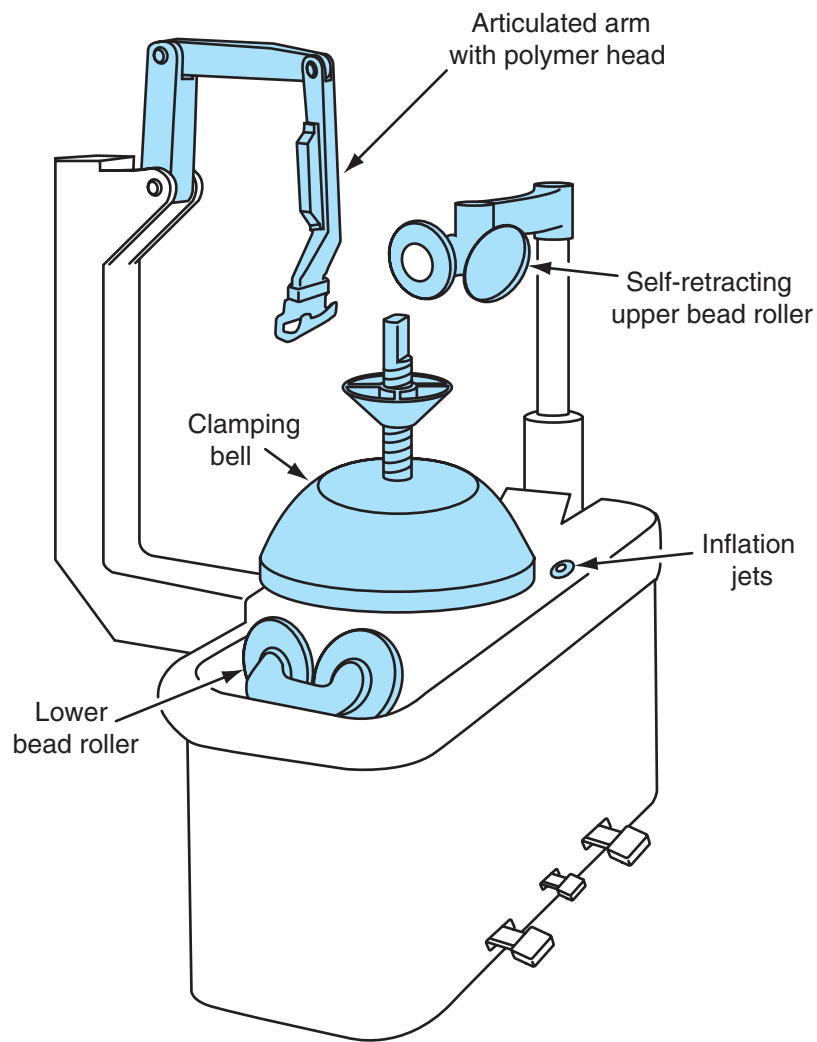
Figure 4-10 Tire changer with horizontal clamping mechanism.
