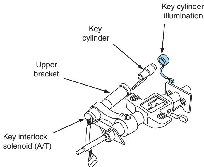
Figure 9-13 Ignition key cylinder illumination mounted above ignition switch cylinder.
