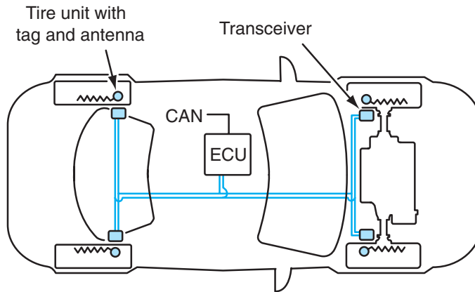
Figure 4-23 Transceivers and ECU in a tire pressure monitoring system.
