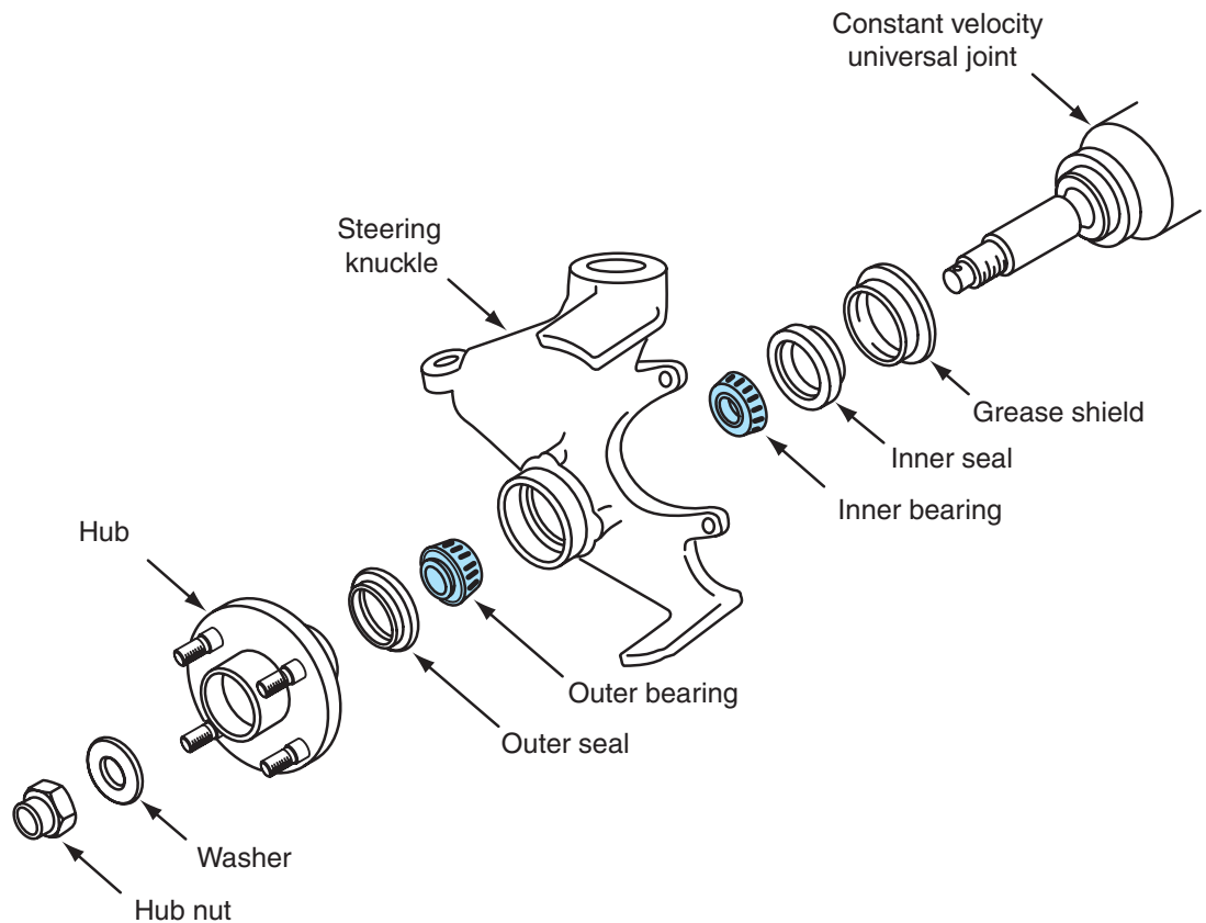
Figure 3-19 Steering knuckle with two separate tapered roller bearings.
