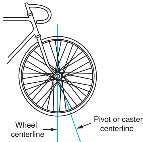
Figure 2-8 If a wheel centerline and pivot point are behind the front fork centerline pivot point, the wheel tends to return to the straight-ahead position after a turn. The wheel also tends to remain in the straight-ahead position as the bicycle is driven.
