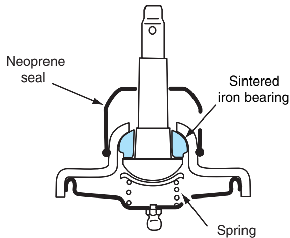
Figure 6-13 Non-load-carrying ball joint.
