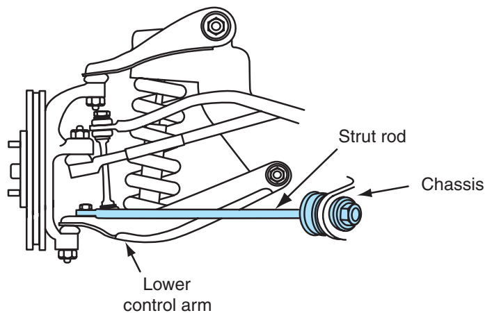
Figure 6-16 Strut, or radius, rod and bushings.
