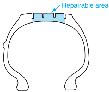
Figure 4-12 Repairable area on bias-ply and belted bias-ply tires.
