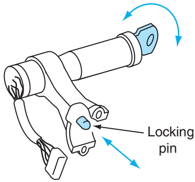
Figure 9-26 Inspecting ignition switch operation.
