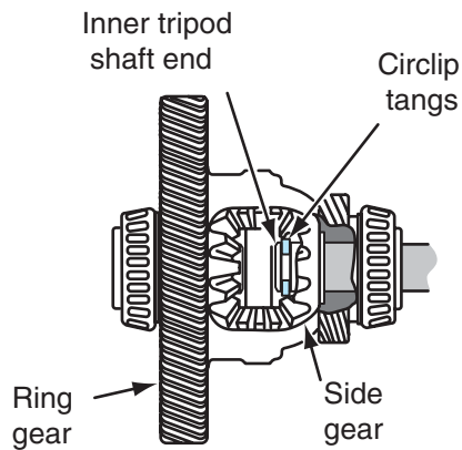
Figure 3-18 Compressible circlips in early model Chrysler transaxles.
