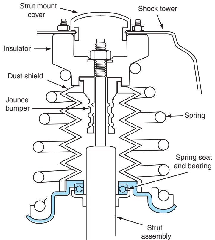
Figure 5-5 Strut assembly with bearing mounted in the lower spring seat.
