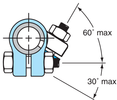
Figure 16-40 Proper tie-rod adjusting sleeve and clamp position.
