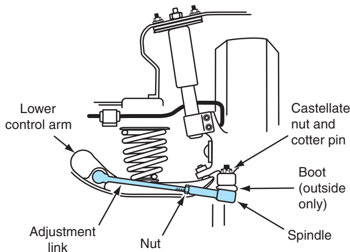
Figure 7-23 Removing the suspension adjustment link from the lower control arm.
