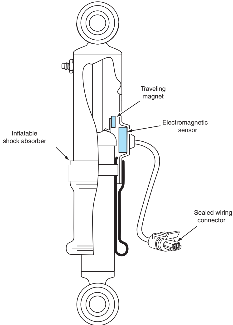
Figure 5-15 Load-leveling strut.
