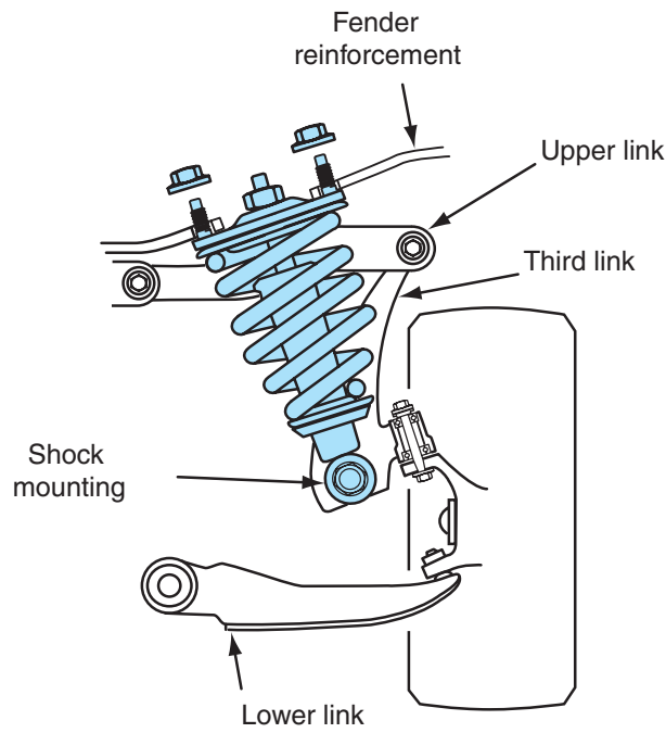
Figure 6-39 Complete multilink suspension system.
