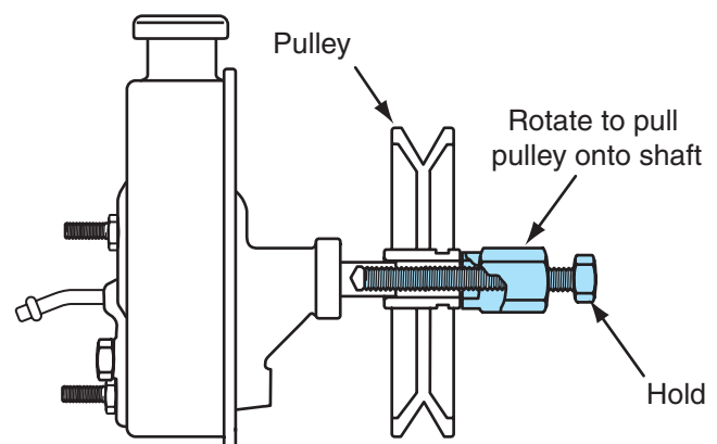
Figure 10-21 Press-on power steering pump pulley installation.
