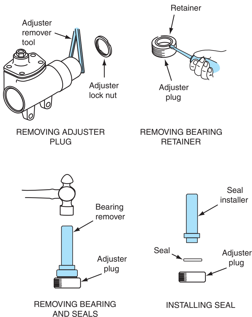
Figure 11-12 Removing and replacing worm shaft adjuster plug, bearing, and seal.
