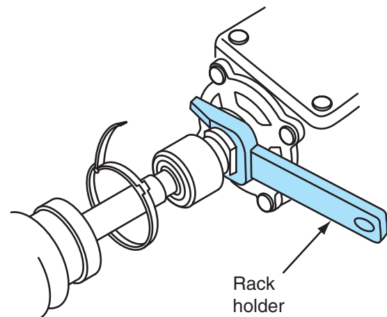
Figure 13-20 Installing the special tool to hold the shaft screw while tightening the inner tie-rod end.
