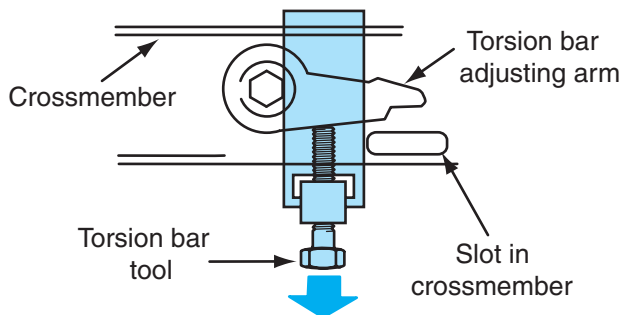
Figure 6-52 Loosening the torsion bar tool.
