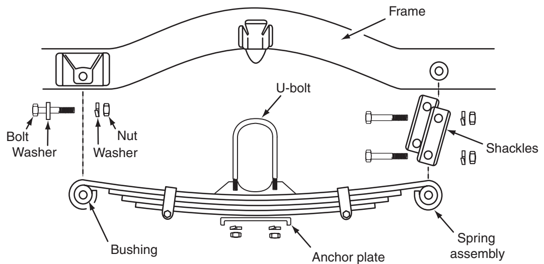
Figure 7-9 Individual leaf-spring suspension components.
