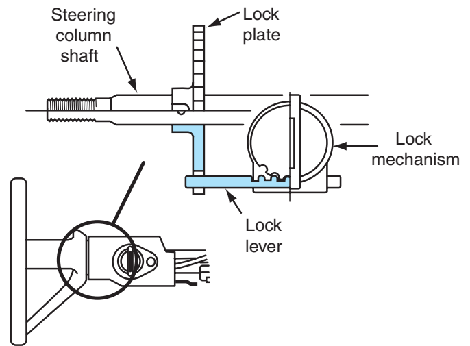
Figure 9-9 Upper steering column with locking plate and lever.
