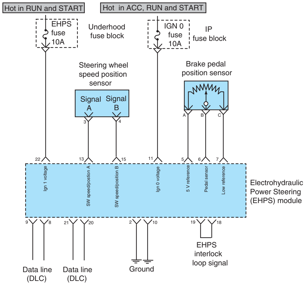
Figure 10-21 EHPS inputs.
