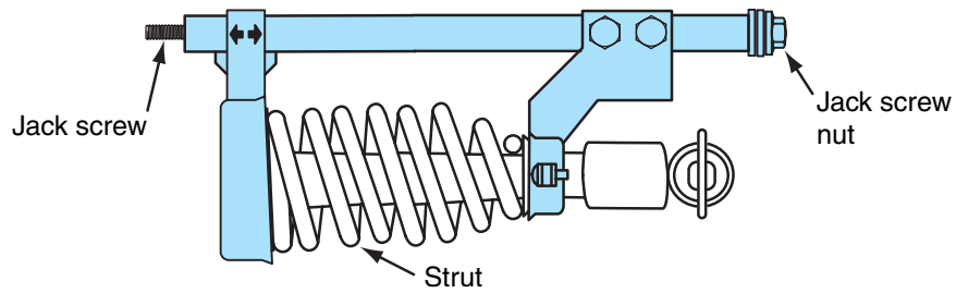
Figure 2-15 MacPherson strut coil spring compressor tool.
