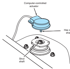
Figure 1-17 Strut actuator.
