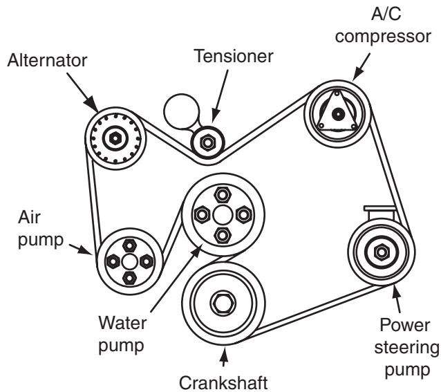
Figure 1-27 Ribbed V-belt.
