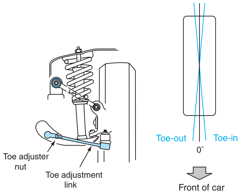
Figure 1-34 Rear wheel toe.
