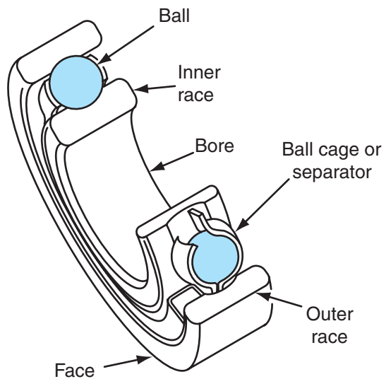
Figure 3-2 Parts of a ball bearing.
