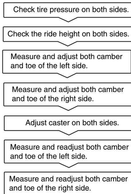
Figure 16-1 Front wheel alignment adjustment procedure.
