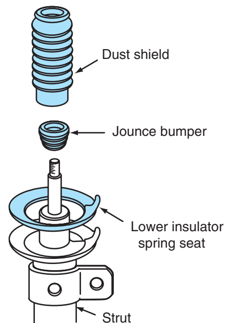
Figure 2-46 Removal of the dust shield, jounce bumper, and lower spring insulator.
