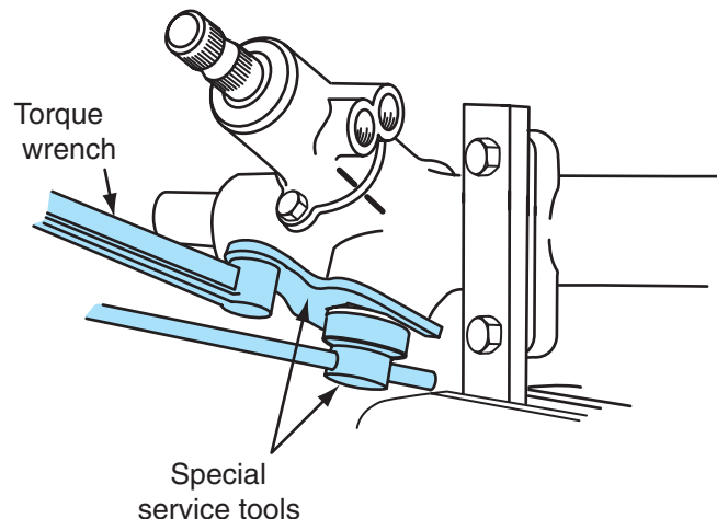
Figure 12-34 Tightening locknut on rack spring cap.
