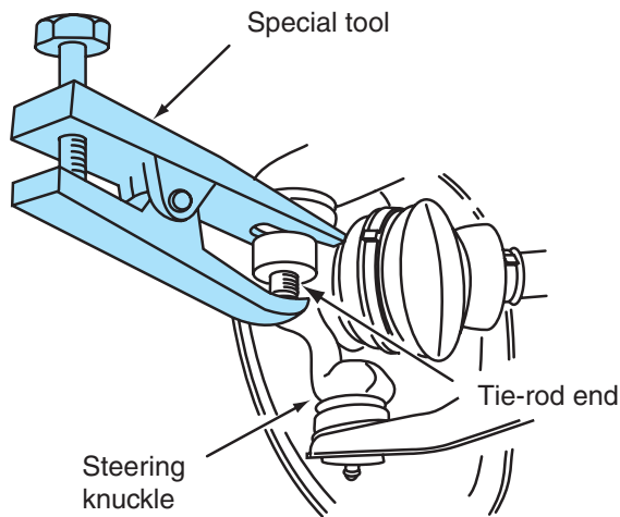
Figure 9-43 Removing tie-rod end.
