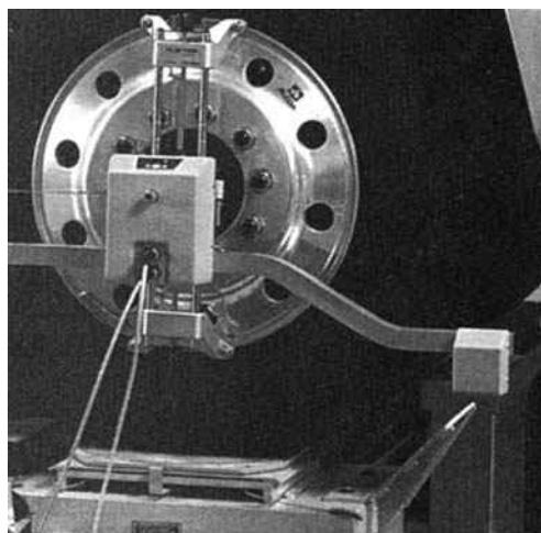
Figure 15-17 Front wheel sensor with optical arm and string connected to the rear wheel sensor.
