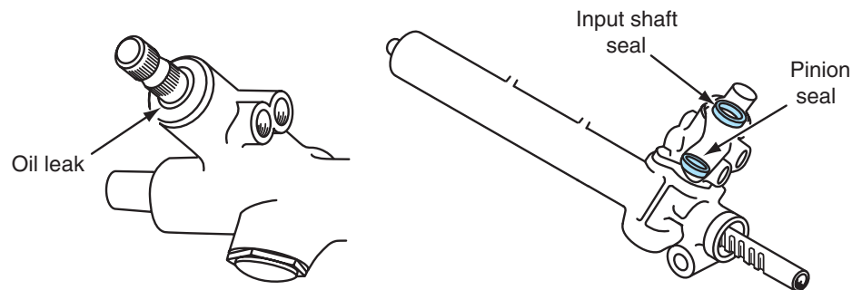
Figure 12-18 Pinion seal leak diagnosis.
