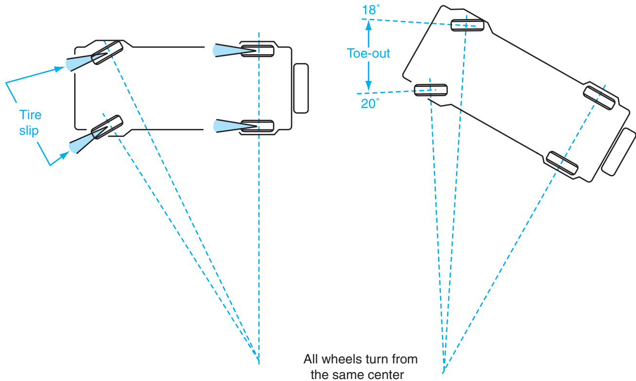
Figure 1-40 Turning radius.
