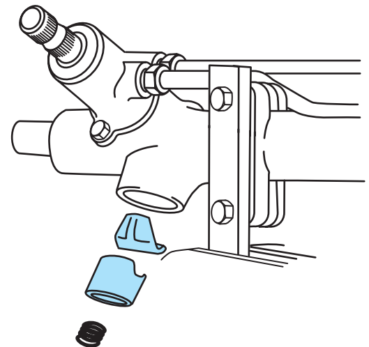
Figure 12-30 Removing spring, rack guide, and seat.
