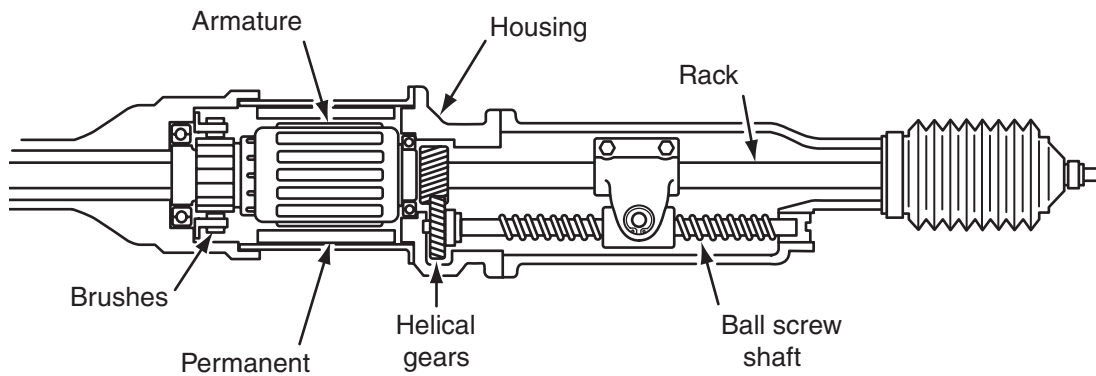
Figure 12-29 Steering gear and electric motor.
