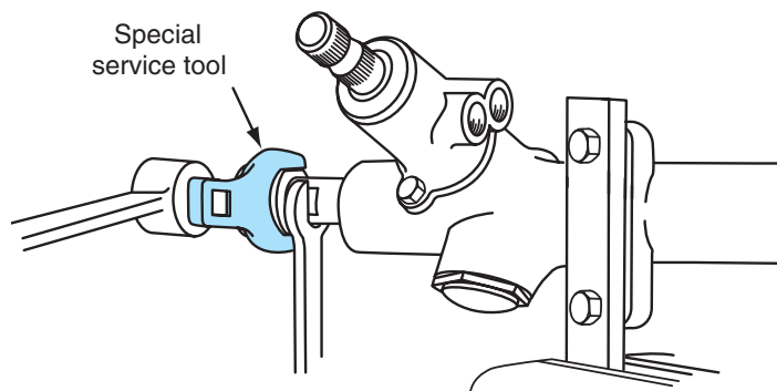
Figure 12-35 Tightening inner tie-rod end on the rack.
