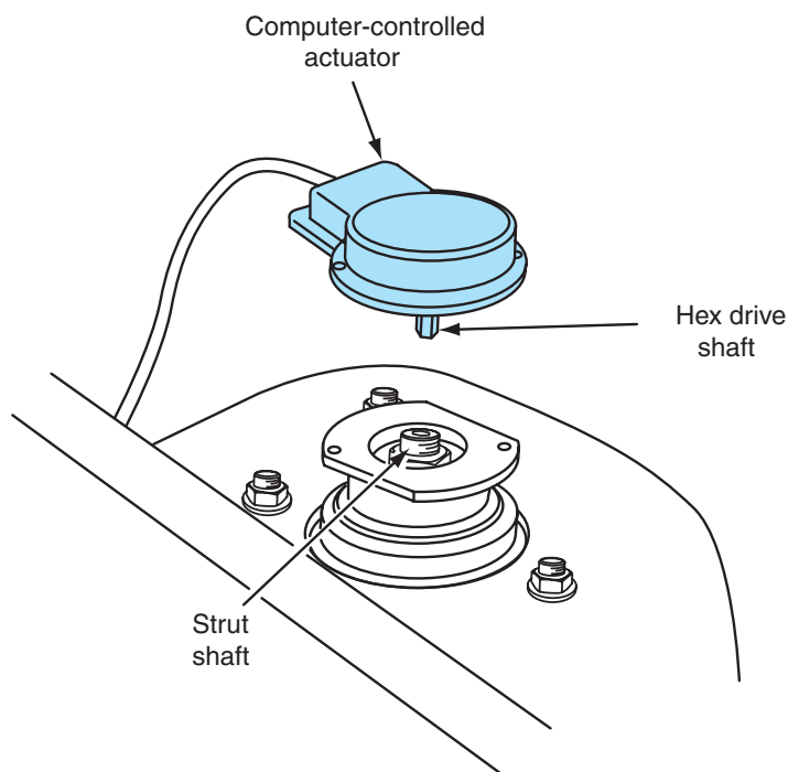
Figure 8-5 Strut actuator.
