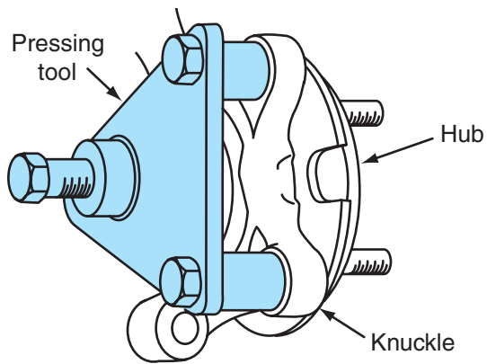
Figure 3-20 Wheel hub removal from bearing.
