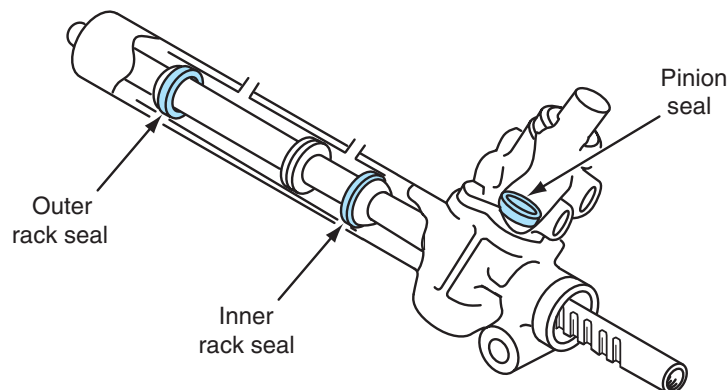
Figure 12-20 Rack seals and pinion seal.
