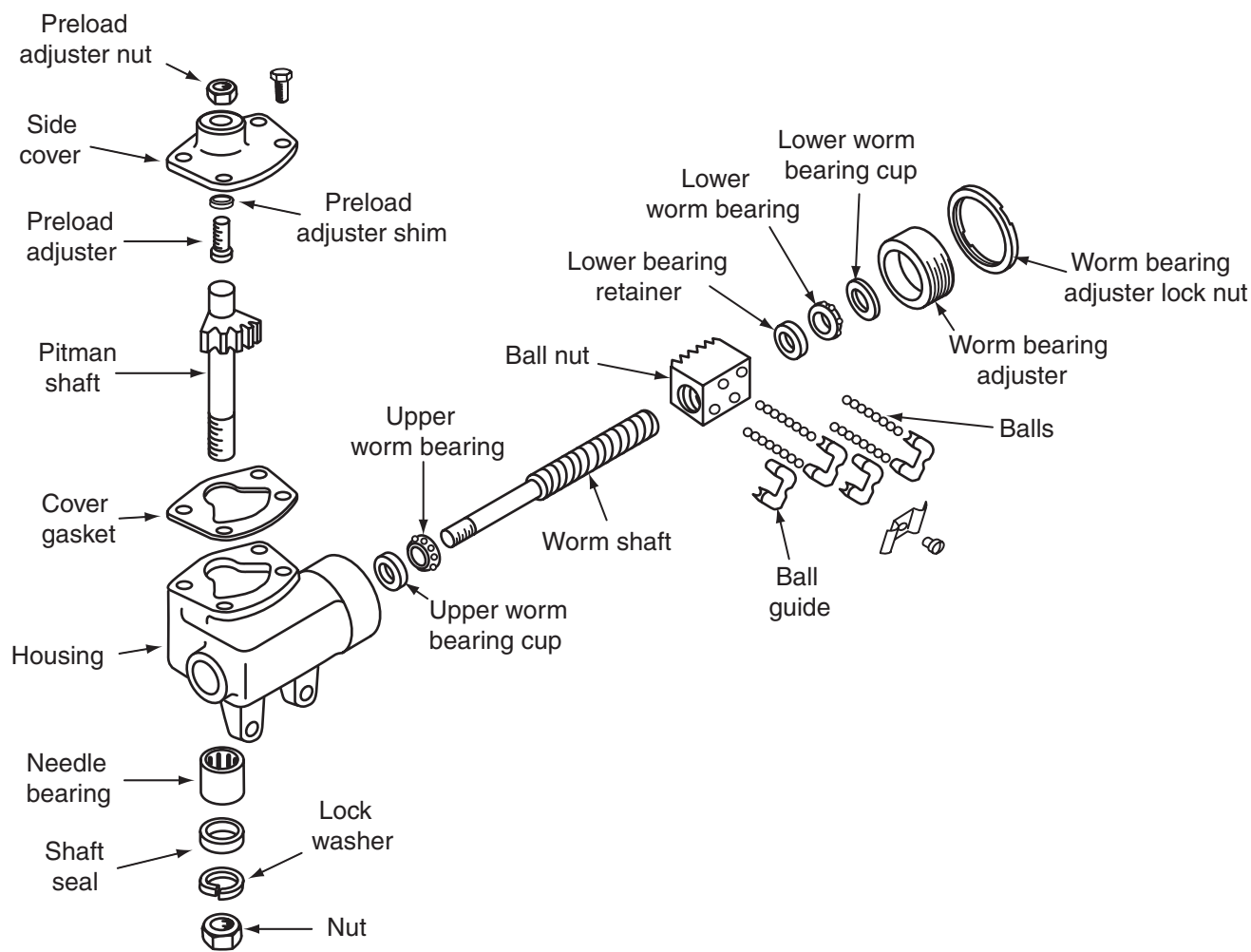
Figure 11-1 Manual recirculating ball steering gear design.
