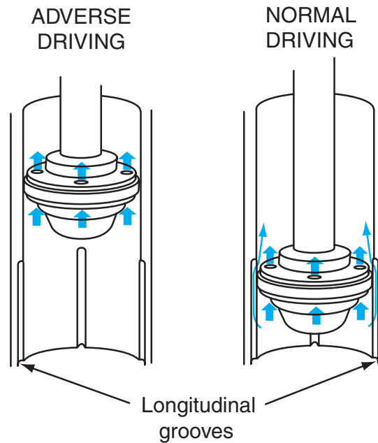
Figure 5-13 Travel-sensitive strut.
