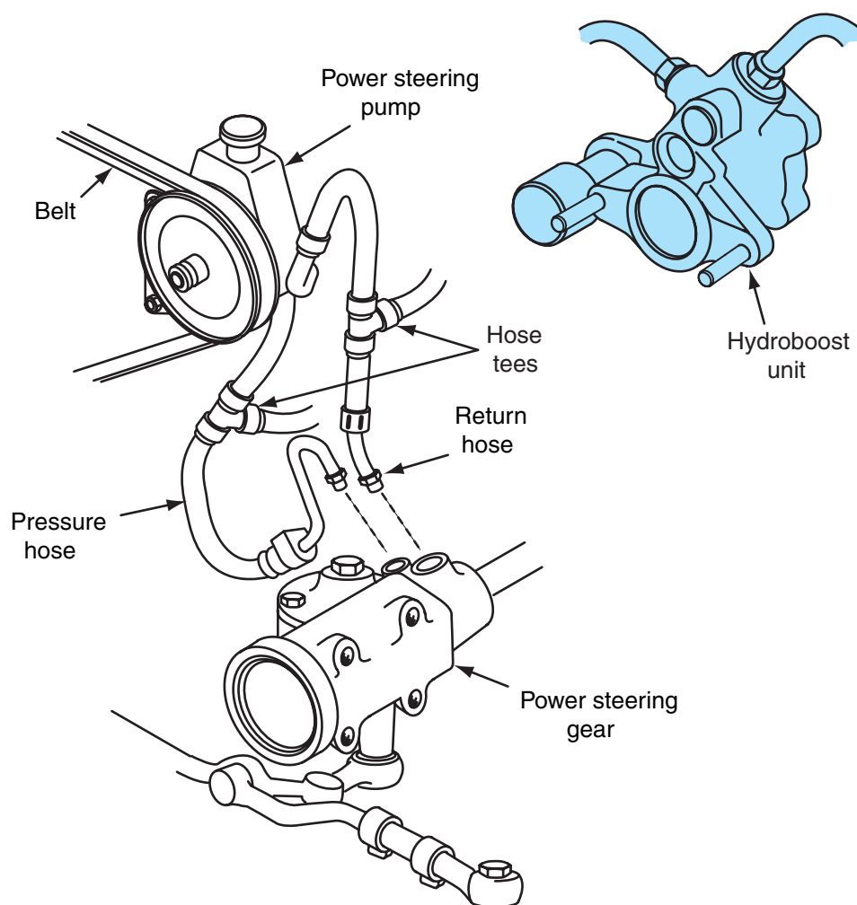
Figure 10-8 Hydroboost power-assisted steering and brake system.
