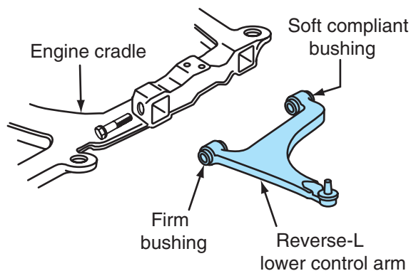
Figure 6-28 Reverse-L front suspension system with firm, front lower control arm bushing and more compliant rear, lower control arm bushing.
