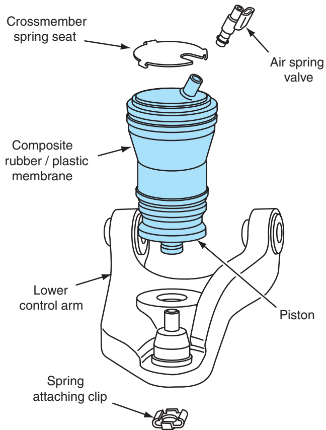
Figure 8-8 Front air spring.
