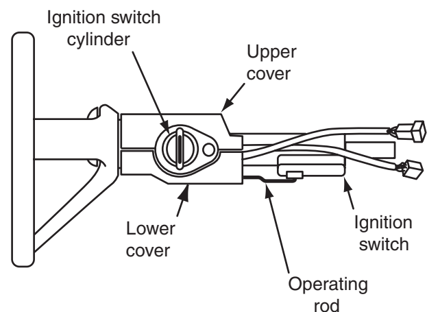
Figure 9-7 Ignition switch and ignition switch cylinder mounted in steering column.
