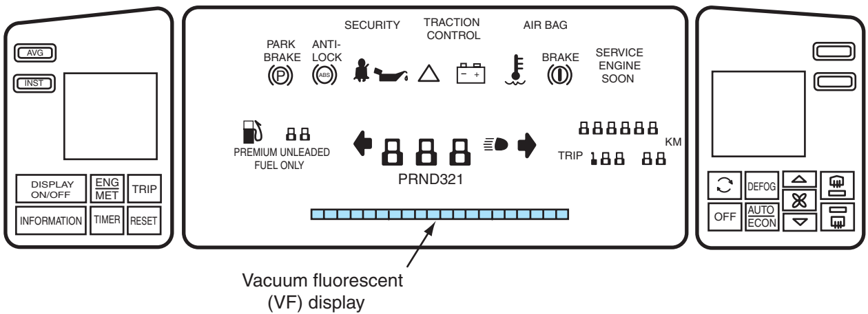
Figure 8-27 Digital instrument panel cluster.
