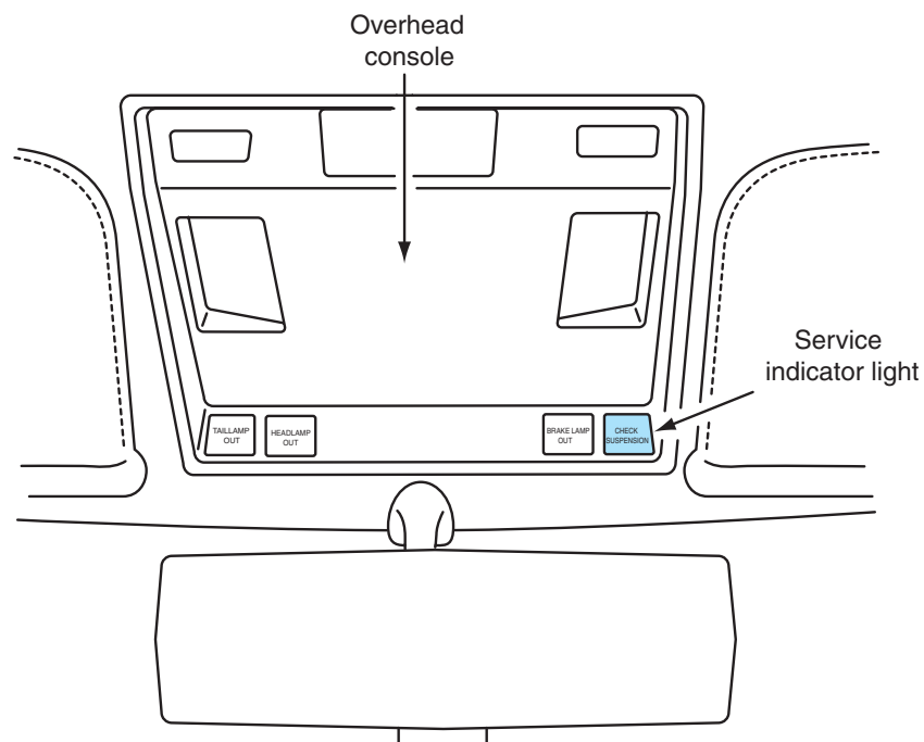
Figure 8-24 Air suspension warning light.
