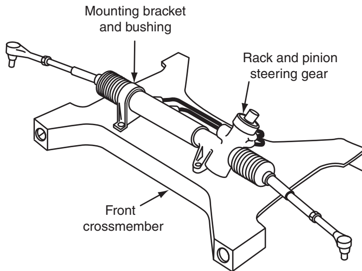
Figure 9-30 Rack and pinion steering gear mounting on front crossmember.
