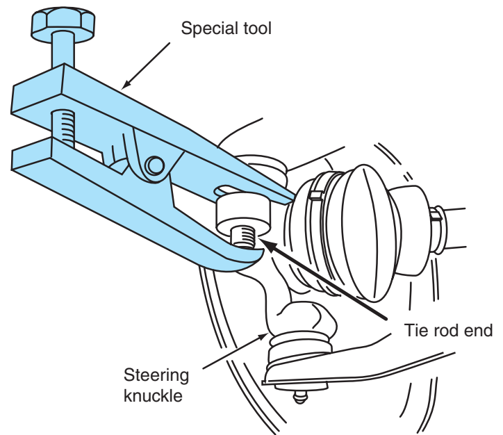
Figure 2-13 Tie rod end and ball joint puller.
