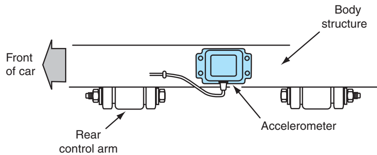
Figure 8-33 Rear accelerometer position.
