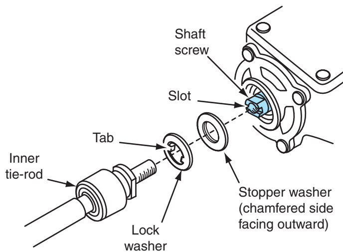
Figure 13-19 Installing the inner tie-rod end on the shaft screw.
