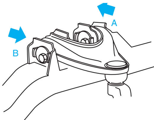
Figure 16-15 To decrease the positive caster move the front of the upper control arm (A) inboard and move the rear of the upper control arm (B) outboard.
