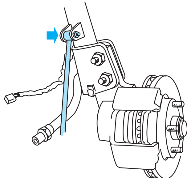
Figure 7-12 Removing stabilizer bar from the rear strut.
