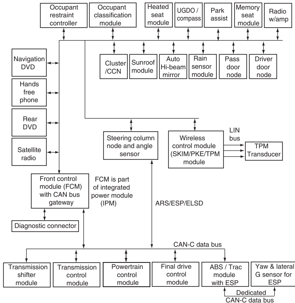
Figure 8-48 Data link systems on a current SUV.
