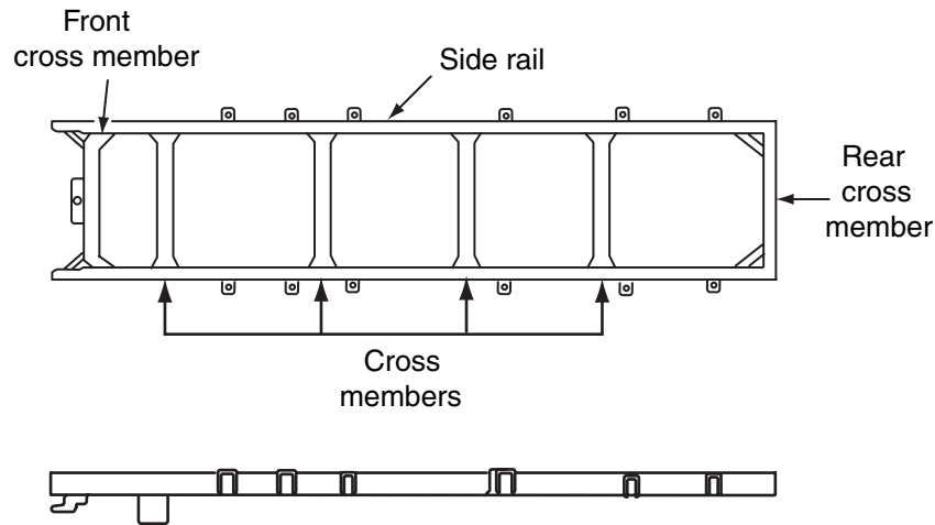
Figure 14-2 Ladder-type frame.
