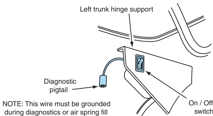
Figure 8-19 On/Off switch.
