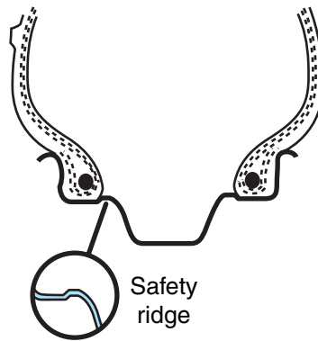
Figure 4-33 Wheel rim with drop center and safety ridges.
