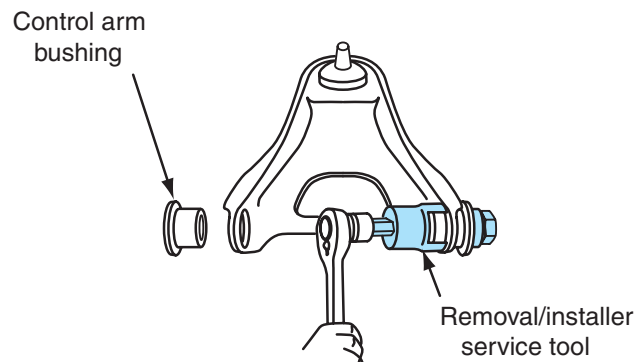
Figure 2-14 Control arm bushing removal and replacement tools.
