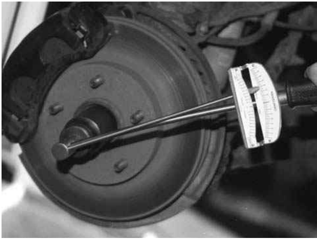
Figure 3-25 Hub nut torquing.
