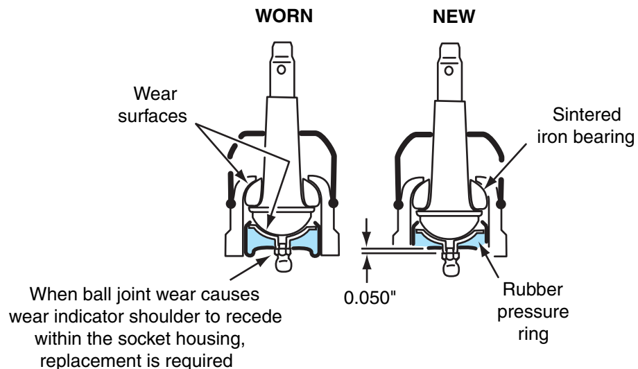
Figure 6-12 Ball joint wear indicator.
