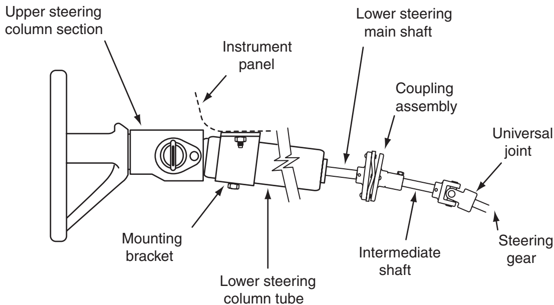
Figure 9-12 Tilt steering column with universal joint, intermediate shaft, combination switch, and steering wheel.
