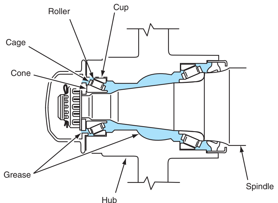
Figure 3-8 Wheel bearing lubrication.
