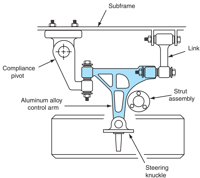
Figure 6-40 Double wishbone front suspension.
