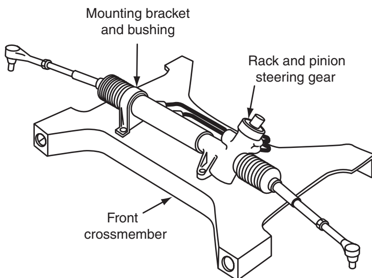
Figure 10-3 Power steering gear mounting.
