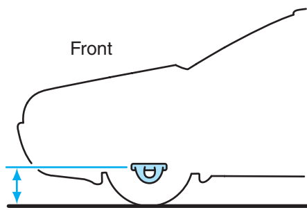
Figure 6-1 Curb riding height measurement, front suspension.
