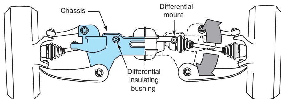
Figure 7-36 Differential to frame mounting bushings.
