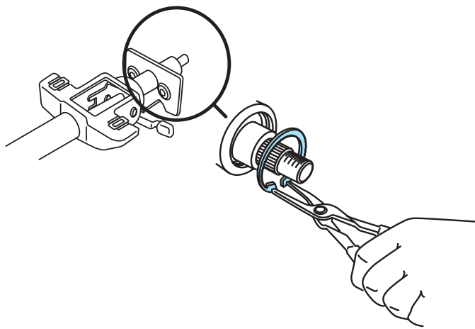
Figure 9-37 Installing snapping in upper column tube.
