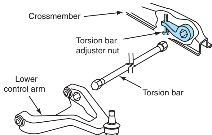
Figure 6-4 Curb riding height adjustment, torsion bar front suspension.
