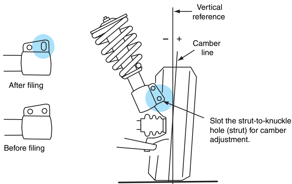
Figure 16-47 Elongating the lower strut bolt hole provides camber adjustment.
