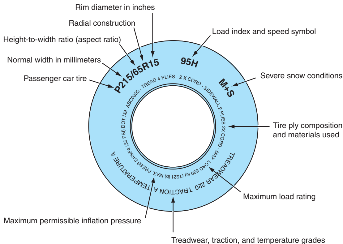
Figure 4-8 Tire sidewall information.
