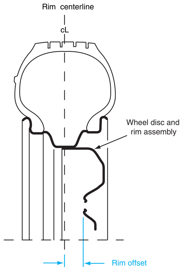
Figure 4-30 Wheel rim design.
