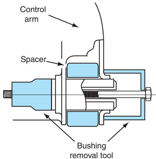
Figure 6-40 Removing the front control arm bushing.
