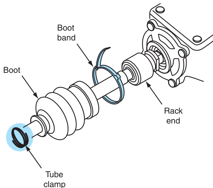
Figure 13-14 Removing boot bands and clamps from the inner tie-rod end.
