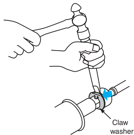
Figure 12-26 Removing claw washers from inner tie-rod sockets.
