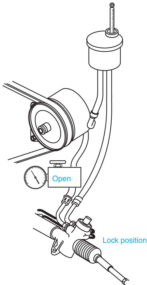
Figure 10-17 Power steering pump pressure test with the front wheels turned fully in one direction.
