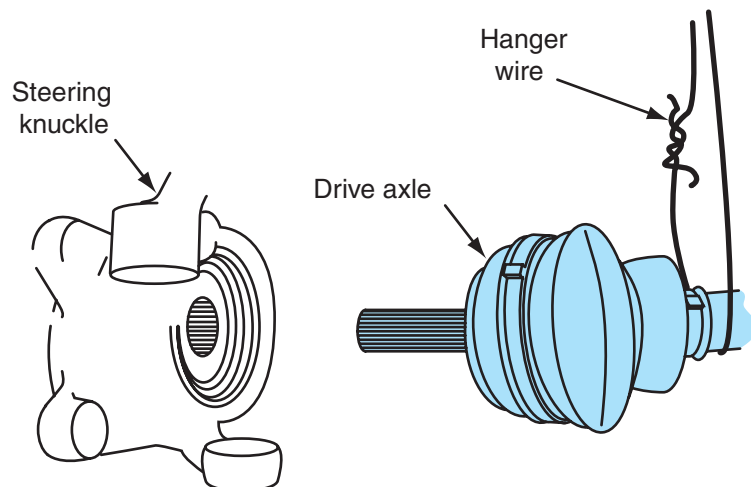
Figure 6-34 Securing the drive axle with a piece of wire.
