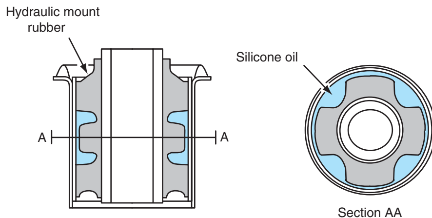
Figure 7-38 Hydraulic mount design.
