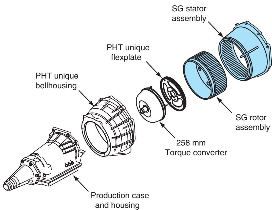
Figure 10-24 Starter/generator.
