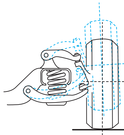
Figure 6-19 Short-and-long arm front suspension system.
