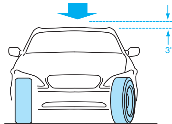
Figure 15-41 If the toe change on one front wheel remains at the original setting while the toe on the opposite wheel toes in or out during wheel jounce, unequal steering linkage height is indicated.
