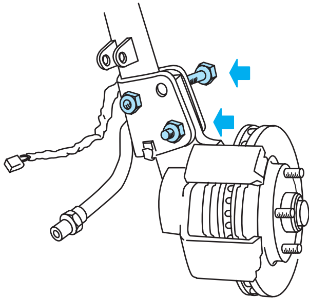
Figure 7-13 Loosening strut-to-rear spindle bolts.
