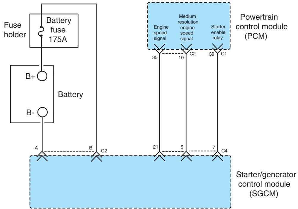
Figure 10-25 Engine speed inputs from the PCM to the SGCM.
