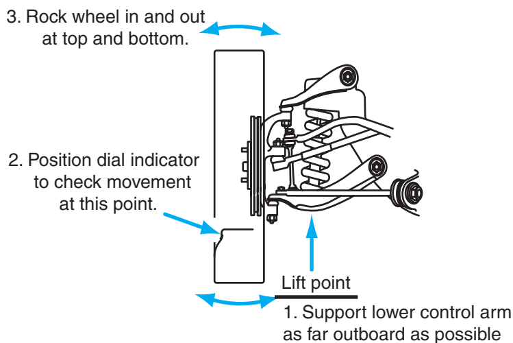
Figure 6-12 Measuring radial ball joint movement.
