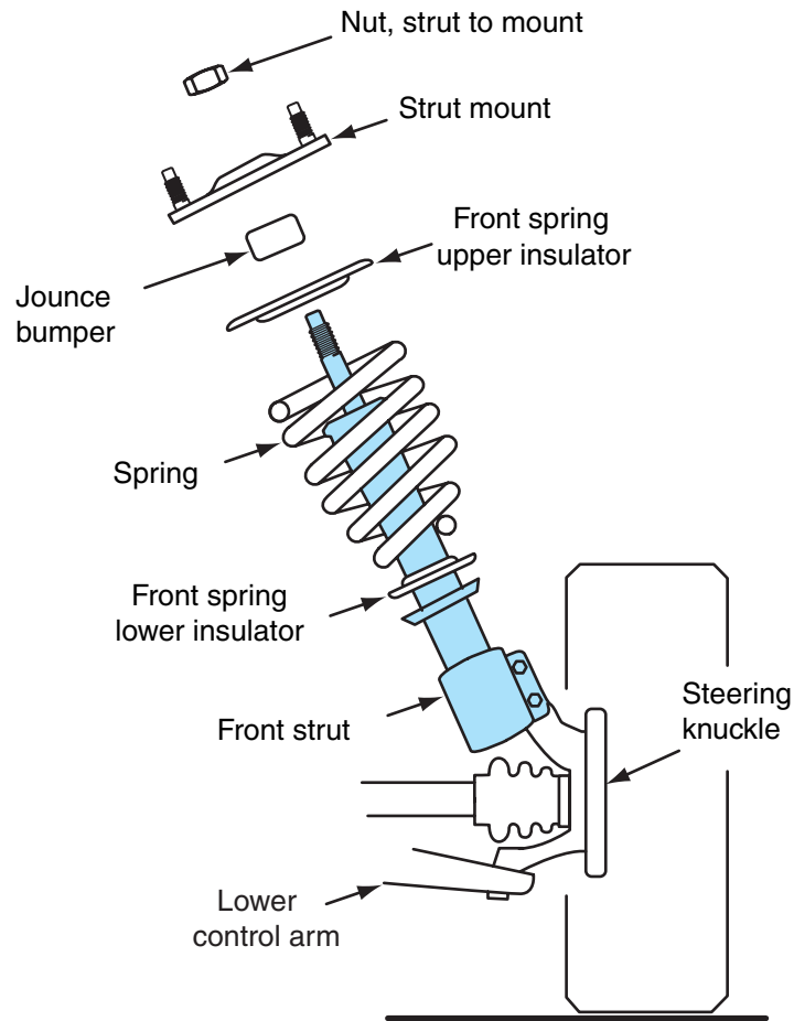
Figure 6-35 Complete MacPherson strut front suspension system.
