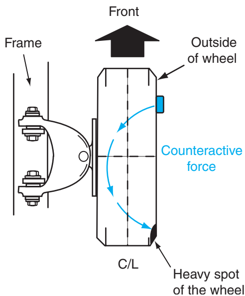
Figure 4-27 Dynamic wheel balance procedure with heavy spot on the outside edge of the tread.
