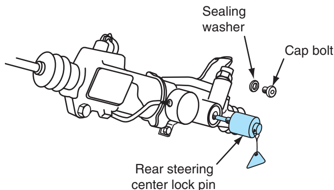
Figure 13-10 Removing the cap bolt and washer, and installing the rear steering center lock pin.
