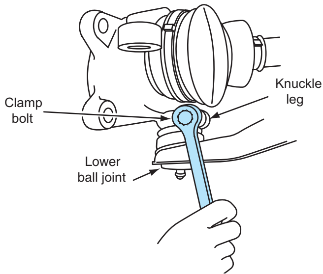
Figure 3-13 Removal of ball joint to steering knuckle clamp bolt.
