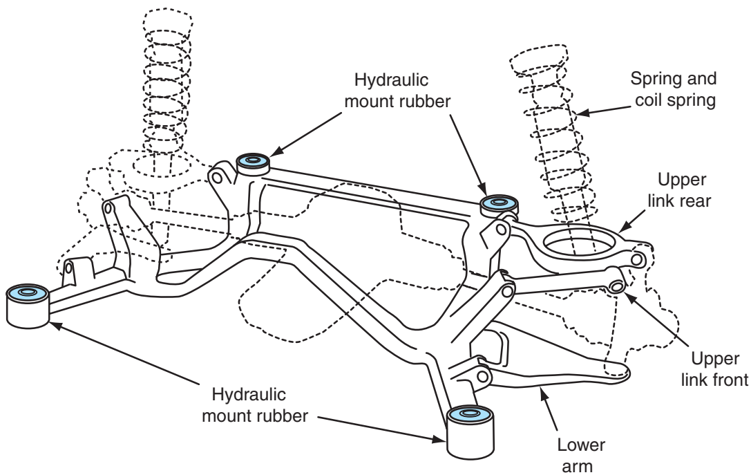
Figure 7-37 Multilink independent rear suspension system with hydraulic mounts.
