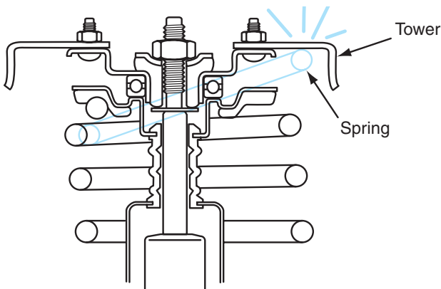
Figure 5-4 Coil spring to upper mount interference.
