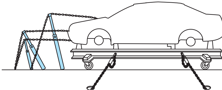
Figure 14-22 Multipull unitized body straightening system.
