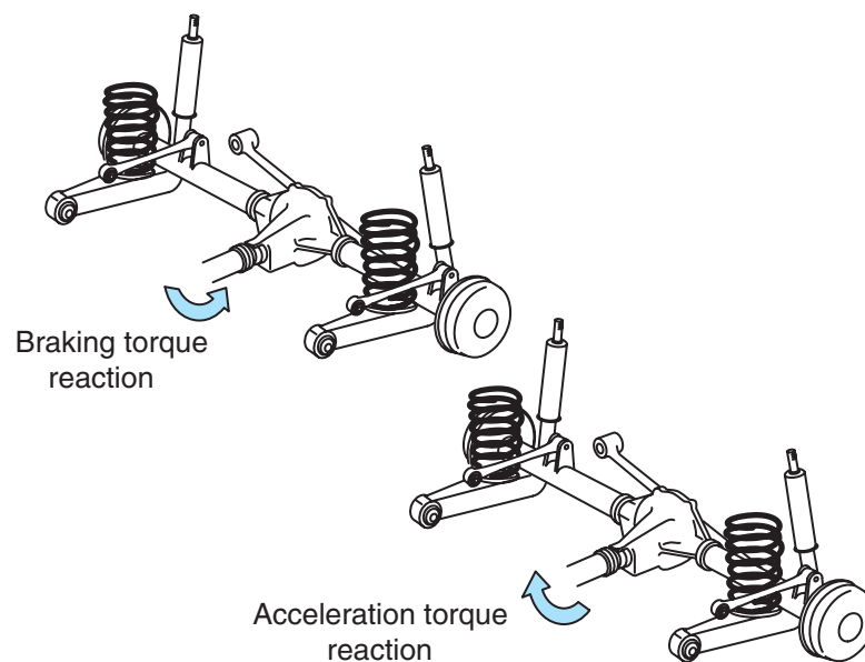
Figure 7-10 Rear axle torque action during acceleration and deceleration.
