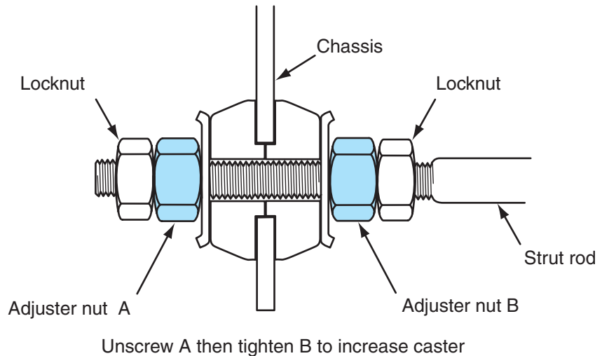
Figure 16-28 Strut rod nuts can be adjusted to lengthen or shorten the strut rod to adjust caster.
