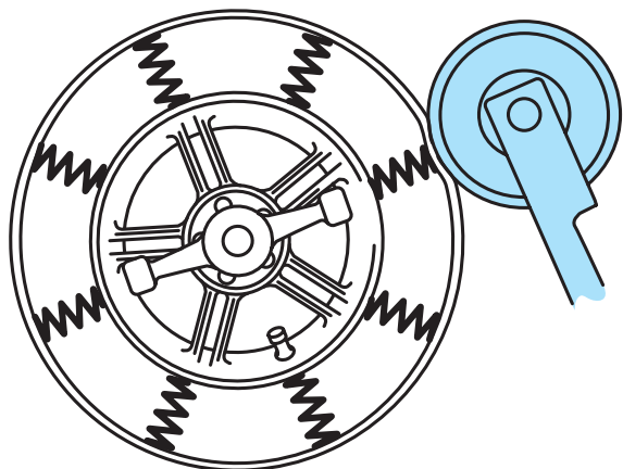
Figure 4-32 The roller on the balancer senses force variation in the tire.
