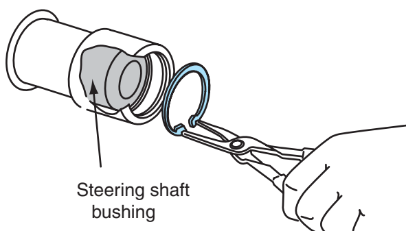
Figure 9-25 Removing snapping above steering shaft bushing.
