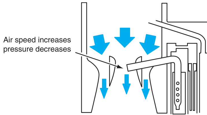
Figure 2-26 A venturi increases air flow speed and produces a vacuum.
