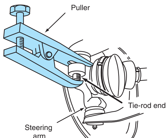
Figure 13-8 Removing a tie-rod end with a special tool.
