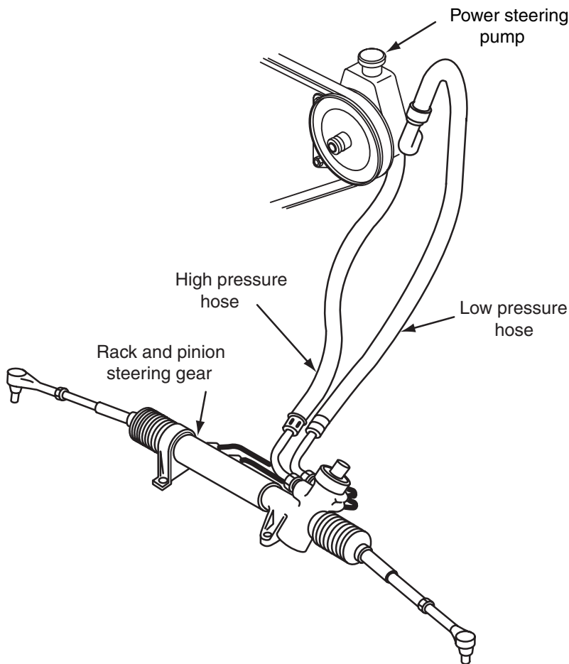
Figure 12-5 Power rack and pinion steering gear with connecting hoses and lines.
