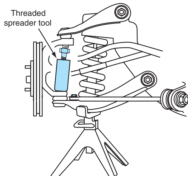
Figure 6-22 Removing the upper ball joint from the steering knuckle.
