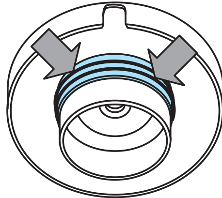
Figure 8-26 O-ring seals on the upper spring mount.
