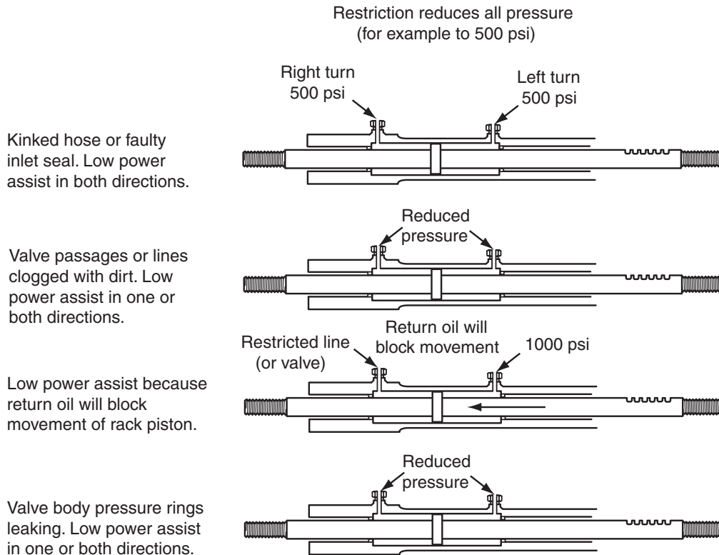
Figure 12-22 Effect of worn rotary valve rings and seals or restricted lines or hoses on steering effort.
