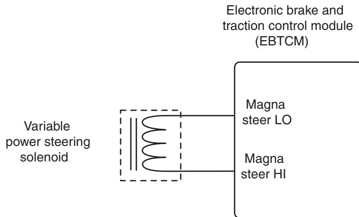
Figure 12-21 Wiring connections between the Magnasteer actuator solenoid and the EBTCM.
