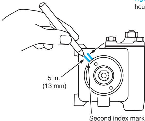
Figure 11-4 Measuring 0.50 in. (13 mm) counterclockwise from the index mark on the steering gear housing.
