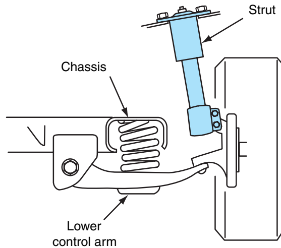
Figure 5-9 Rear suspension system with coil springs mounted separately from the struts.
