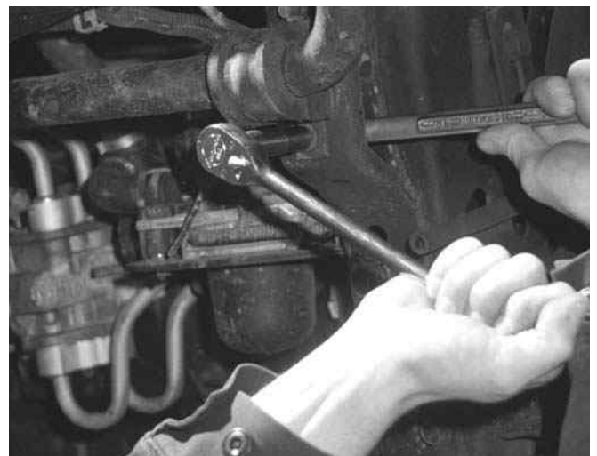
Figure 12-8 Removing stabilizer bar mounting bolts.
