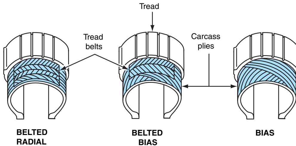
Figure 4-3 Three types of tire construction: bias-ply, belted bias-ply, and belted radial-ply.
