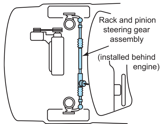
Figure 2-21 Steering gear, linkages, and arms connected to the front wheels.
