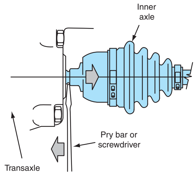
Figure 3-14 Removal of inner axle joint from transaxle.
