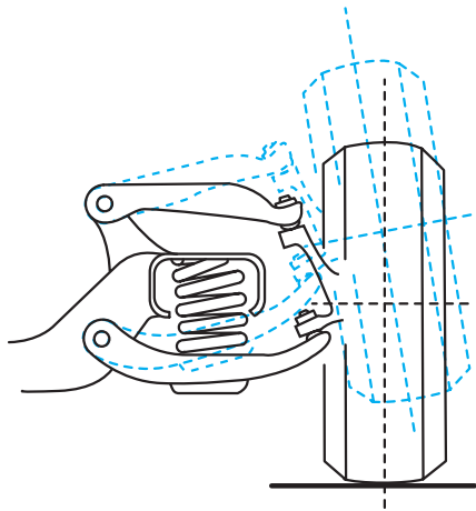
Figure 6-18 Early front suspension system with equal length upper and lower control arms.
