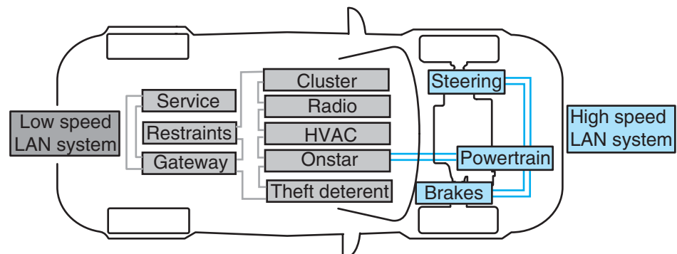
Figure 8-47 Low-speed LAN and high-speed LAN data link systems.
