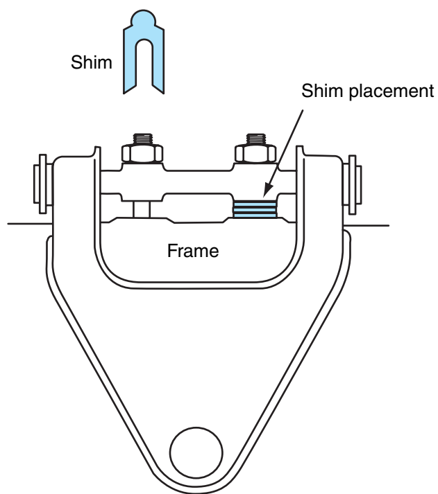
Figure 16-3 Shim-type camber adjustment between upper control arm mounting and the inside of the frame.
