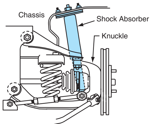
Figure 7-35 Shock absorber mounting.
