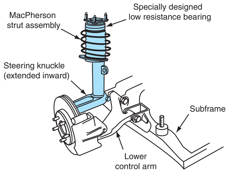
Figure 6-36 MacPherson strut front suspension system on Jaguar X-type car.
