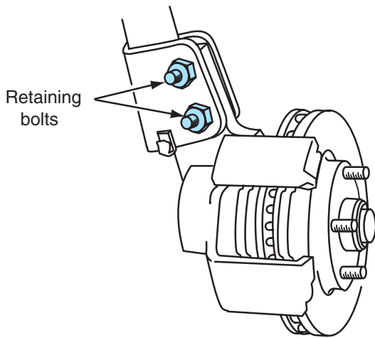
Figure 5-8 Removing strut-to-steering knuckle retaining bolts.
