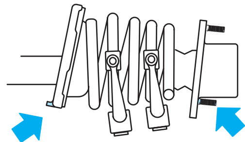
Figure 5-21 Aligning lowest bolt on upper strut mount with tab on lower spring seat.
