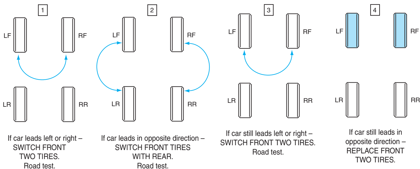
Figure 4-2 Tire conicity diagnosis.
