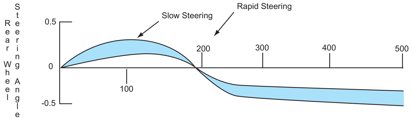
Figure 13-5 Rear steering angle in relation to vehicle speed and steering wheel rotation.
