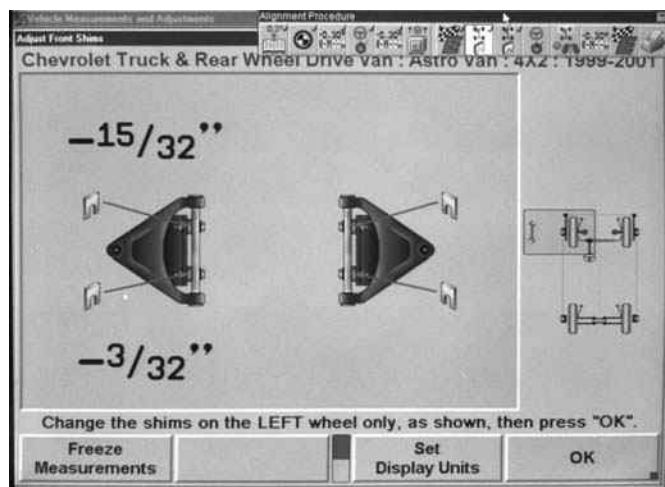
Figure 15-39 Control arm movement monitor indicates the required shim thickness to provide specified camber and caster.
