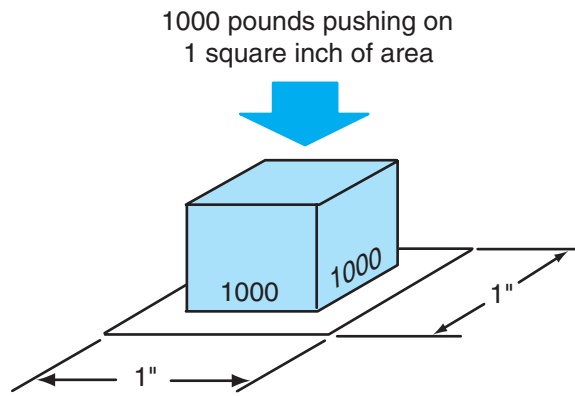
Figure 2-20 Hydraulic pressure is applied equally to every square inch in a container.
