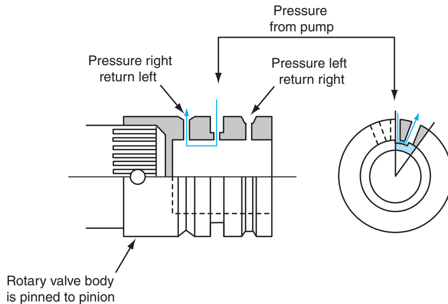
Figure 12-6 Spool valve movement inside the rotary valve.
