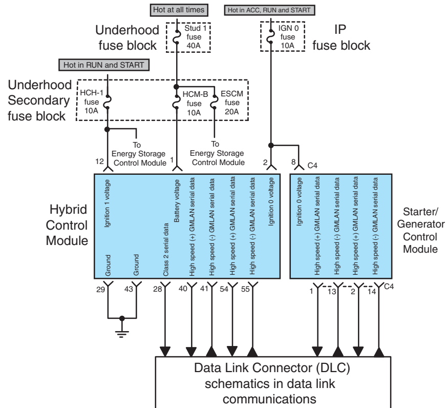
Figure 10-30 Ignition inputs to the HCM.
