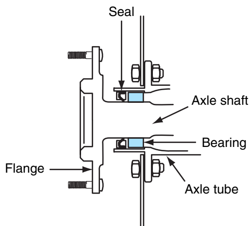
Figure 3-22 Rear-axle bearing, rear-wheel-drive car.
