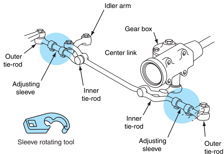
Figure 16-39 Rotating tie-rod sleeves to adjust front wheel toe.
