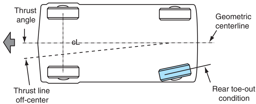
Figure 15-3 Excessive toe-out on the left rear wheel moves the thrust line to the left of the geometric centerline.
