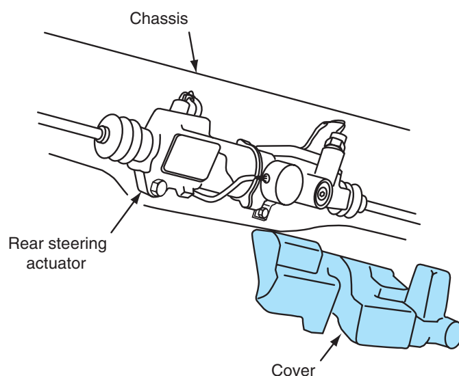
Figure 13-9 Removing the rear steering actuator cover.
