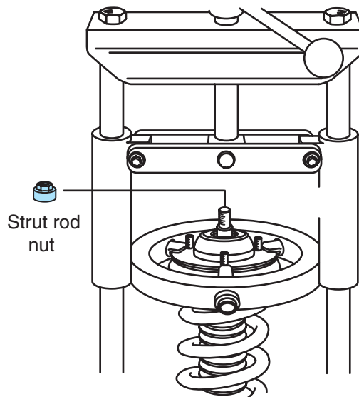
Figure 7-17 After the compressing tool is operated to remove all the spring tension, remove the strut rod nut.
