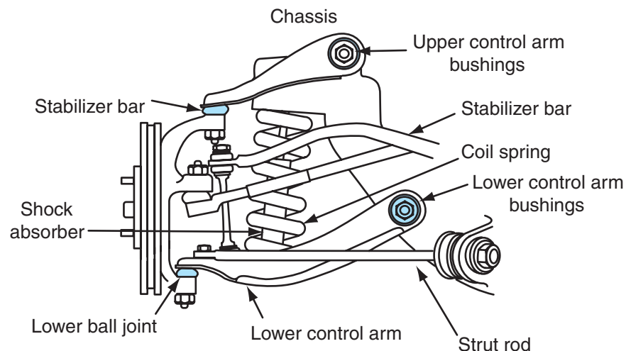
Figure 1-5 Typical short-and-long arm (SLA) front suspension system.
