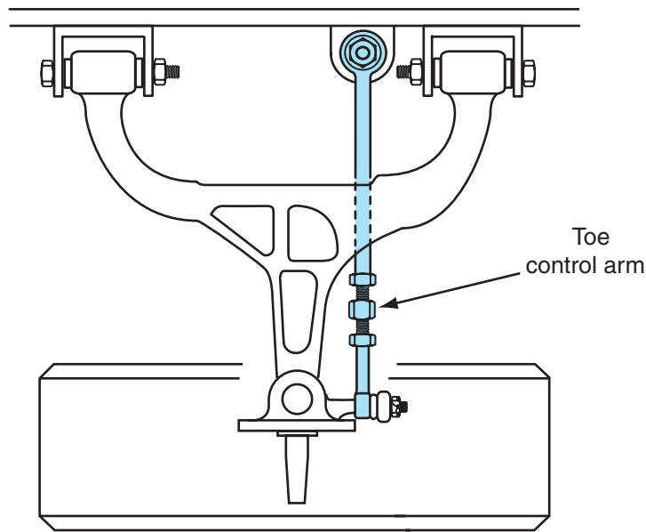
Figure 7-45 Double wishbone rear suspension and toe control arm.
