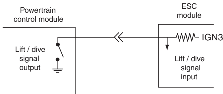
Figure 8-36 The lift-dive signal is sent from the powertrain control module (PCM) to the ESC module.
