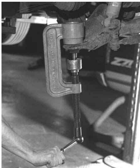
Figure 7-25 Removing the ball joint from the lower control arm.
