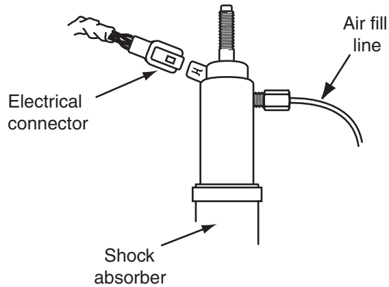
Figure 8-26 Electrical and air fill line connections to the shock absorber.
