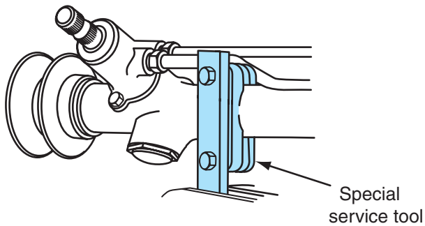
Figure 12-23 Steering gear holding tool.
