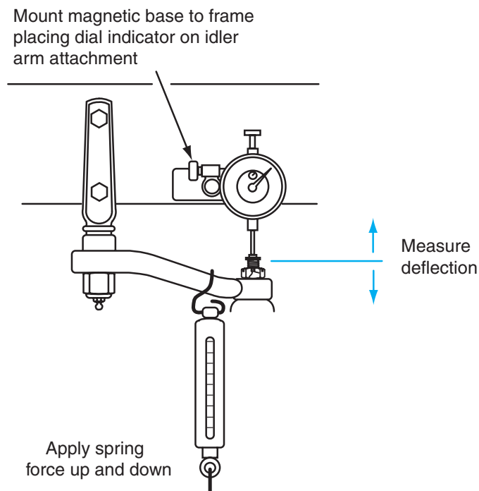
Figure 9-50 Measuring idler arm vertical movement.
