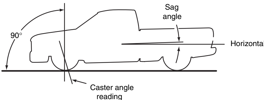
Figure 6-61 Effects of front spring sag on caster angle.
