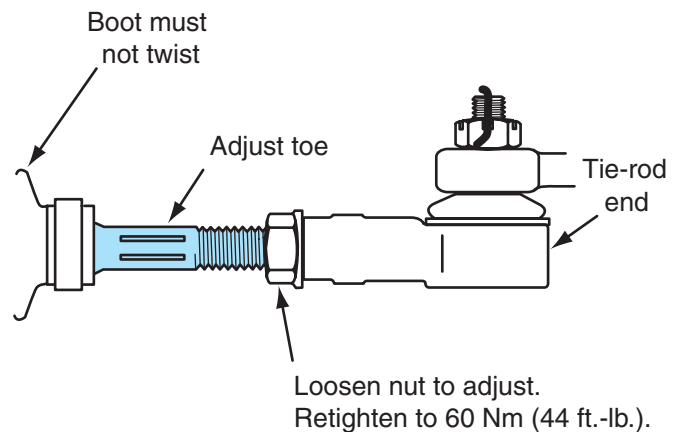
Figure 16-41 Rotating tie-rod to adjust the toe on a rack and pinion steering gear.
