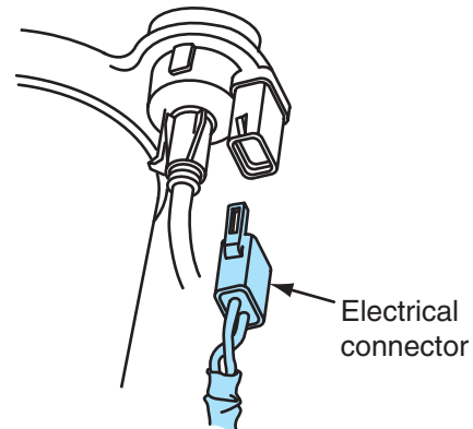
Figure 8-18 Disconnecting the electrical connector from the air spring solenoid valve.
