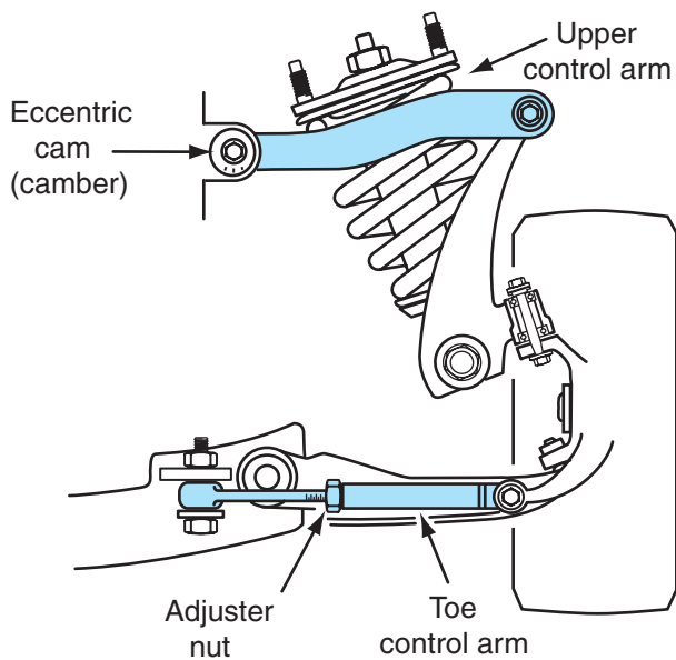
Figure 7-46 Rear suspension camber and toe adjustments.
