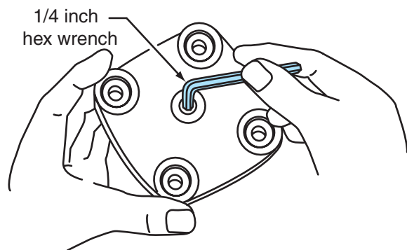
Figure 11-10 Removing steering gear side cover.
