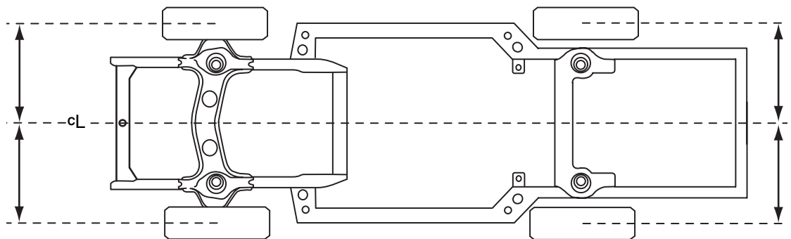
Figure 14-5 Front and rear wheels must be the same distance from the vehicle centerline to provide proper tracking.
