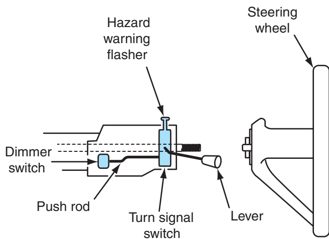
Figure 9-8 Turn signal switch, hazard warning switch, dimmer switch, and wipe/wash switch mounted in steering column.
