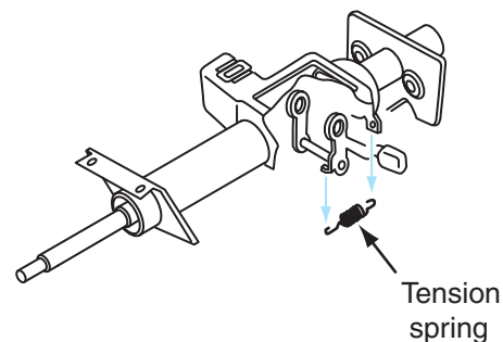
Figure 9-18 Removing tension spring.
