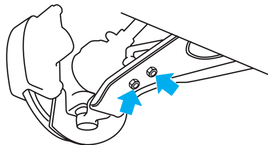
Figure 6-31 Removing stabilizer brackets from the lower control arm.
