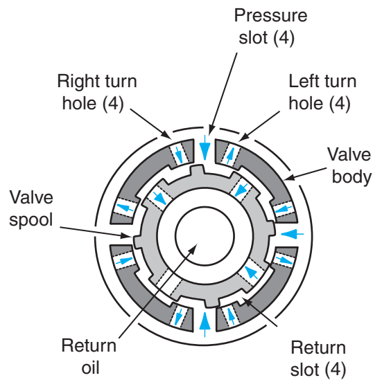
Figure 11-7 Spool valve position during a left turn.
