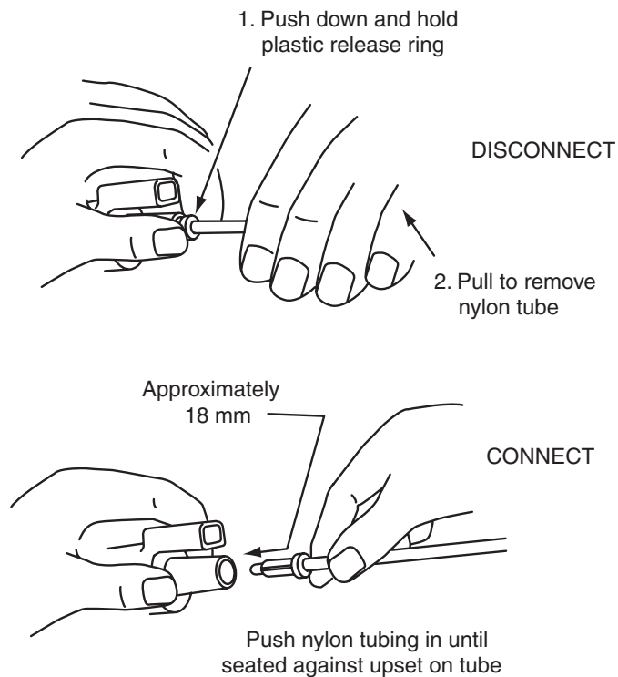
Figure 8-13 Air line removed from the air spring valve or compressor outlets.
