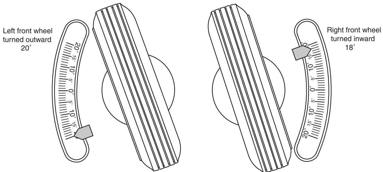
Figure 15-23 Turning angle screen.
