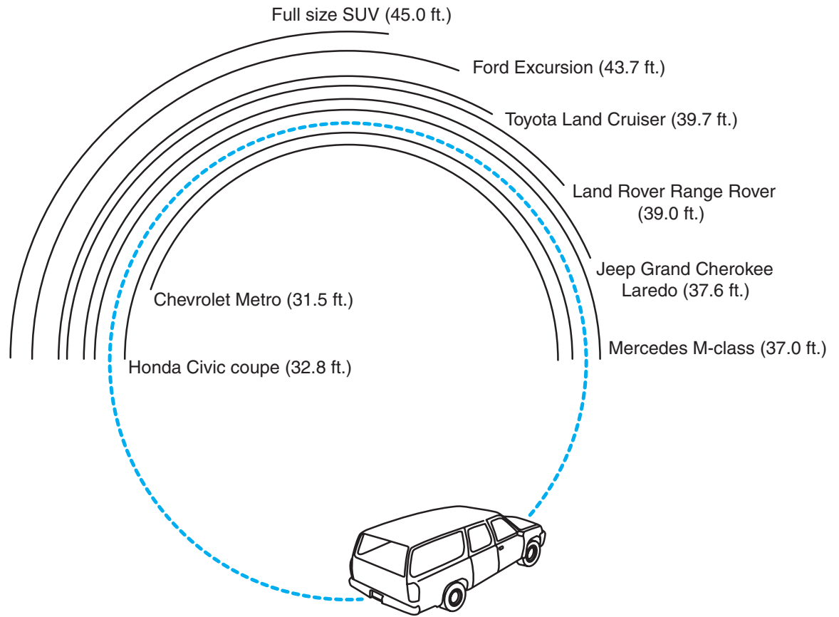
Figure 13-17 Turning circle diameter, four-wheel steering system.
