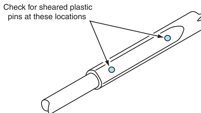
Figure 9-5 Injection plastic in collapsible lower steering shaft.
