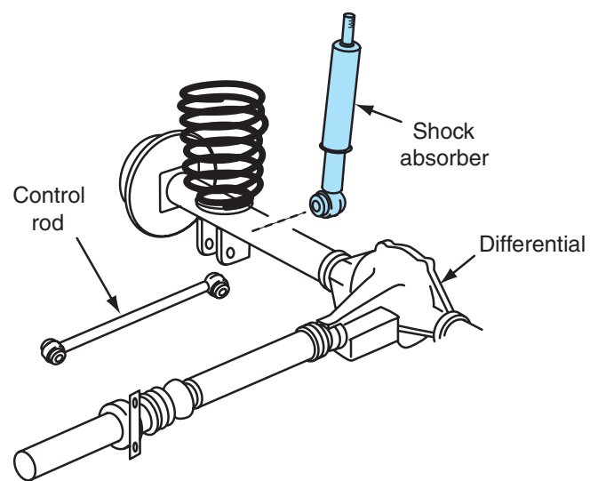
Figure 7-13 Rear suspension system with coil springs and shock absorbers mounted separately.
