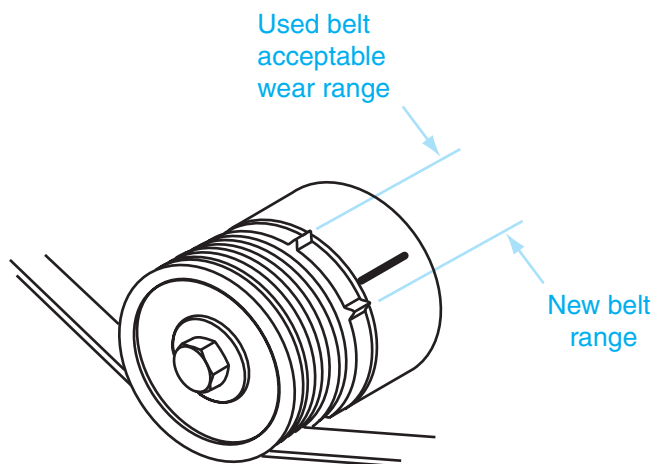
Figure 10-4 Belt tension scale.
