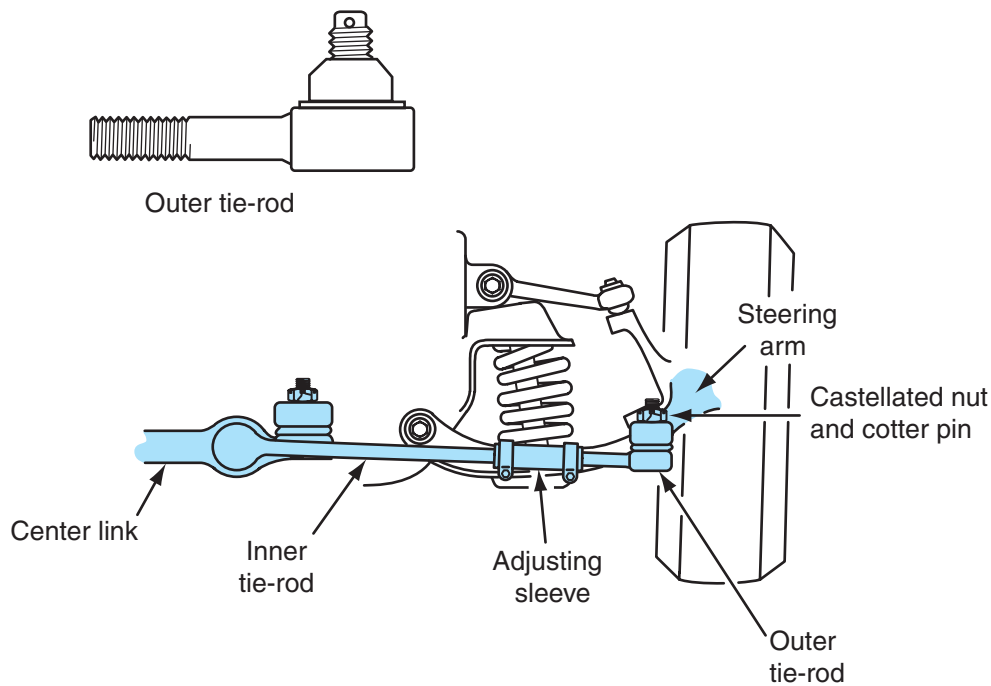
Figure 9-19 Tie-rod design.
