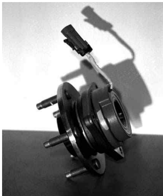
Figure 8-52 Wheel speed sensor.
