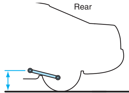
Figure 6-2 Curb riding height measurement, rear suspension.
