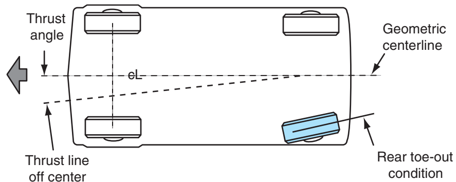
Figure 1-33 Excessive toe-out on the left rear wheel moves the thrust line to the left of the geometric centerline.
