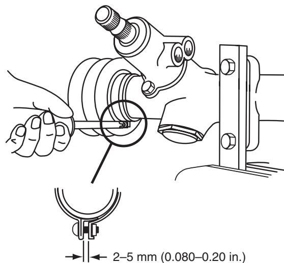
Figure 12-38 Minimum clearance between boot clamp ends.
