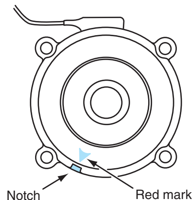
Figure 9-7 Centering clock spring electrical connector.
