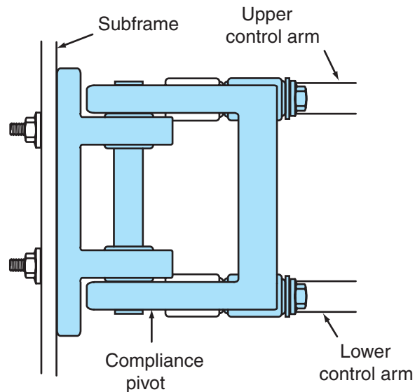
Figure 6-41 Compliance pivot on double wishbone front suspension.
