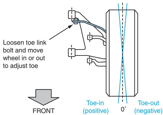
Figure 16-59 Loosening toe link bolt to adjust rear wheel toe.
