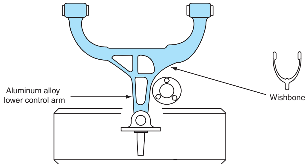
Figure 7-43 Double wishbone rear suspension.
