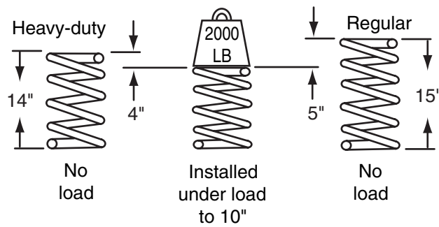
Figure 6-2 Comparison of heavy-duty and regular-duty coil springs.
