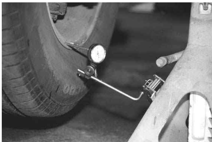
Figure 6-11 Dial indicator installed to measure radial ball joint movement.
