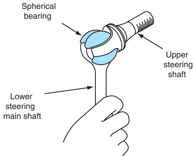
Figure 9-11 Spherical bearing acts as a pivot between the upper steering shaft and the lower steering main shaft in some tilt steering columns.
