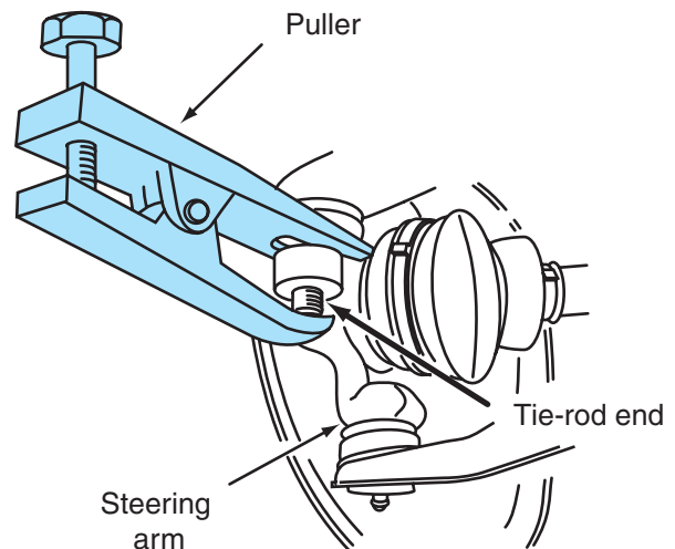
Figure 12-6 Removing outer tie-rod ends.
