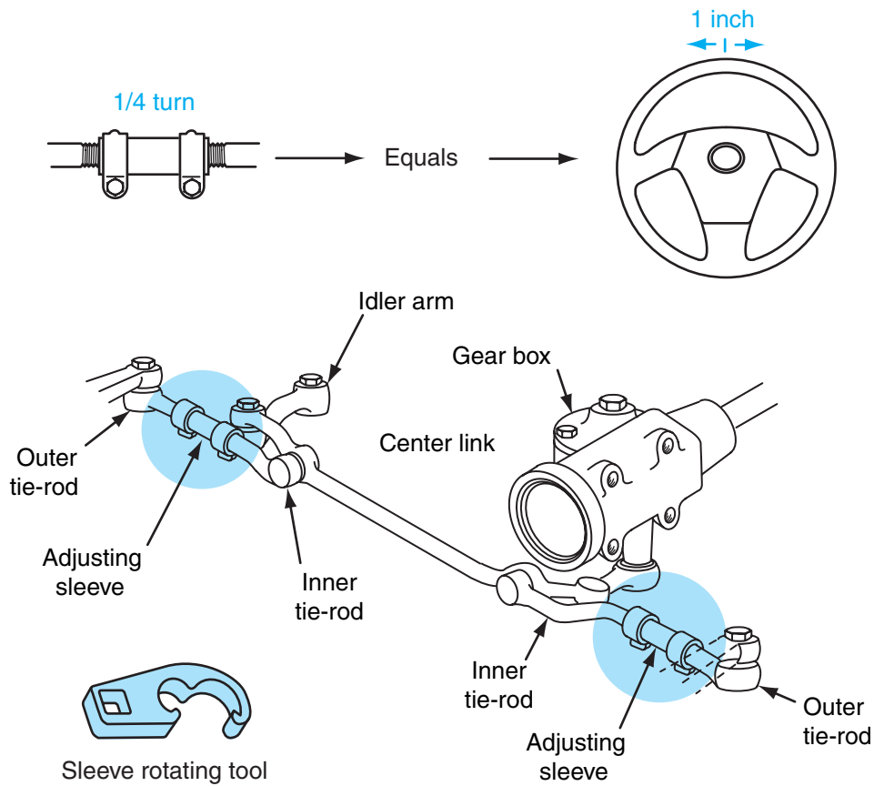
Figure 16-44 Rotating tie-rod sleeves to center steering wheel.
