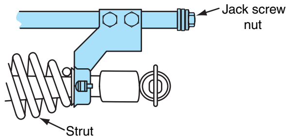
Figure 6-24 Lower end of spring compressing tool.
