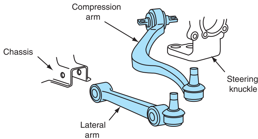
Figure 6-43 Multilink front suspension with lateral and compression lower arms.
