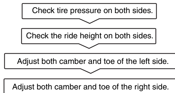
Figure 16-2 Rear wheel alignment adjustment procedure.
