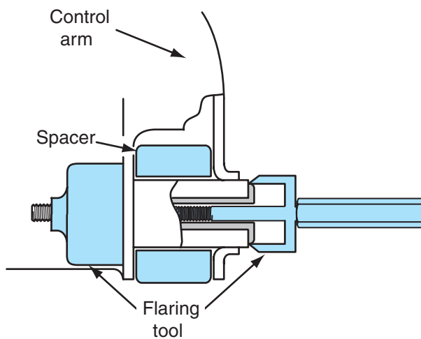
Figure 6-42 Flaring the front control arm bushing.
