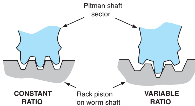
Figure 11-3 Constant and variable ratio steering gears.
