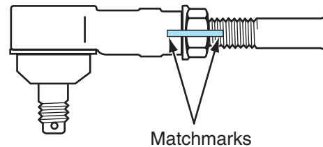
Figure 12-24 Marking outer tie-rod ends, jam nuts, and tie-rods prior to outer tie-rod end removal.
