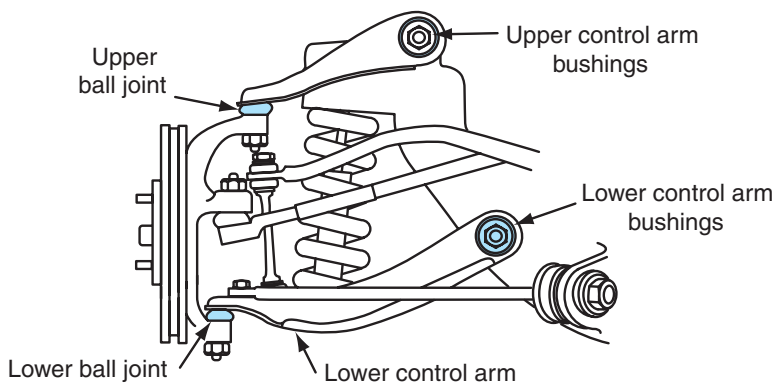
Figure 6-20 Ball joints and complete short-and-long arm front suspension system.
