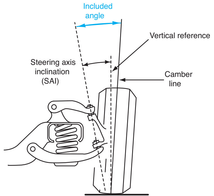
Figure 16-2 Steering axis inclination and included angle.
