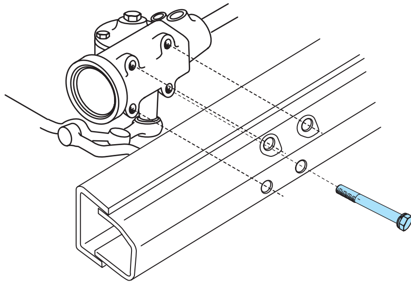
Figure 11-1 Removing steering gear from the chassis.
