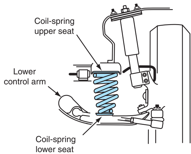
Figure 7-27 Coil-spring mounting.
