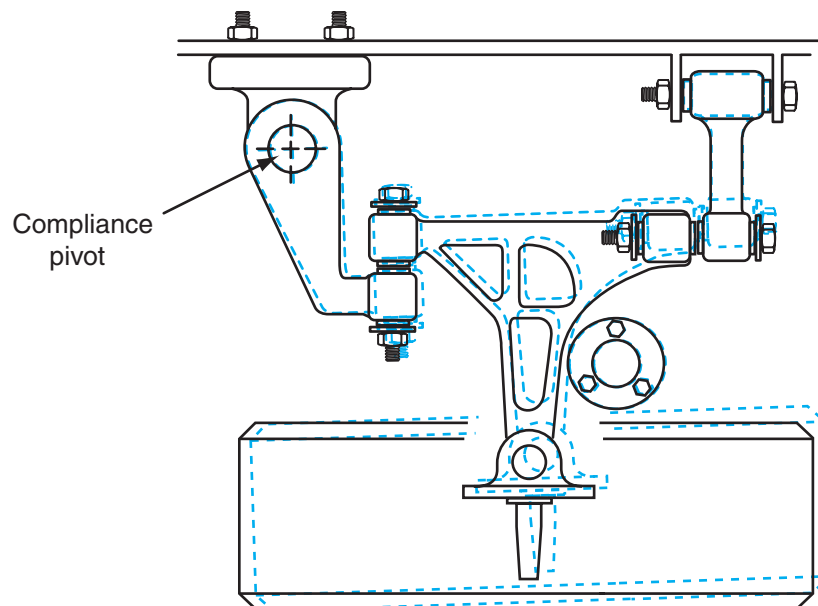
Figure 6-42 Compliance pivot action.
