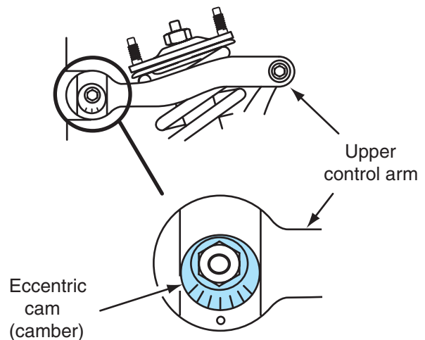
Figure 7-47 Eccentric cam for camber adjustment on rear upper control arm bolt.
