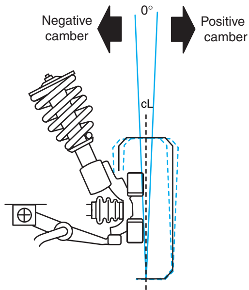
Figure 6-62 Positive and negative camber.
