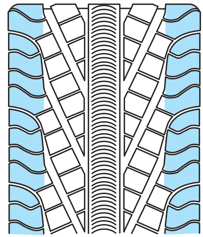
Figure 4-6 Reinforced tread shoulders improve tread gripping quality while cornering.
