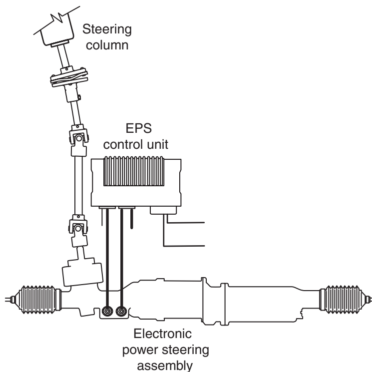
Figure 12-24 Electronic power steering (EPS) control unit and steering gear.
