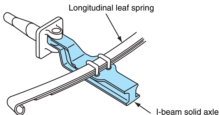
Figure 6-17 I-beam front suspension with longitudinally mounted leaf springs.
