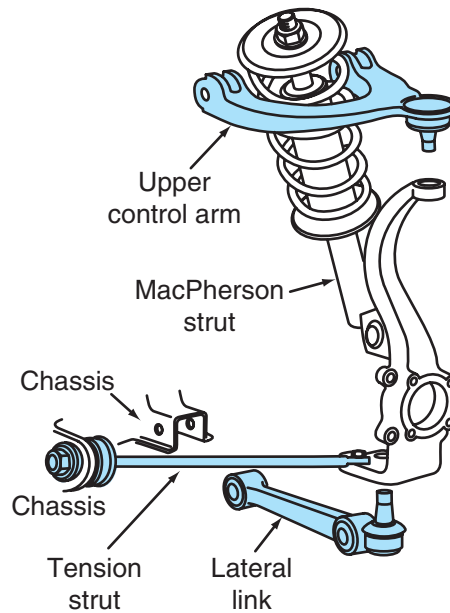
Figure 6-29 Front suspension system with lateral link and tension strut in place of lower control arm.
