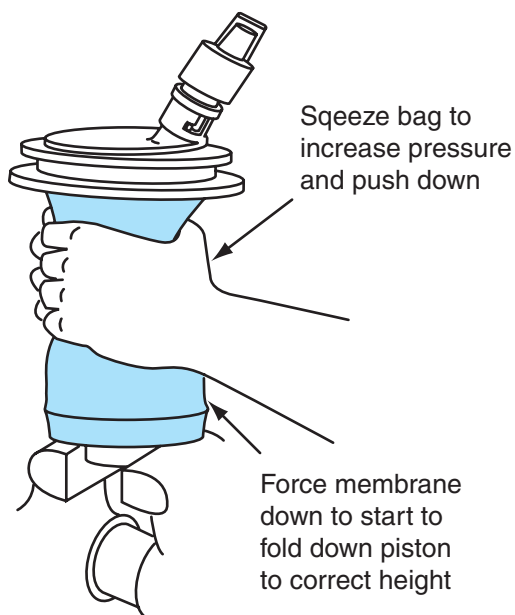
Figure 8-5 Air spring folding.
