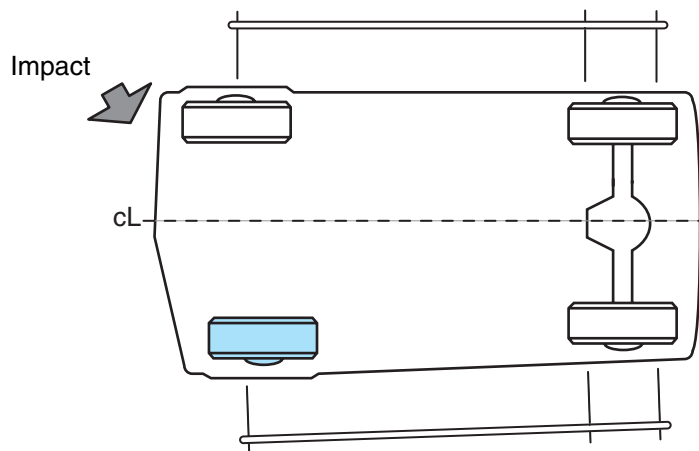
Figure 16-66 Track bar measurement of a left front wheel that is moved rearward to a setback position.
