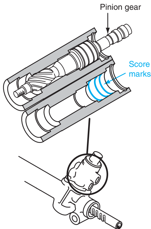
Figure 12-8 Score marks in a rack and pinion steering gear housing.
