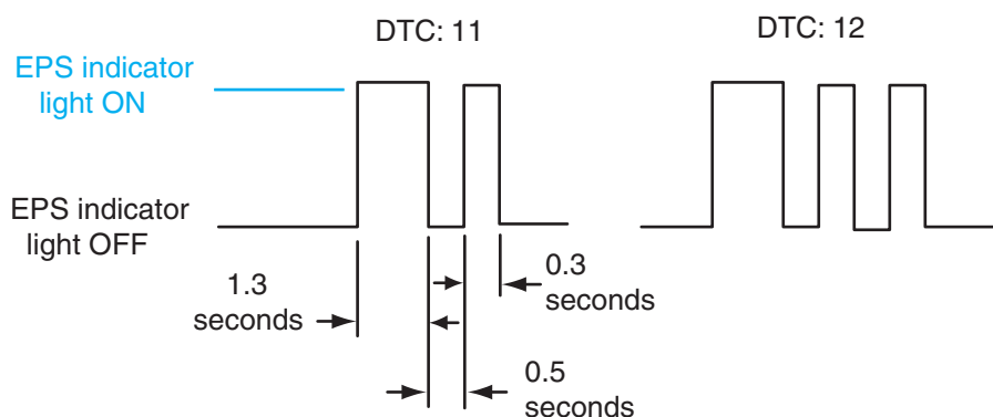
Figure 12-43 DTC 11 is one long flash followed by a short flash, and DTC 12 is one long flash followed by two short flashes.
