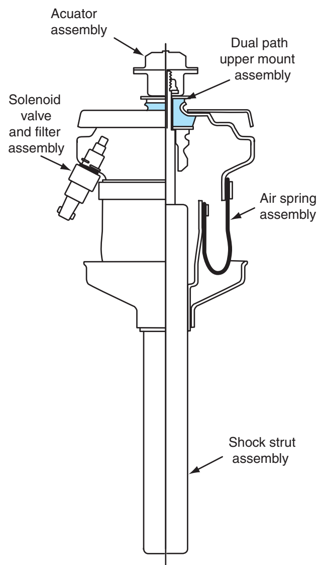
Figure 8-11 Rear air spring and strut assembly.
