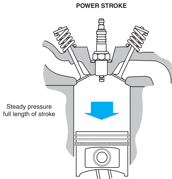
Figure 2-14 Hot, expanding gases push the piston downward and rotate the crankshaft.
