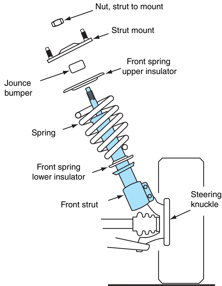
Figure 5-5 Front strut assembly.
