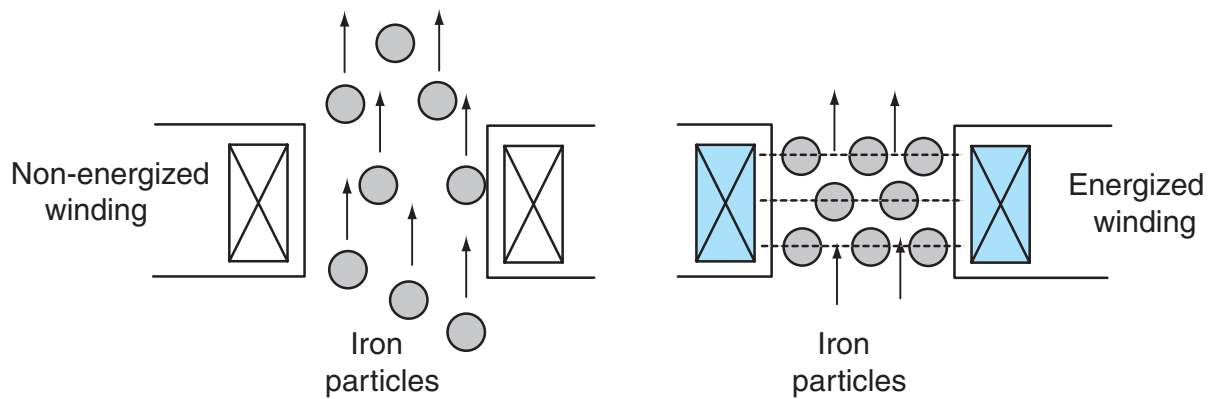
Figure 5-17 Magneto-rheological fluid action in a strut or shock absorber.
