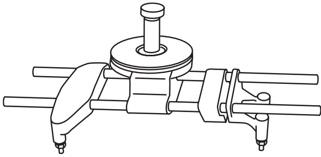
Figure 2-25 Rim clamps.
