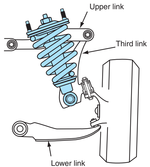
Figure 5-8 Multilink front suspension with knuckle and wheel pivots at the upper link bearing and lower ball joint, and a nonrotating upper strut mount.
