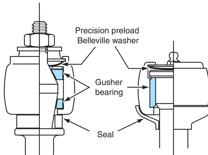
Figure 9-24 Idler arm internal design.
