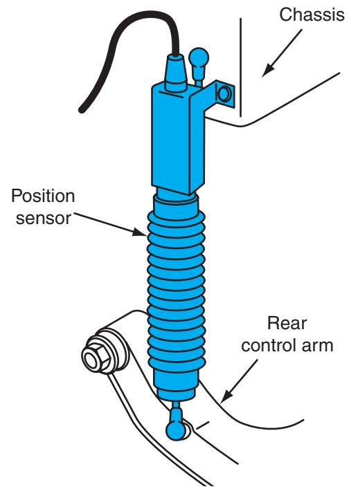
Figure 8-30 Rear wheel position sensor.
