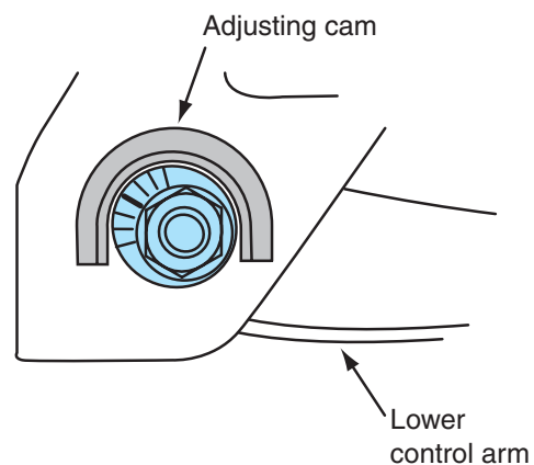
Figure 16-16 Factory-set eccentric cam on lower control arm attaching bolts.
