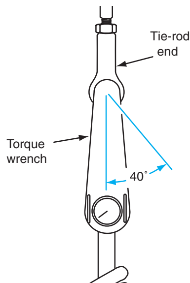
Figure 9-45 Measuring turning torque on a rubber-encapsulated tie-rod end.
