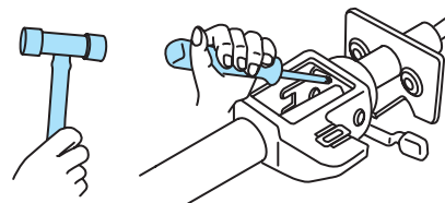
Figure 9-20 Loosening staked parts in upper column tube.
