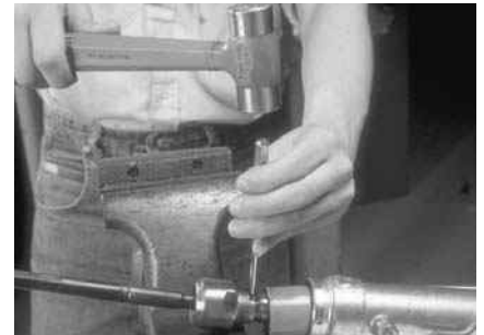
P12-9 Support the inner tie-rod on a vise, and stake both sides of the inner tie-rod joint with a hammer and punch.
