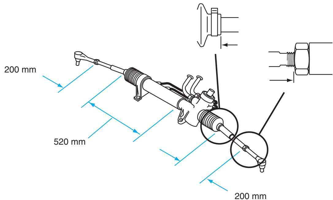
Figure 12-11 Right and left tie-rod position in relation to the steering gear housing prior to installation.
