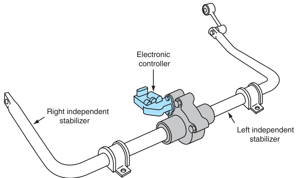
Figure 6-33 Electronically controlled stabilizer bar.
