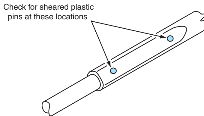
Figure 9-12 Inspecting for sheared injected plastic in steering shaft.
