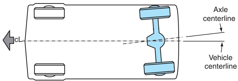
Figure 14-8 Rear axle offset occurs when the rear axle is rotated so the axle centerline and the vehicle centerline are no longer at a 90° angle.
