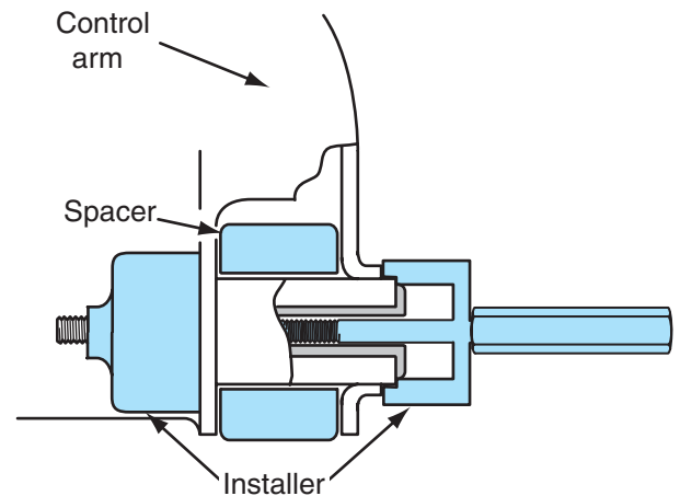
Figure 6-41 Installing the front control arm bushing.
