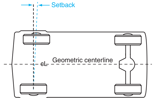
Figure 15-28 Front or rear wheel setback.
