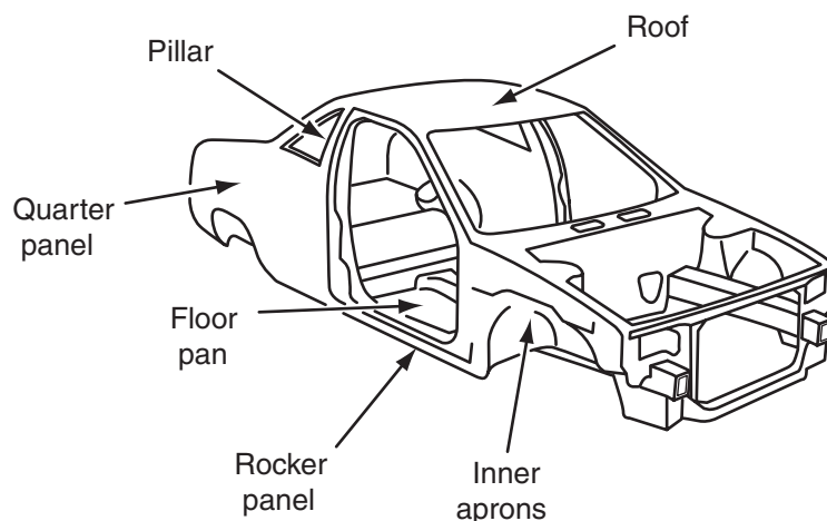
Figure 14-4 Unitized body design.
