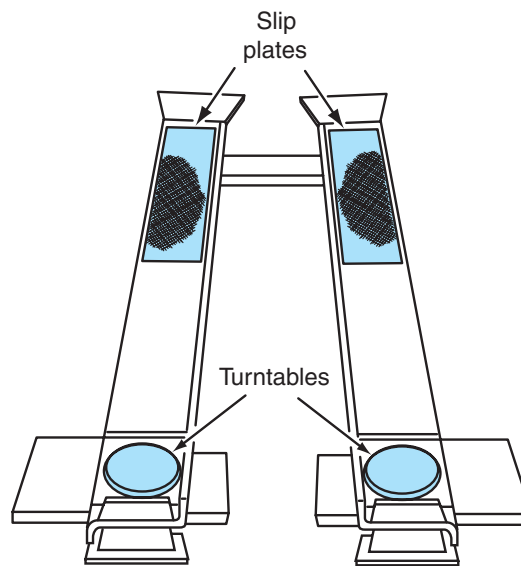
Figure 15-7 Alignment ramp with turntables.
