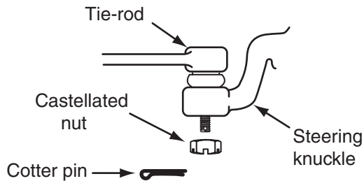
Figure 6-15 Removing the cotter pin and nut from the outer tie-rod end.
