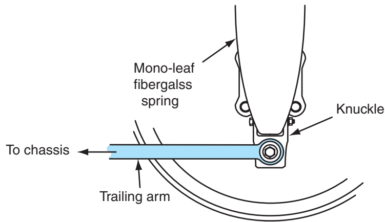
Figure 7-48 Independent rear suspension with mono-leaf transverse fiberglass spring.
