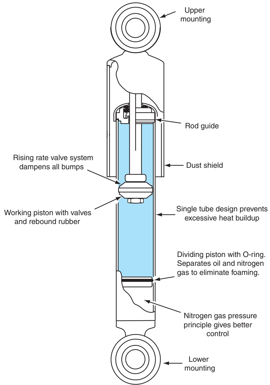
Figure 5-3 Heavy-duty shock absorber.
