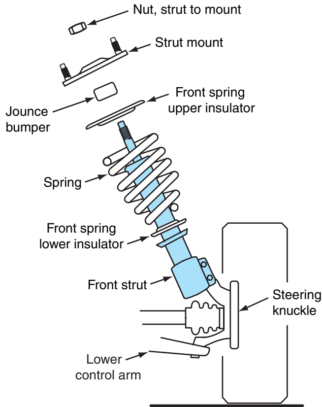
Figure 1-6 Typical MacPherson strut front suspension system.
