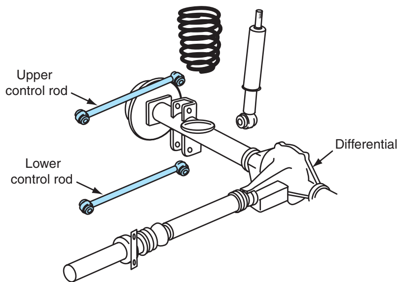
Figure 7-14 Rear suspension system with upper and lower control rods.
