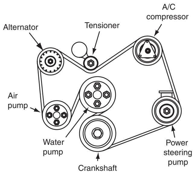
Figure 10-2 Ribbed V-belt.
