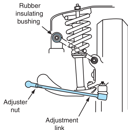
Figure 7-29 Upper control arm, short-and-long arm independent rear suspension system.
