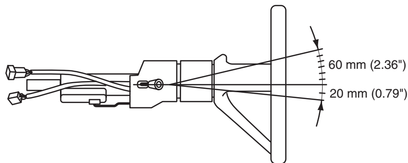
Figure 9-1 Tilt steering column.
