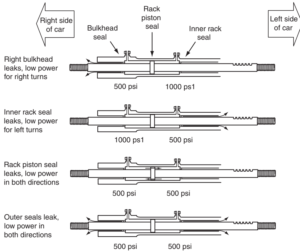
Figure 12-21 Effect of defective rack seals on steering effort imbalance and low power assist.
