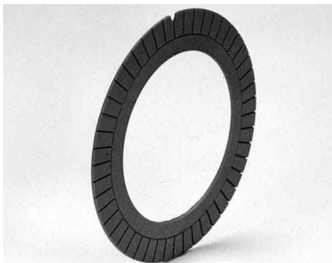
Figure 16-46 Circular shim for rear wheel camber and toe adjustment.
