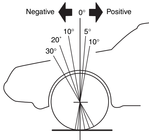
Figure 6-59 Positive and negative caster.
