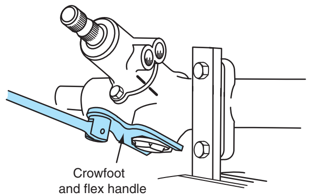
Figure 12-28 Loosening adjuster plug locknut.
