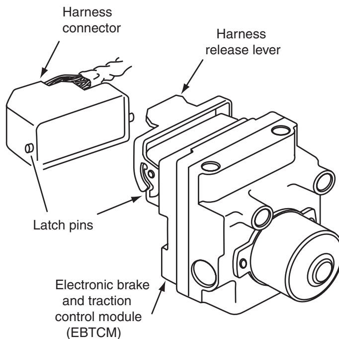
Figure 12-20 Electronic brake and traction control module (EBTCM).
