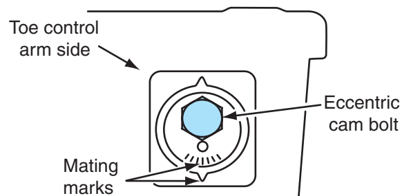
Figure 7-40 Eccentric cam bolt on inner end of toe control arm.
