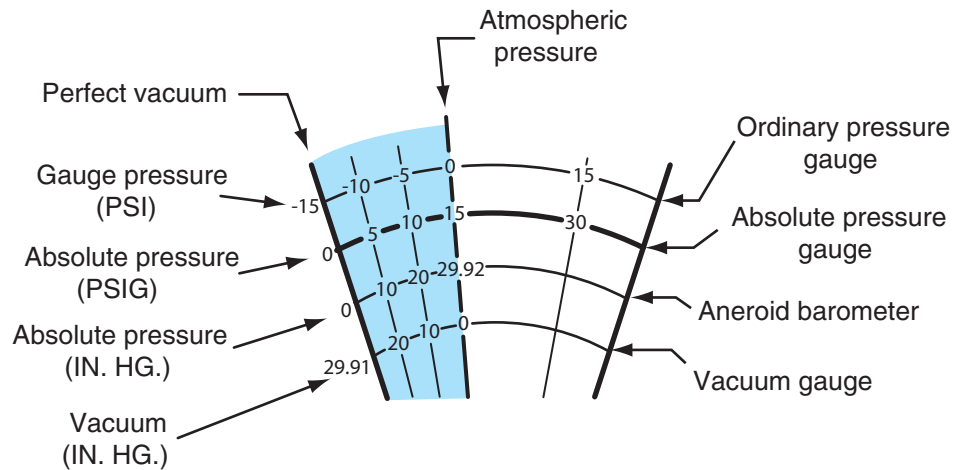
Figure 2-23 Pressure and vacuum scales.
