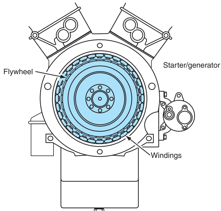
Figure 10-17 Starter/generator.
