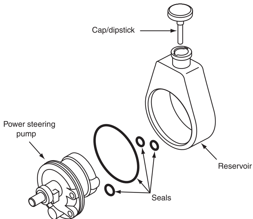
Figure 10-23 Integral power steering pump reservoir seal and O-ring.
