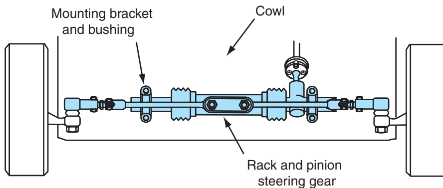
Figure 9-31 Rack and pinion steering gear mounted on cowl.
