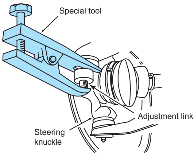
Figure 7-27 Removing the suspension adjustment link from the knuckle.
