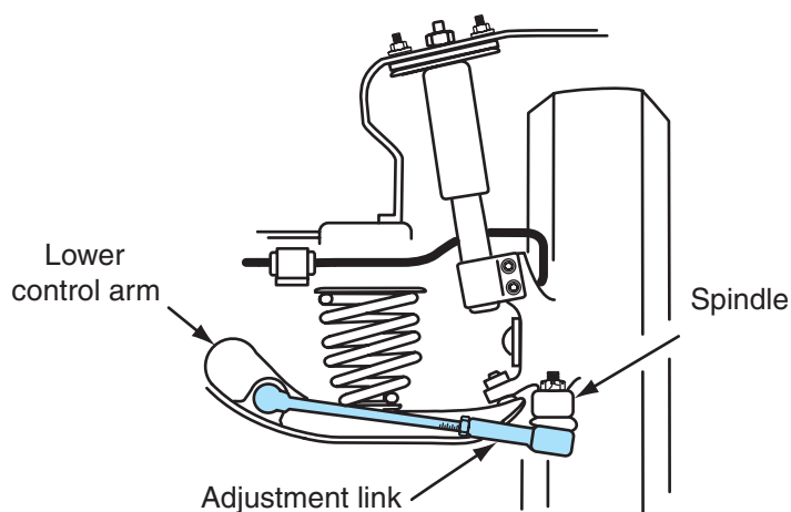
Figure 7-26 Suspension adjustment link.
