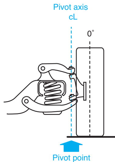
Figure 16-3 Front suspension with a 0^\circ SAI line.
