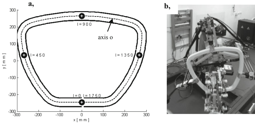
Fig. 3 Closed-frame-core—the sizes (on the left) and in the frame core connected to the robot-end-effector (on the right)
