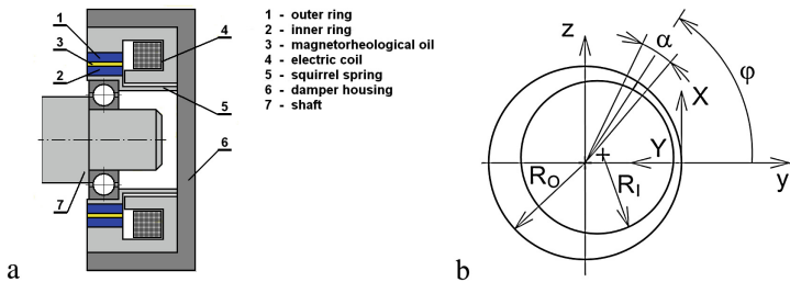
Fig. 1 The scheme of a MR squeeze film damper (a) and the damper (xyz) and the fluid film (XYZ) coordinate systems (b)
