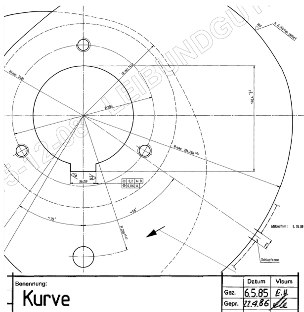
Fig. 3 Cutouts from the drawing of a double cam
