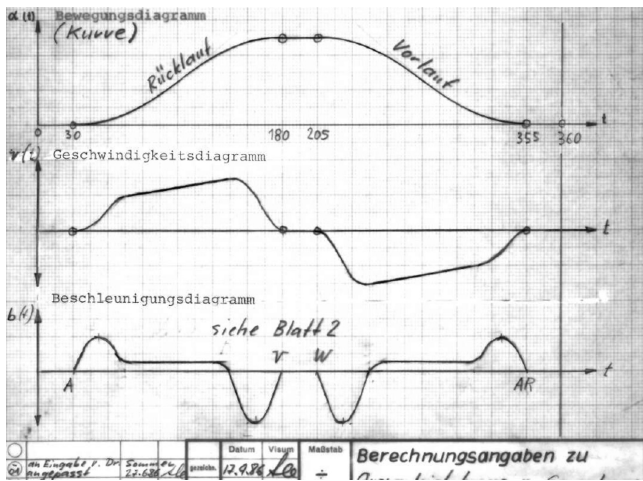
Fig. 4 Scheme of the motion function of the working link
