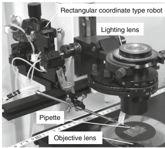
a) Rectangular coordinate type robot arm
