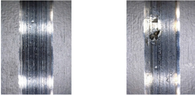
Micropitting, steel 14 220, 11 \times 10^6 cycles Macropitting, steel 14 220, 202 \times 10^6 cycles
