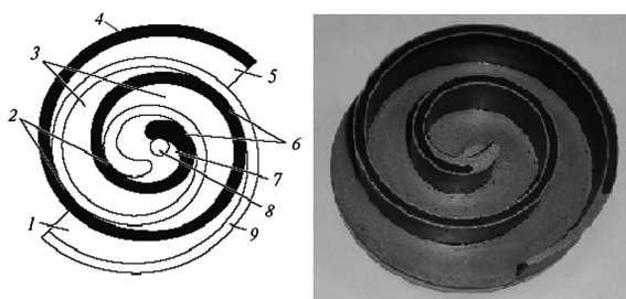
Fig. 1 Scheme of scroll air motor. 1 and 5—exhaust chambers, 2 and 6—scroll contact points, 3—closed expansion chambers, 4—fixed scroll, 7—central chamber, 8—inlet port, 9—moving scroll
