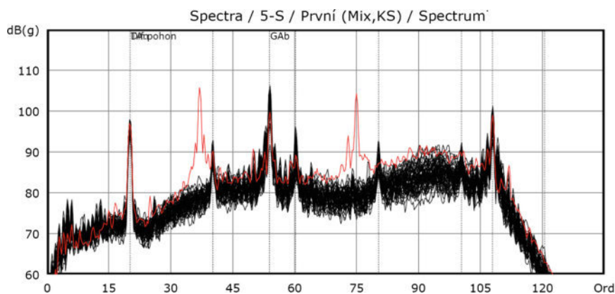
Fig. 7 Noise spectrum 5-S (MIX)
