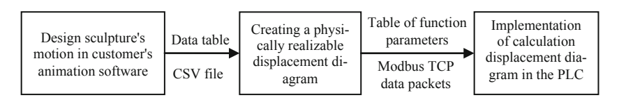
Fig. 3 Data flow diagram in the creating of displacement diagram
