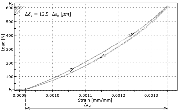
Fig. 5 Loading cycles of three-dimensional body and cylindrical body
