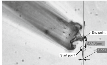
b) Measurement of a pipette motion on the horizontal plane using the microscopic image processing
