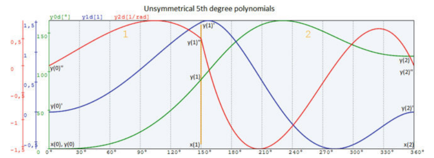
Fig. 2 Creating of displacement diagram by folding polynomials
