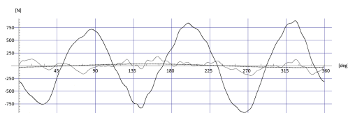
Fig. 6 Resonance force Z ( thick line ), force Z with filtered-out third harmonic ( thin line ) and first harmonic component of the force ( dotted ) at 1450 rpm after balancing
