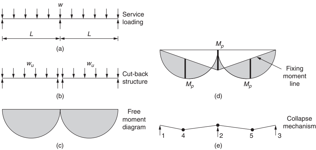
FIGURE 8.4 Statical method of design.
