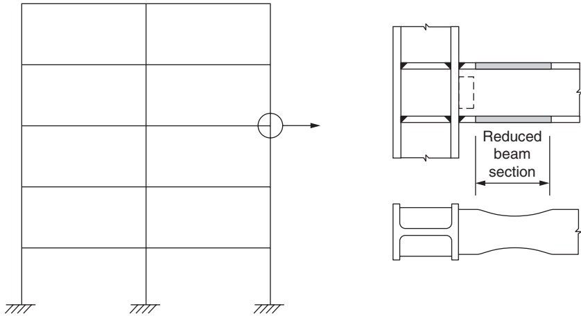
FIGURE 1.9 Moment-resisting frame.
