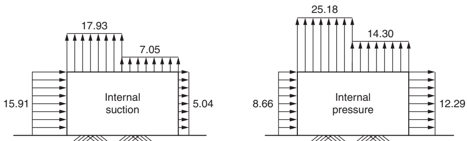
FIGURE 2.34 Wind pressure diagrams, in lb/ft², for Example 2.19.
