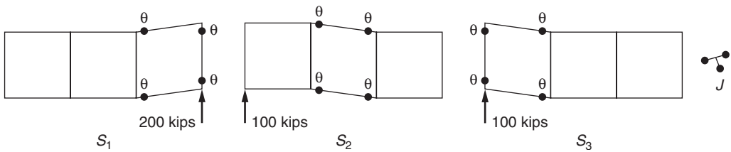
FIGURE 8.13 Independent mechanisms.
