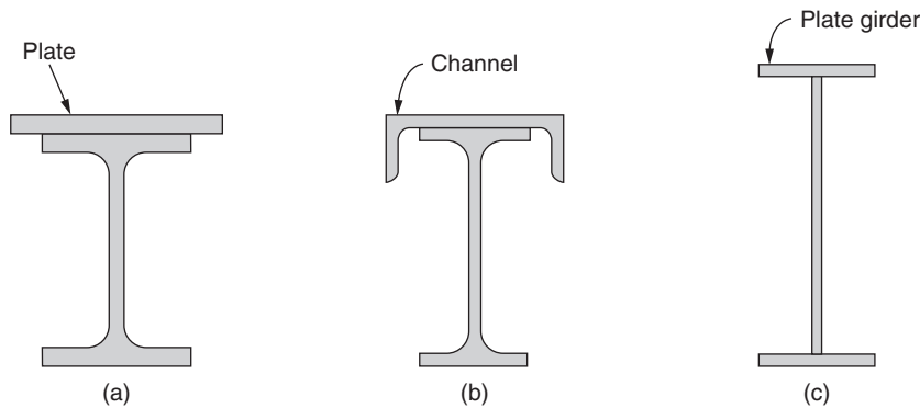
FIGURE 5.4 Built-up sections.
