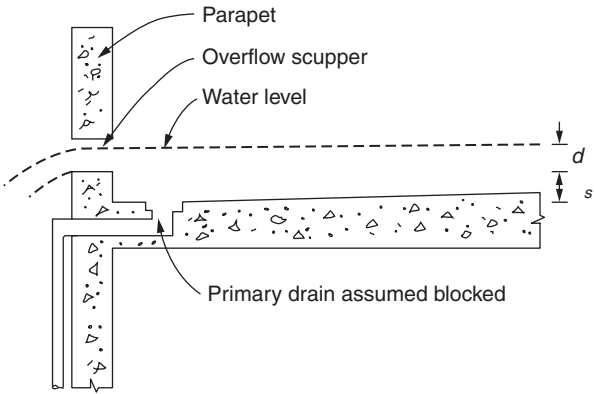
FIGURE 2.30 Roof drainage.
