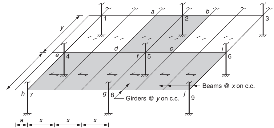
FIGURE 2.14 Influence areas.
