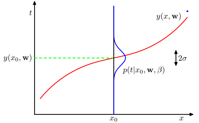
Figure 1.16 Schematic illustration of a Gaussian conditional distribution for t given x given by (1.60), in which the mean is given by the polynomial function y(x, \mathbf{w}) , and the precision is given by the parameter \beta , which is related to the variance by \beta^{-1} = \sigma^2 .
