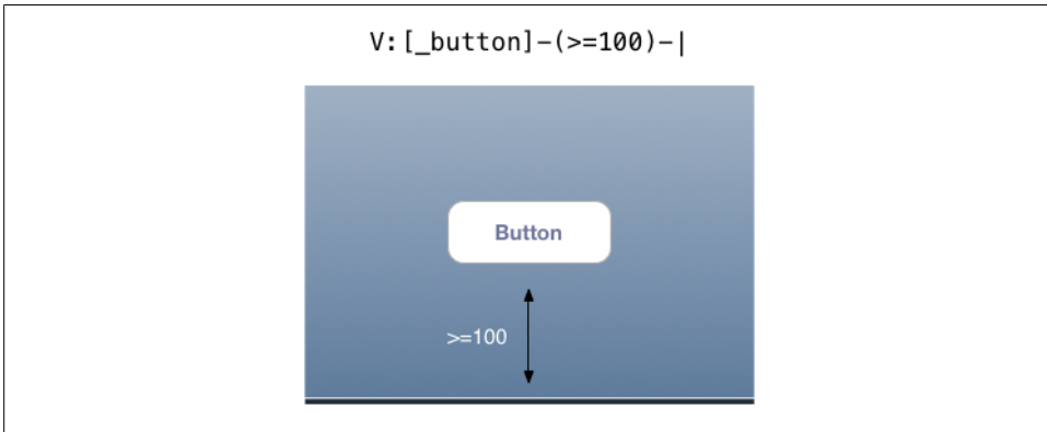
Figure 3-5. An example of setting vertical alignment using the Visual Format Language
