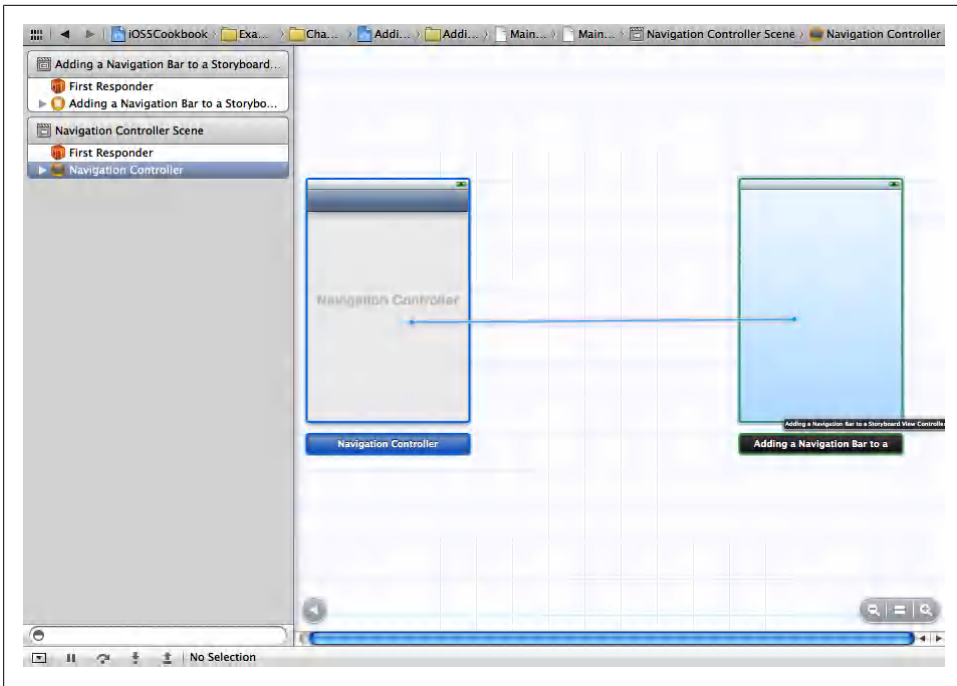
Figure 5-10. Connecting the navigation controller to the initial view controller
