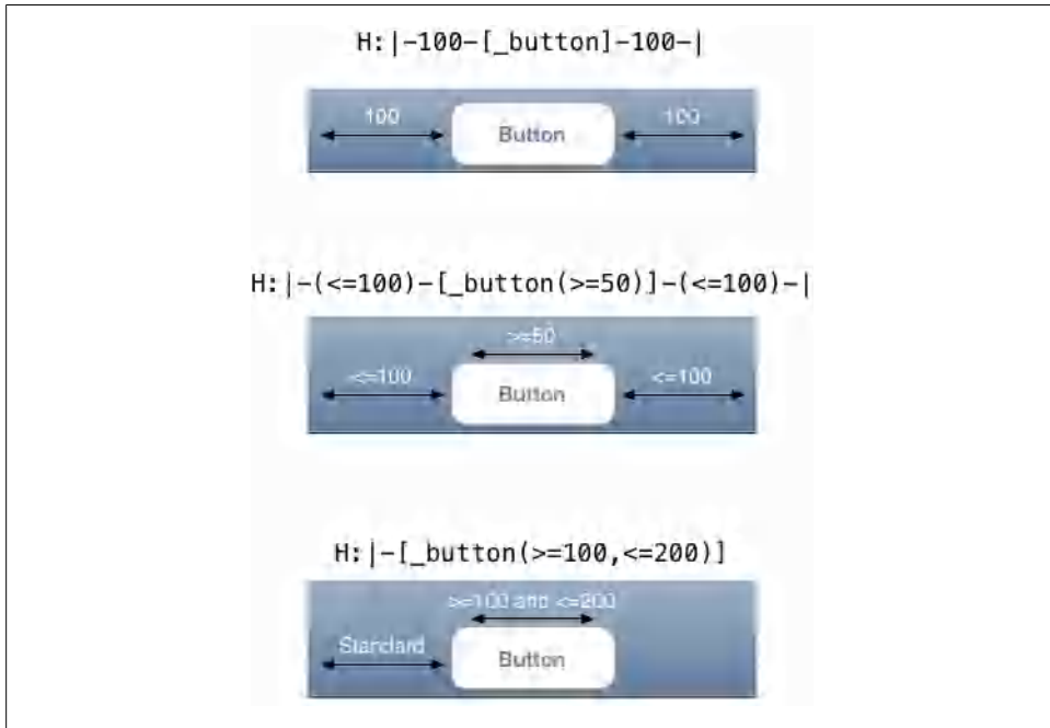
Figure 3-4. Three simple examples of the usage of the Visual Format Language for horizontal constraints
