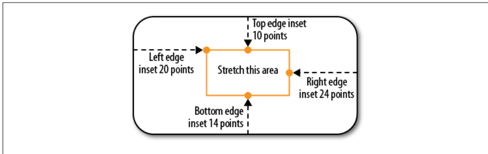
Figure 17-20. The stretchable portion of the image is defined by the edge insets
