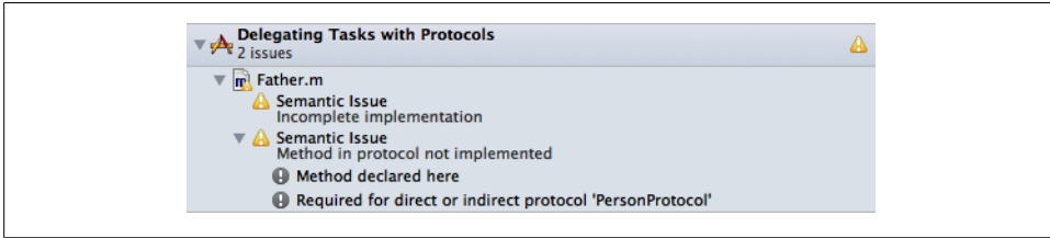
Figure 1-32. The Father class does not implement the breathe method defined in the PersonProtocol protocol
