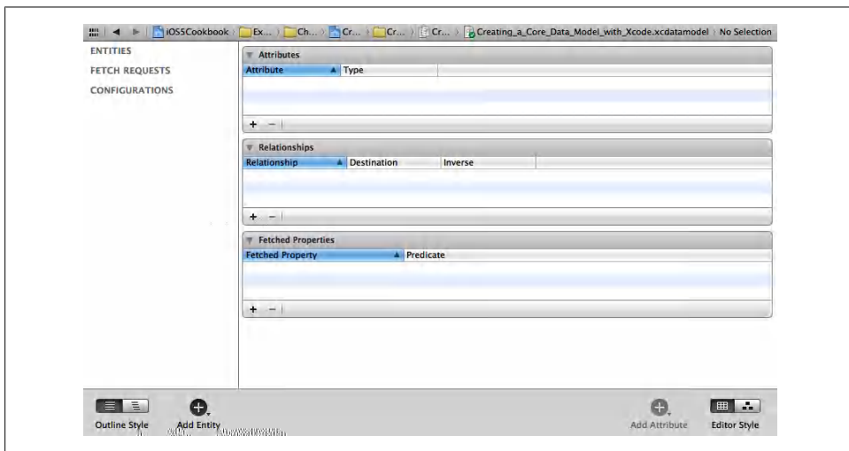
Figure 15-4. Visual data editor in Xcode
