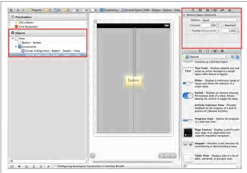
Figure 3-15. Modifying a constraint in Interface Builder
