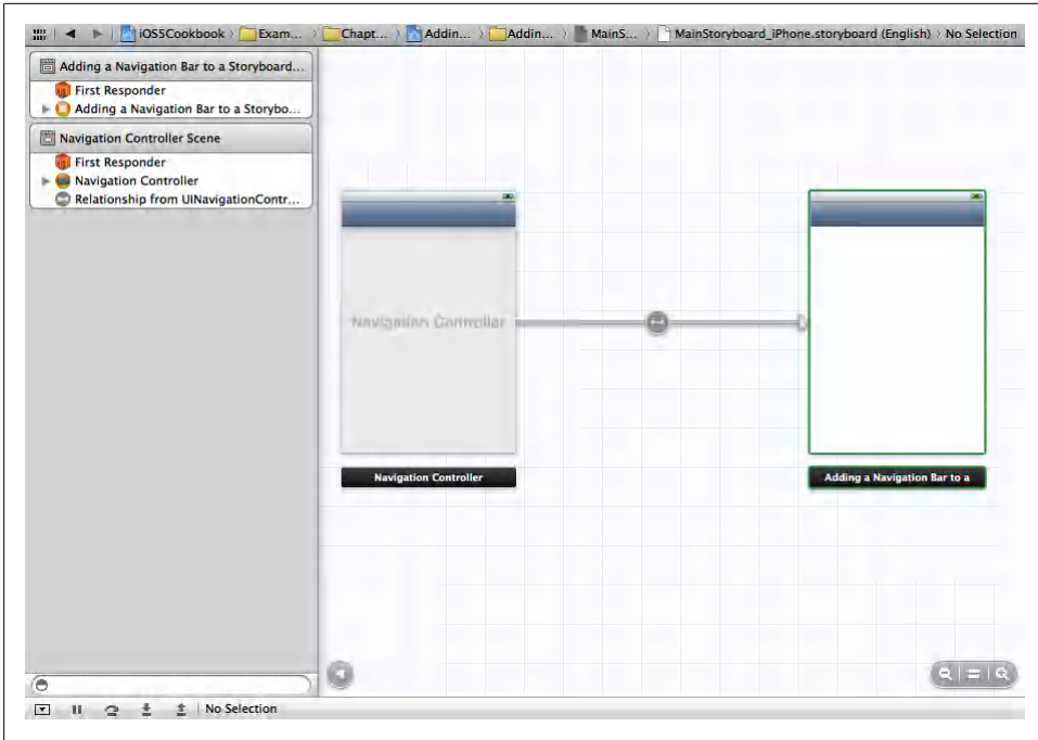
Figure 5-12. The navigation controller is connected to the initial view controller
