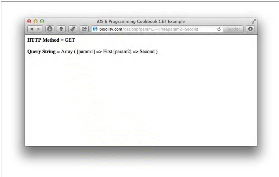
Figure 9-2. Query string parameters sent to the GET web service
