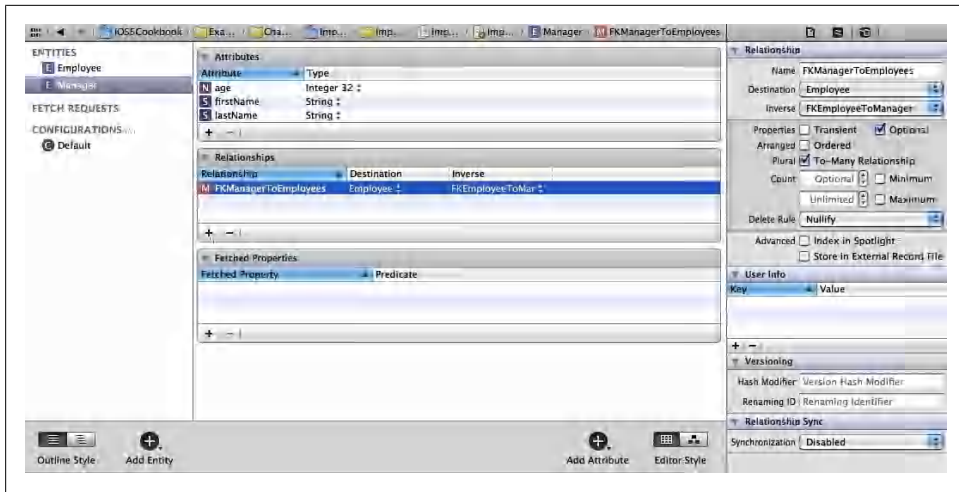
Figure 15-18. The Manager inverse relationship established with employees
