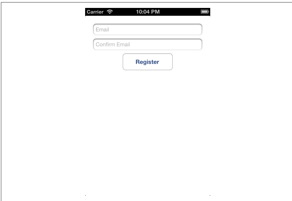
Figure 3-6. The UI that we want to achieve using constraints and the Visual Format Language
