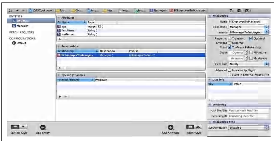
Figure 15-19. Creating a Many-to-Many relationship between the Manager and Employee entities
