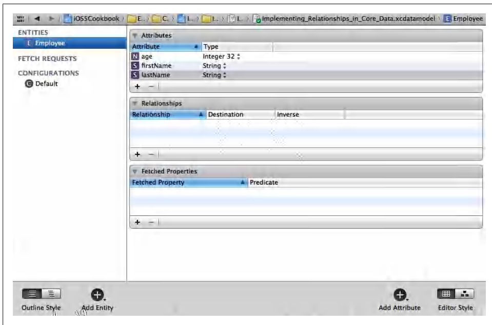
Figure 15-13. The Employee entity with three attributes
