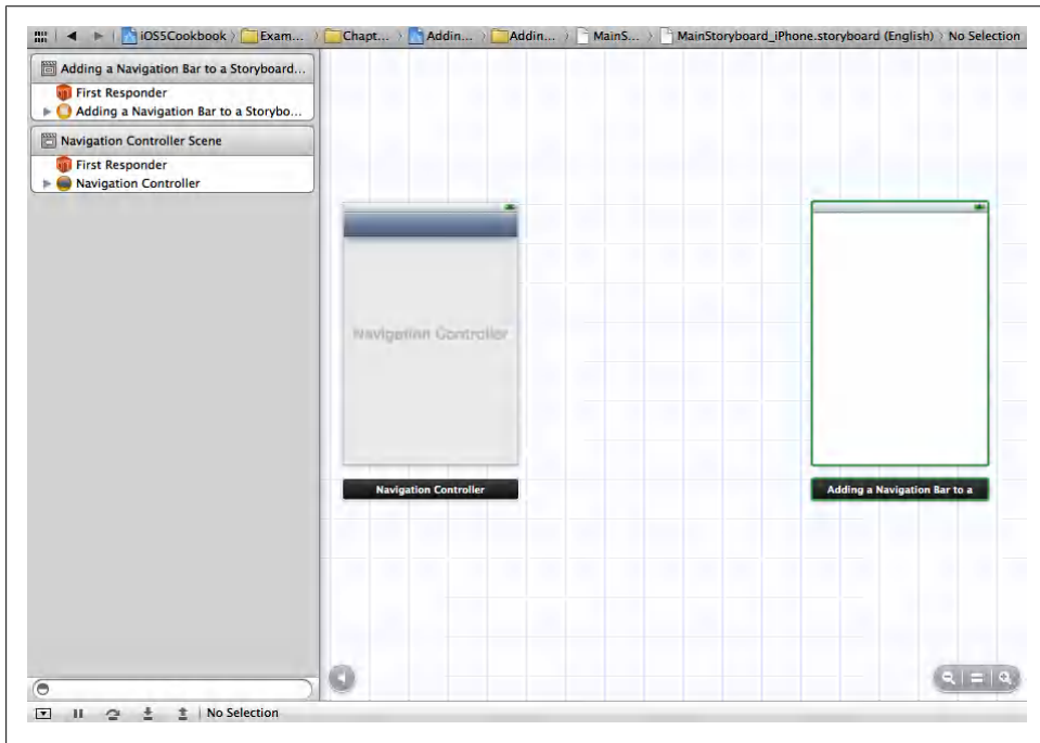
Figure 5-9. Removing the root view controller that comes with the navigation controller object
