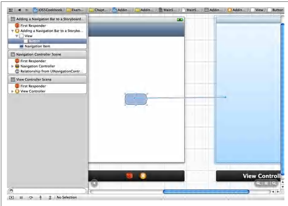
Figure 5-20. Connecting a button to another view controller in a storyboard
