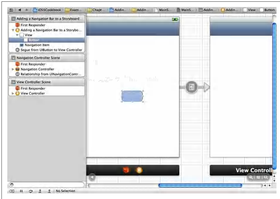
Figure 5-22. The first view controller is connected to the second view controller through a segue
