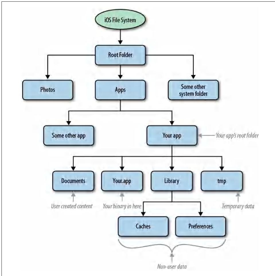
Figure 12-1. Depiction of the iOS file system
