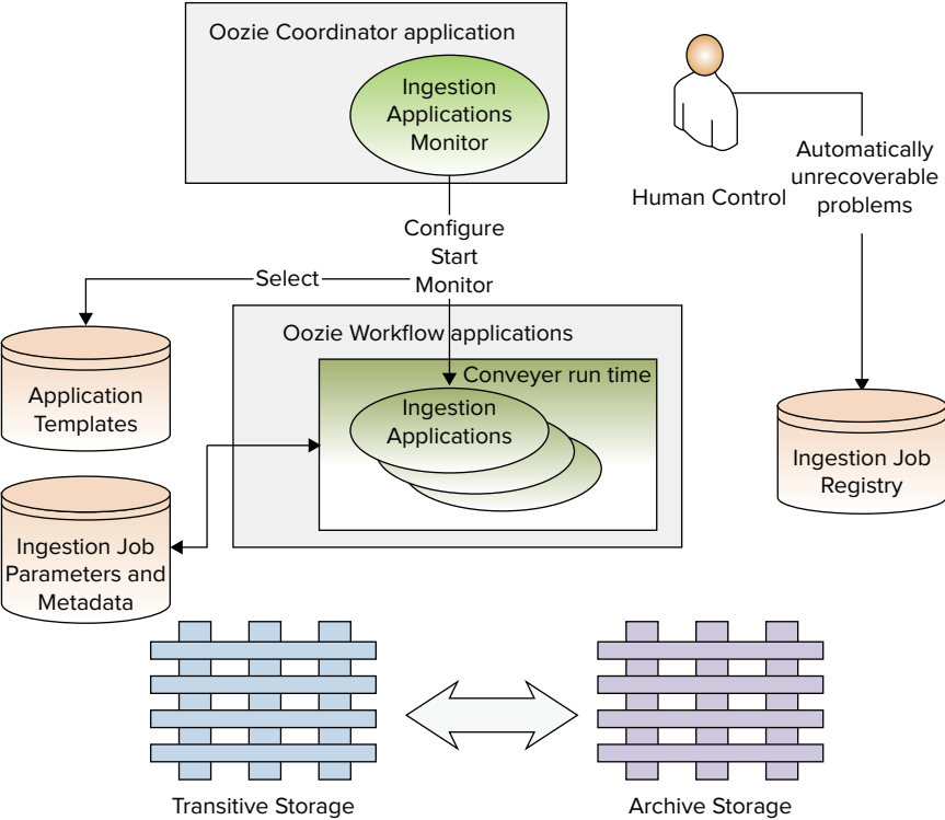
FIGURE 8-5: High-level components of the data ingestion conveyor
