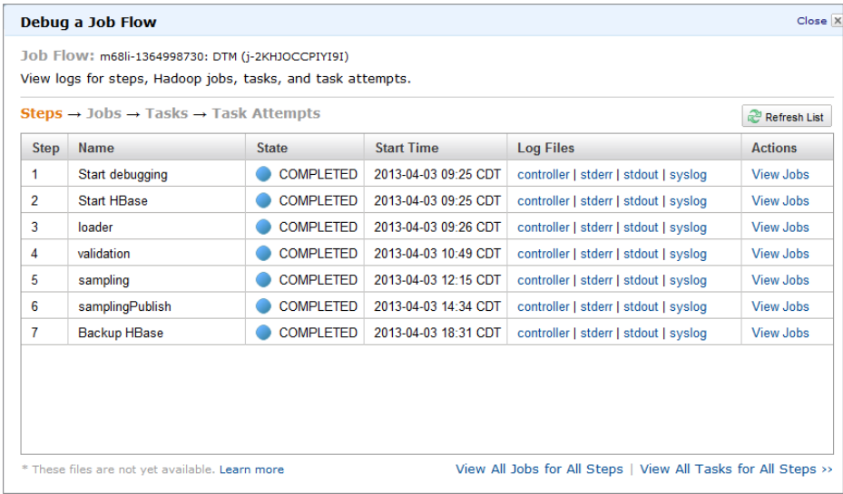
FIGURE 11-10: Using the AWS console to debug EMR execution
