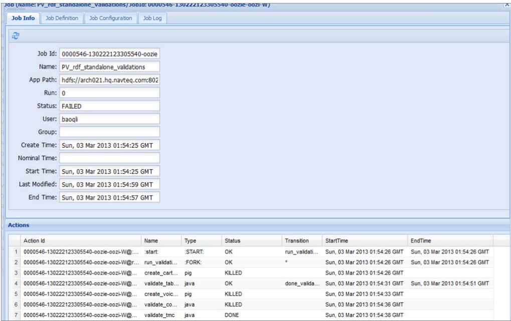
FIGURE 6-12: Oozie job execution details
