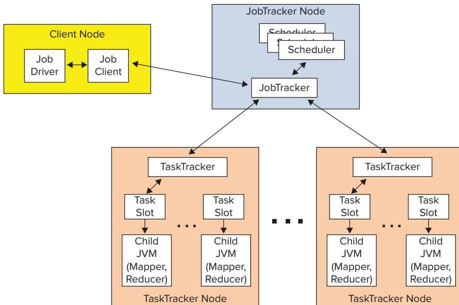
FIGURE 3-3: MapReduce execution
