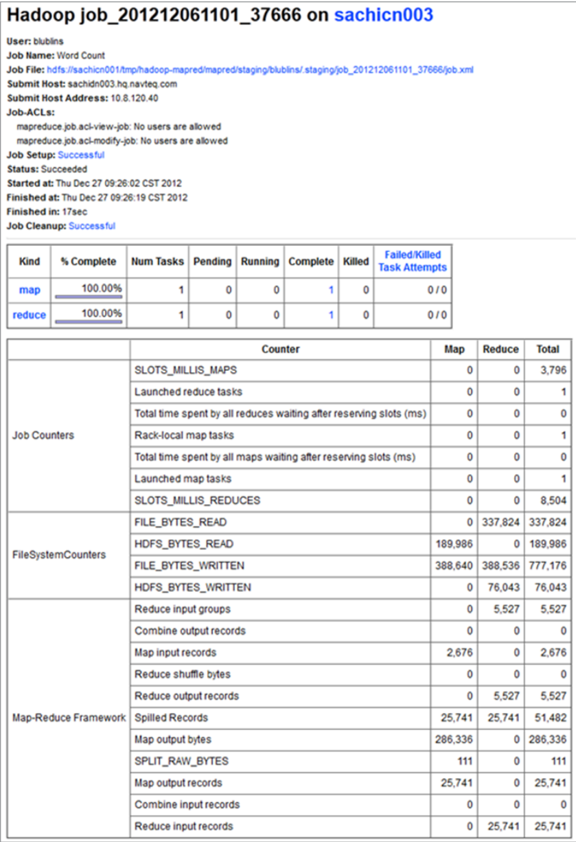
FIGURE 3-5: WordCount job page
