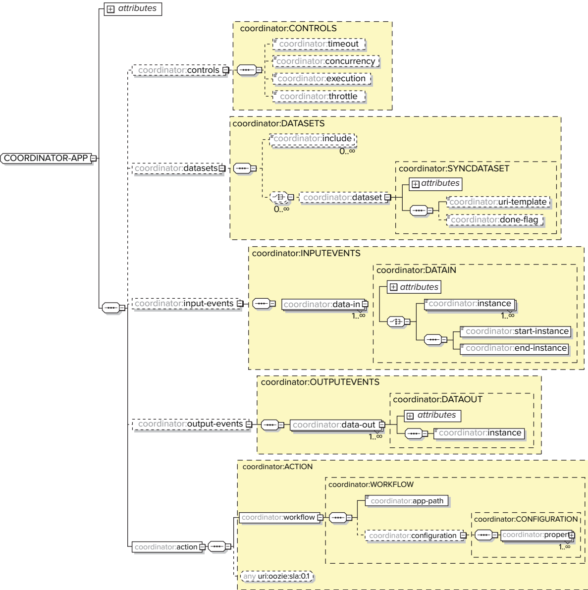
FIGURE 6-5: Coordinator language schema
