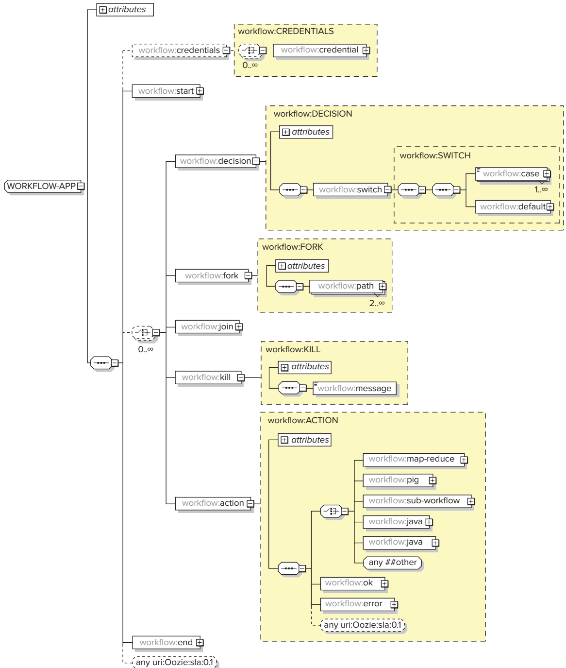
FIGURE 6-2: hPDL schema
