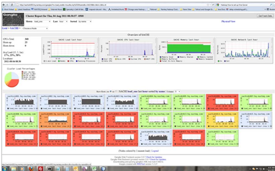
FIGURE 4-1: Nodes utilization in the case of traditional data locality
