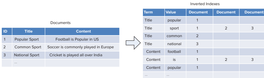
FIGURE 3-6: Inverted index
