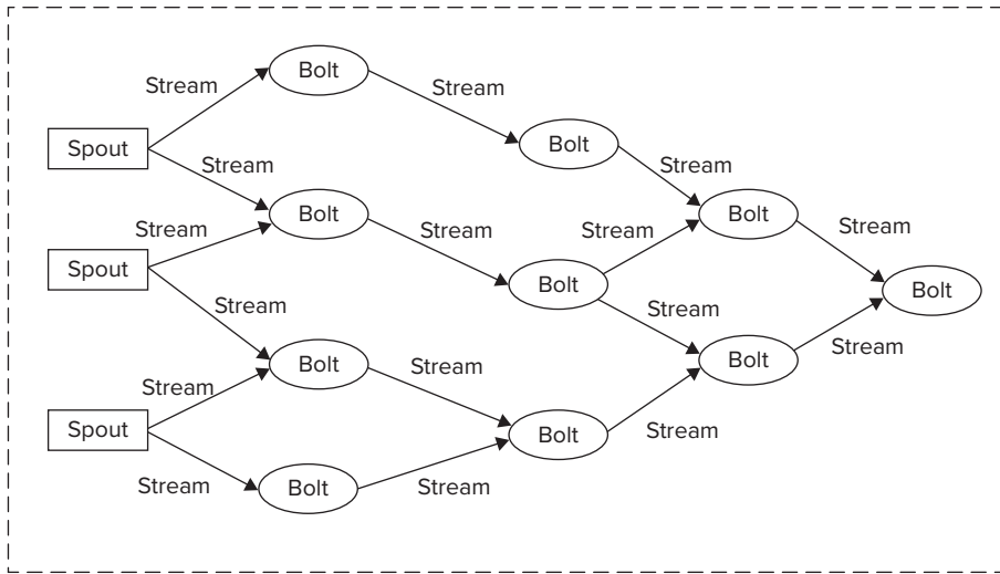
FIGURE 9-19: Storm application
