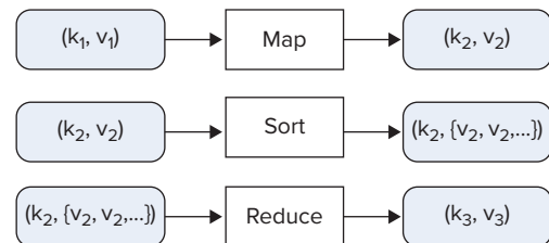
FIGURE 3-1: The functionality of mappers and reducers
