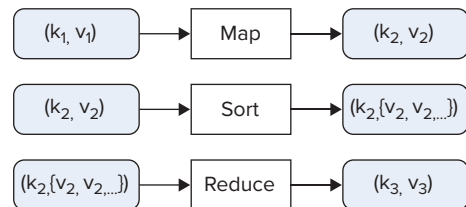
FIGURE 9-16: MapReduce processing
