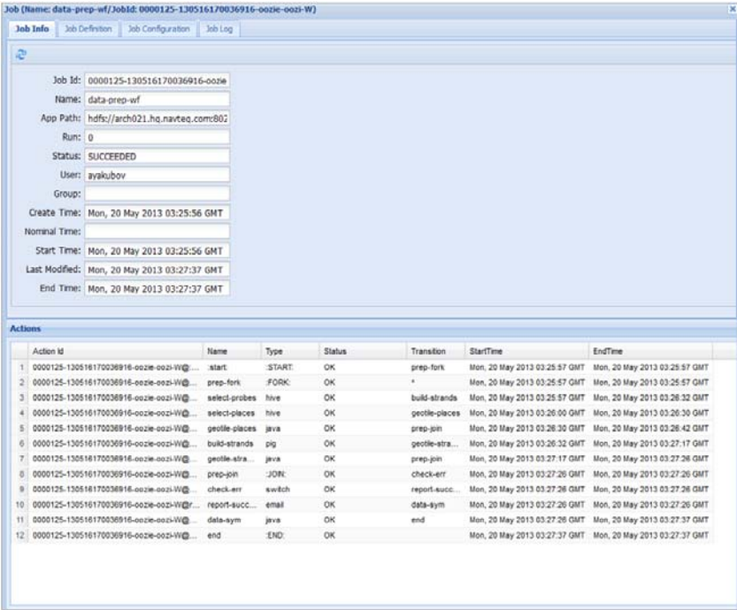
FIGURE 7-14: Workflow job after completion
