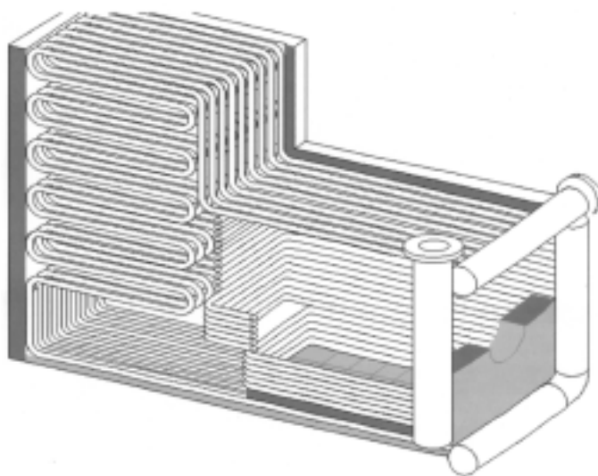
Figure 4-6. HTHW generator
