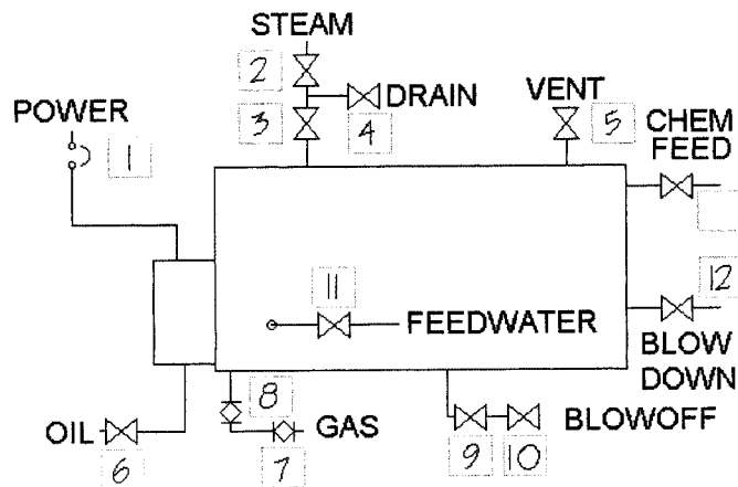
Figure 5-2. Lock-out/tag-out diagram
