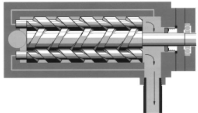
Figure 9-83. Screw pump
