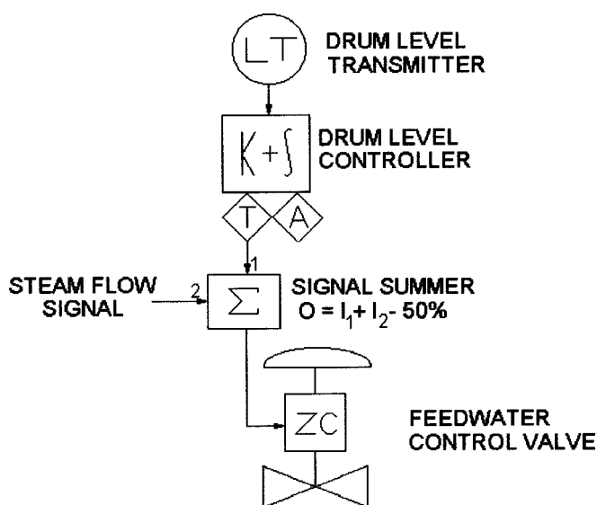
Figure 10-25. Two element level control schematic
