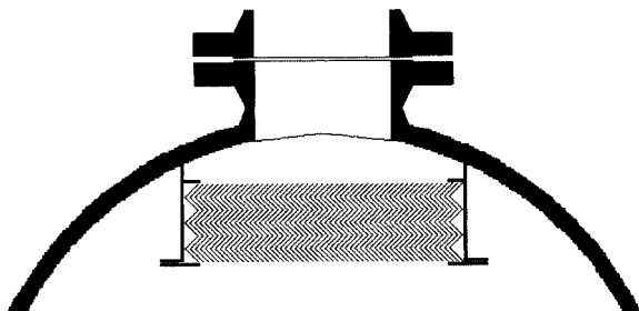
Figure 9-29. Chevron separator
