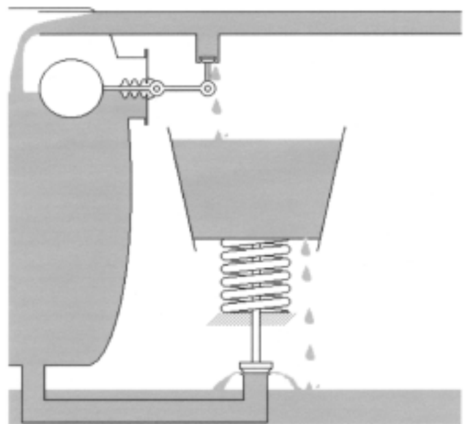
Figure 10-2. Bucket valve control
