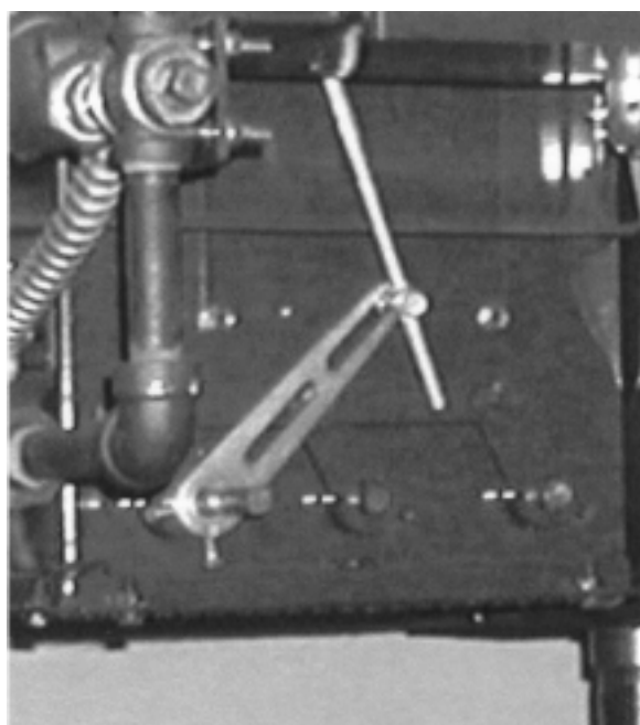
Figure 10-29. Link to fan damper
