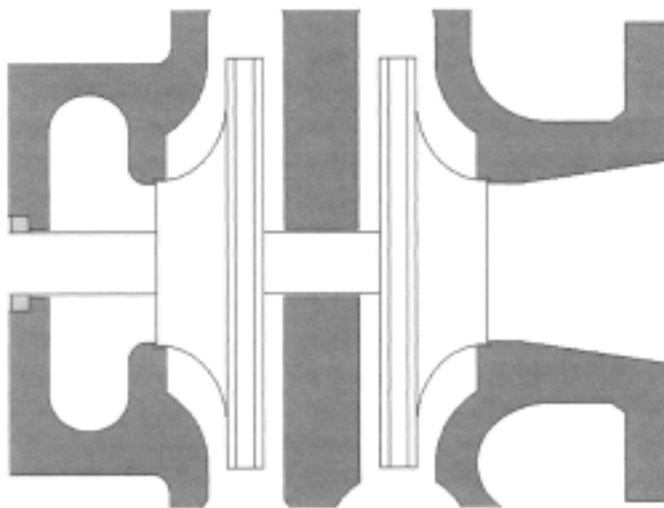
Figure 9-75. Opposing stages of centrifugal pump
