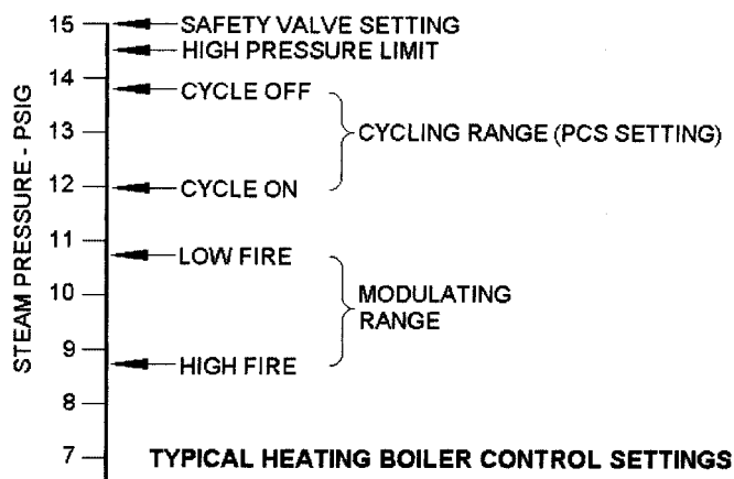
Figure 10-20. Range of control, modulating and on-off
