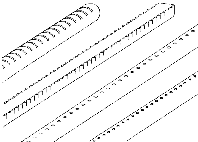
Figure 9-47. Flame runners
