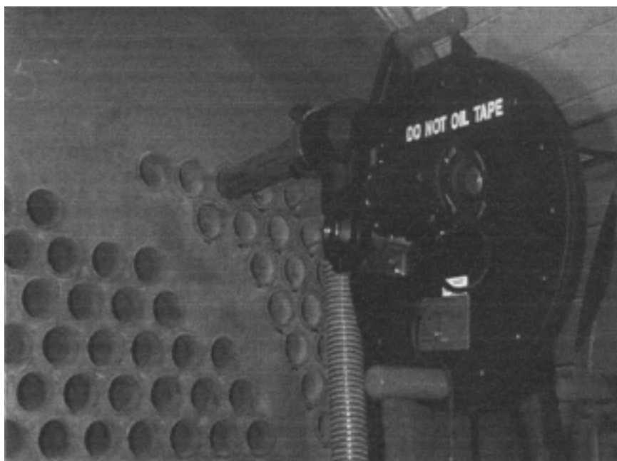
Figure 5-9A. Firetube cleaner
