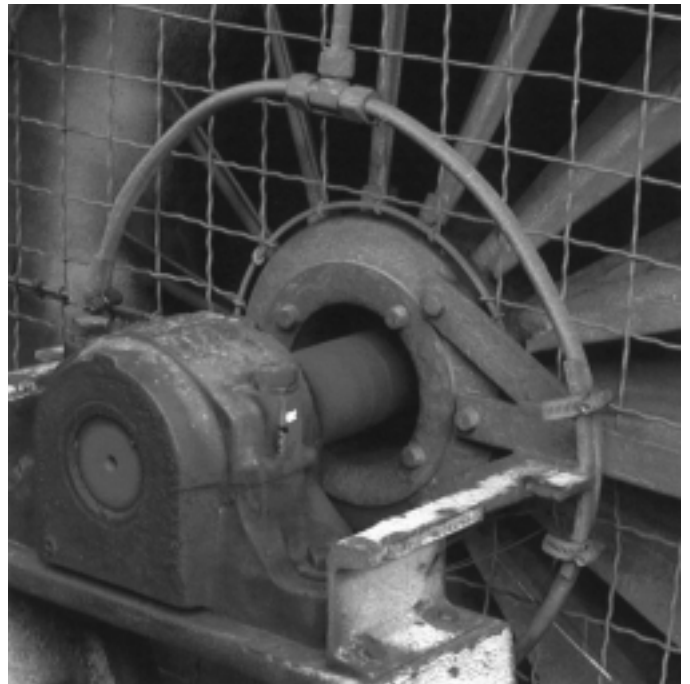
Figure 10-31. Fan inlet flow measuring ring
