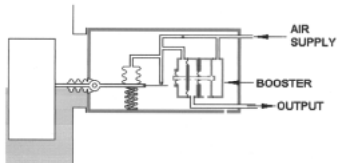
Figure 10-4. Booster for transmitter
