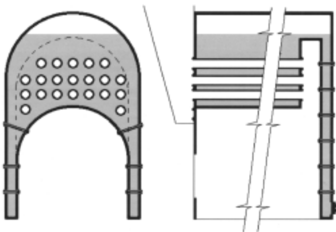
Figure 9-9. Firebox boiler
