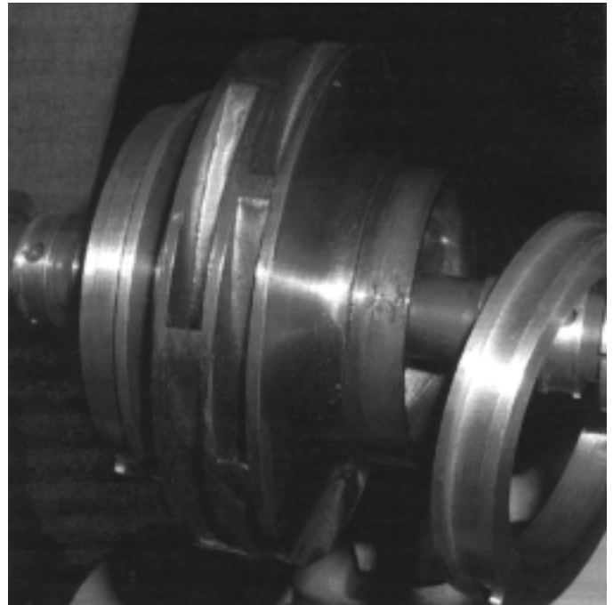
Figure 9-72. Wear rings
