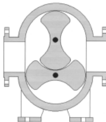
Figure 9-97. Lobe type rotary compressor
