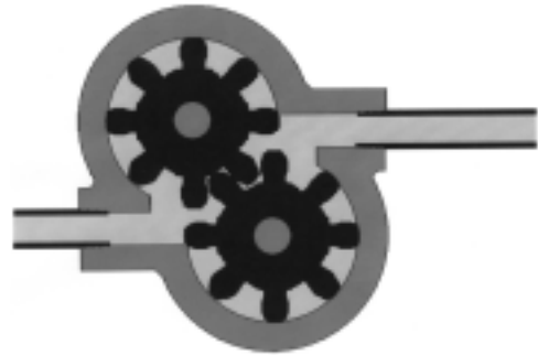
Figure 9-81. Gear pump
