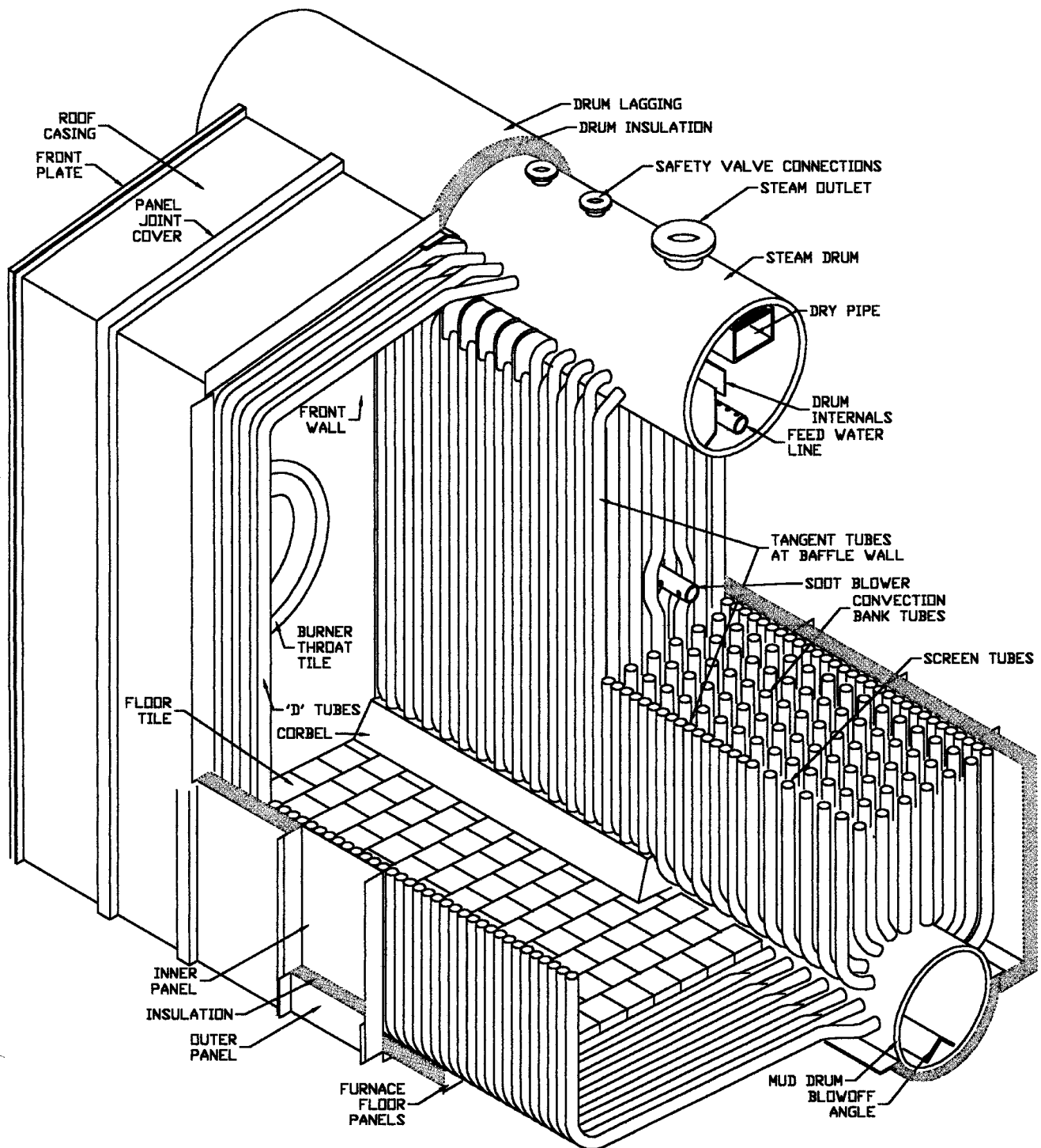
Figure 9-22. "D" type boiler details
