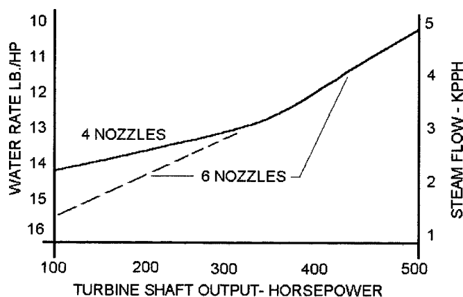
Figure 2-8. Willans line
