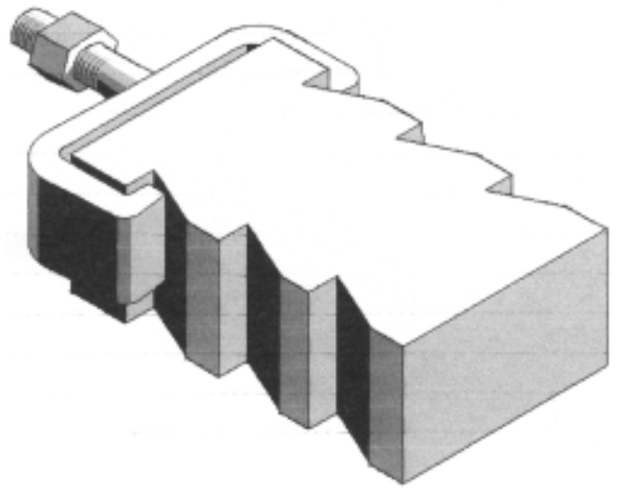
Figure 5-6. Refractory anchor
