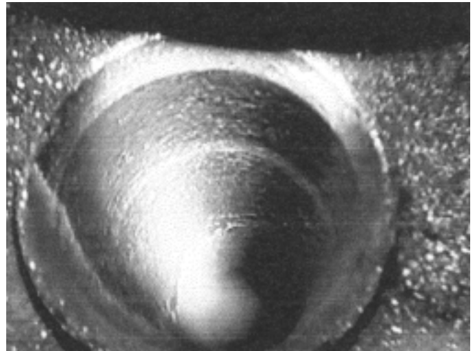
Figure 5-12A. Rolled tubes - flared
