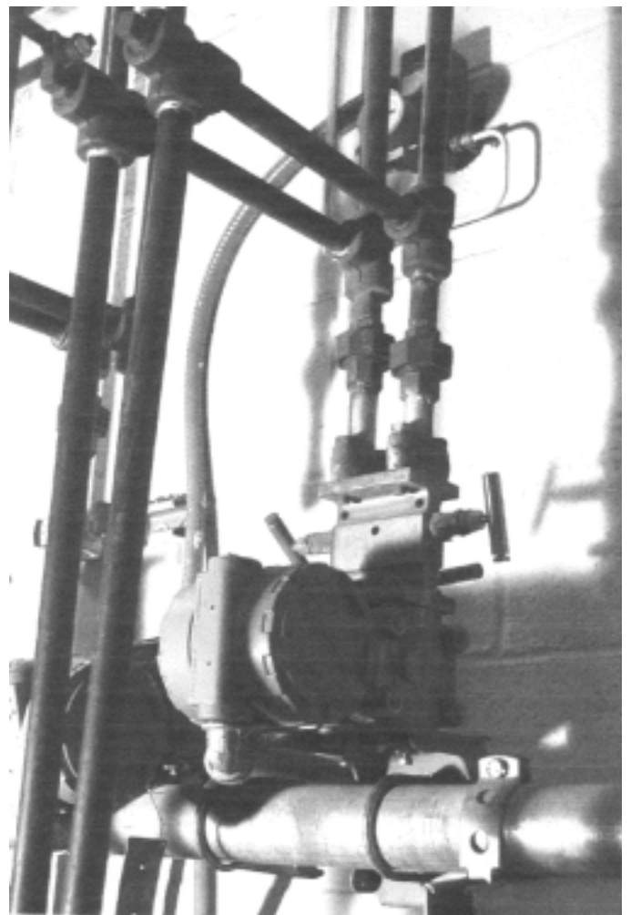
Figure 10-35. Improper transmitter installation
