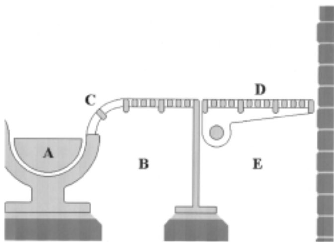
Figure 9-59. Dump grate
