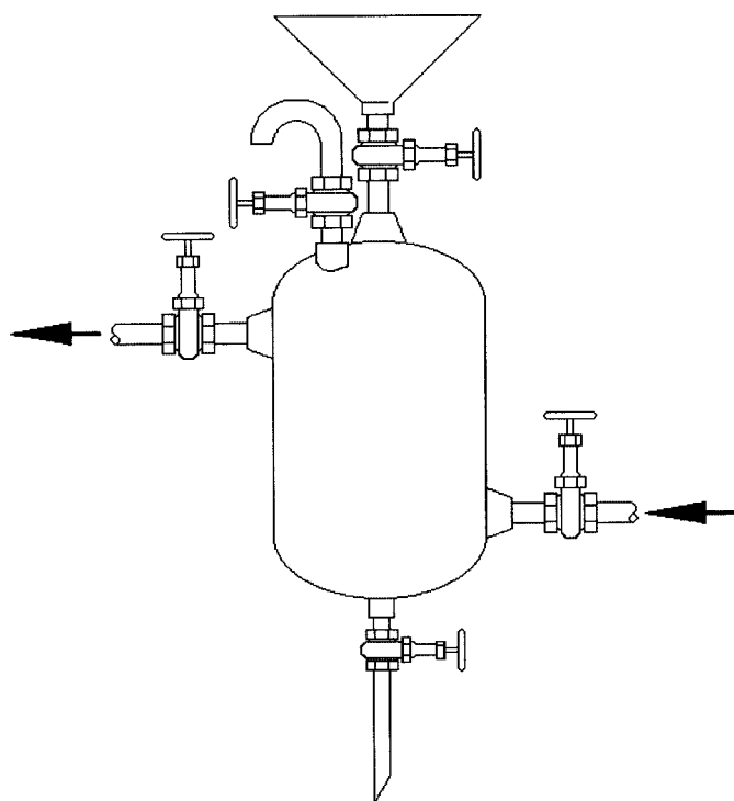
Figure 6-2. Shot feeder
