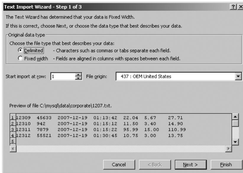
Figure 38-1. Microsoft Excel's Text Import Wizard
