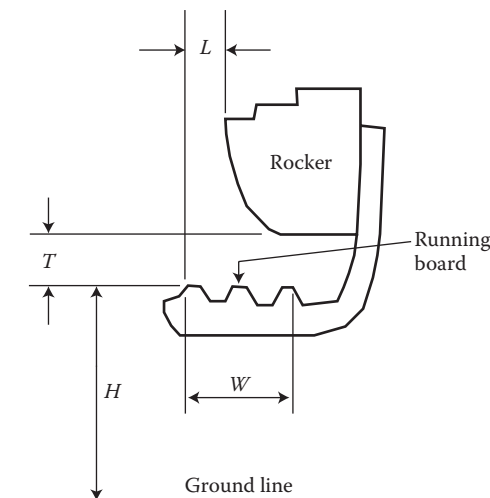
FIGURE 8.7 Running board dimensions.
