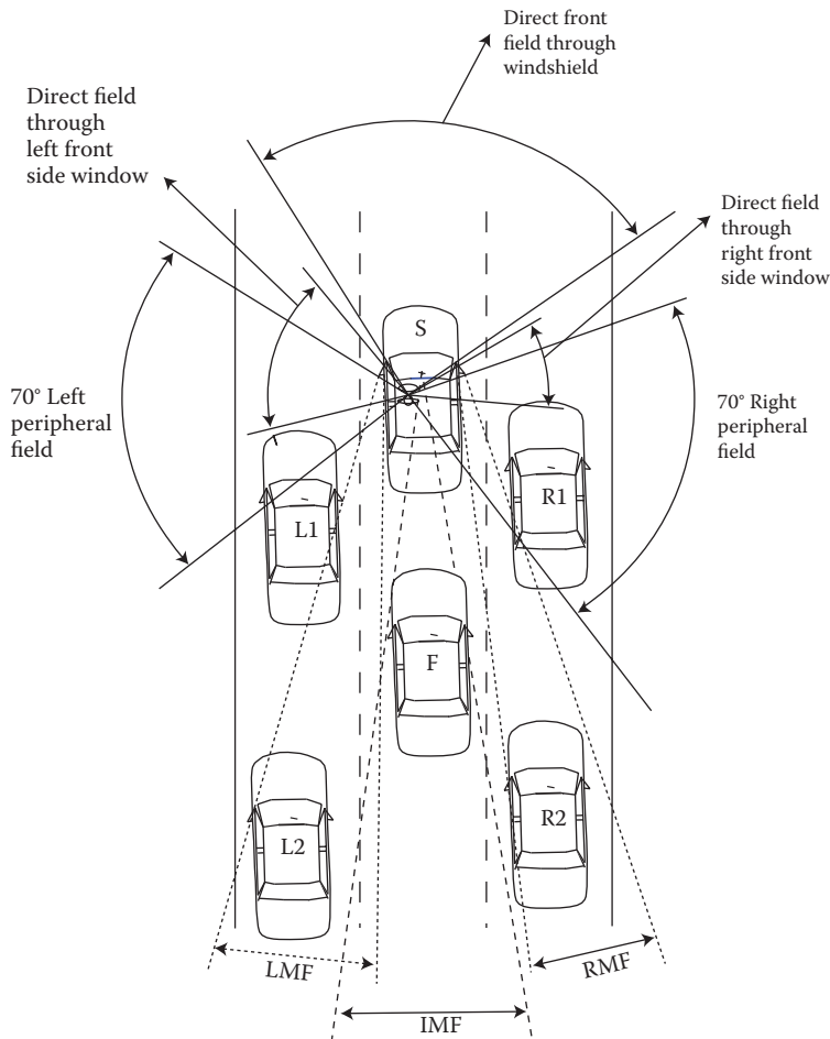
FIGURE 6.2 A 360-degree visibility from direct, indirect, and peripheral fields. (Note that the driver in vehicle S can see at least a portion of any of the vehicles on his front, sides, or rear.)
