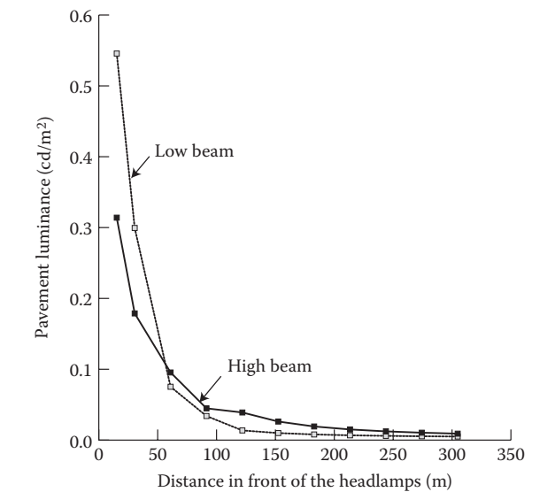
FIGURE 7.6 Pavement luminance in the middle of the driving lane with low and high beam.
