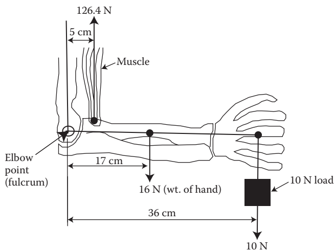
FIGURE 2.4 Upper-arm lever and force configuration while holding a weight of 10 N in the hand. (Redrawn from Chaffin, D. B., G. B. J. Andersson, and B. J. Martin: Occupational Biomechanics . 1999. Copyright Wiley-VCH Verlag GmbH & Co. KGaA. Reproduced with permission.)
