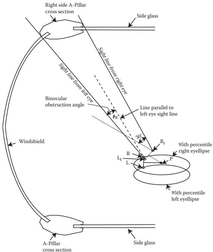
(b) Obstruction due to right A-pillar
