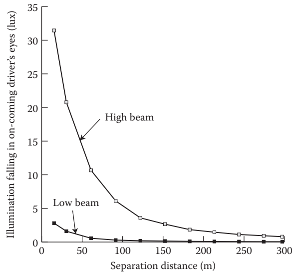
FIGURE 7.8 Illumination falling into oncoming driver's eyes from properly aimed high and low beams on a two-lane straight-level roadway.
