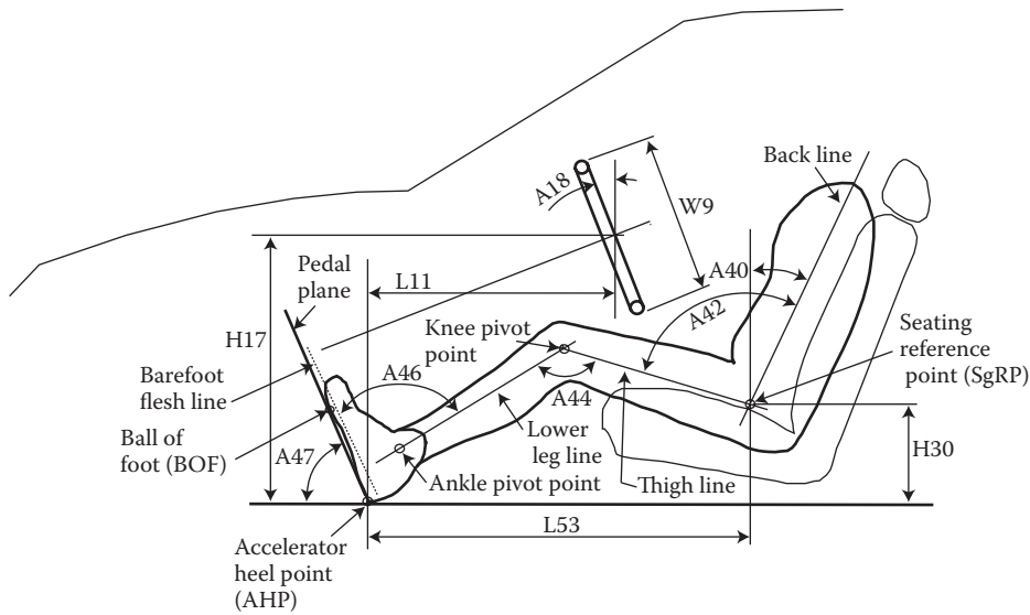
FIGURE 3.3 Interior package reference points and dimensions.
