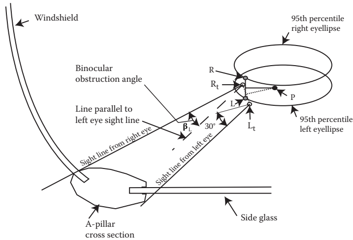
(a) Obstruction due to left A-pillar
