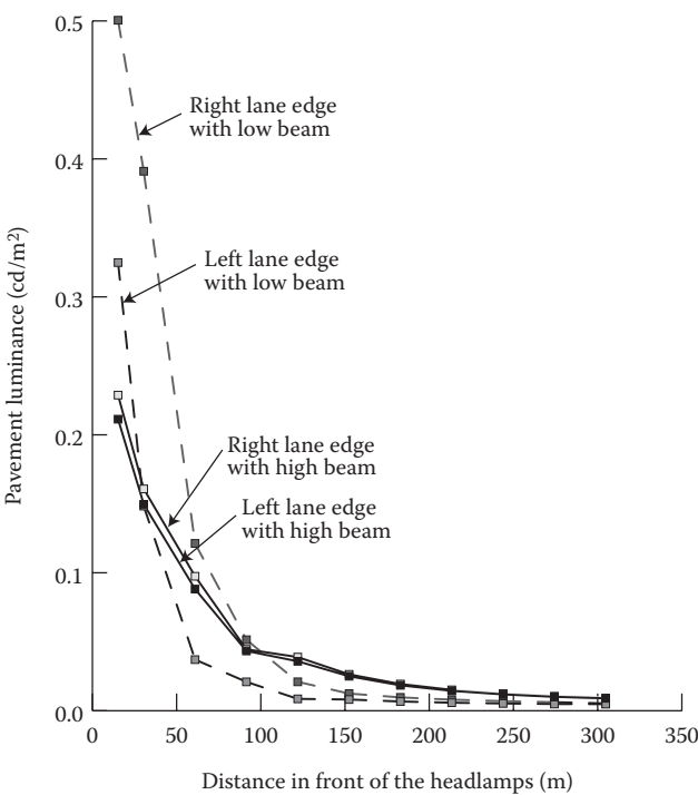
FIGURE 7.7 Pavement luminance at the lane edges of the driving lane with low and high beam.
