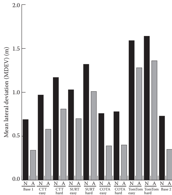
FIGURE 14.3 Mean lateral deviations (MDEV) values obtained by using the normative (N) and the adaptive (A) models for the baseline (called base 1 and base 2) and dual-task conditions.
