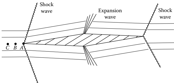
FIGURE 8.4 A diamond-shaped airfoil traveling at supersonic velocity.
