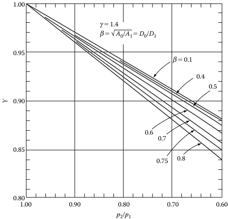
FIGURE 10.29 Compressibility factor Y as a function of pressure ratio p_2/p_1 , for square-edged orifices where the fluid has \gamma=1.4 . (Reprinted from Fluid Meters—Their Theory and Application , 5th ed., The American Society of Mechanical Engineers, New York, 1959. With permission.)
