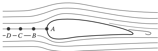
FIGURE 8.3 A wing traveling at subsonic velocity through air.
