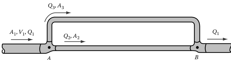
FIGURE 5.27 Pipes in parallel.
