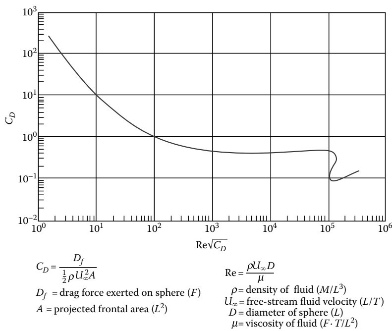
FIGURE 6.17 Drag coefficient as a function of \text{Re}\sqrt{C_D} for spheres. (Note on how this figure was developed: An enlarged copy of Figure 6.16 was scanned into a computer. The drawing was scaled and digitized to yield tabular data of C_D versus \text{Re} . The data were then manipulated appropriately to obtain \text{Re}\sqrt{C_D} , which was graphed versus C_D .)
