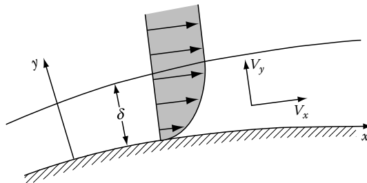
FIGURE 13.4 Flow in the boundary layer.
