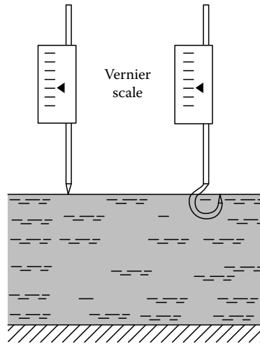
FIGURE 10.35 Point gauge and hook gauge used to measure liquid depth.
