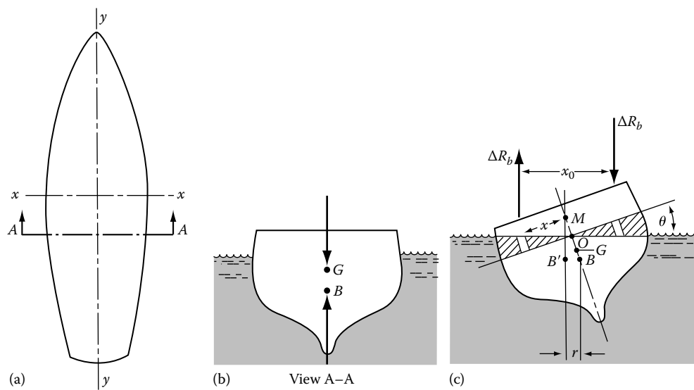
FIGURE 2.31 A sketch for calculating metacentric height.
