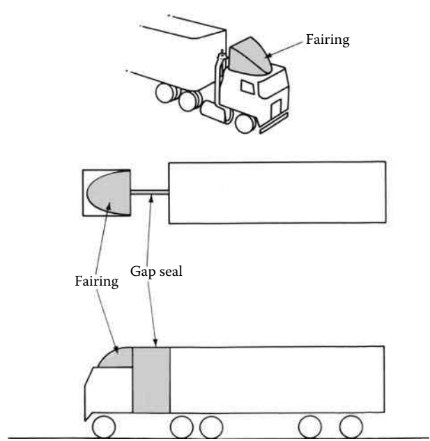
FIGURE 6.27 A fairing and gap seal attached to a tractor-trailer truck.
