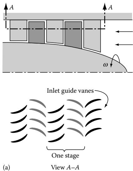
FIGURE 9.18 (a) An axial-flow compressor.
