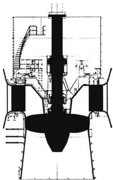
FIGURE 9.11 (a) Axial-flow propeller turbine. (b) Kaplan runner of an axial-flow turbine. (Courtesy of Allis-Chalmers Hydro Turbine Division. With permission.) (c) Typical installation of an axial-flow turbine system. (Courtesy of Allis-Chalmers Hydro Turbine Division. With permission.)
