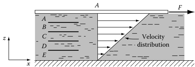
FIGURE 5.4 Layers of fluid flow between parallel plates.
