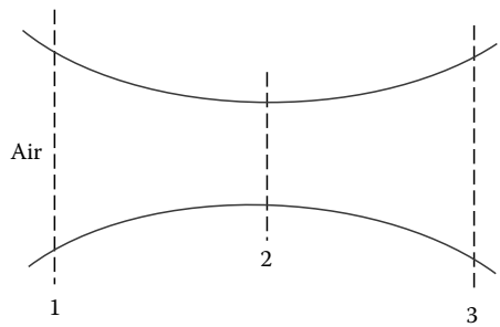
FIGURE 8.12 Converging–diverging nozzle of Example 8.4.
