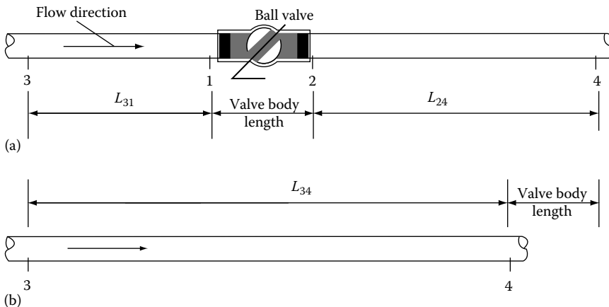
FIGURE 4.5 Sketch of pipe and valve systems.
