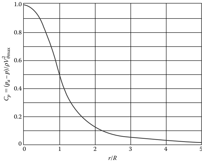
FIGURE 12.14 Pressure profile in the tornado of Example 12.3.
