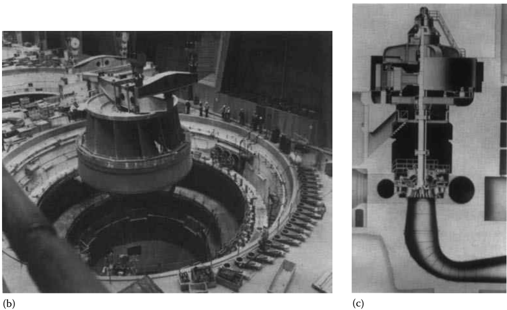
FIGURE 9.25 (continued) (b) Francis turbine runner during installation. (Courtesy of Allis-Chalmers Hydro Turbine Division. With permission.) (c) A Francis turbine installation. (Courtesy of Allis-Chalmers Hydro Turbine Division.)
