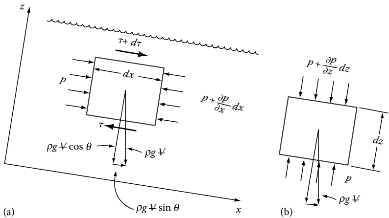
FIGURE 7.10 Control volume with forces acting on it for uniform open-channel flow.
